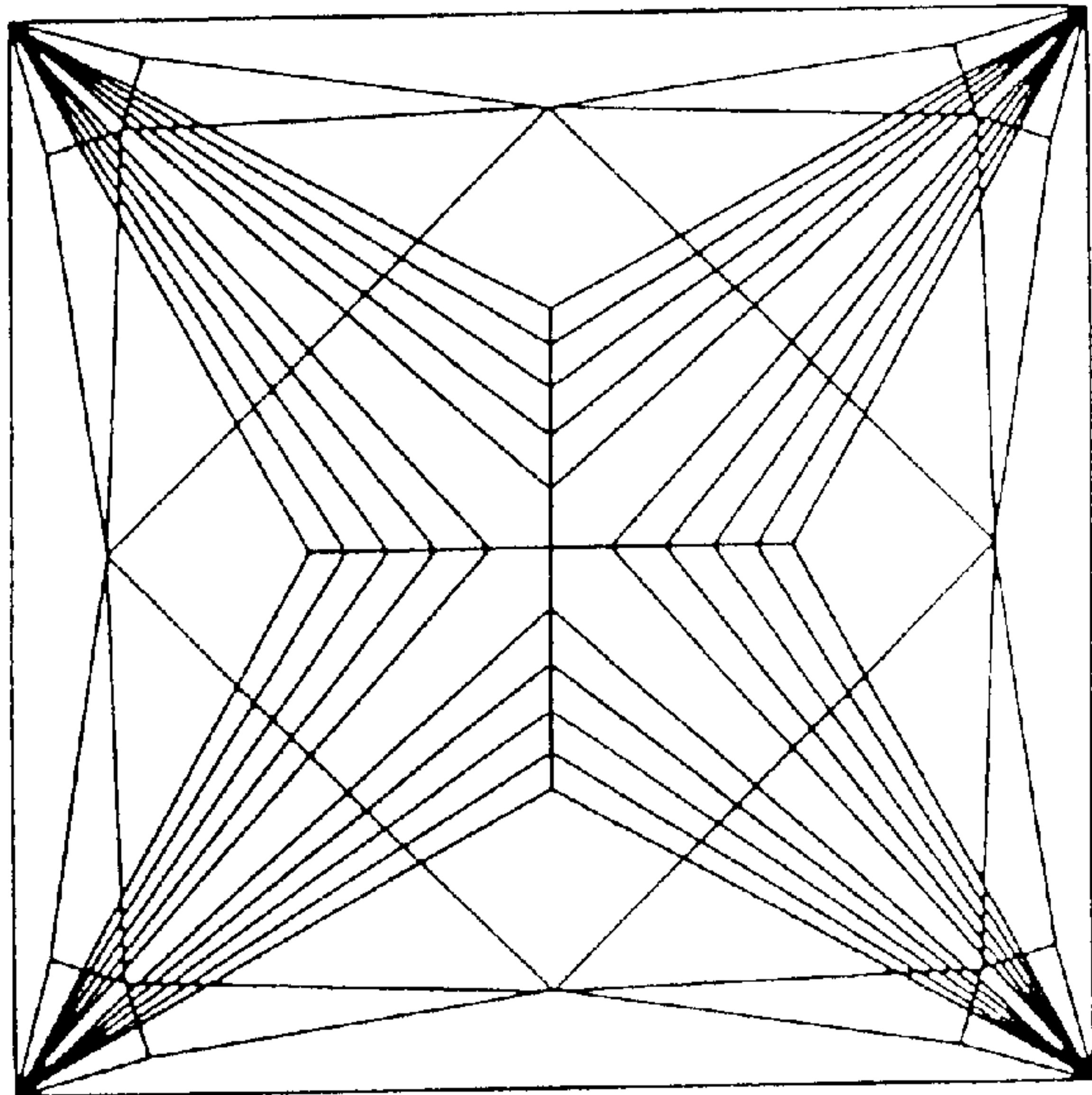
FIG.4 BOTTOM VIEW
