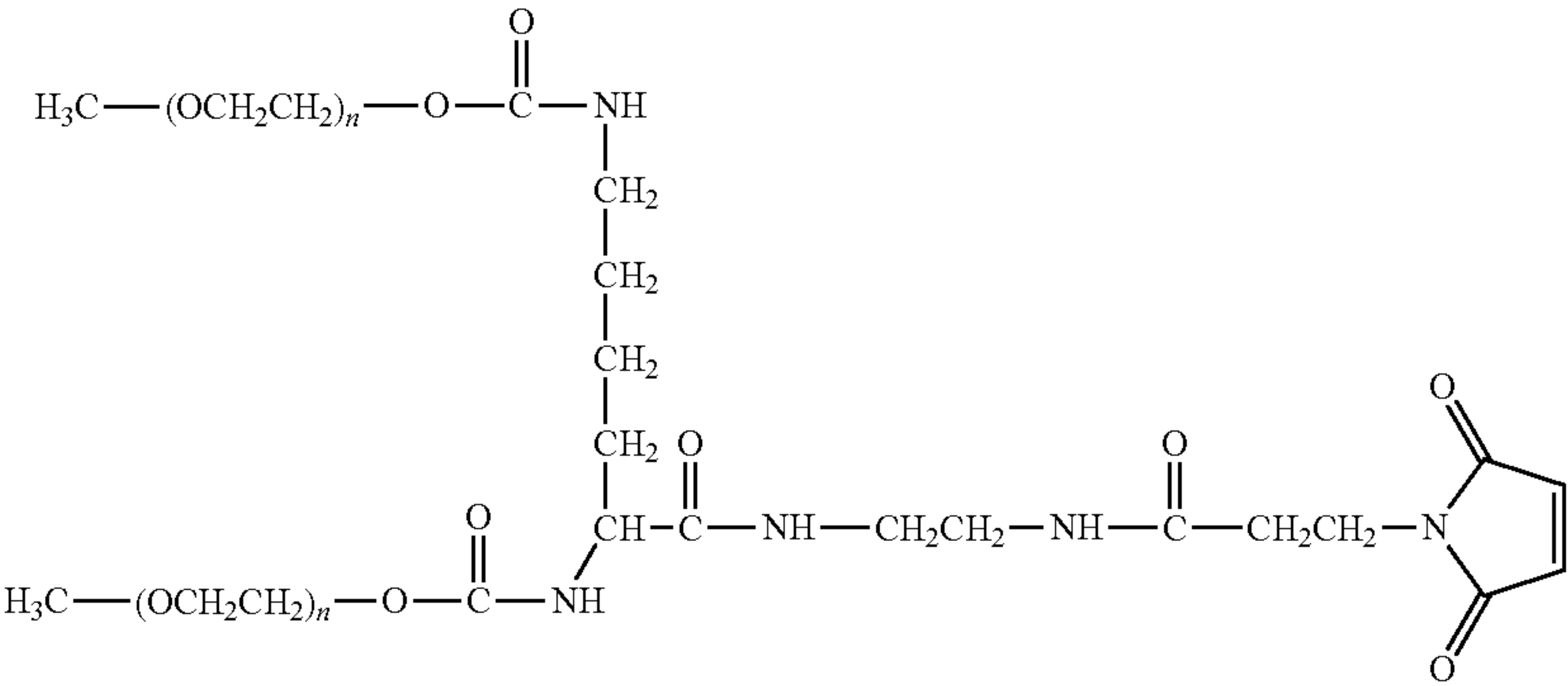
branched mPEG2 Maleimide Derivative (under certain reaction conditions such as pH > 8)
