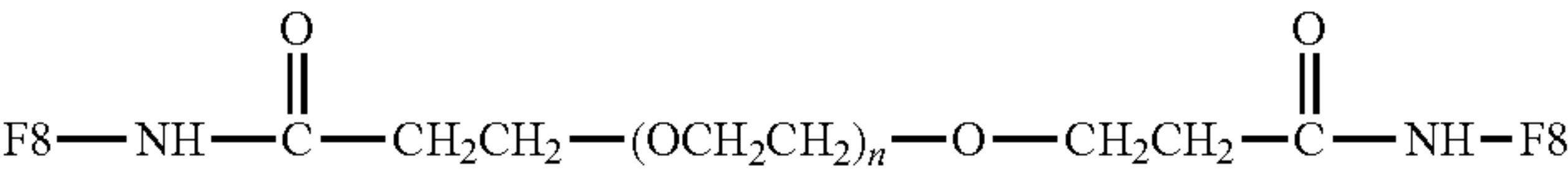
Amide Linkages
