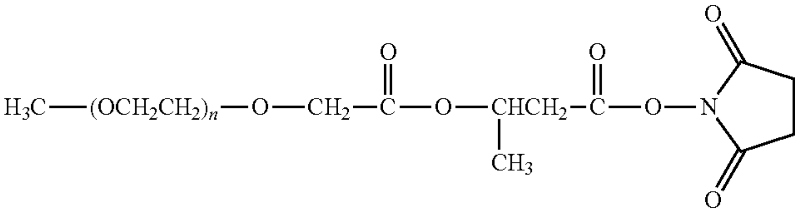
mPEG-Succinimidyl Derivative
