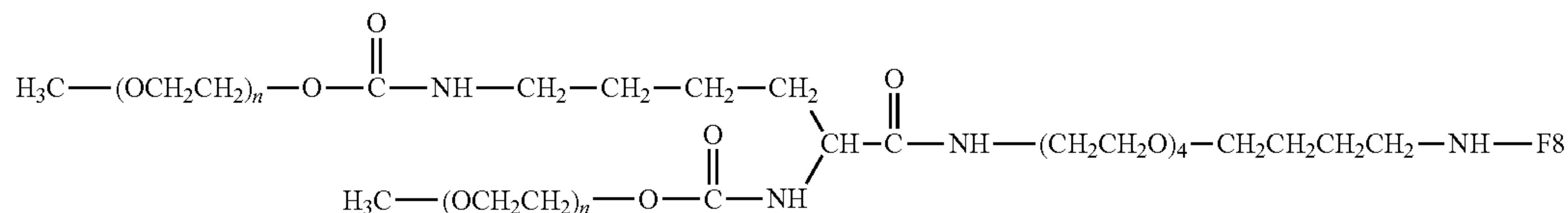
Secondary Amine Linkage
