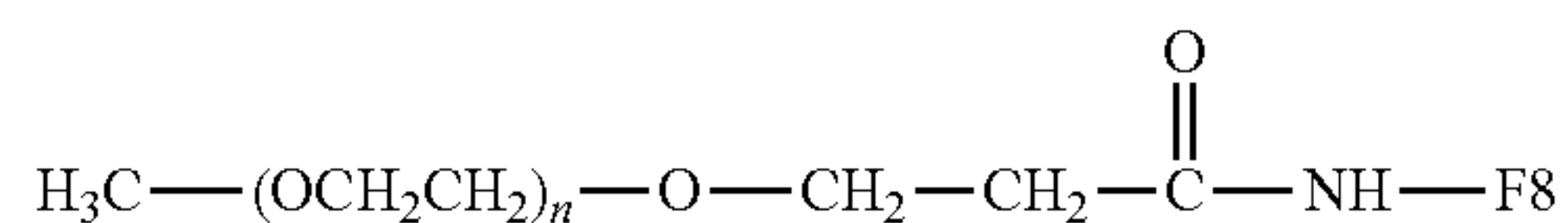
Amide Linkage
