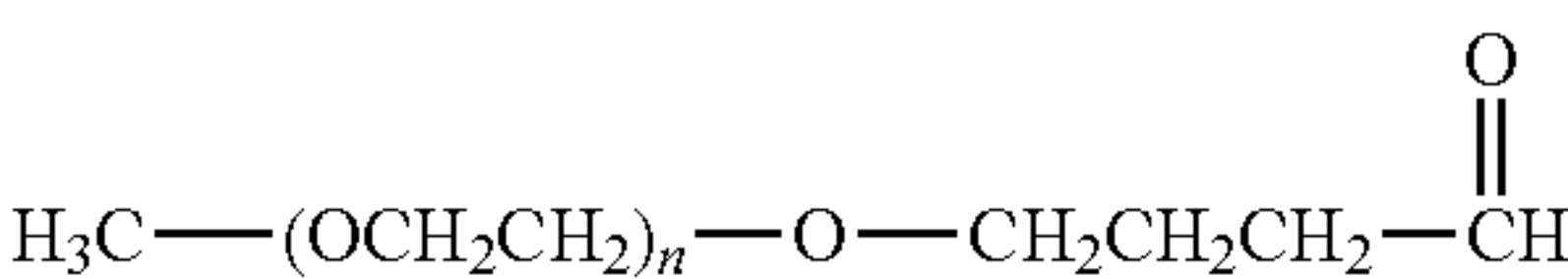
mPEG Butryaldehyde
