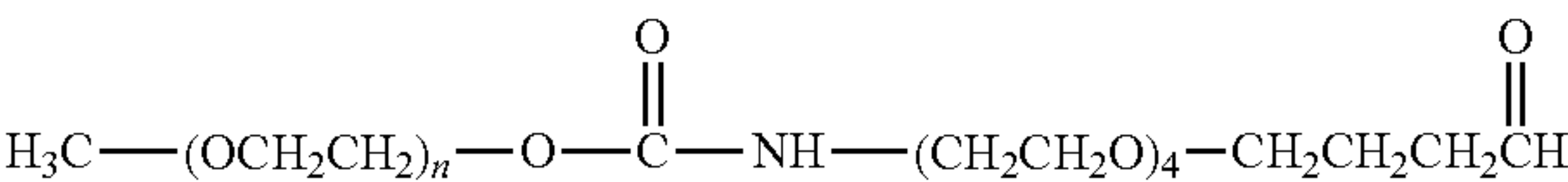
mPEG Butryaldehyde Derivative
