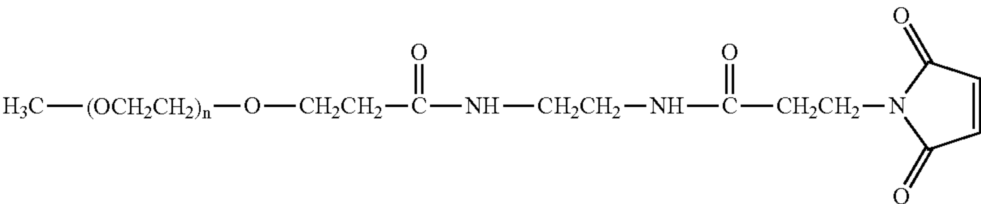
mPEG Maleimide Derivative (under certain reaction conditions such as pH > 8)
