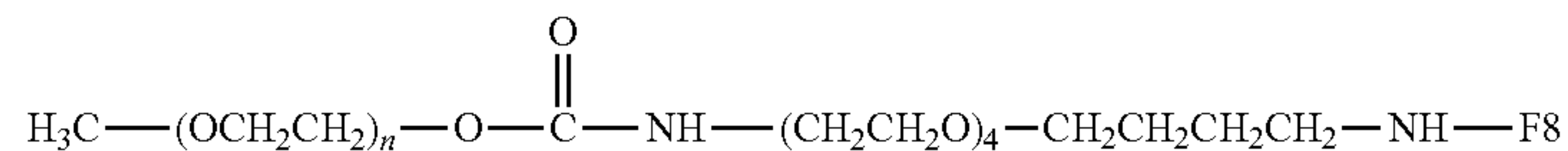
Secondary Amine Linkage
