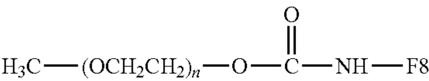
Carbamate Linkage
