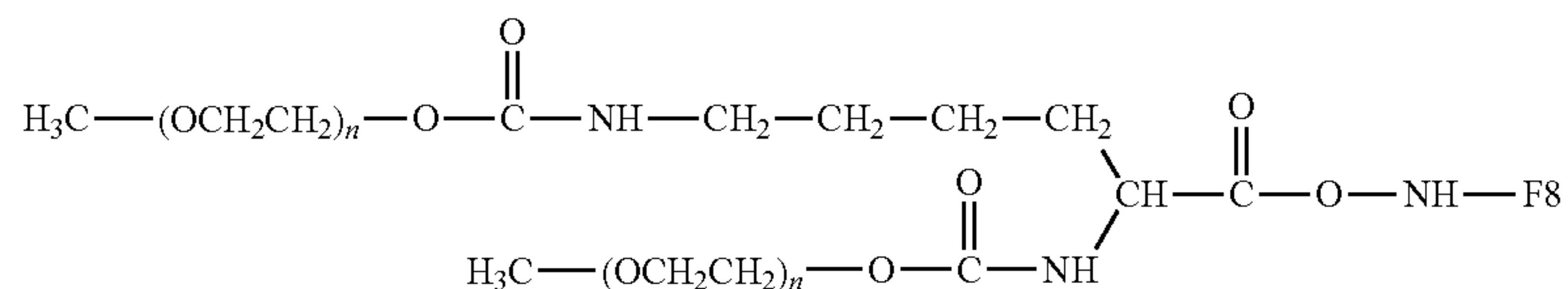
Amide Linkage
