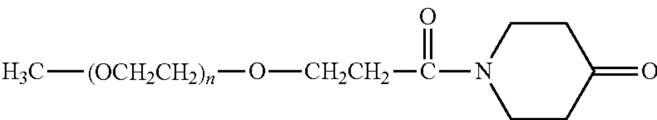
mPEG Piperidone
