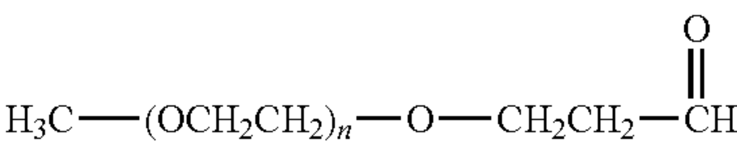
mPEG Propionaldehyde
