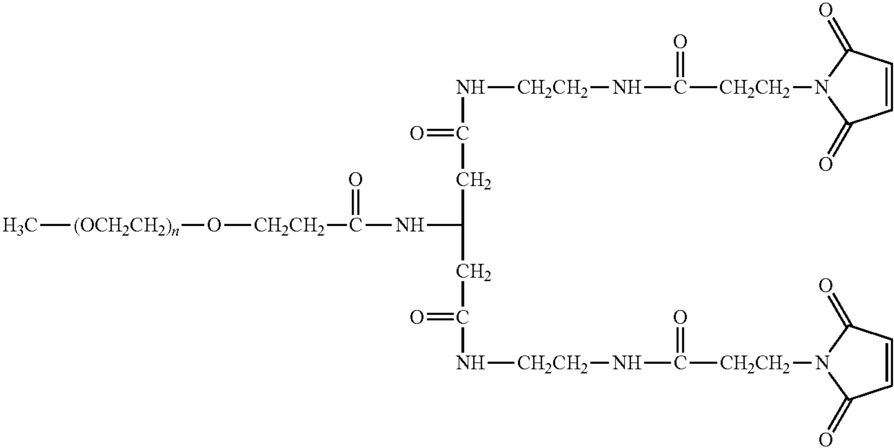
mPEG Forked Maleimide Derivative (under certain reaction conditions such as pH > 8)
