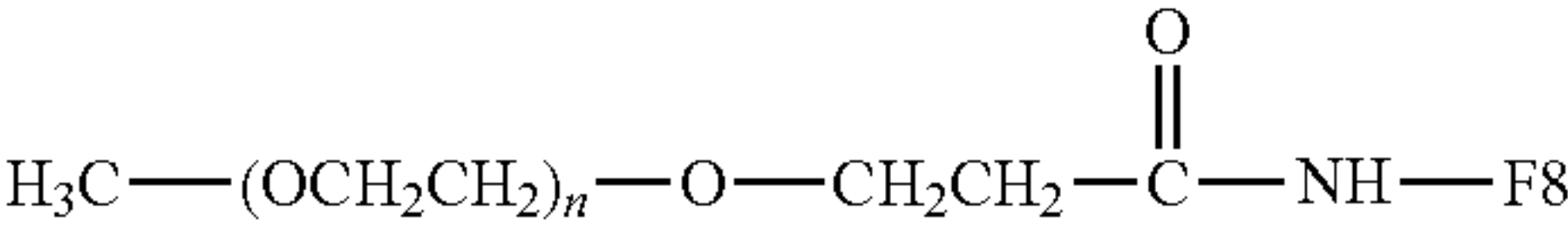
Amide Linkage
