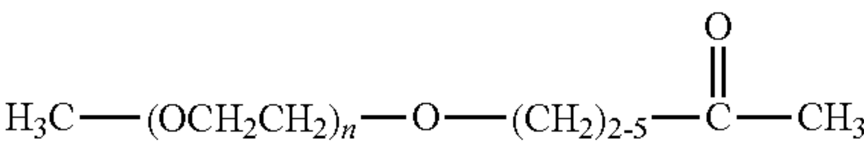
mPEG Methylketone
