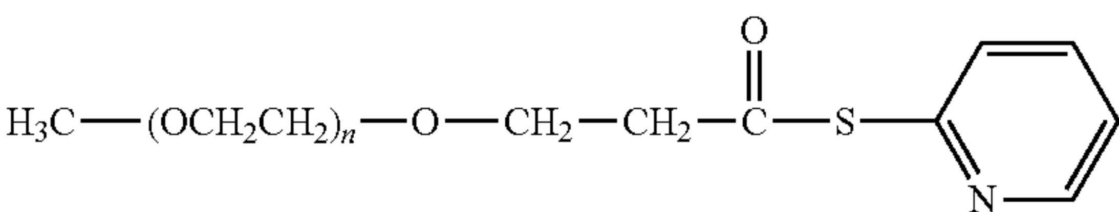
mPEG-Succinimidyl Derivative
