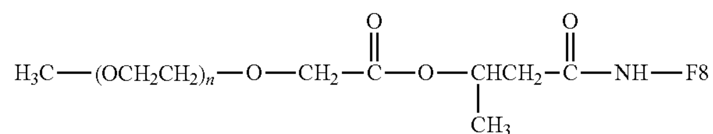
Amide Linkage
