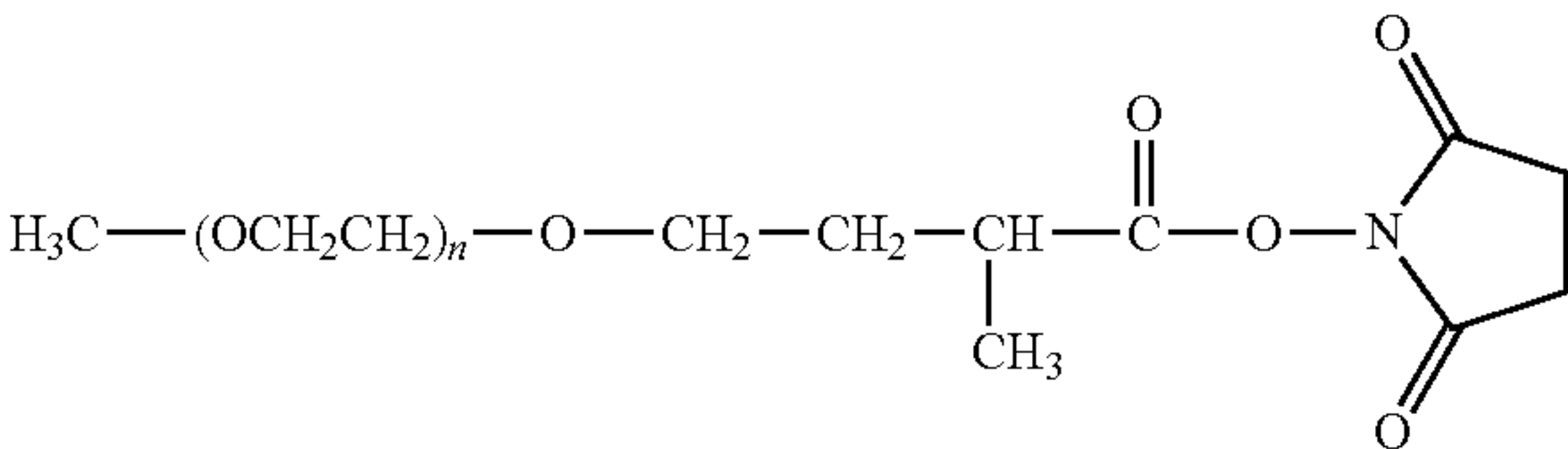
mPEG-Succinimidyl Derivative
