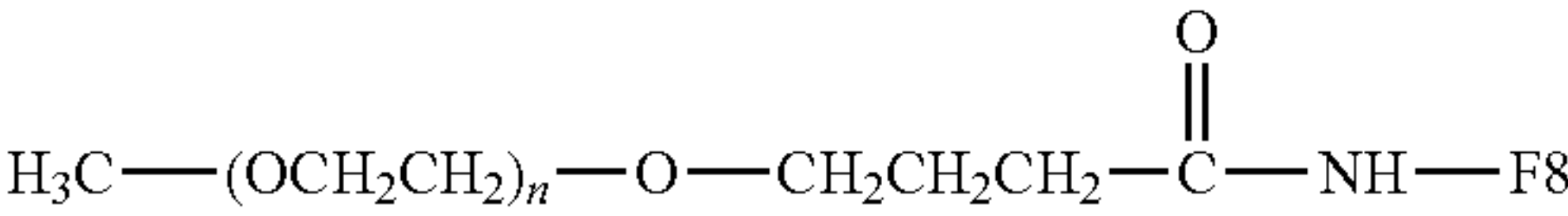
Amide Linkage
