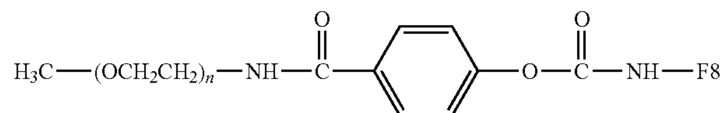
Carbamate Linkage
