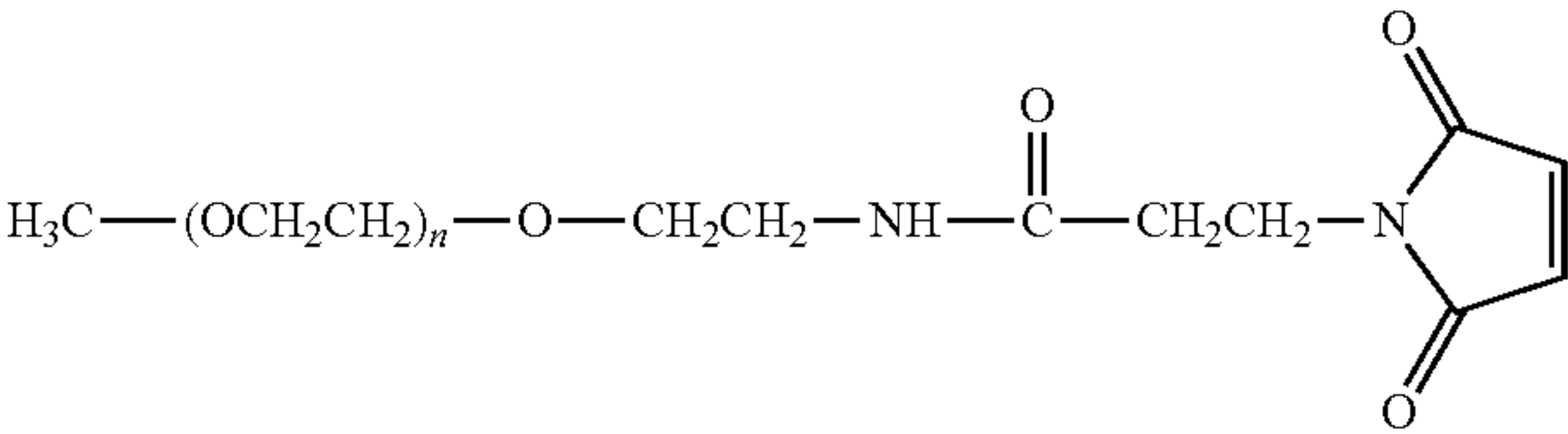
mPEG Maleimide Derivative
