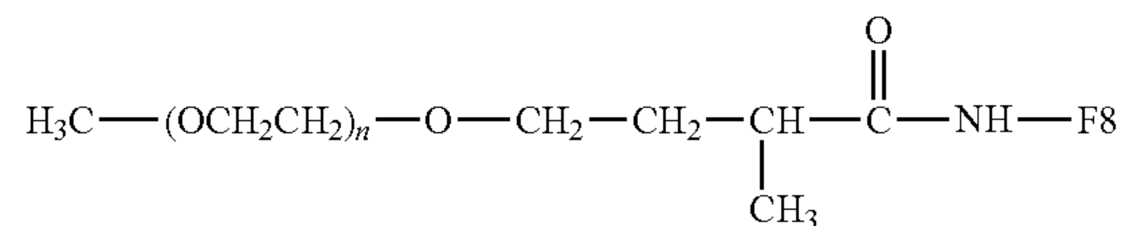
Amide Linkage
