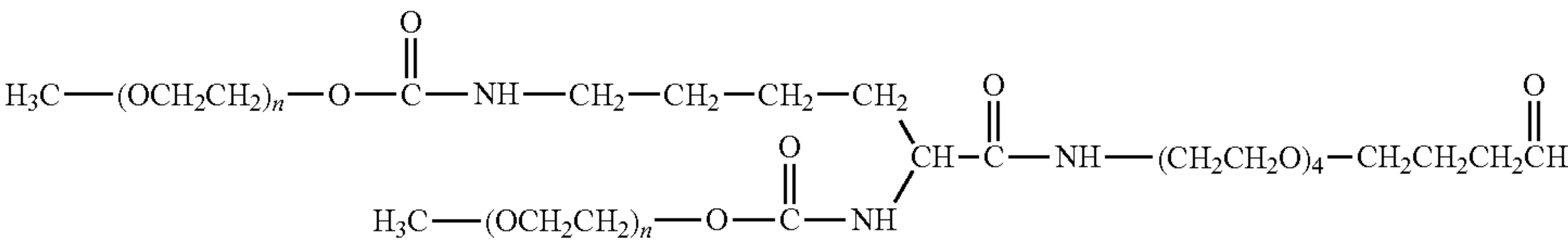
Branched mPEG2 Butyraldehyde
