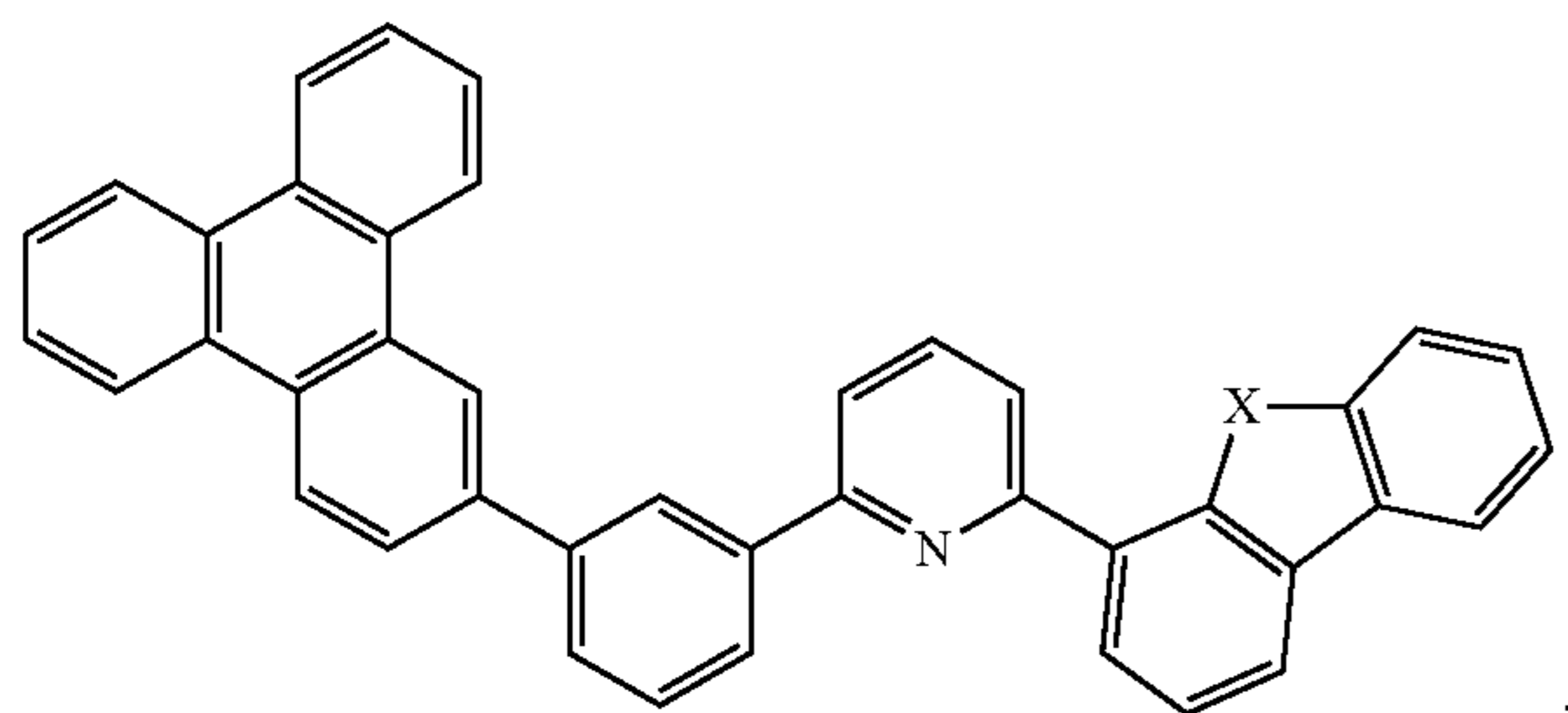
Compound 22
