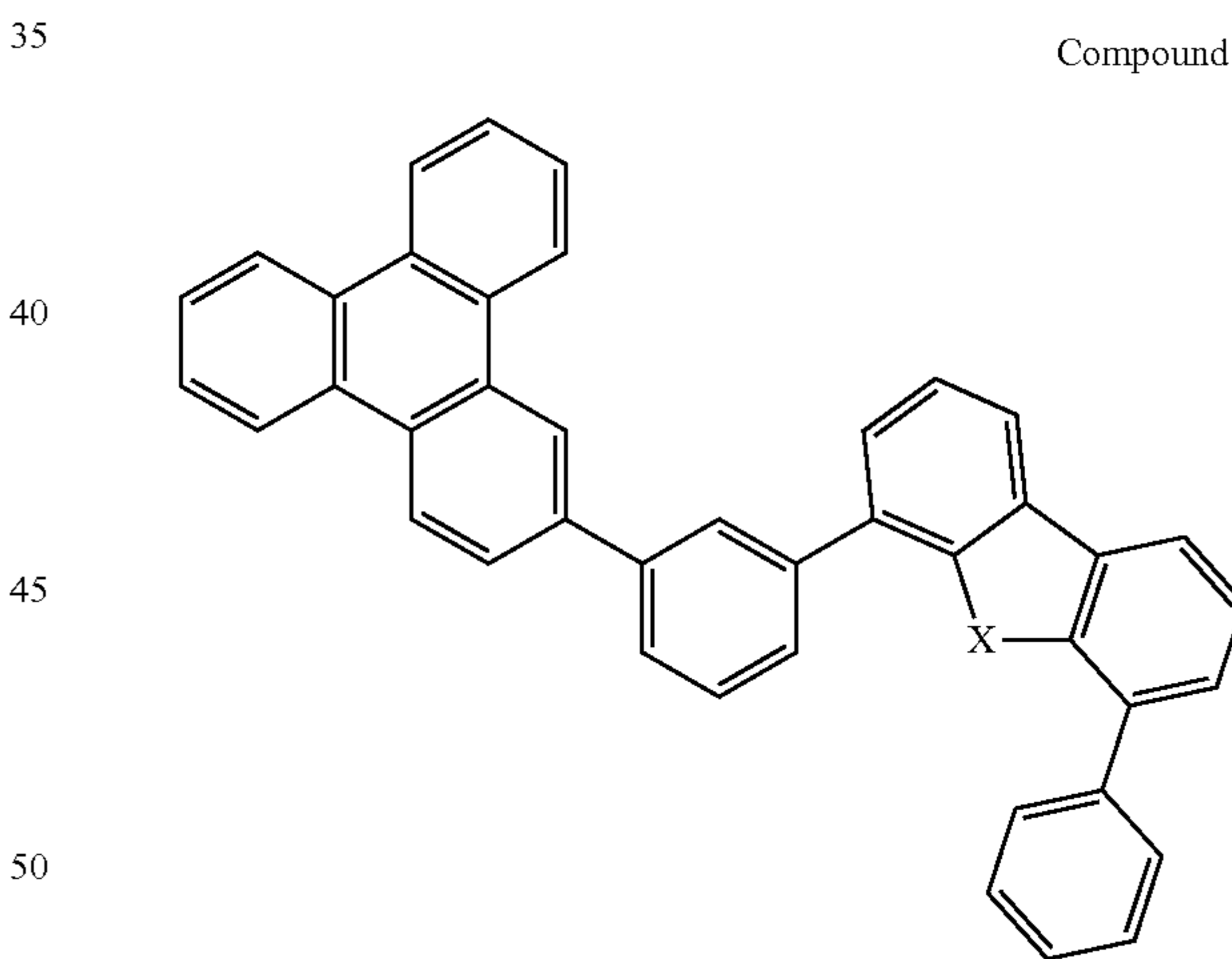
Compound 8
