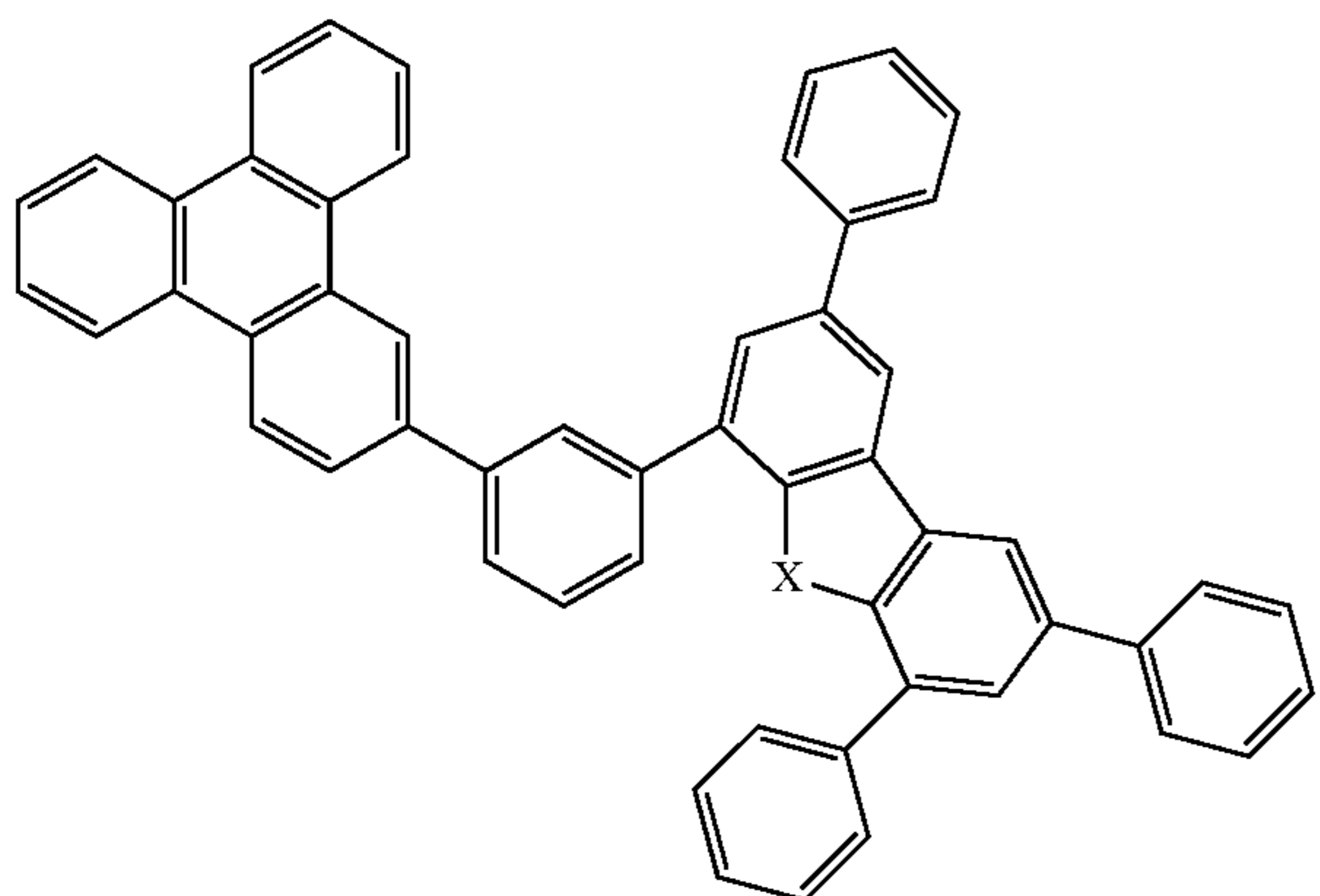
Compound 25
