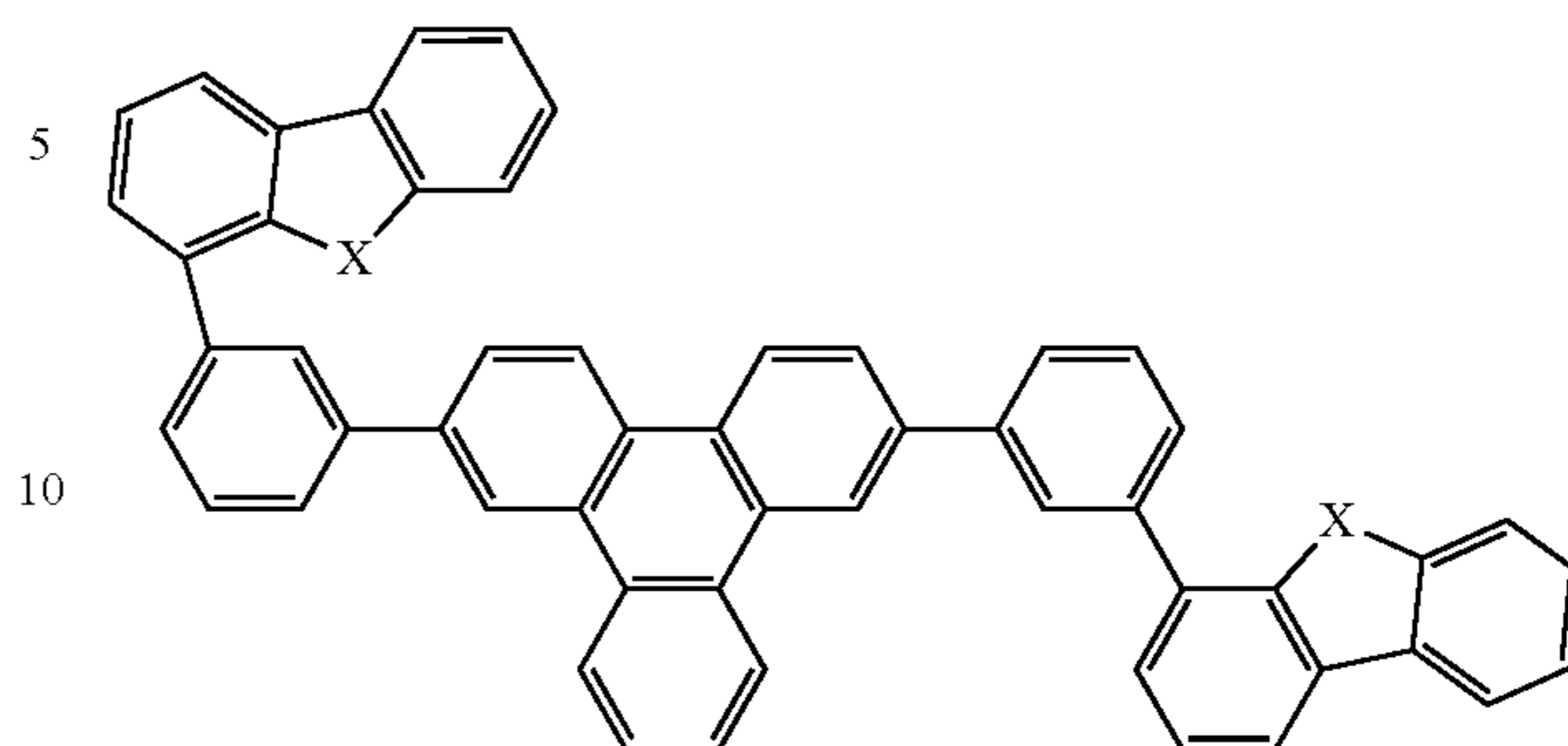
Compound 26
