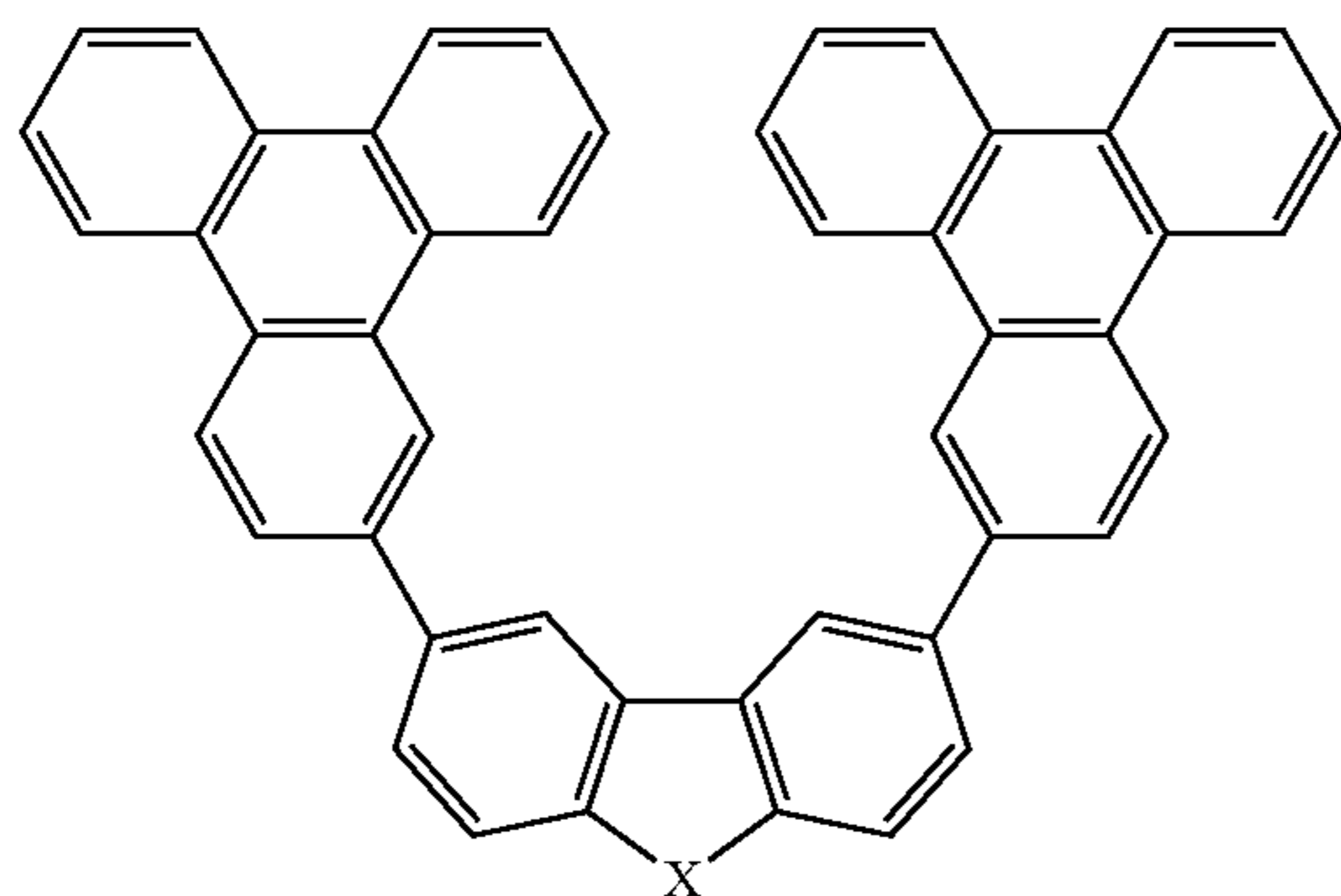
Compound 5
