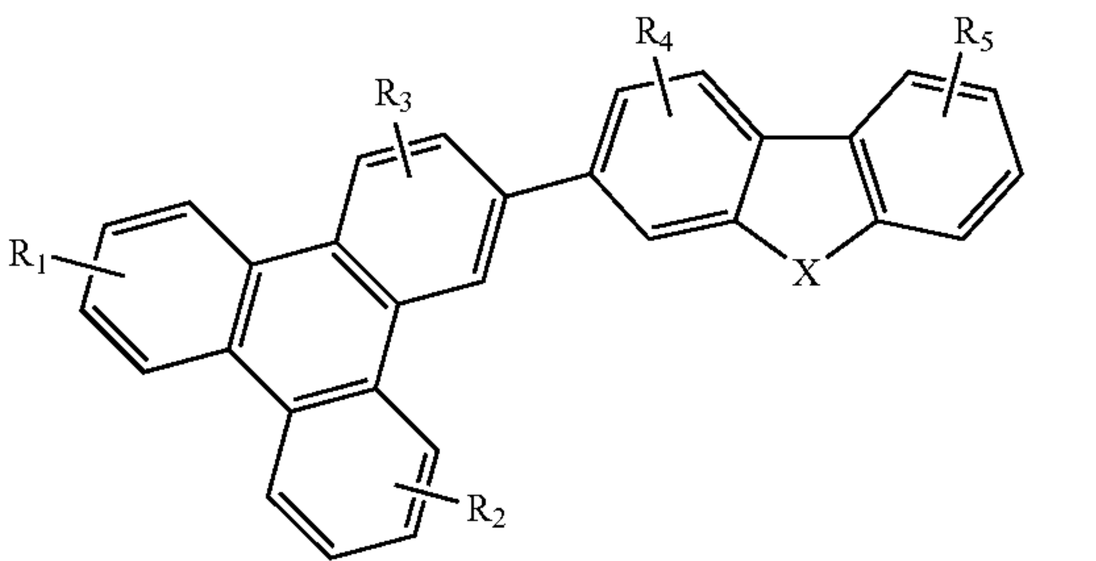
Compound 8G
