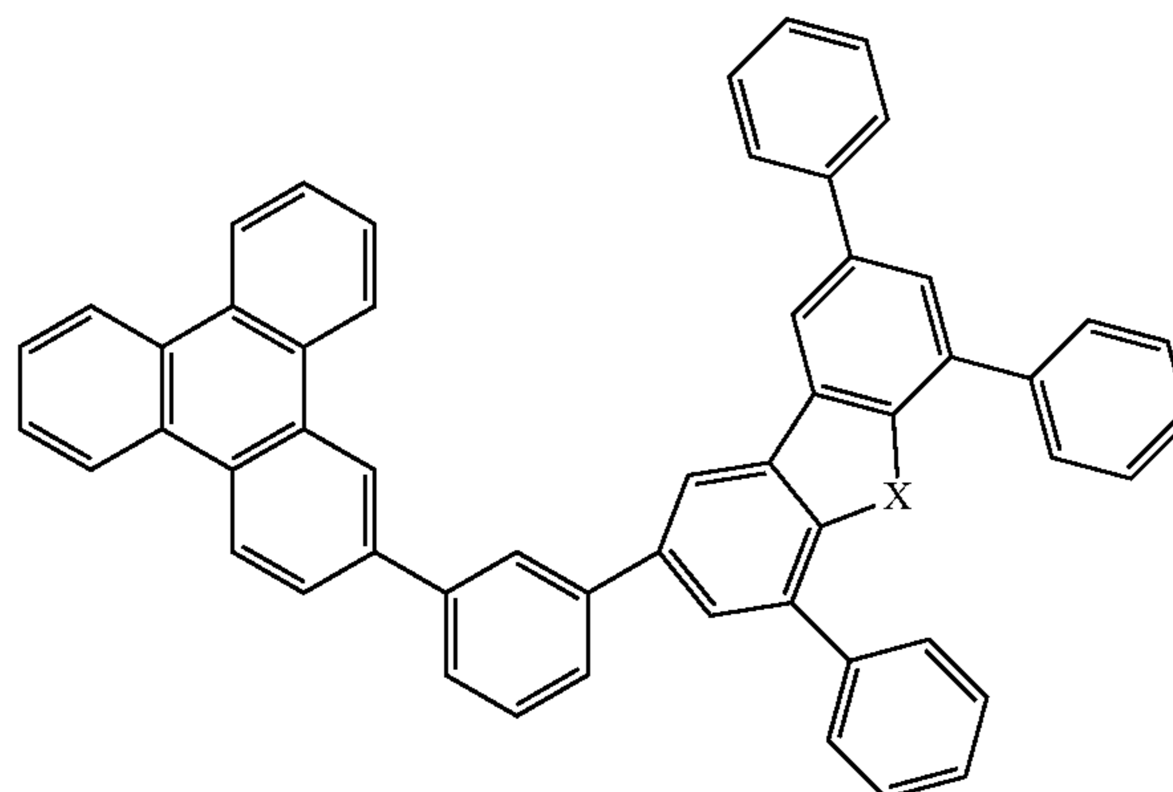
Compound 36
