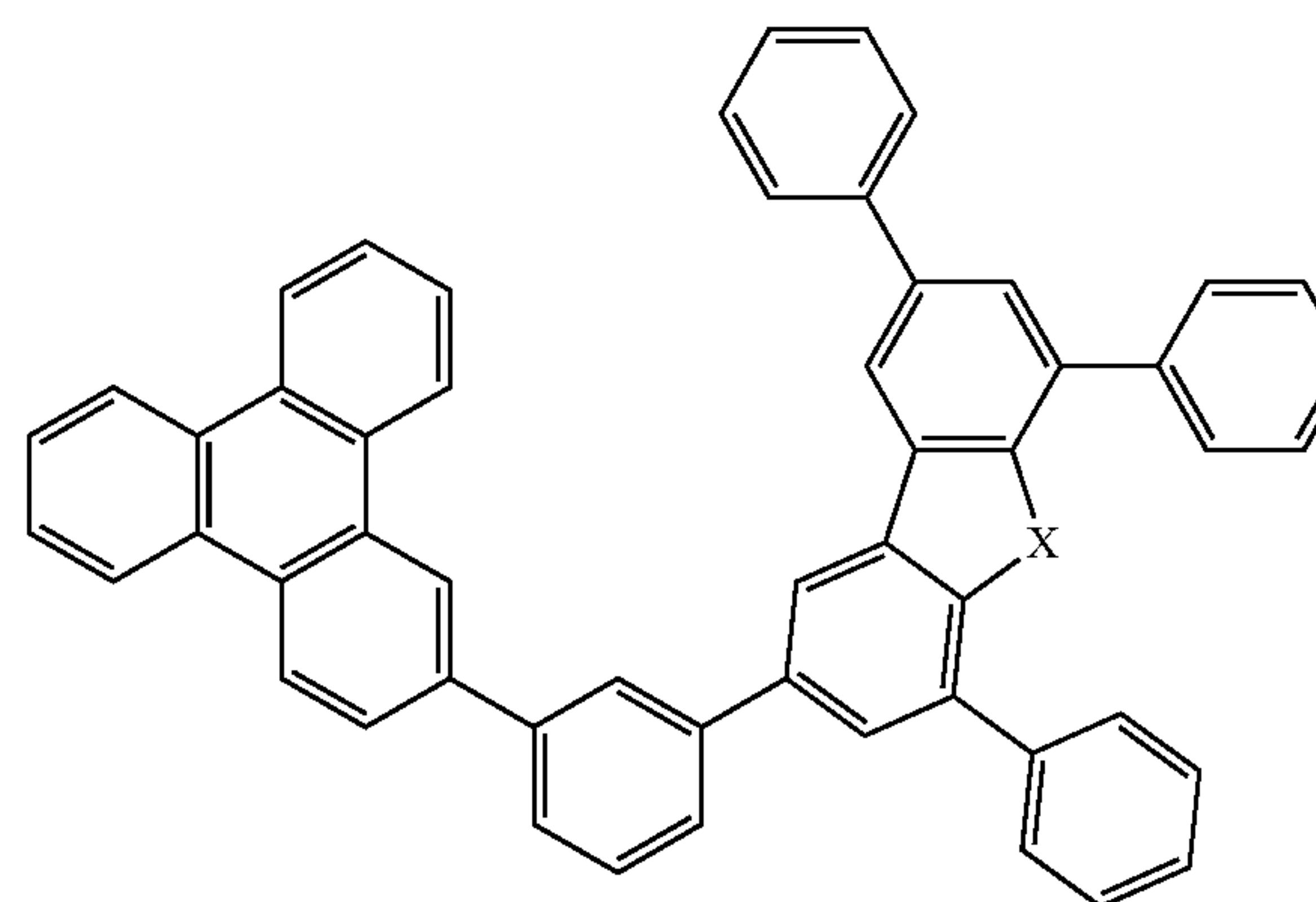
Compound 38
