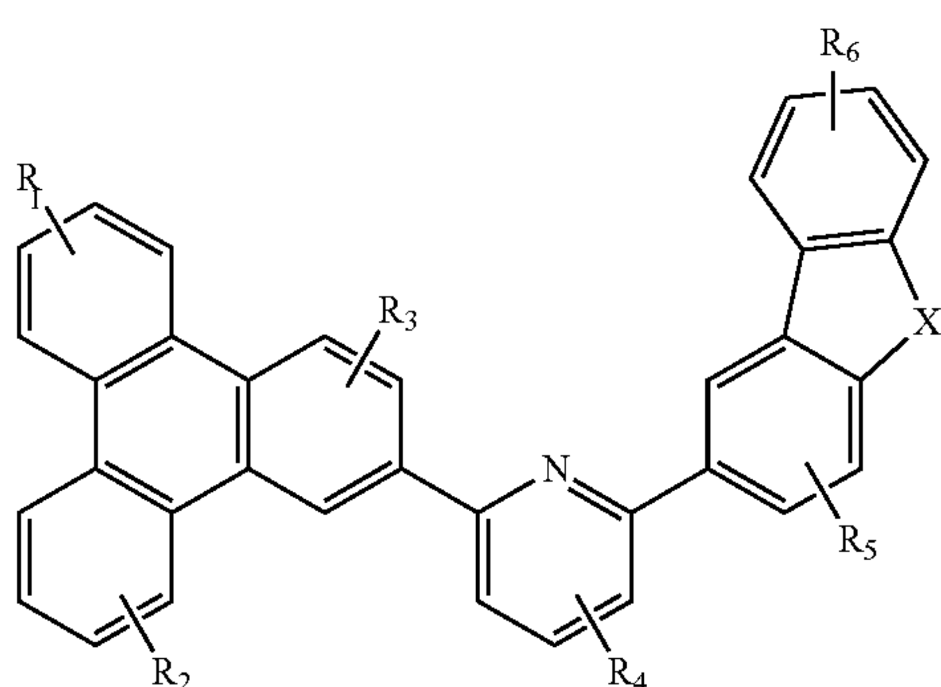
Compound 43
