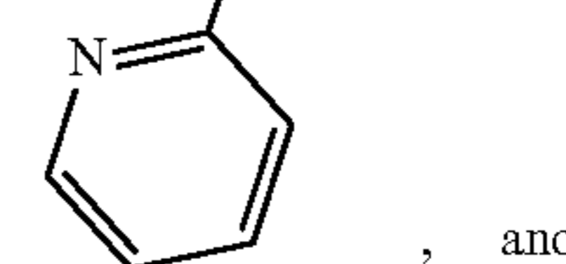
Compound 48
