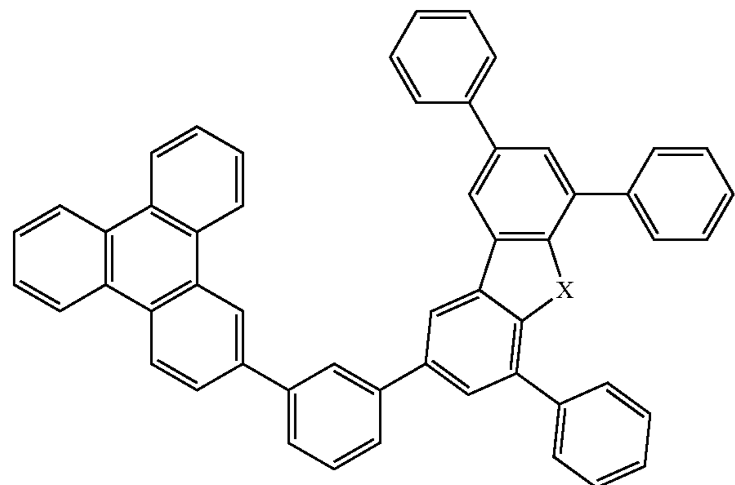
Compound 38
