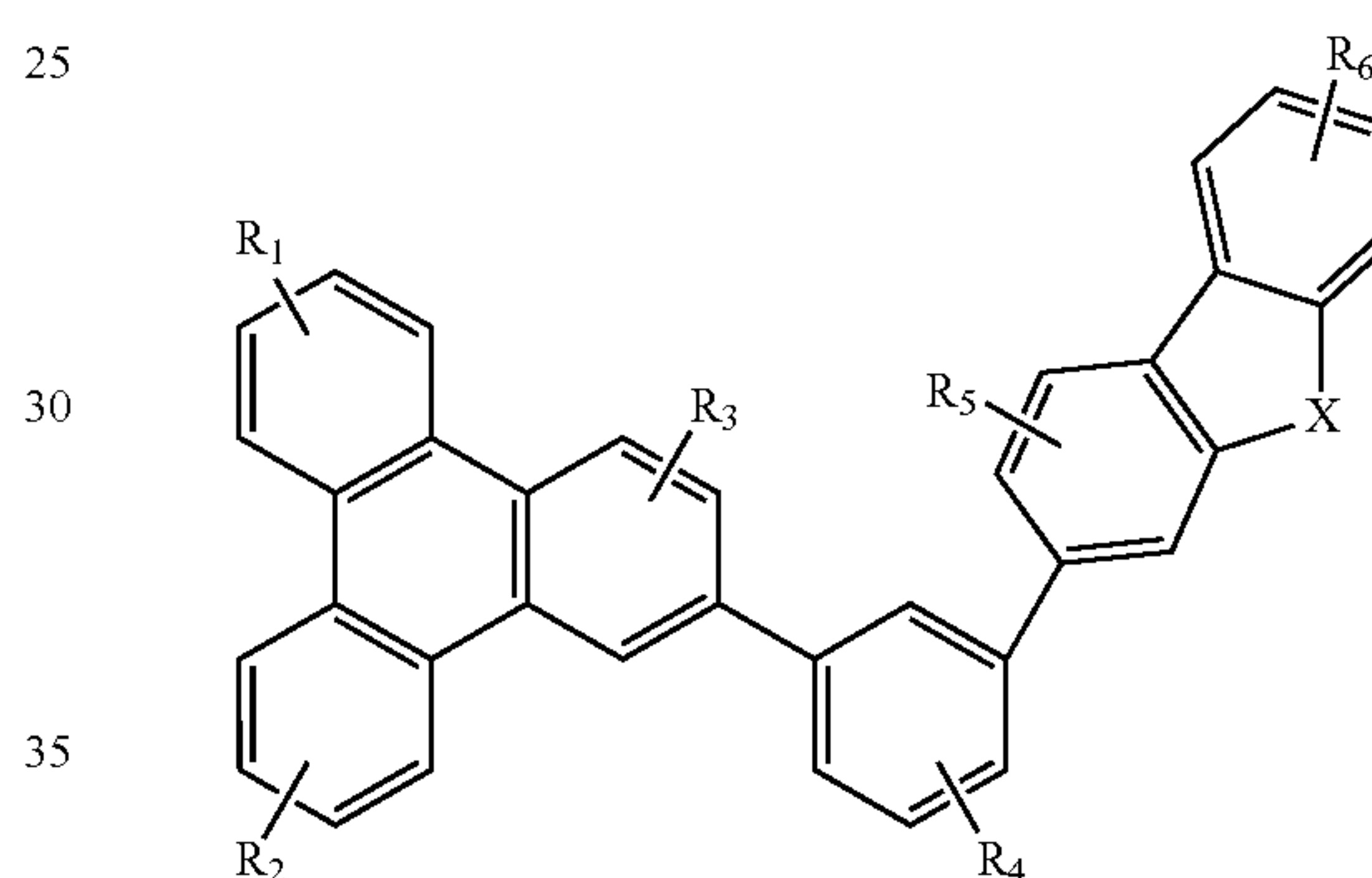
Compound 40G
