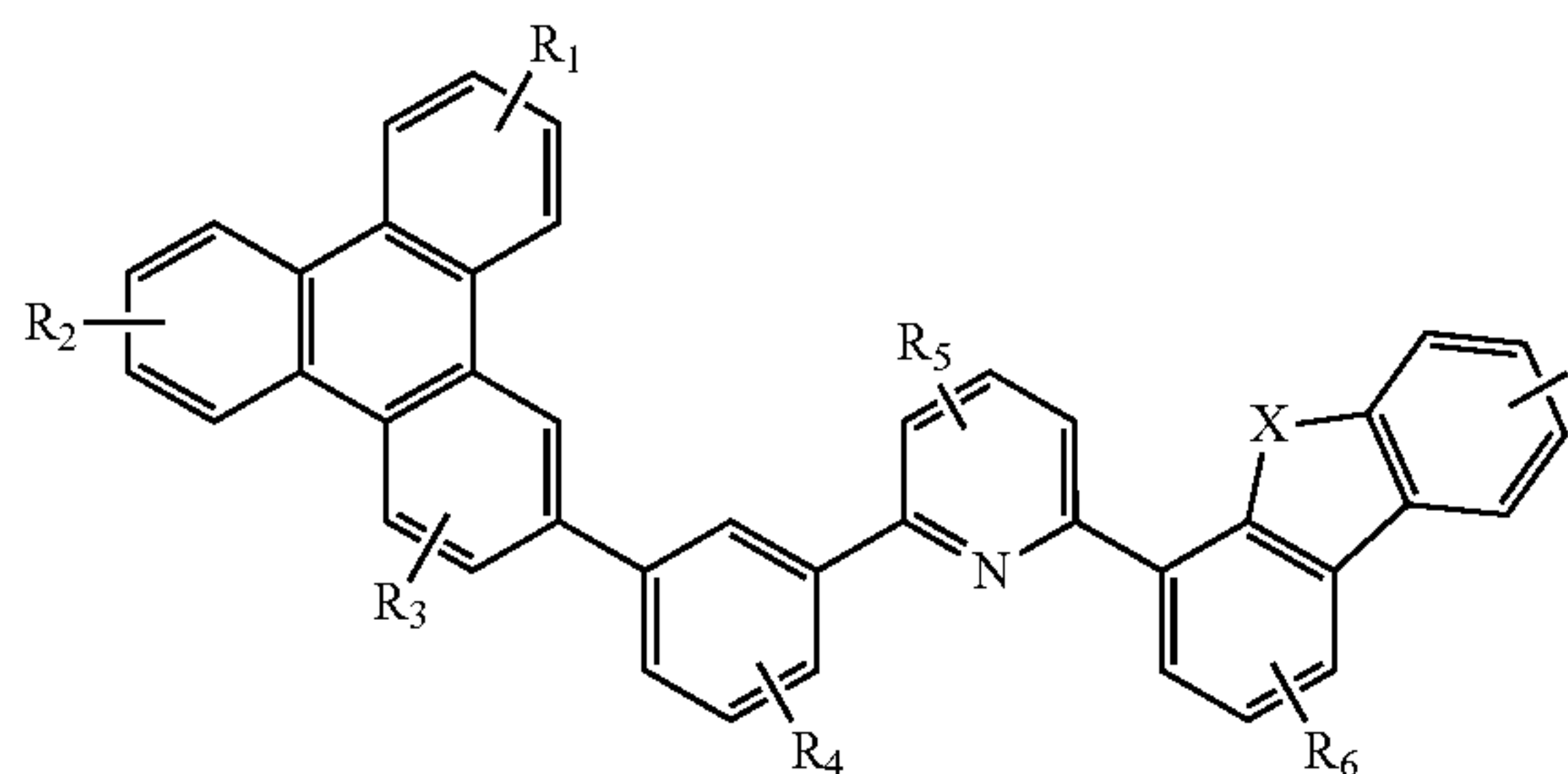
Compound 21
