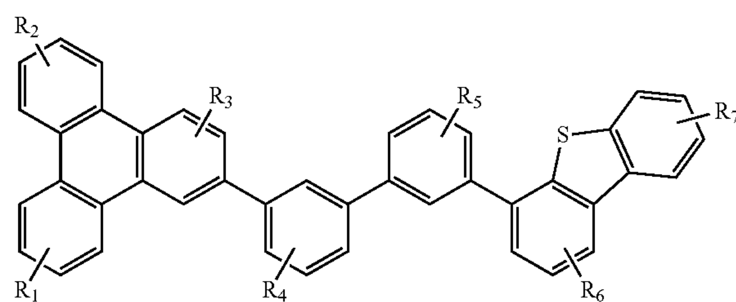
Compound 9'G
