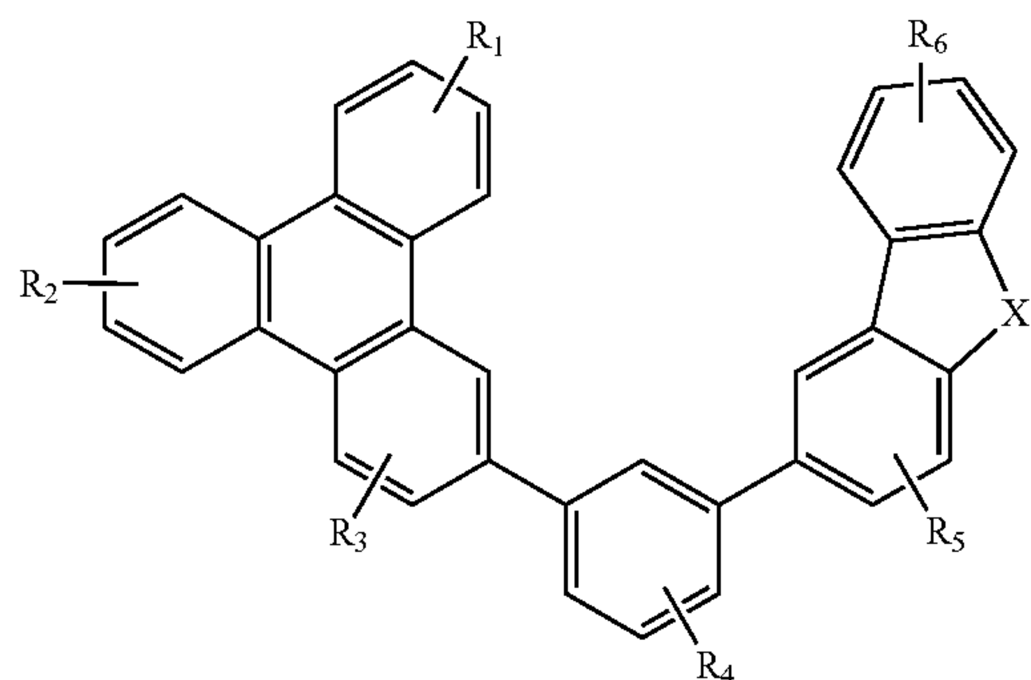
Compound 20
