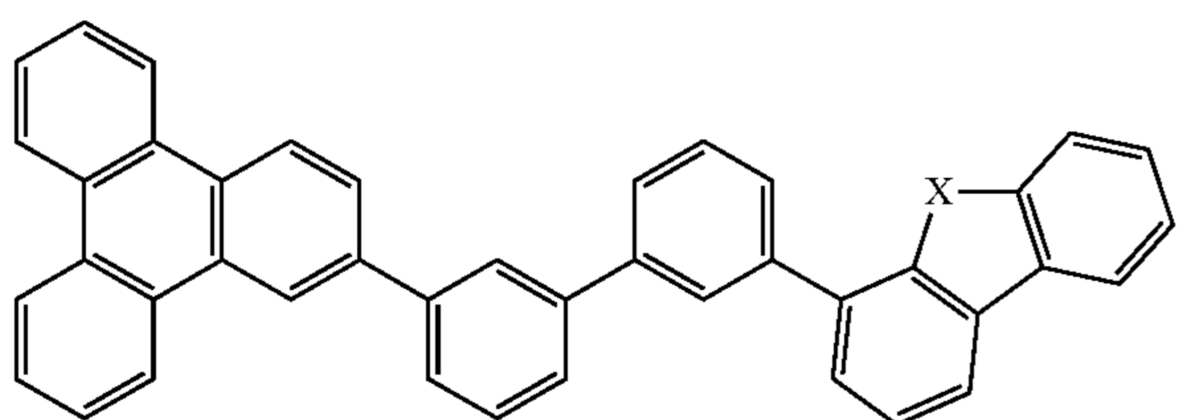
Compound 9
