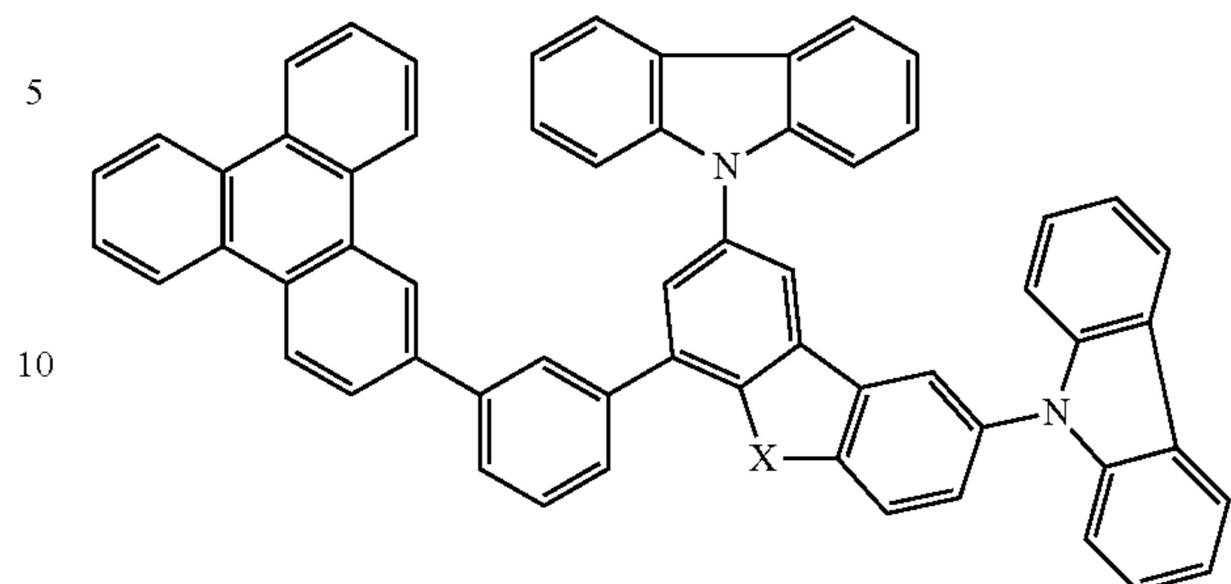
Compound 27
