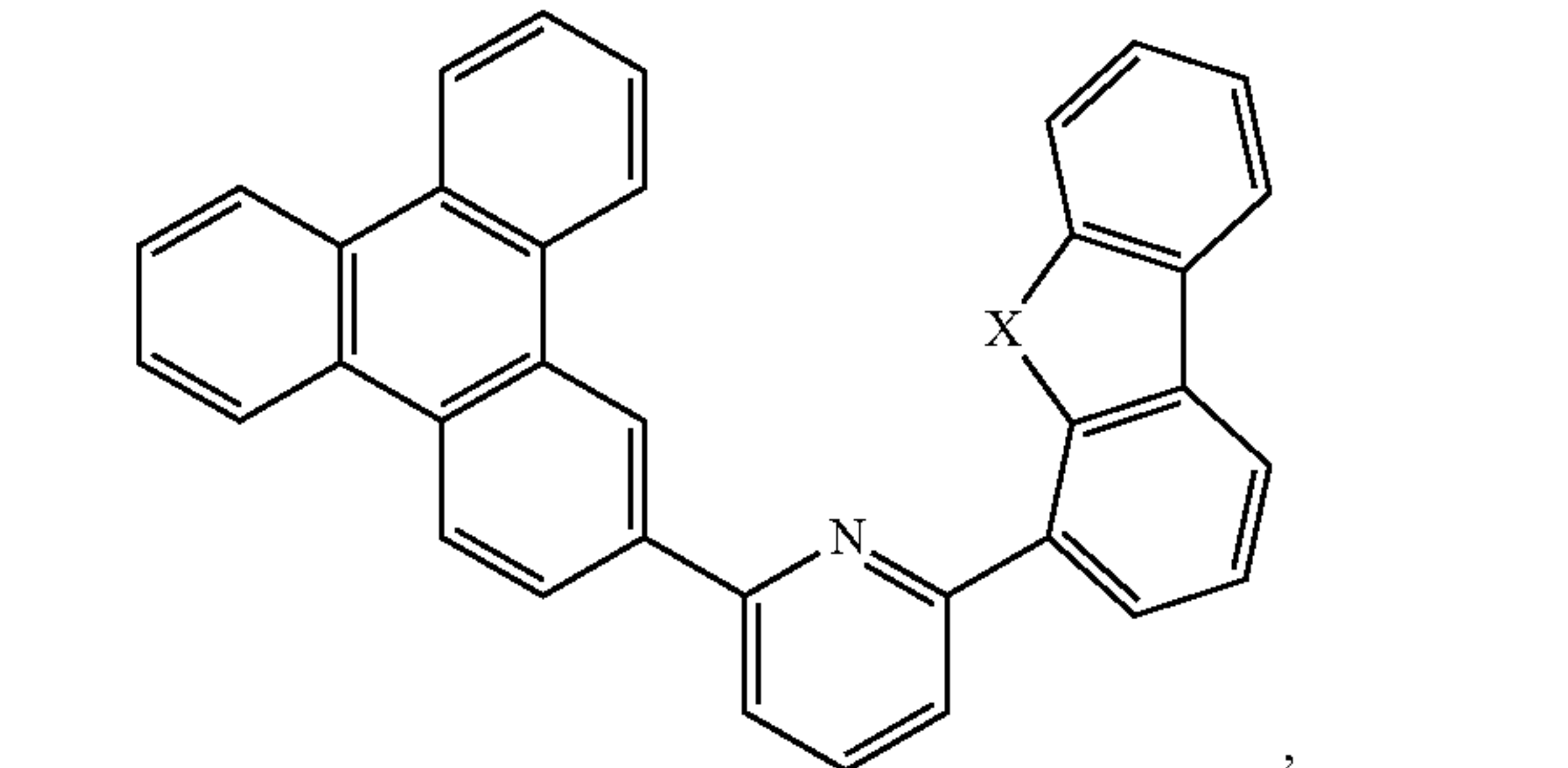
Compound 22
