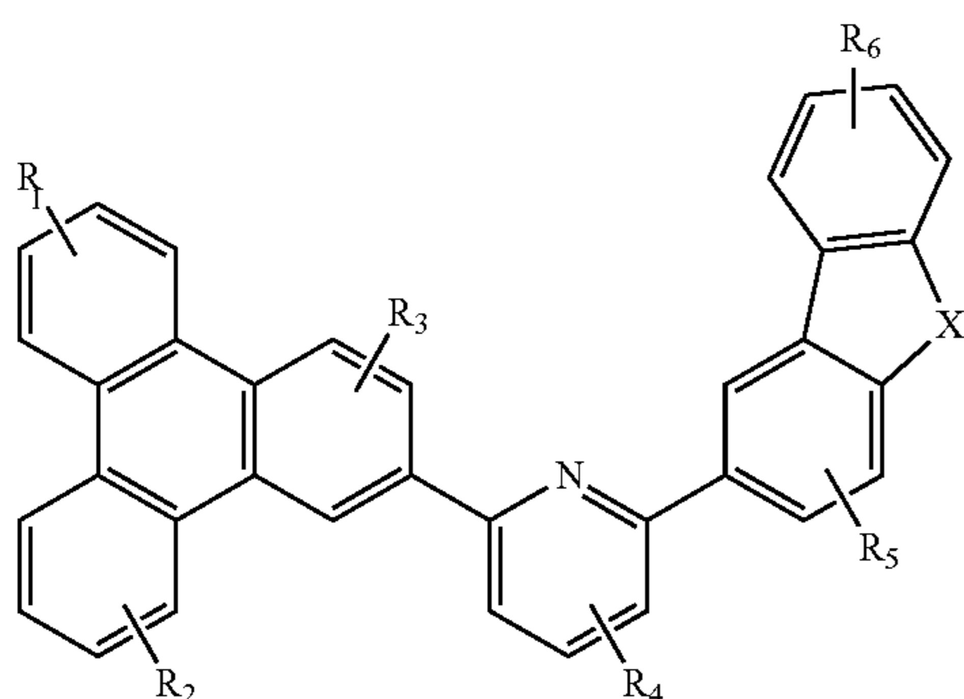
Compound 43G
