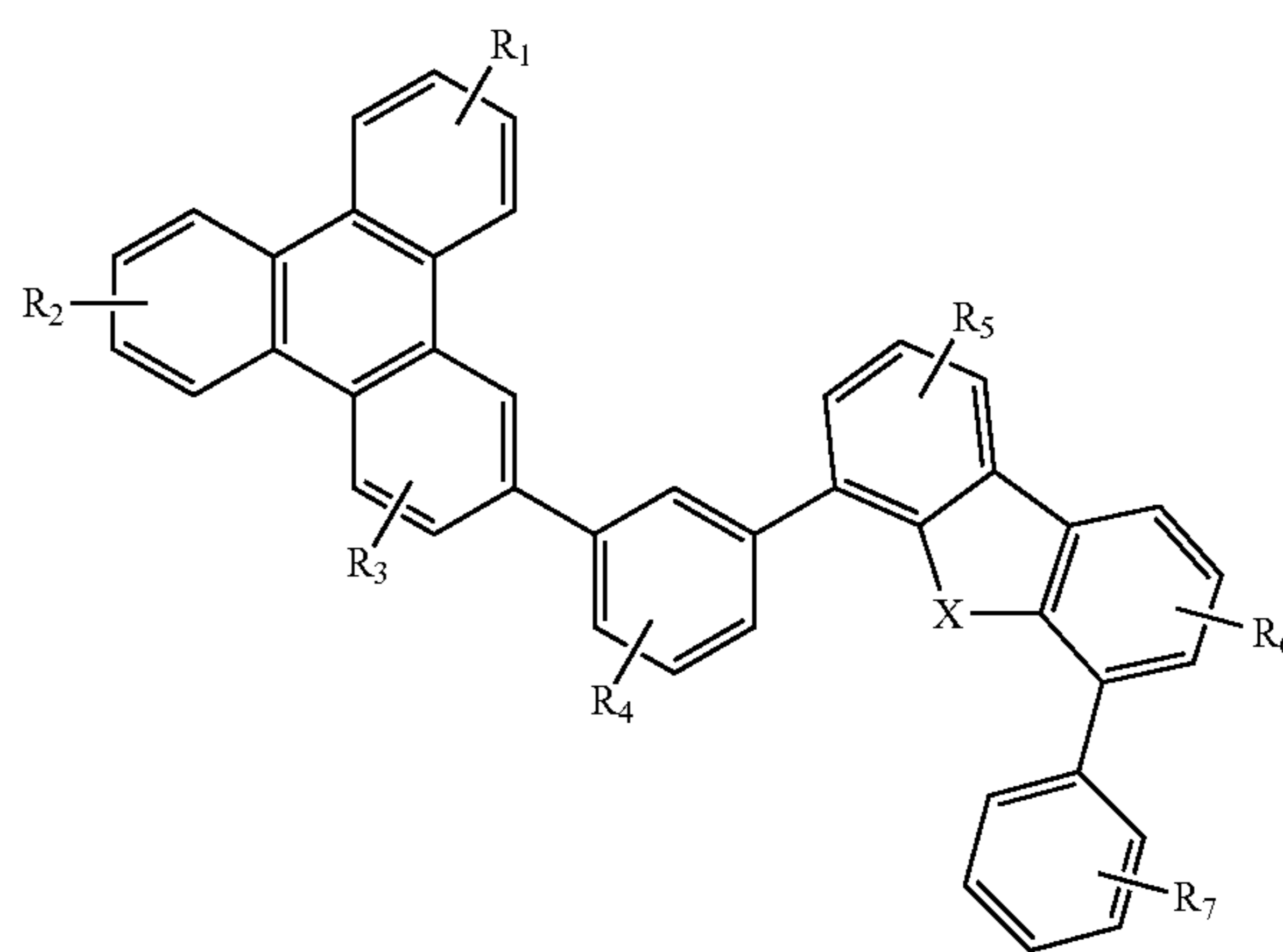
Compound 23G
