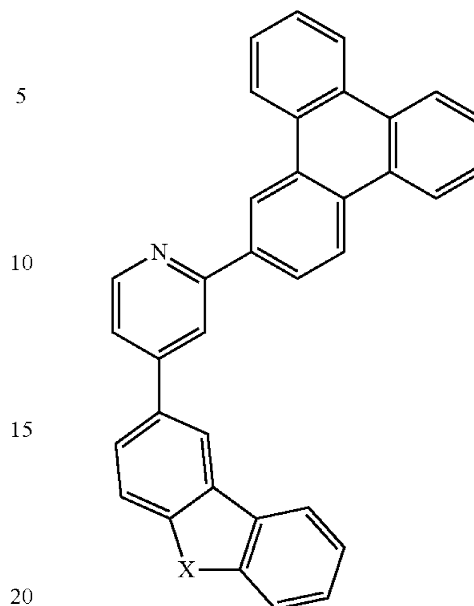
Compound 47
