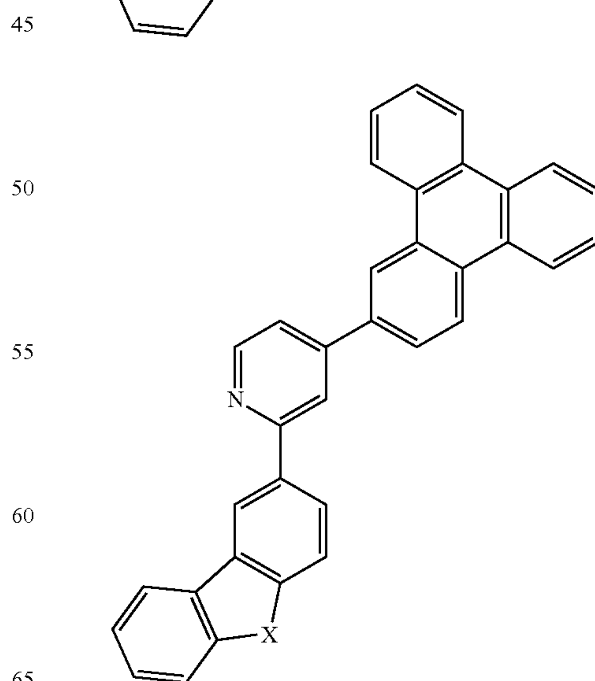
Compound 43
