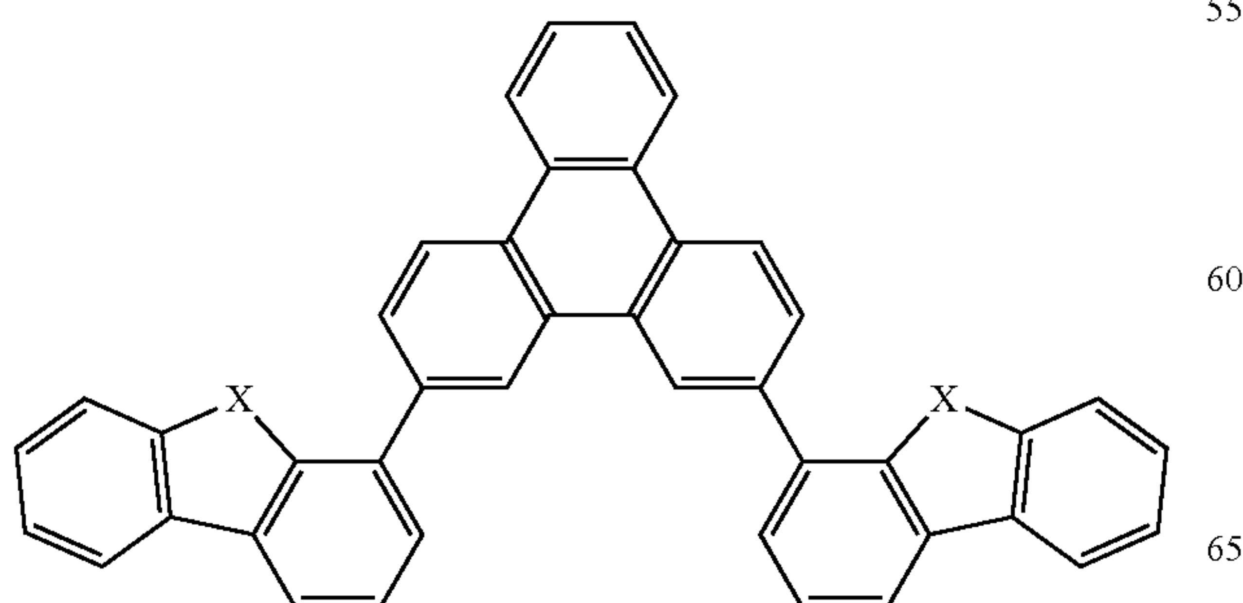
Compound 10
