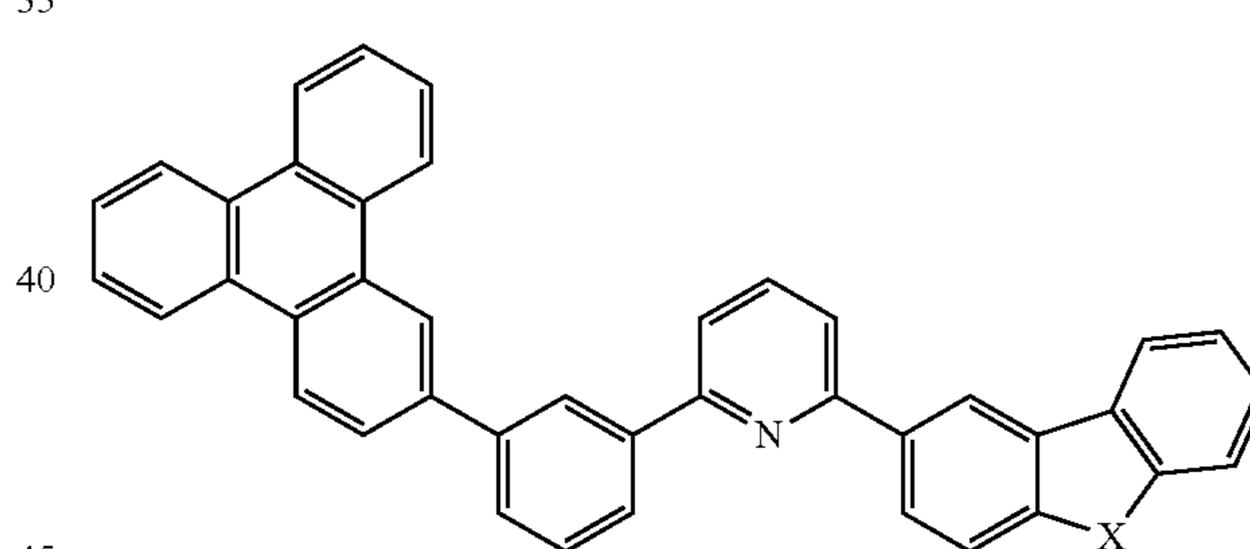
Compound 44
