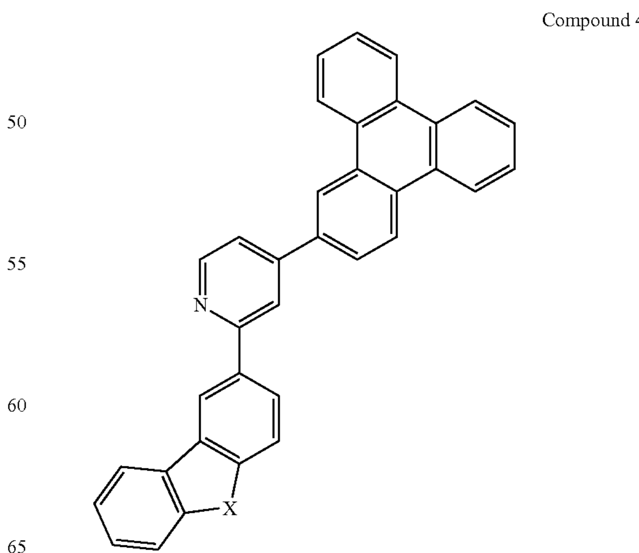
Compound 43
