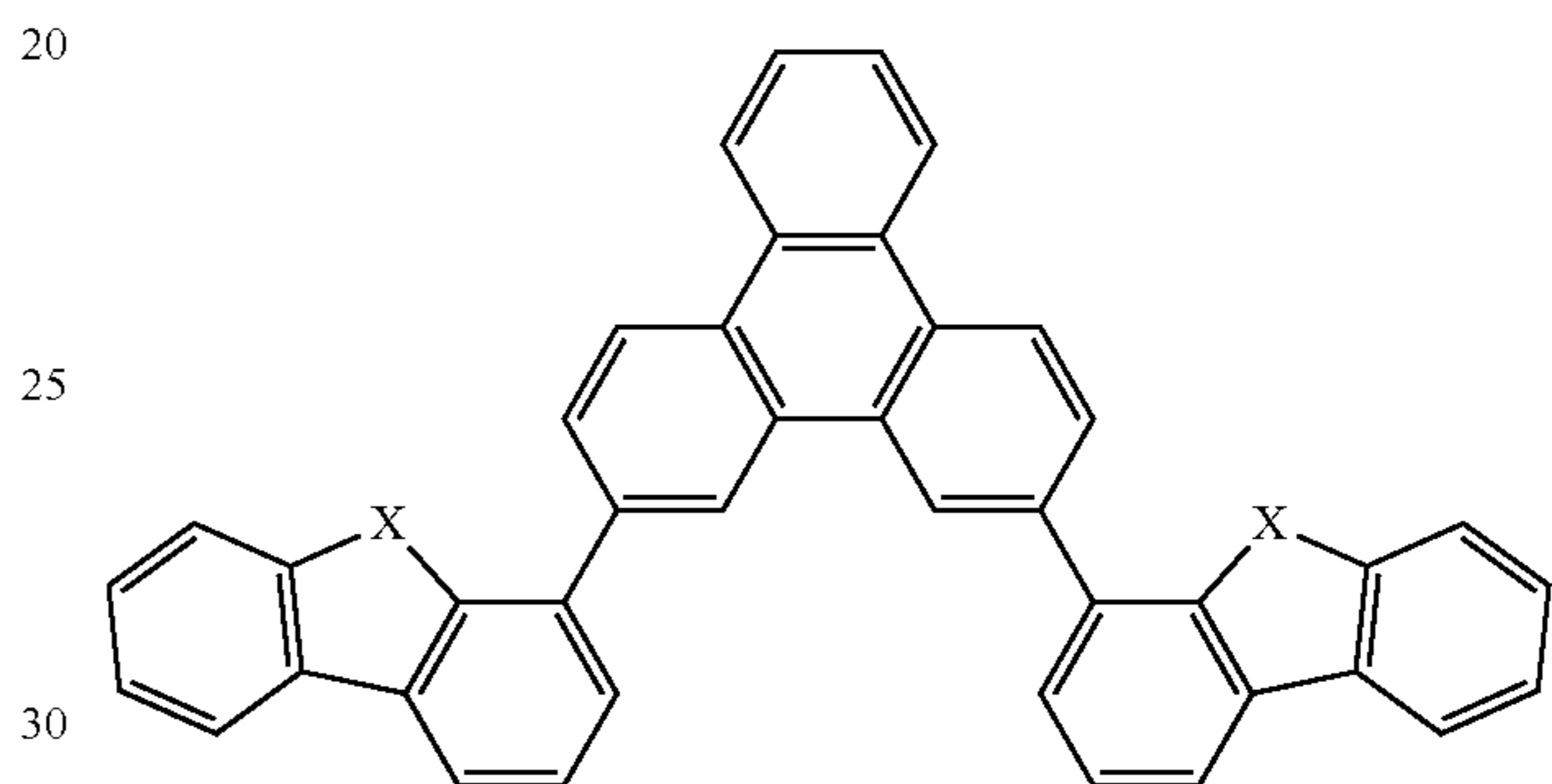
Compound 10
