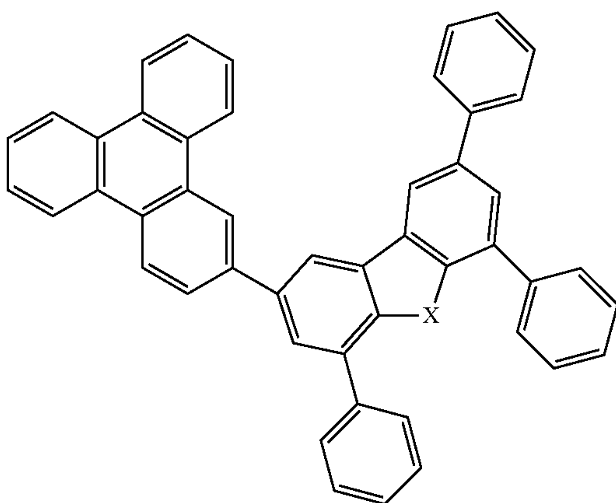
Compound 35
