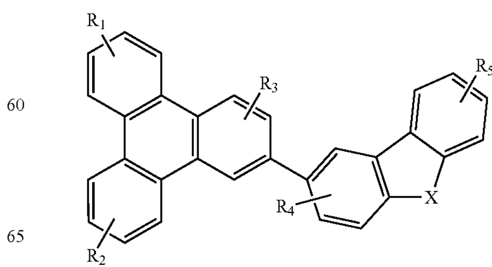
Compound 41G
