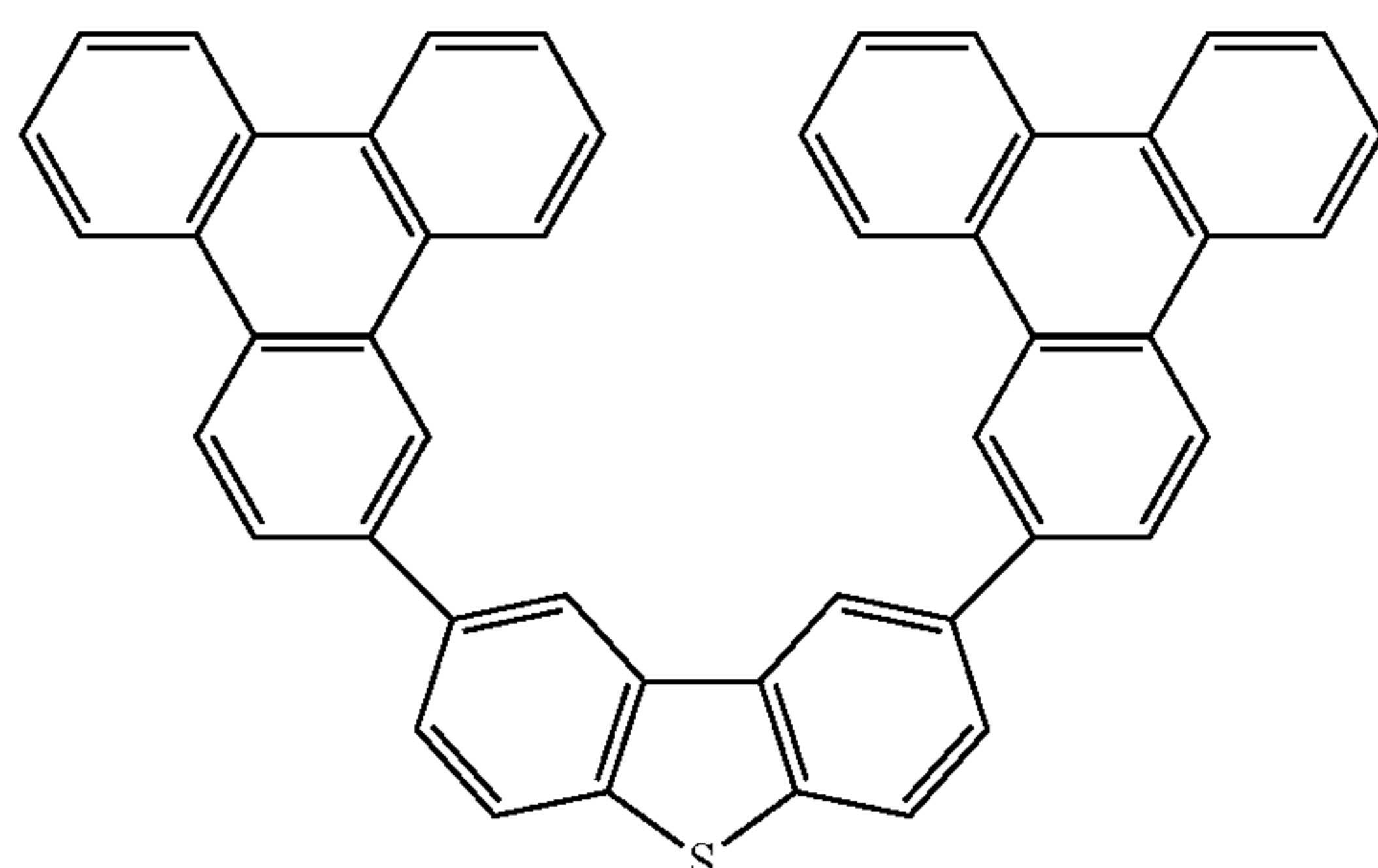
Compound 6'G
