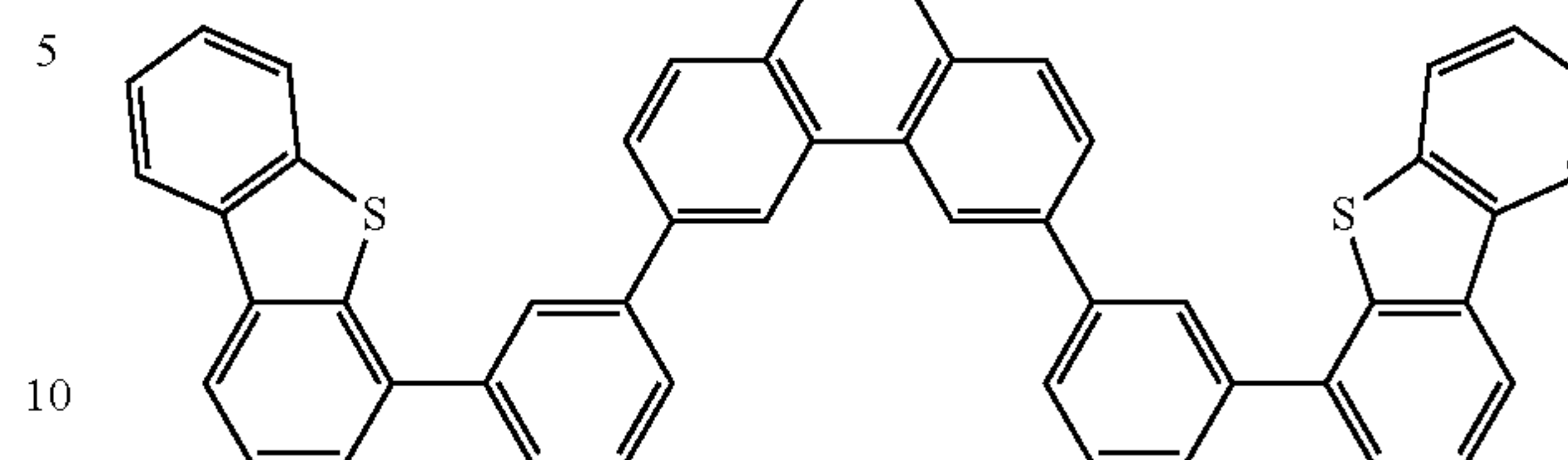
Compound 4S
