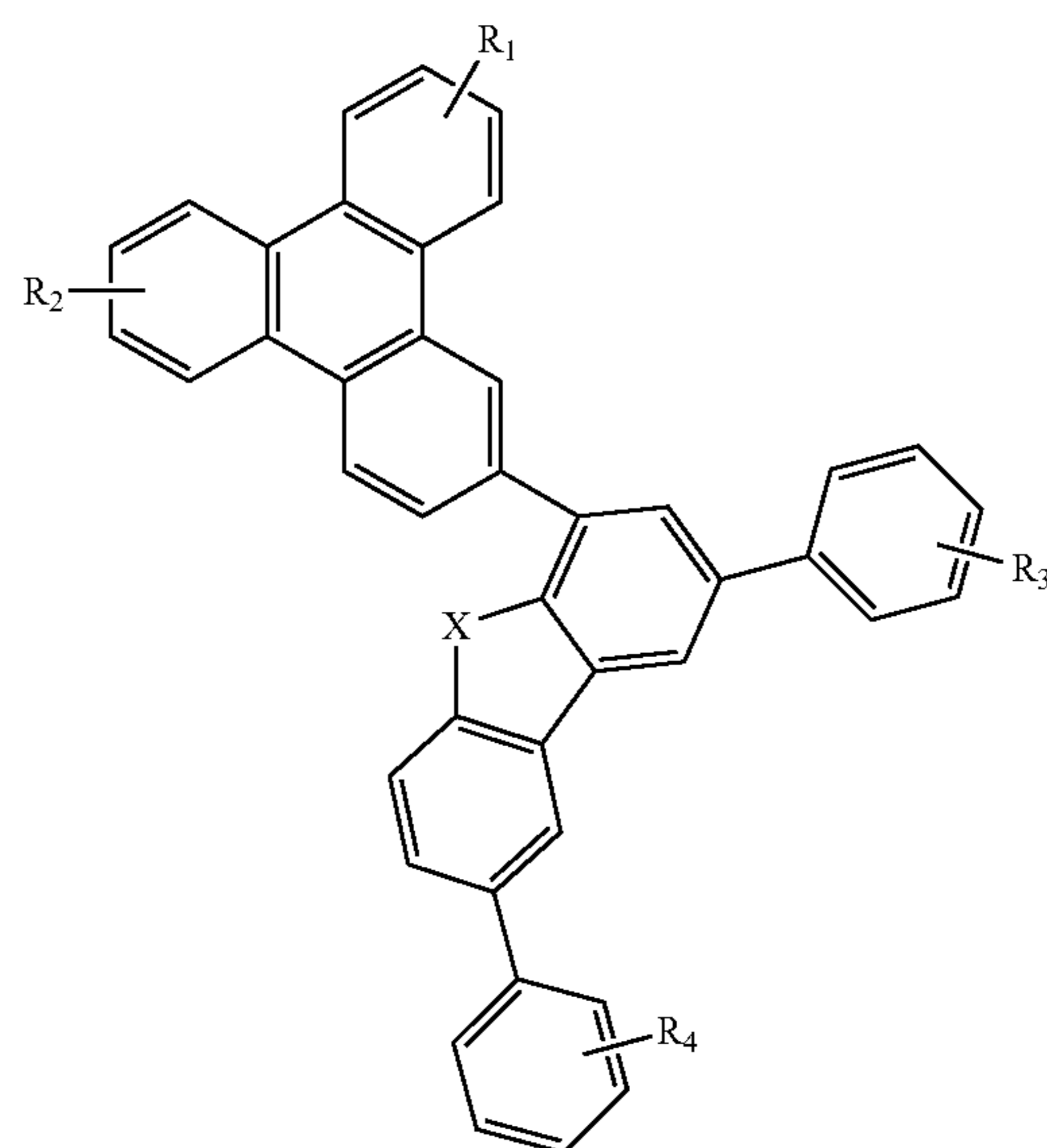
Compound 31G
