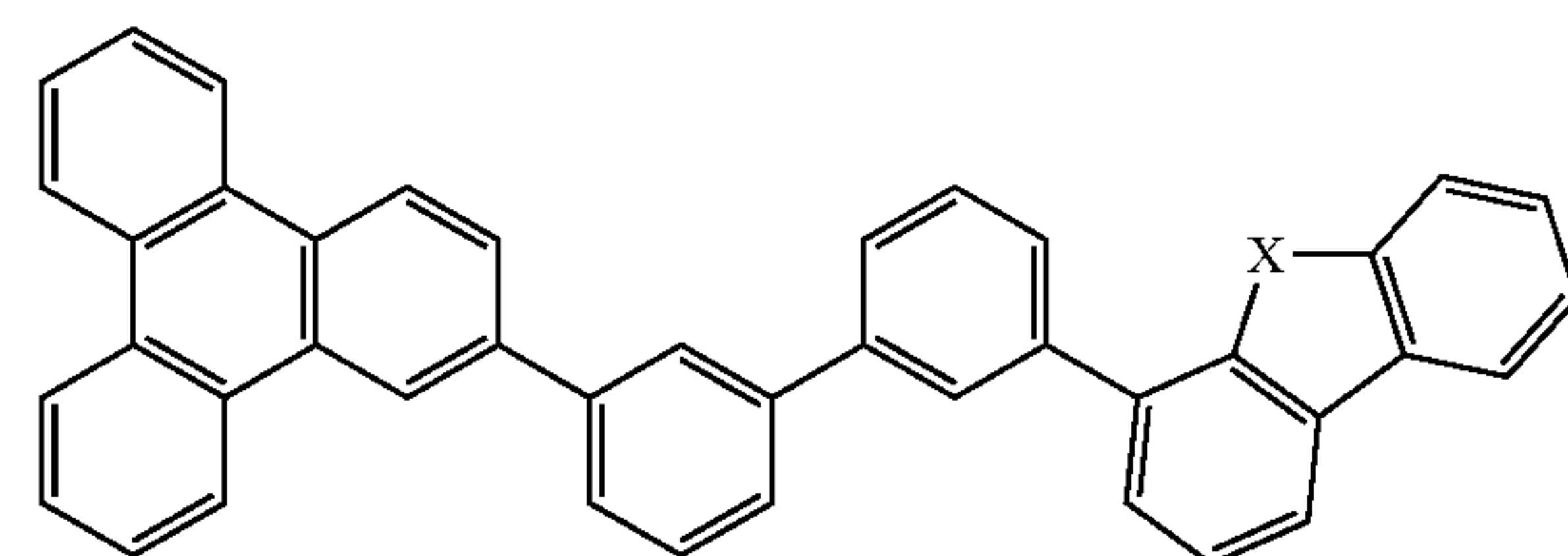
Compound 9
