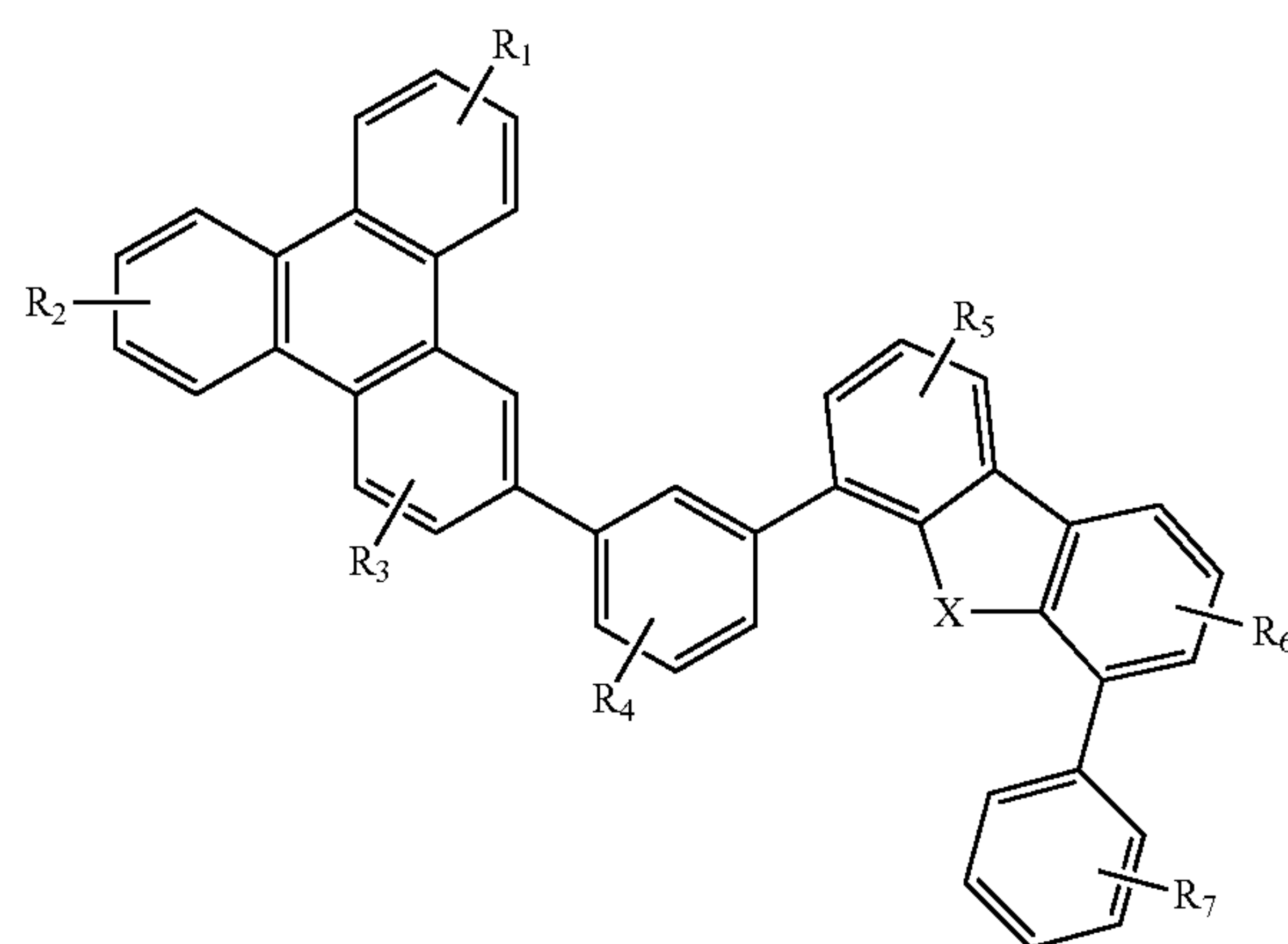
Compound 23G
