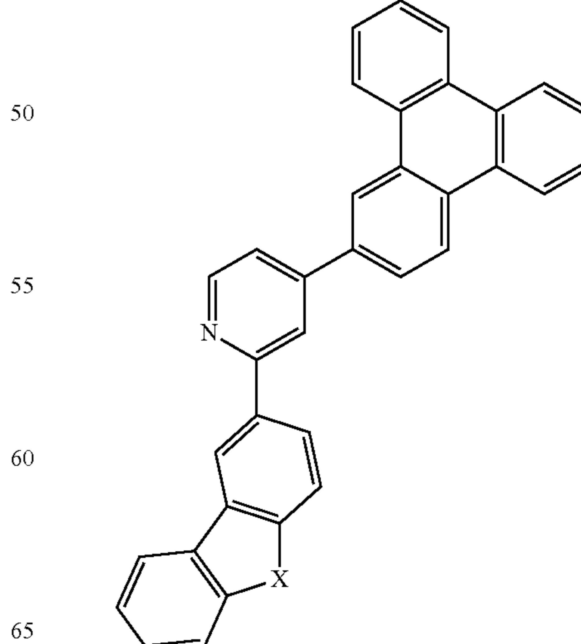
Compound 22
