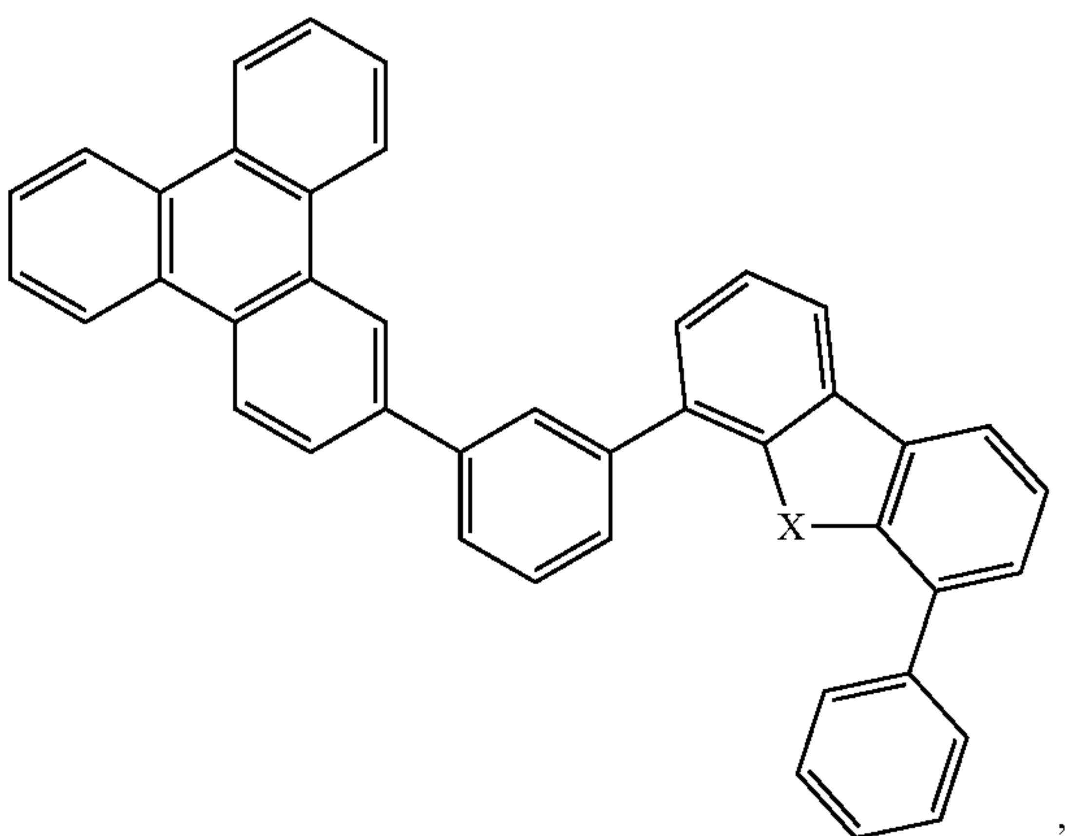
Compound 23
