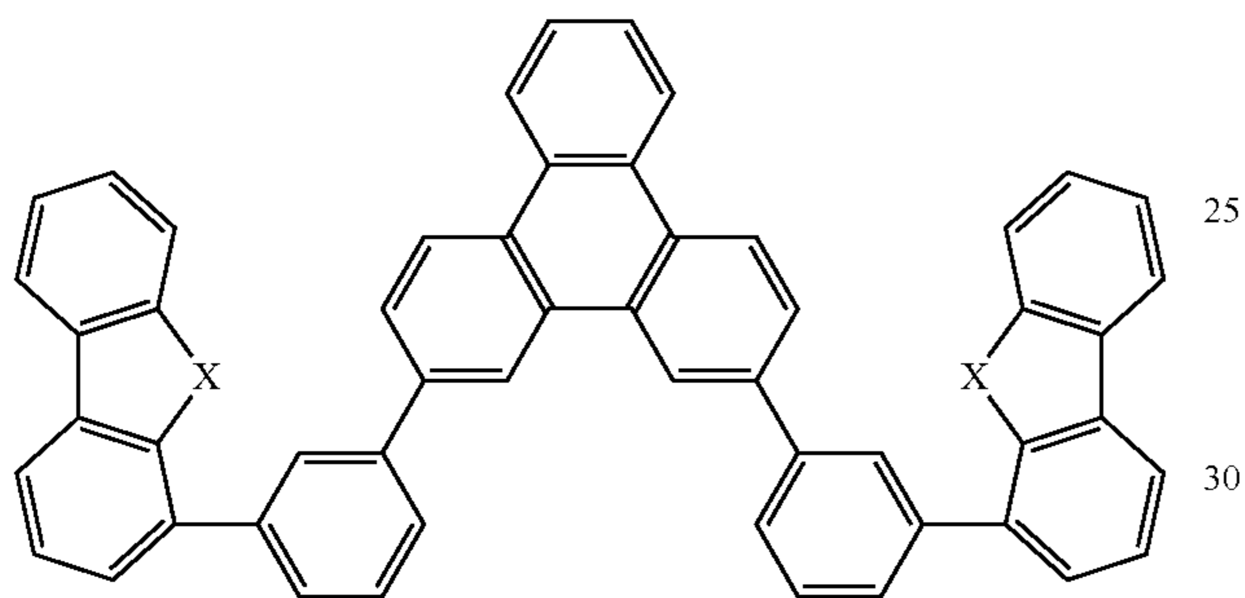
Compound 4
