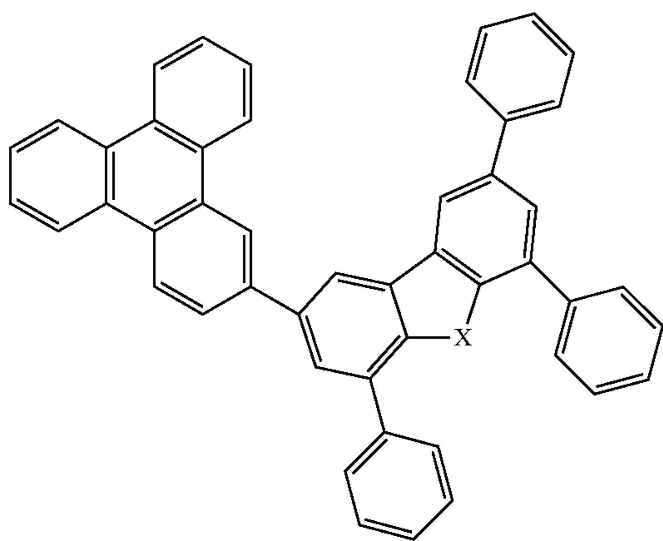
Compound 35
