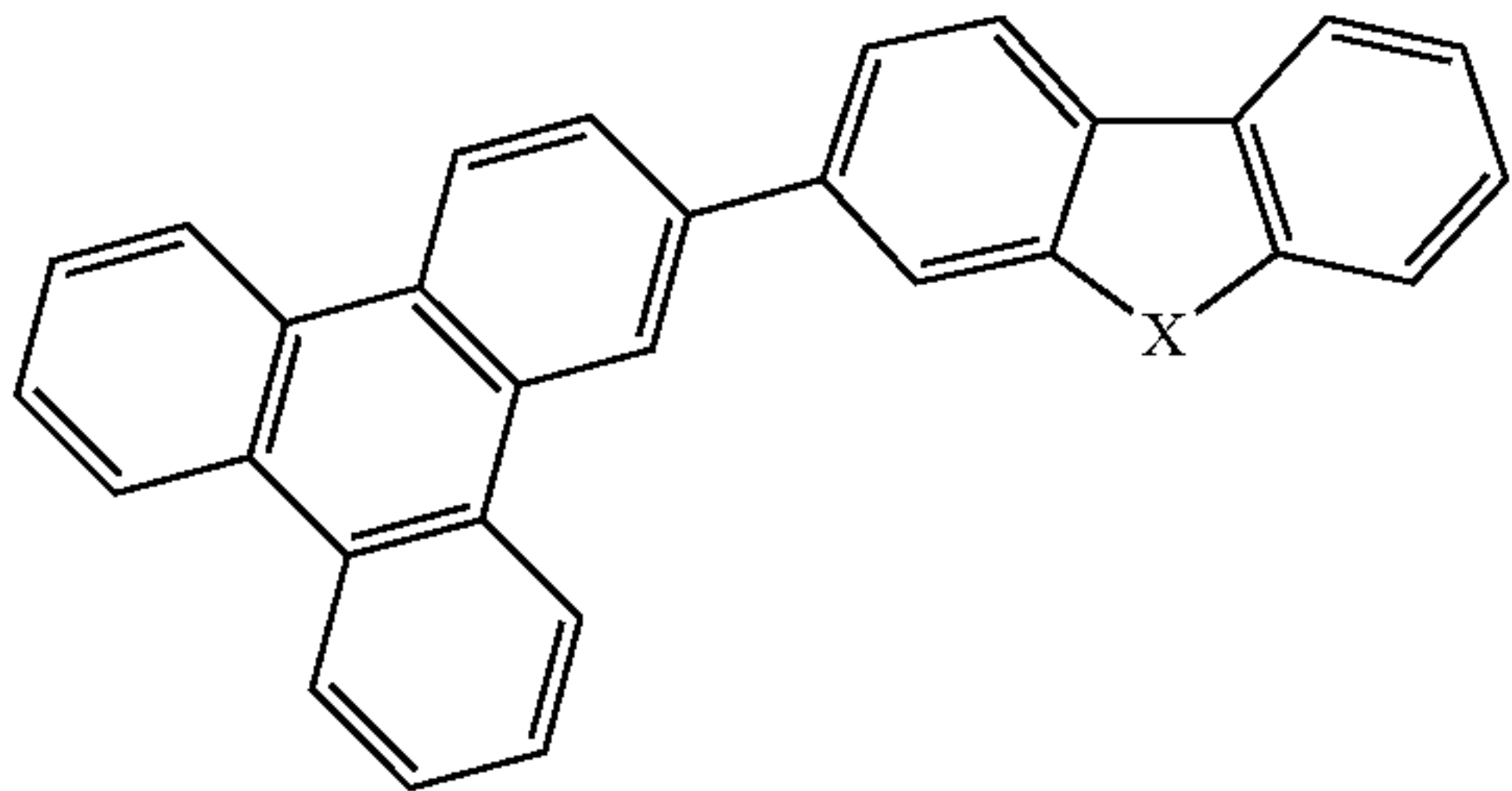
Compound 9
