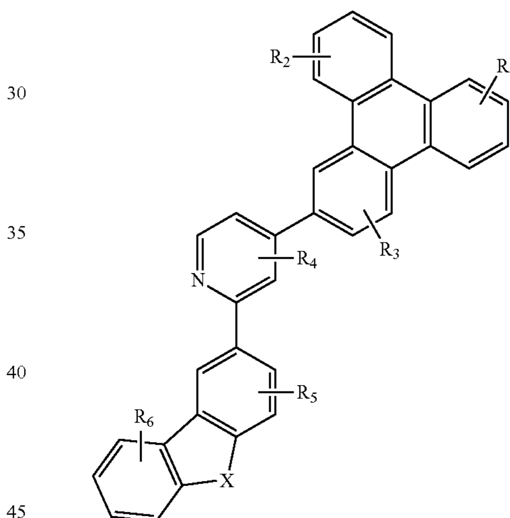
Compound 43G
