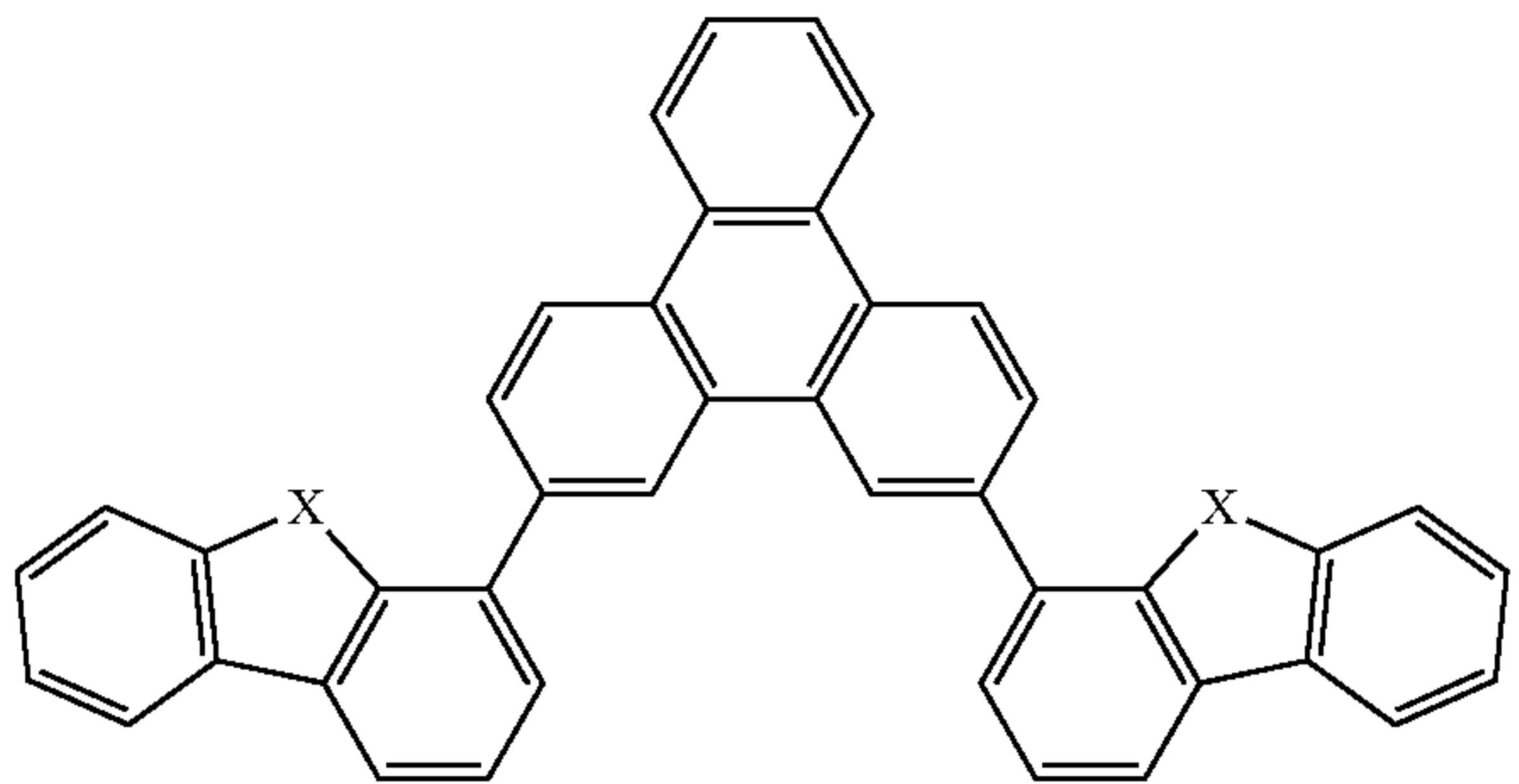
Compound 10
