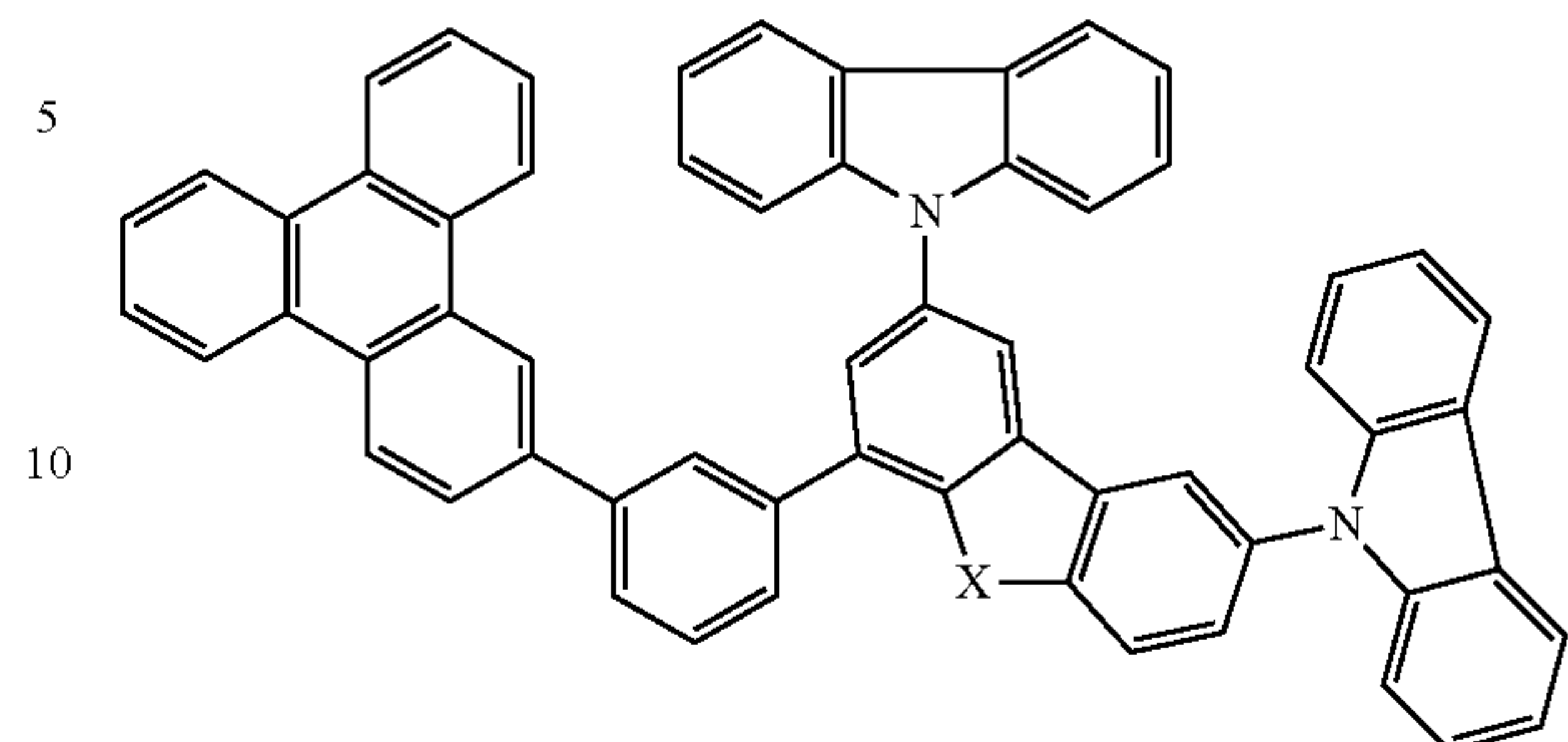
Compound 27
