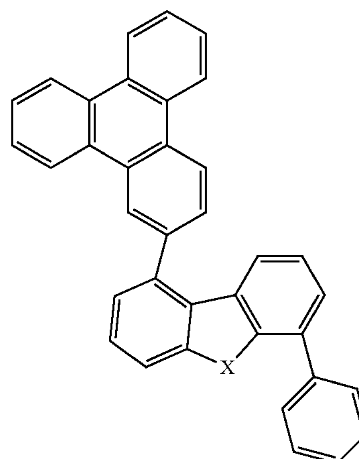
Compound 29G
