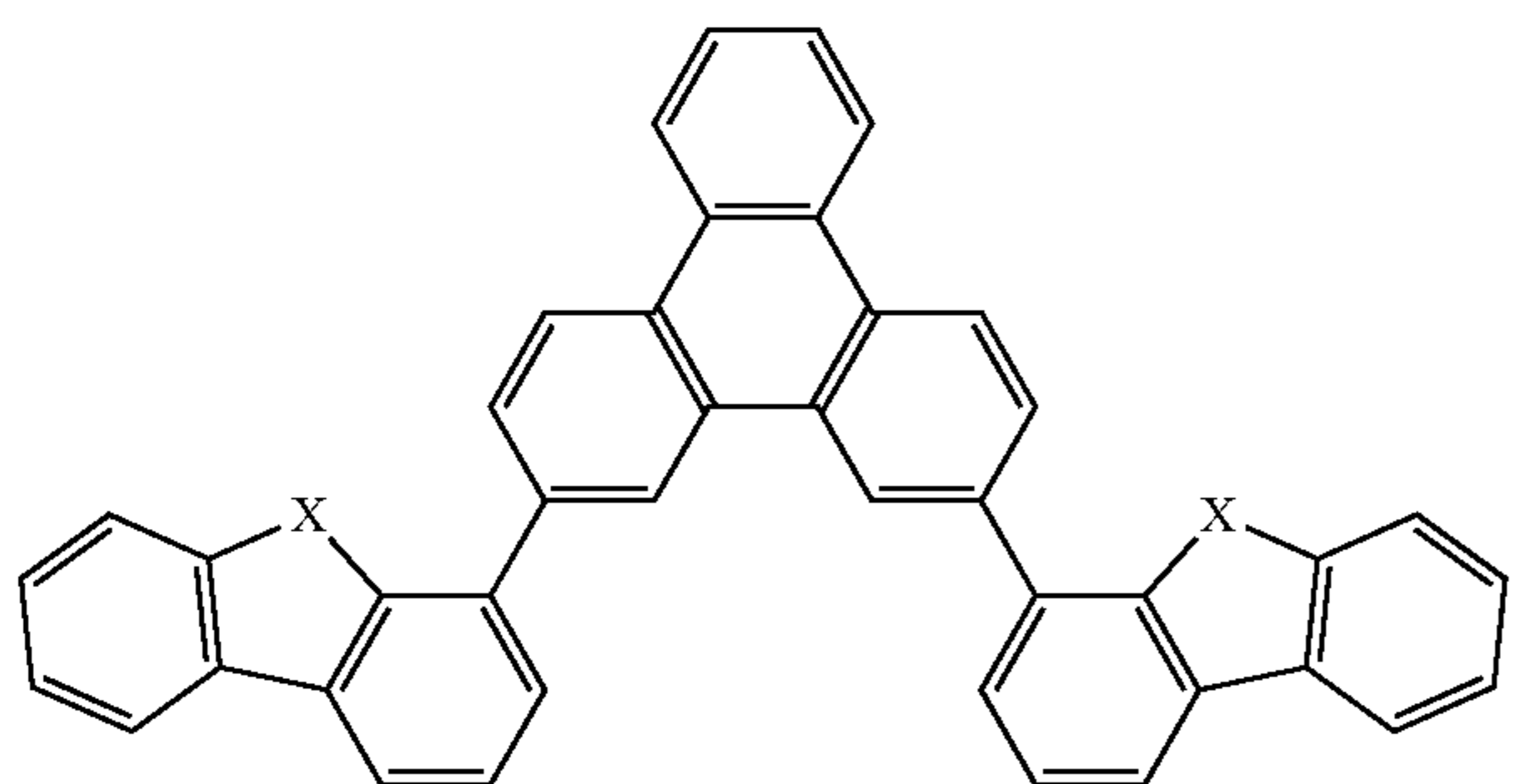
Compound 10
