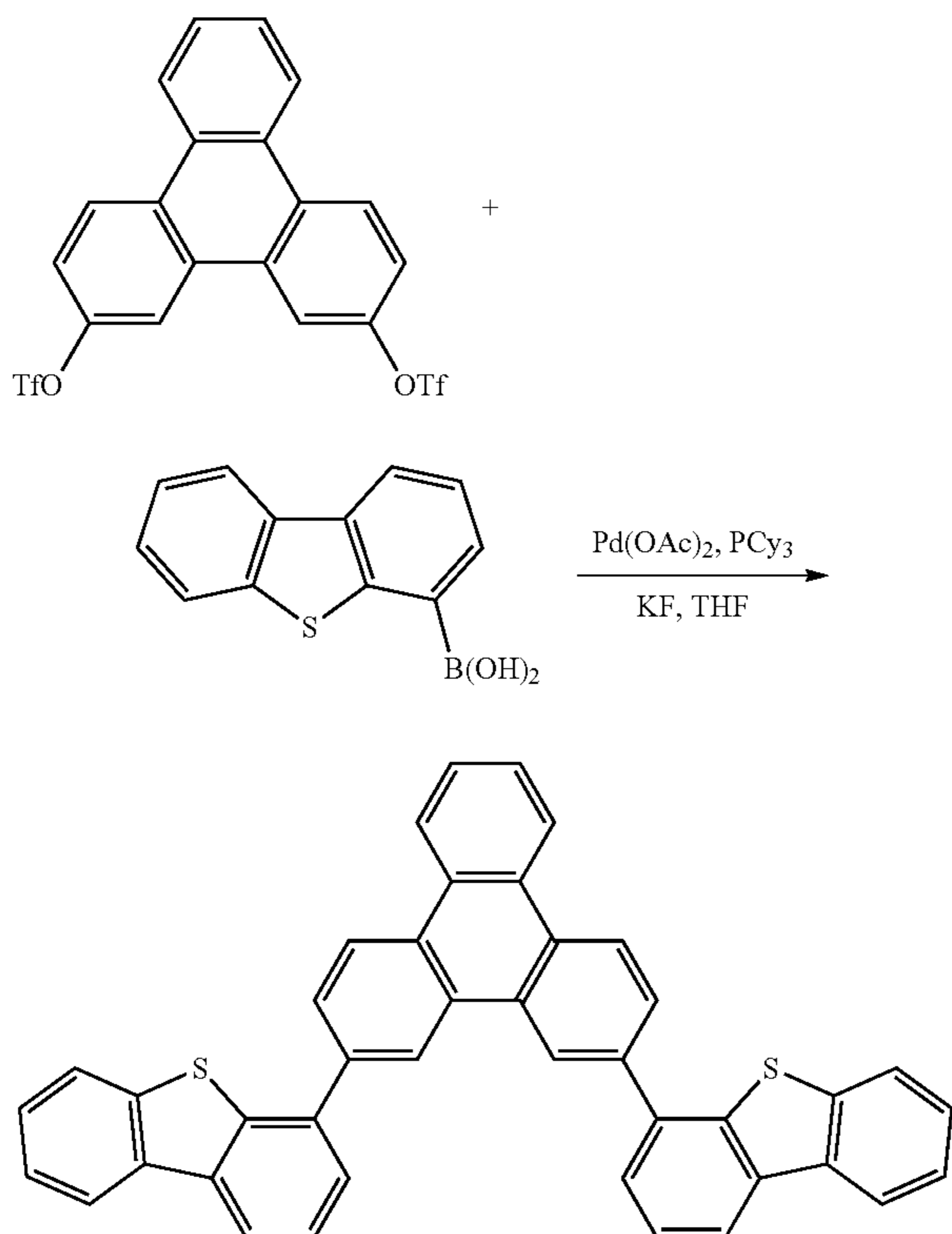
Compound 10S
