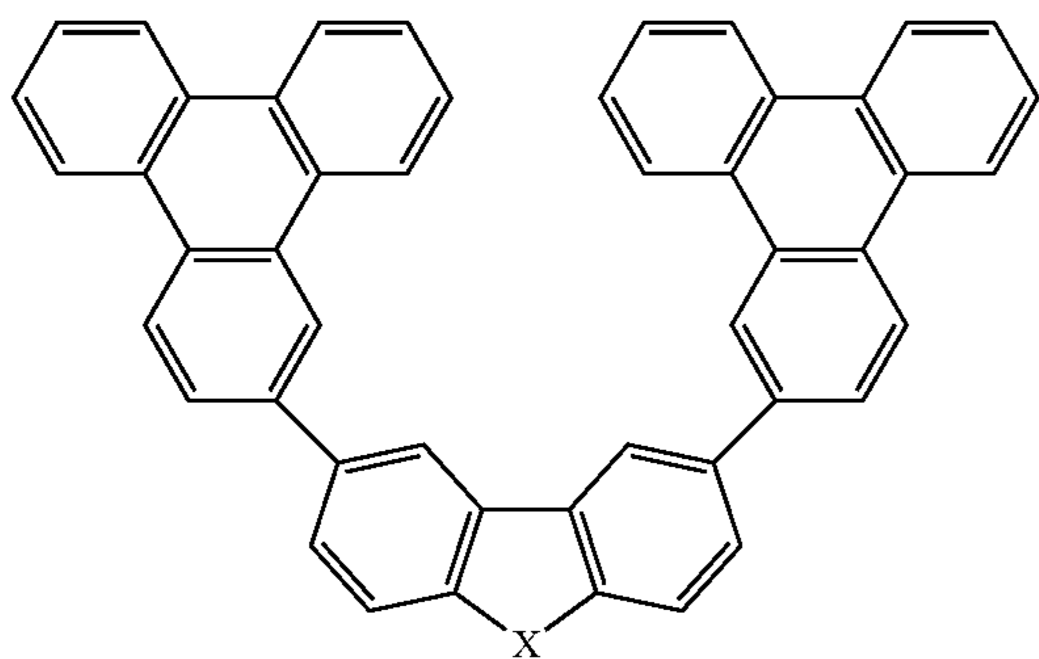
Compound 5
