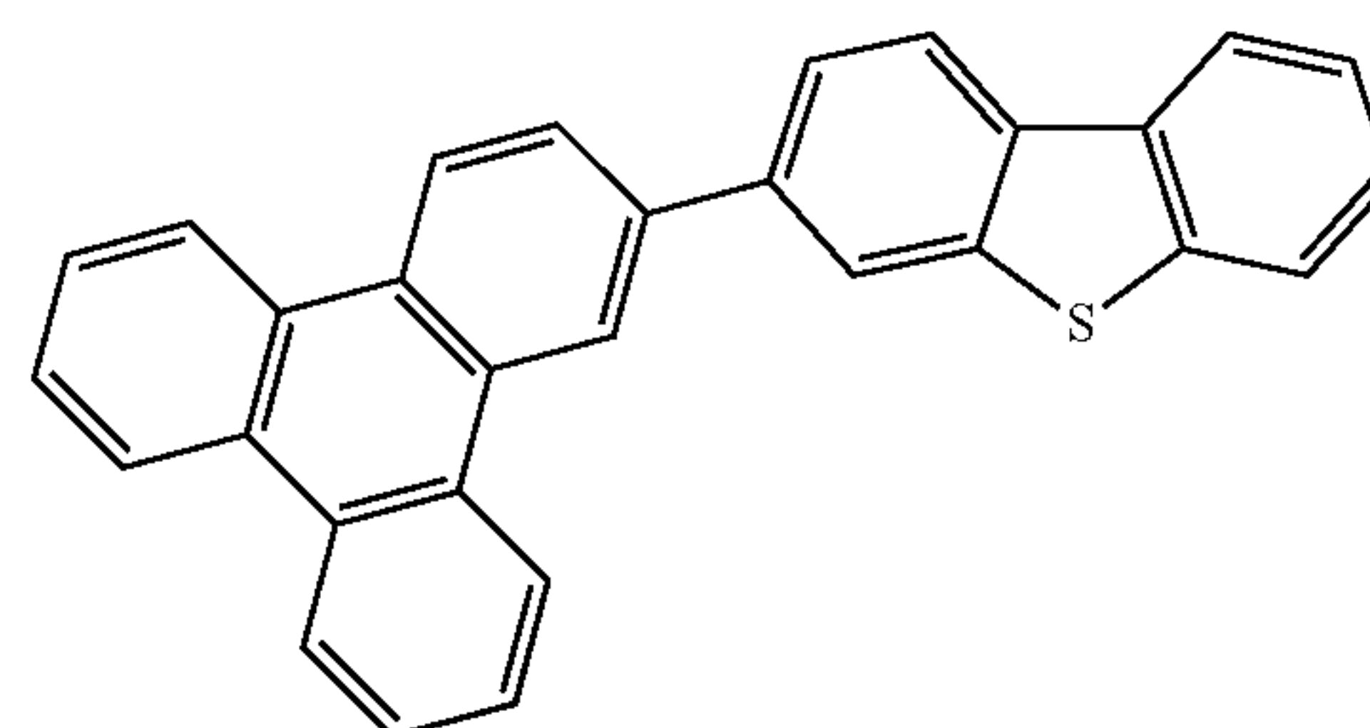
Compound 8'
