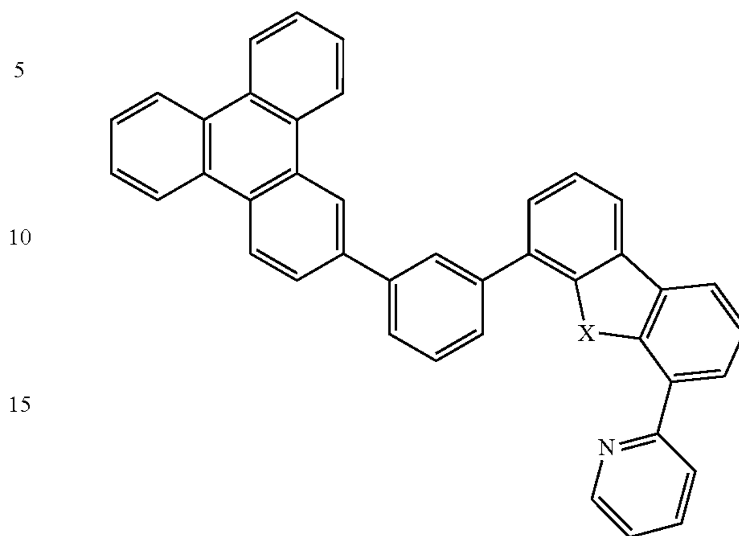
Compound 48G
