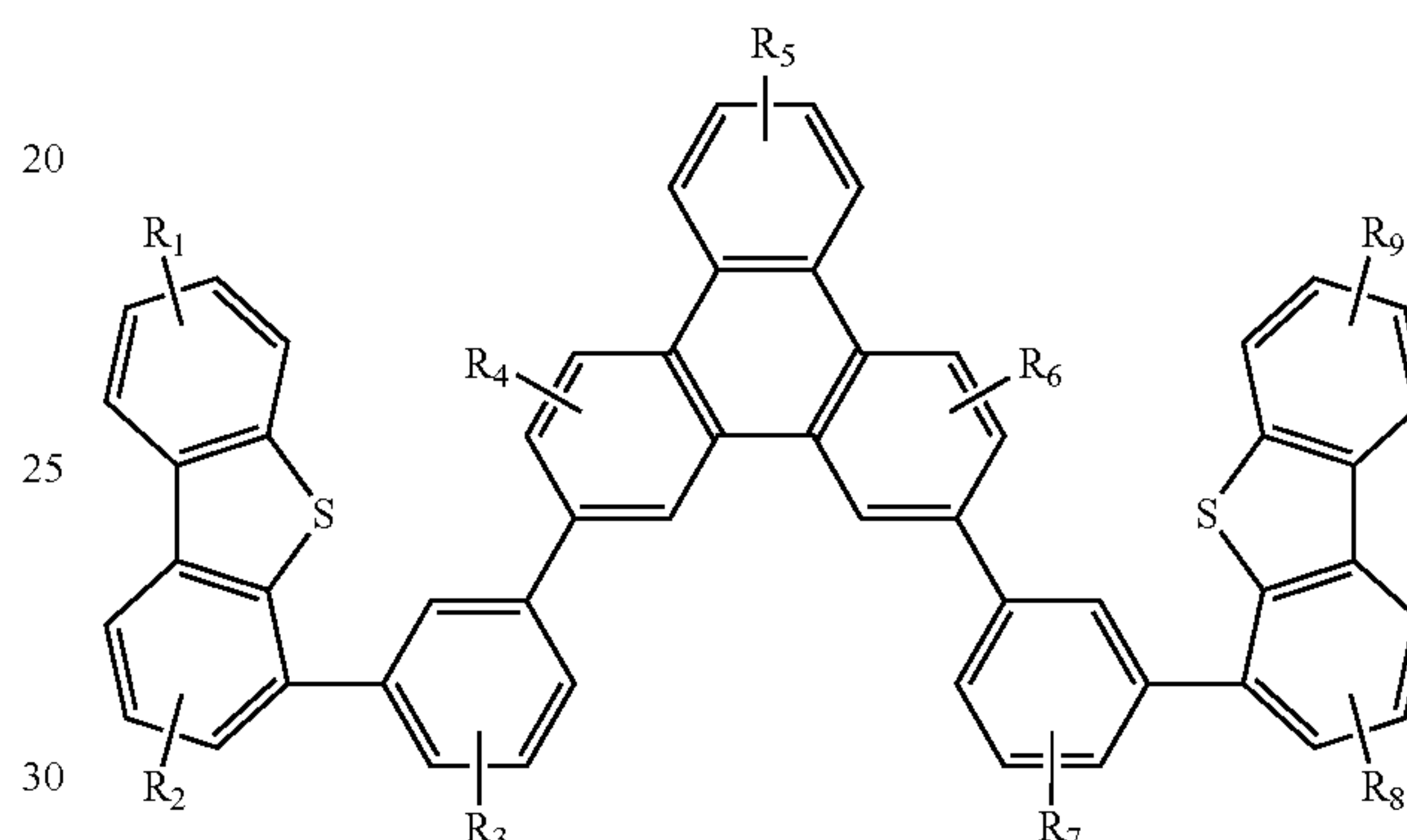
Compound 4'G
