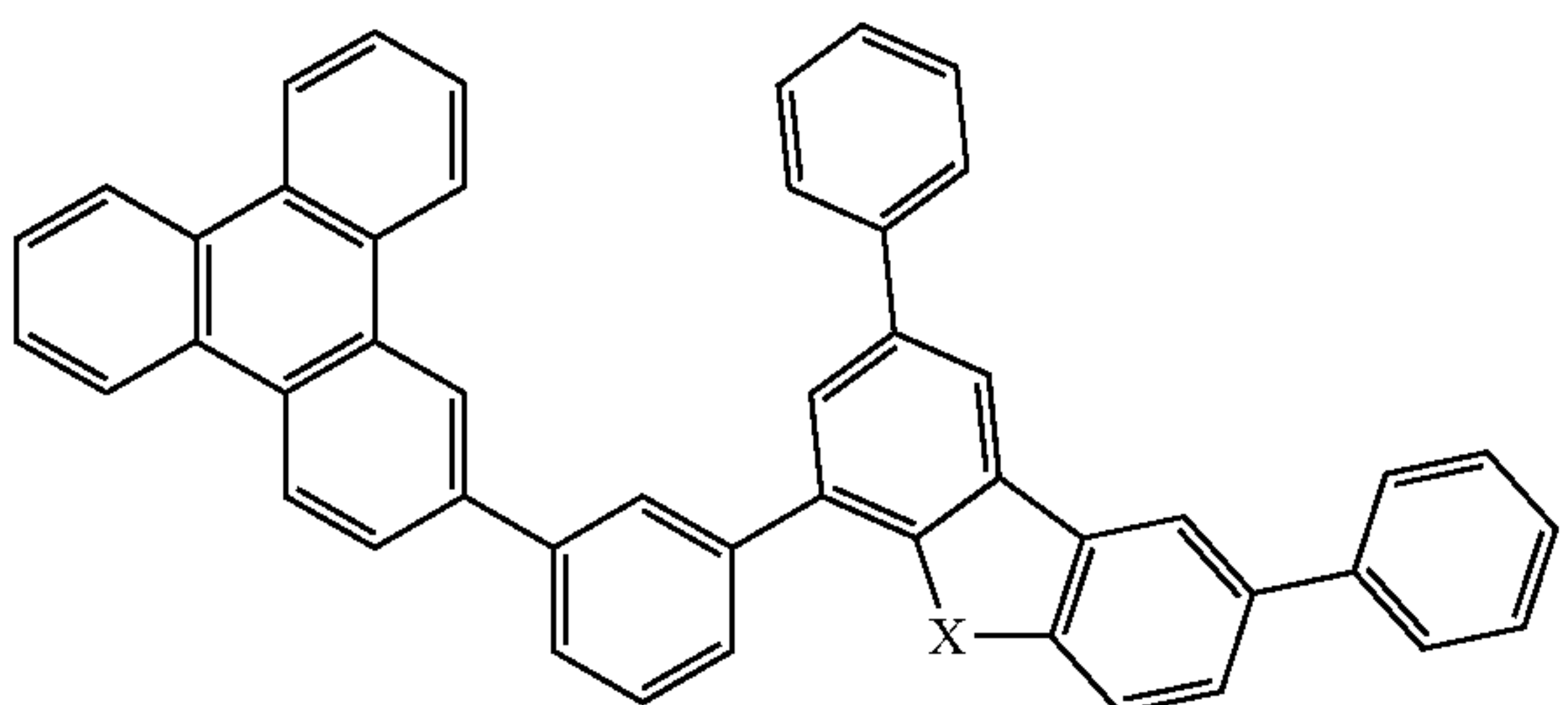
Compound 24
