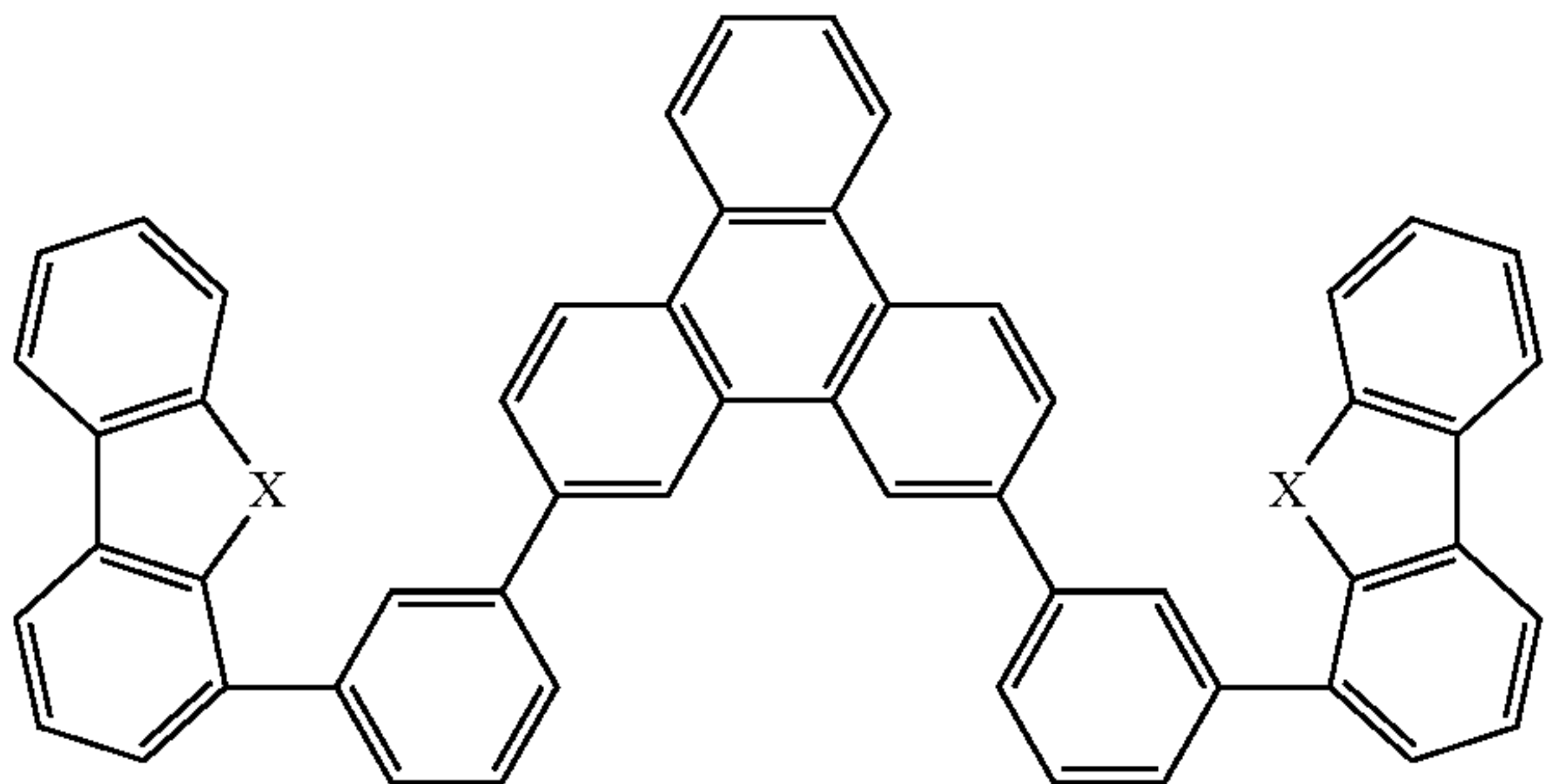
Compound 4
