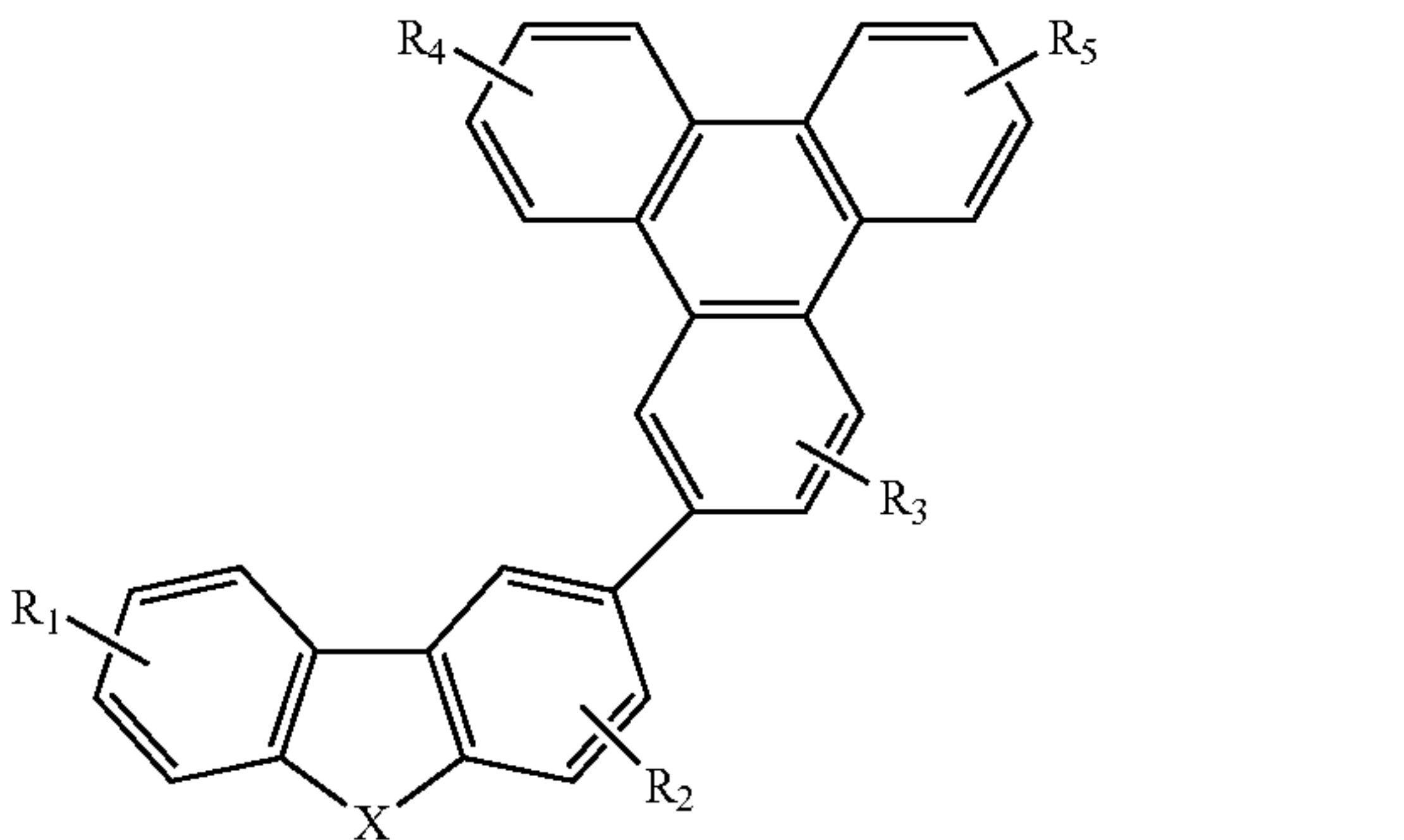
Compound 6
