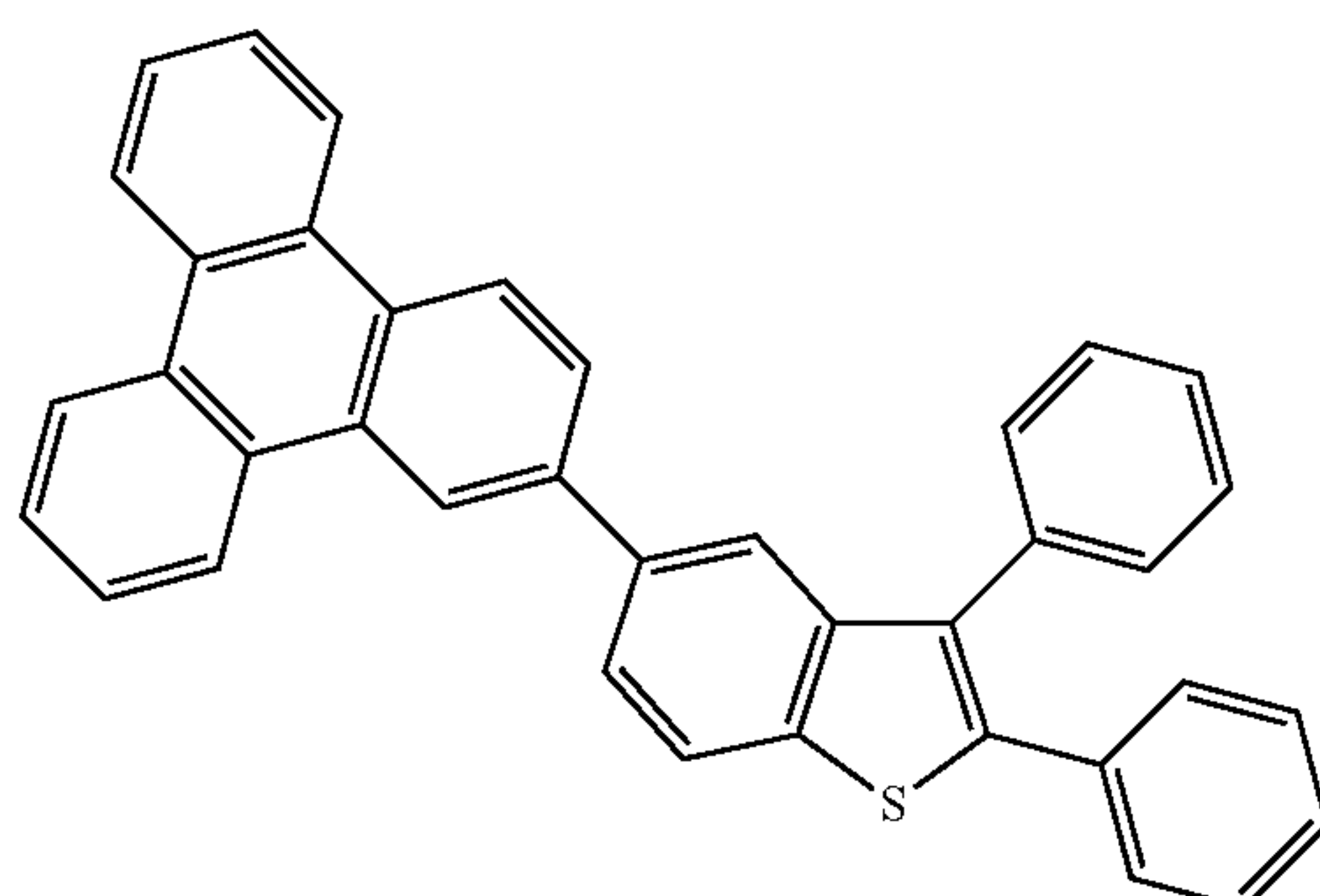
Compound 13'
