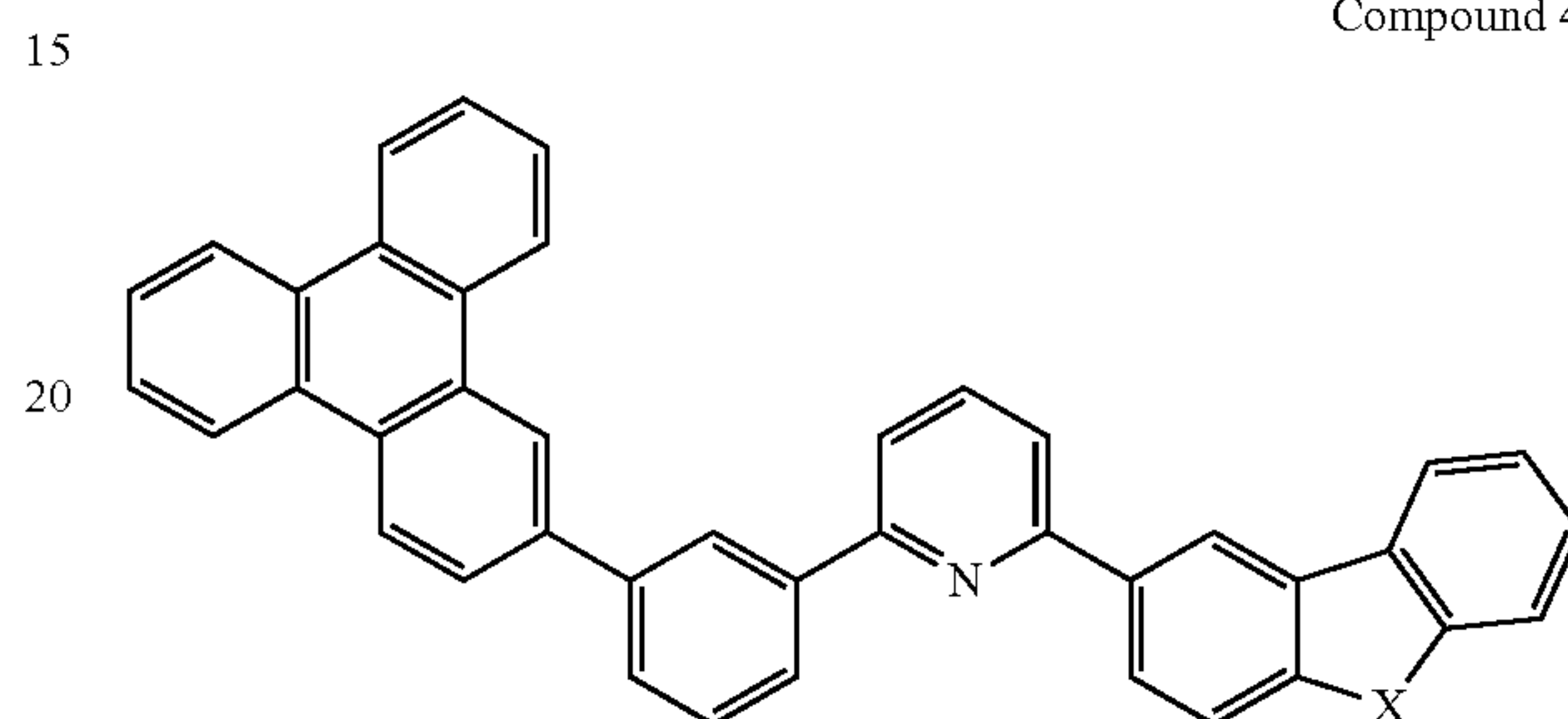
Compound 45G
