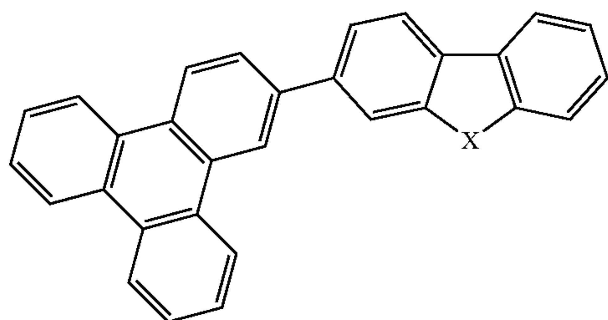
Compound 8
