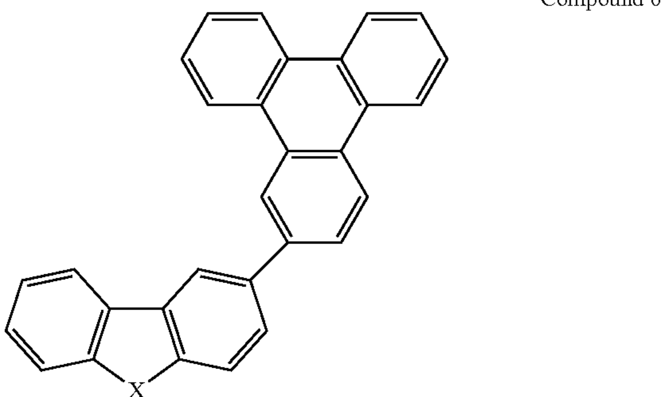
Compound 7G
