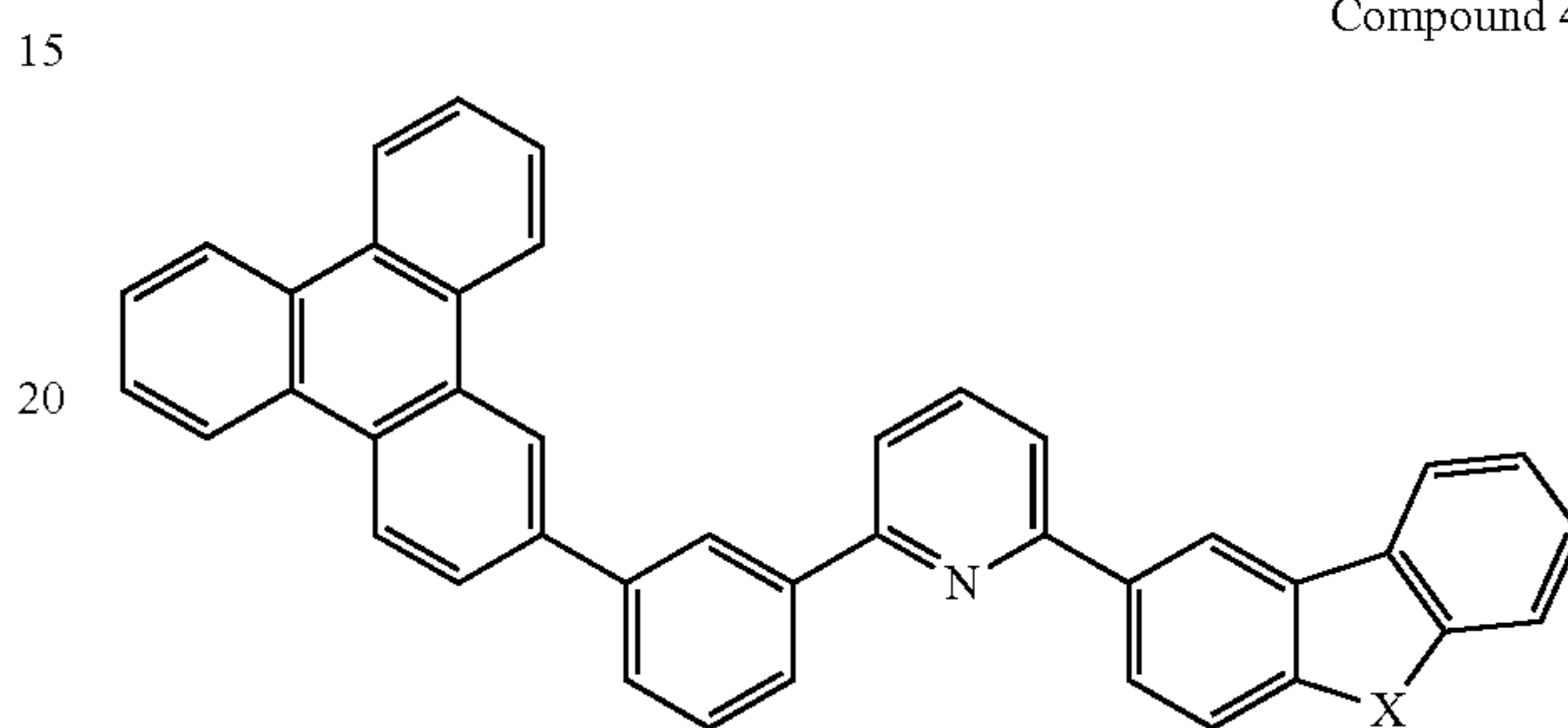
Compound 45G
