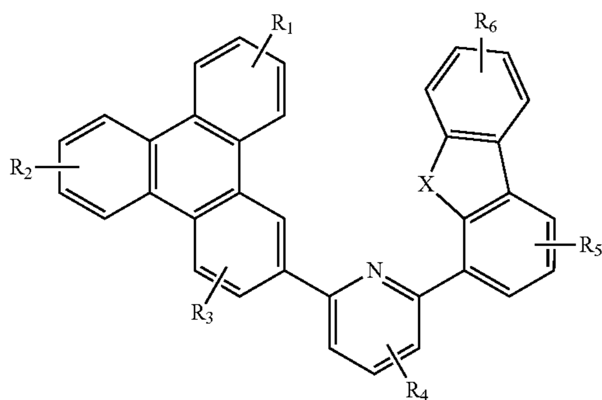
Compound 22G
