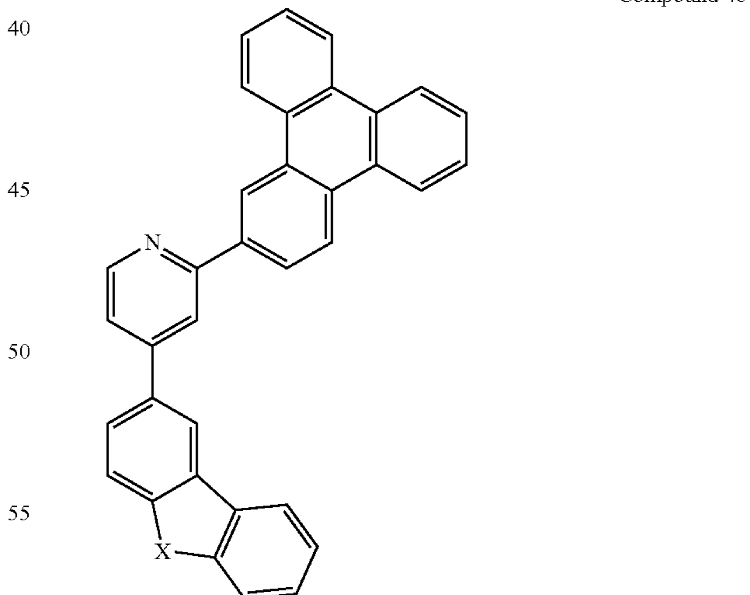
Compound 48
