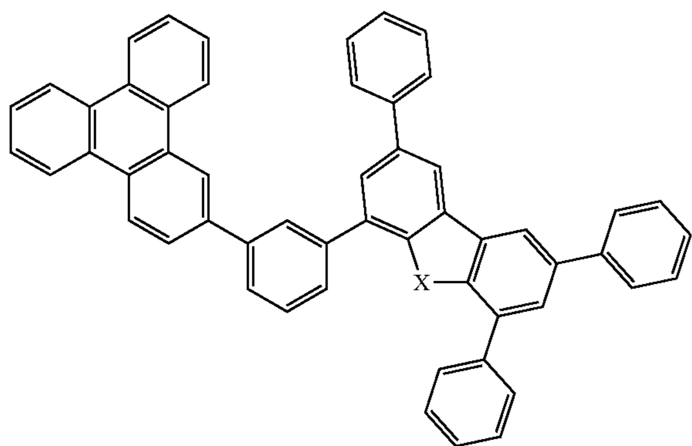
Compound 25
