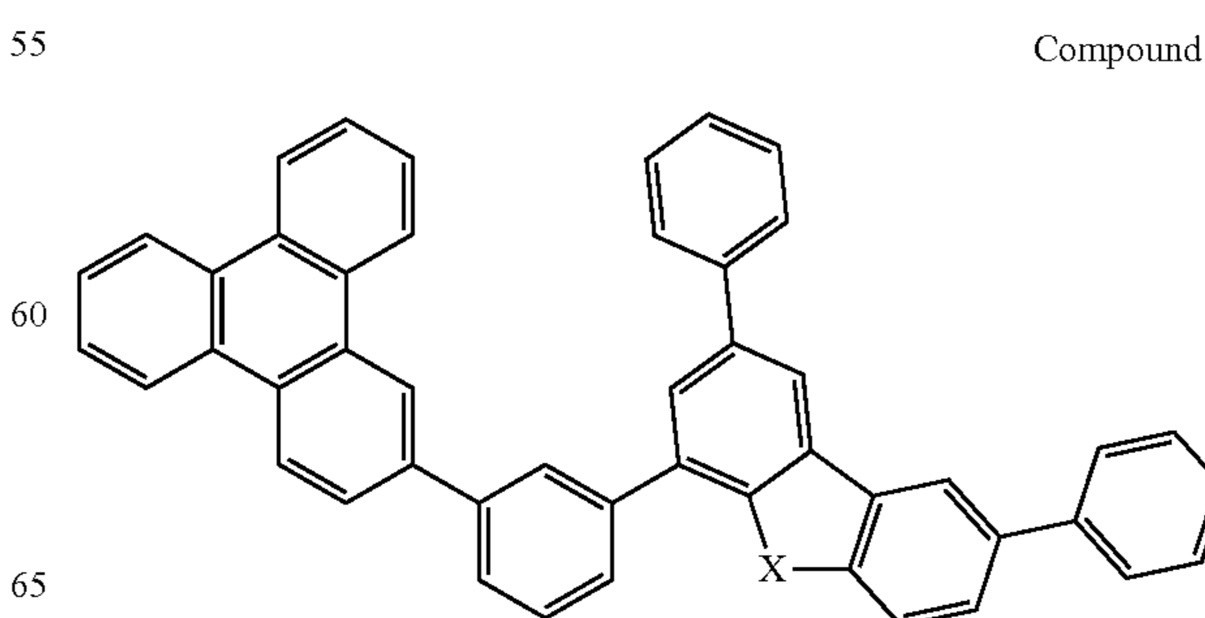
Compound 9
