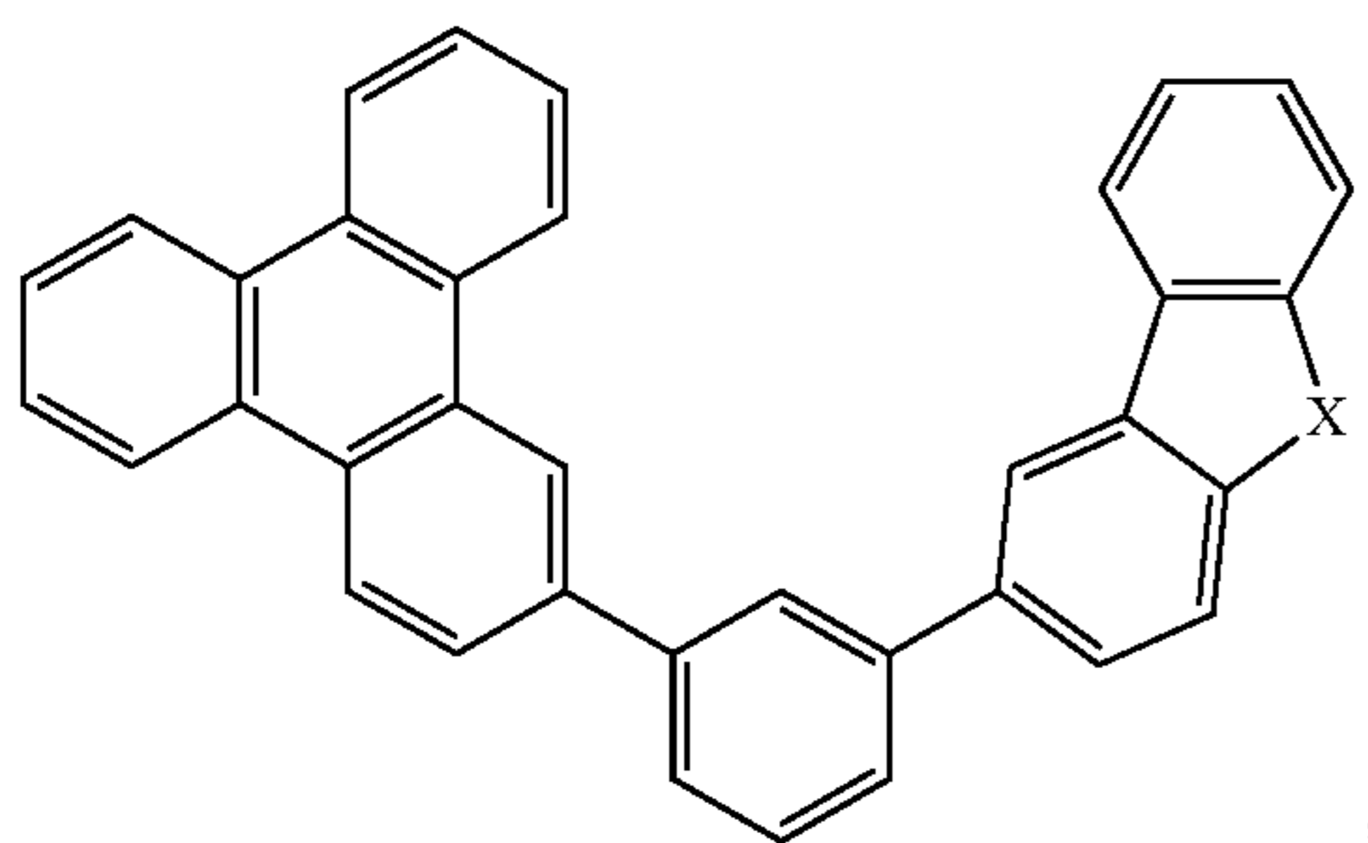
Compound 20
