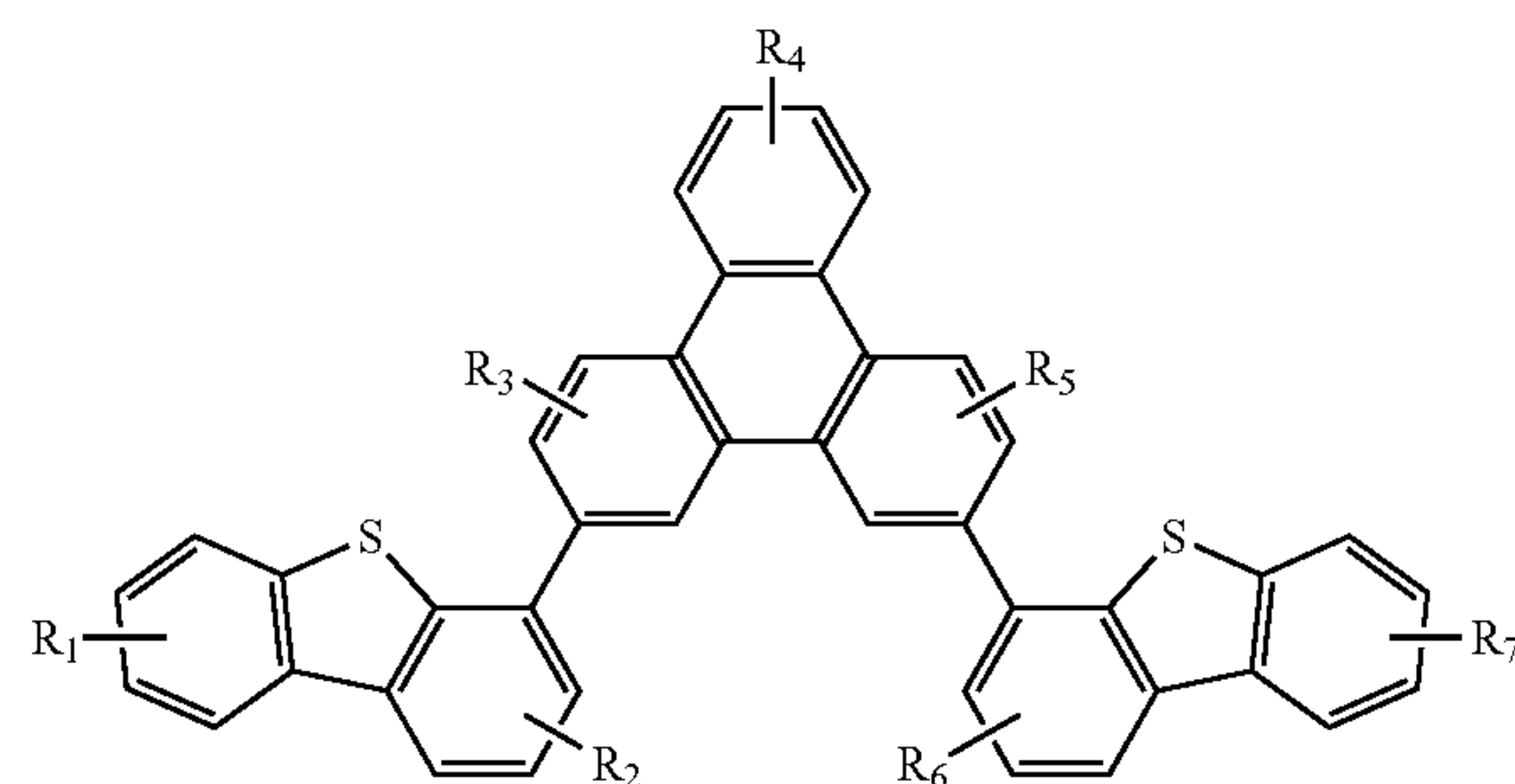
Compound 10'G
