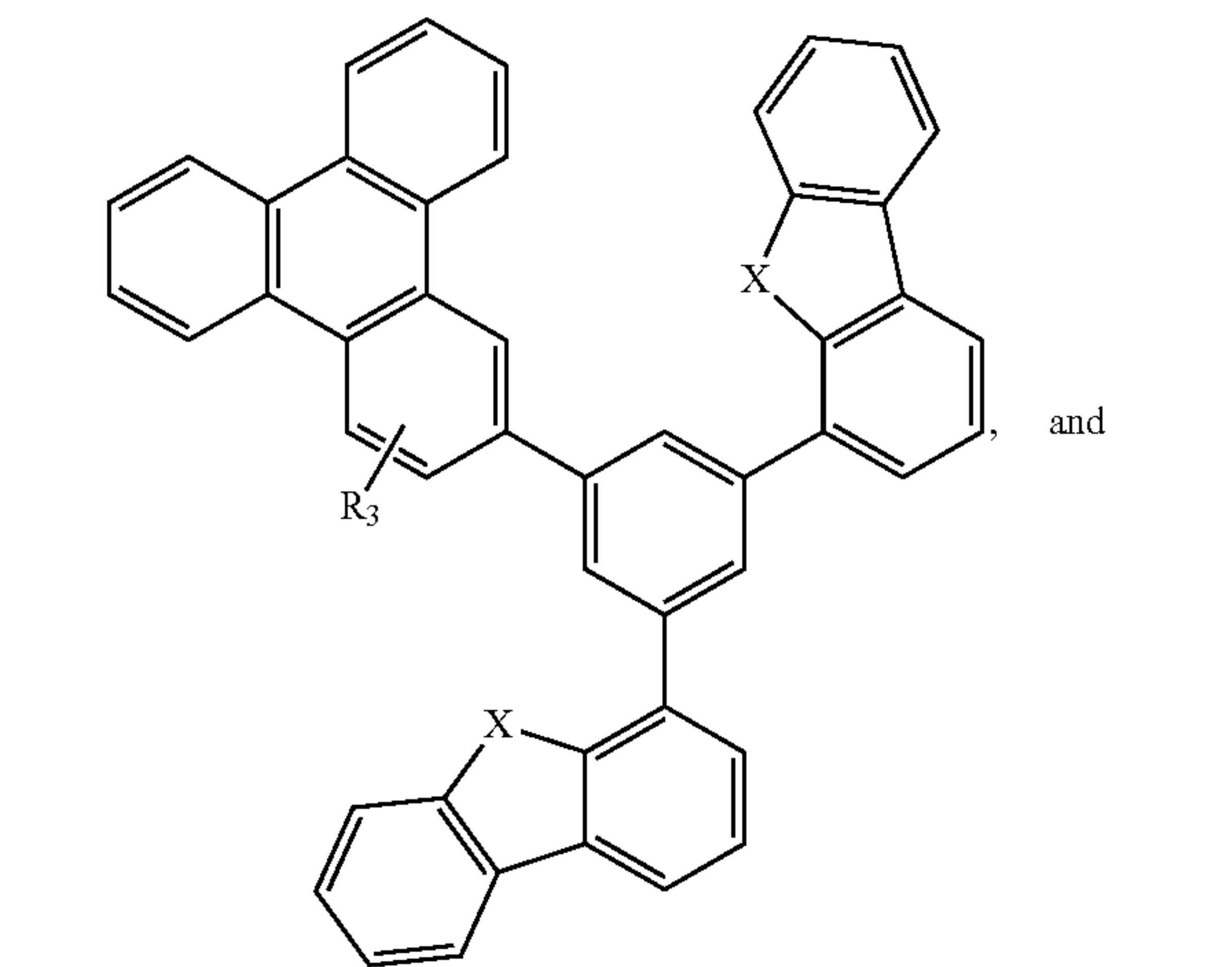
Compound 37
