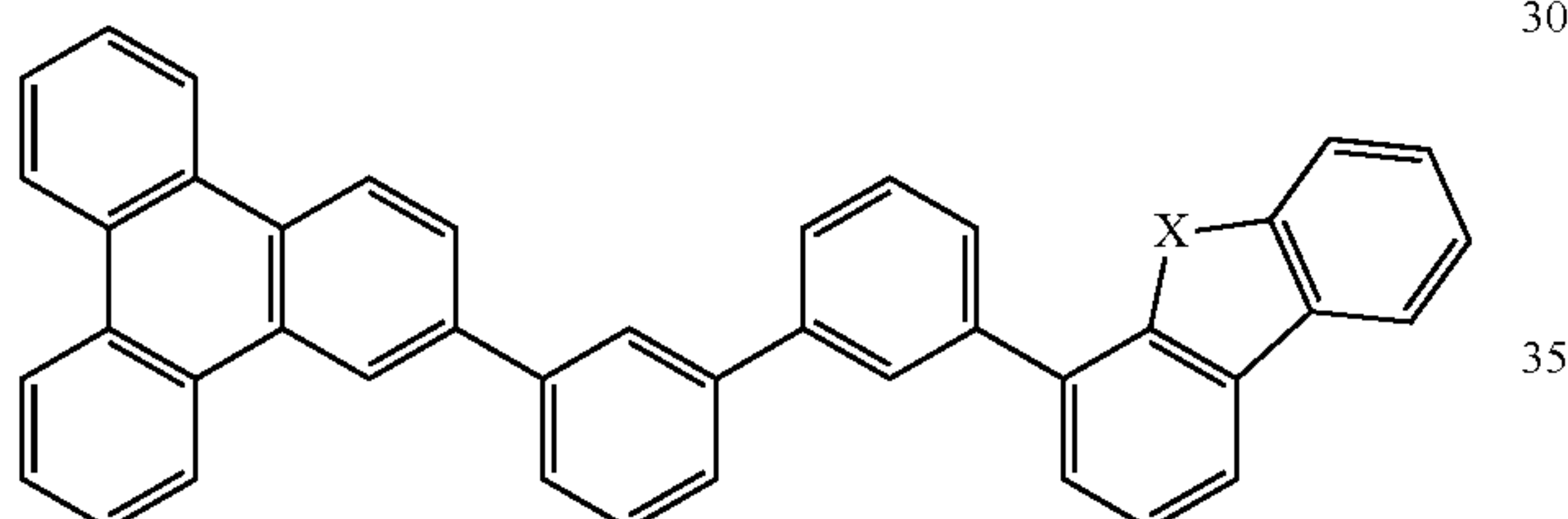
Compound 9
