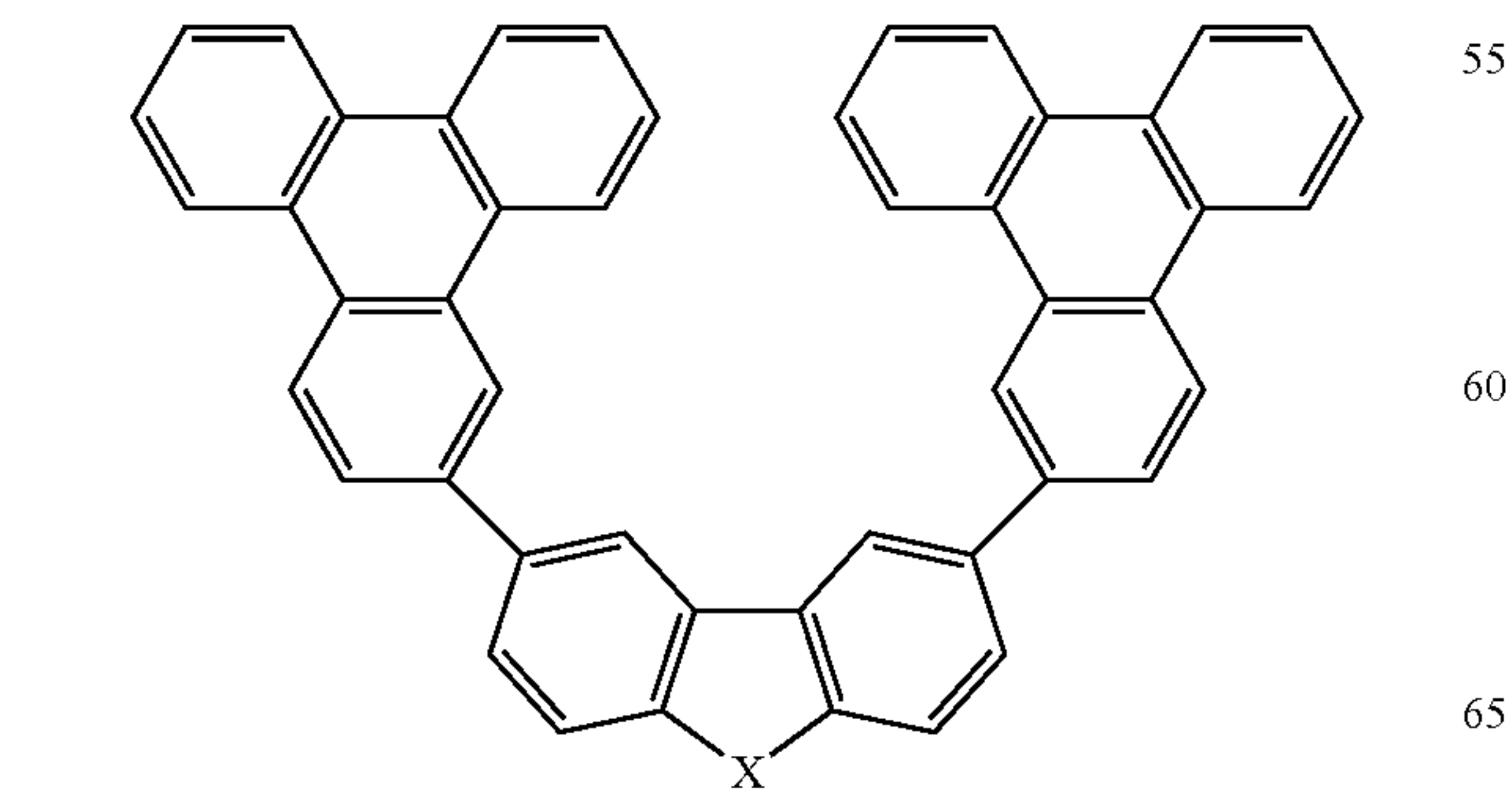
Compound 5
