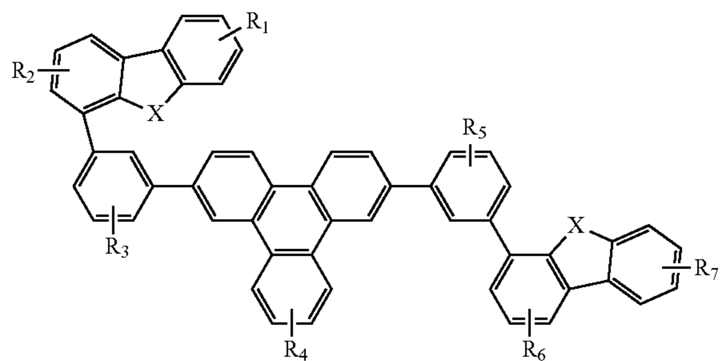
Compound 26G
