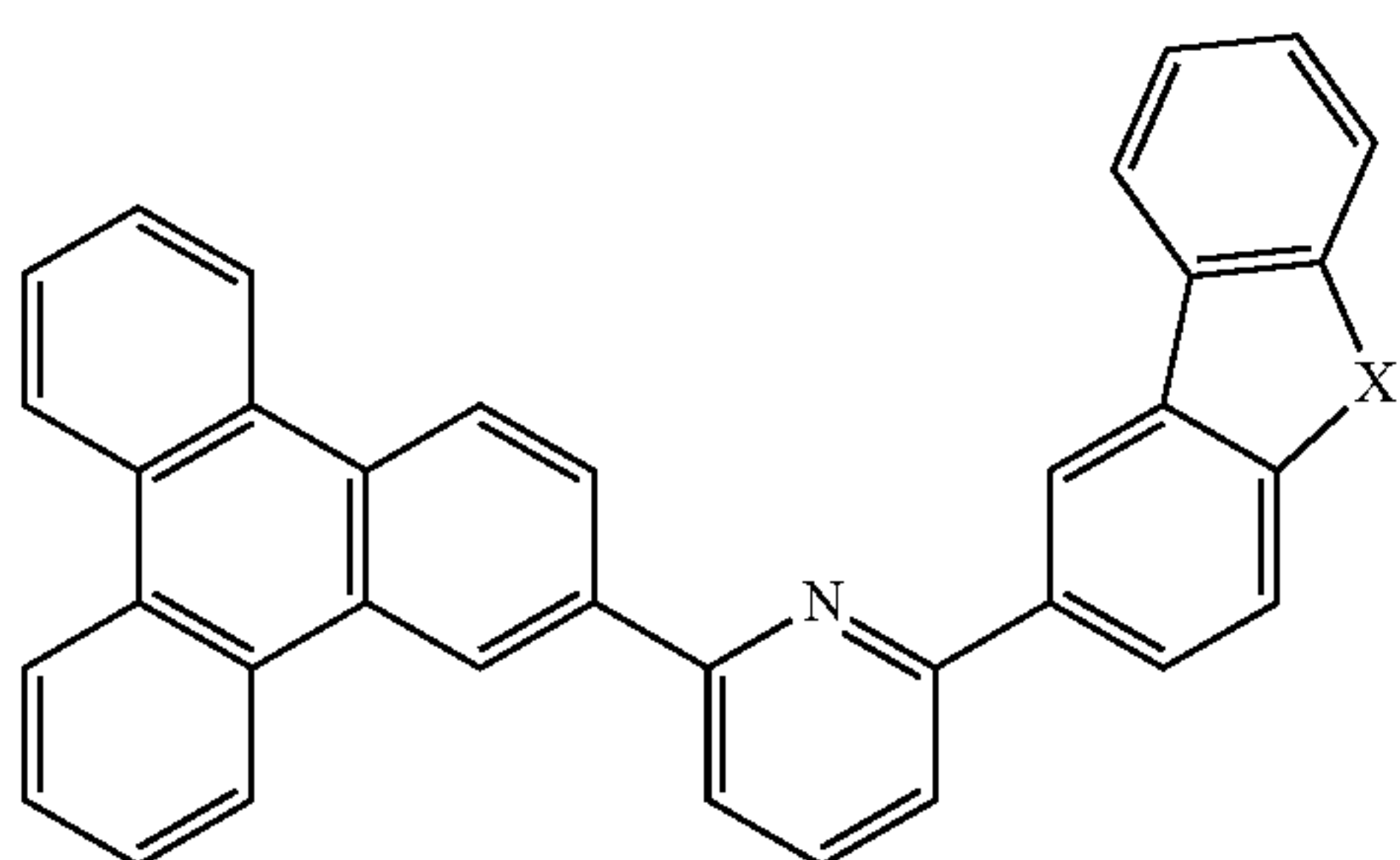
Compound 43
