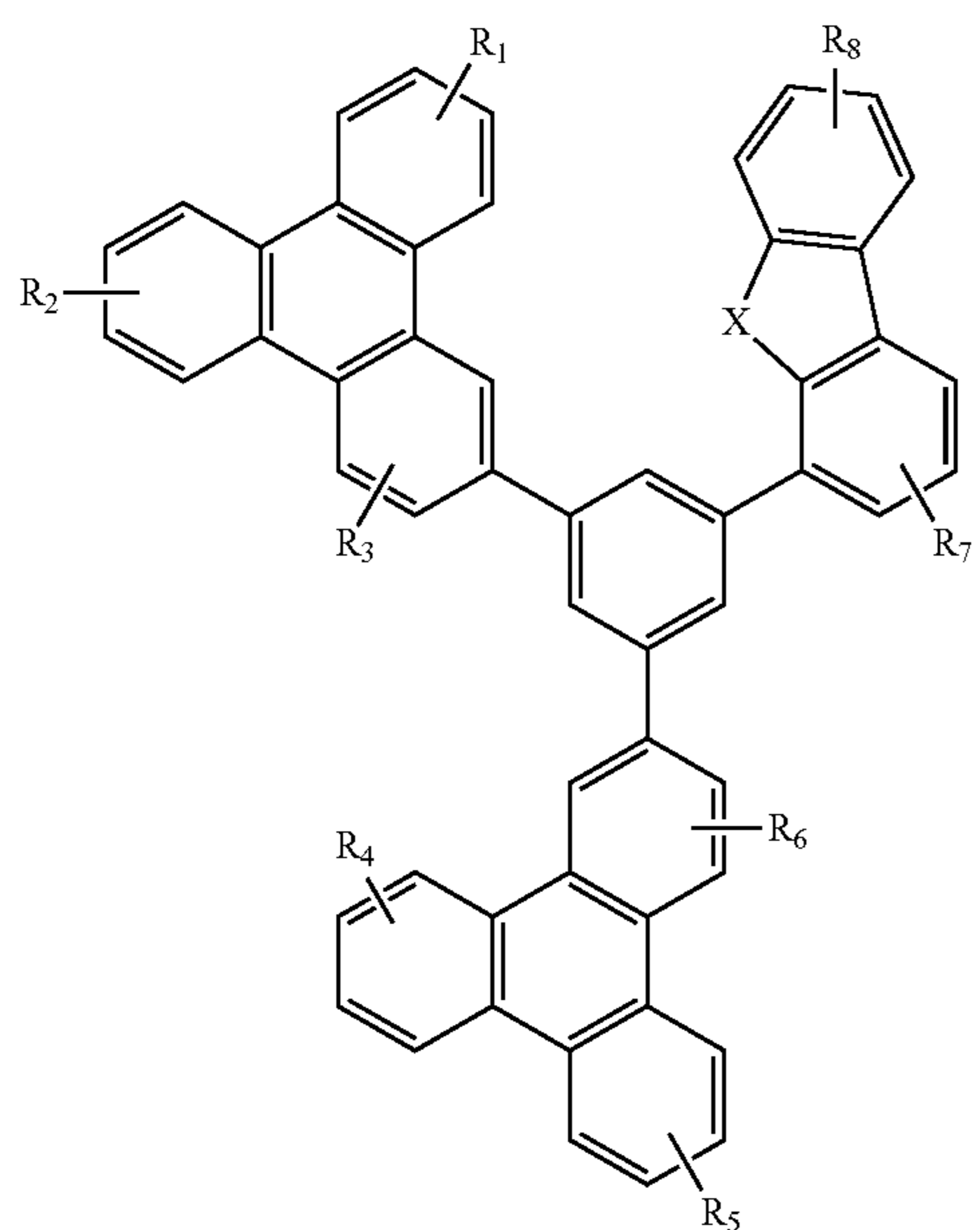
Compound 38
