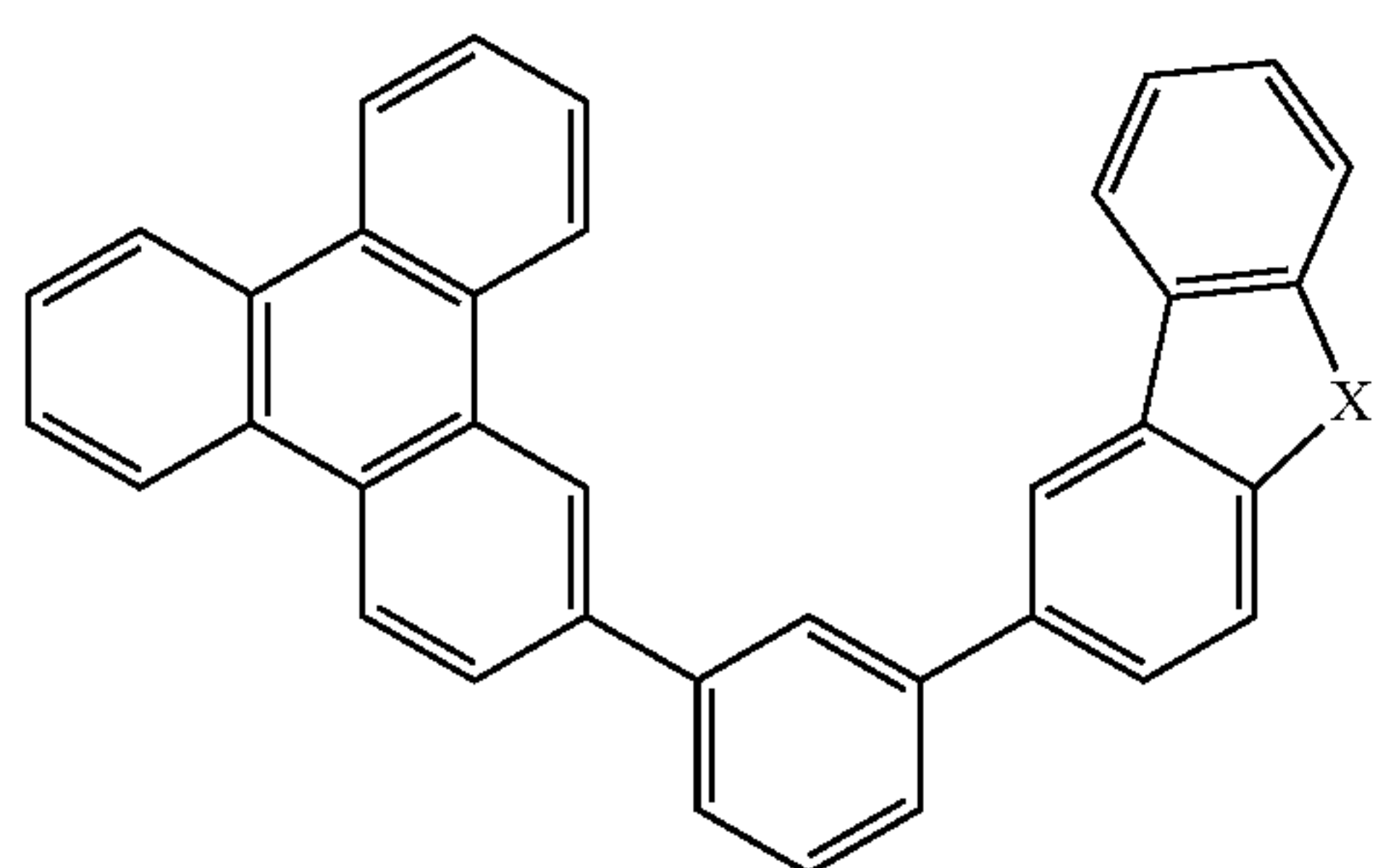
Compound 21G
