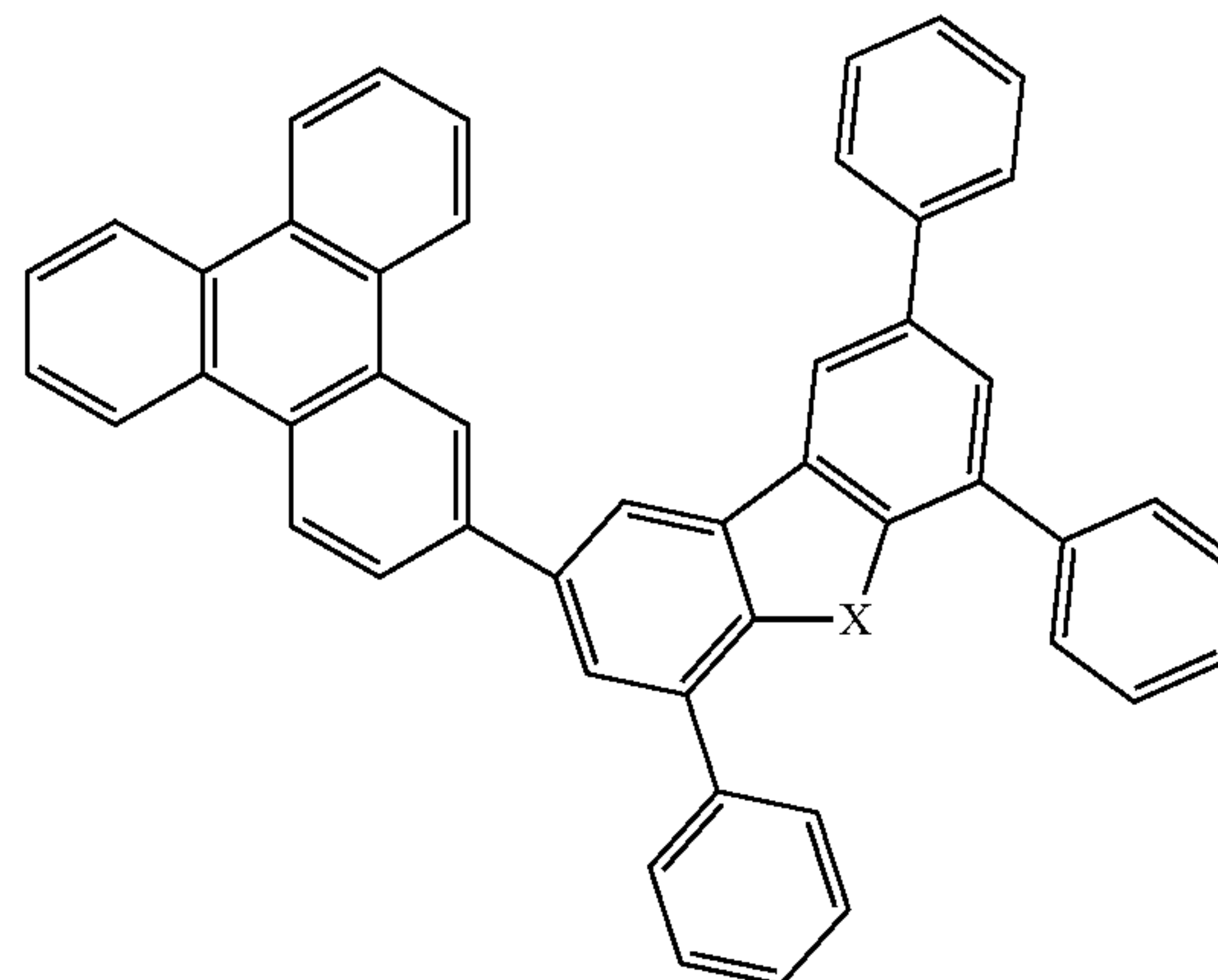
Compound 36
