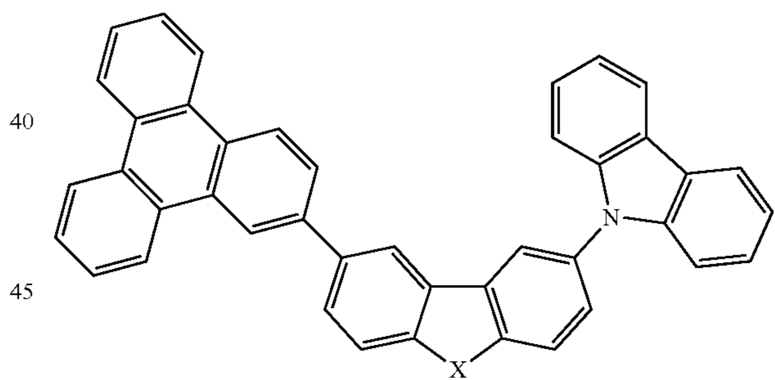
Compound 15
