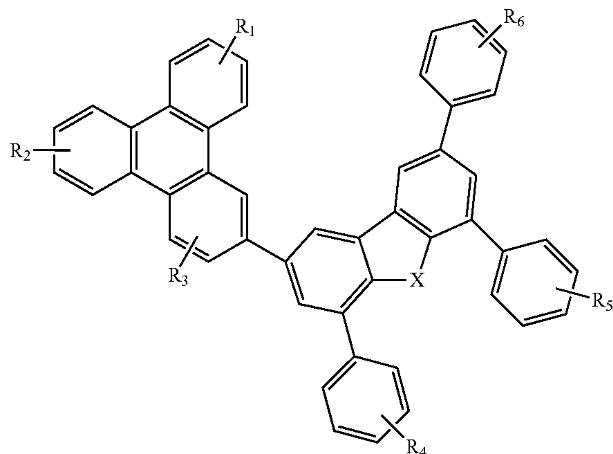
Compound 35G
