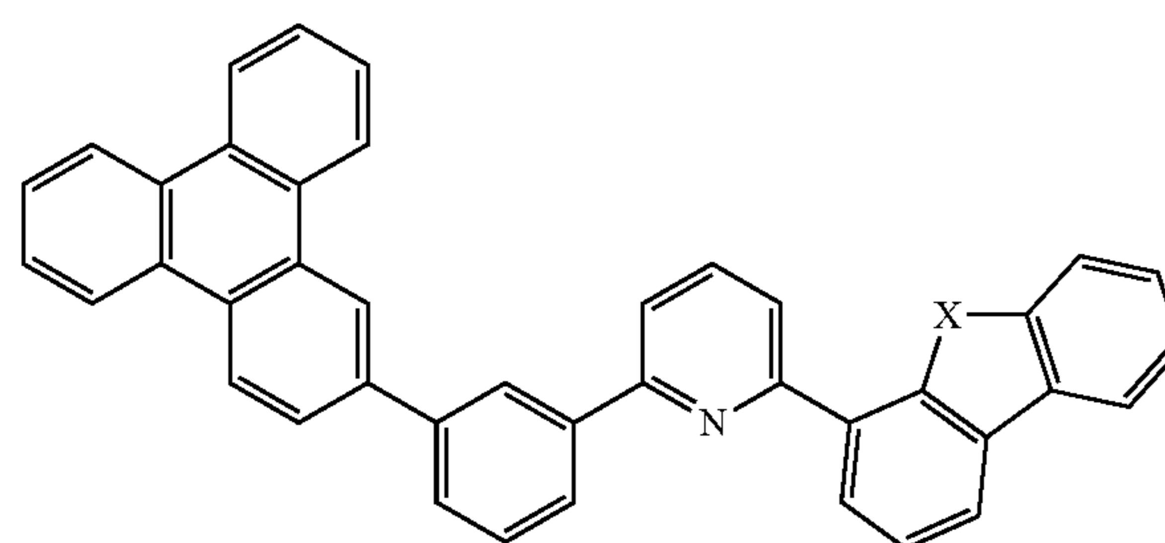
Compound 22
