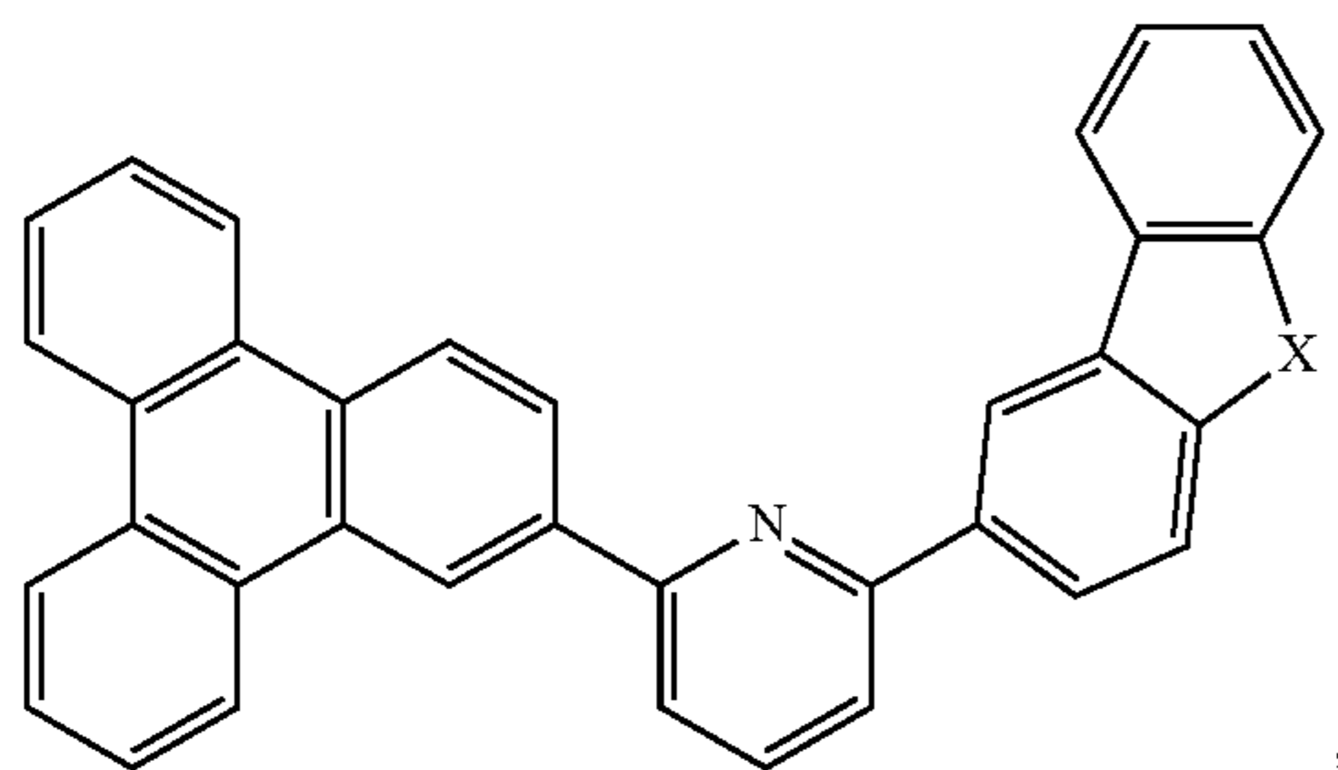
Compound 43
