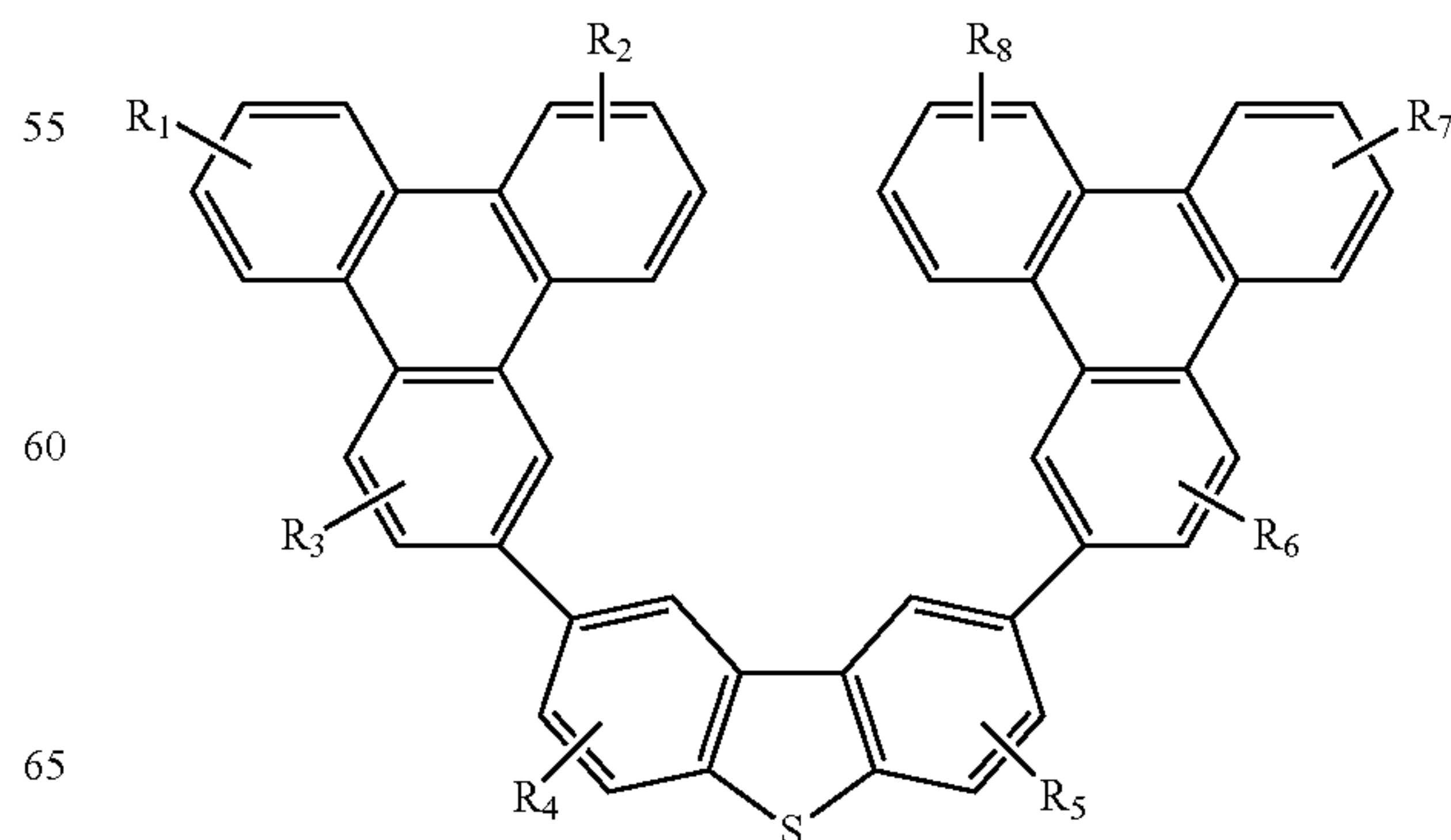
Compound 5'G
