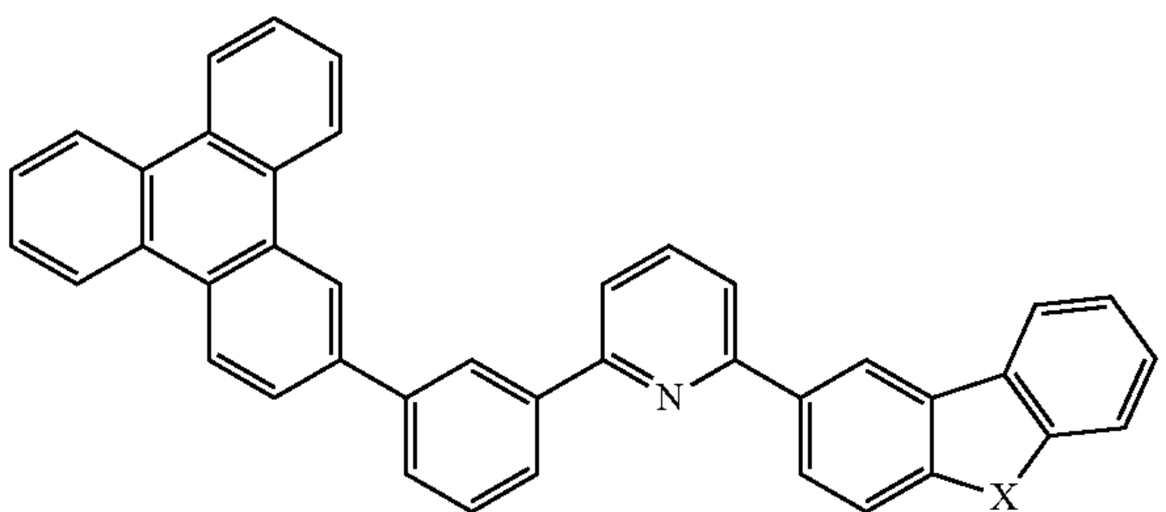
Compound 44
