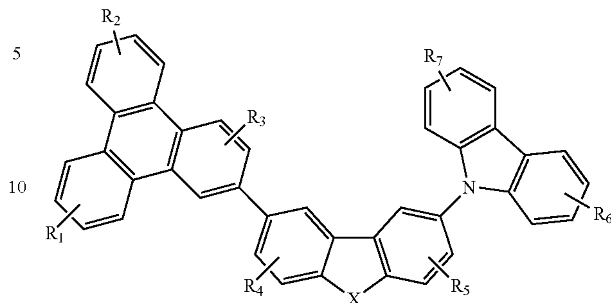
Compound 15G
