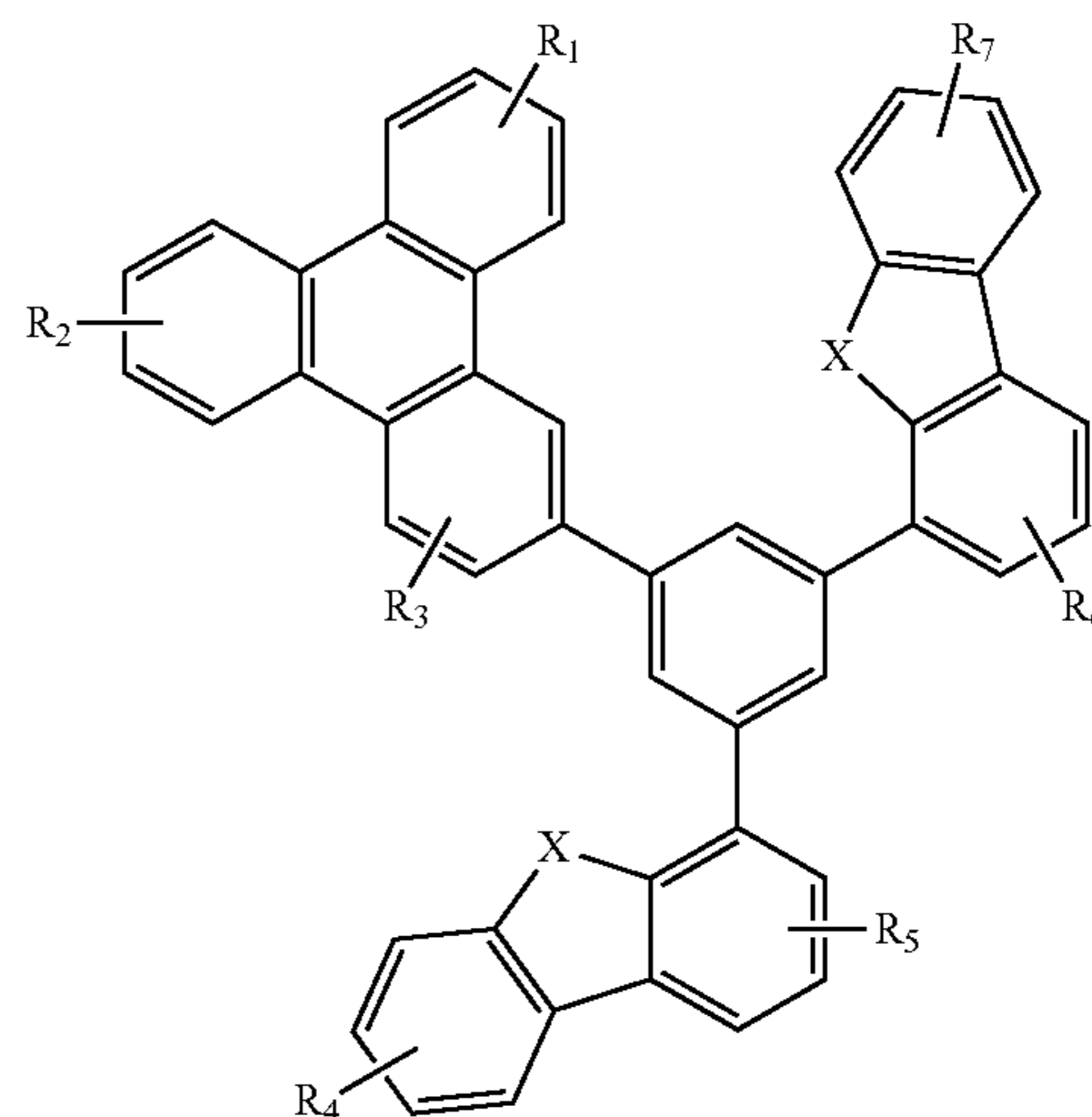
Compound 37G
