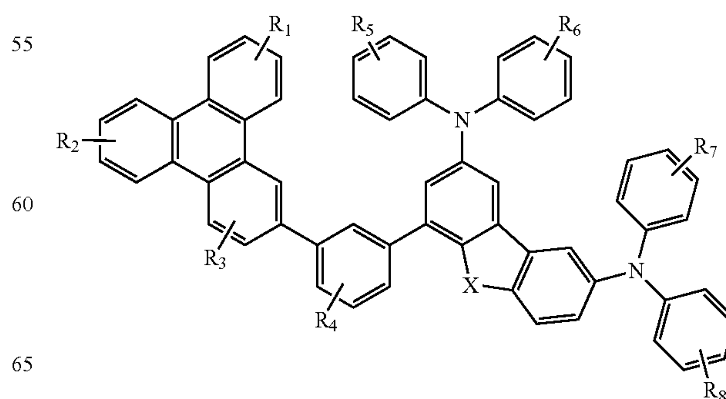
Compound 28G
