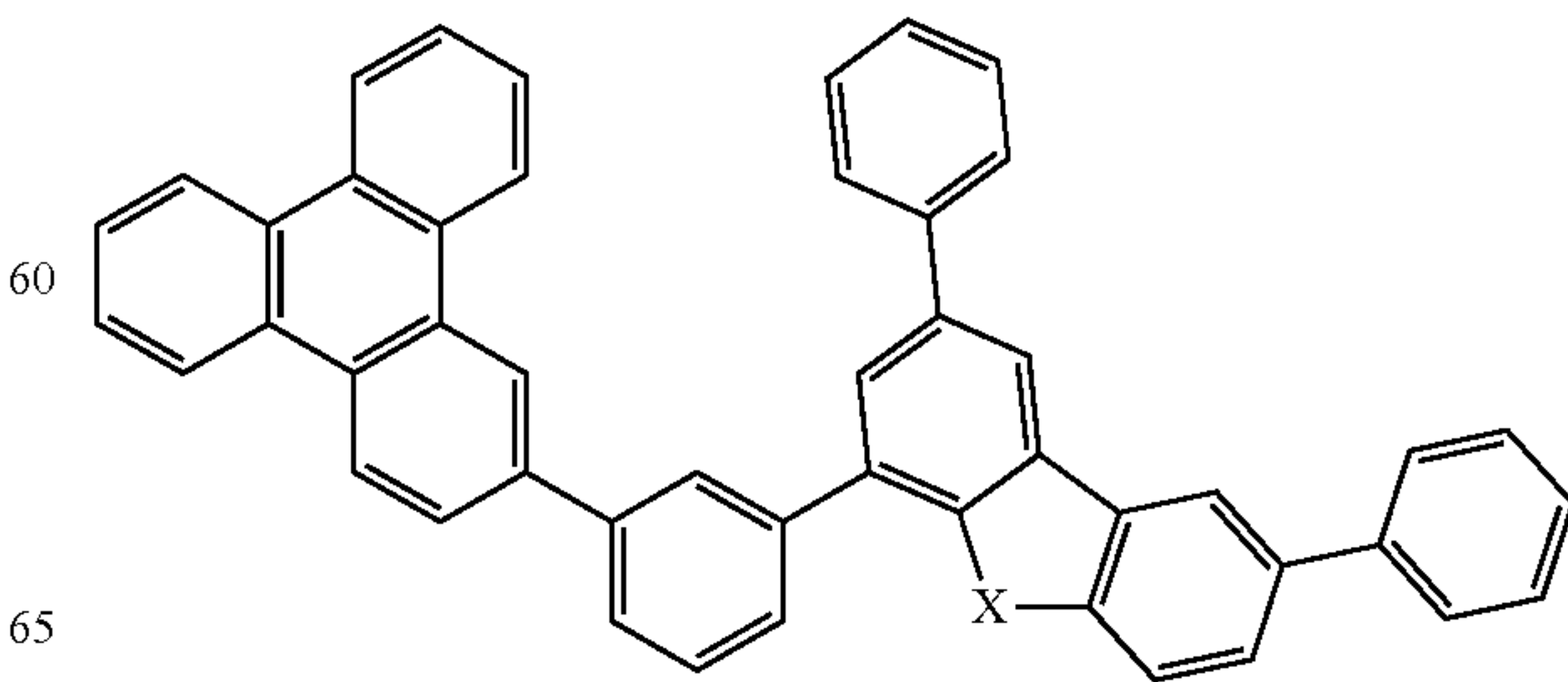
Compound 24
