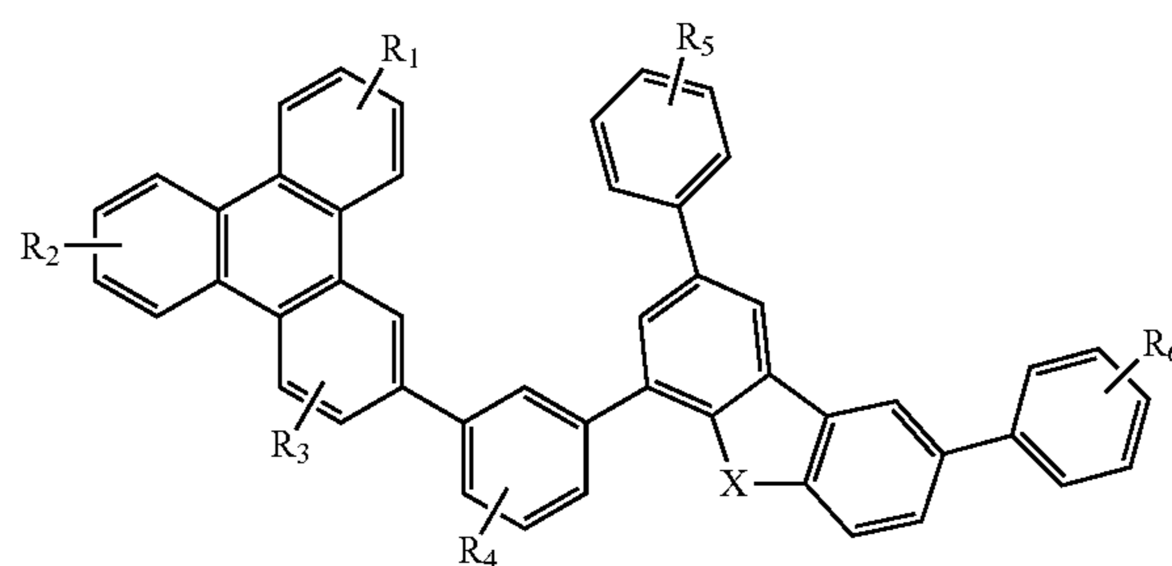
Compound 24G
