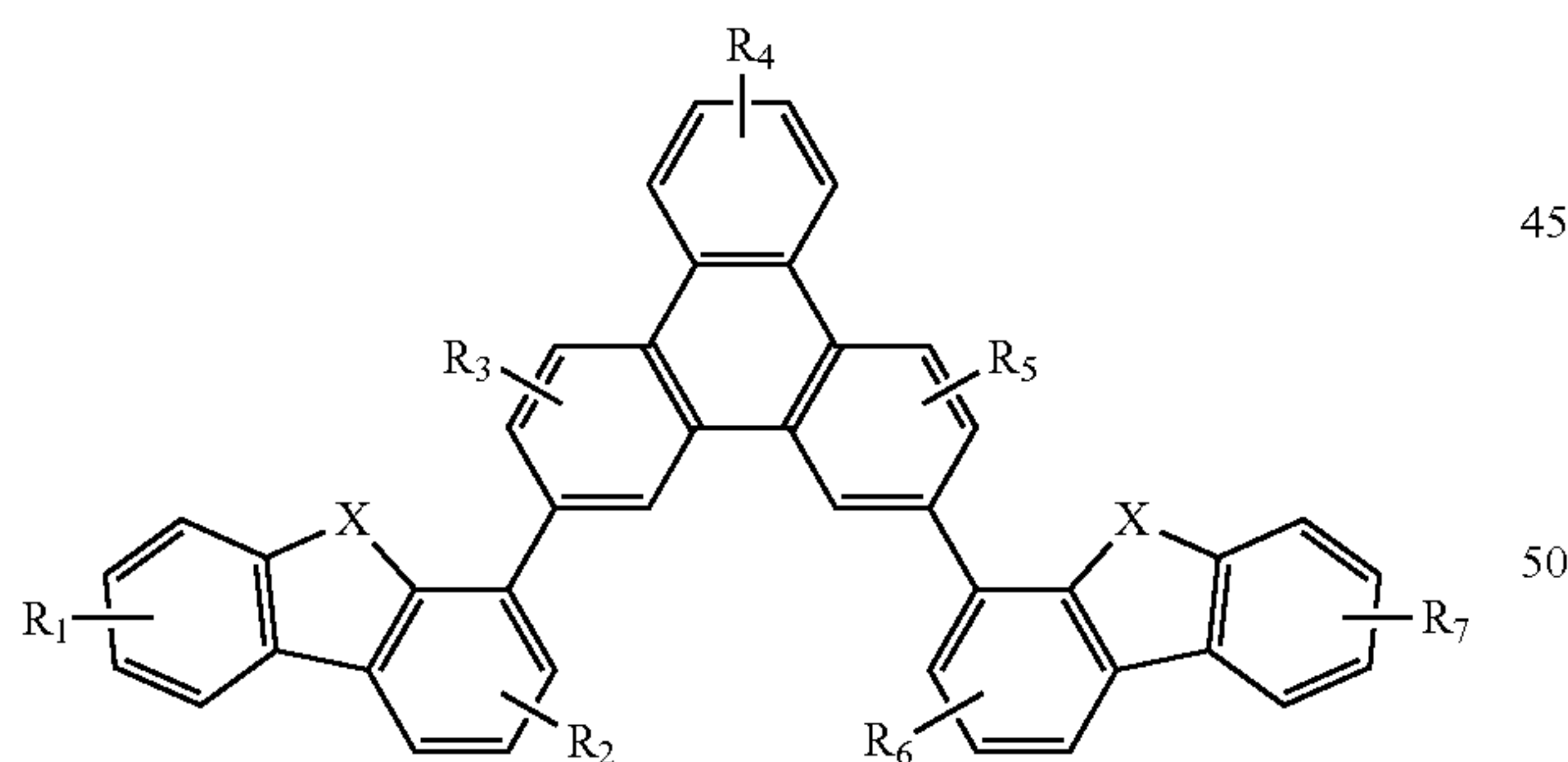
Compound 10
