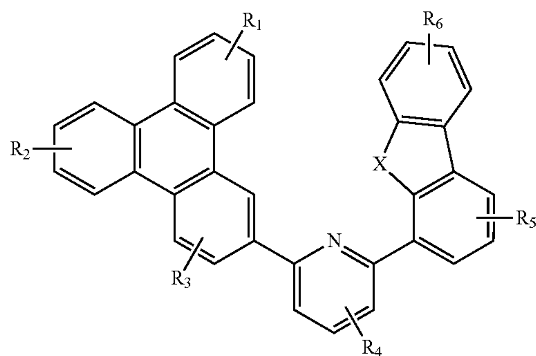
Compound 22G
