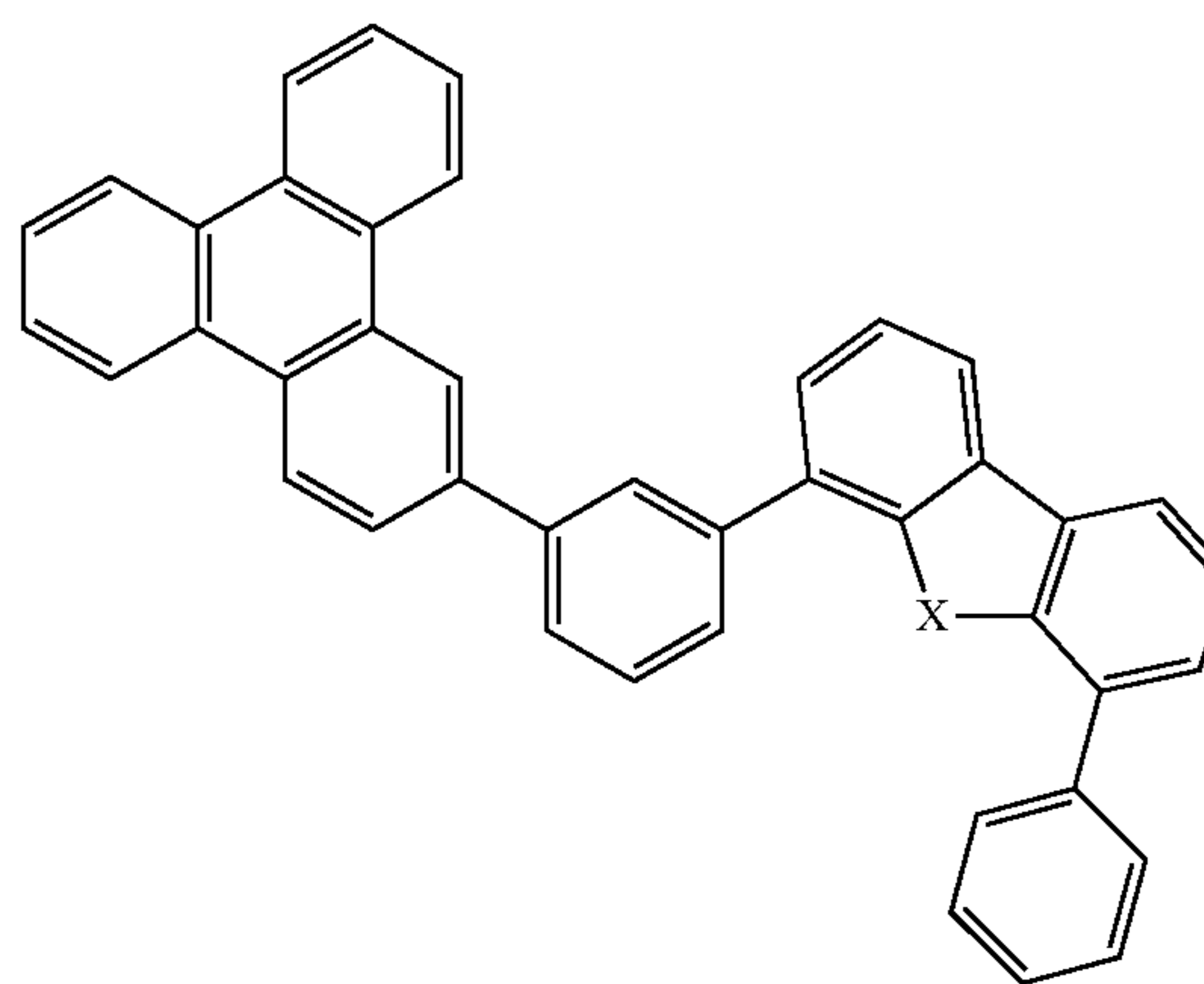
Compound 23
