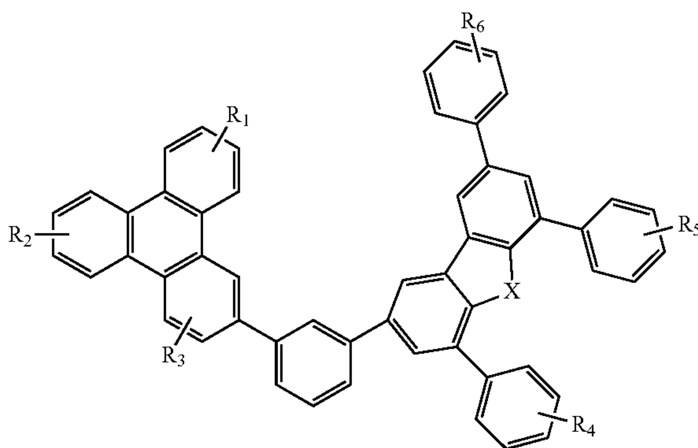
Compound 36G
