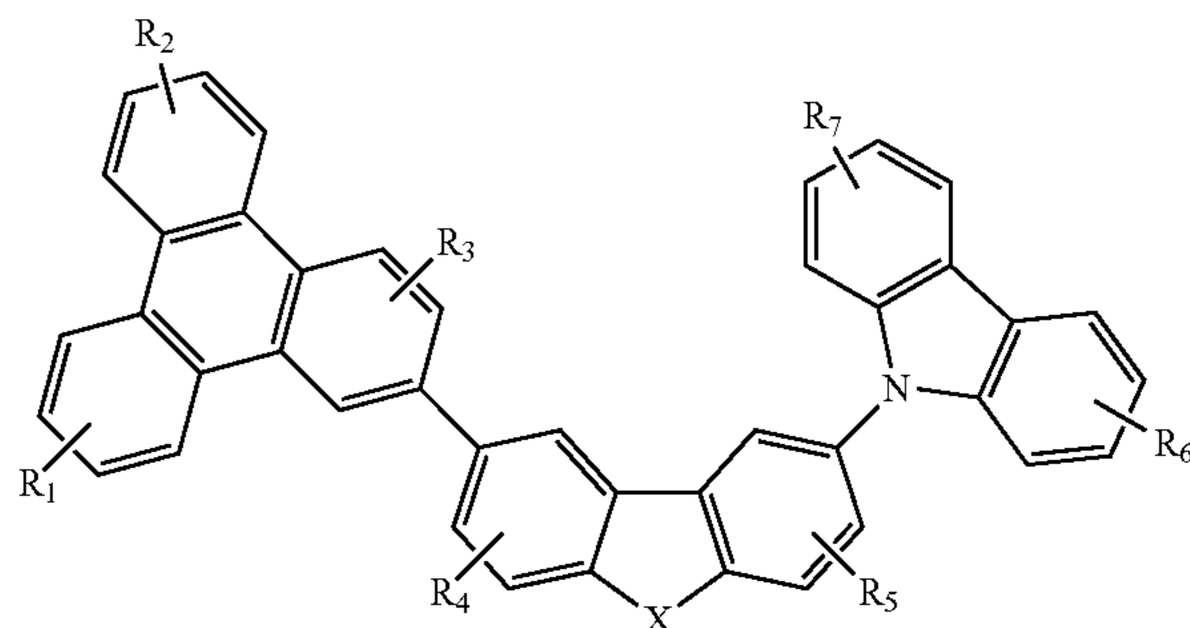
Compound 15G
