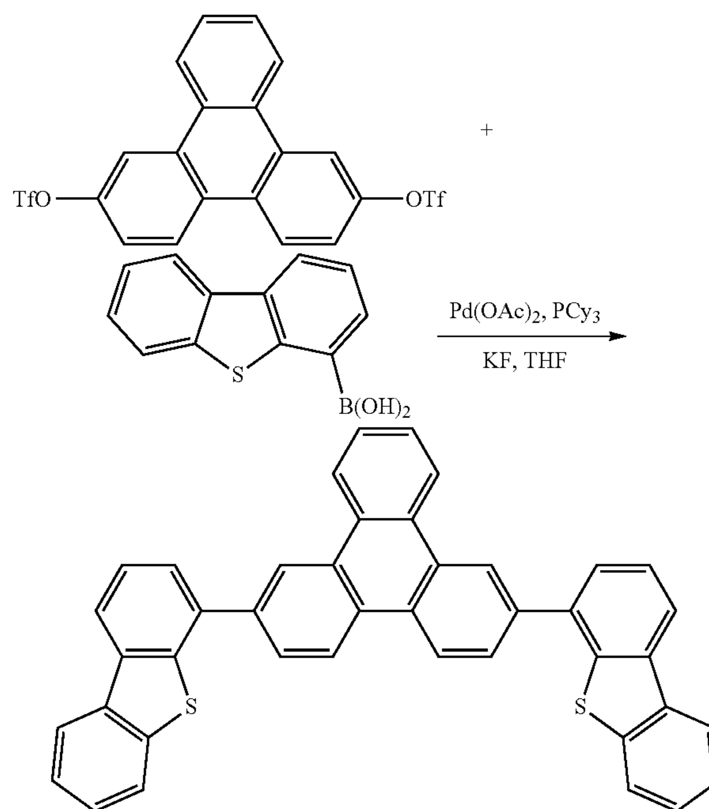
Compound 19S
