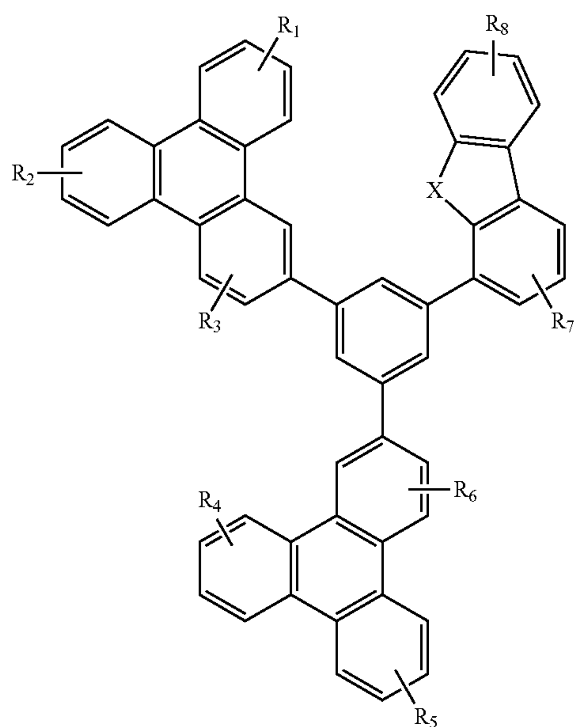
Compound 38
