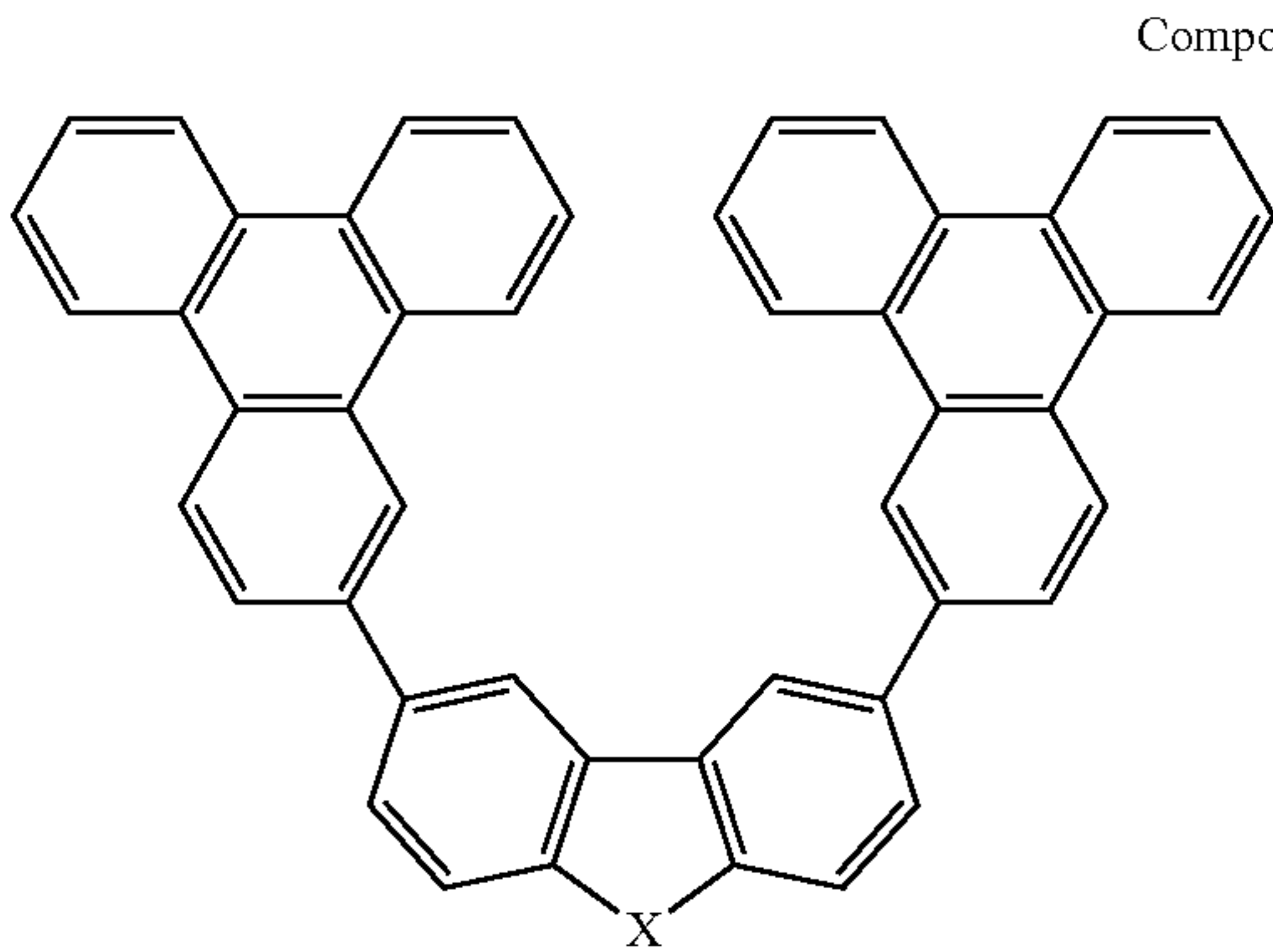
Compound 6
