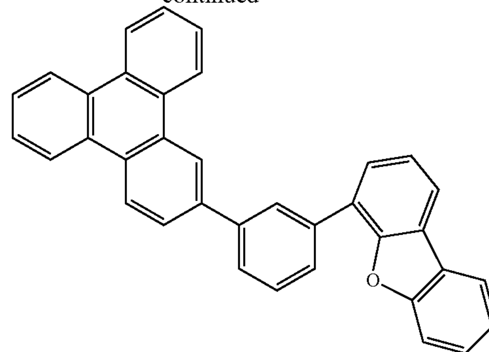
Compound 20
