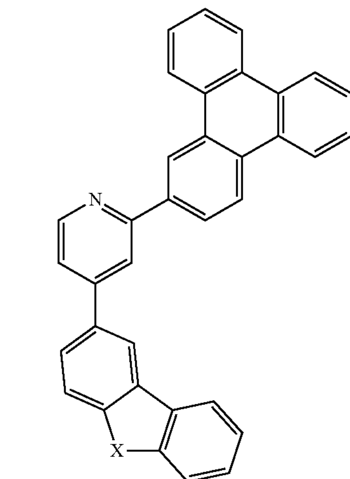
Compound 45
