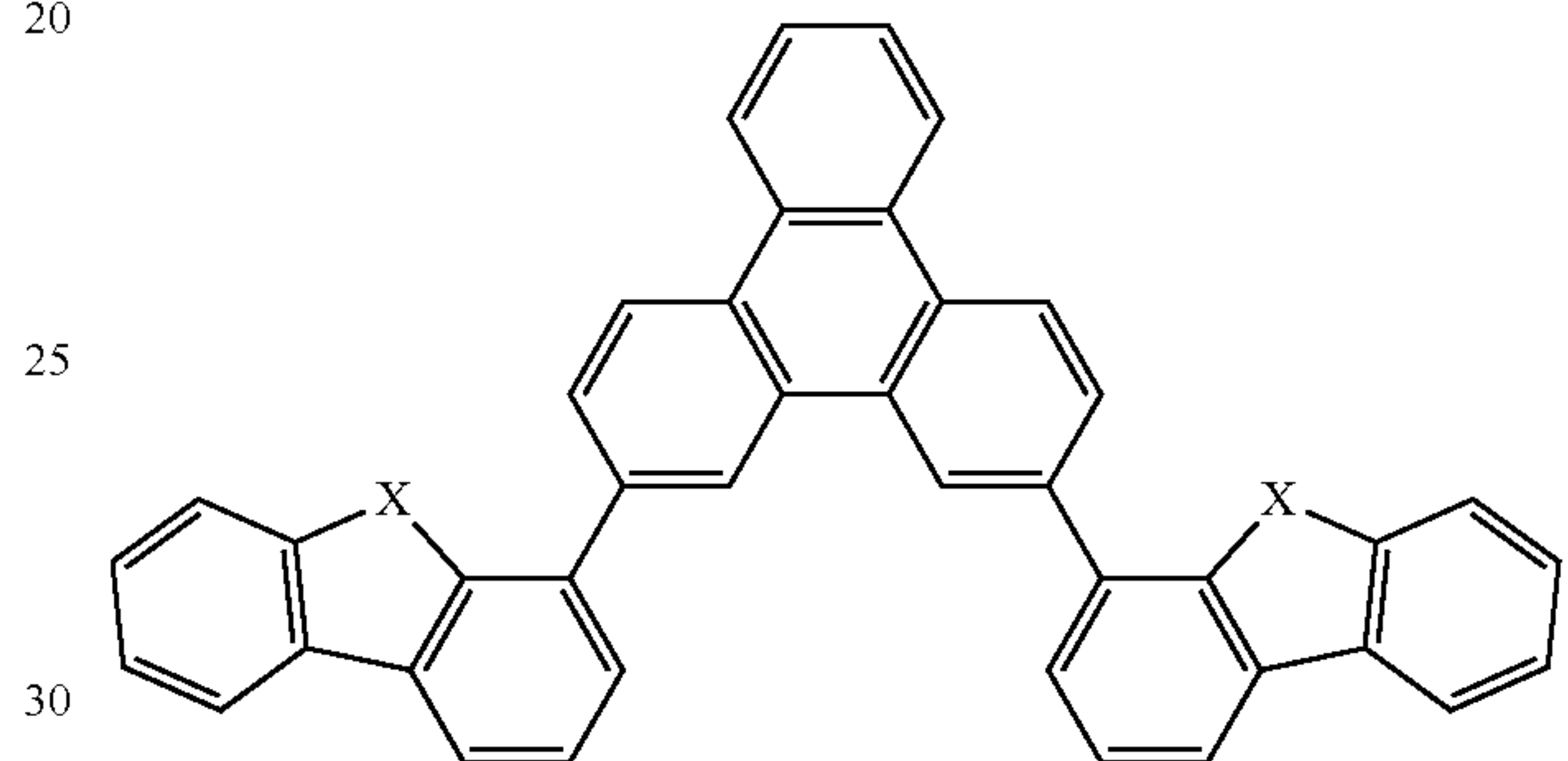
Compound 10
