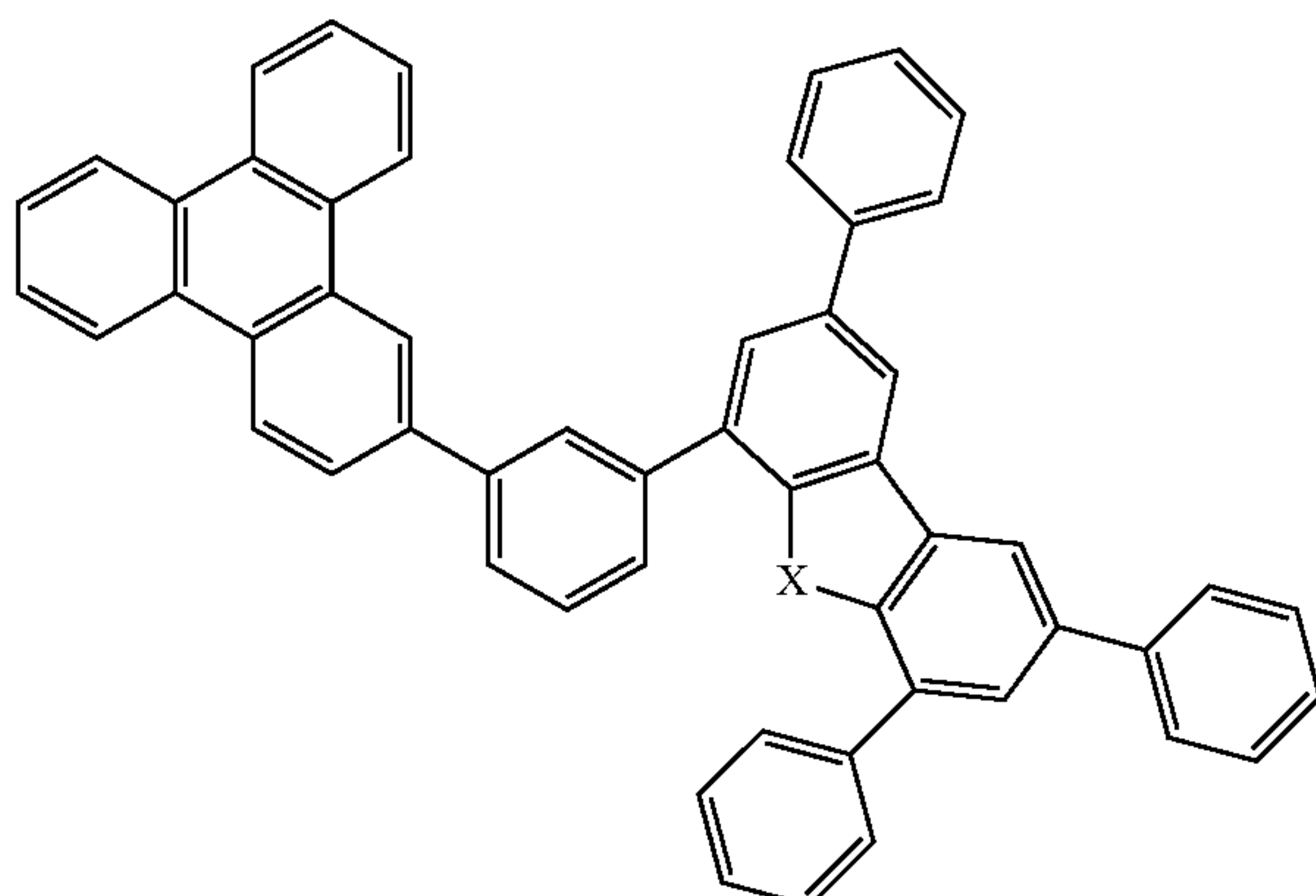
Compound 25
