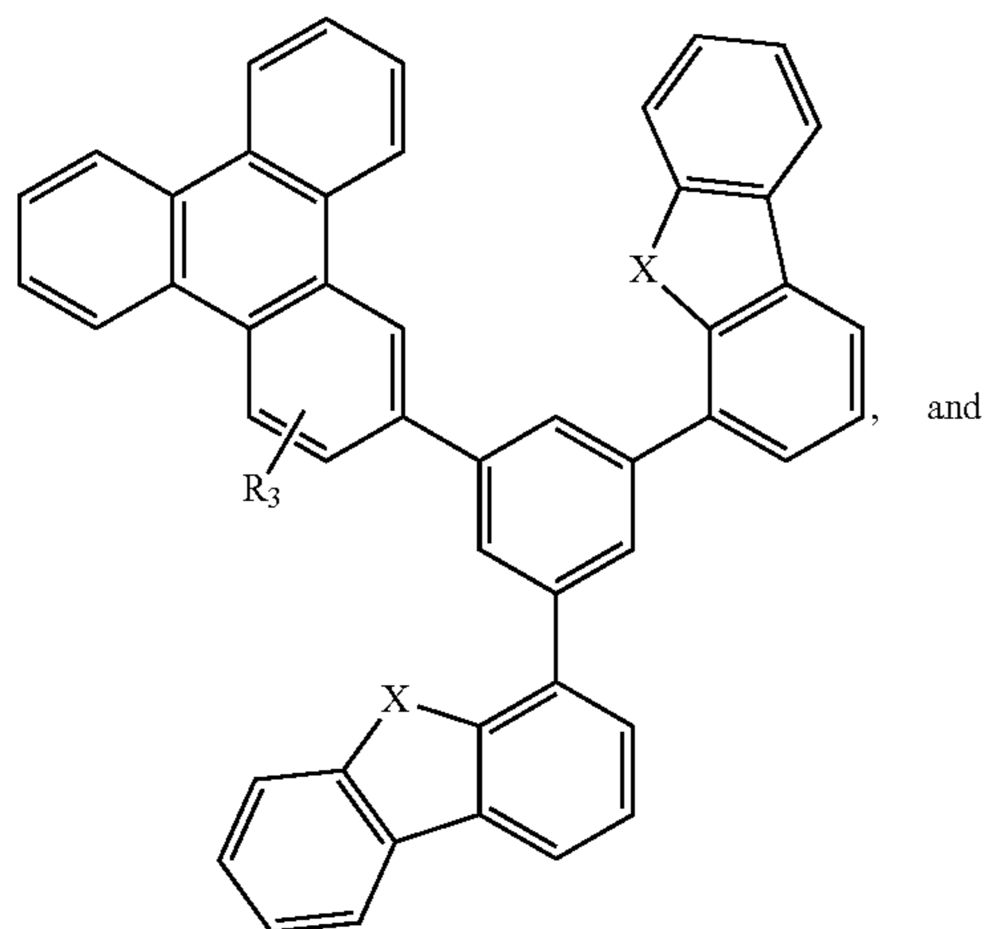
Compound 37
