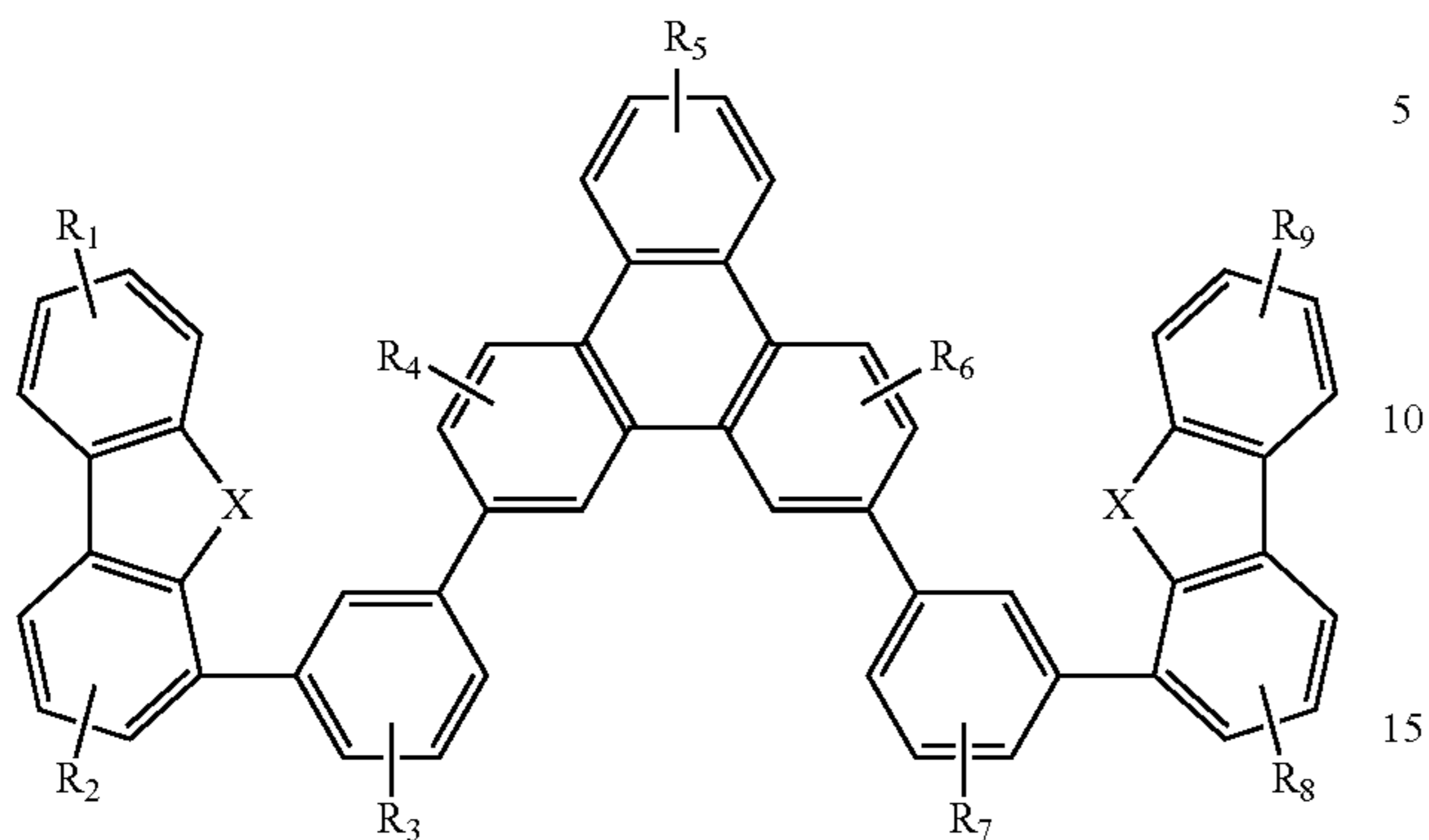
Compound 4G
