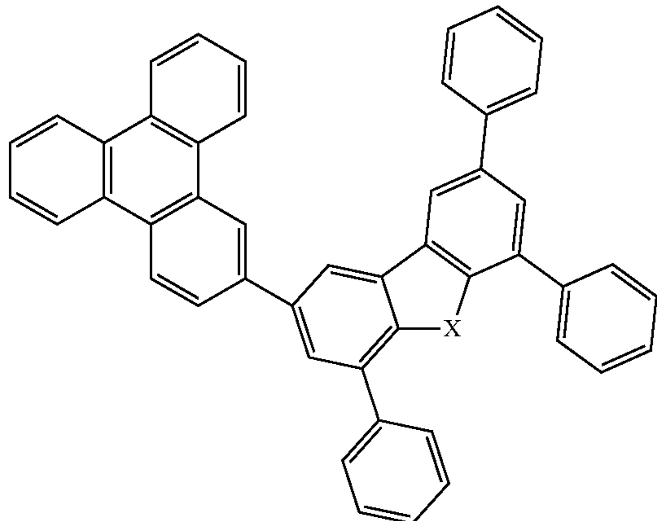
Compound 36
