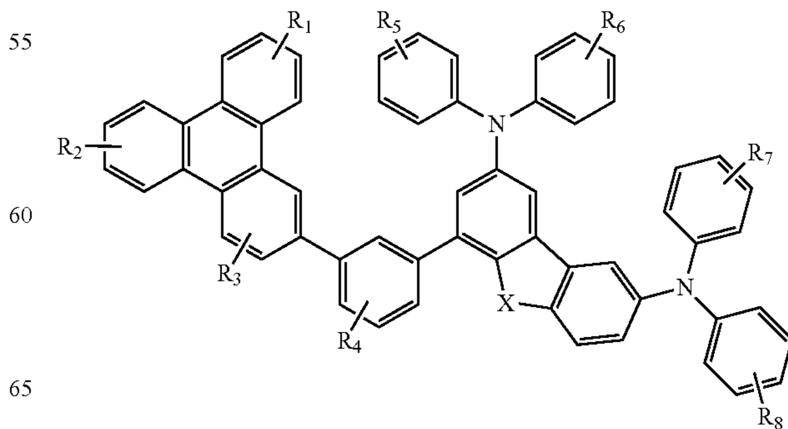
Compound 28G
