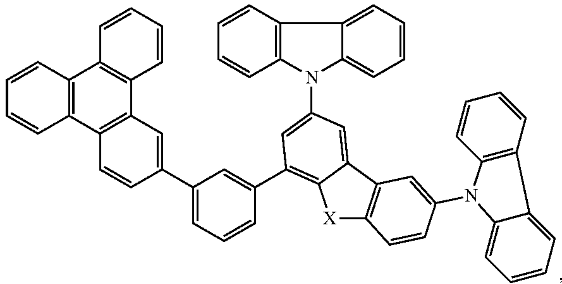
Compound 27
