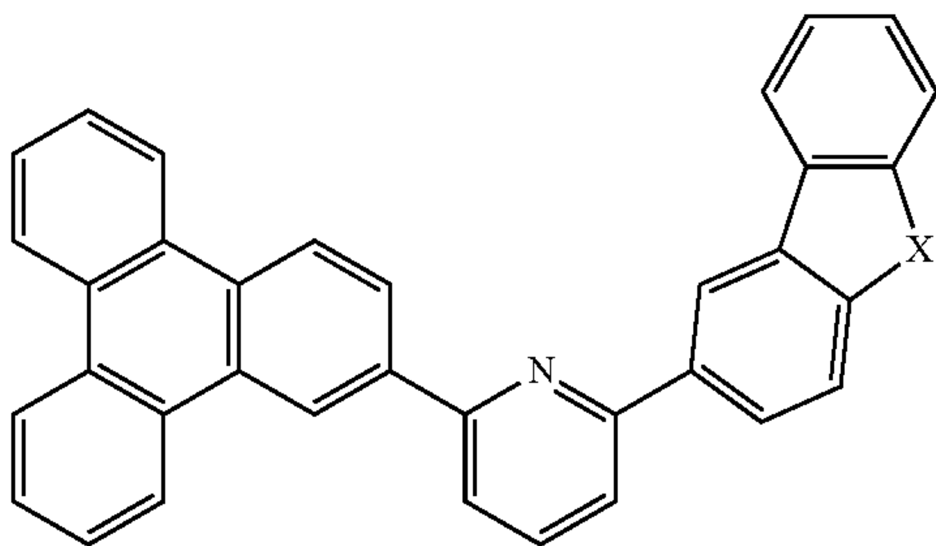
Compound 43
