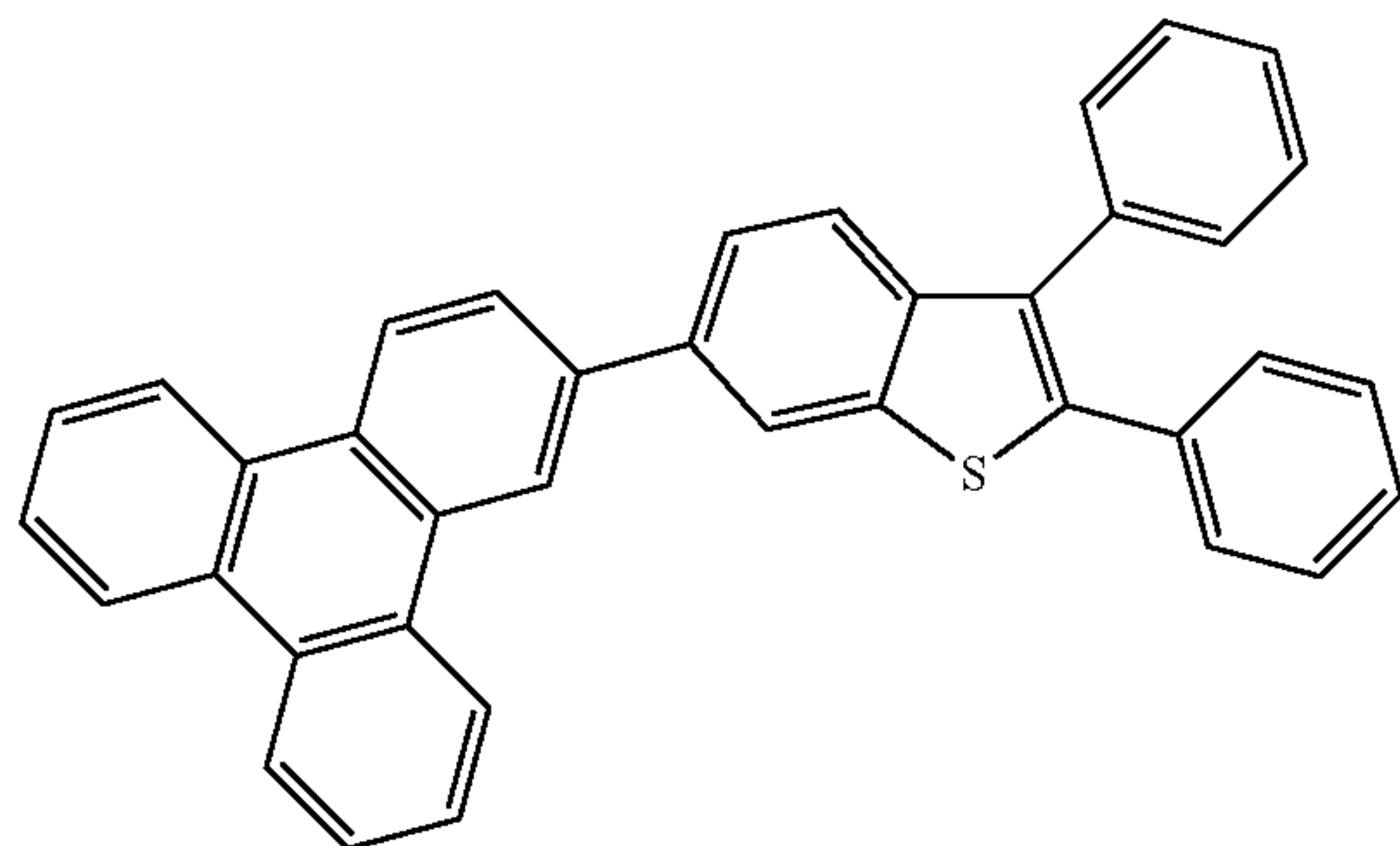
Compound 18'G
