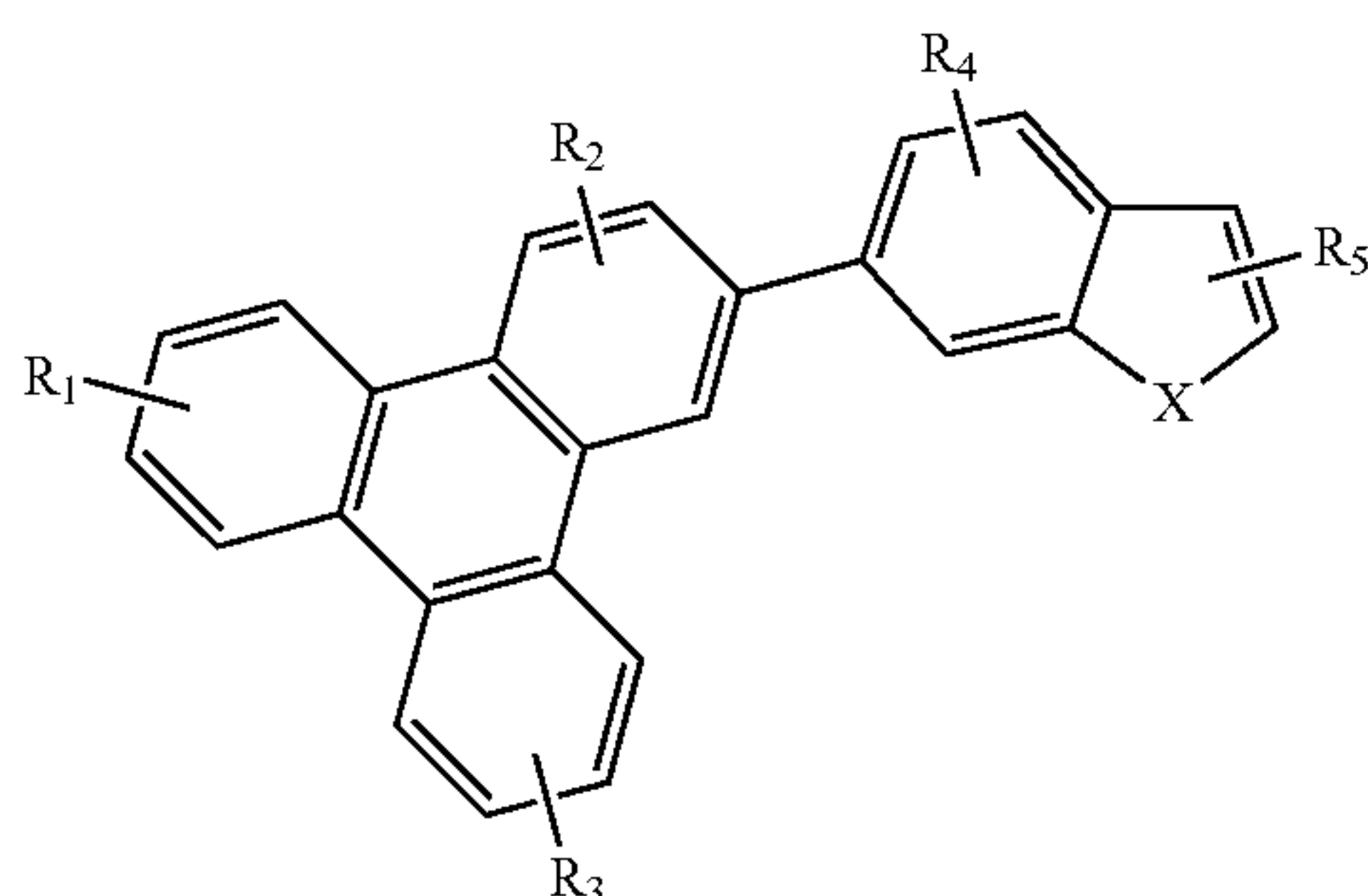
Compound 17G
