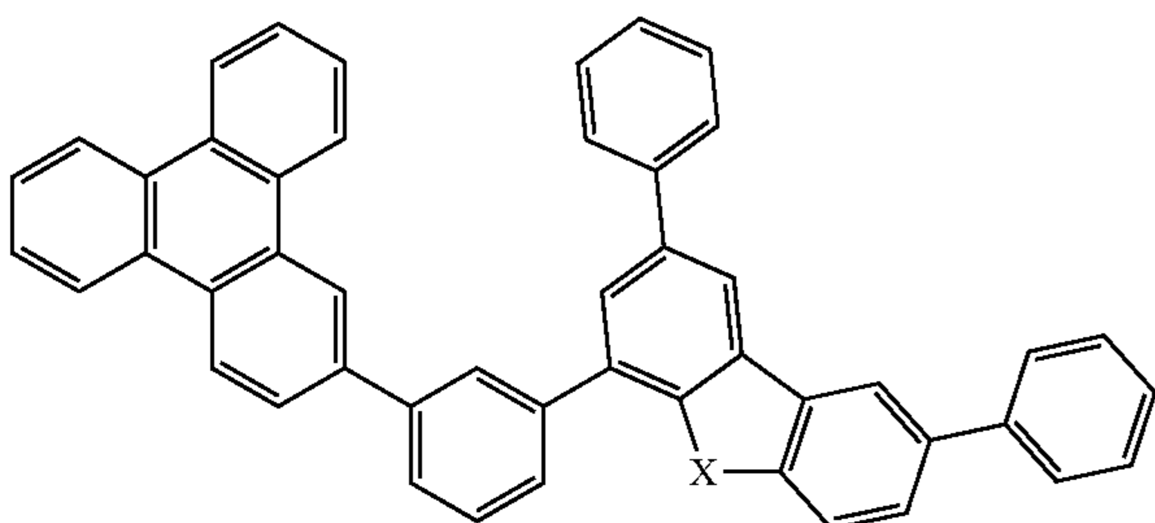
Compound 24
