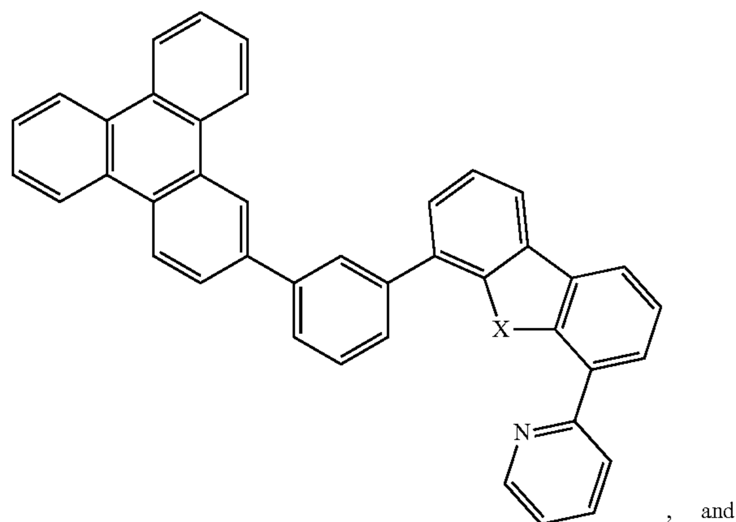
Compound 47
