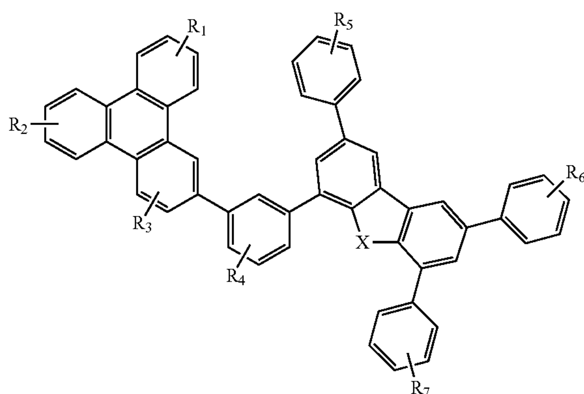
Compound 25G
