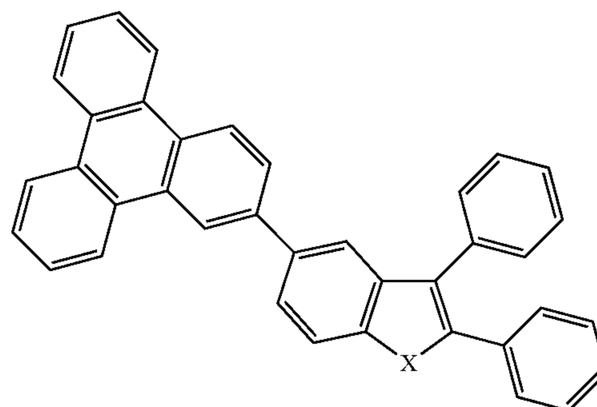
Compound 13
