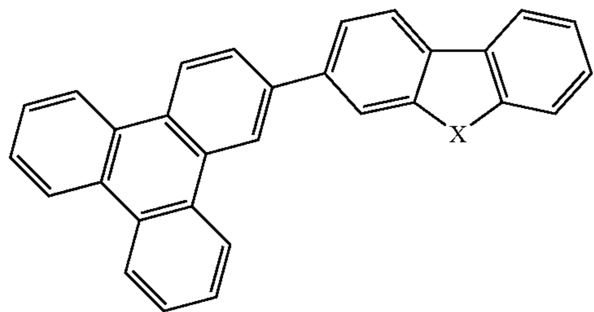
Compound 8
