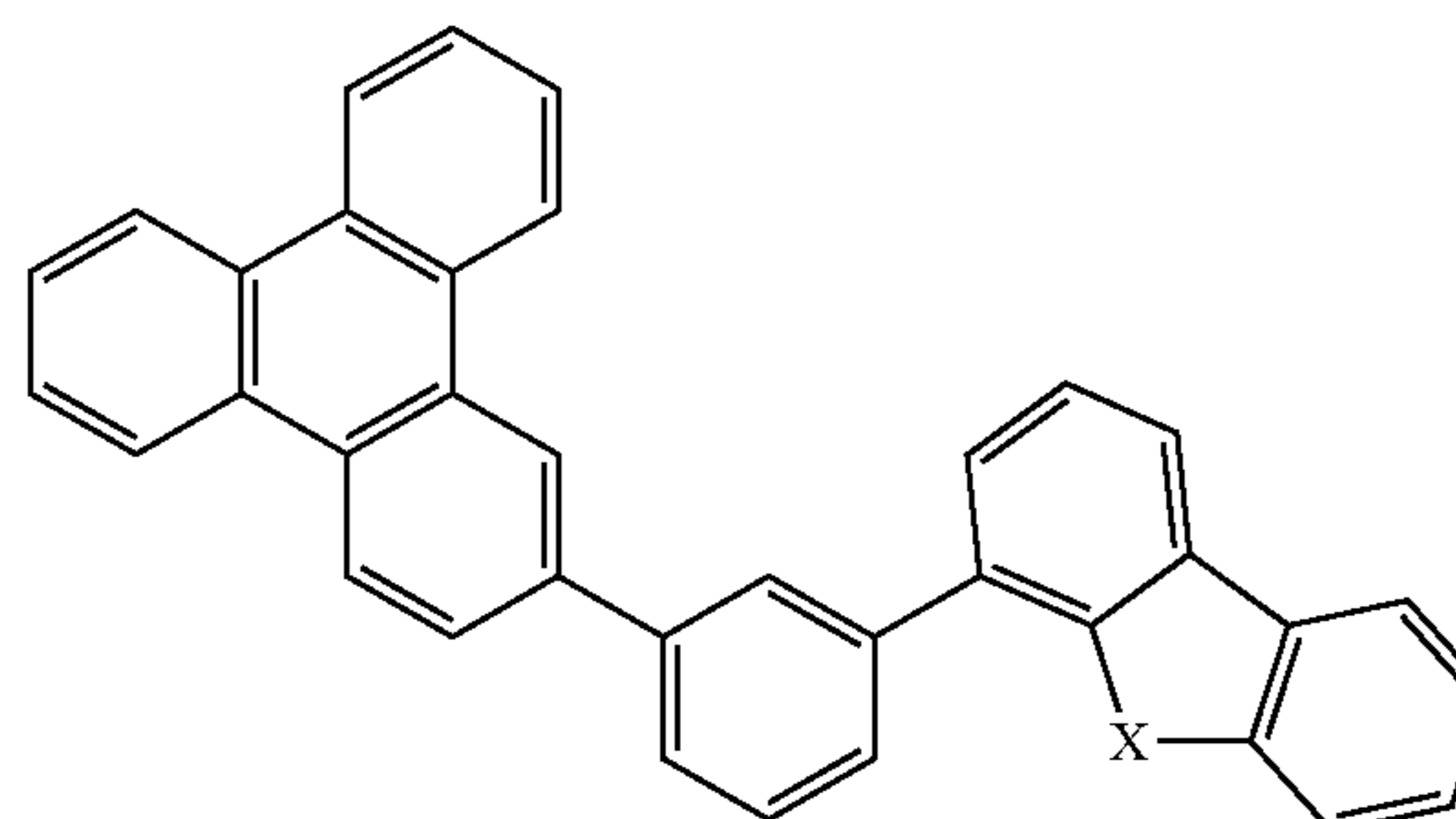
Compound 47
