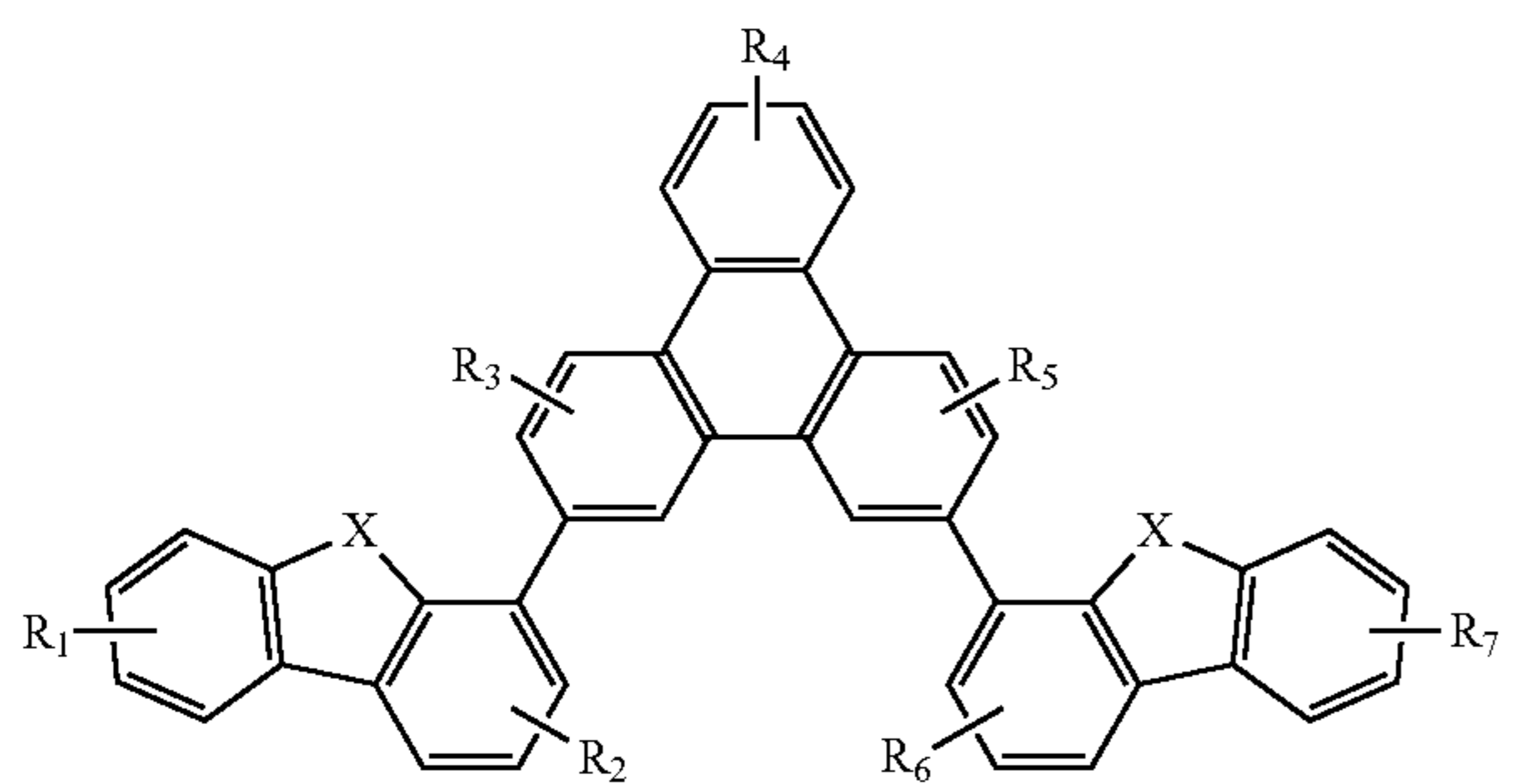
Compound 10
