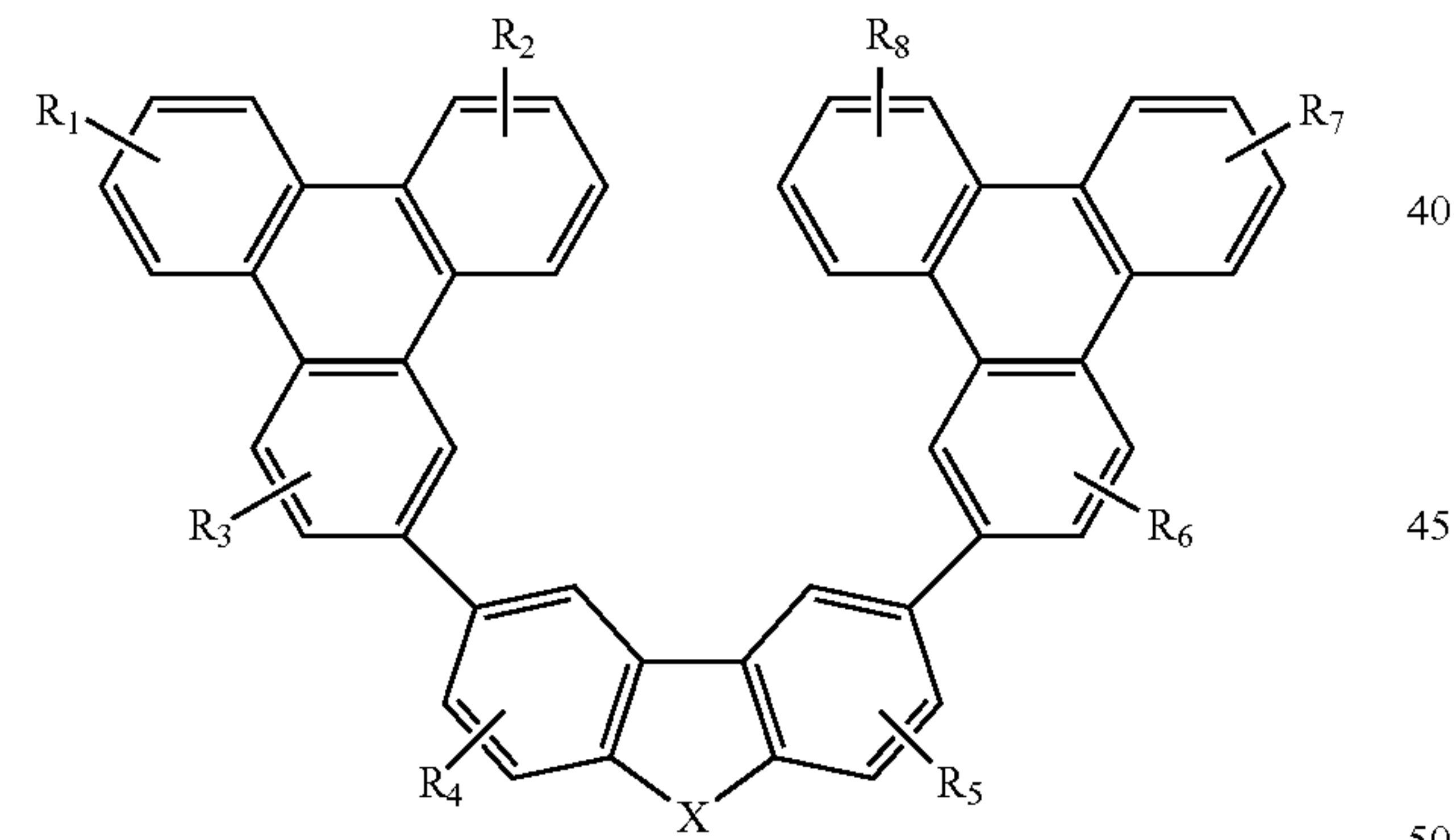
Compound 5G
