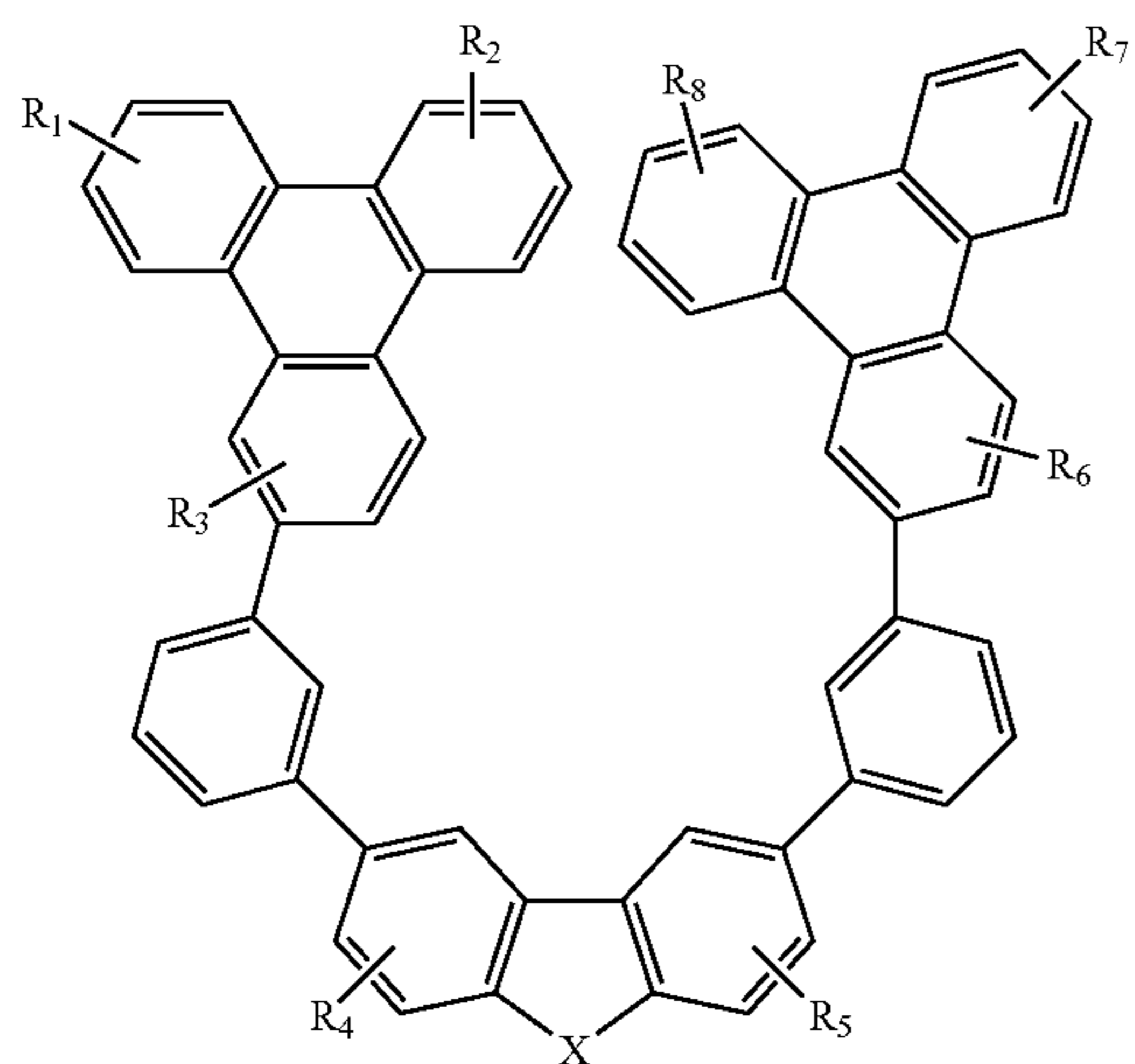
Compound 39G
