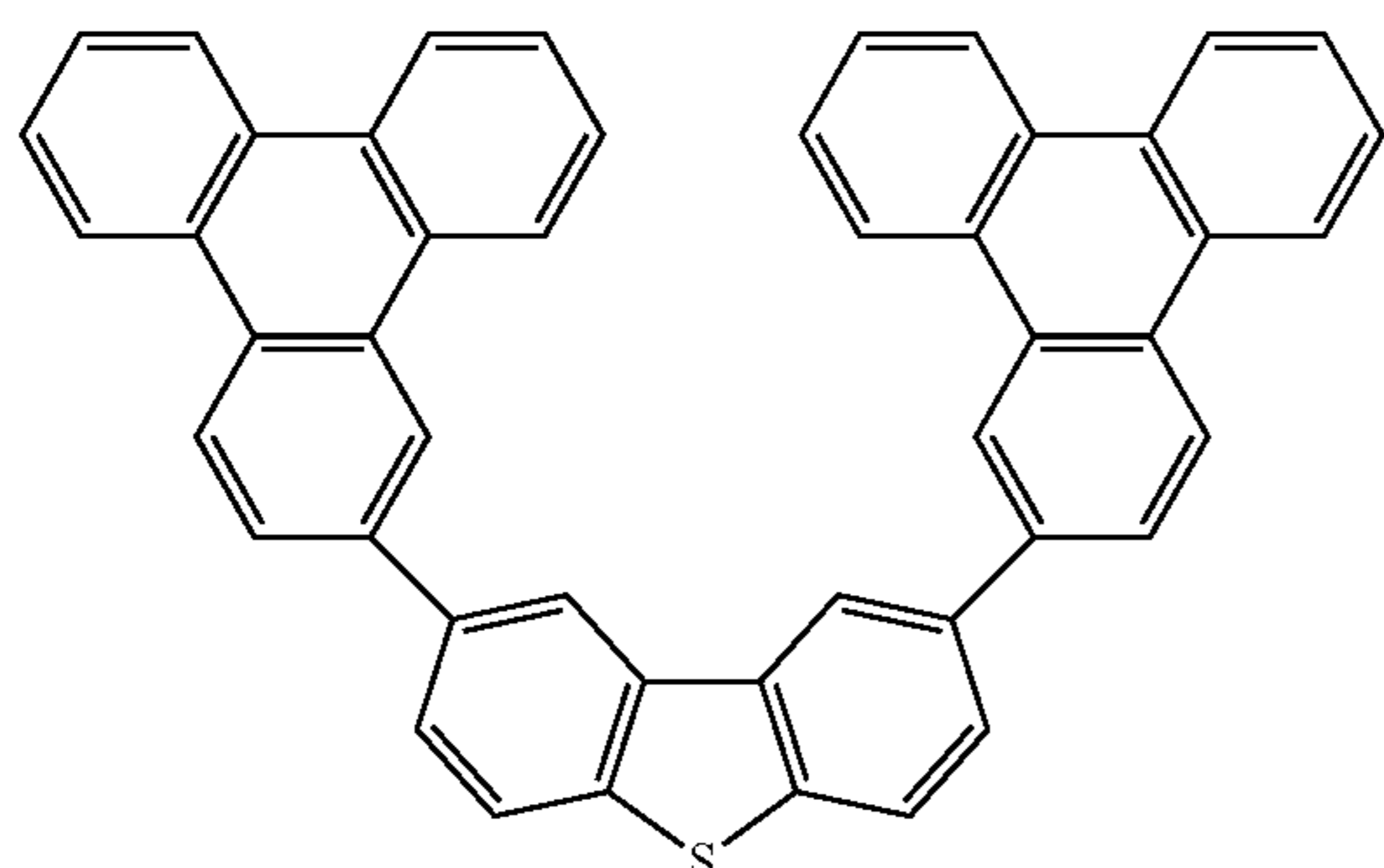
Compound 6'G
