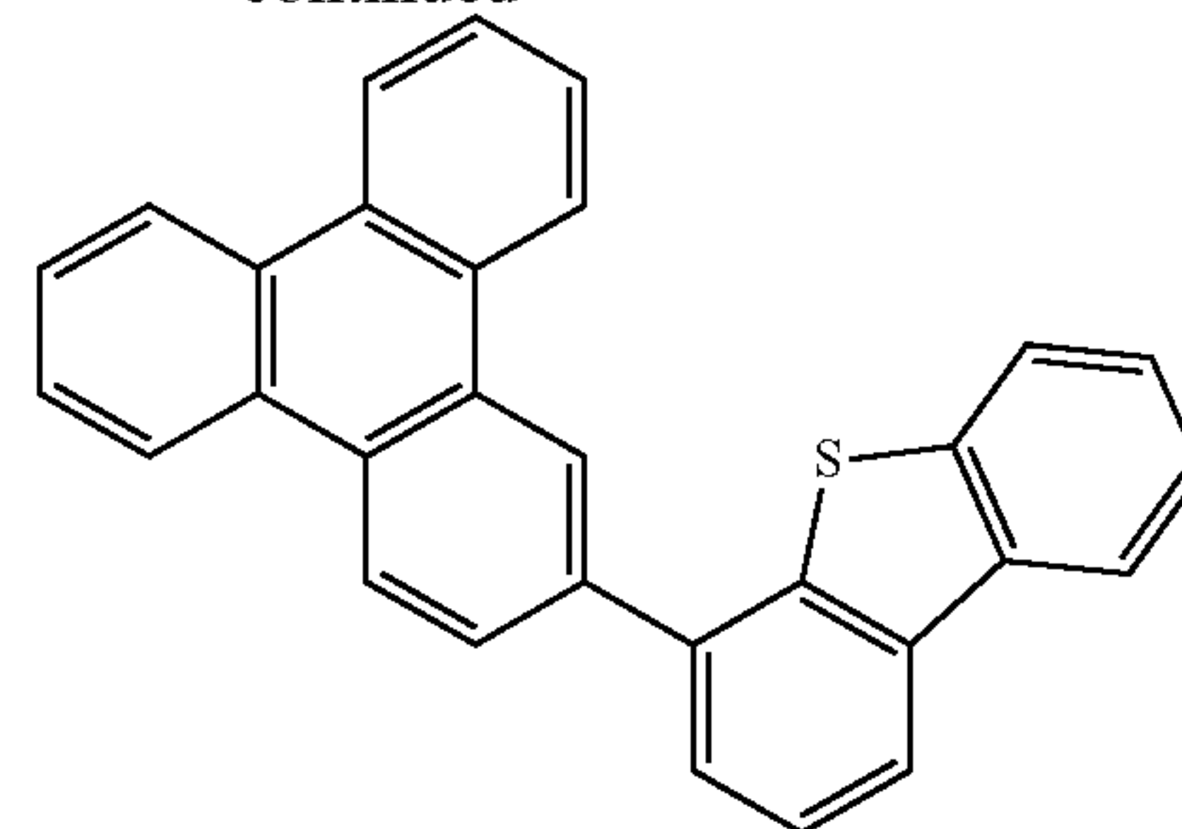
Compound 1S
