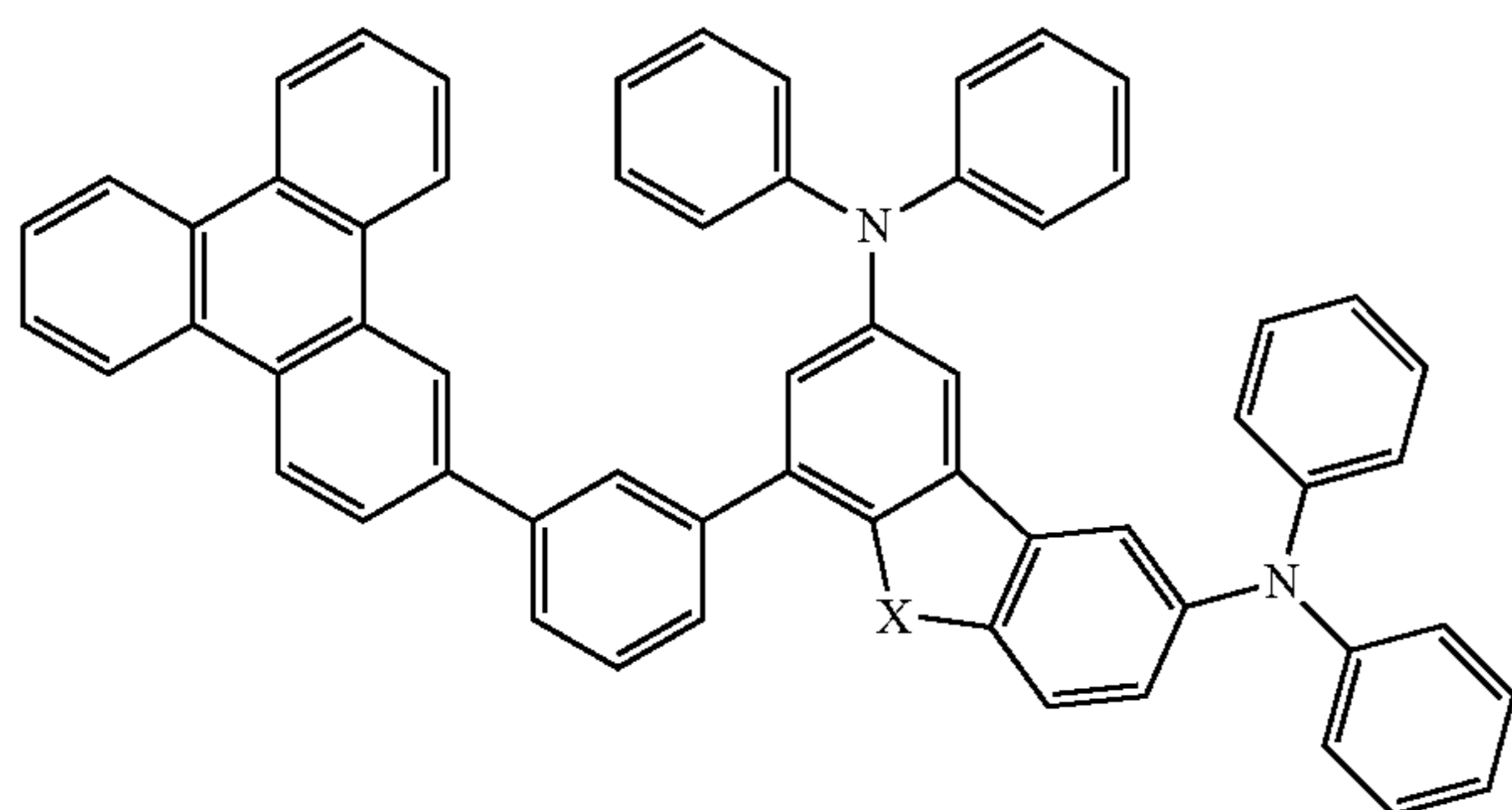
Compound 28
