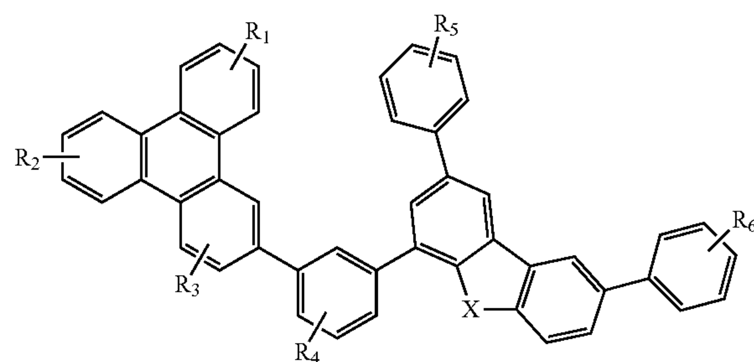
Compound 24G
