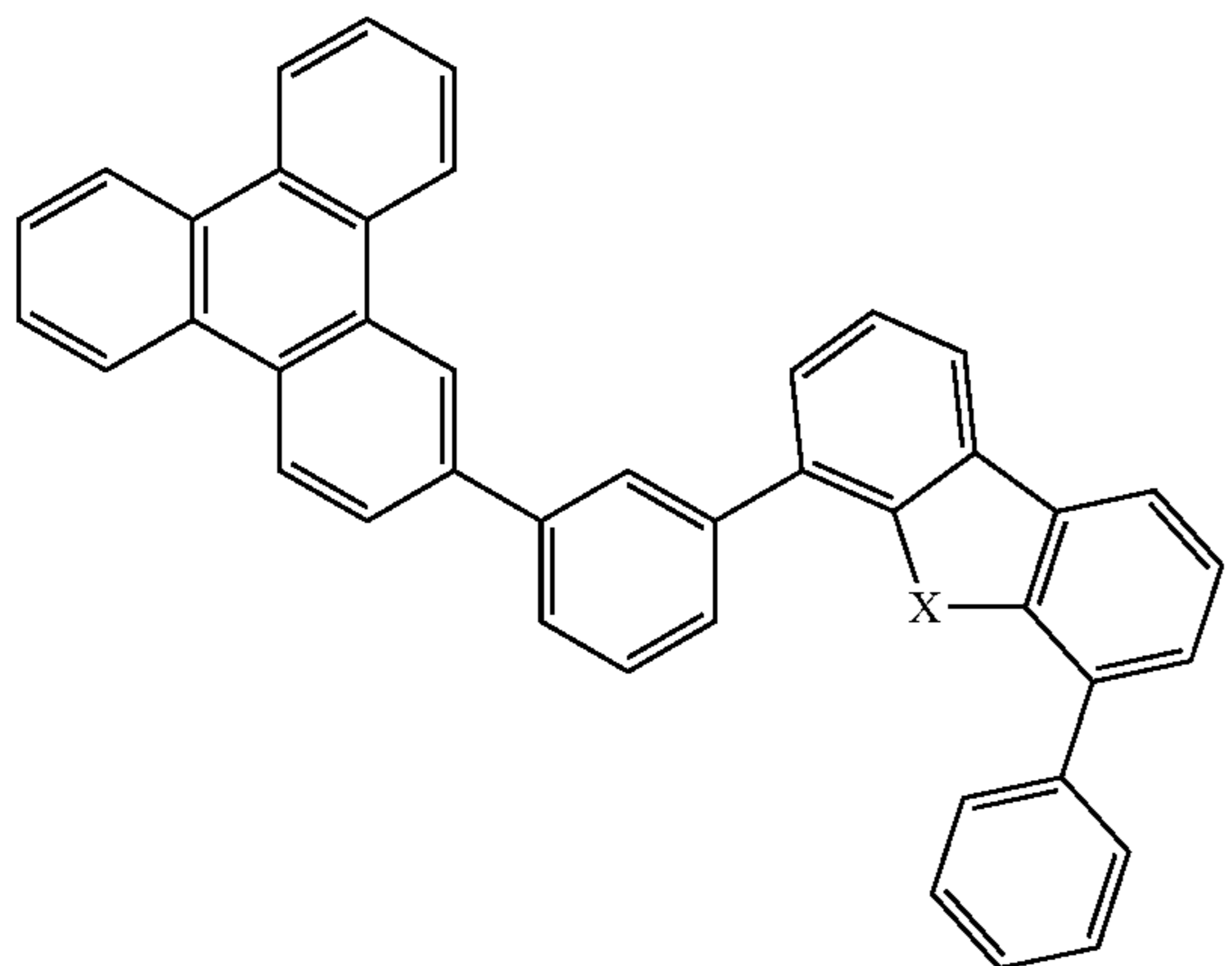
Compound 23
