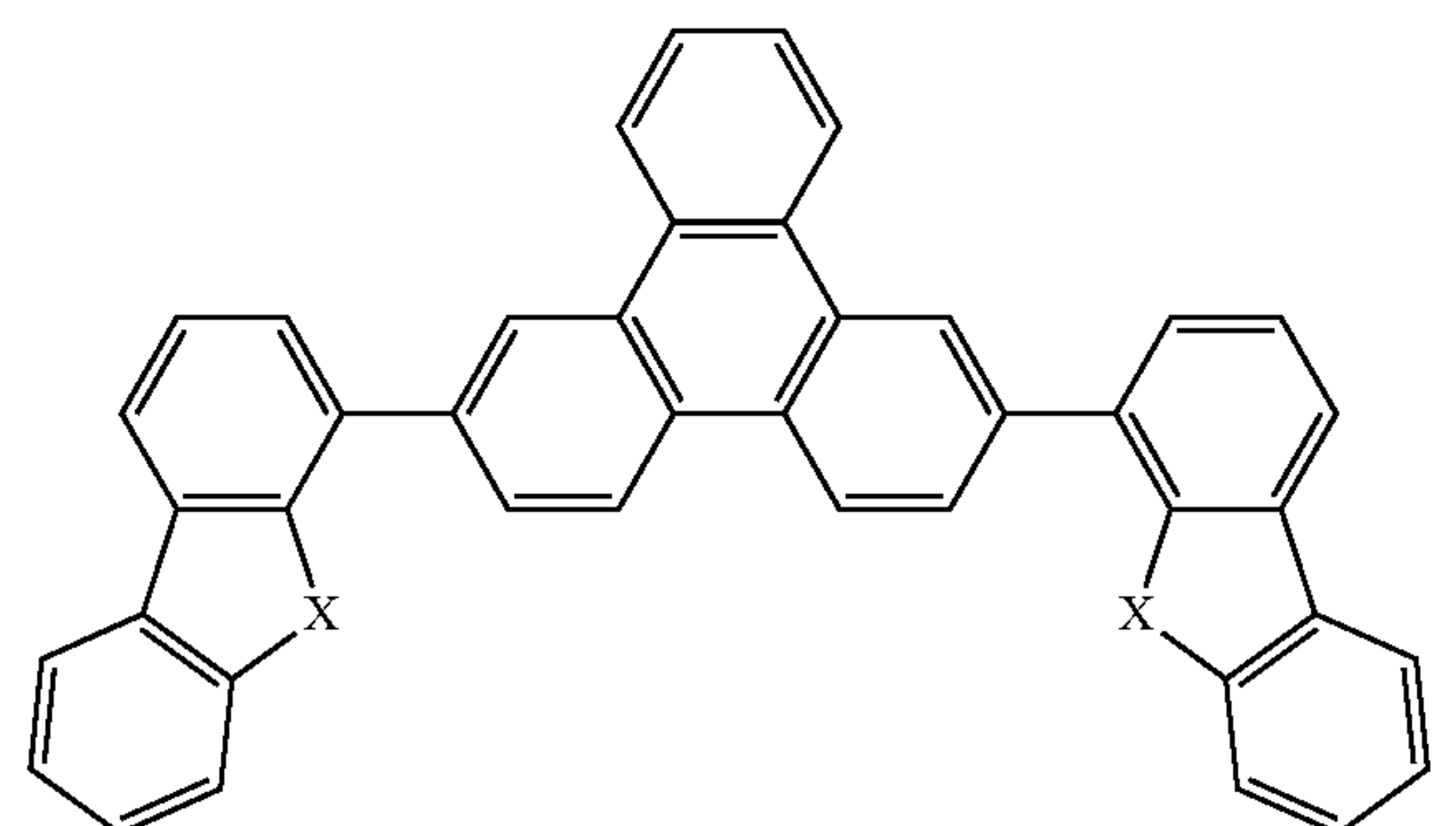
Compound 19
