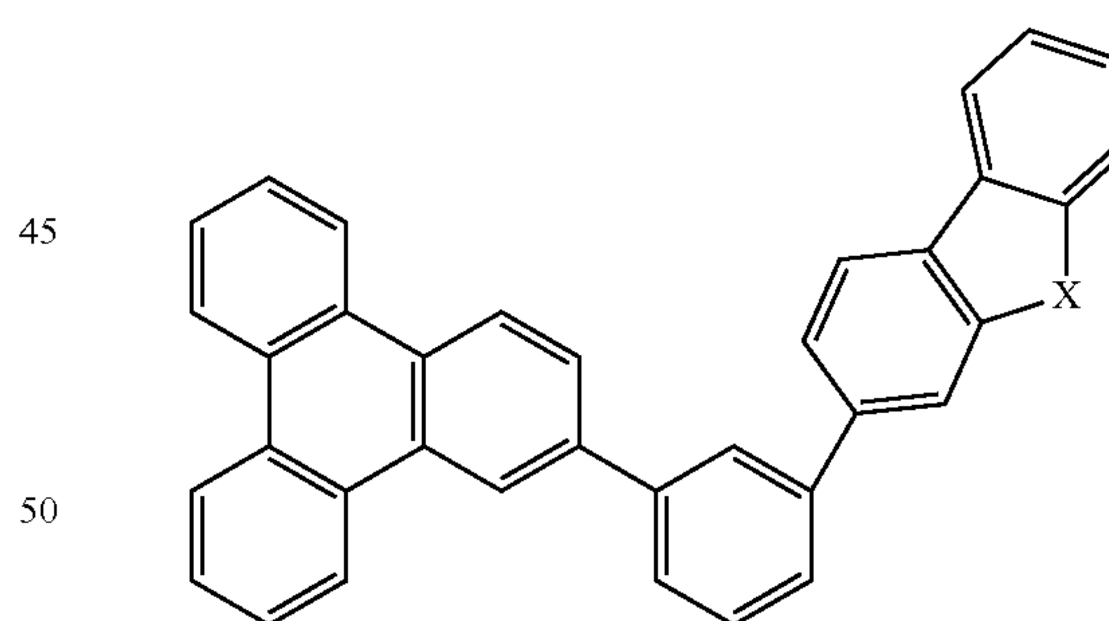
Compound 39G
