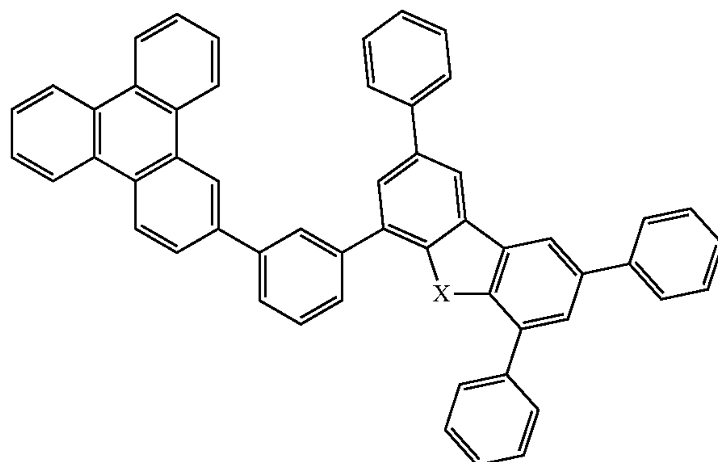
Compound 25
