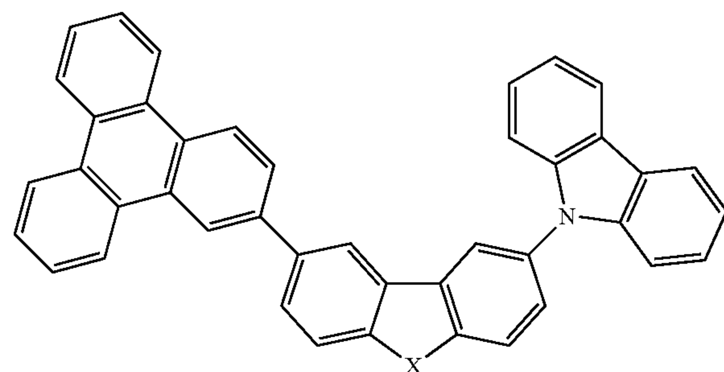
Compound 15
