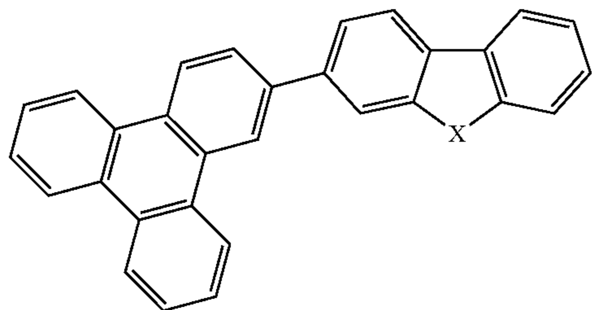
Compound 9
