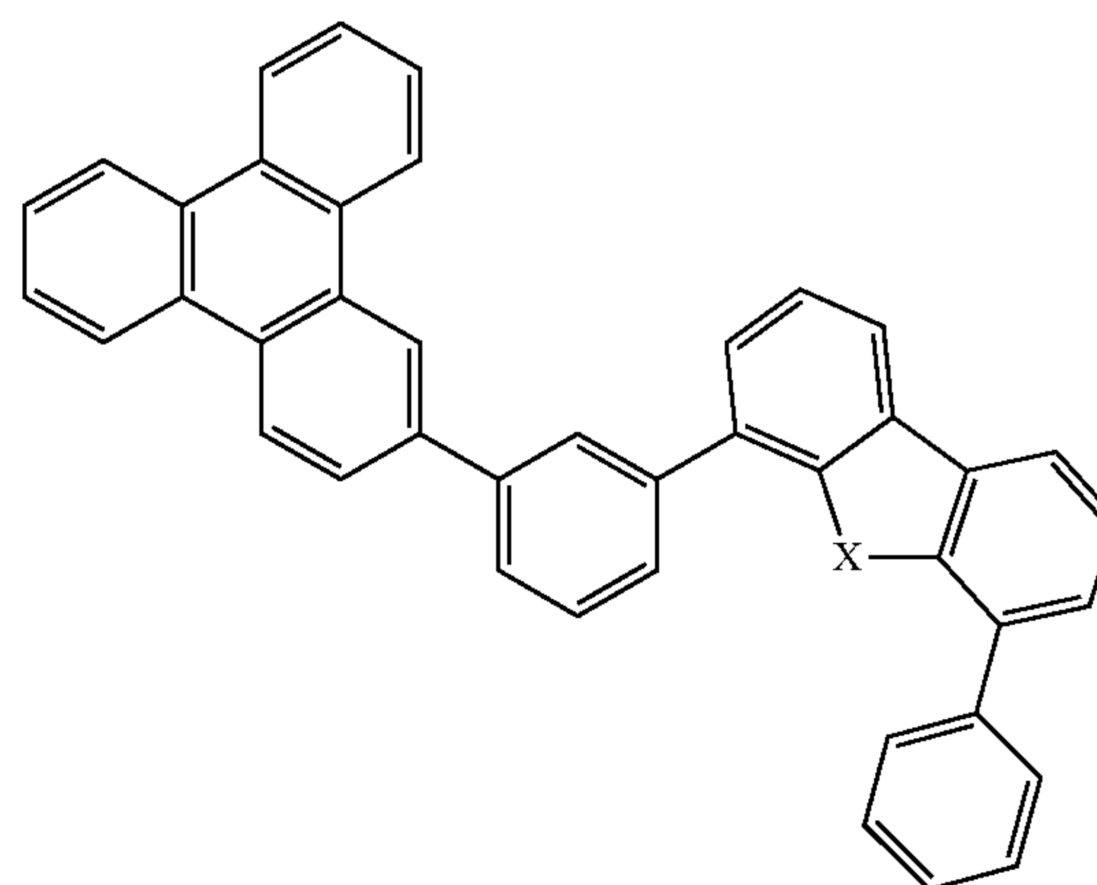
Compound 23
