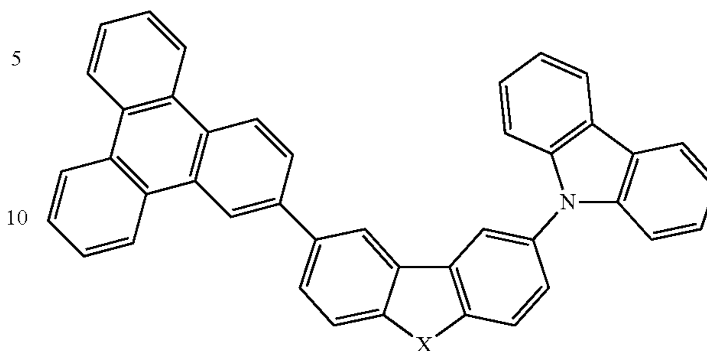
Compound 15
