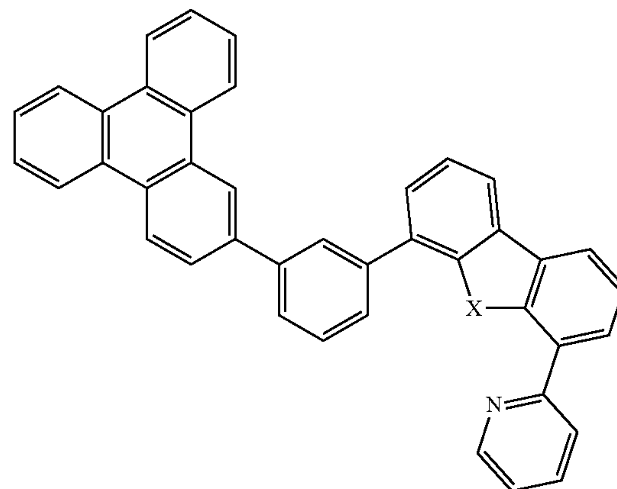
Compound 47
