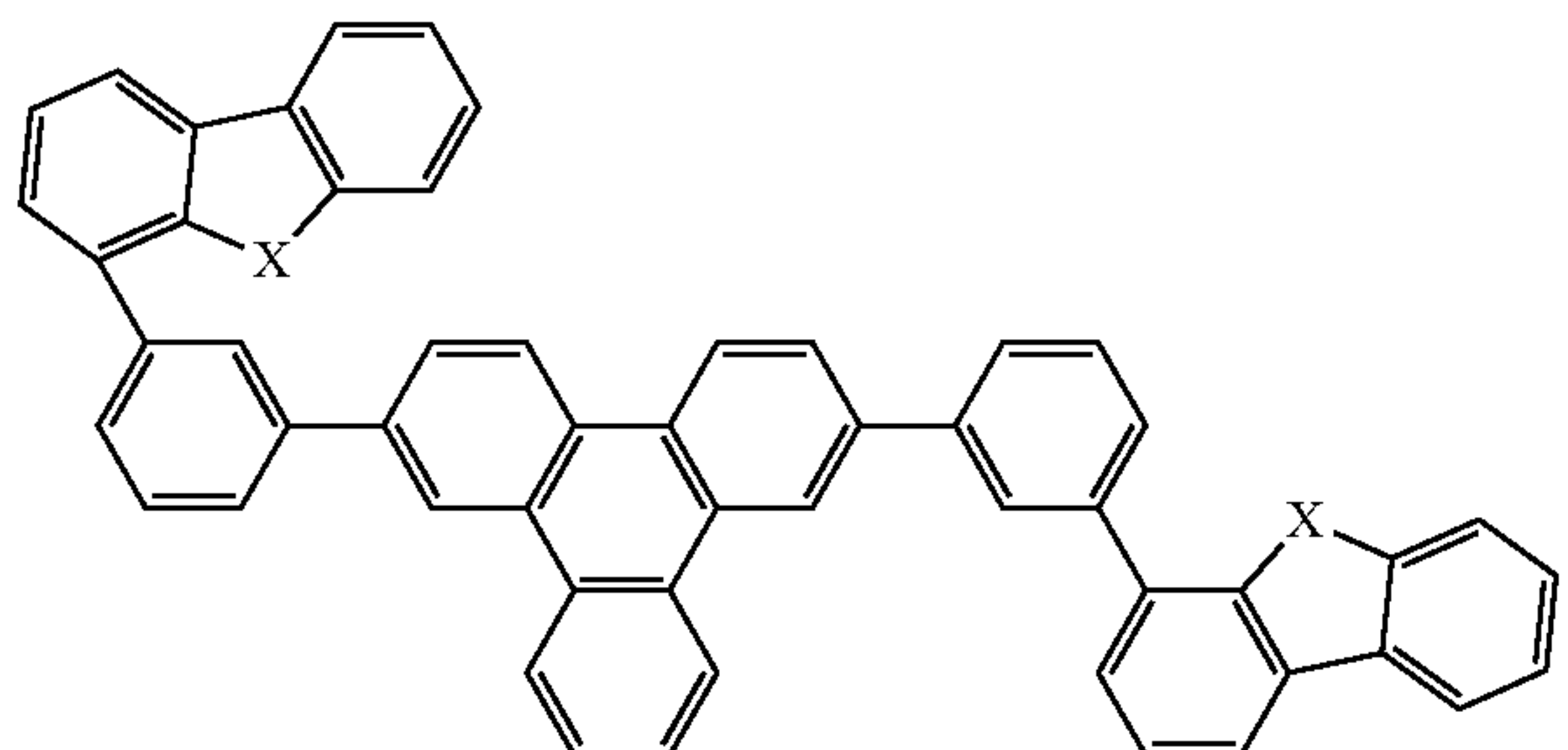
Compound 26
