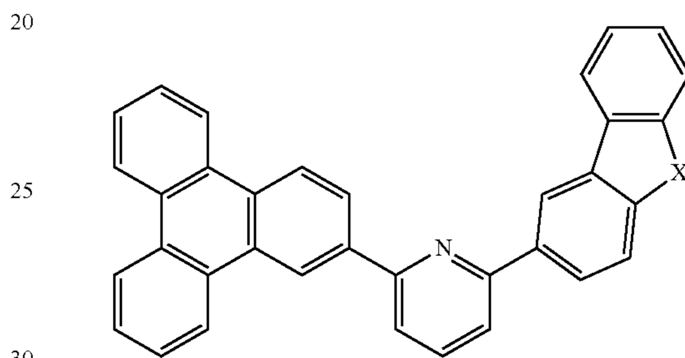
Compound 43
