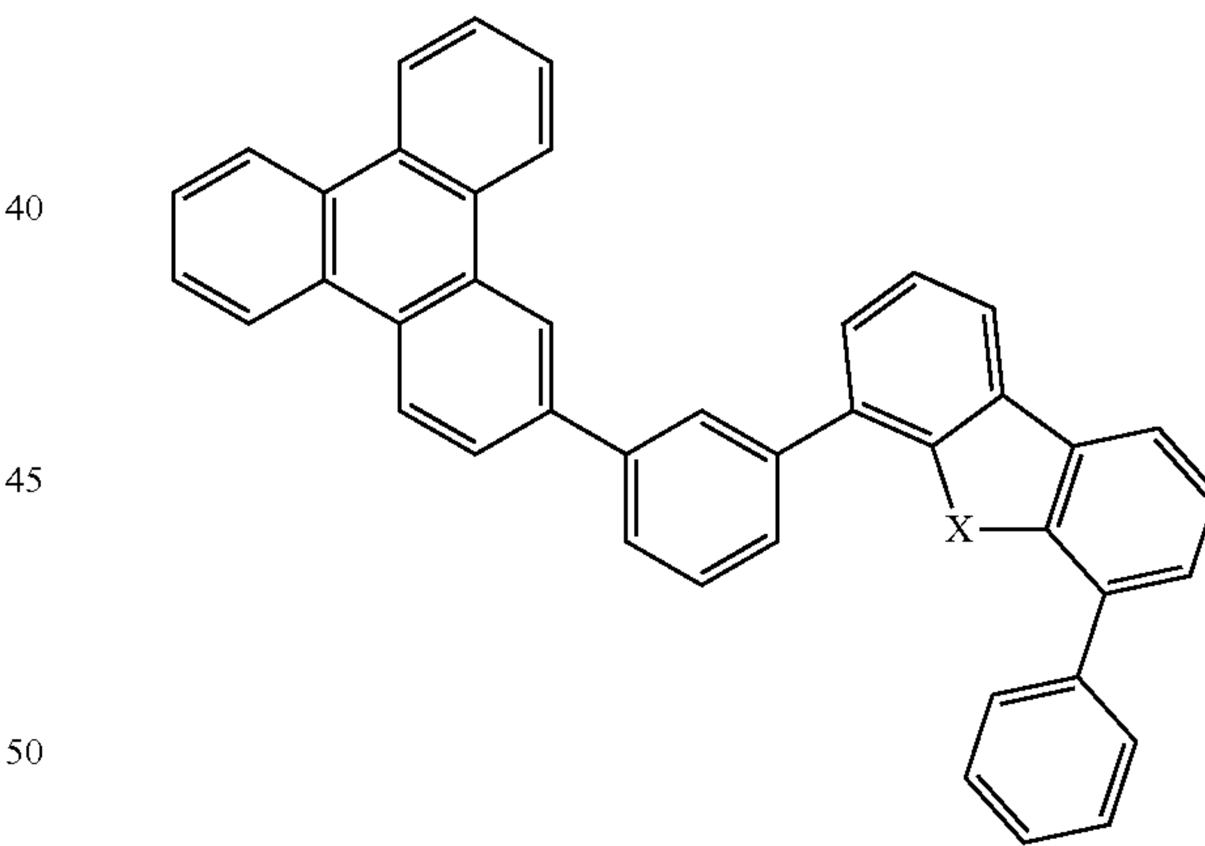
Compound 23
