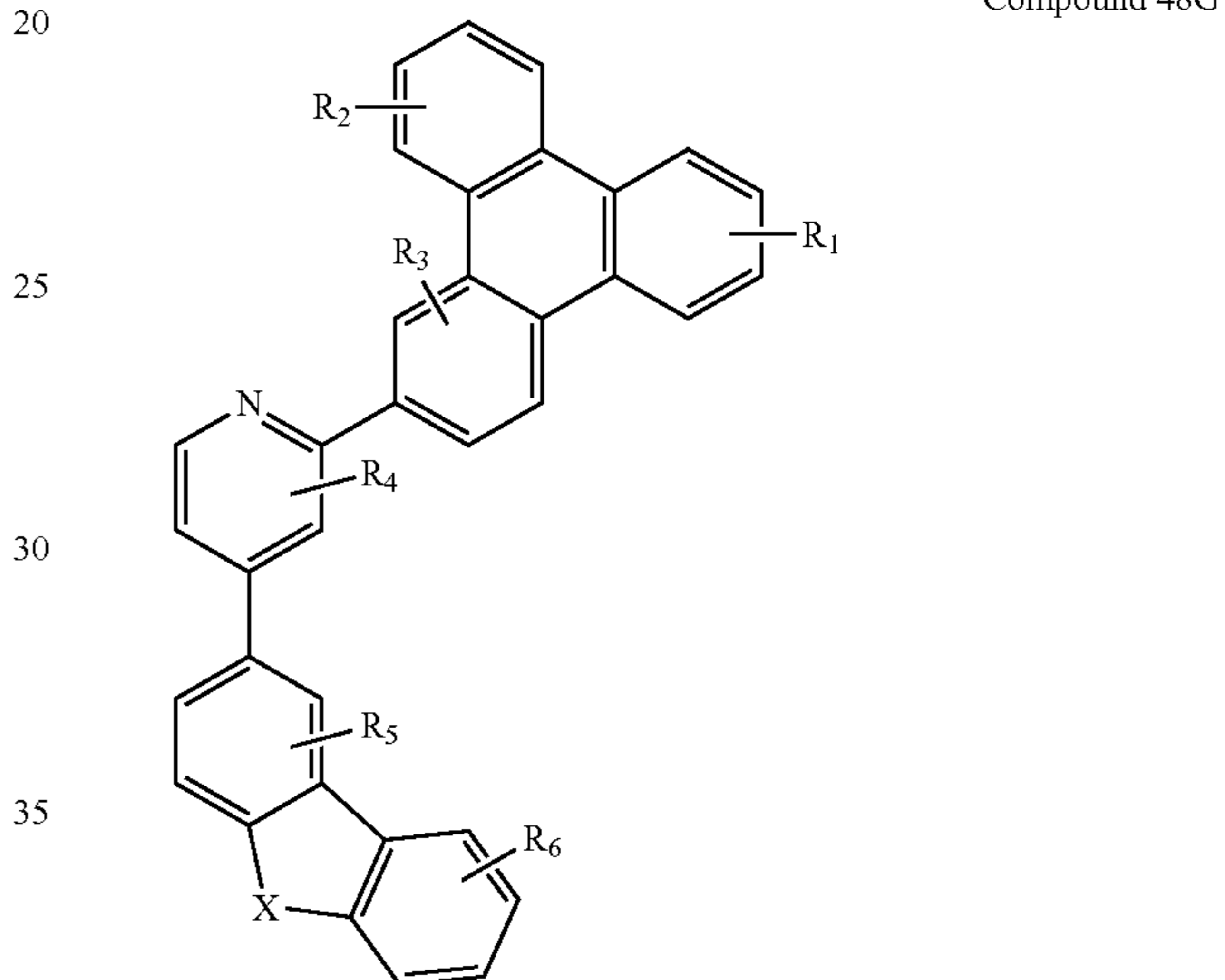
Compound 48
