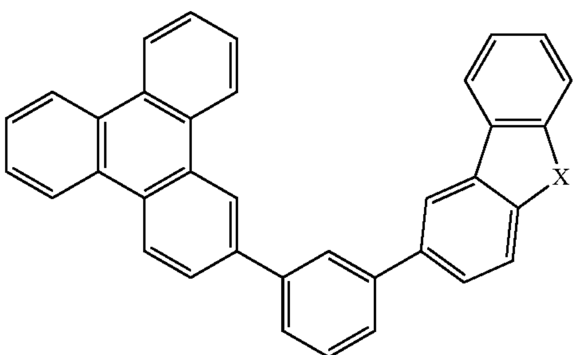
Compound 20
