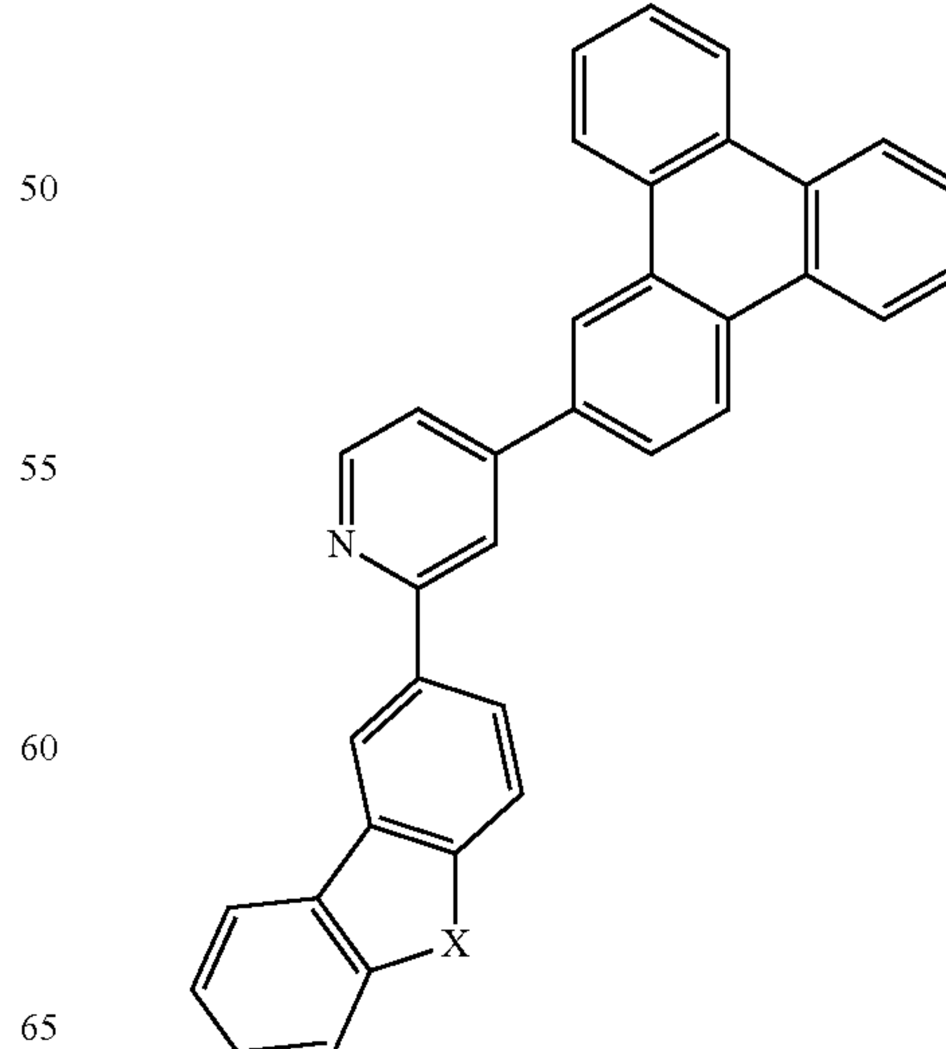
Compound 22
