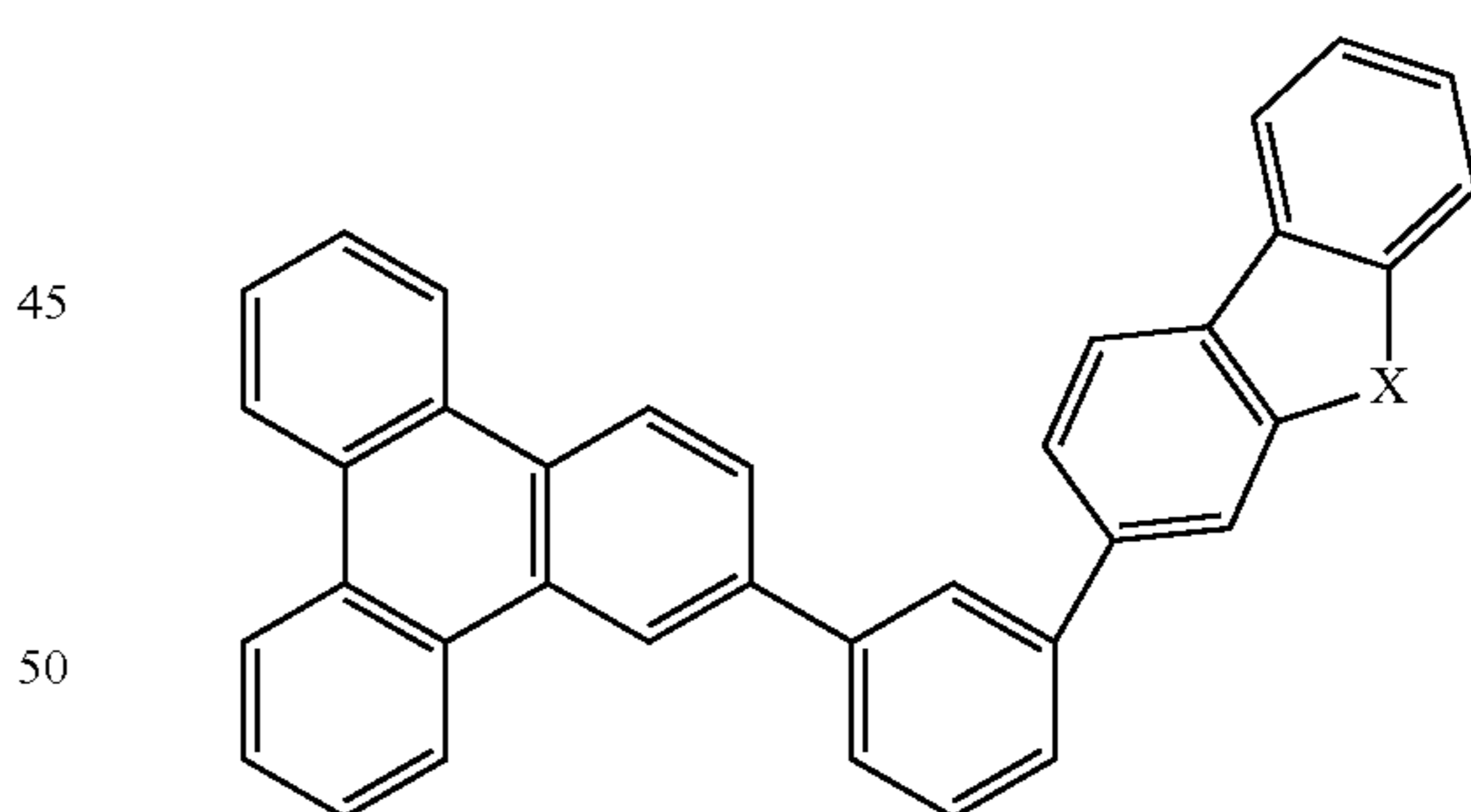
Compound 40
