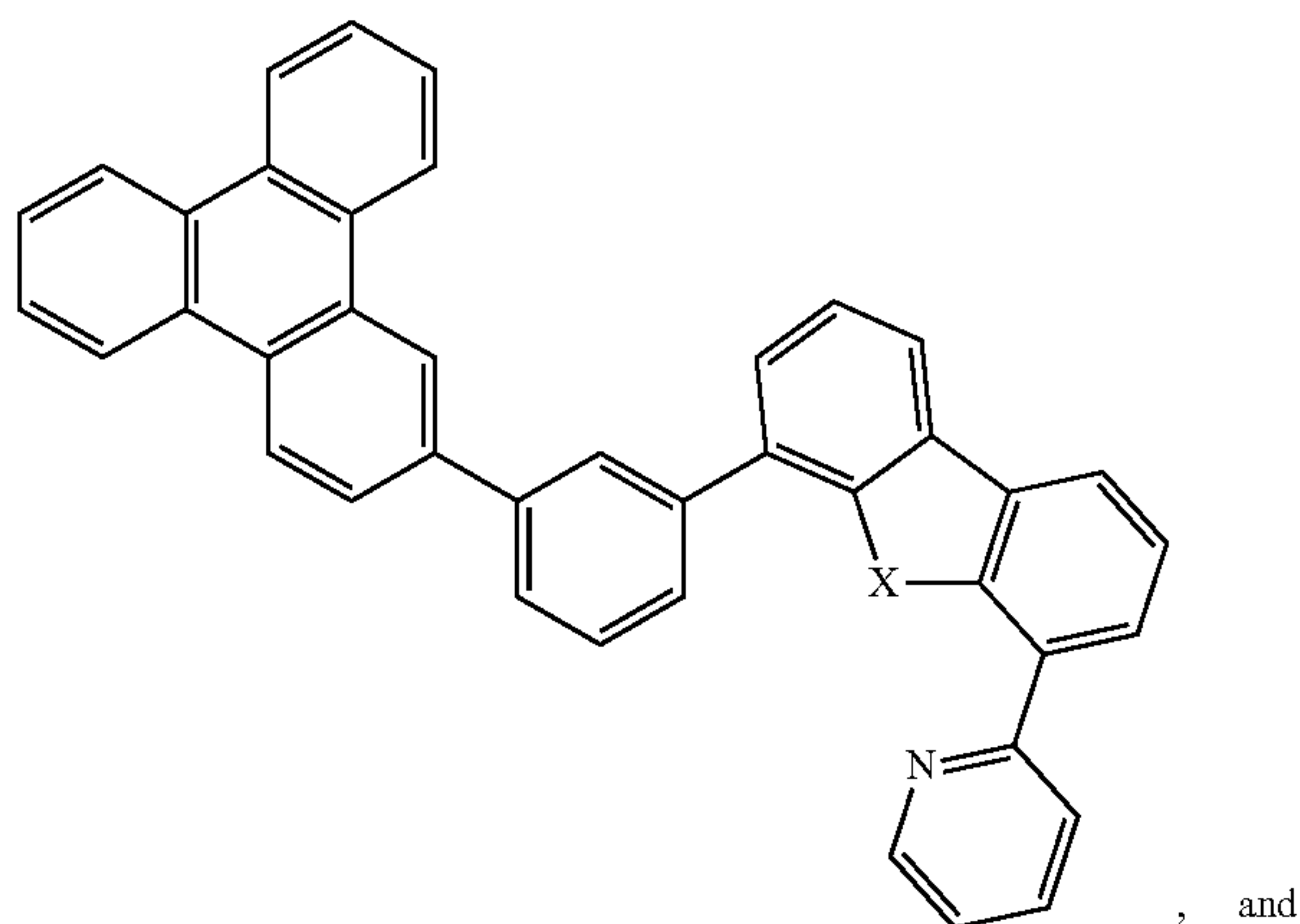
Compound 47
