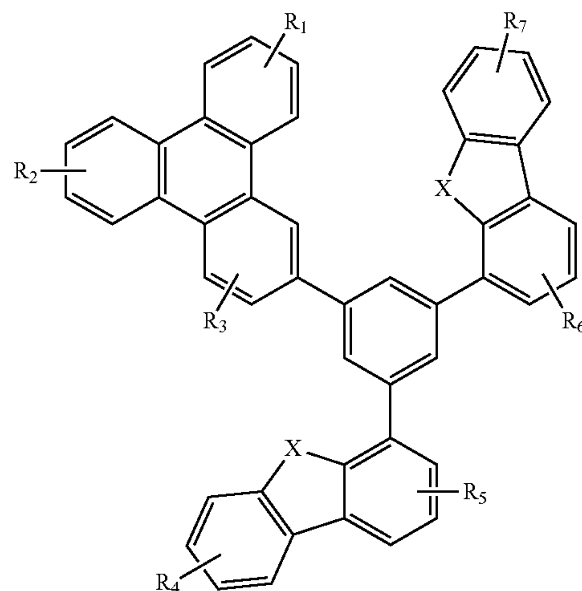
Compound 37G
