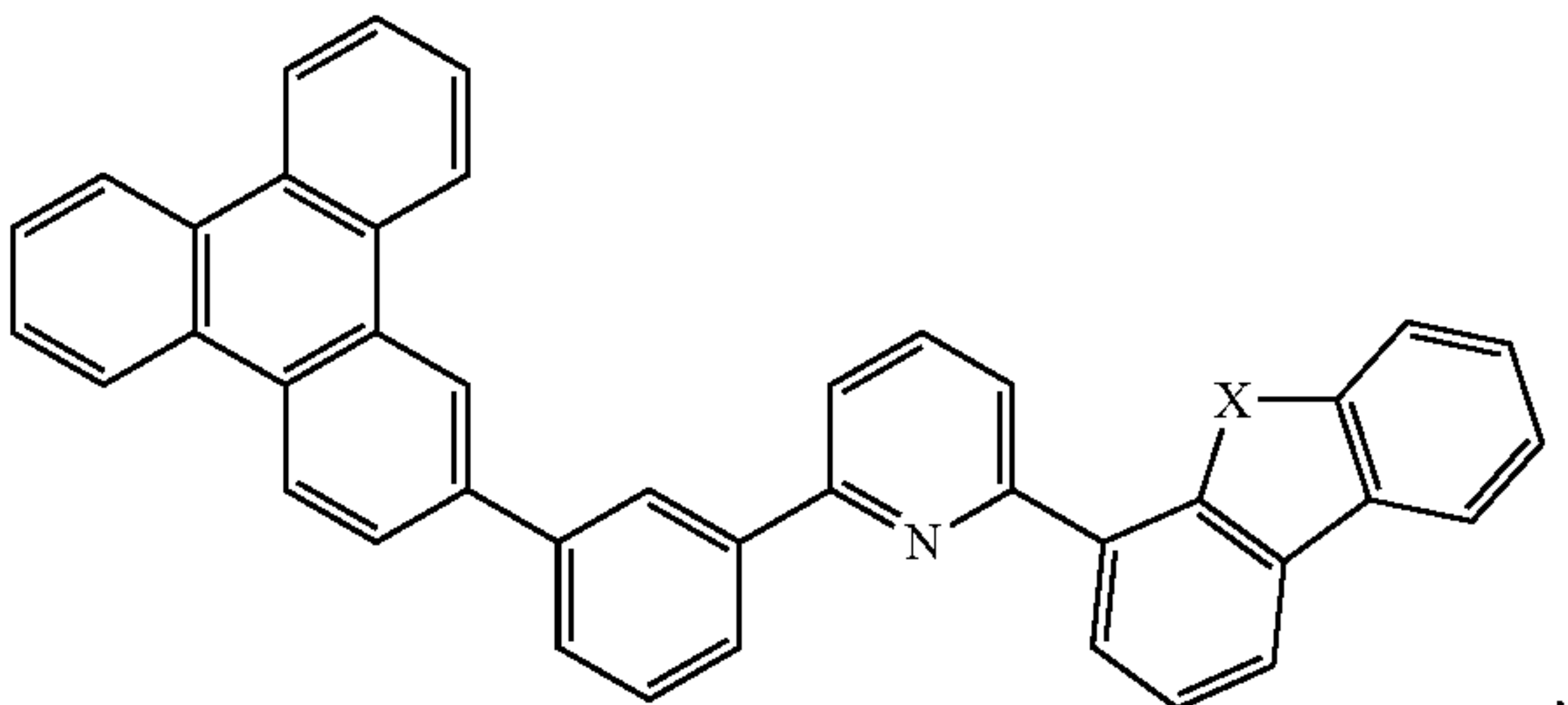
Compound 22
