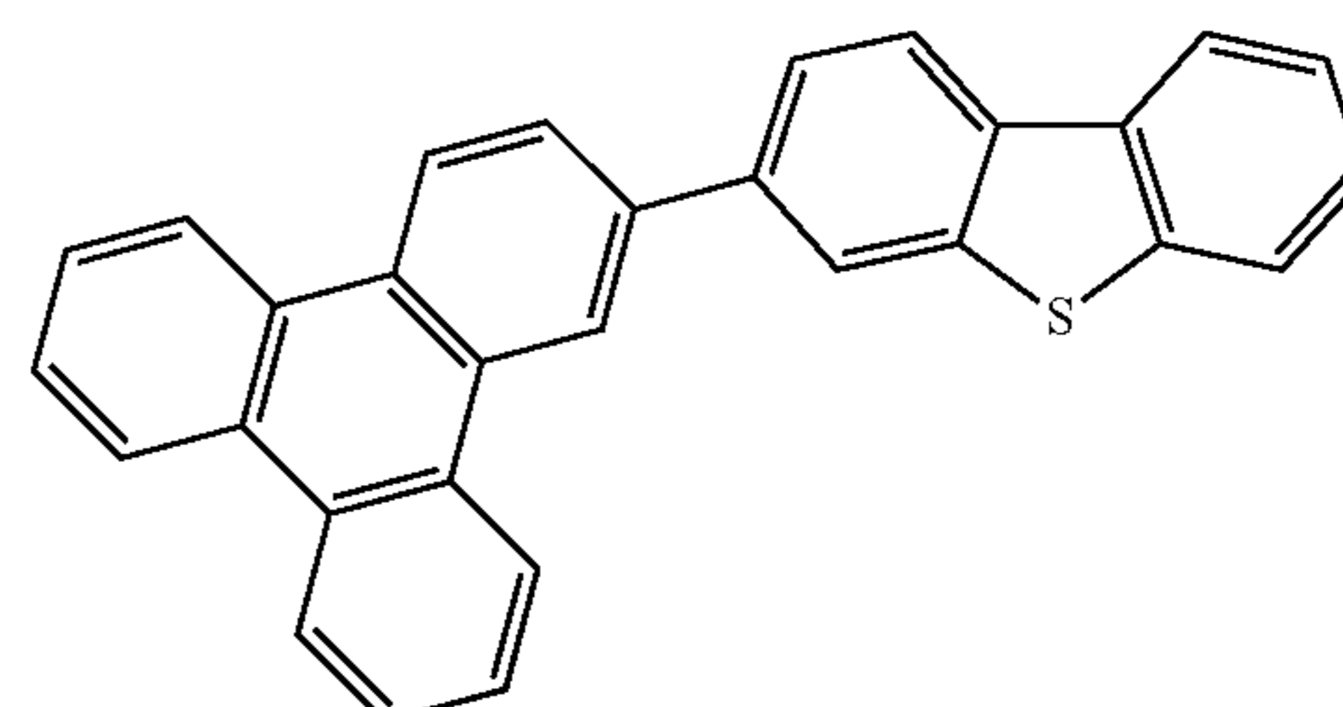
Compound 8'
