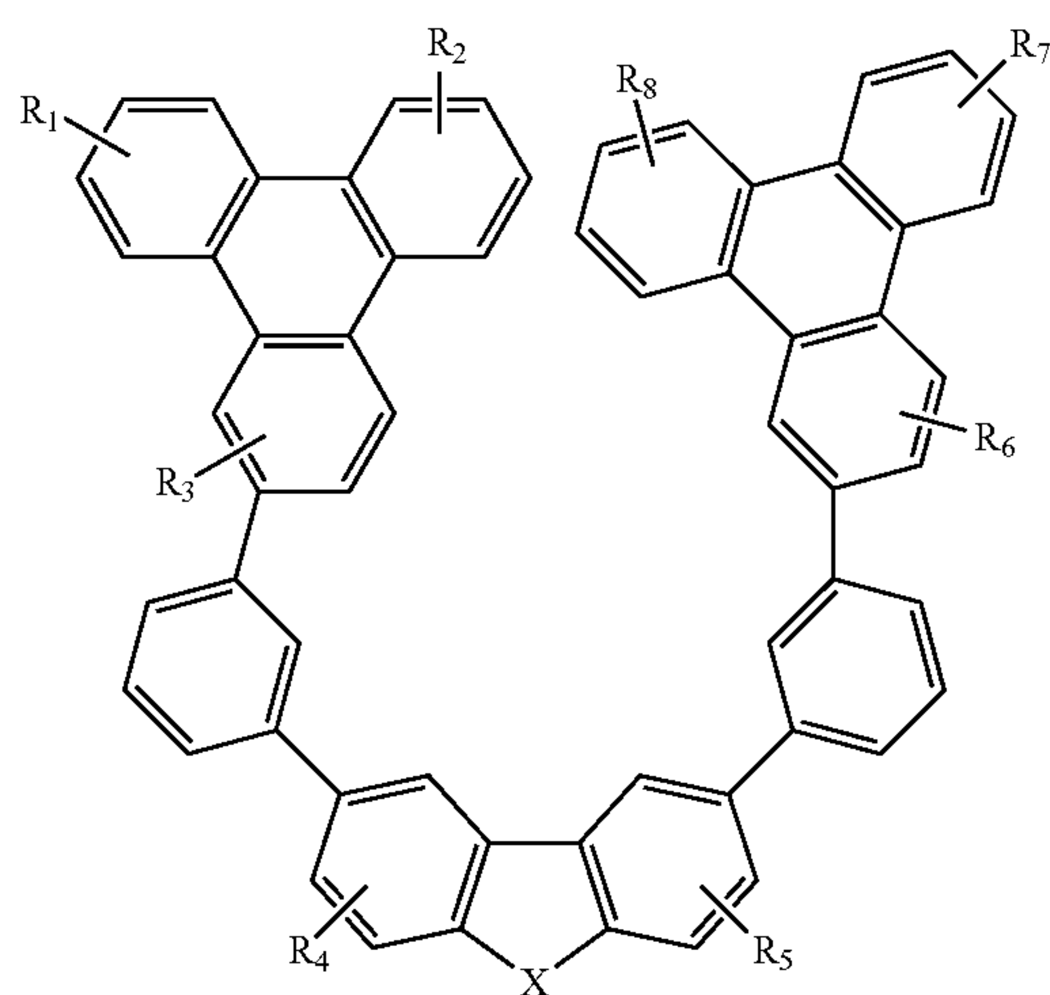
Compound 39G
