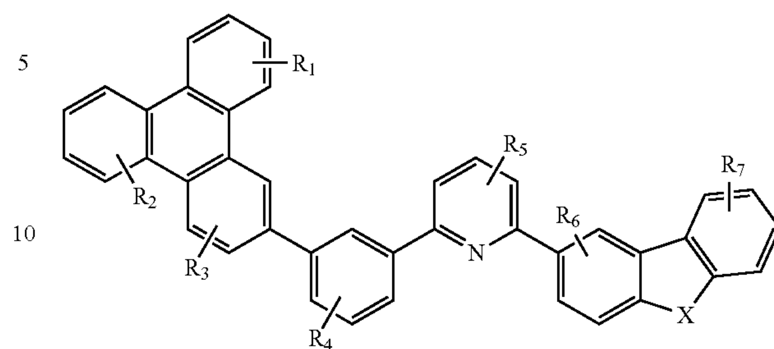
Compound 44
