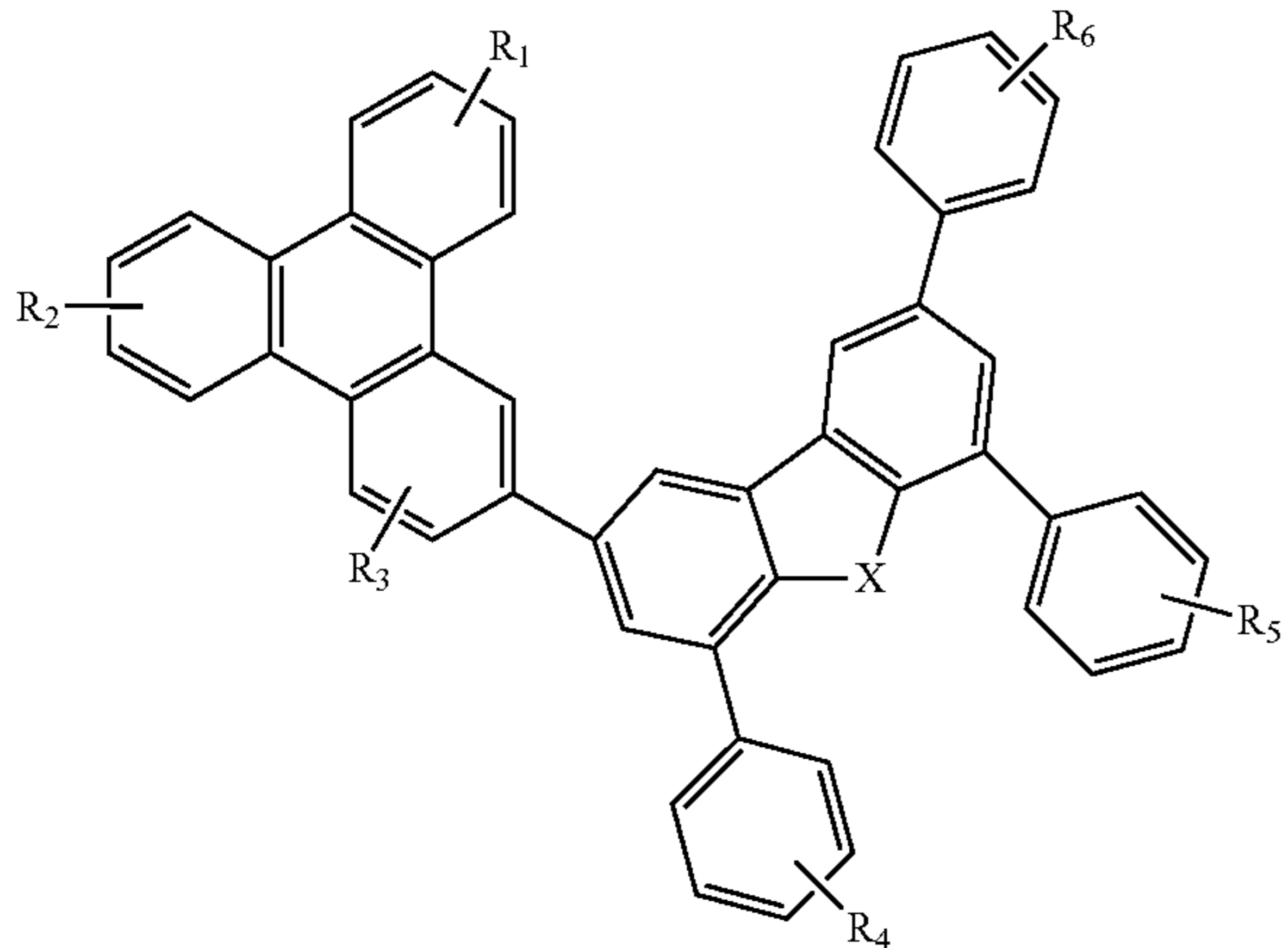
Compound 35G
