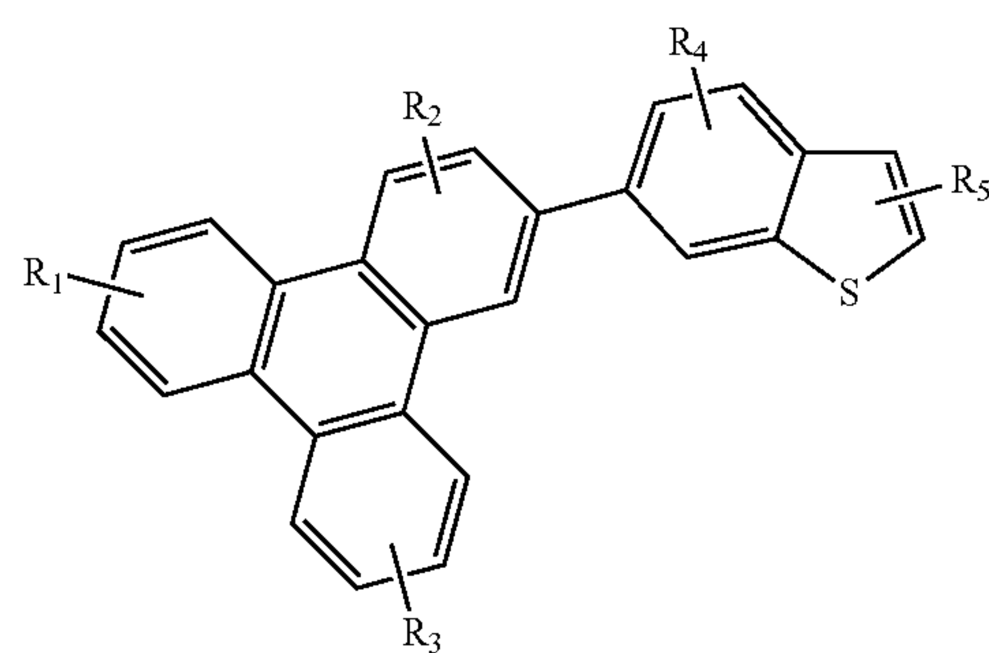
Compound 17'G
