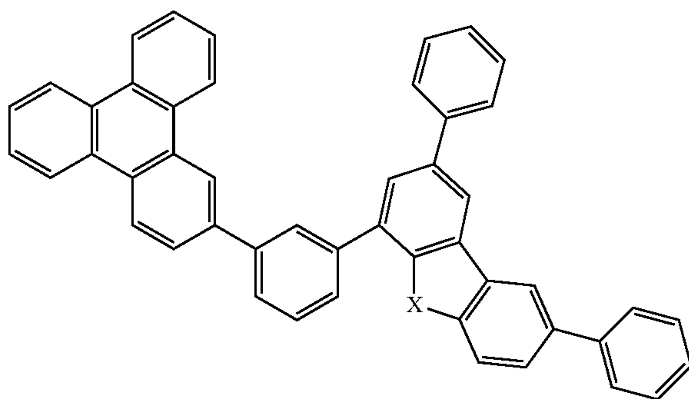
Compound 25G
