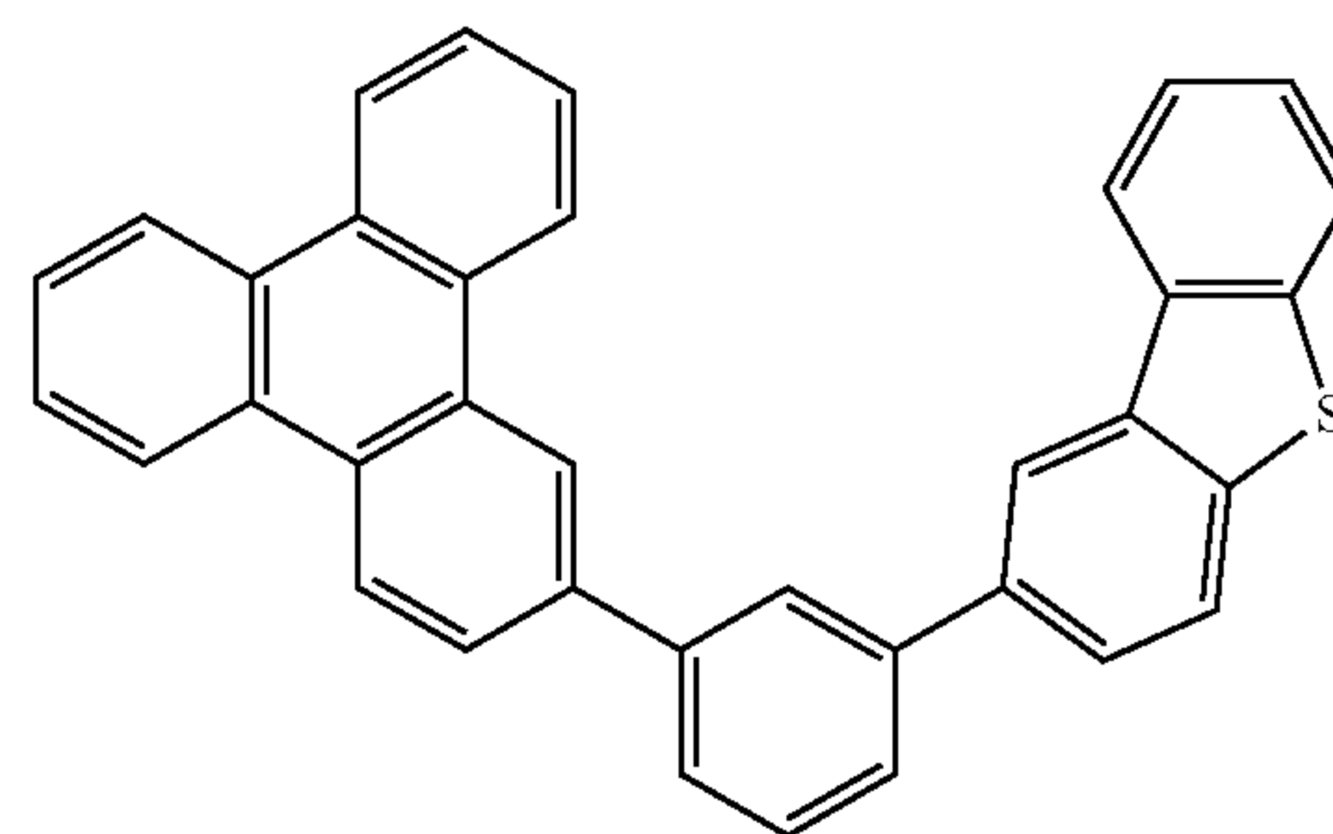
Compound 20S
