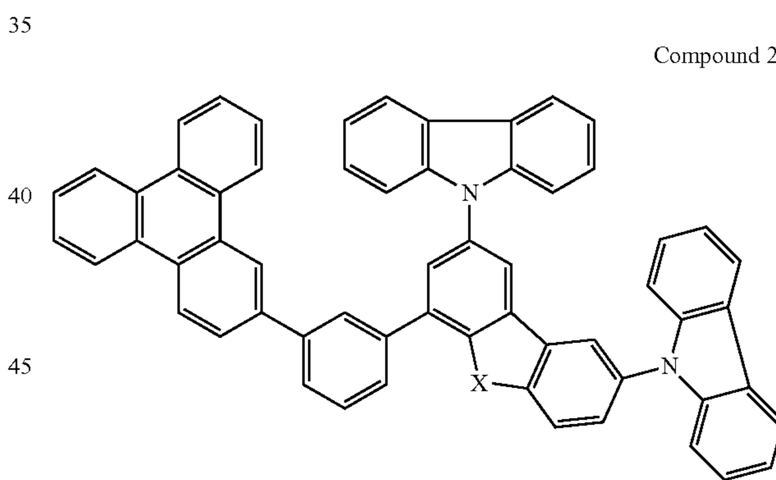
Compound 25
