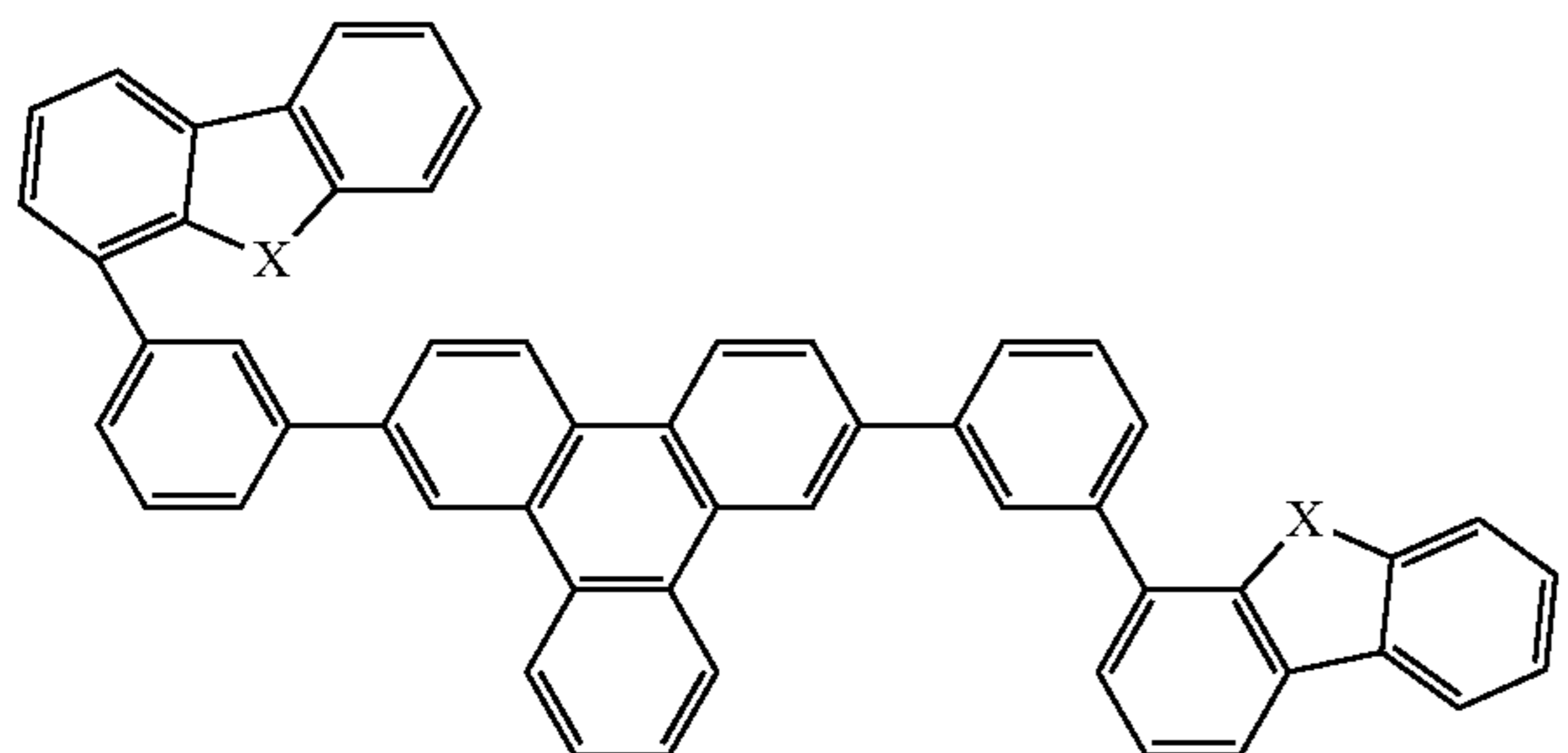
Compound 26
