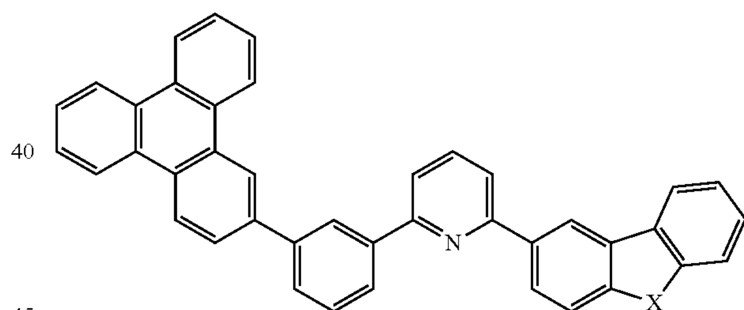
Compound 45
