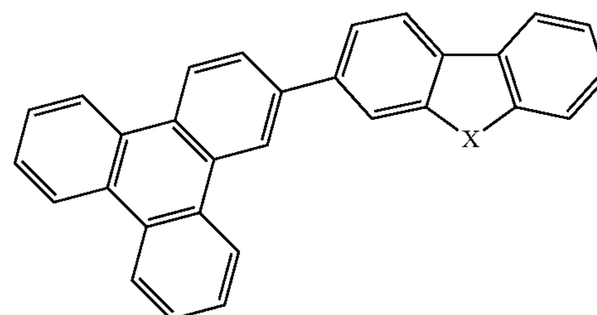
Compound 8
