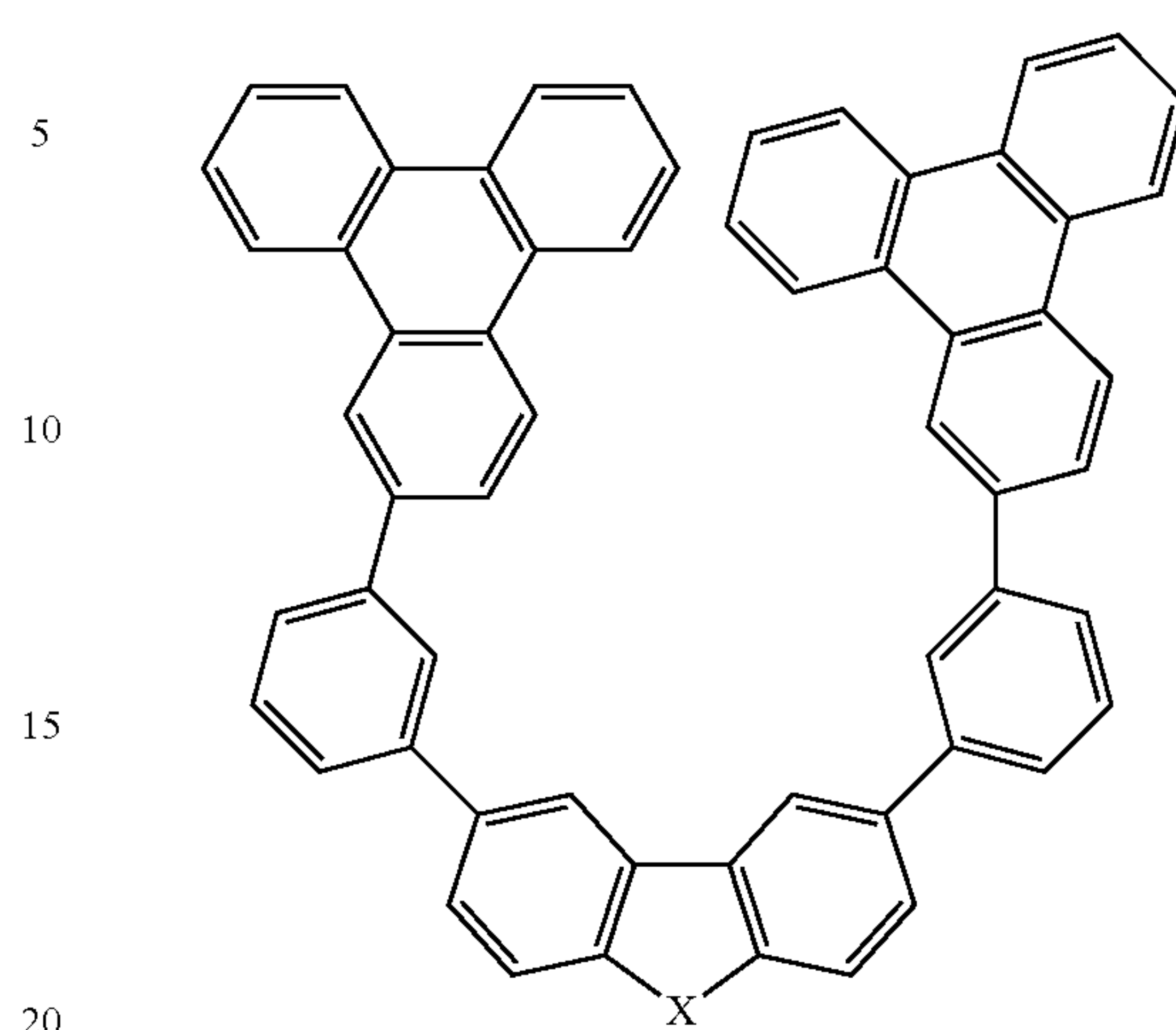
Compound 40G
