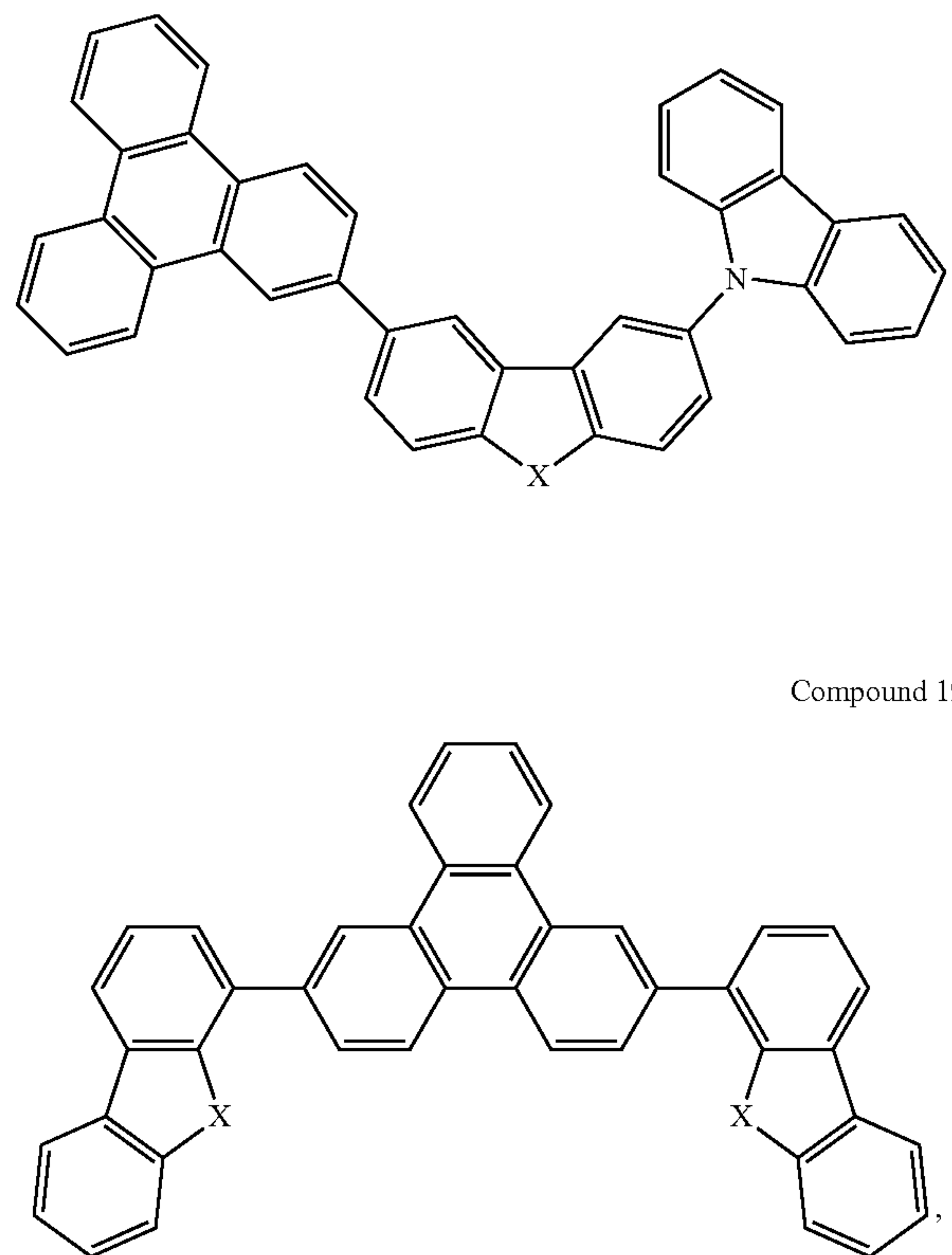
Compound 15
