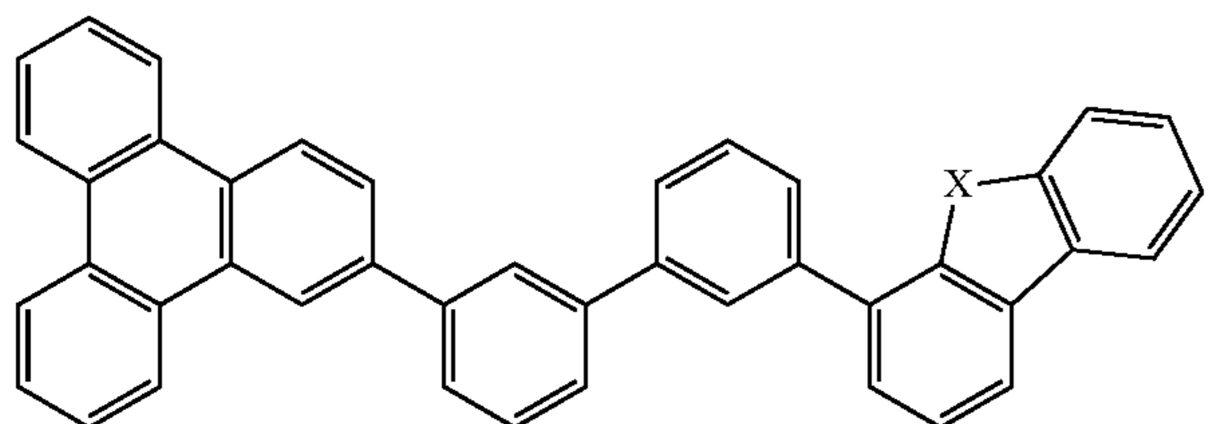
Compound 9
