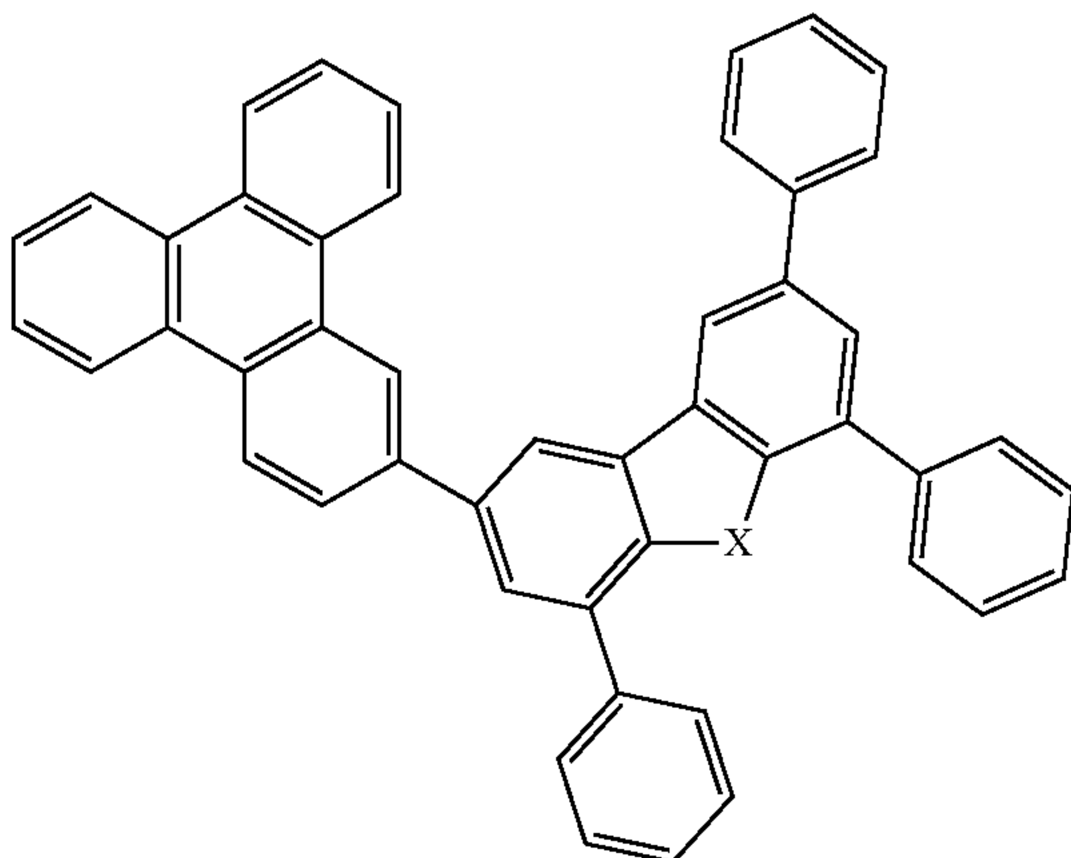
Compound 36
