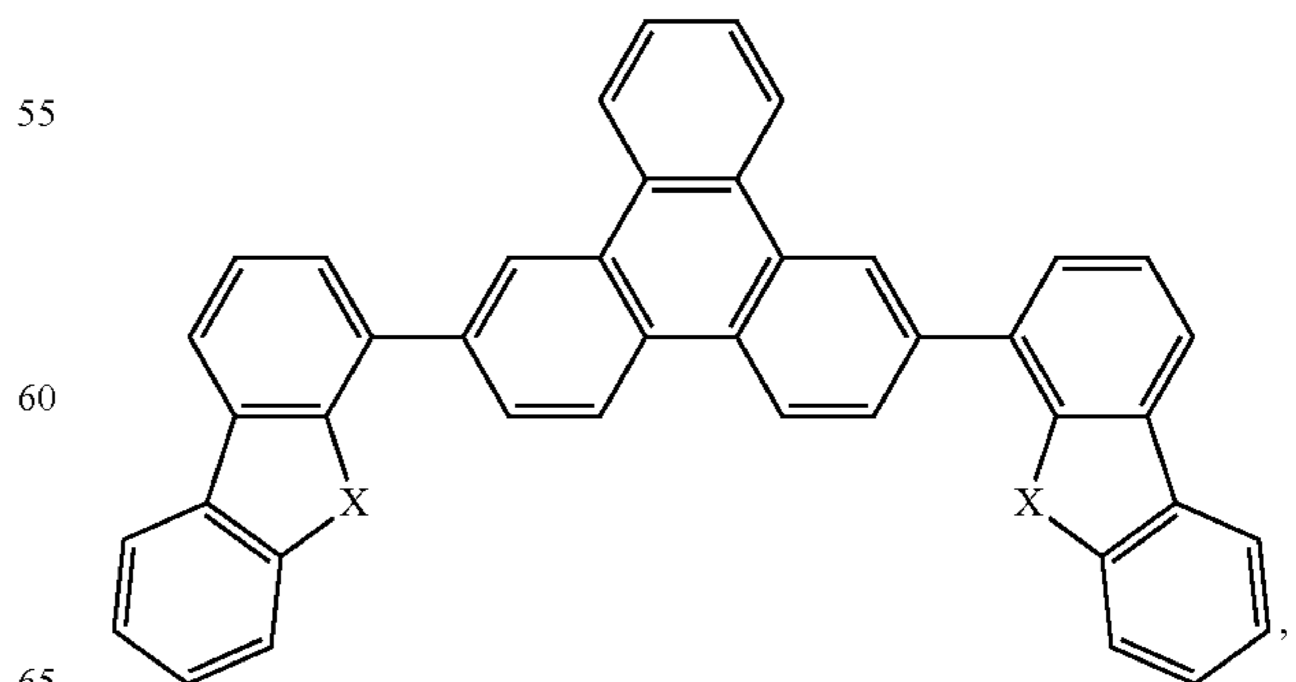
Compound 19
