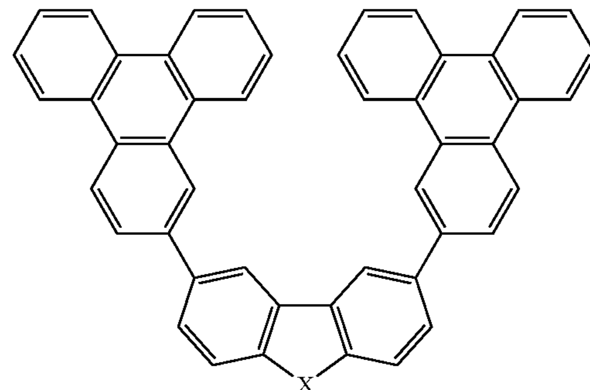
Compound 5
