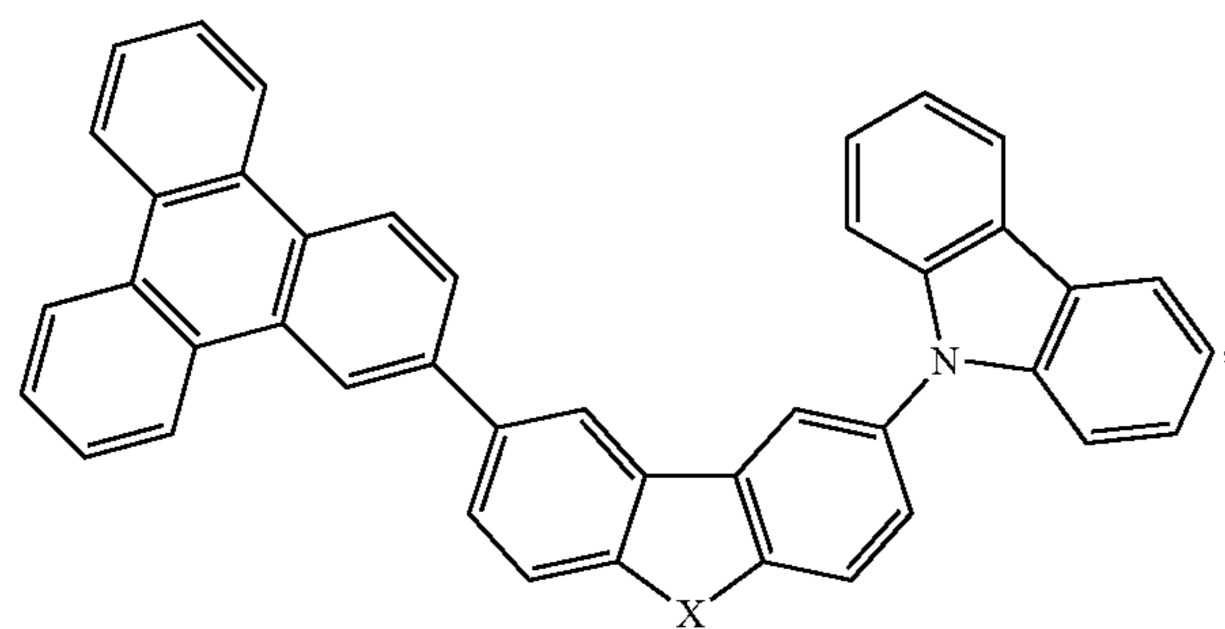
Compound 15
