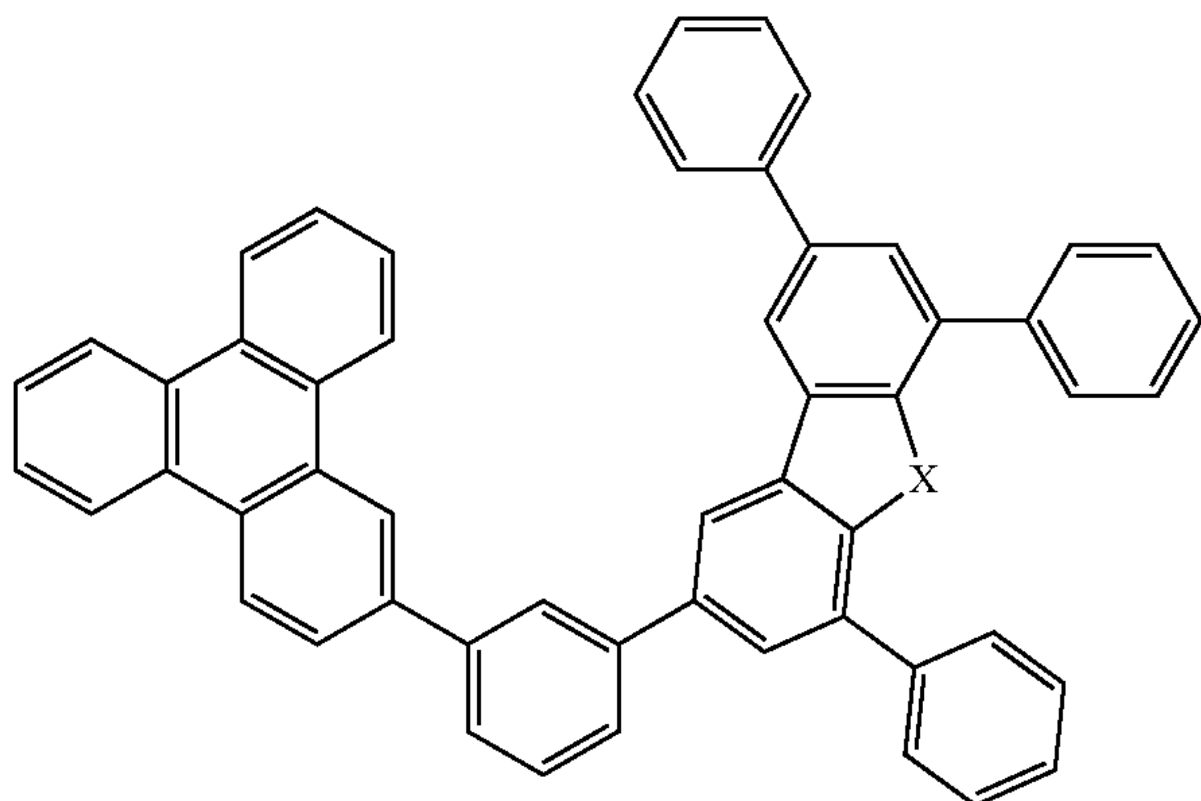
Compound 38
