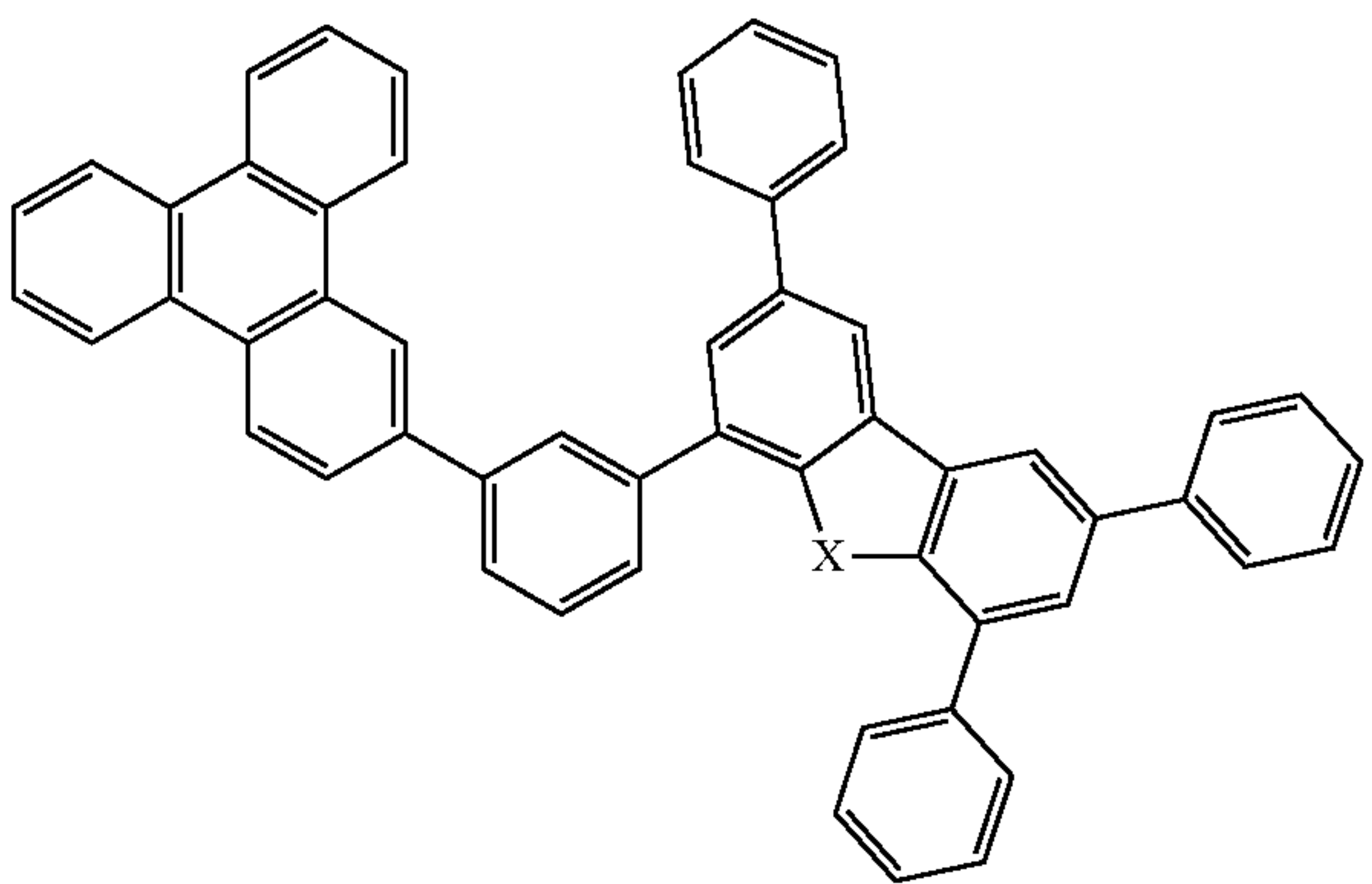
Compound 25
