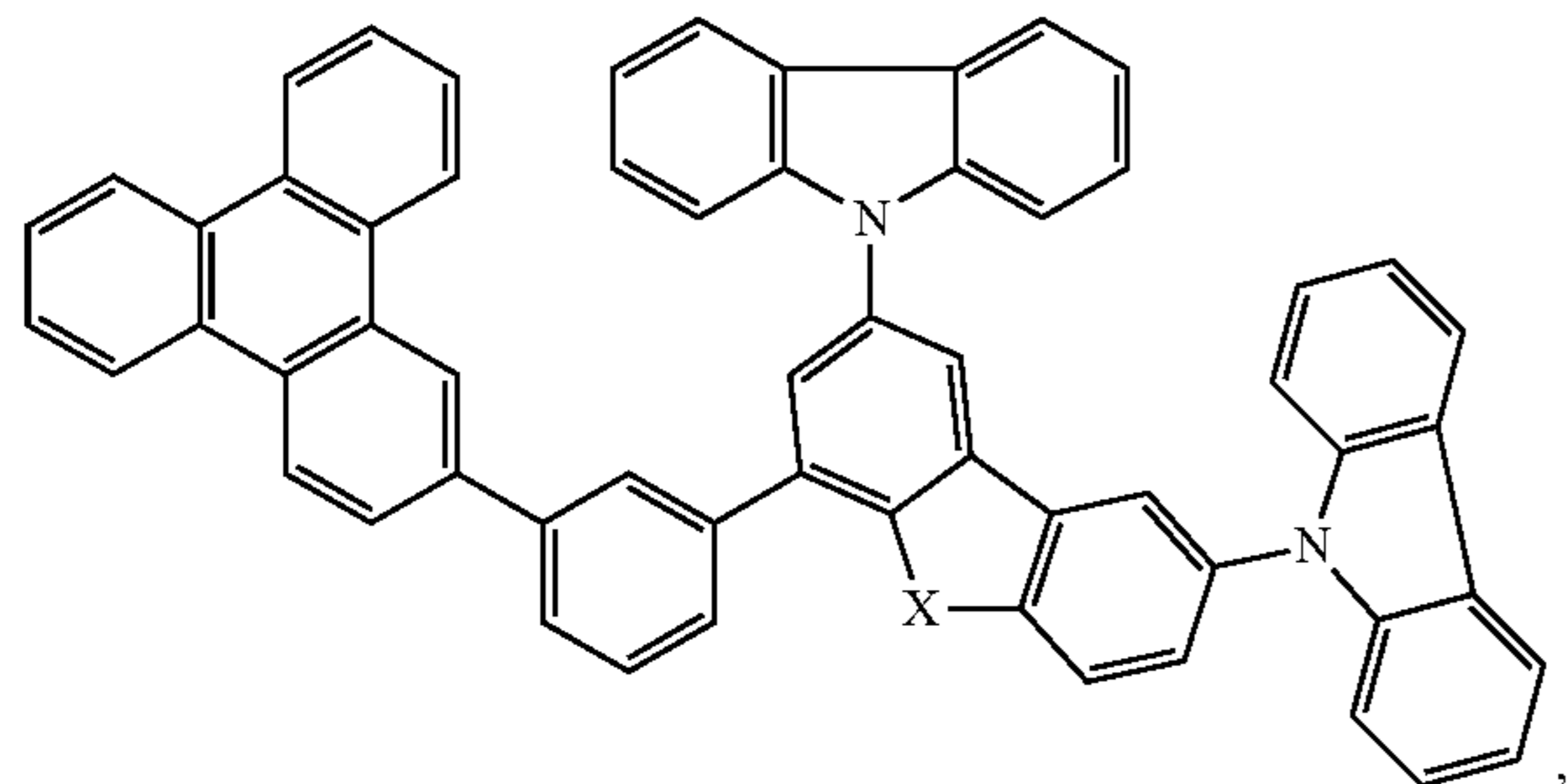
Compound 27
