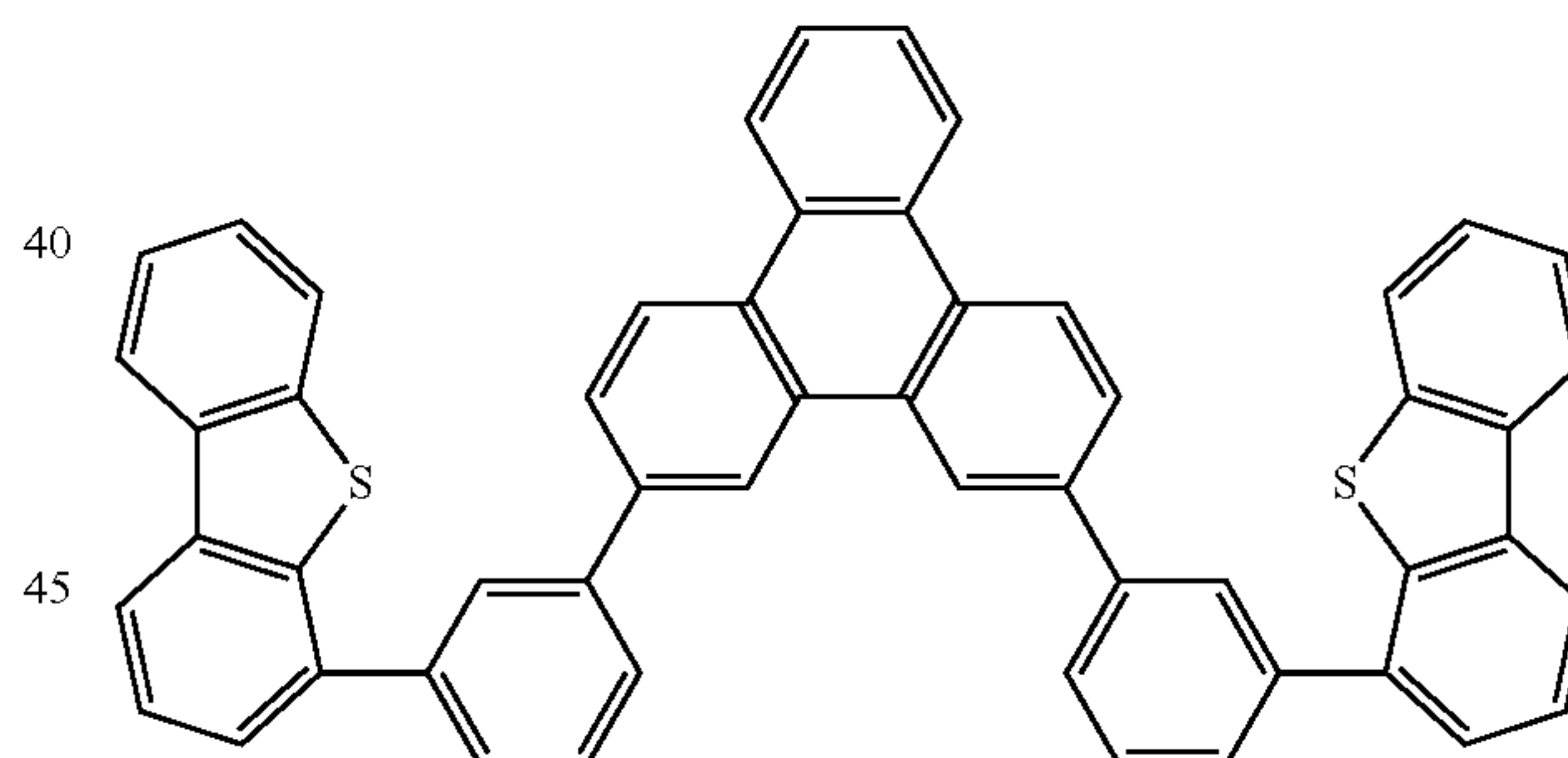
Compound 4'
