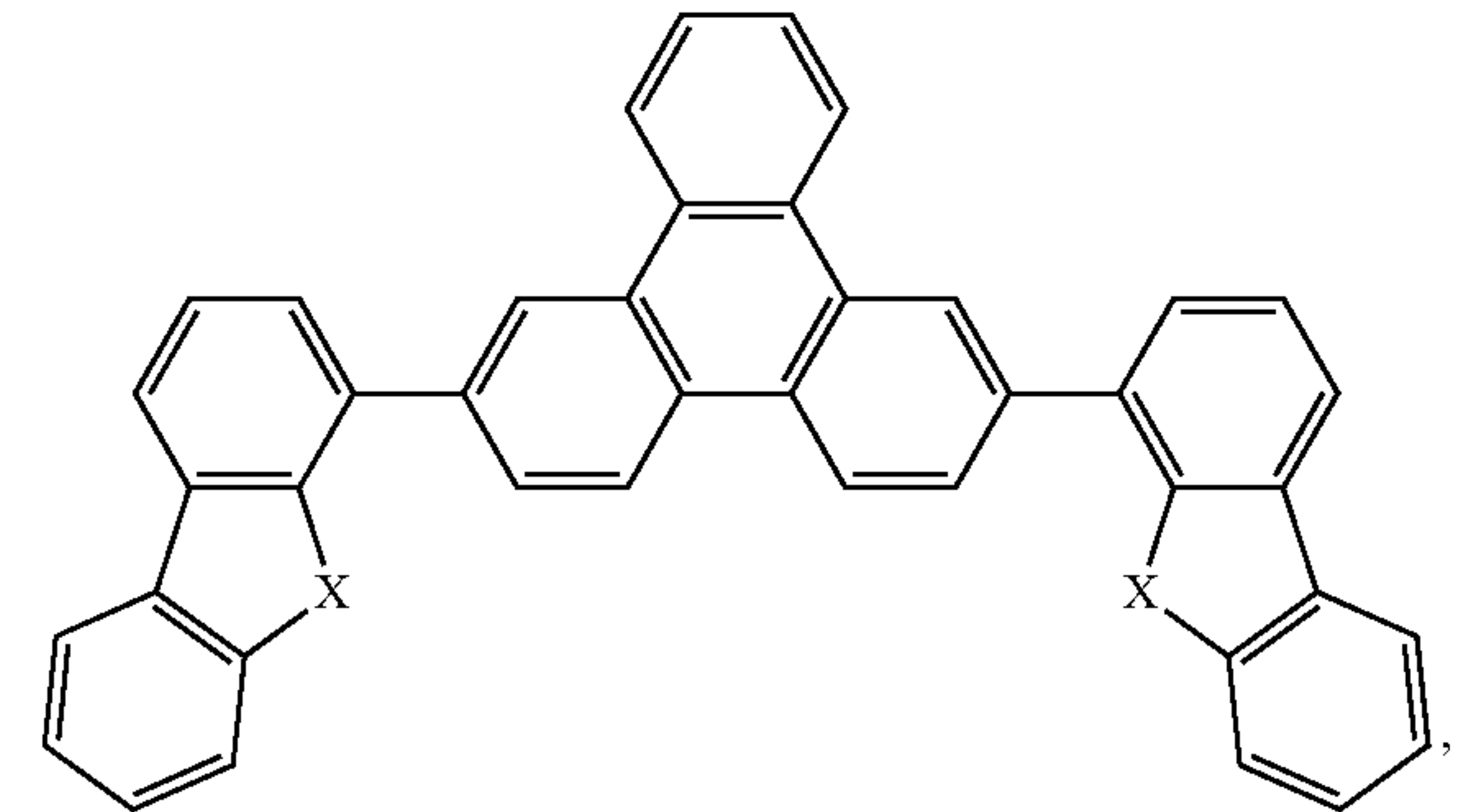
Compound 19
