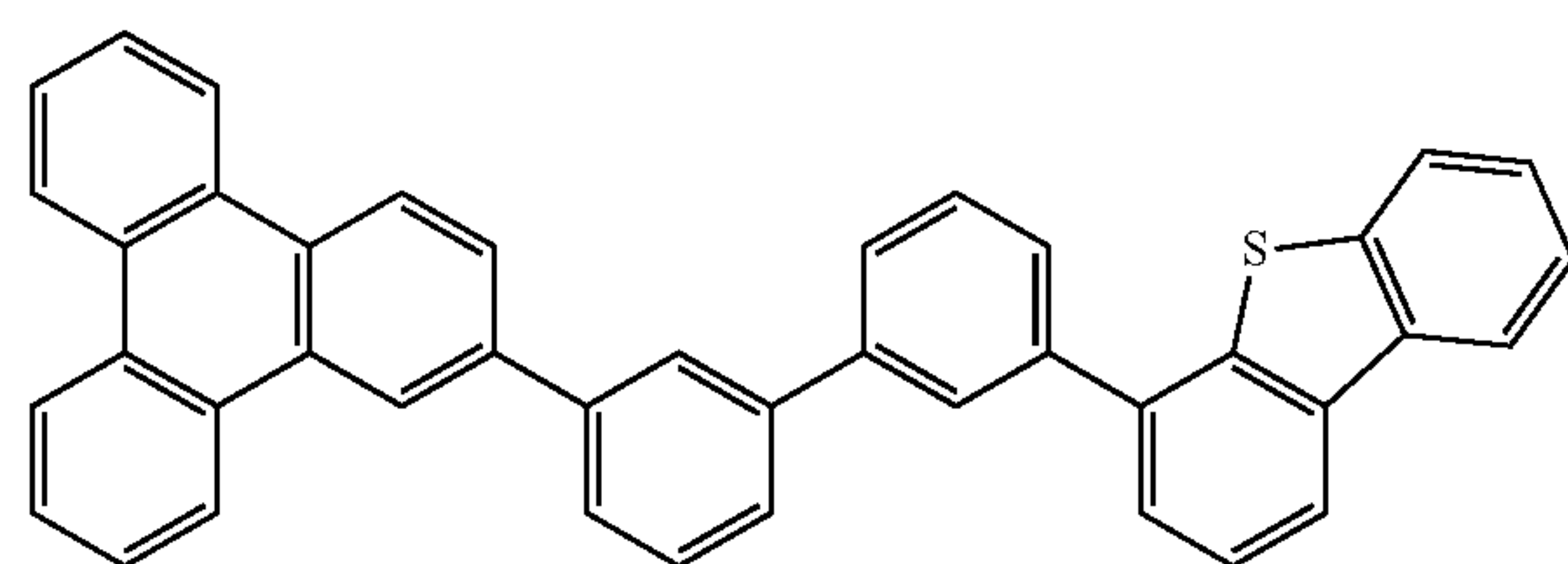
Compound 10'G
