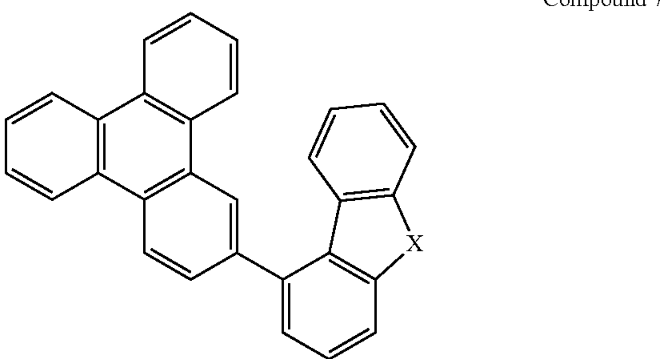
Compound 8G
