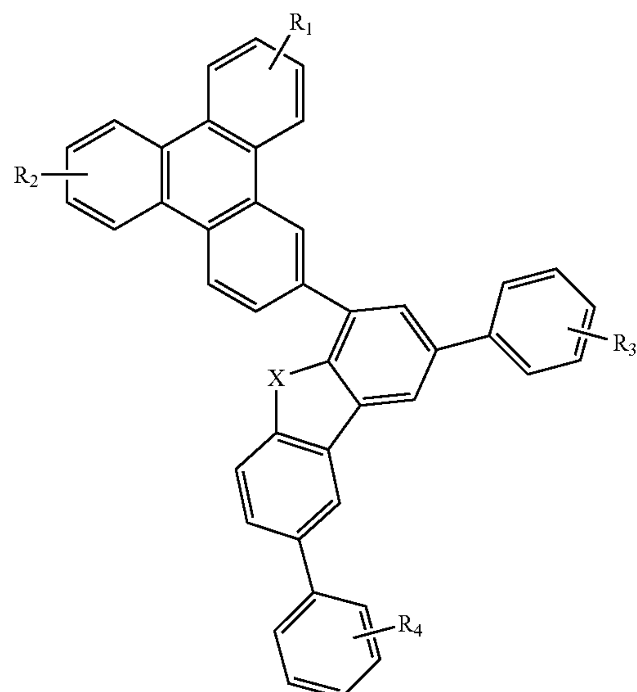
Compound 31G
