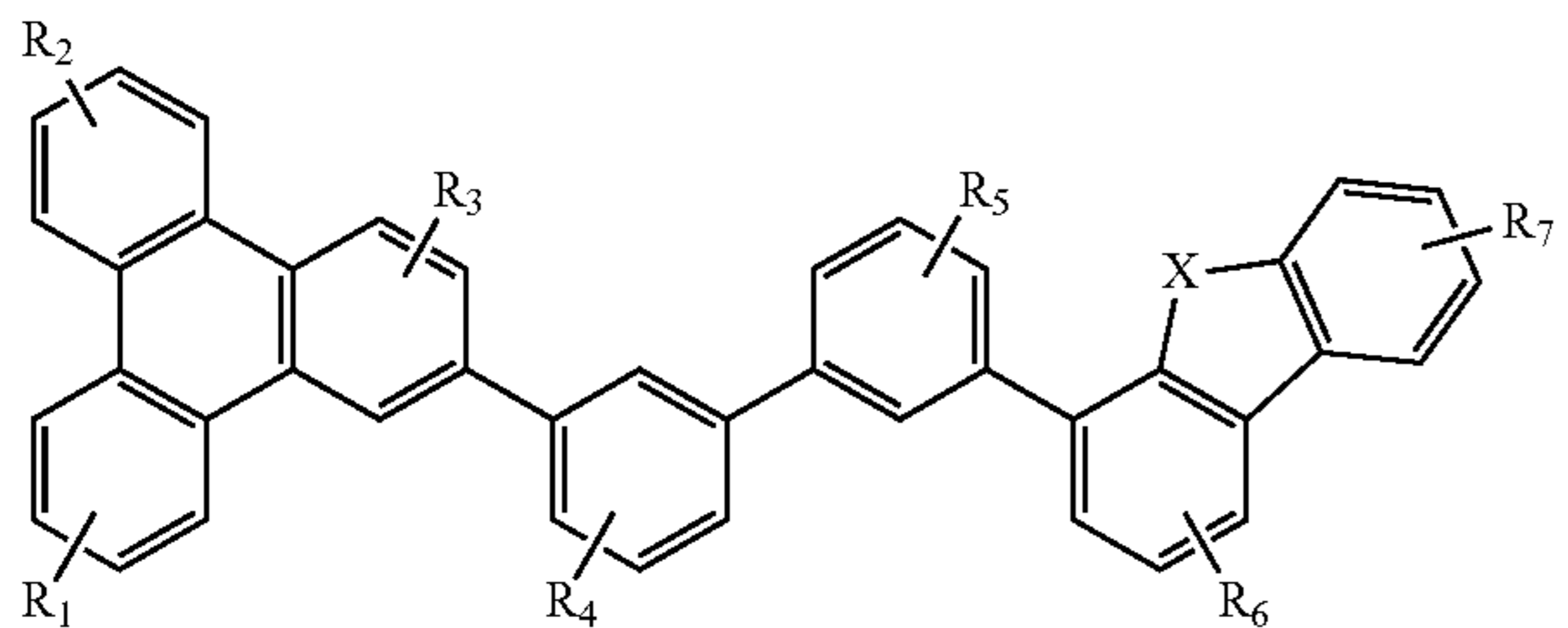
Compound 9G
