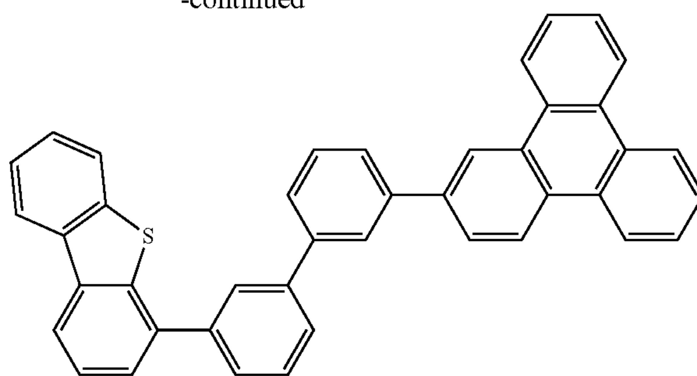
Compound 9S
