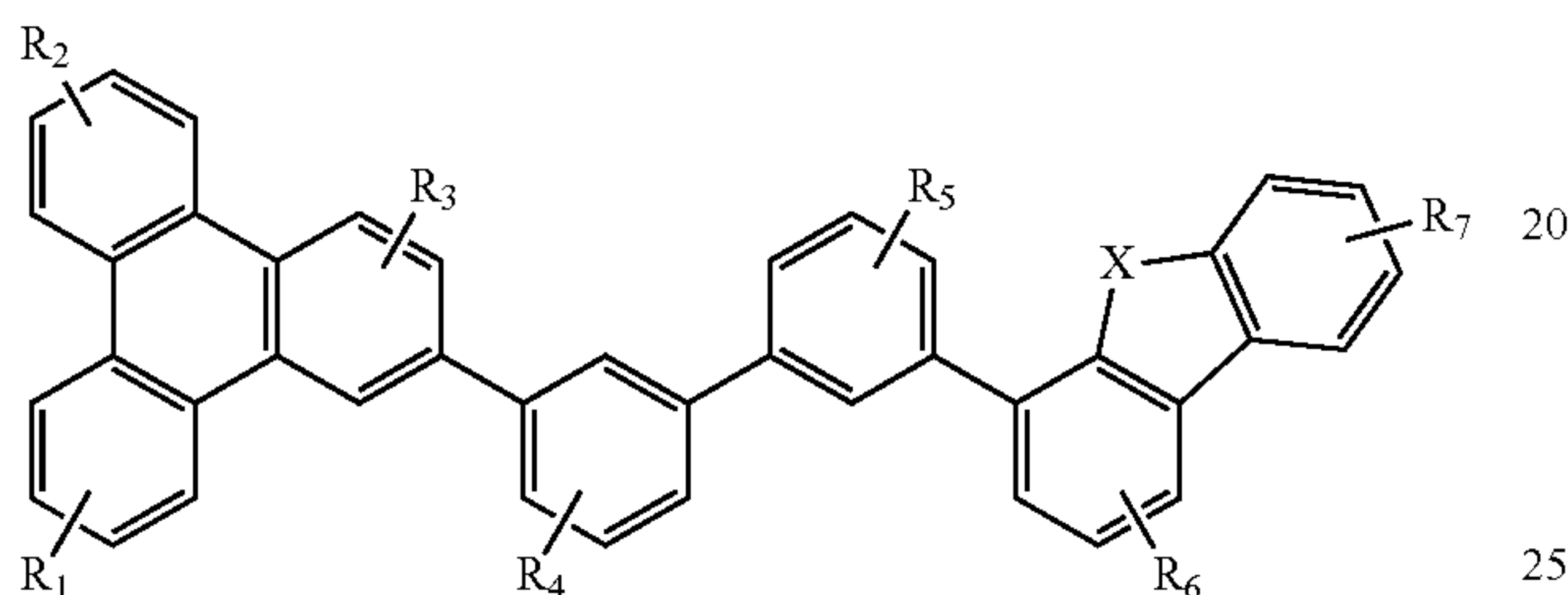
Compound 9G
