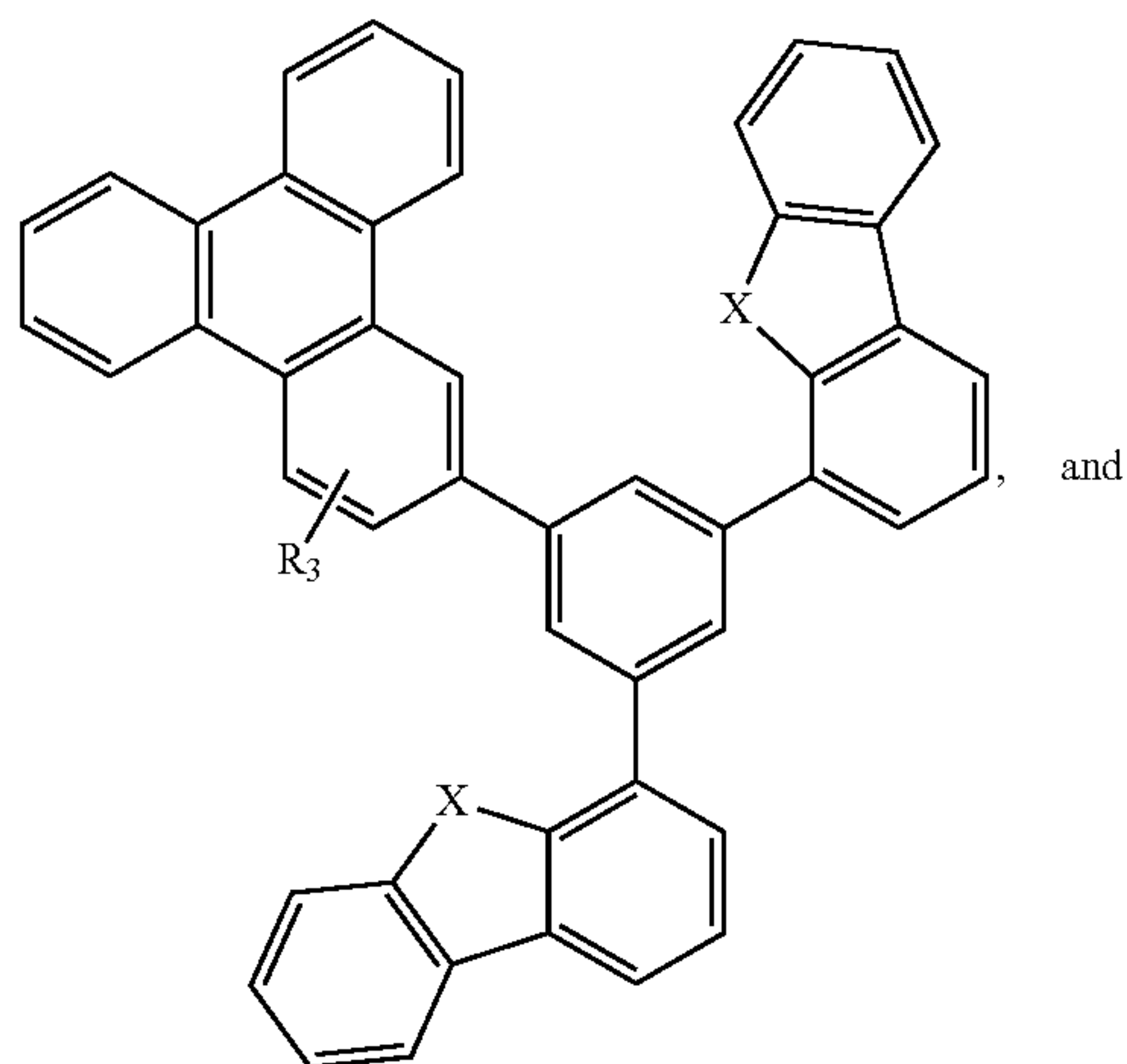
Compound 37
