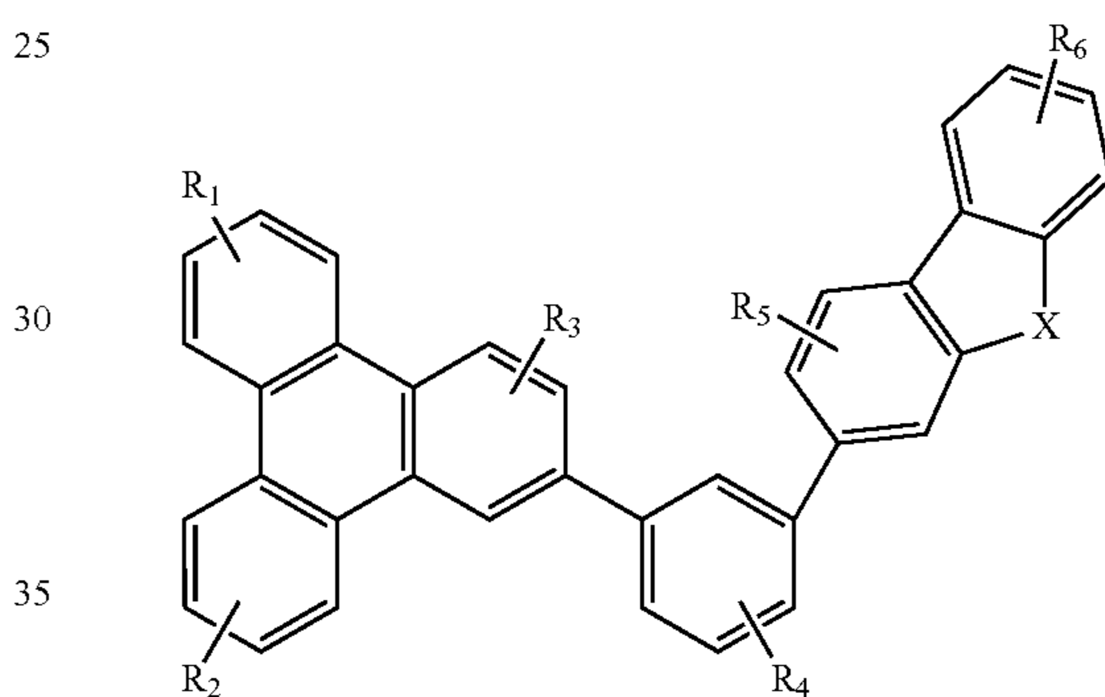
Compound 40G
