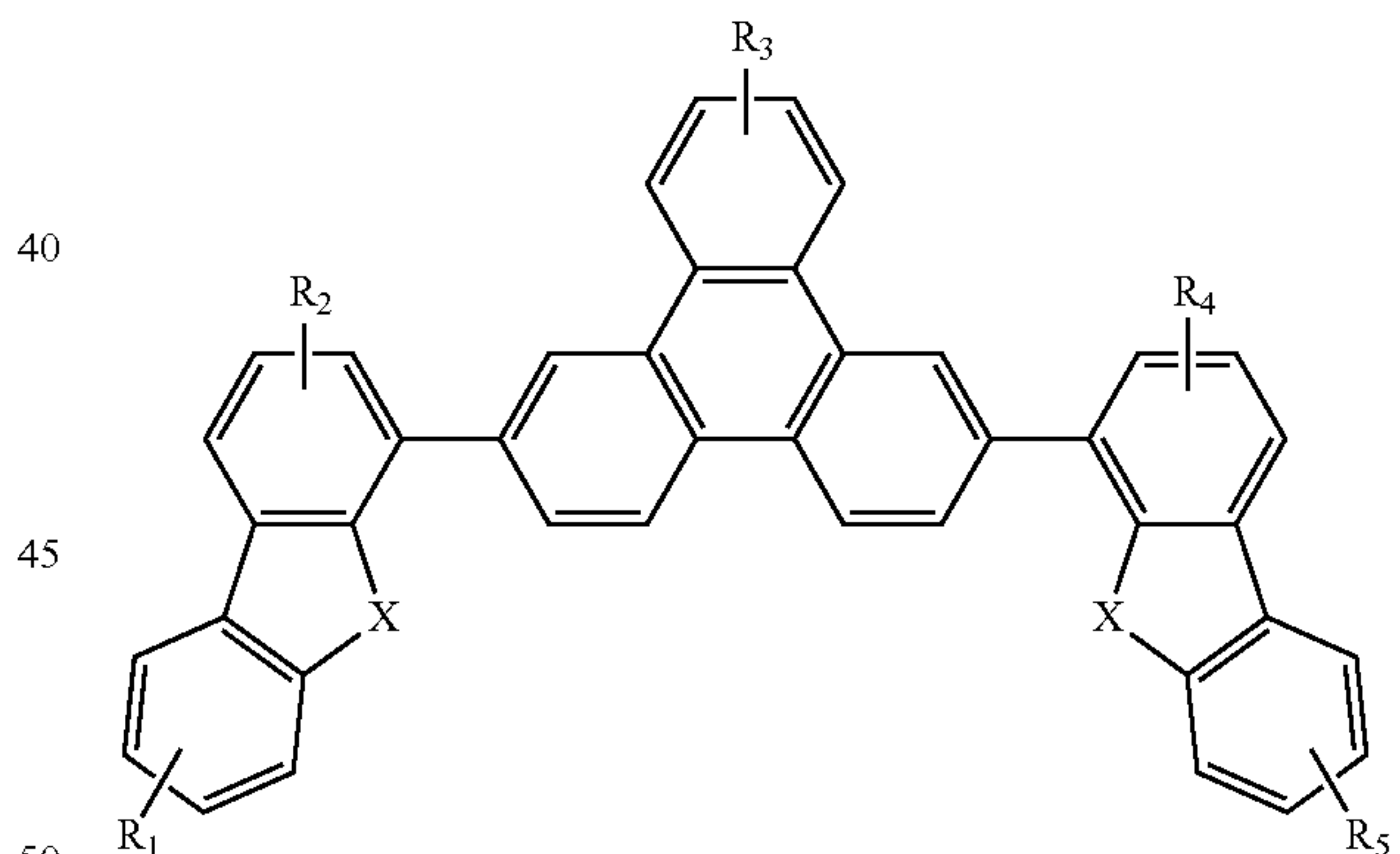
Compound 19G
