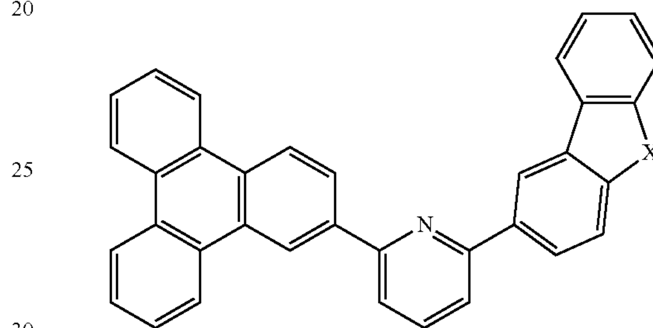
Compound 43
