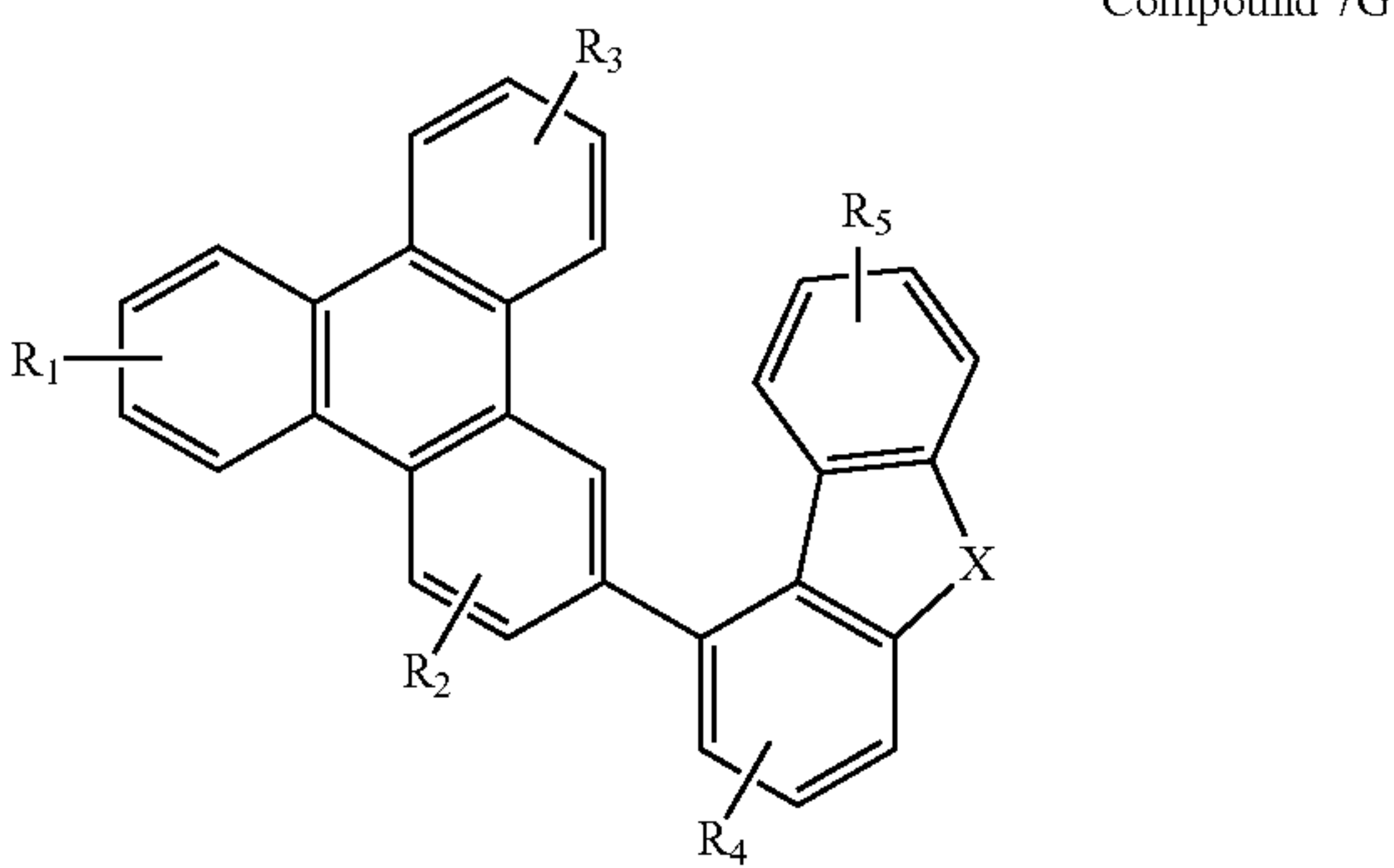
Compound 7
