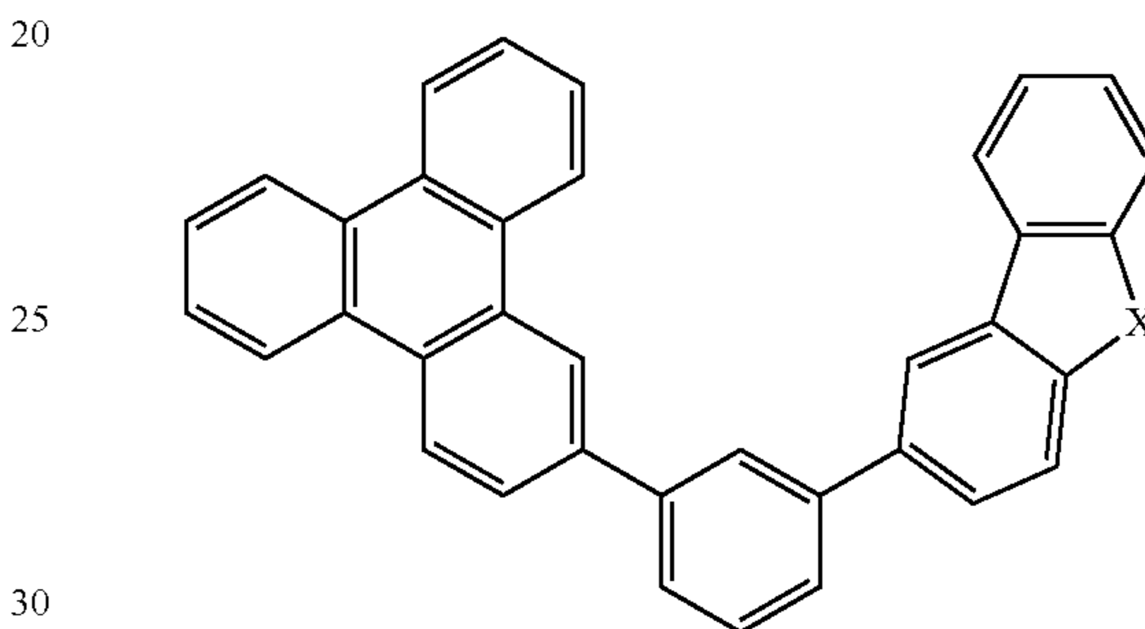
Compound 20
