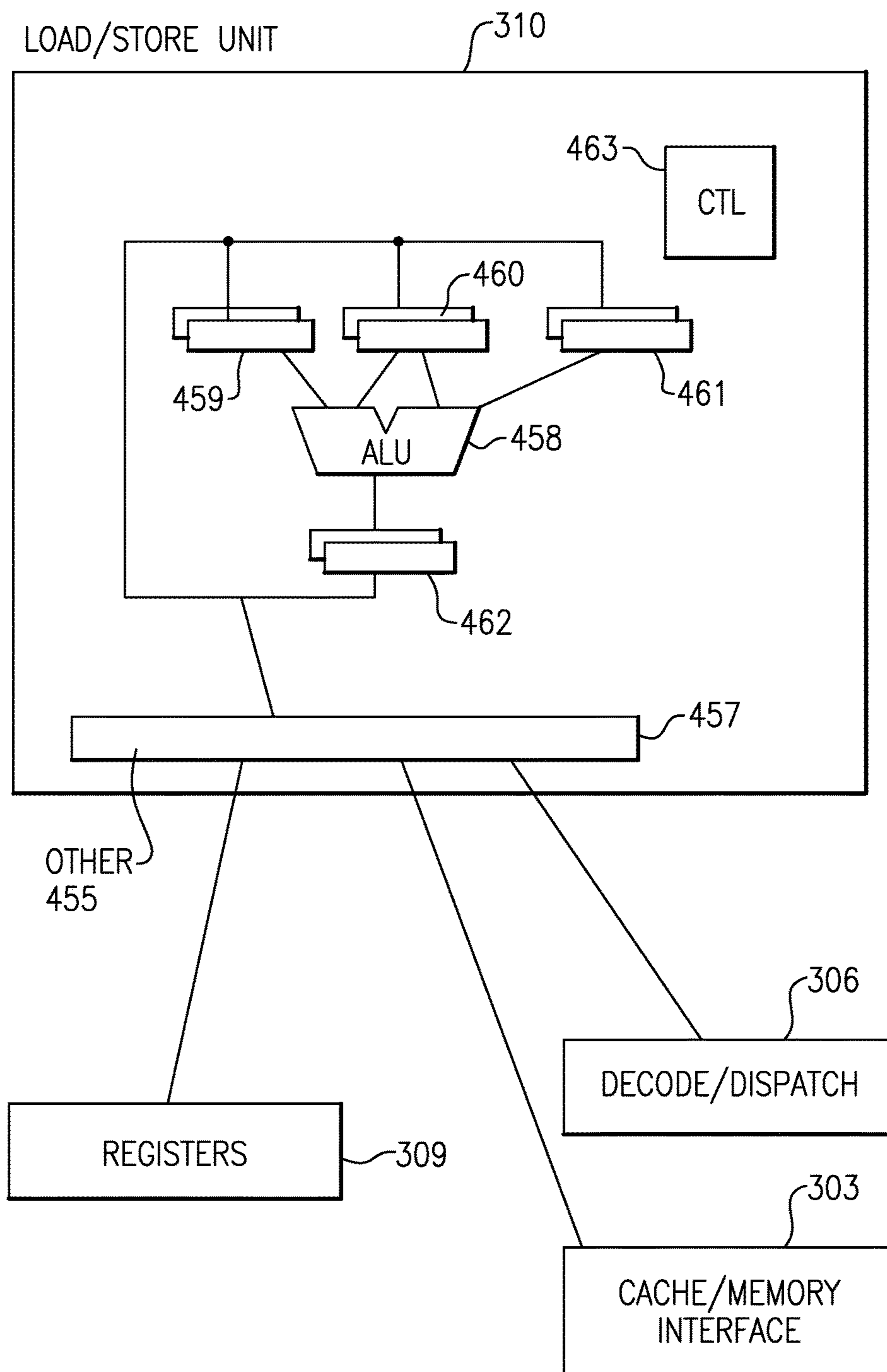
FIG.4C Prior Art
