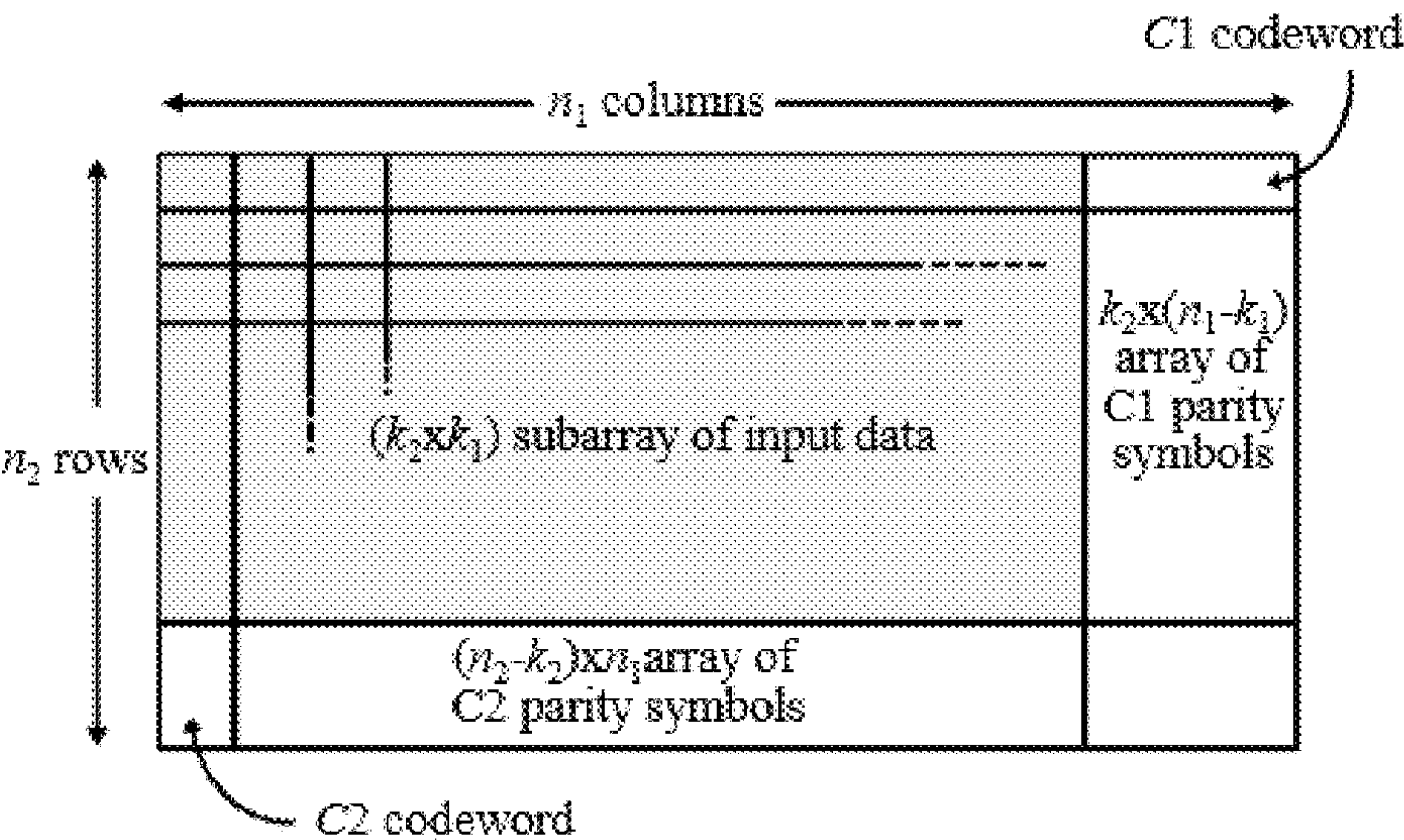
Figure 1(PRIOR ART)
