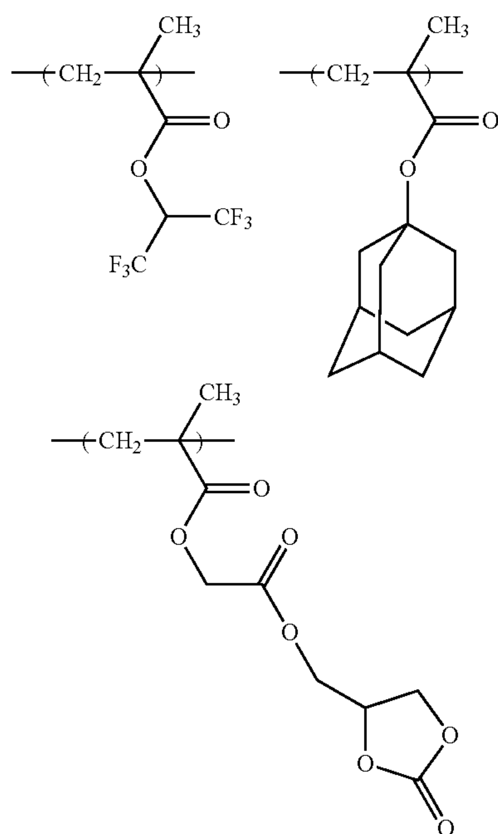
Synthesis Example 6
