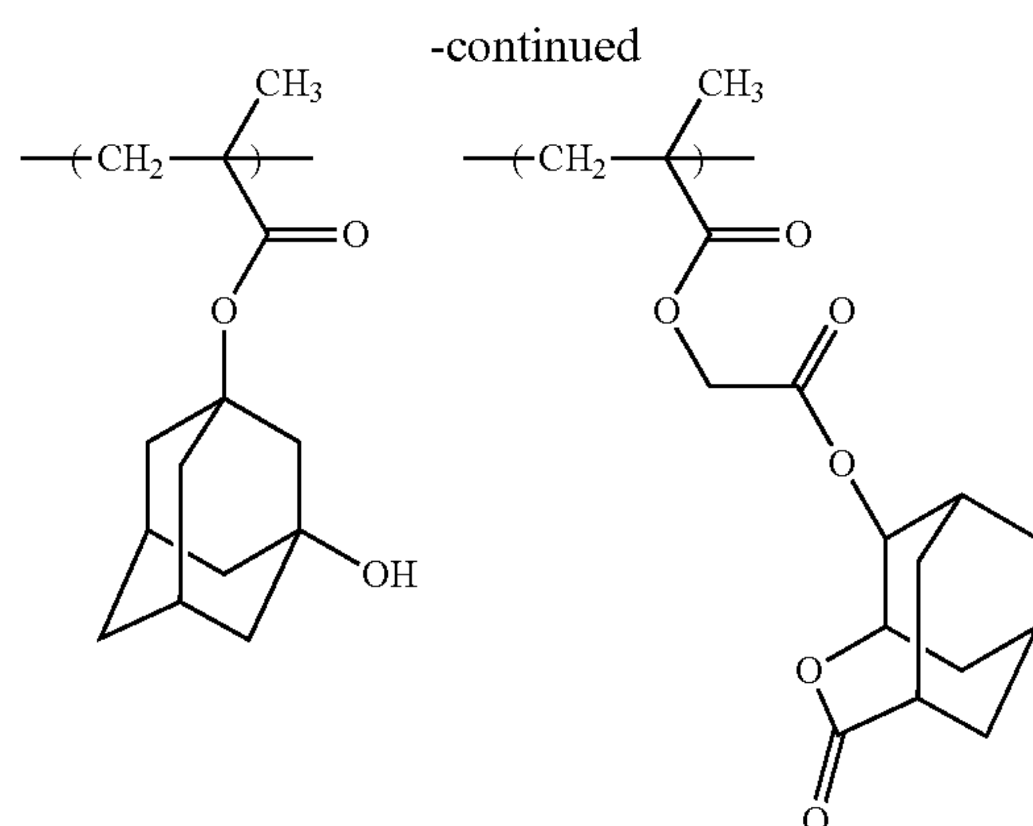
Synthesis Example 8
