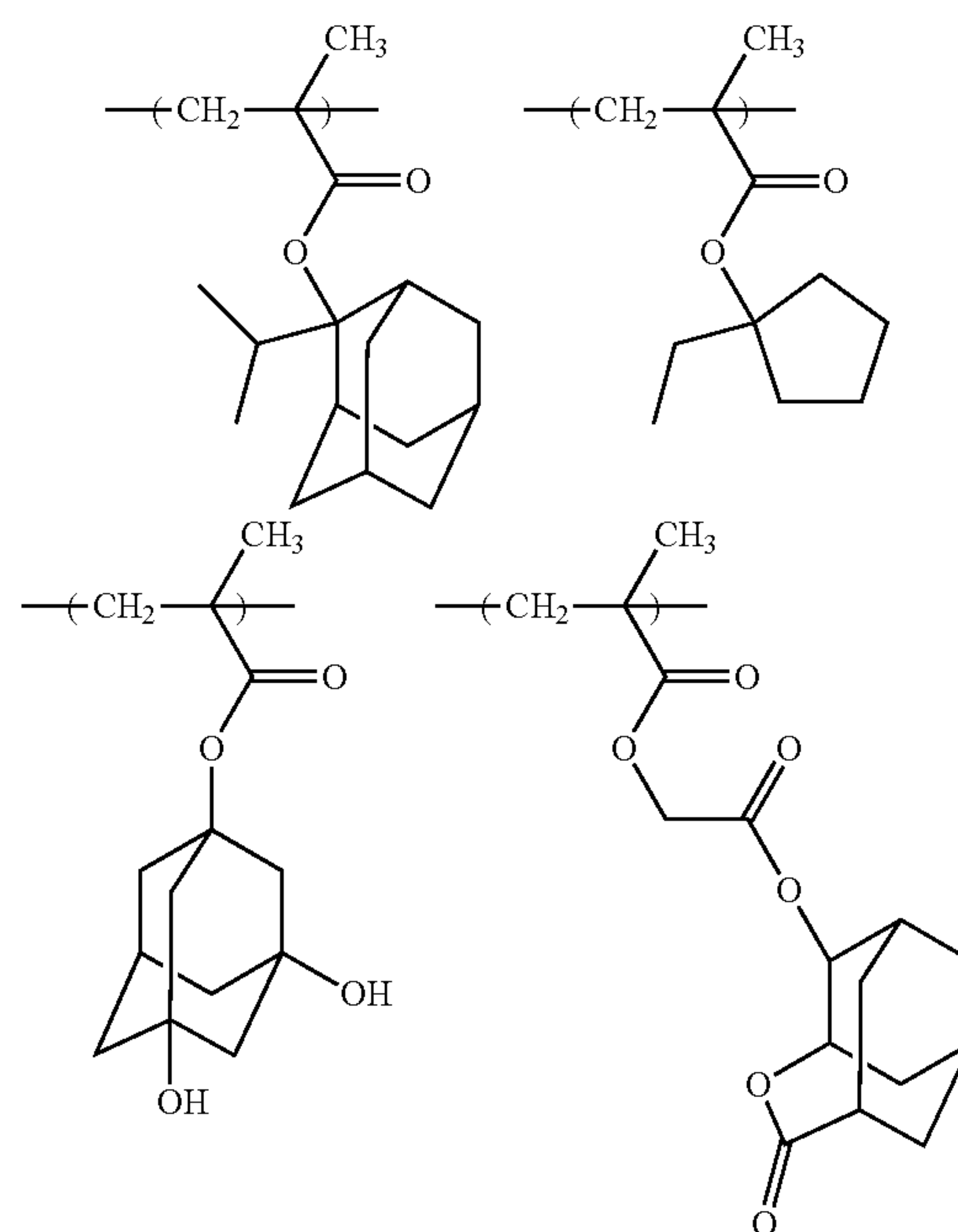
Synthesis Example 7
