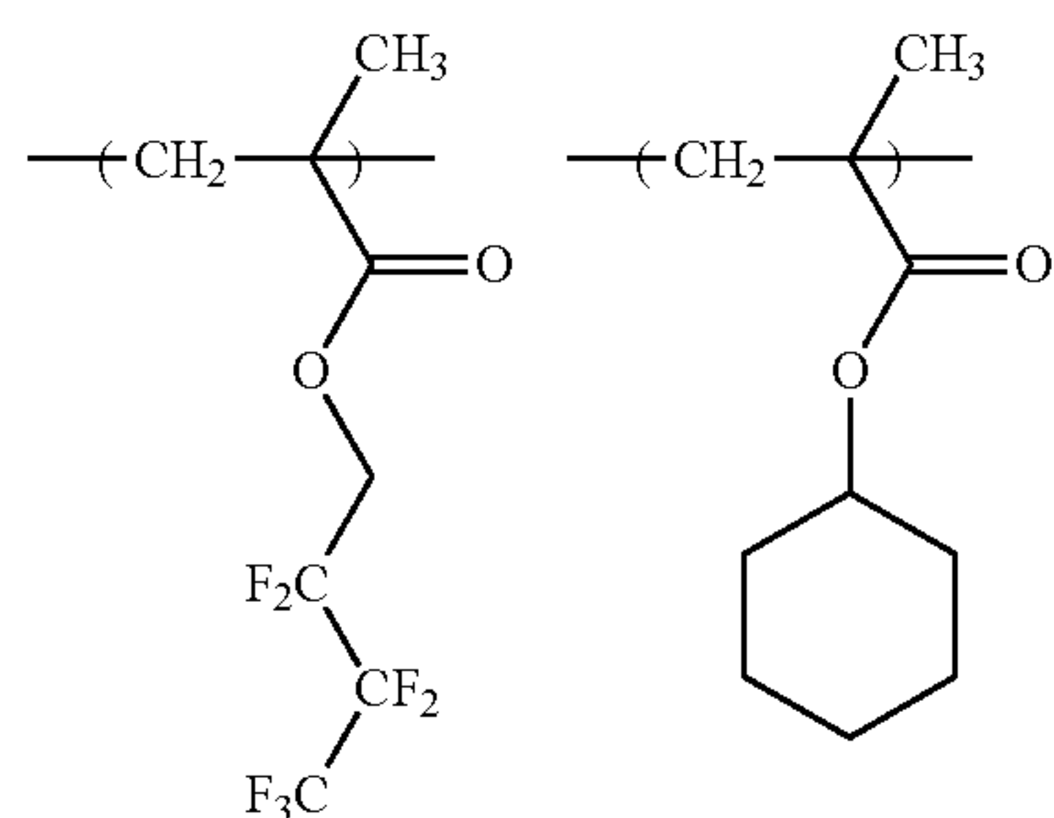
Synthesis Example 9
