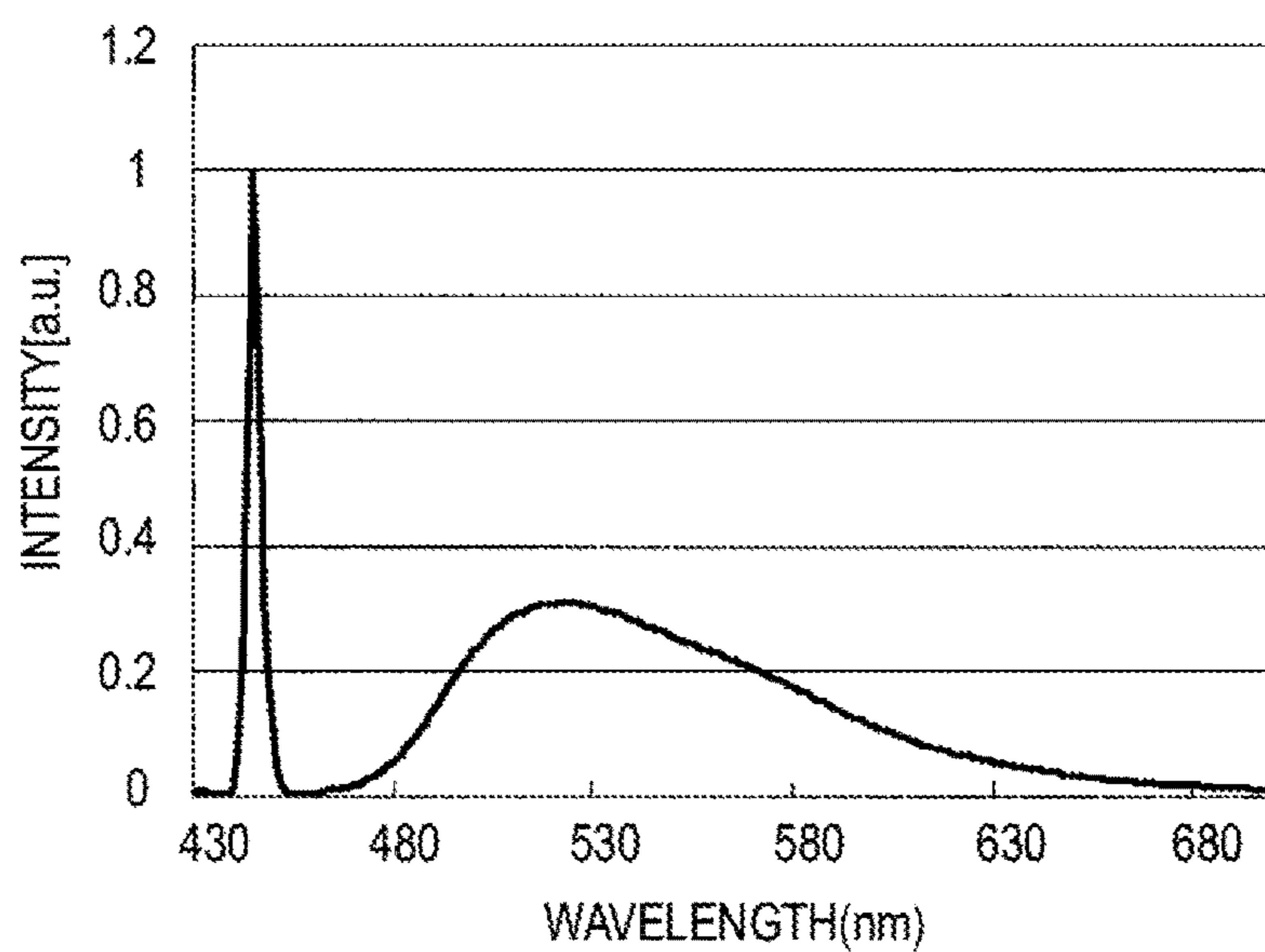
SPECTRAL CHARACTERISTIC OF EMITTED LIGHT
