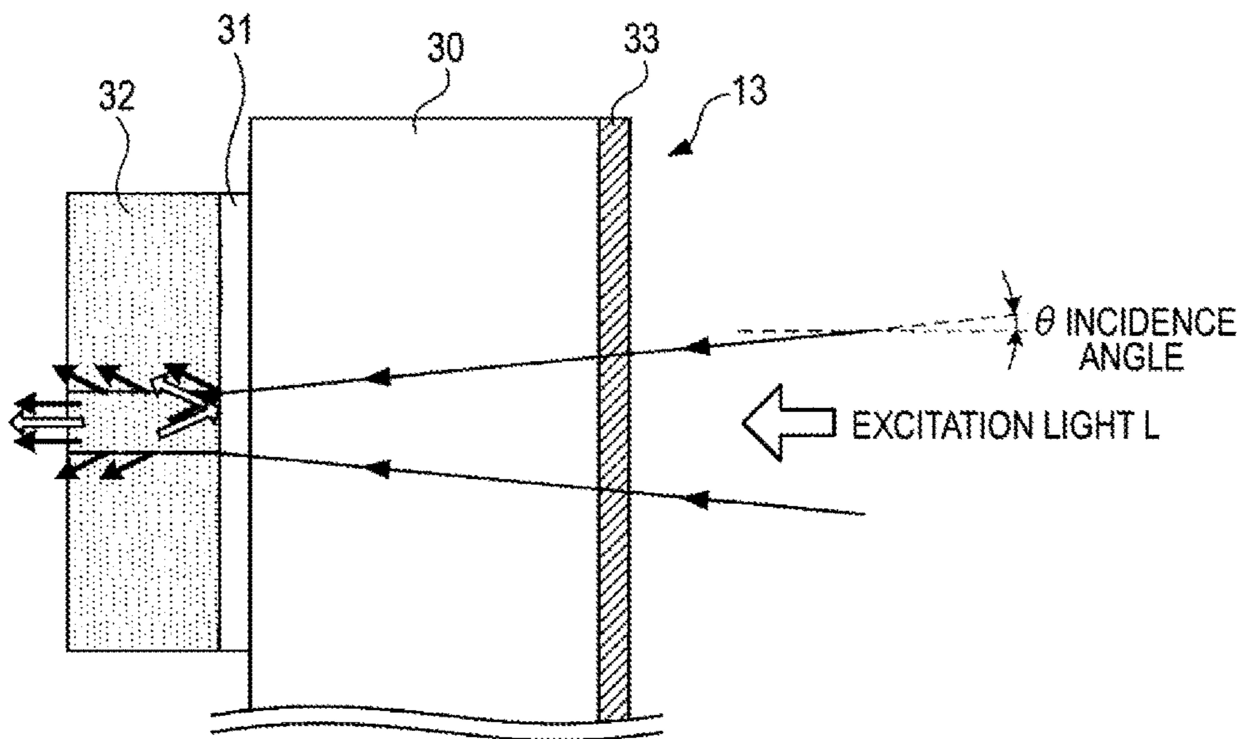
LIGHT EMITTING OPERATION OF ILLUMINATION DEVICE
