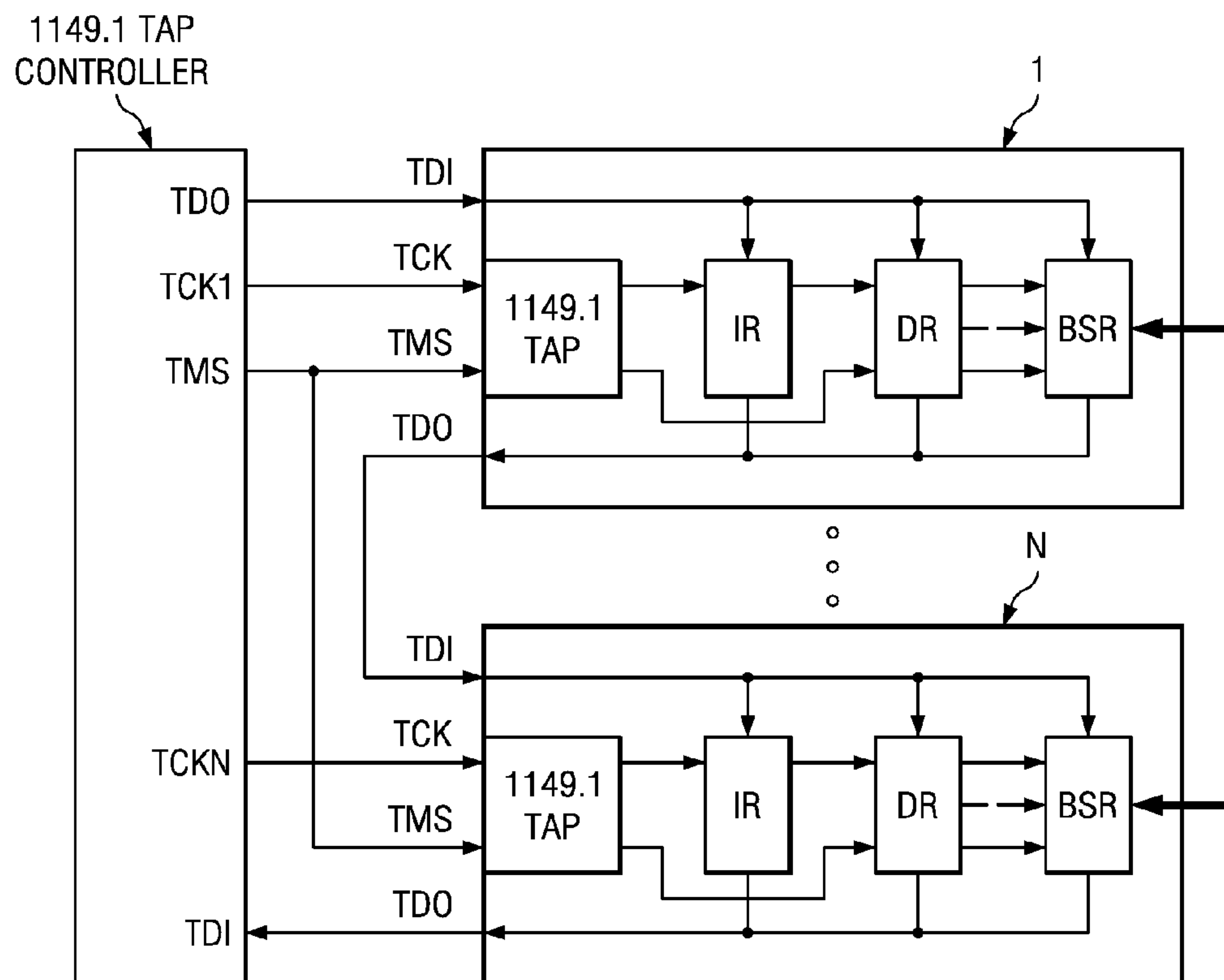
FIG. 5 (PRIOR ART)
