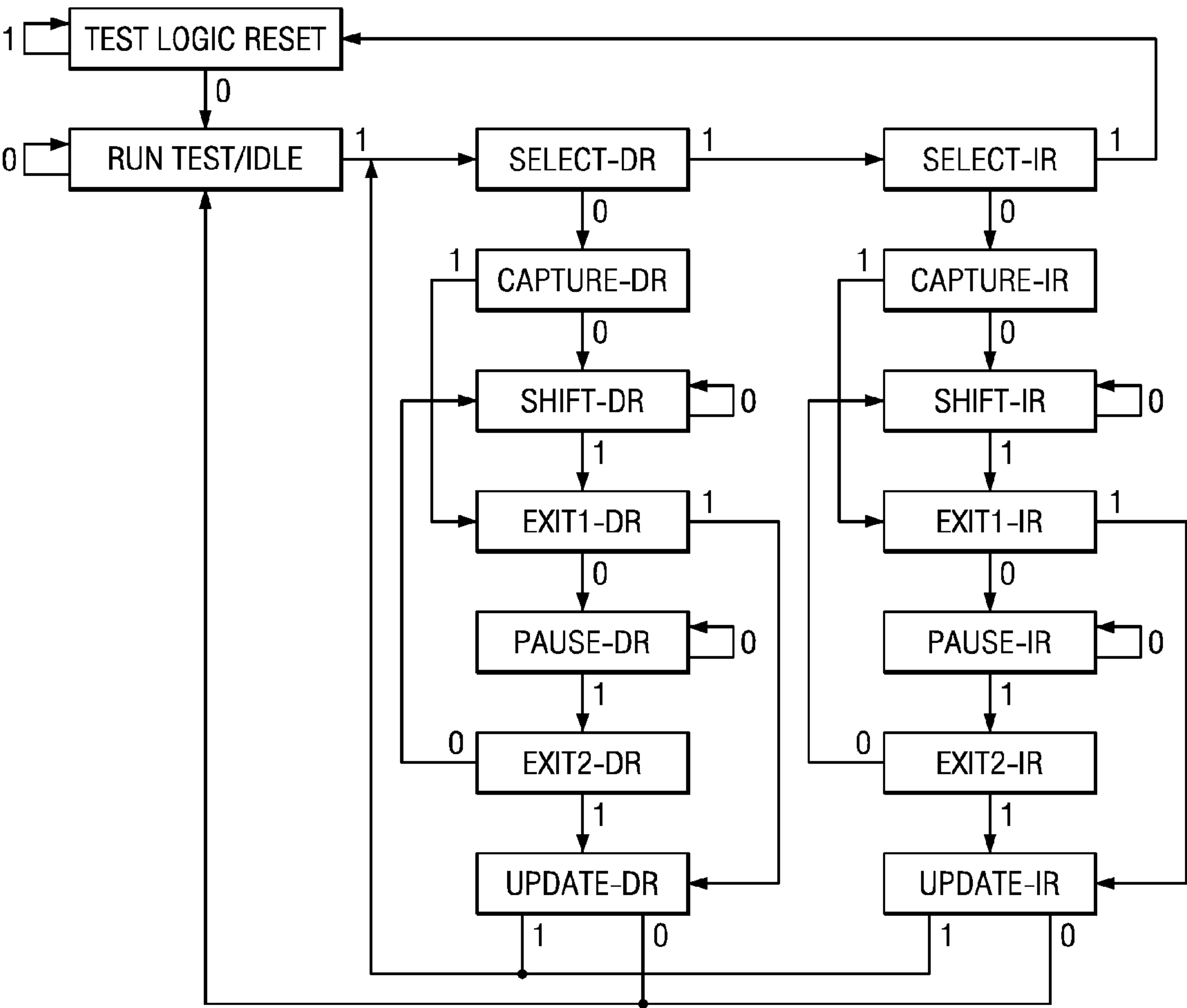
FIG. 2 (PRIOR ART)
