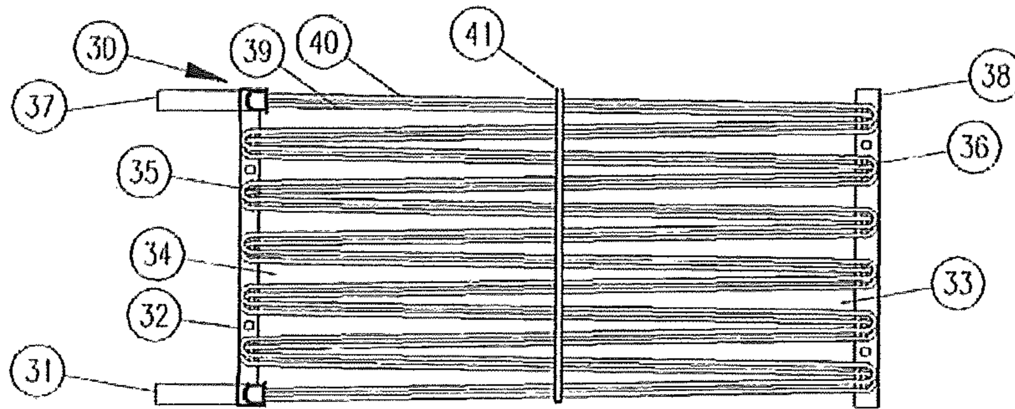
Figure 2 PRIOR ART
