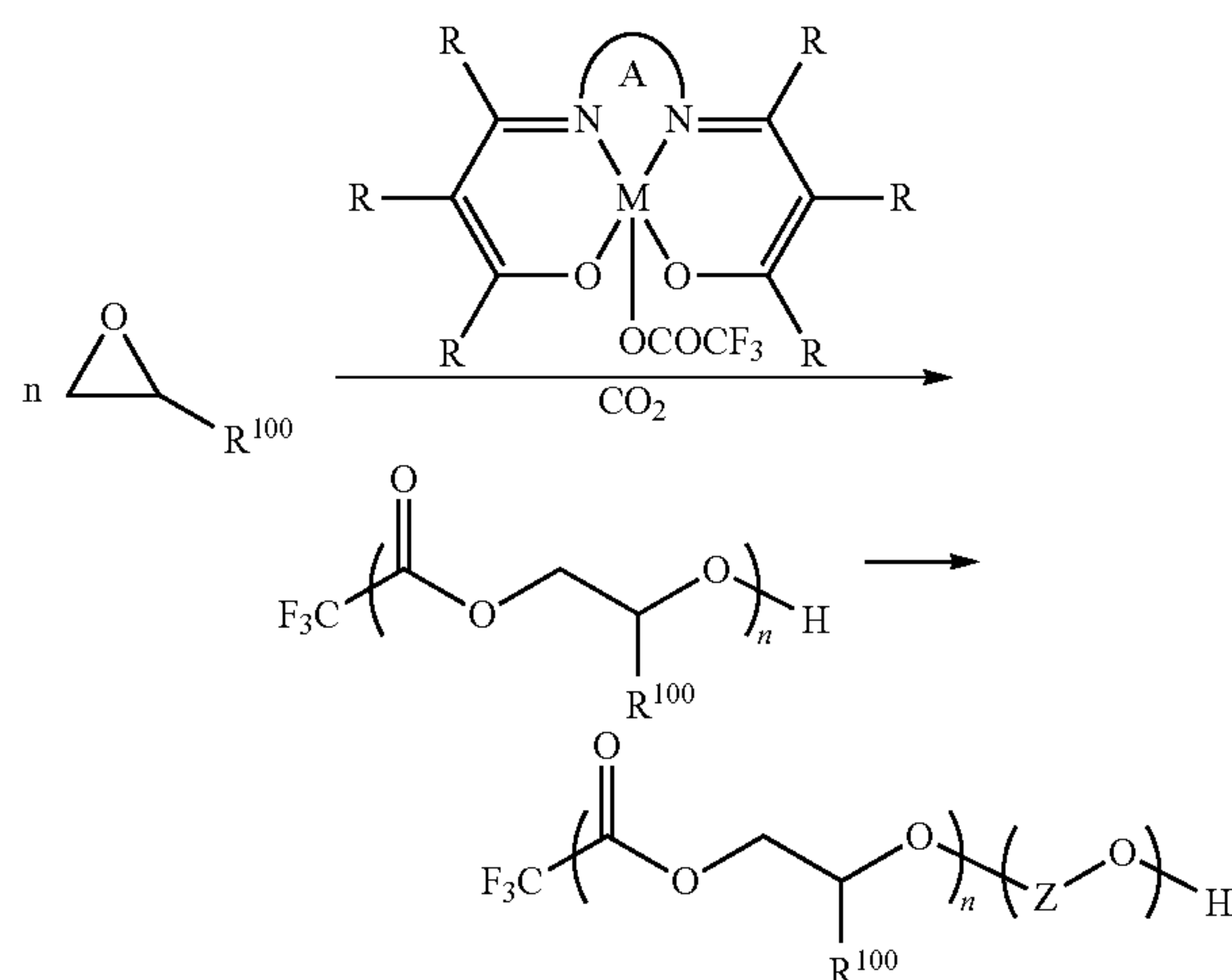
Scheme 5
