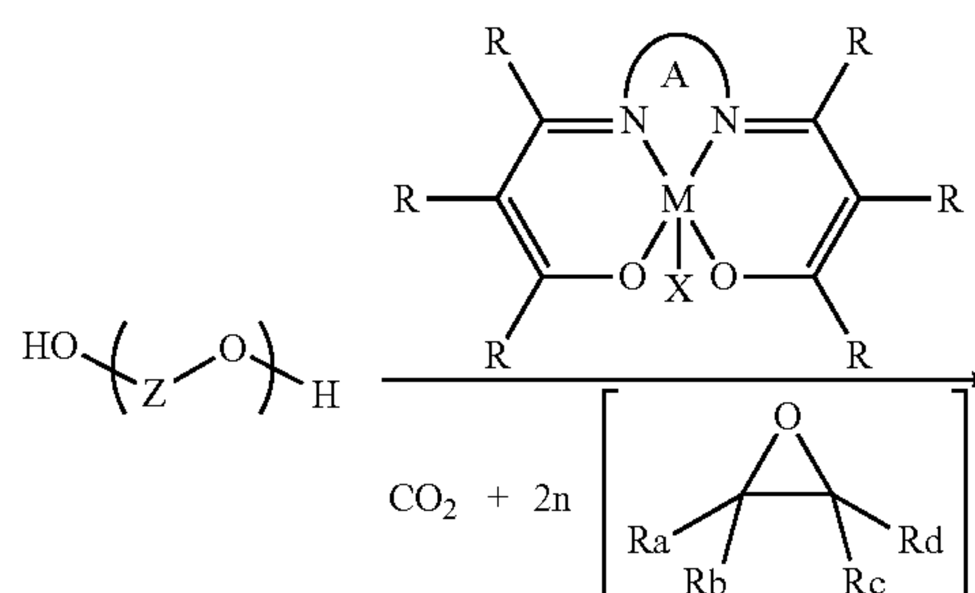
Scheme 3
