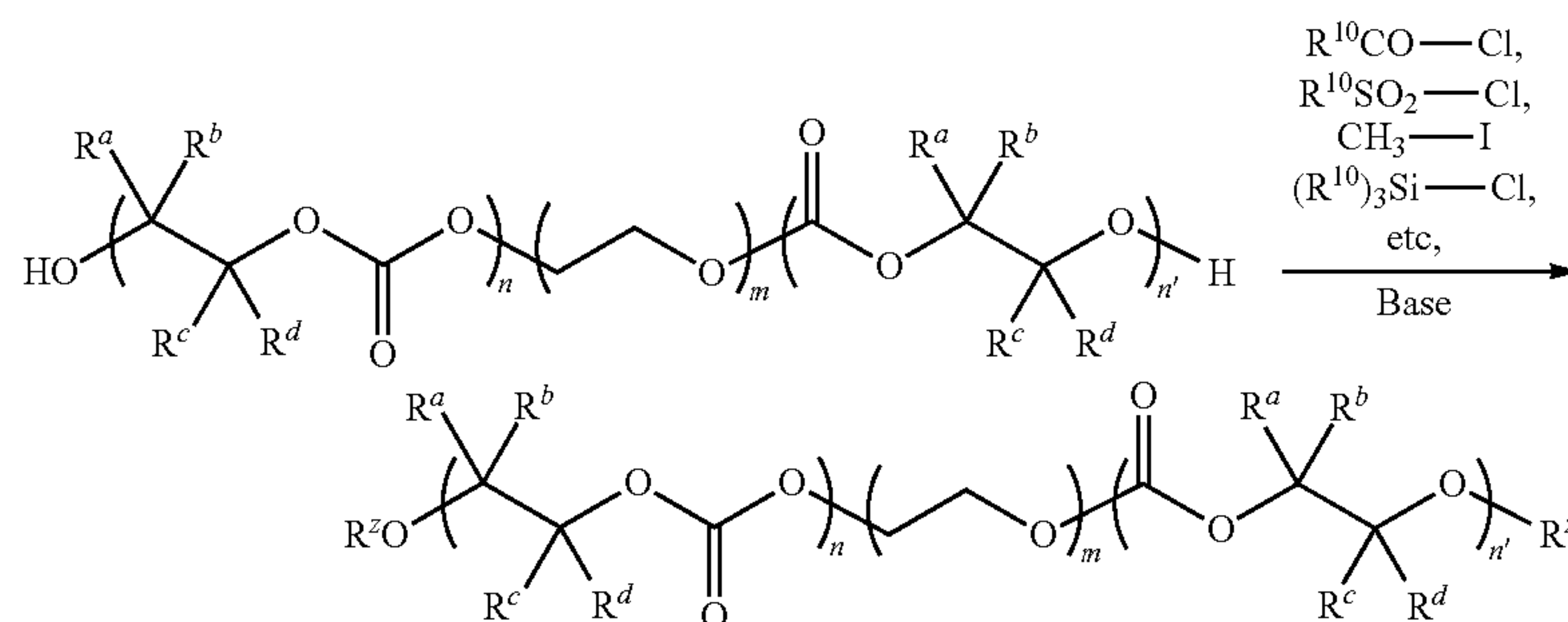
Scheme 4
