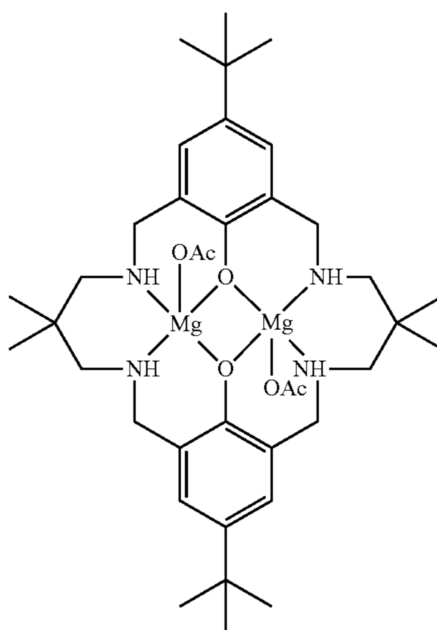
[\text{L}^1\text{Mg}_2(\text{OAc})_2]
