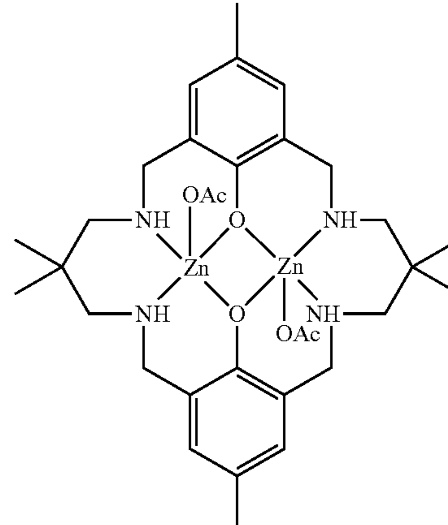
[\text{L}^2\text{Zn}_2(\text{OAc})_2]
