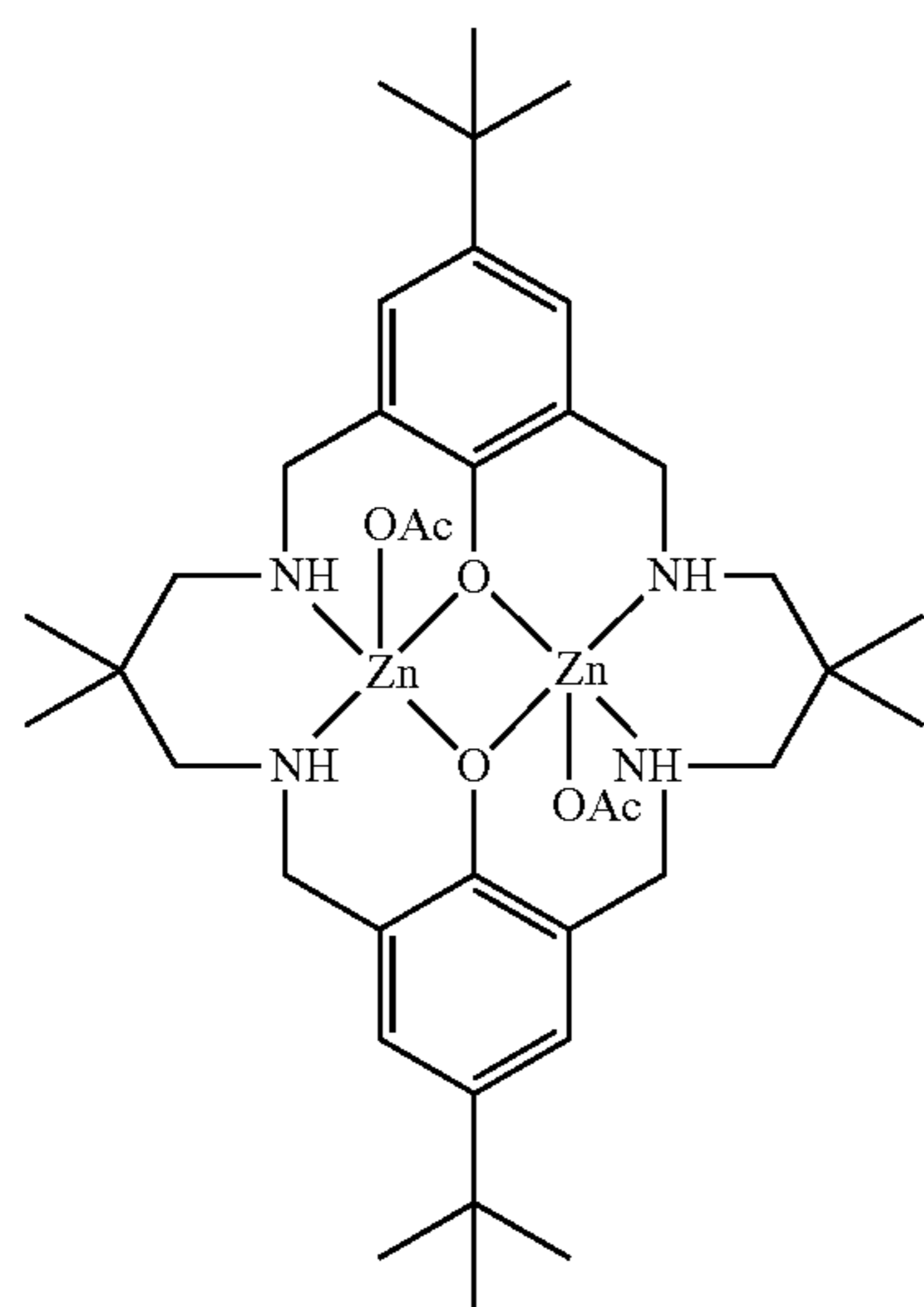
[\text{L}^1\text{Zn}_2(\text{OAc})_2]
