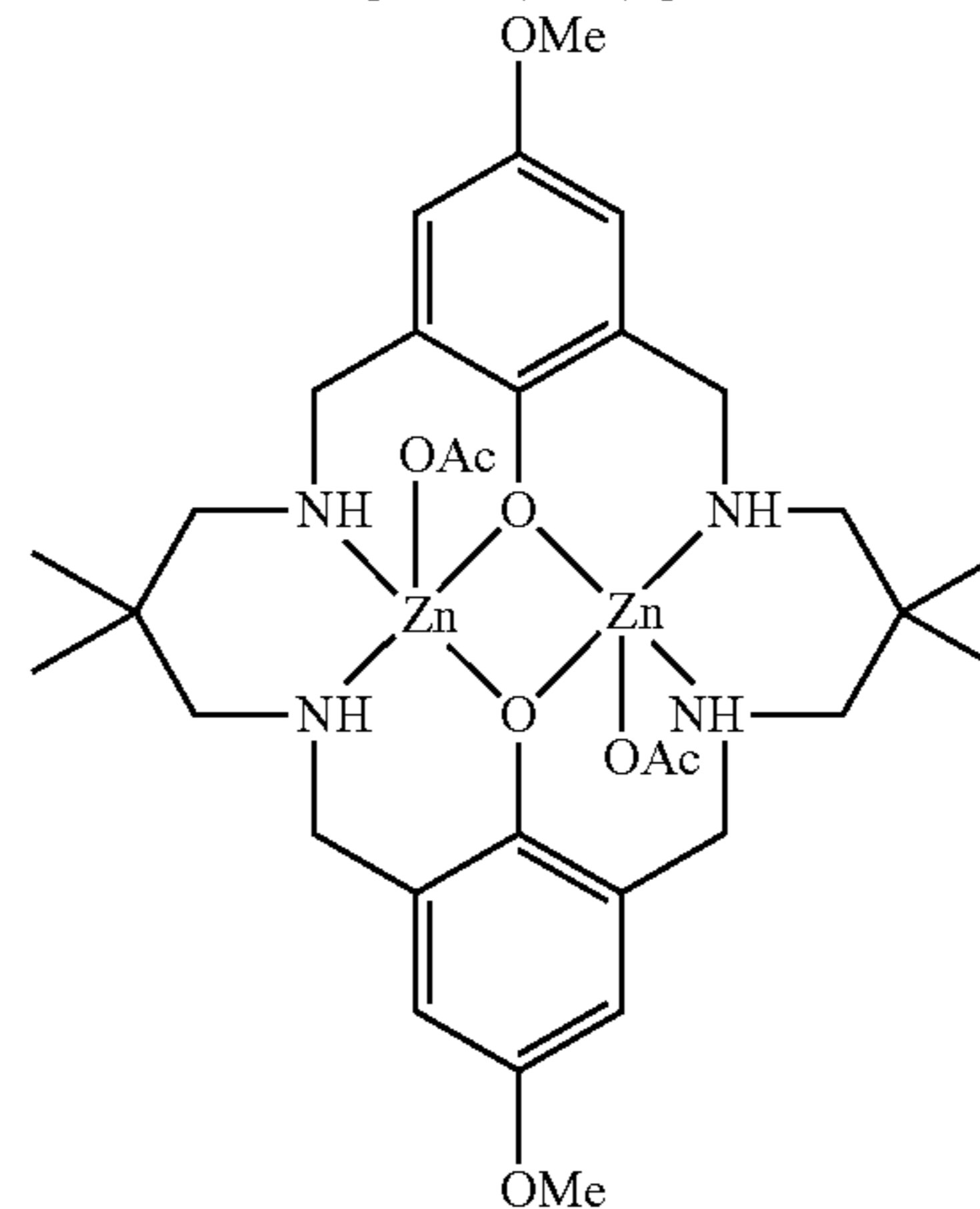
[\text{L}^3\text{Zn}_2(\text{OAc})_2]
