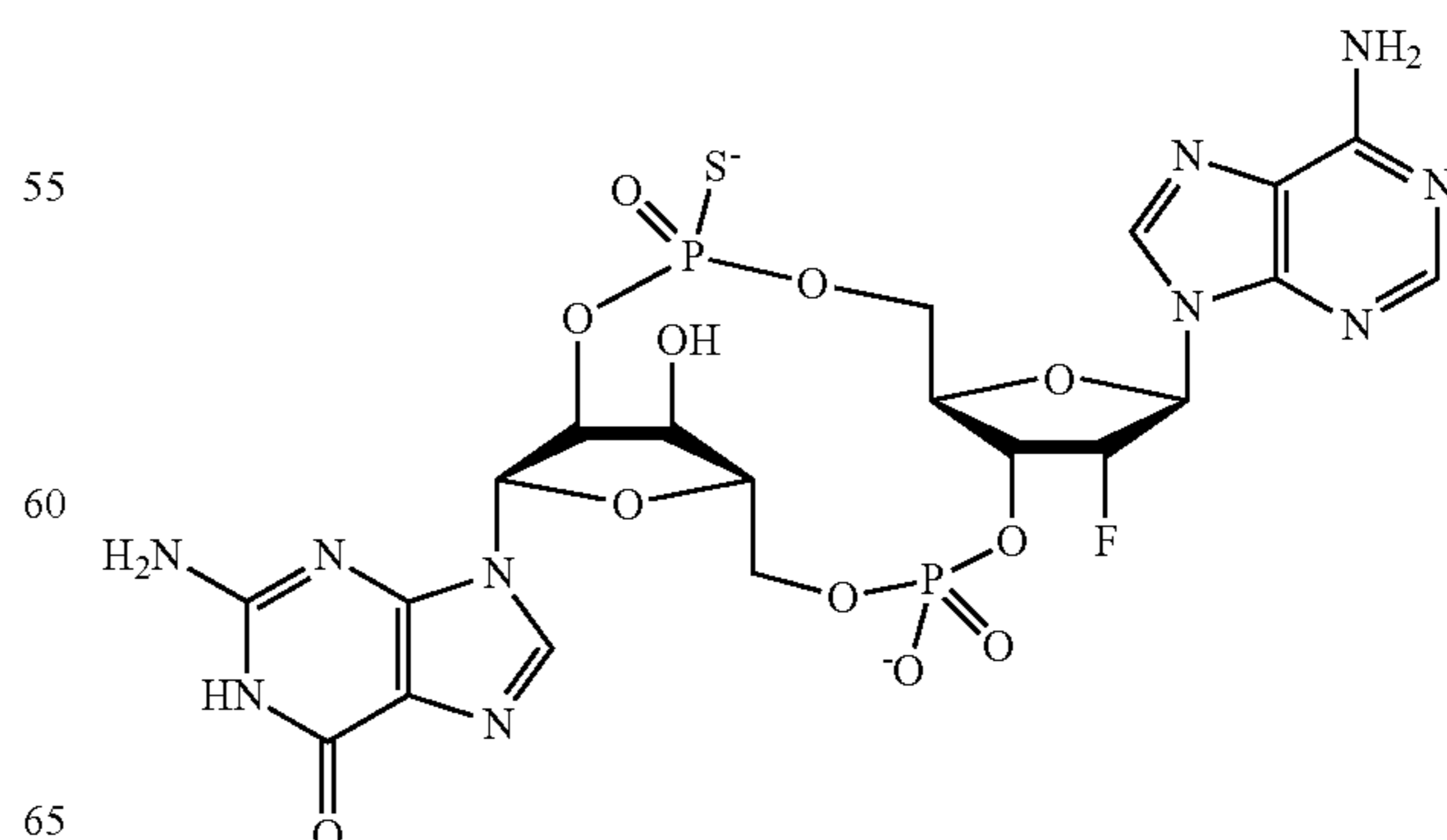
Compound 28
