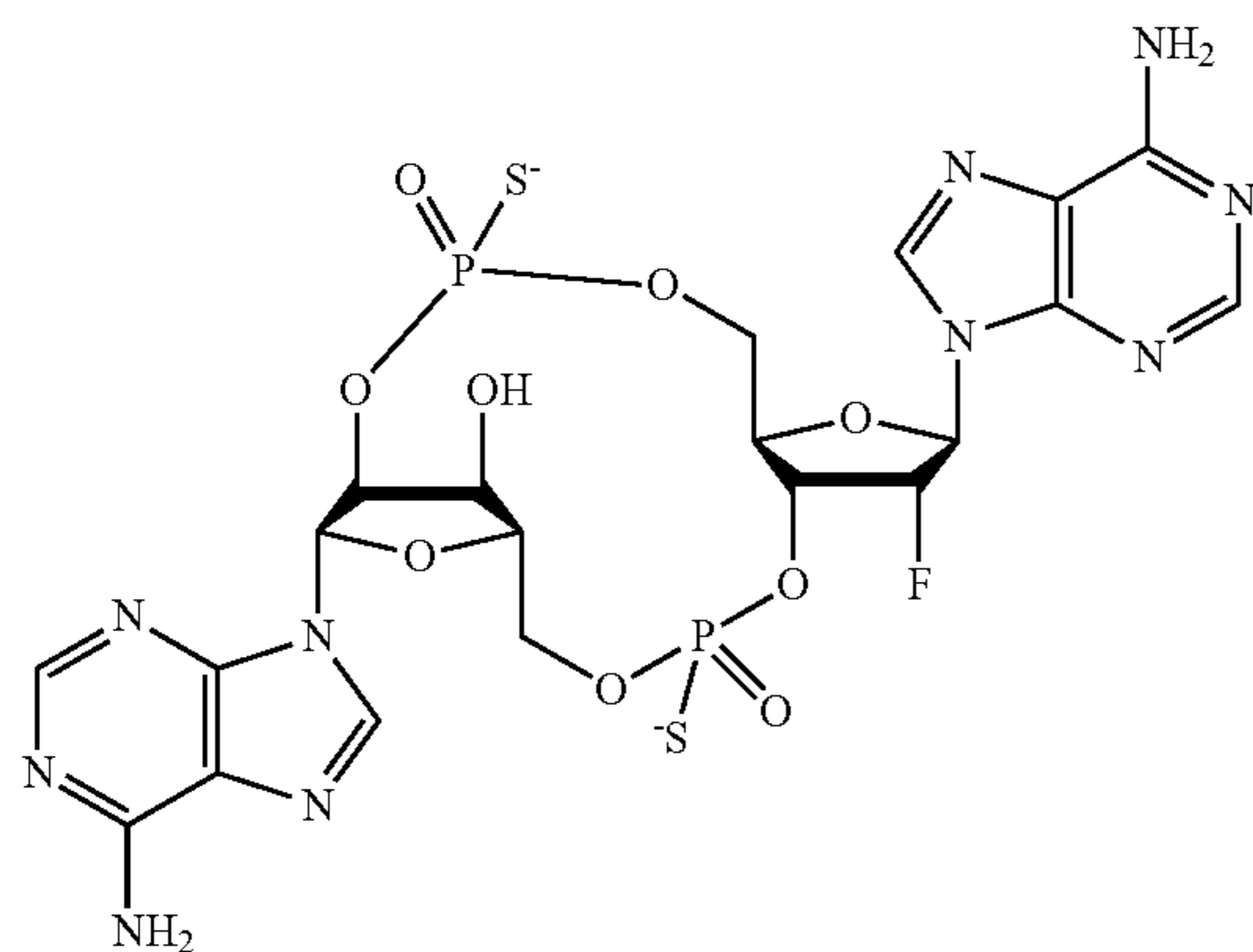
1a-Isomer 1 1b-Isomer 2
