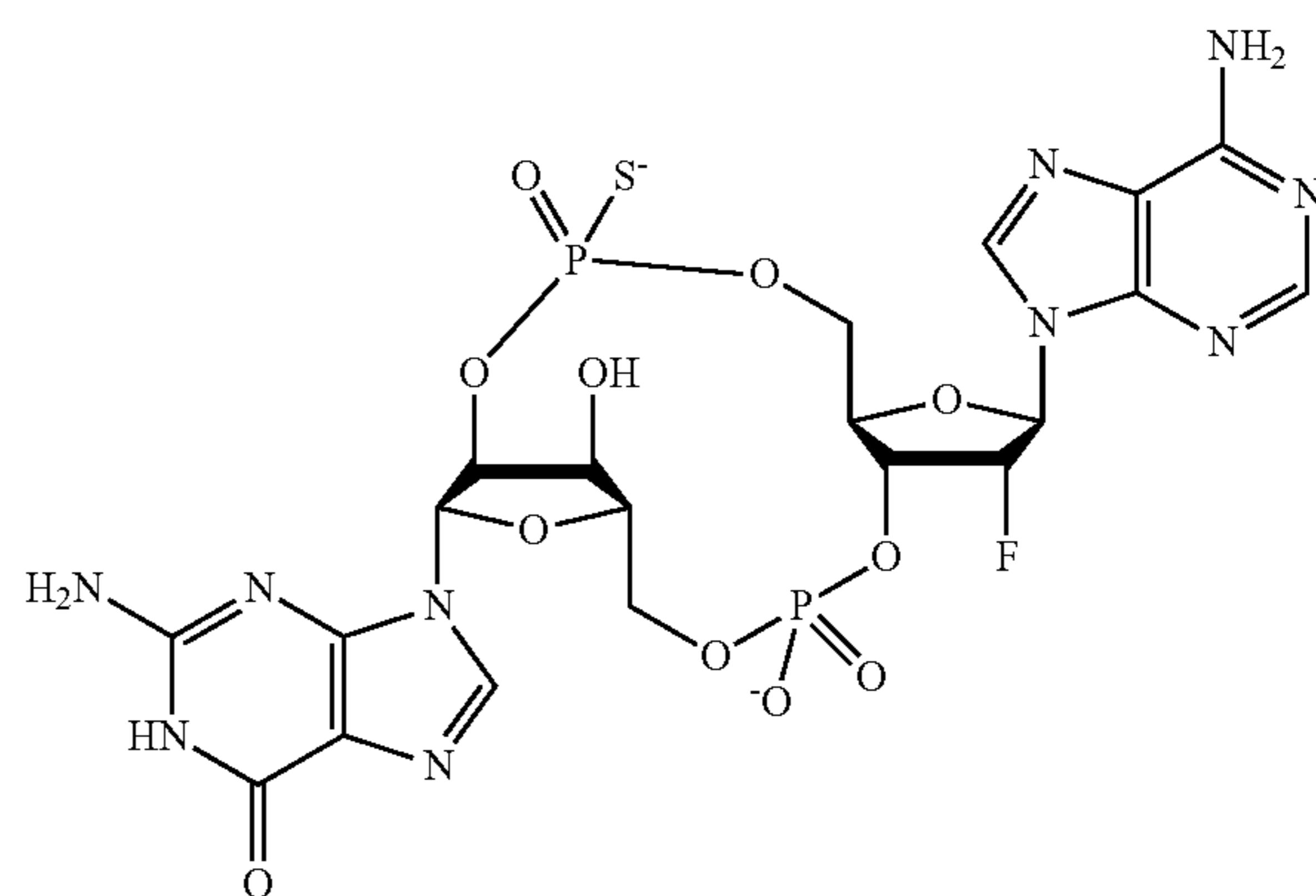
28a-Isomer 1 28b-Isomer 2
