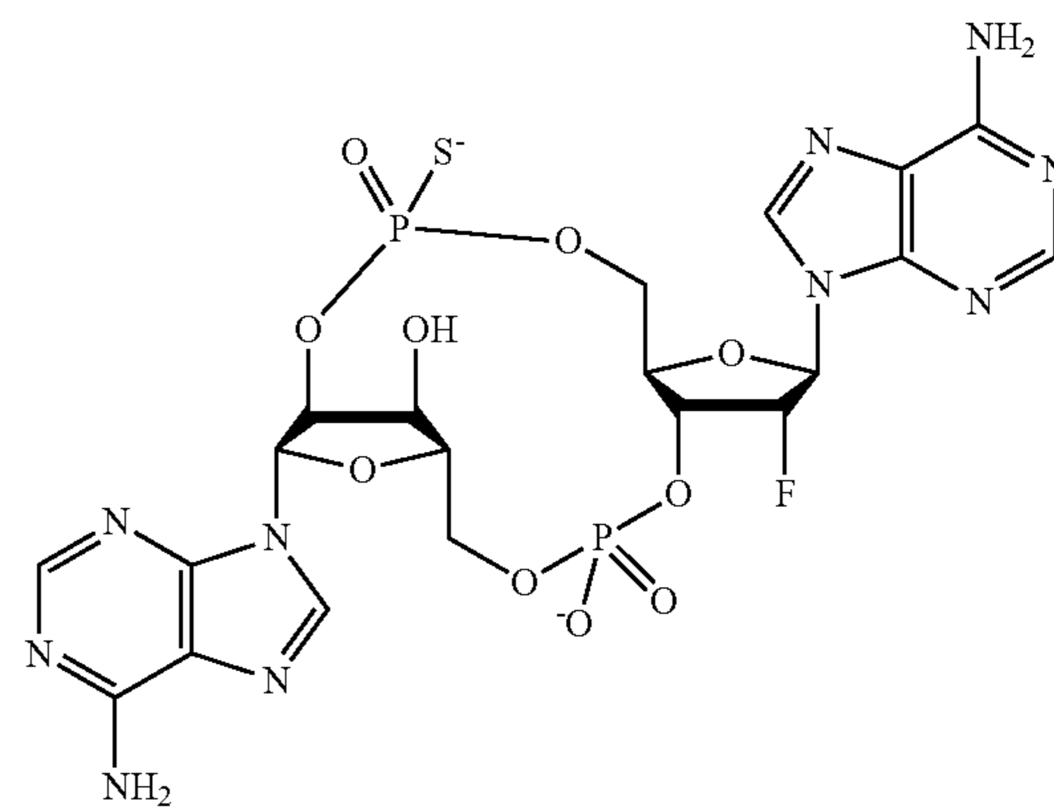
2a-Isomer 1 2b-Isomer 2
