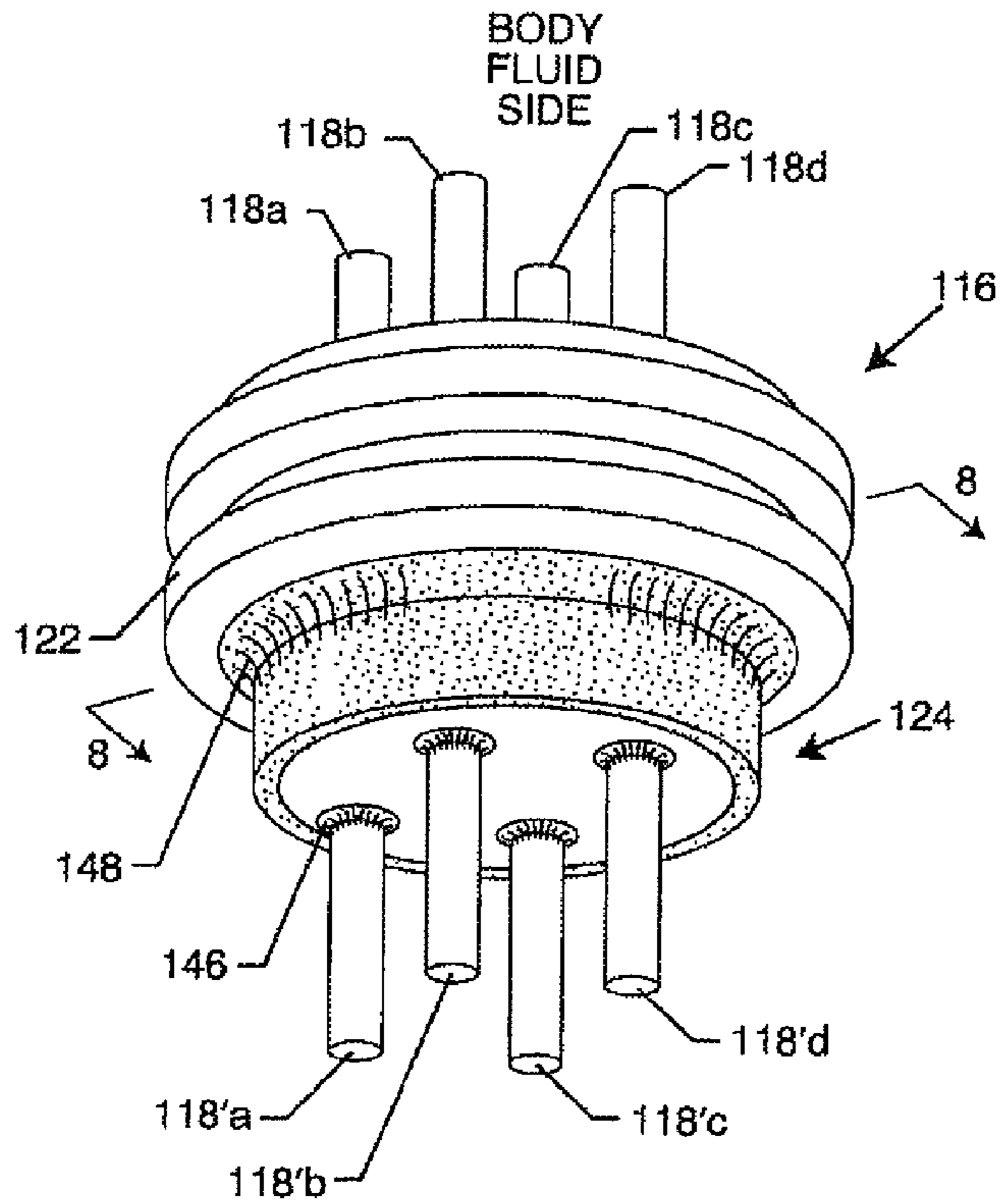
FIG. 7 PRIOR ART
