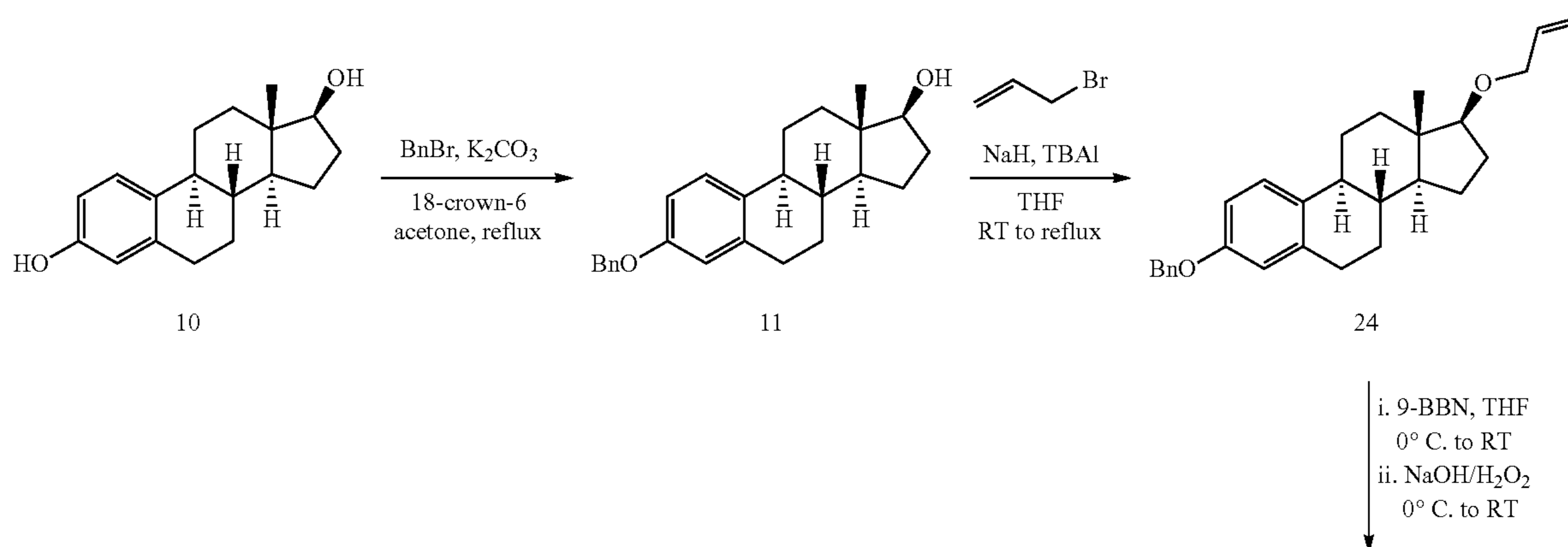
Scheme 1
