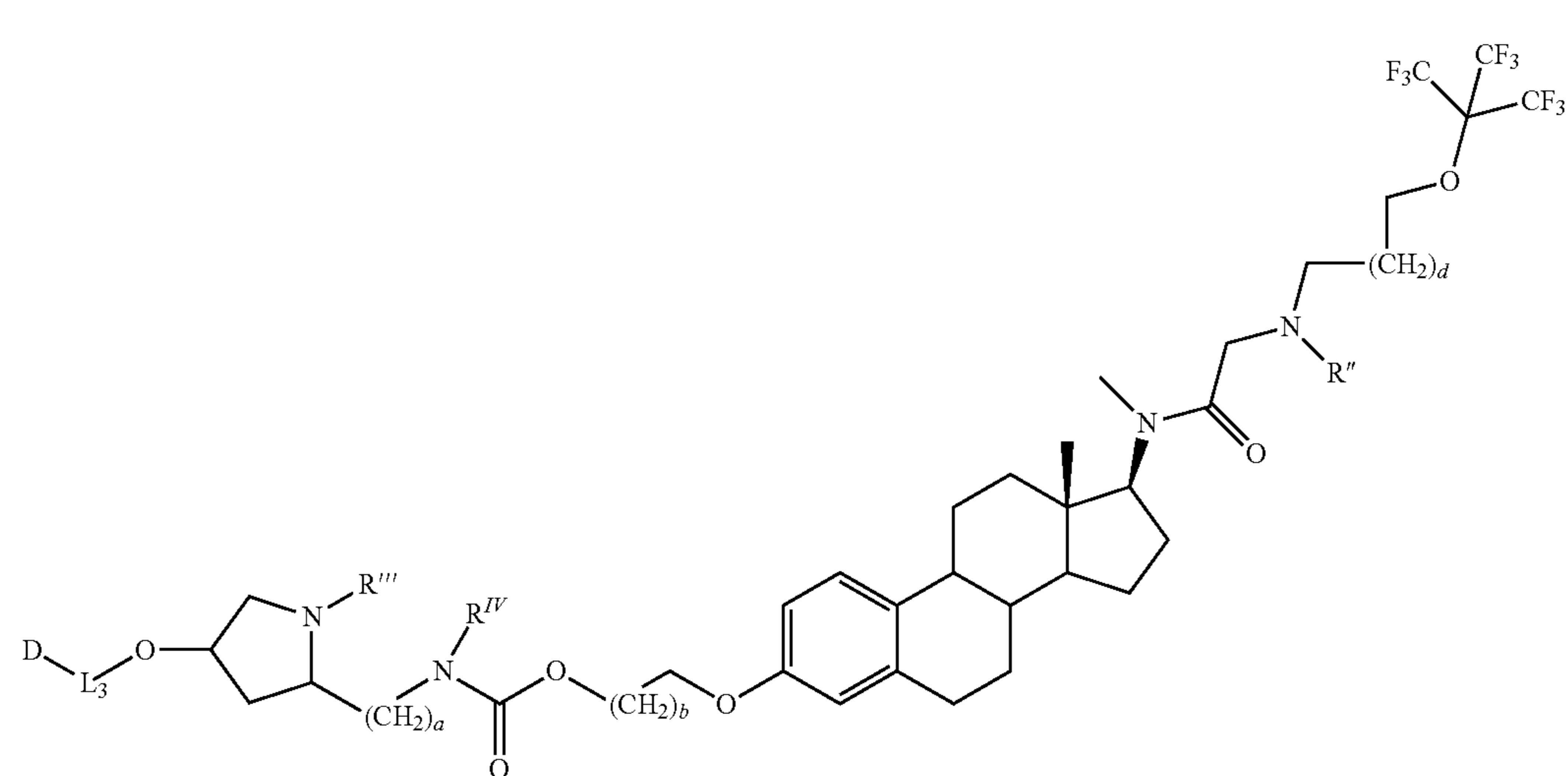
Formula (XIb)
