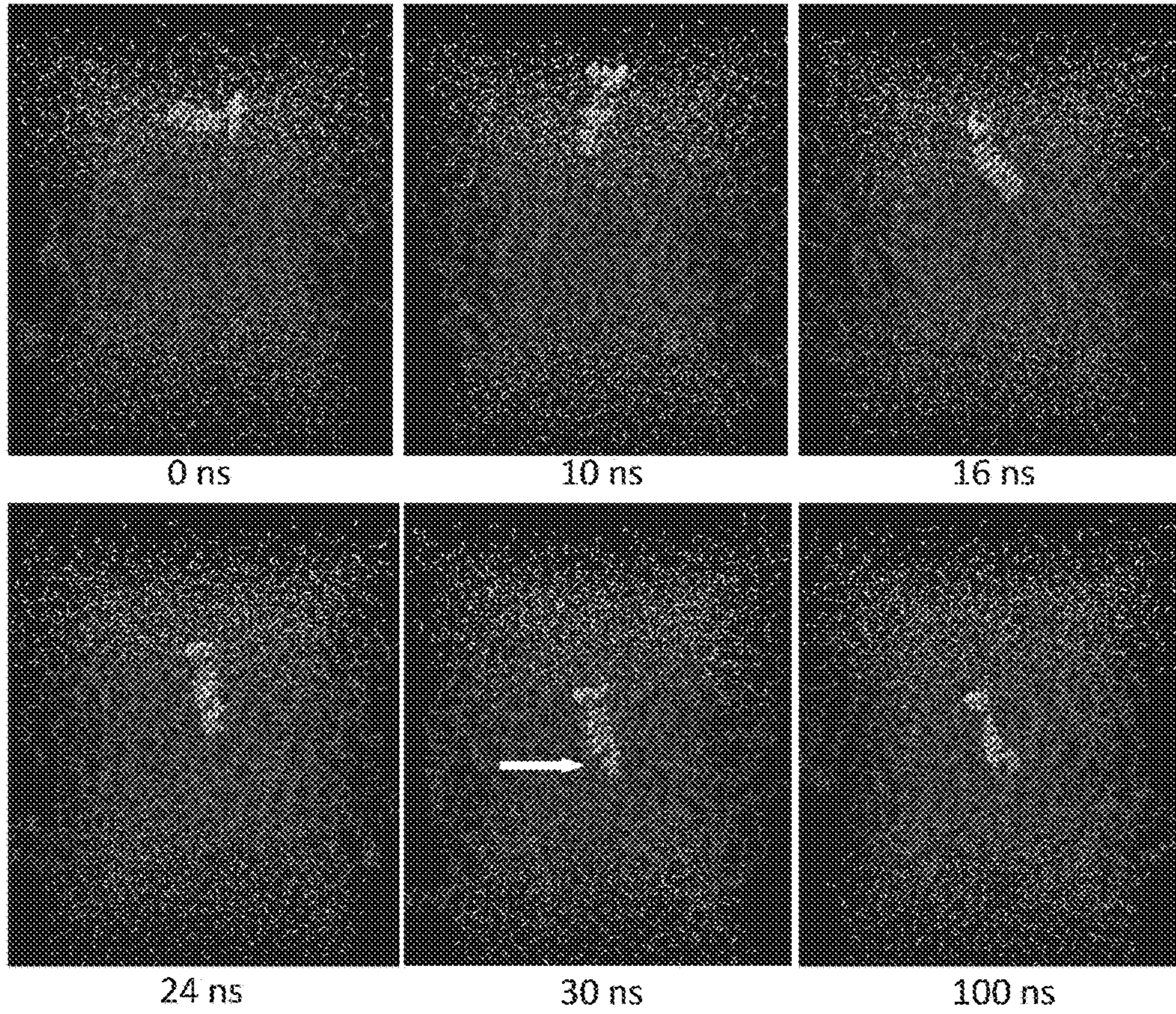
APO-Si-X2 simulation (100ns)
