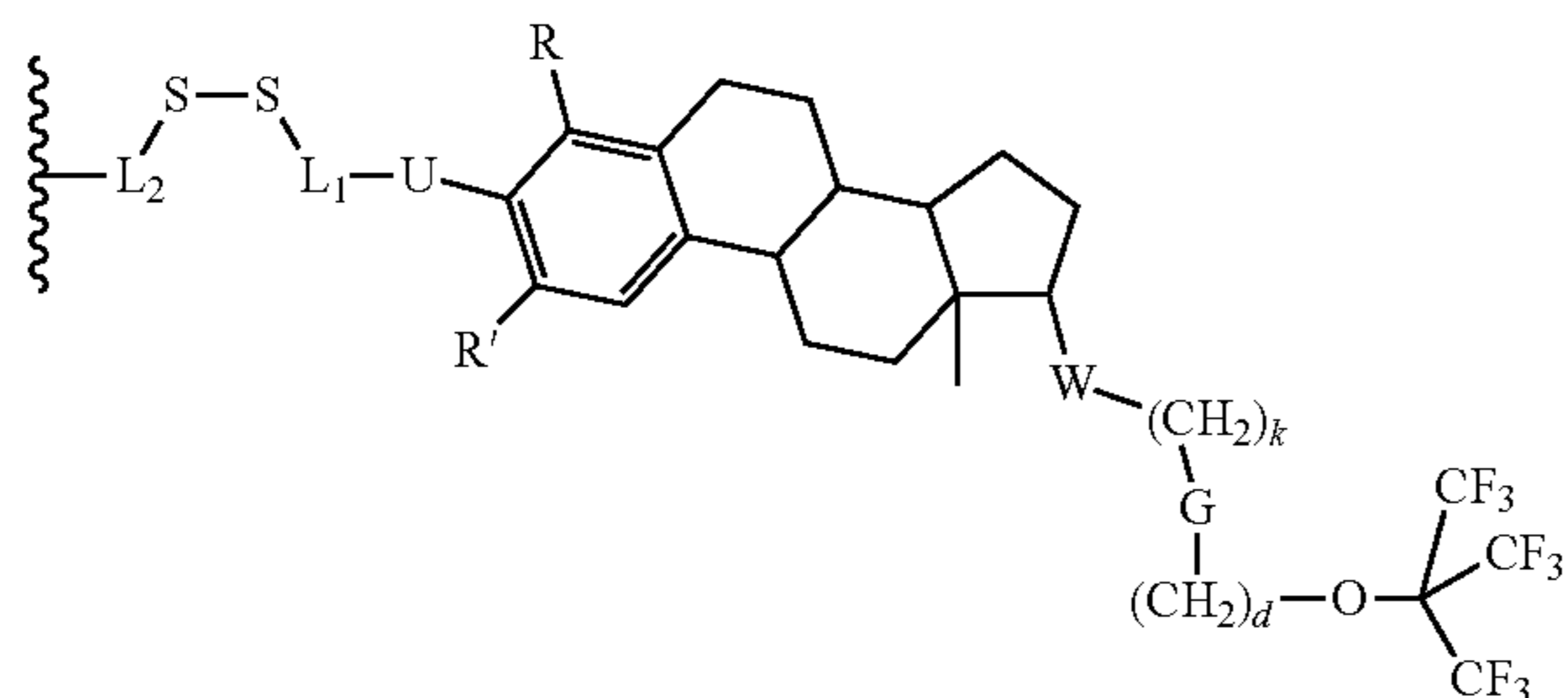
Formula (IX)
