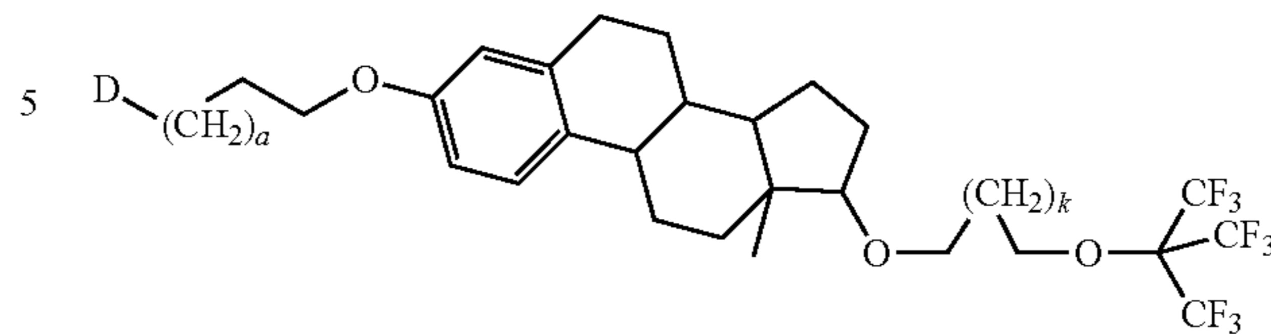
Formula (VIIa)
