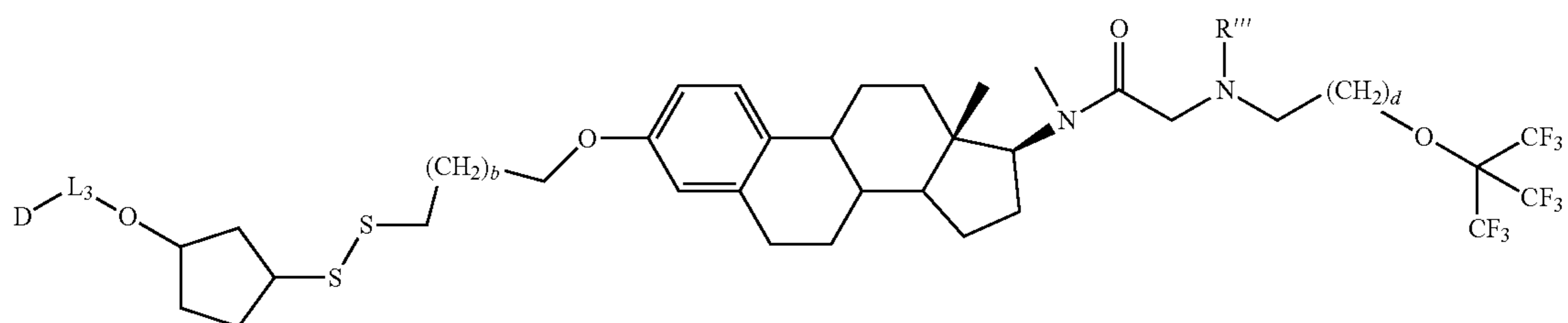
Formula (IXf)
