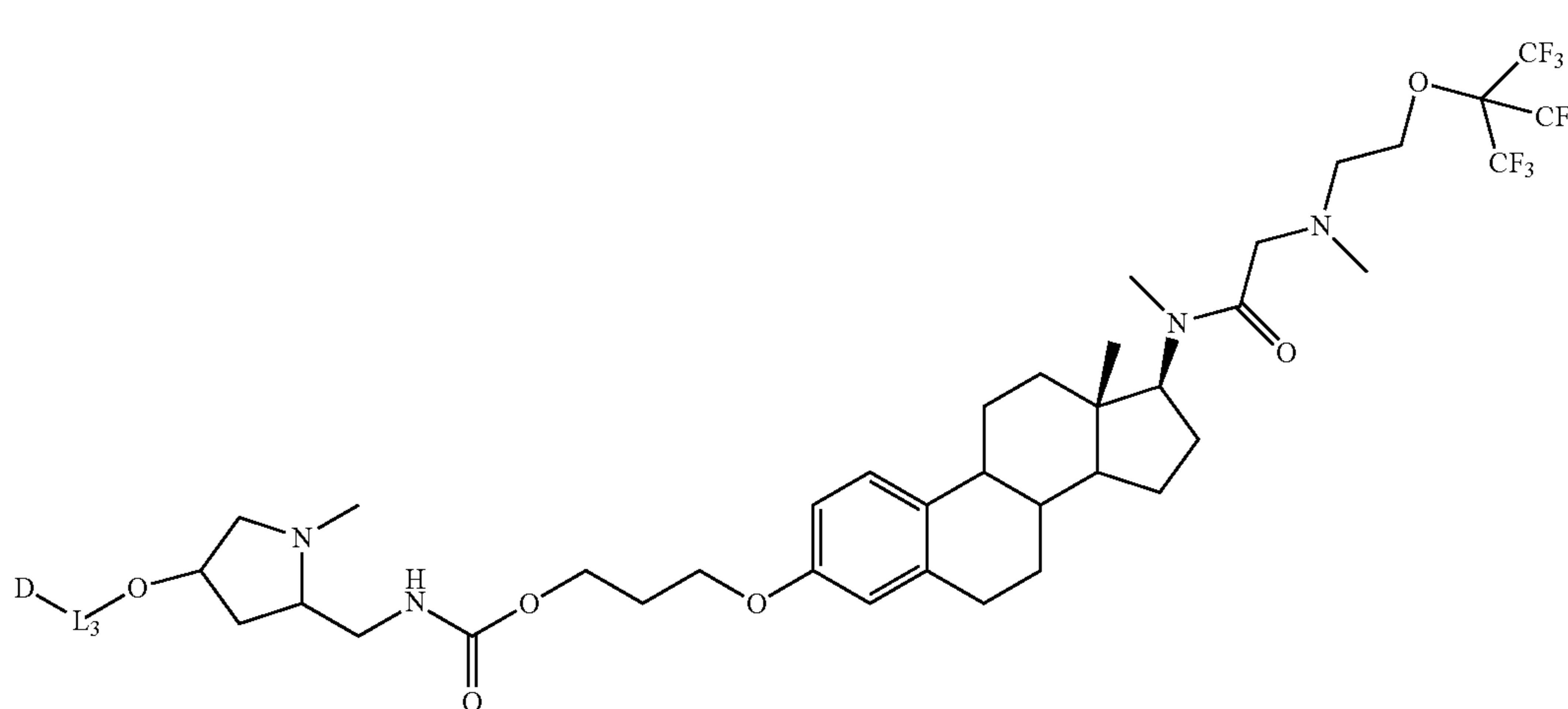
Formula (XIId)
