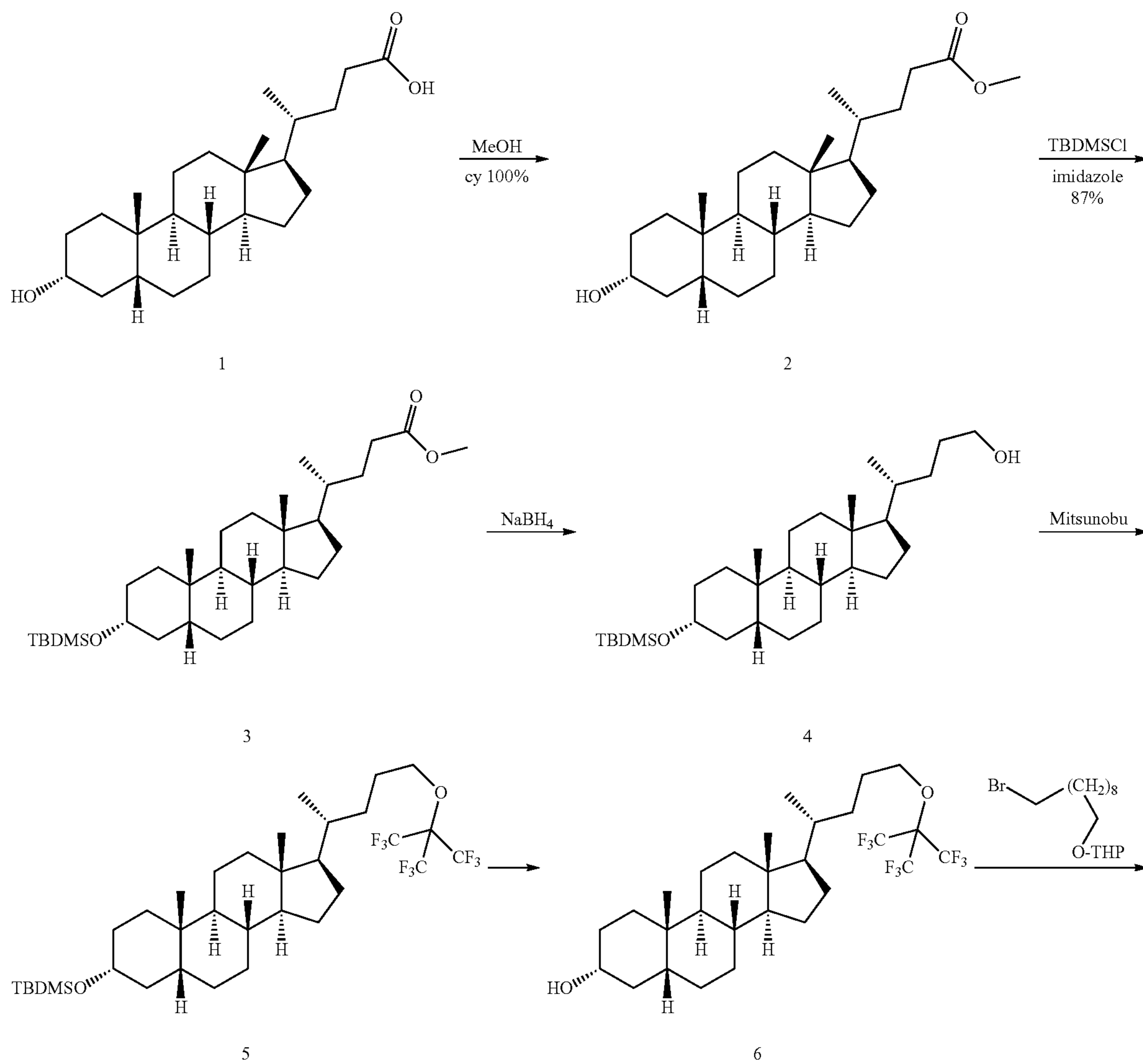
Scheme 2
