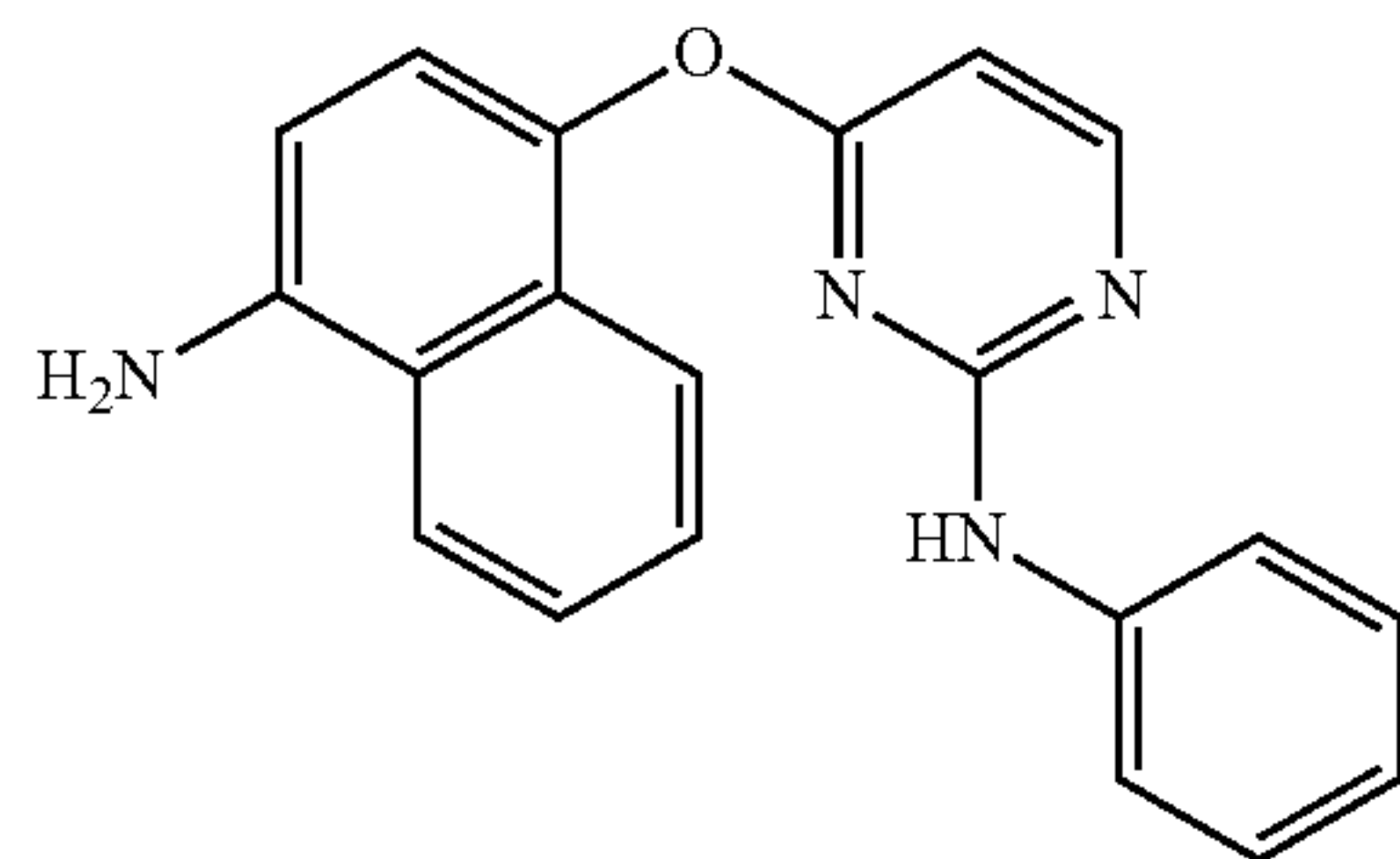
Intermediate B1
