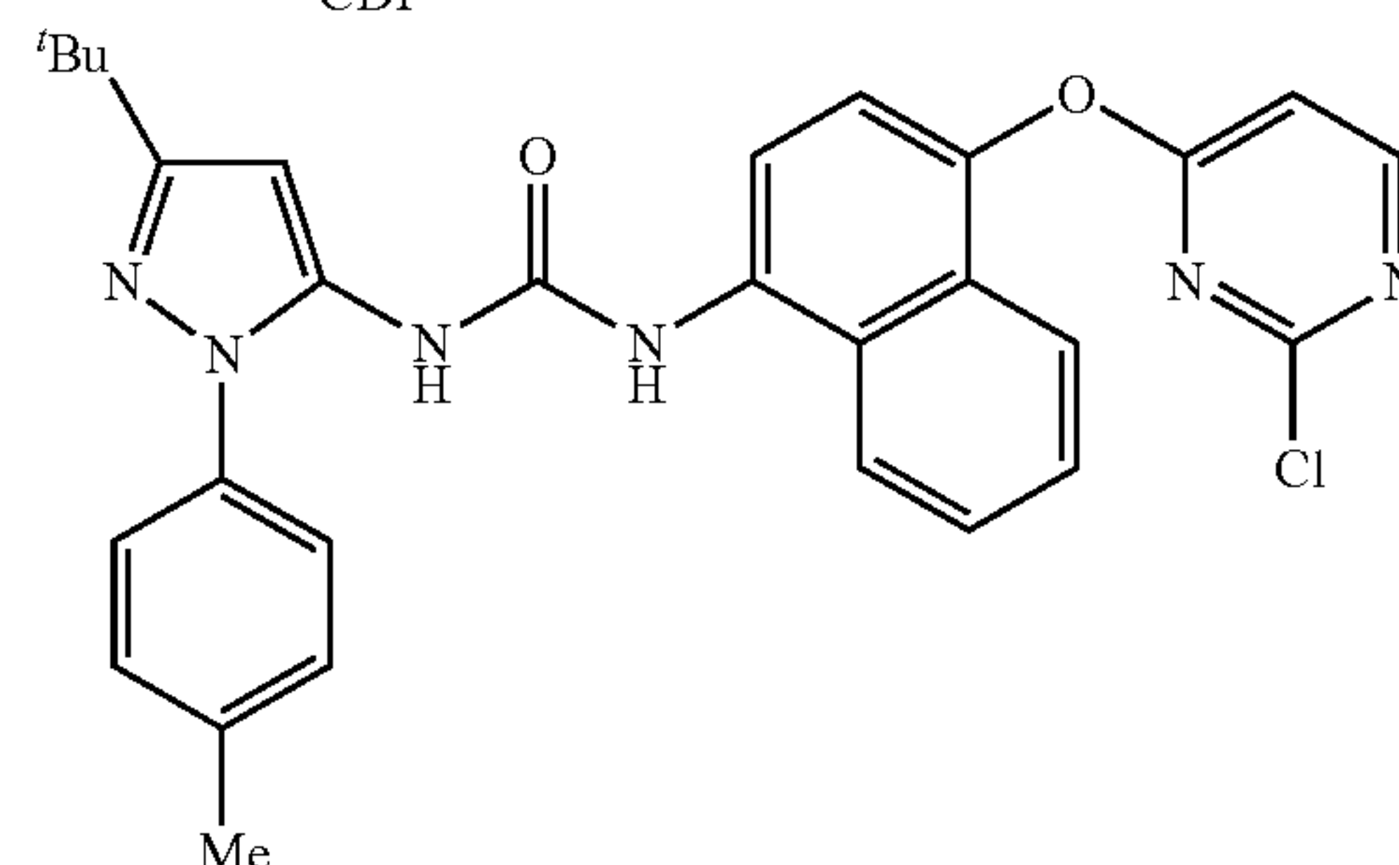
Intermediate C1
