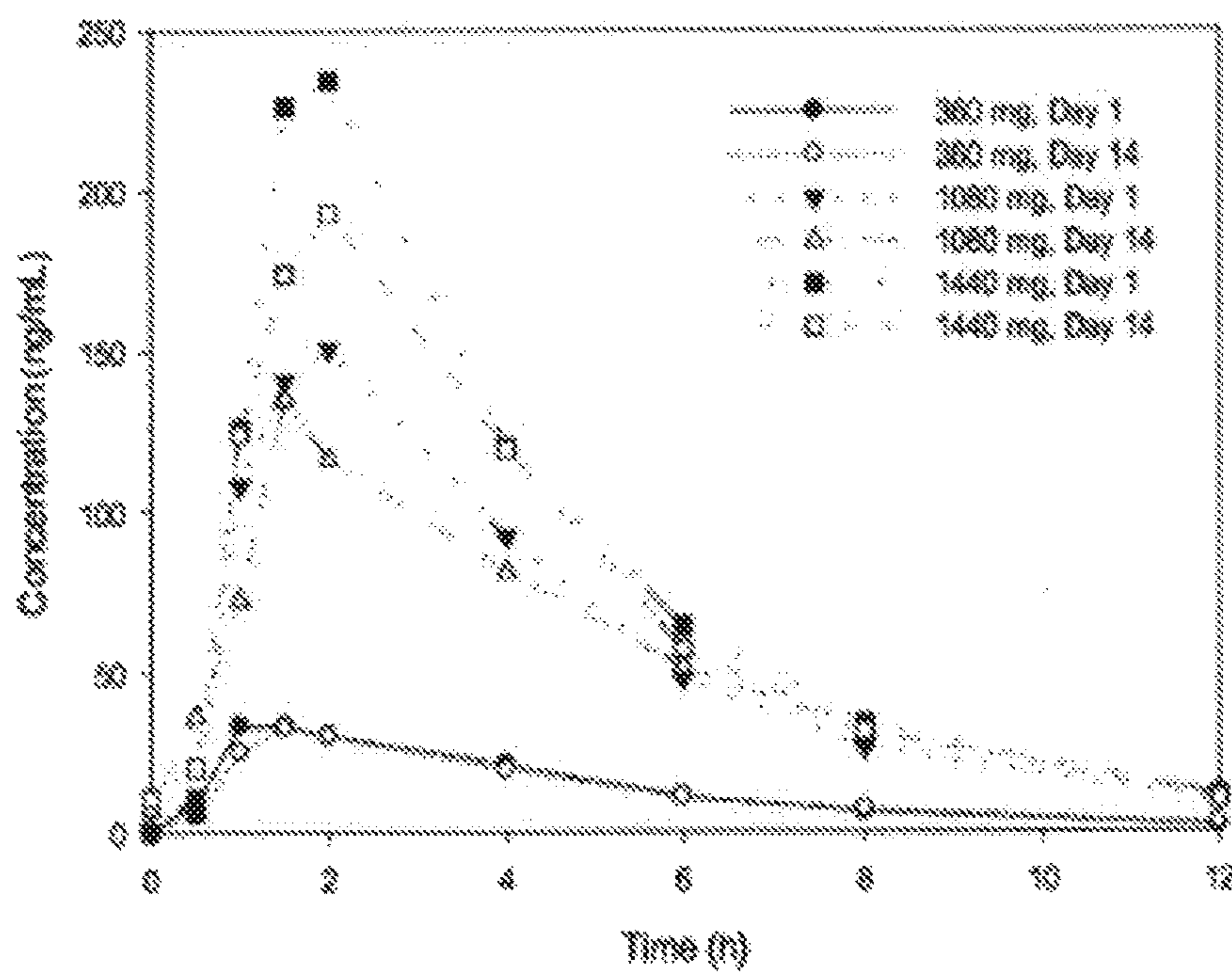
Figure 2. Mean (n = 12 or 13) plasma concentrations of 7-chlorokynurenic acid on Days 1 and 14 after oral administration of once-daily doses of AV-101.
