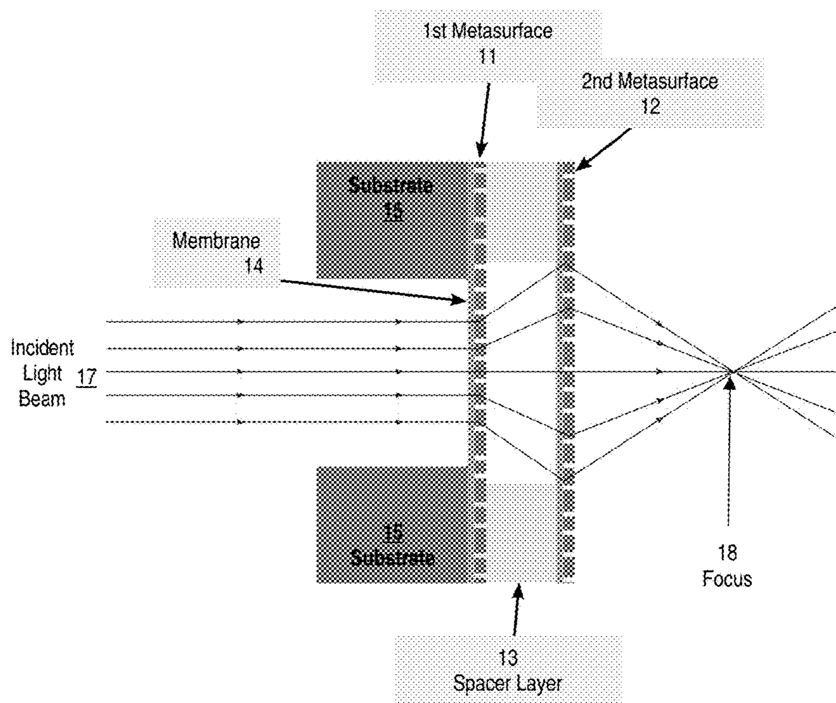
Example Optical System with Tunable Focus 10
