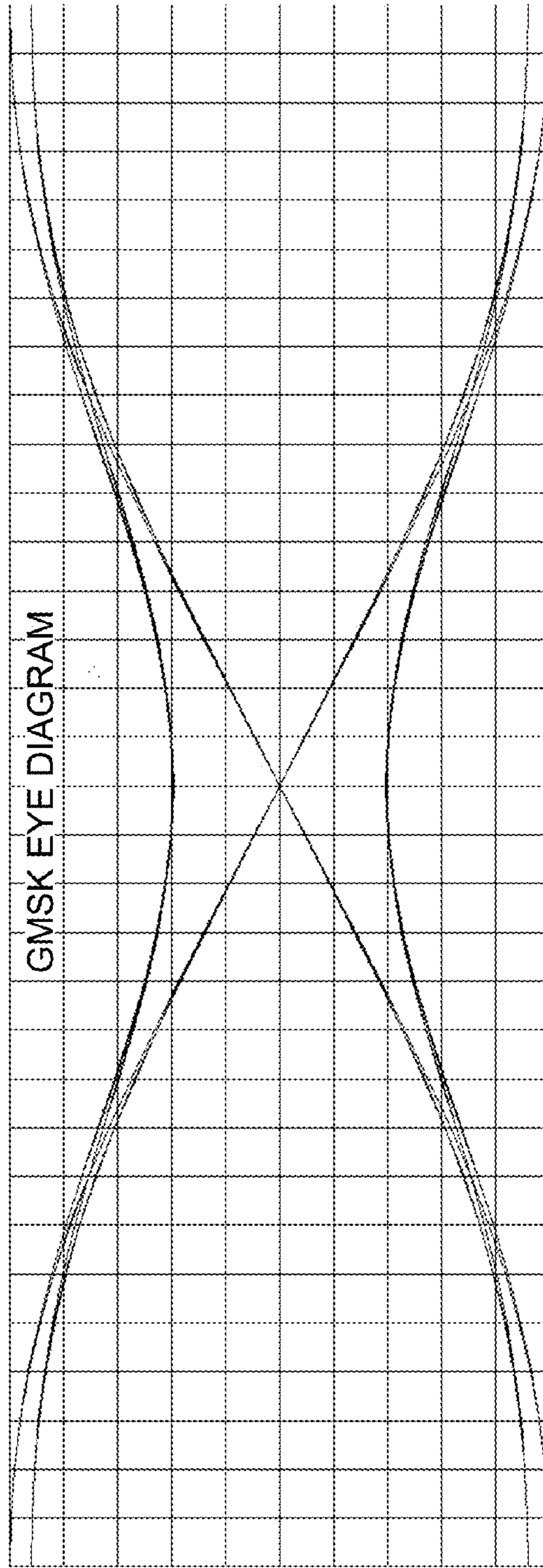
I,Q Eye Diagram for GSMK with a Gaussian BT = 0.3
