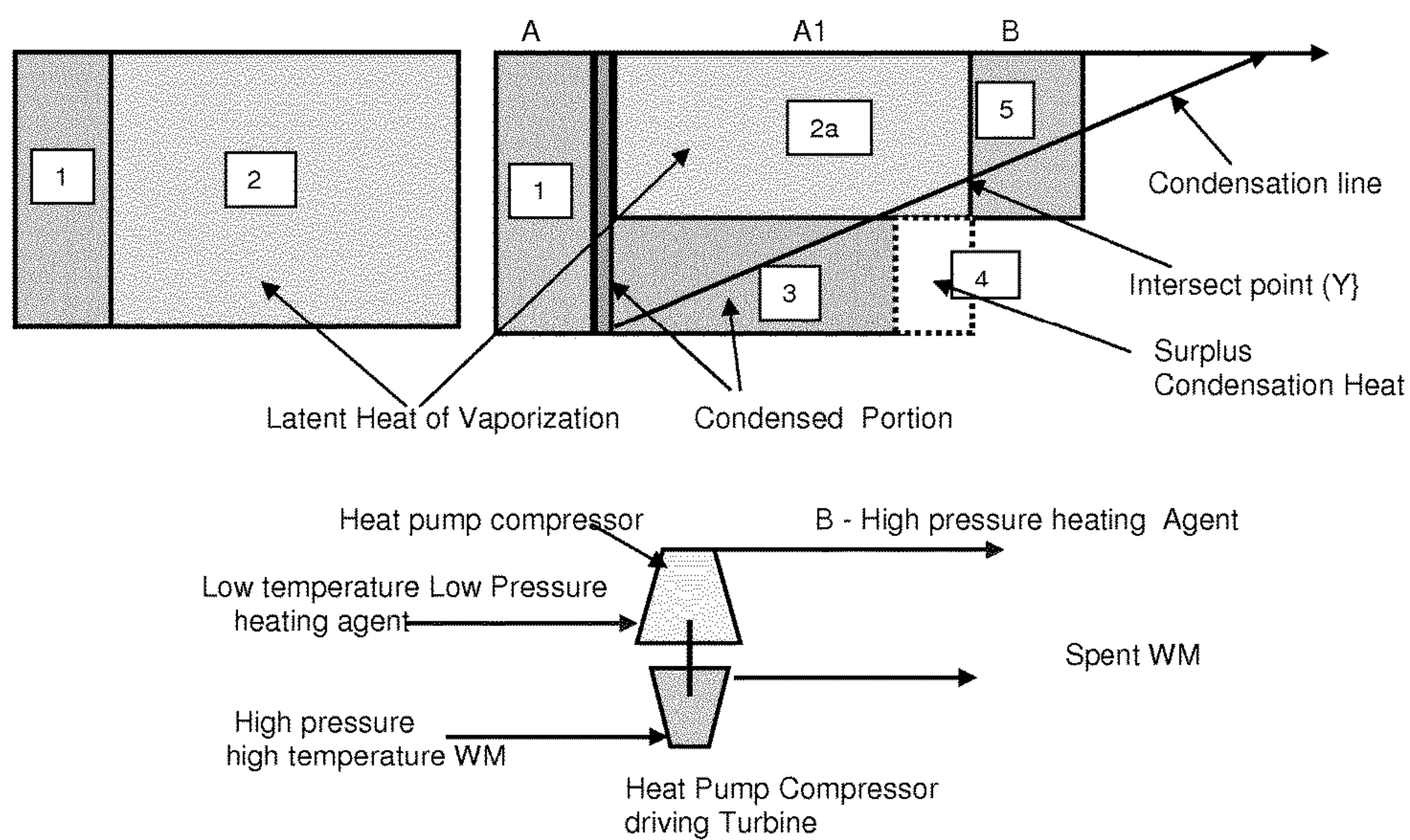
Figure 23 Temperature-Entropy (T-s) diagram of n-Octane showing steps of the energy preservation loop with single stage compression of n-octane from the saturation state at point B, and representation of energy constituents by corresponding areas,
