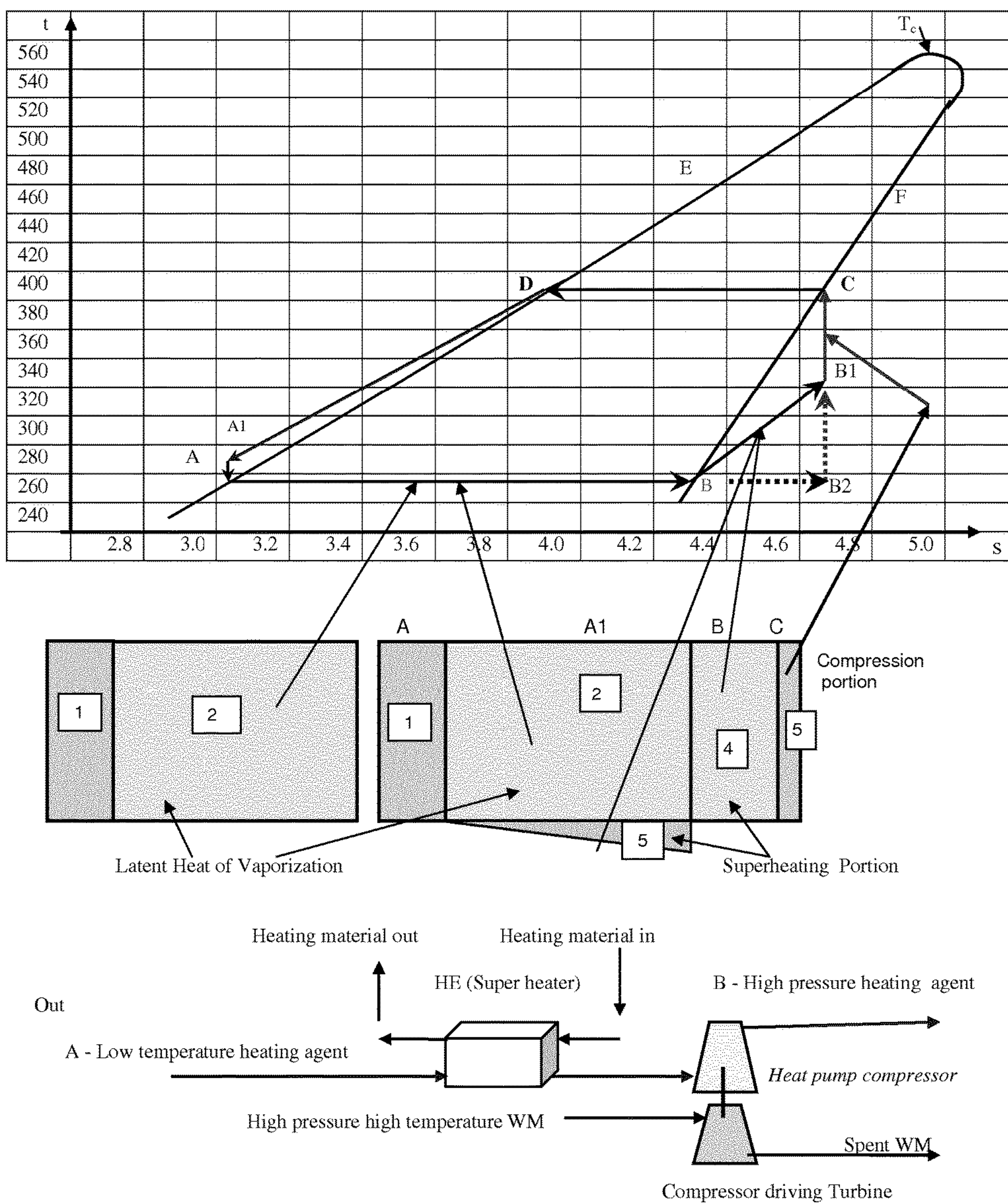
Figure. 27 Temperature-Entropy (T-s) diagram of n-Octane showing steps of the energy preservation loop with superheating of n-octane prior to feeding to the compressor, - Energy constituents are represented by the corresponding areas,
