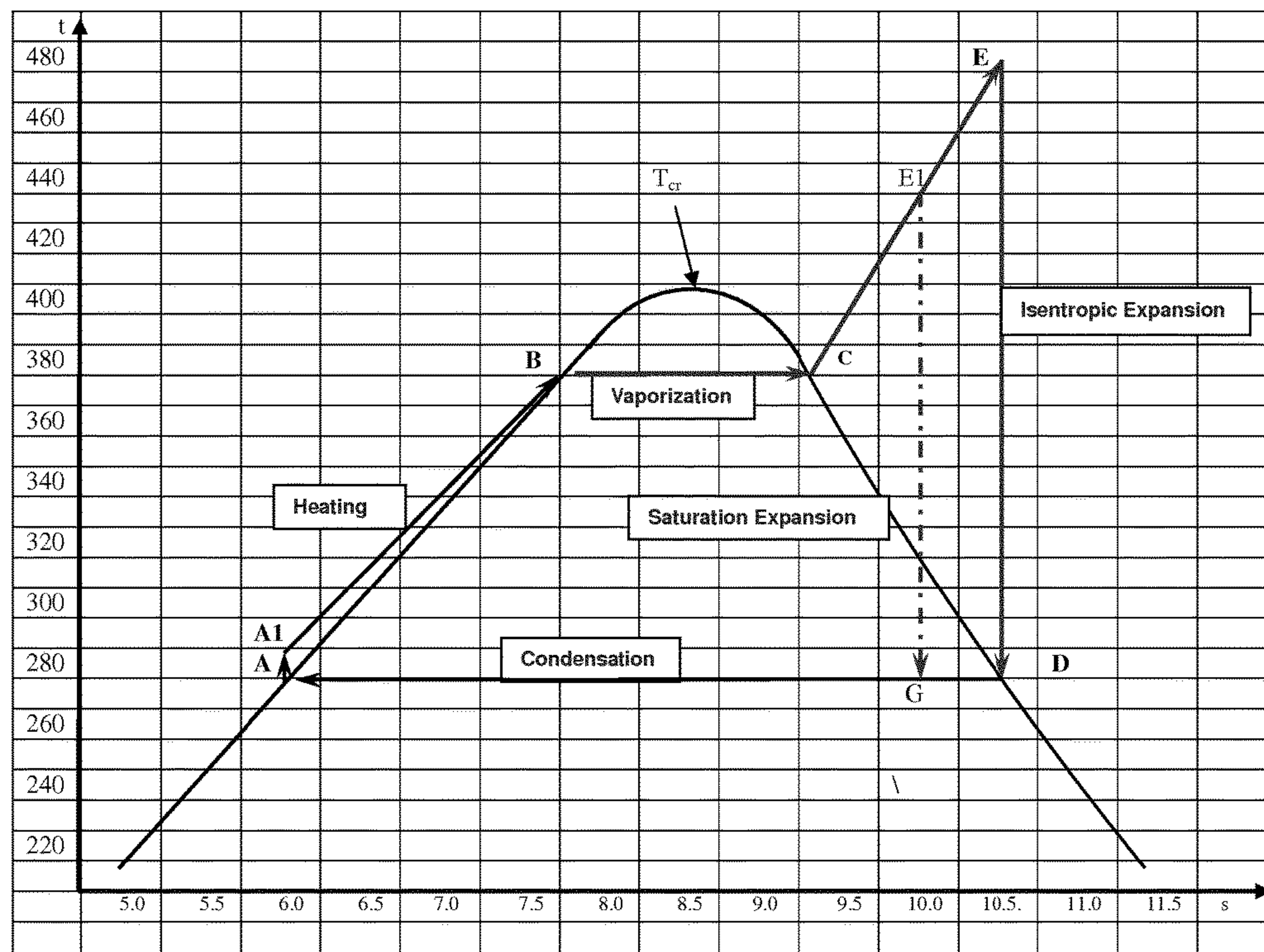
Figure 16 Temperature-Entropy (T-s) diagram of Ammonia showing steps of a power generation loop with superheating of high pressure ammonia and isentropic expansion
