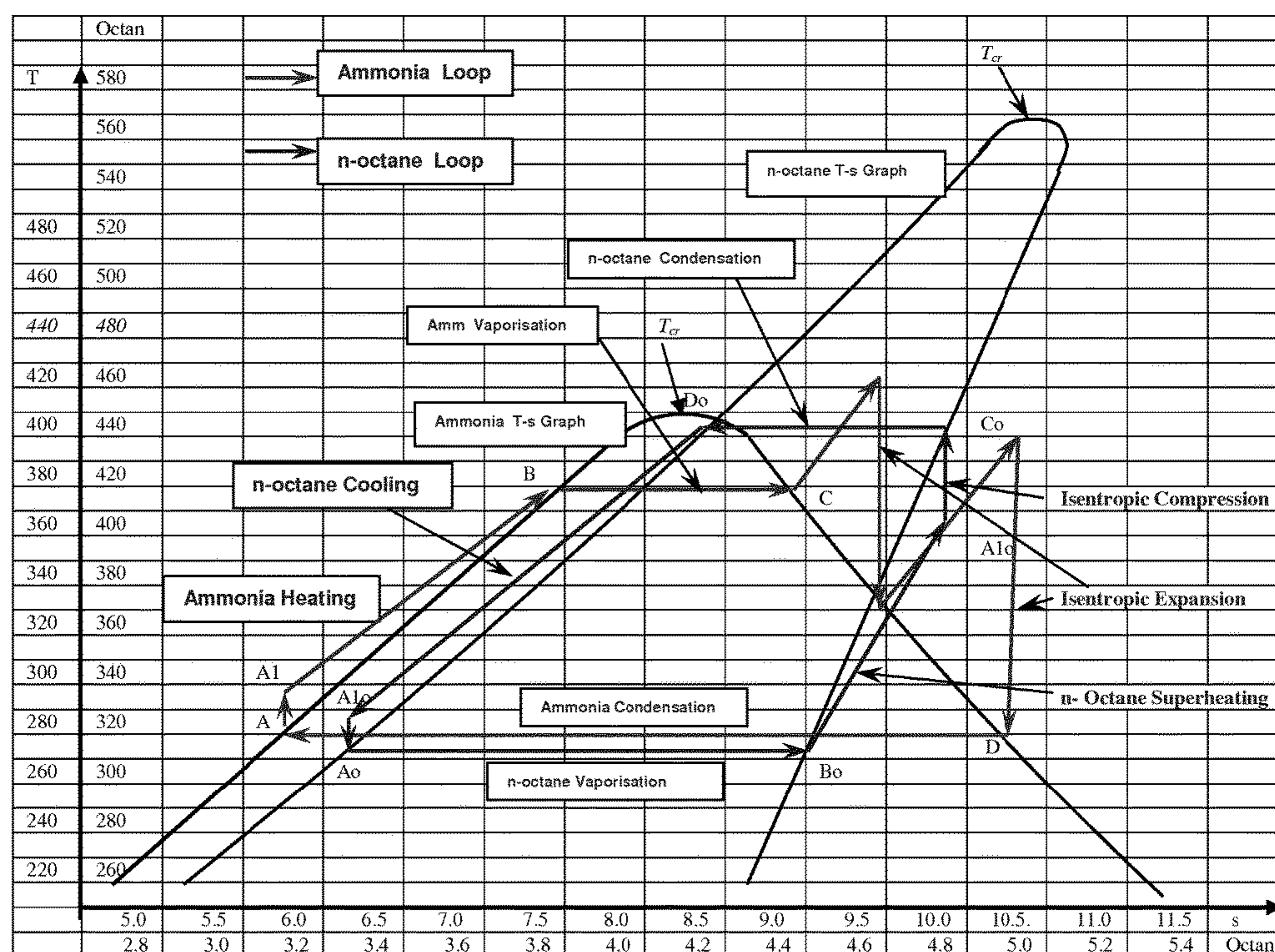
Figure 31, Superimposed temperature-entropy (T-s) diagrams of n-Octane (as the heating agent) and Ammonia (as the working medium) to form the integrated "Atalla Harwen Cycle"
