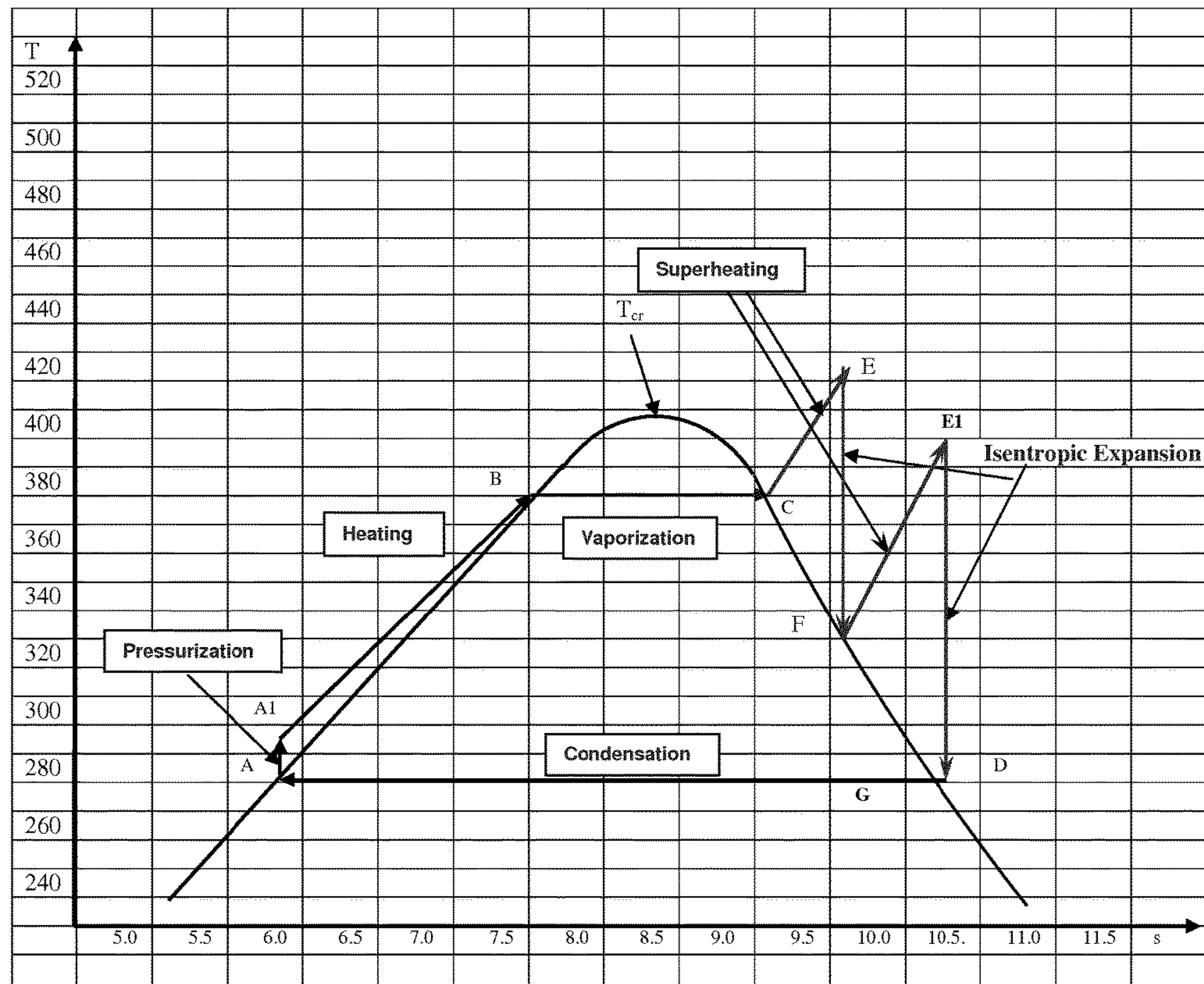
Figure 19 Temperature-Entropy (T-s) diagram of Ammonia showing steps of a power generation loop with superheating of the high pressure vaporized ammonia with two stage ammonia expansion and interim superheating
