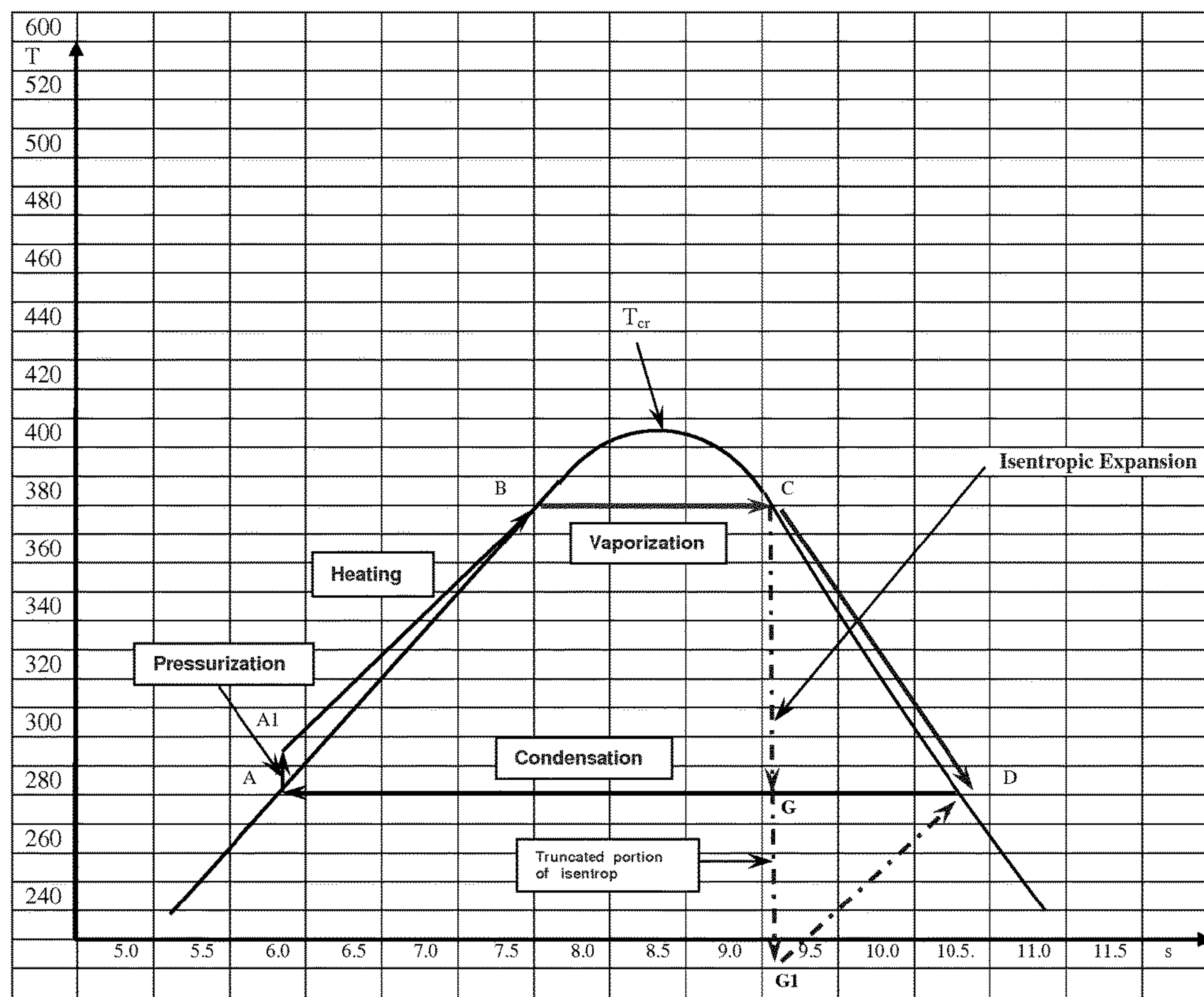
Figure 18 Temperature-Entropy (T-s) diagram of Ammonia showing steps of a power generation loop with expansion of high pressure ammonia from the saturation point C
