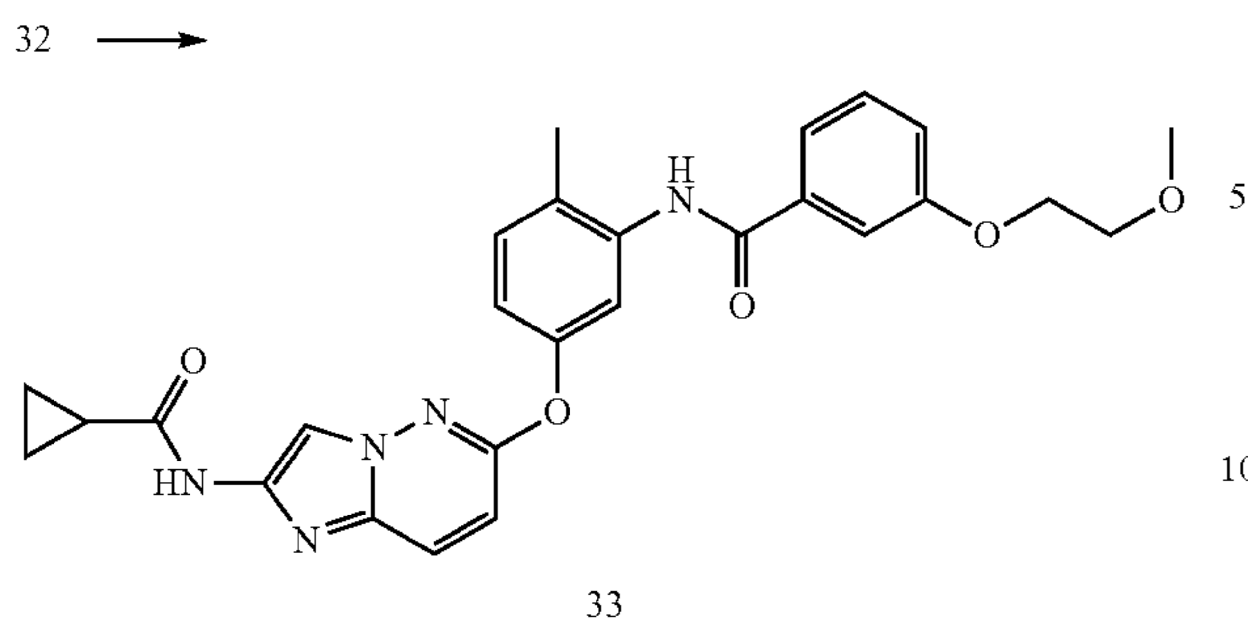
Compound 33
