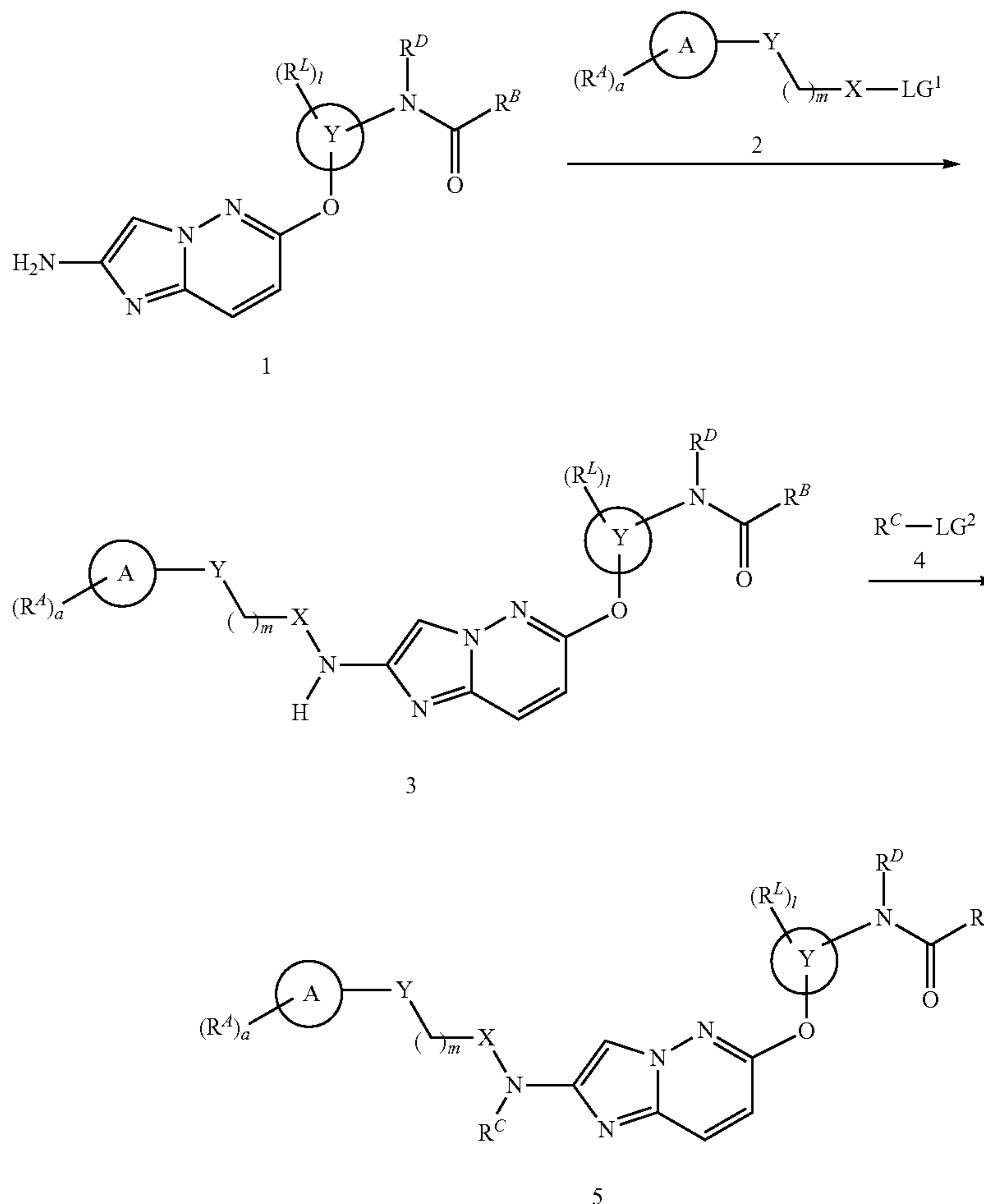
Scheme 1. Exemplary synthesis of compounds of Formula (I).
