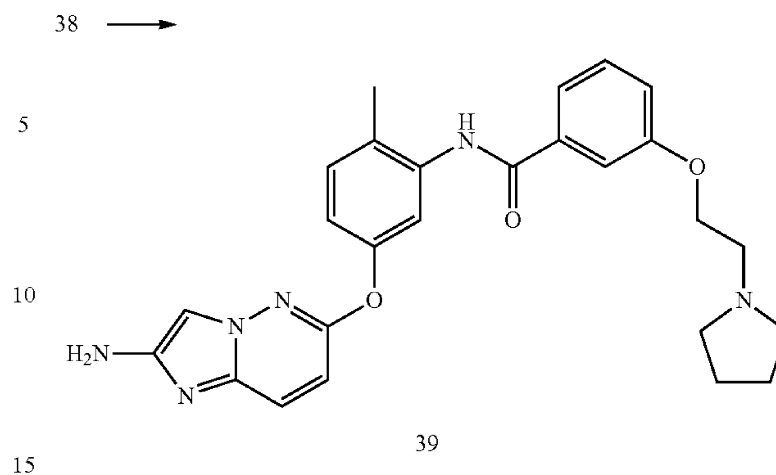
Compound 39
