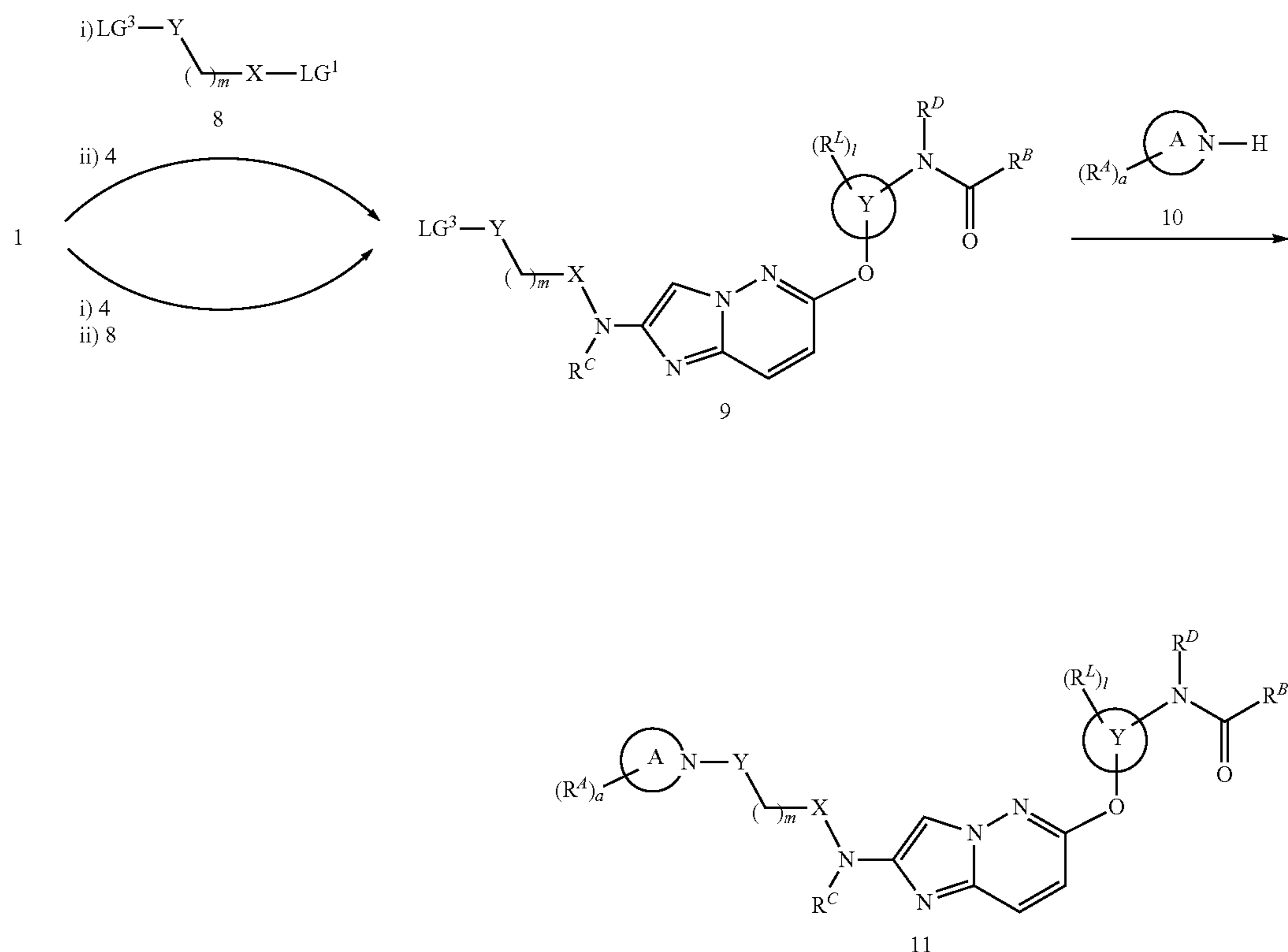
Scheme 2. Exemplary synthesis of certain compounds of Formula (I).
