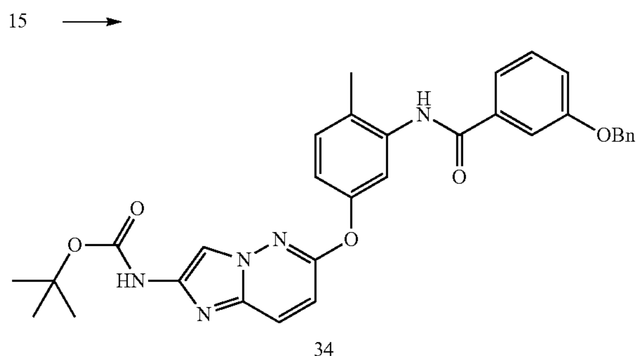
Compound 34
