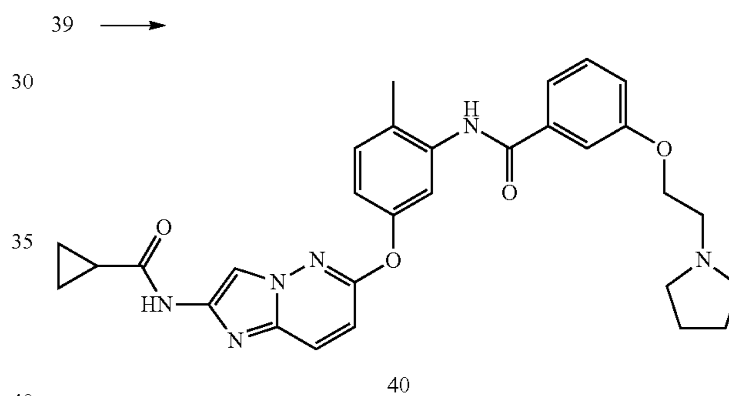
Compound 40
