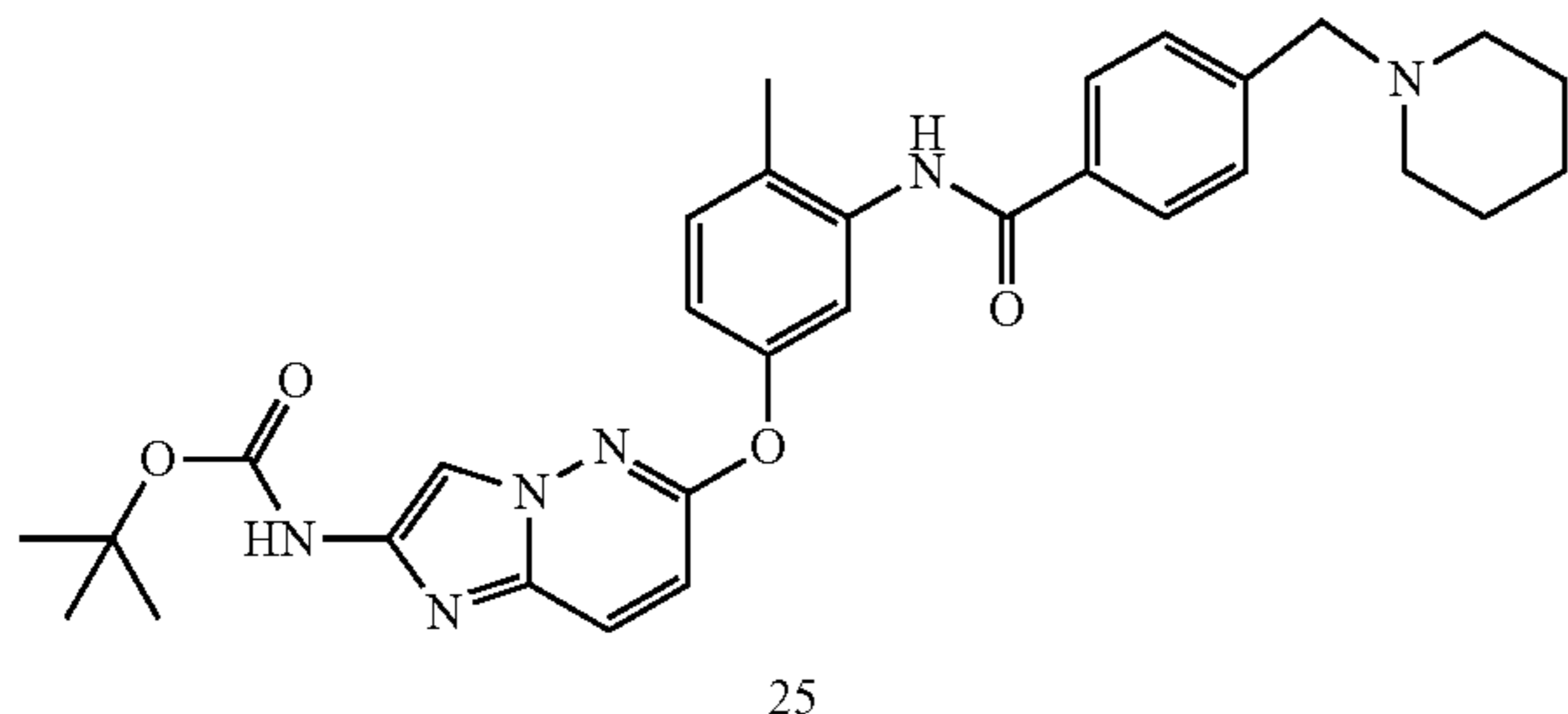
Compound 25
