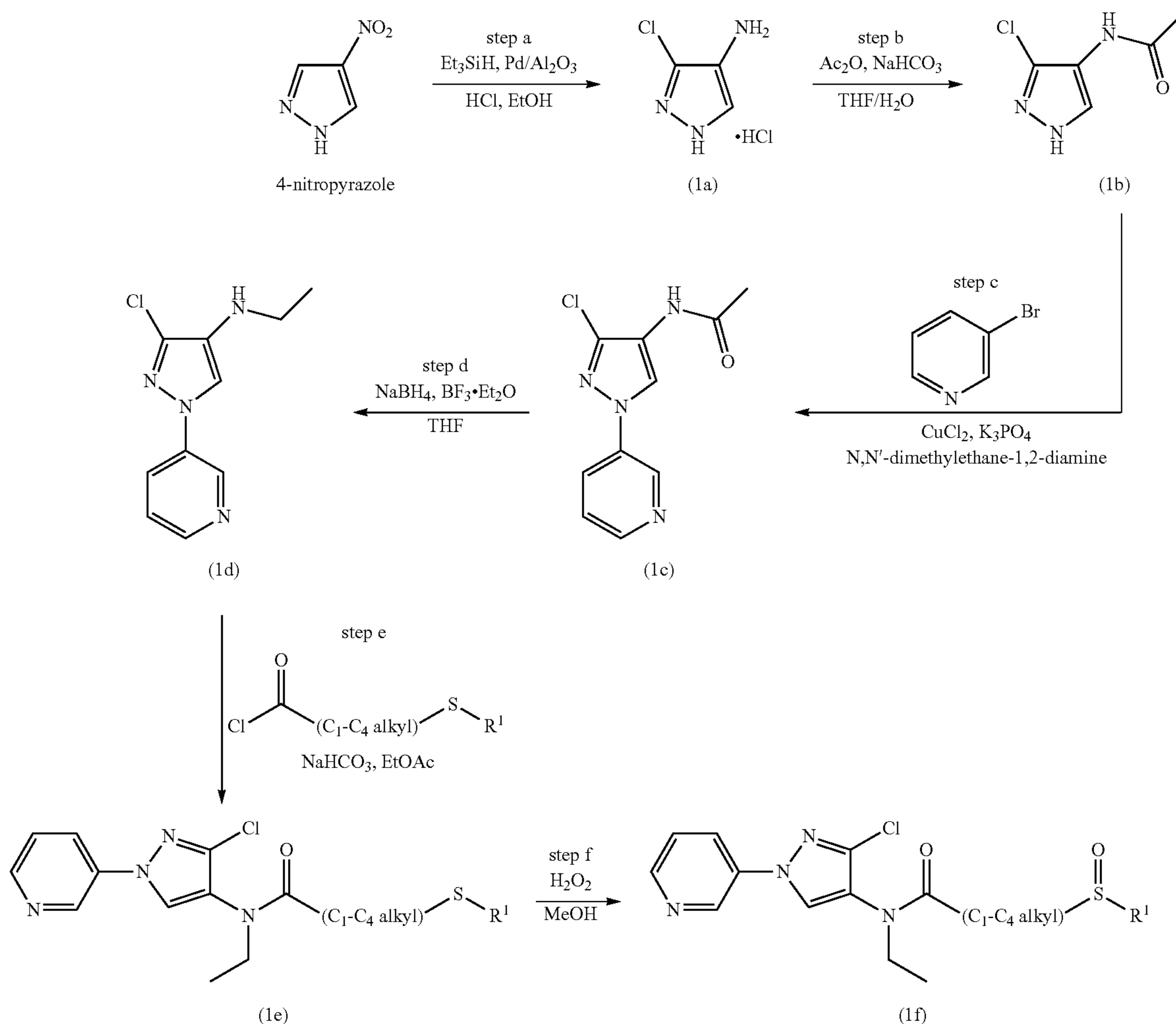
Scheme 1
