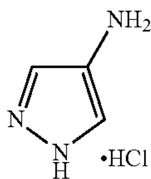
1H-pyrazol-4-amine hydrochloride
