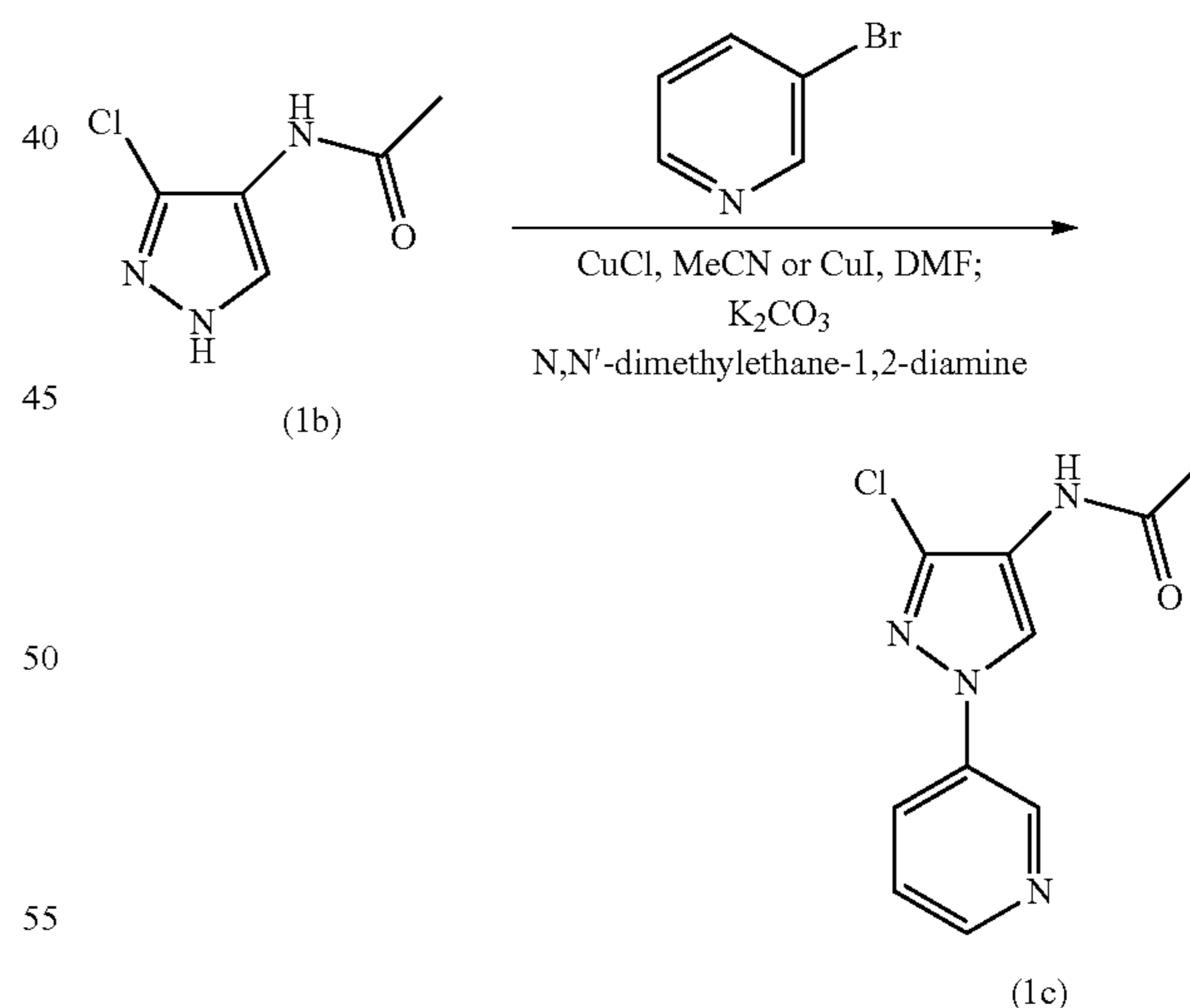
Scheme 2
