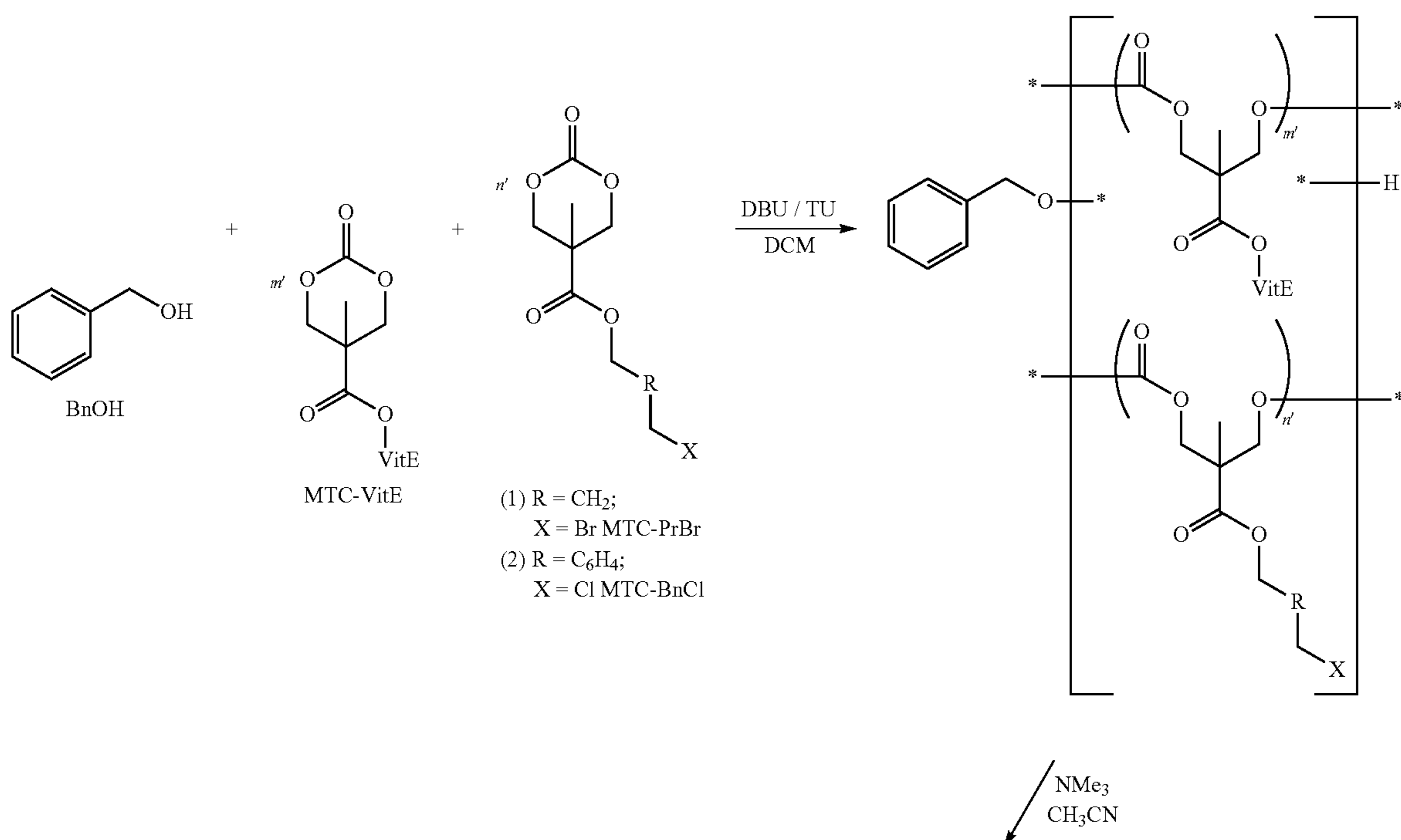
Scheme 1
