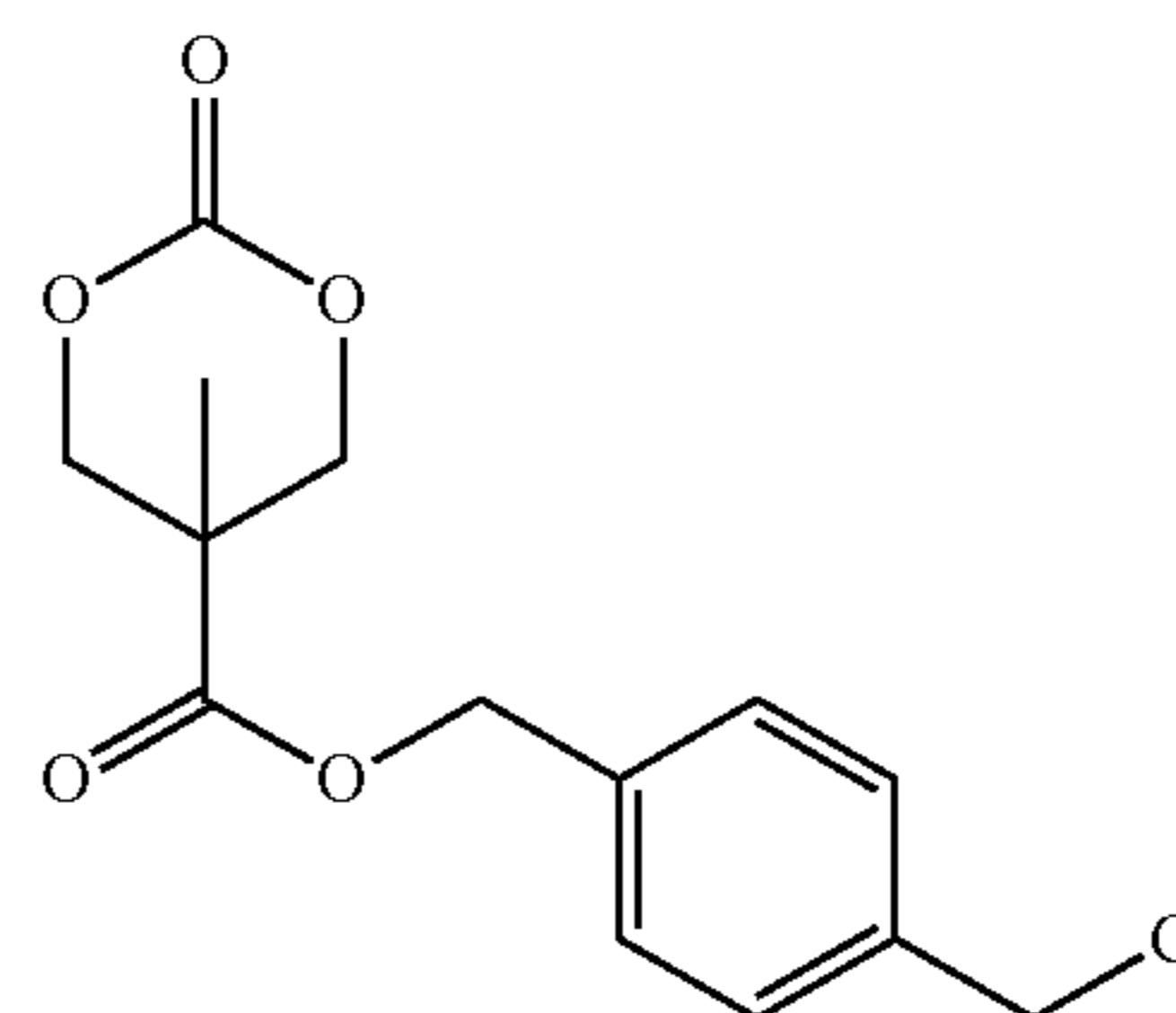
(MTC-BnCl)
