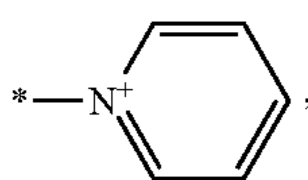
(pyridinium)
