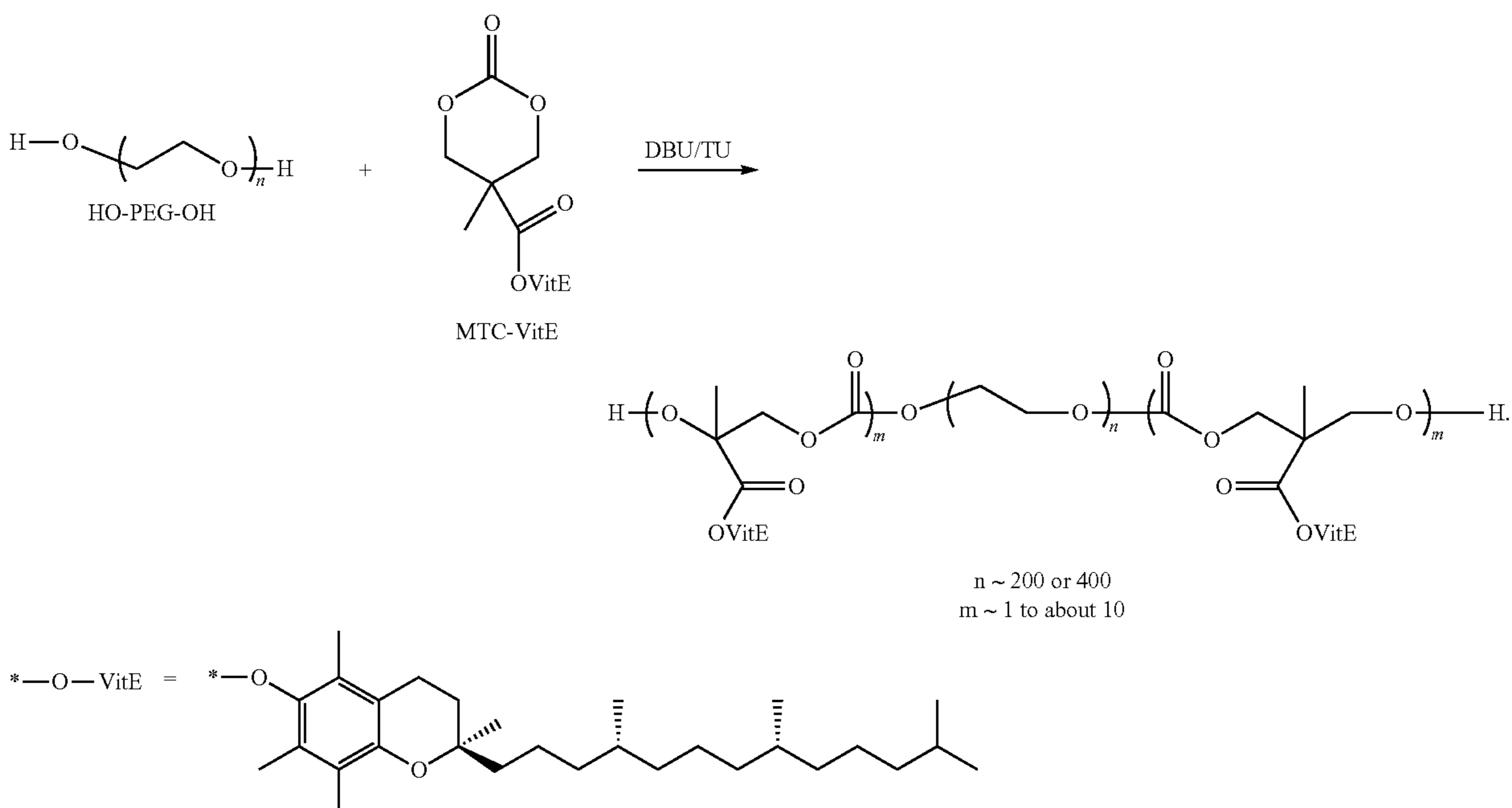
Scheme 2
