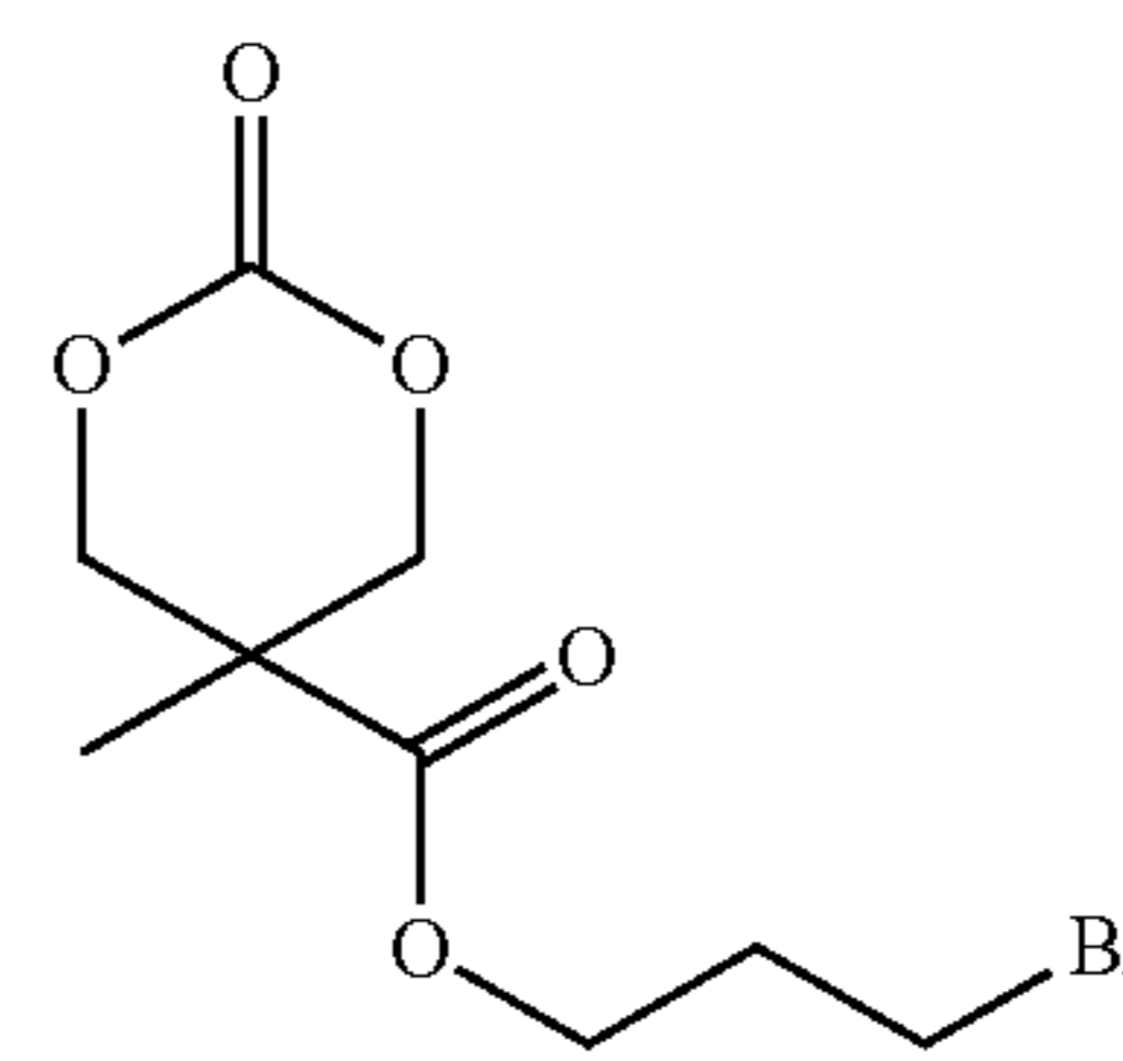
(MTC-PrBr)
