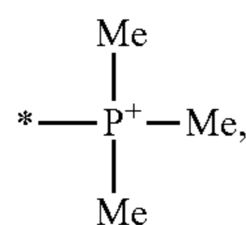
(trimethyl phosphonium)
