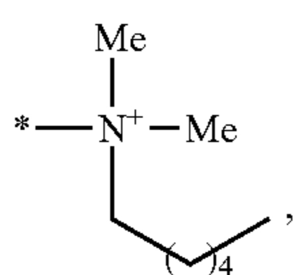
(dimethyl hexyl ammonium)
