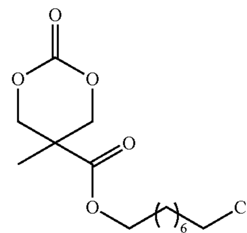
(MTC-C8Cl)
