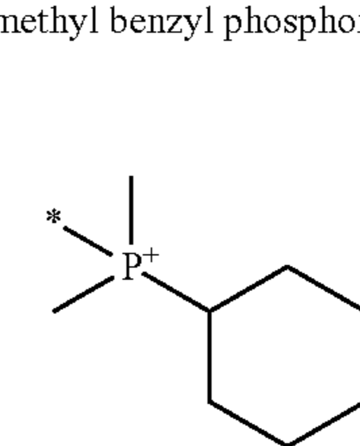
(dimethyl cyclohexyl phosphonium)
