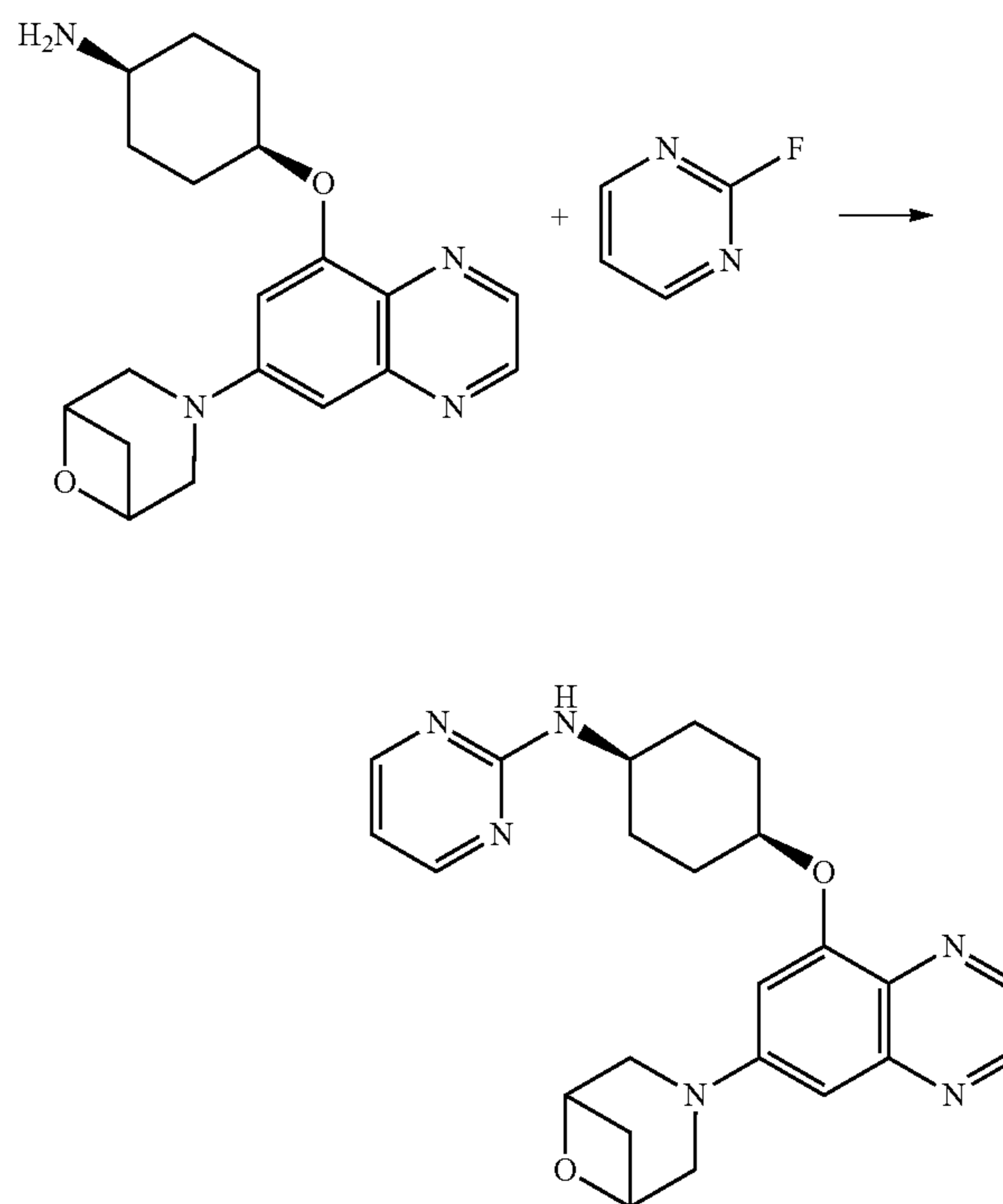
Scheme 10d
