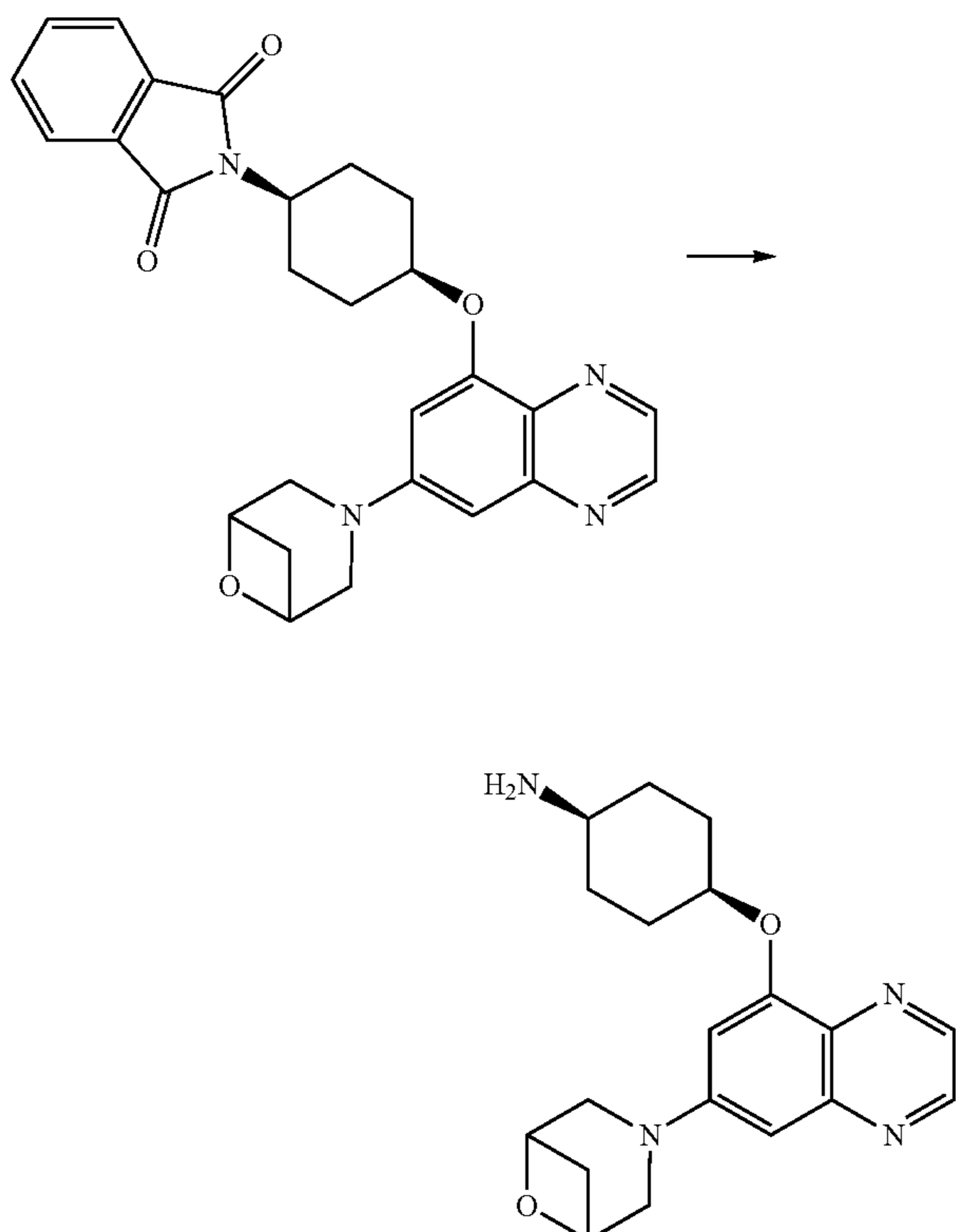
Scheme 10c
