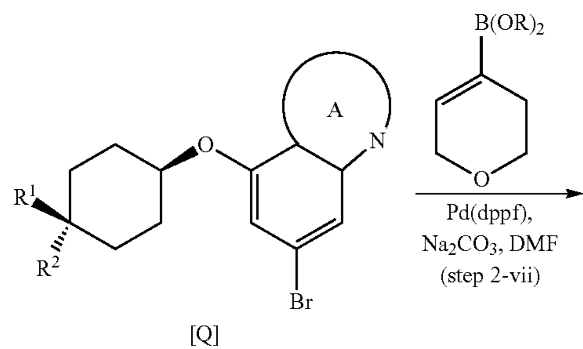
Scheme 2c
