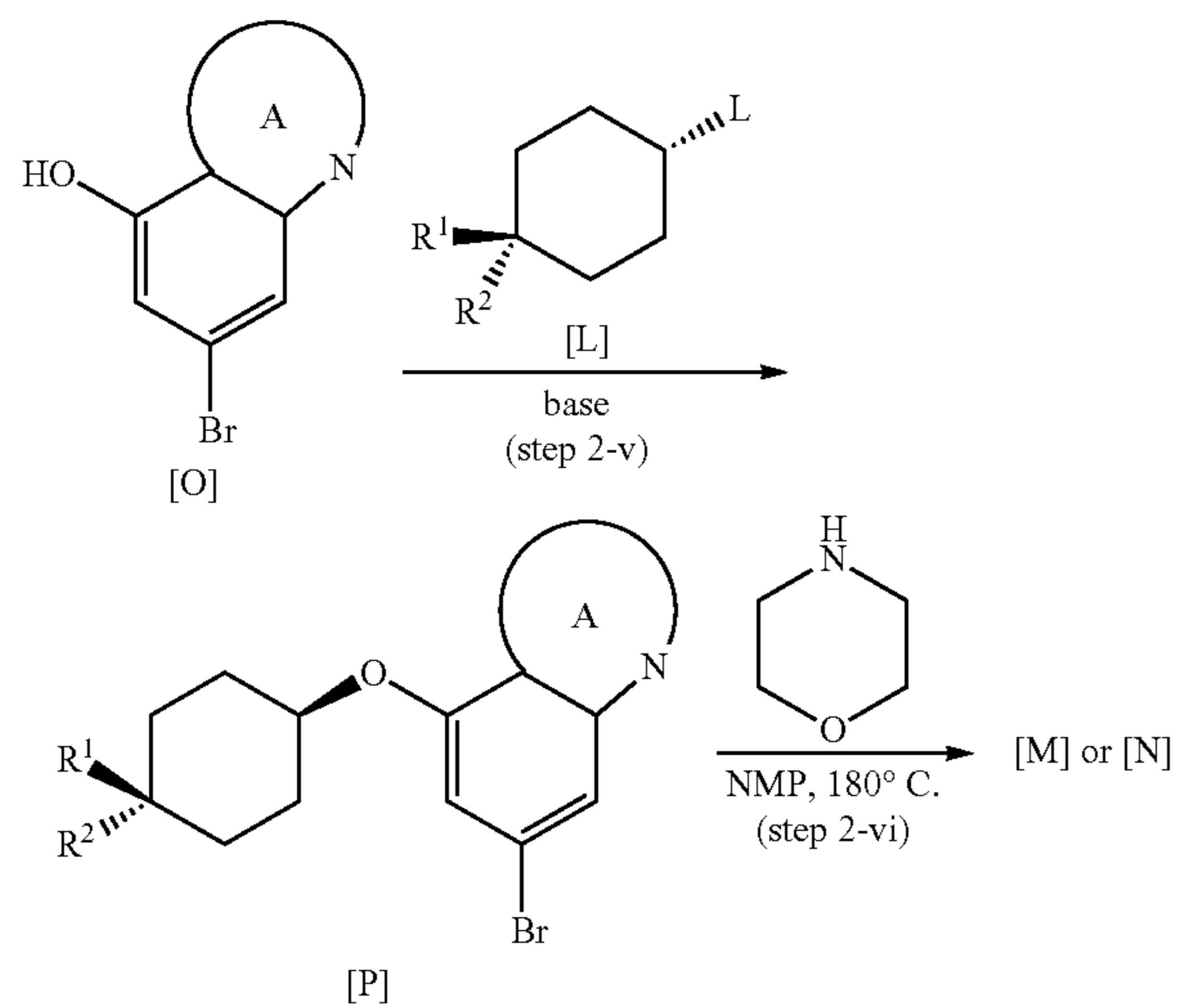
Scheme 2b
