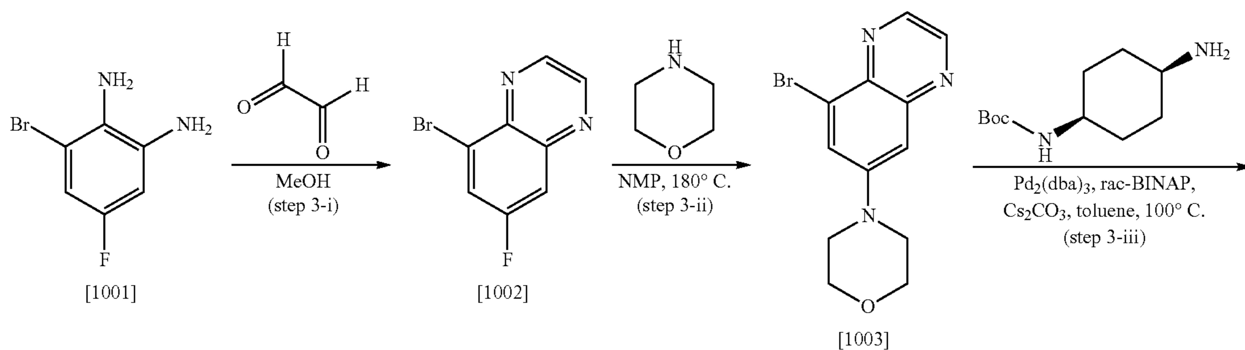
Scheme 3
