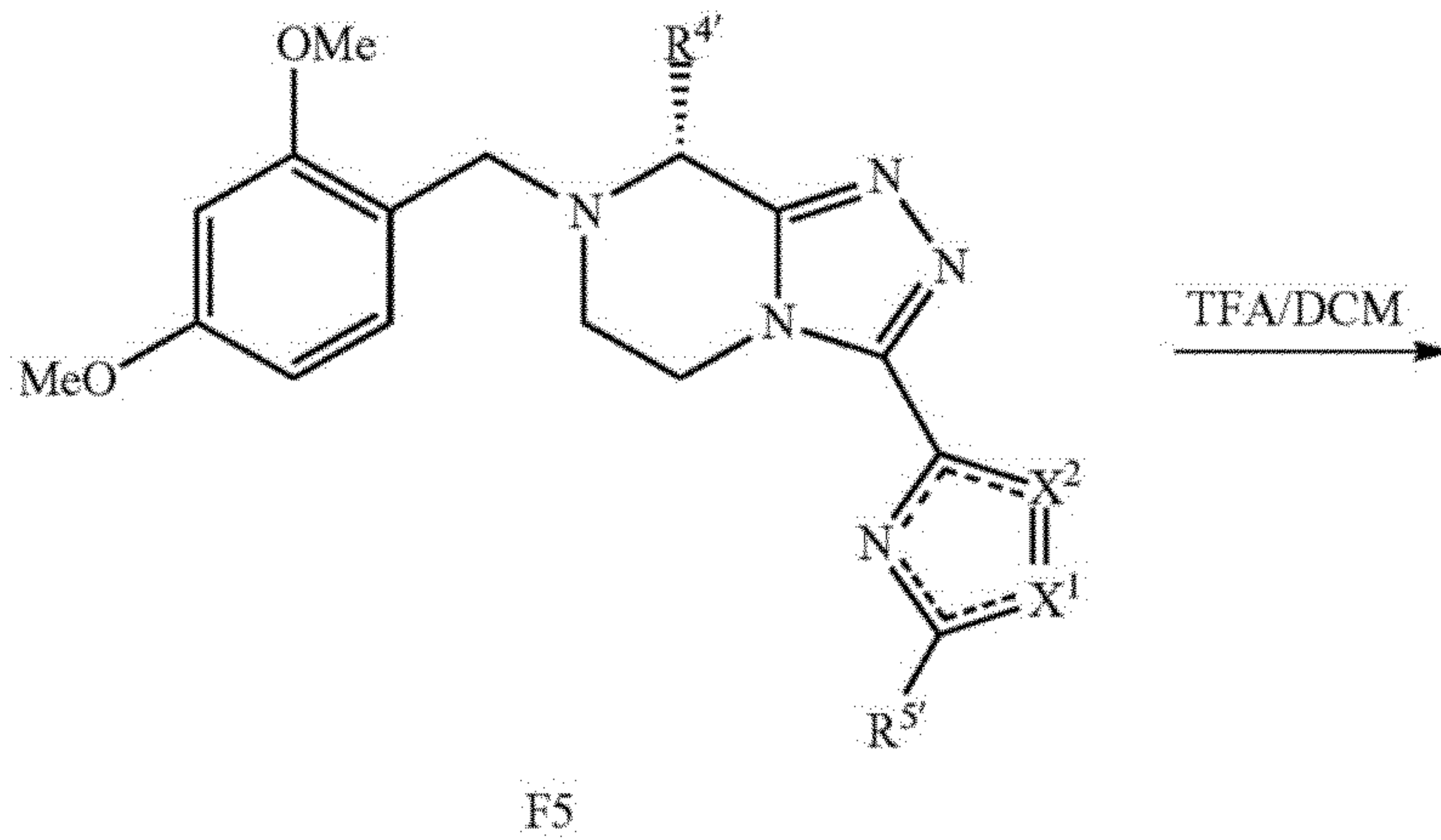
Scheme 14: DMB deprotection.
