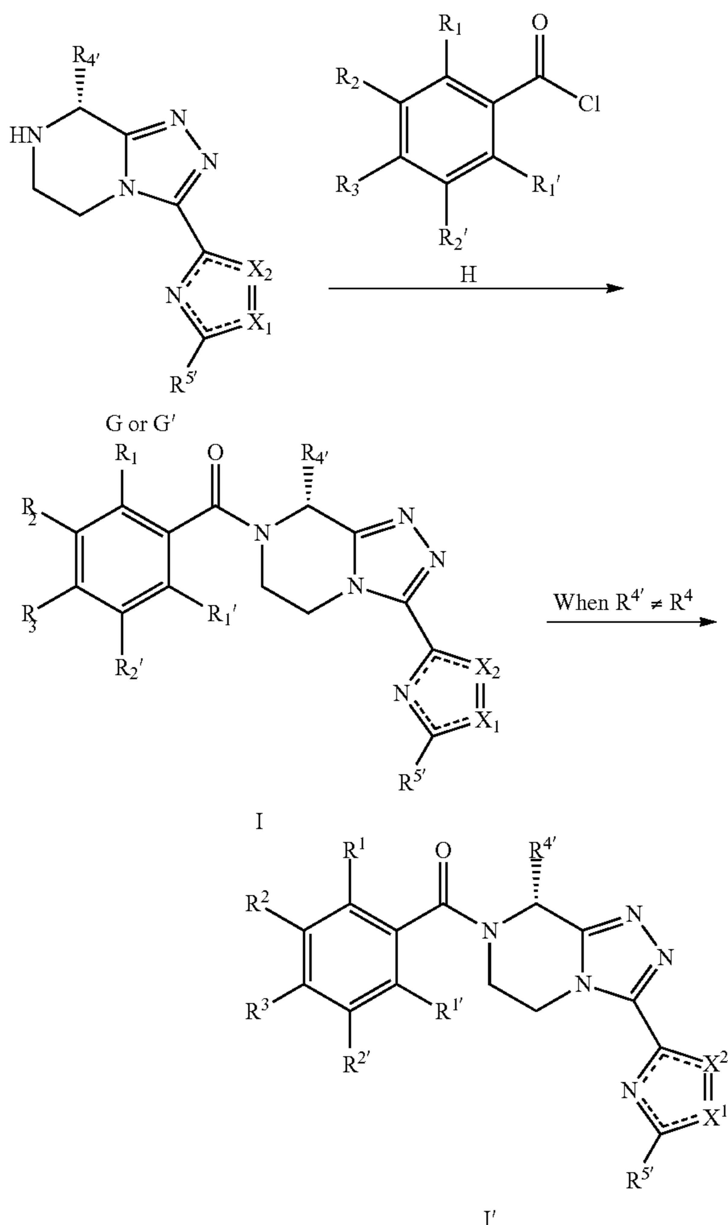
Scheme 16: Acylation.
