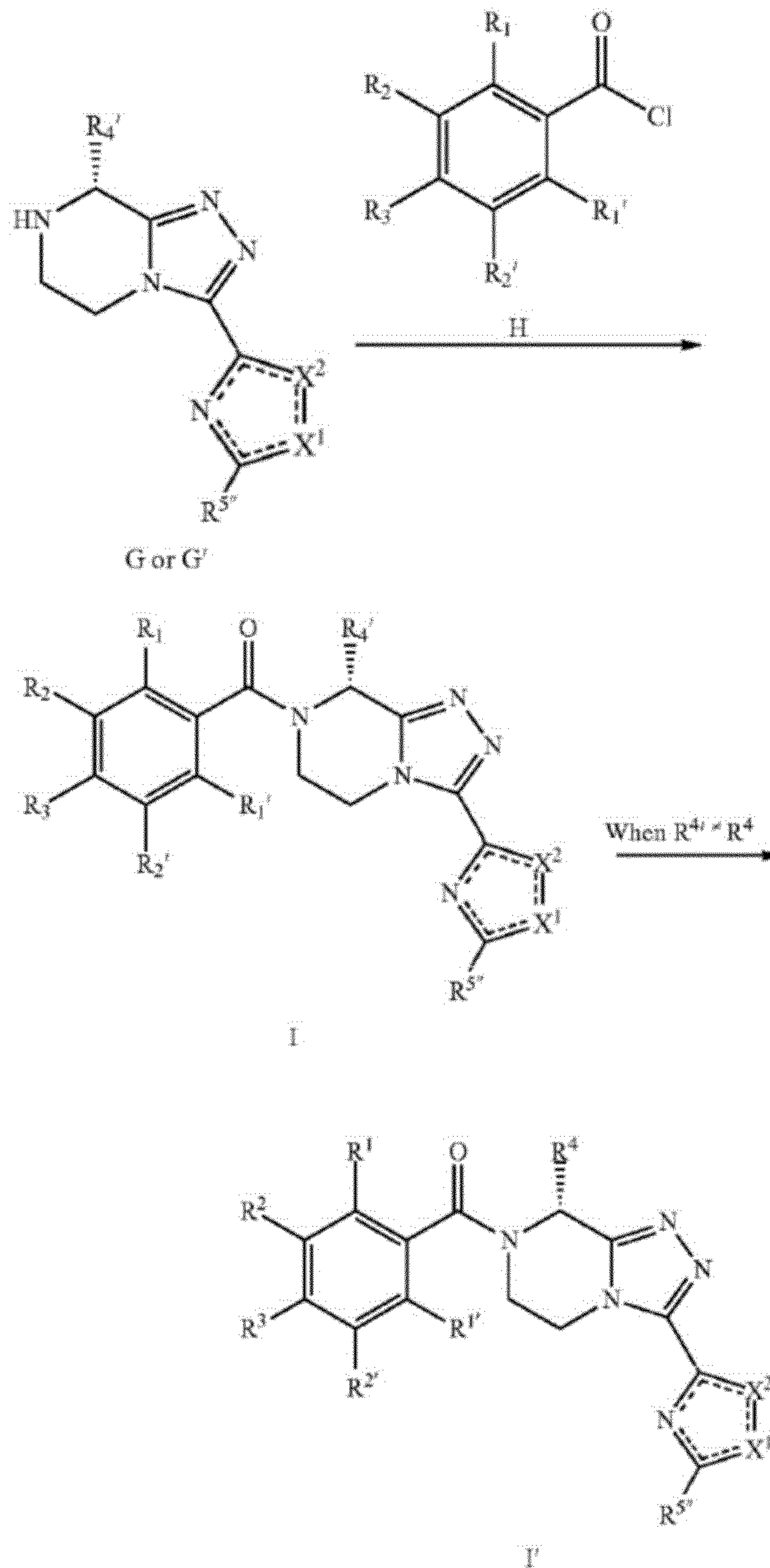
Scheme 16: Acylation.
