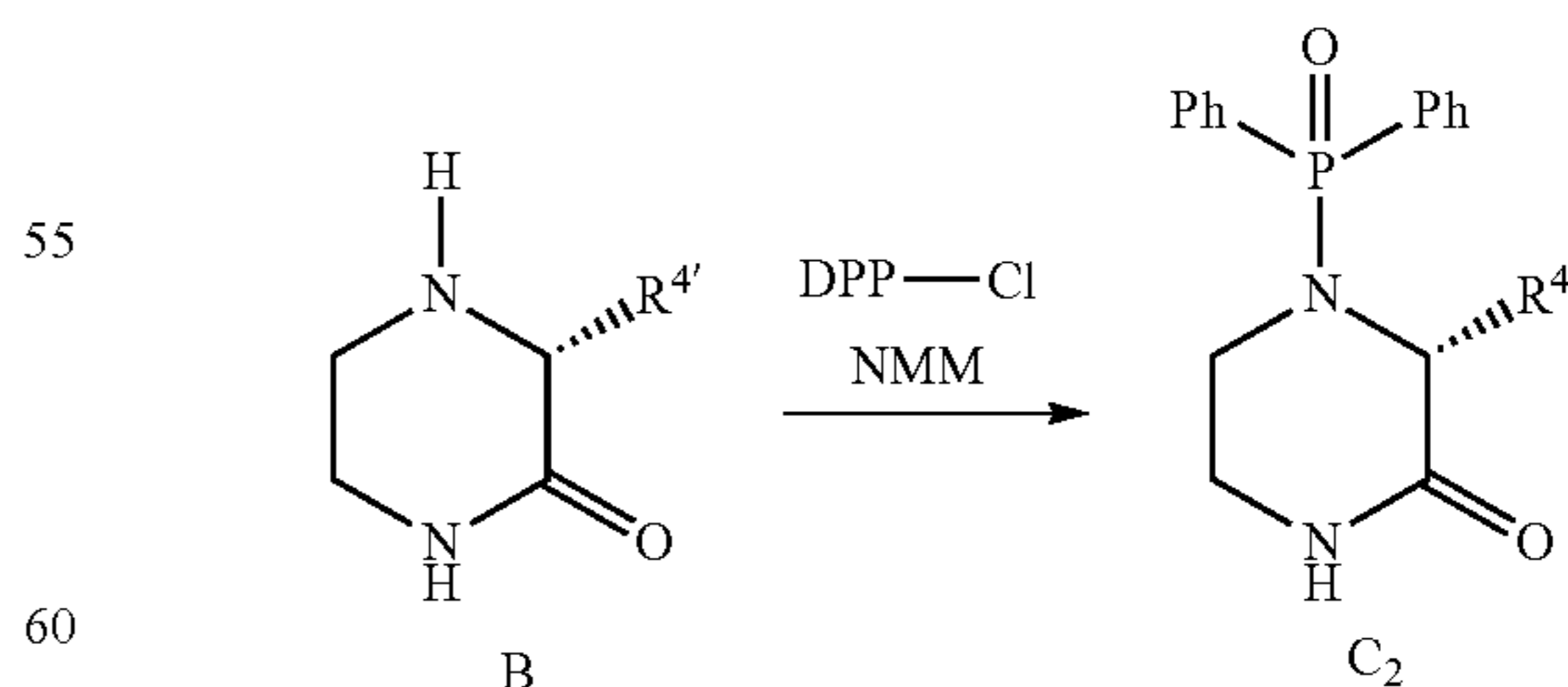
Scheme 9: DPP protection of B.
