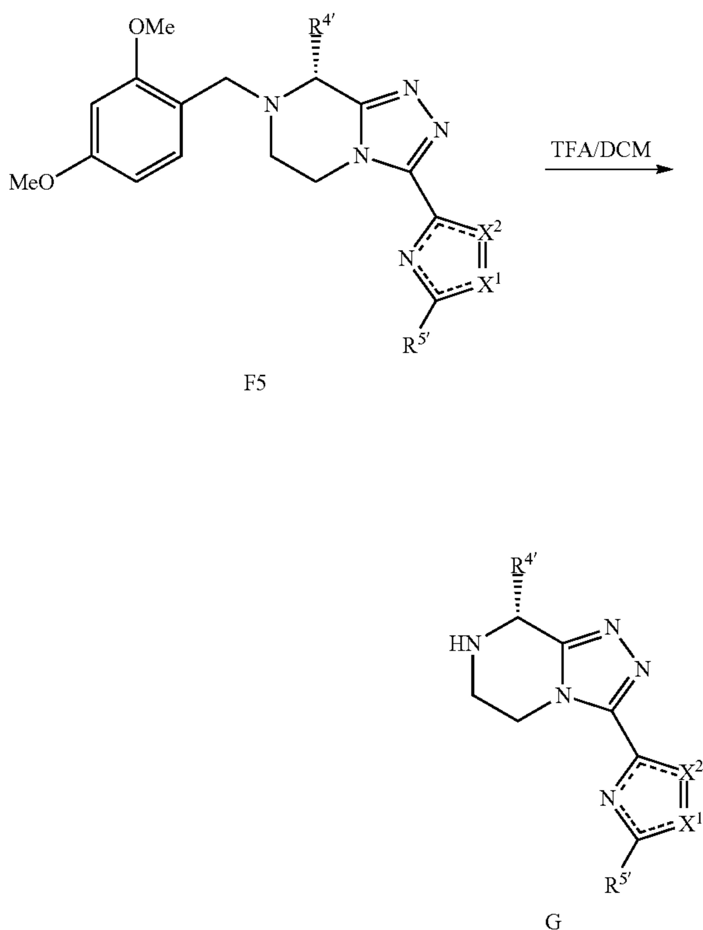
Scheme 14: DMB deprotection.
