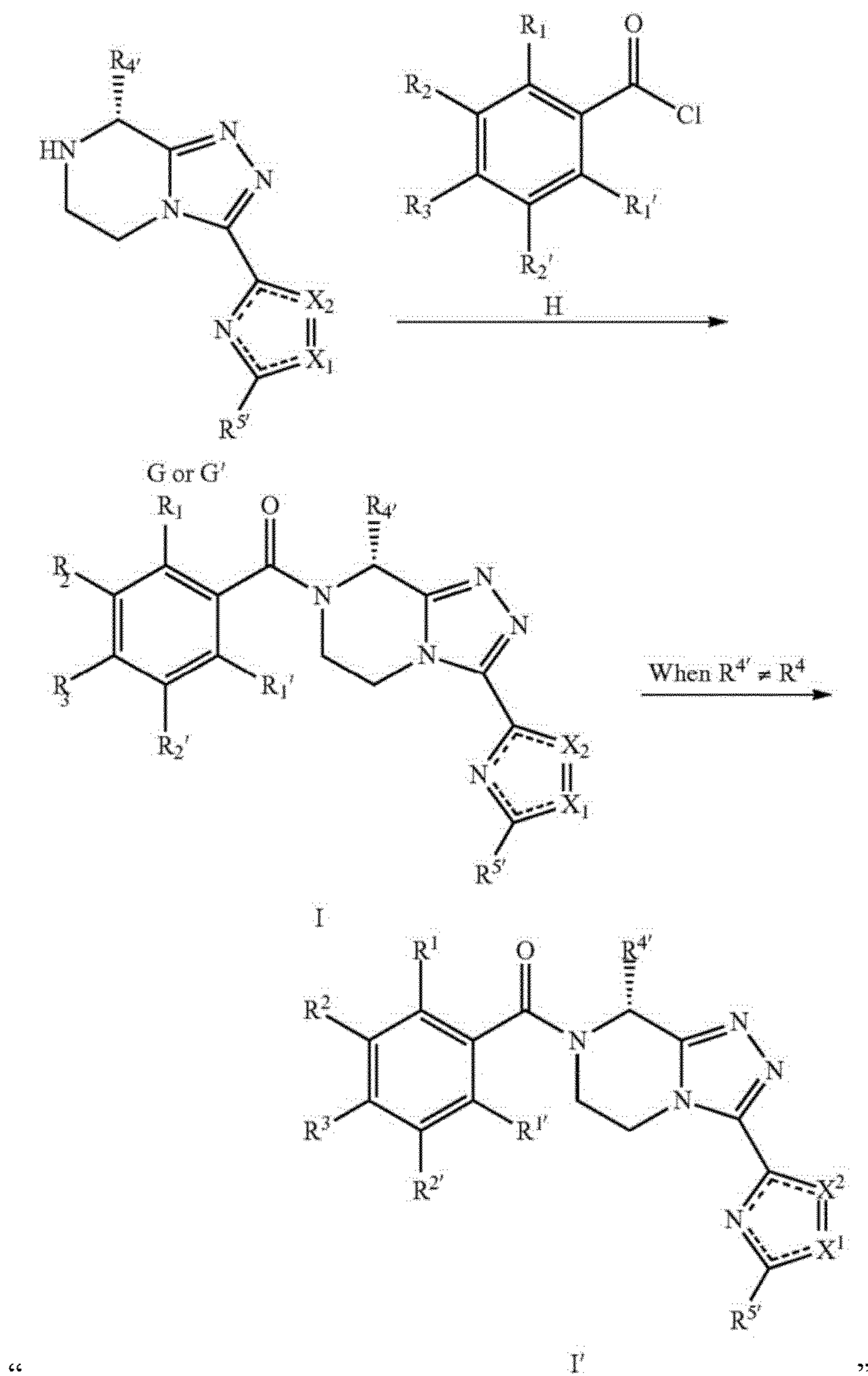
Scheme 16: Acylation.
