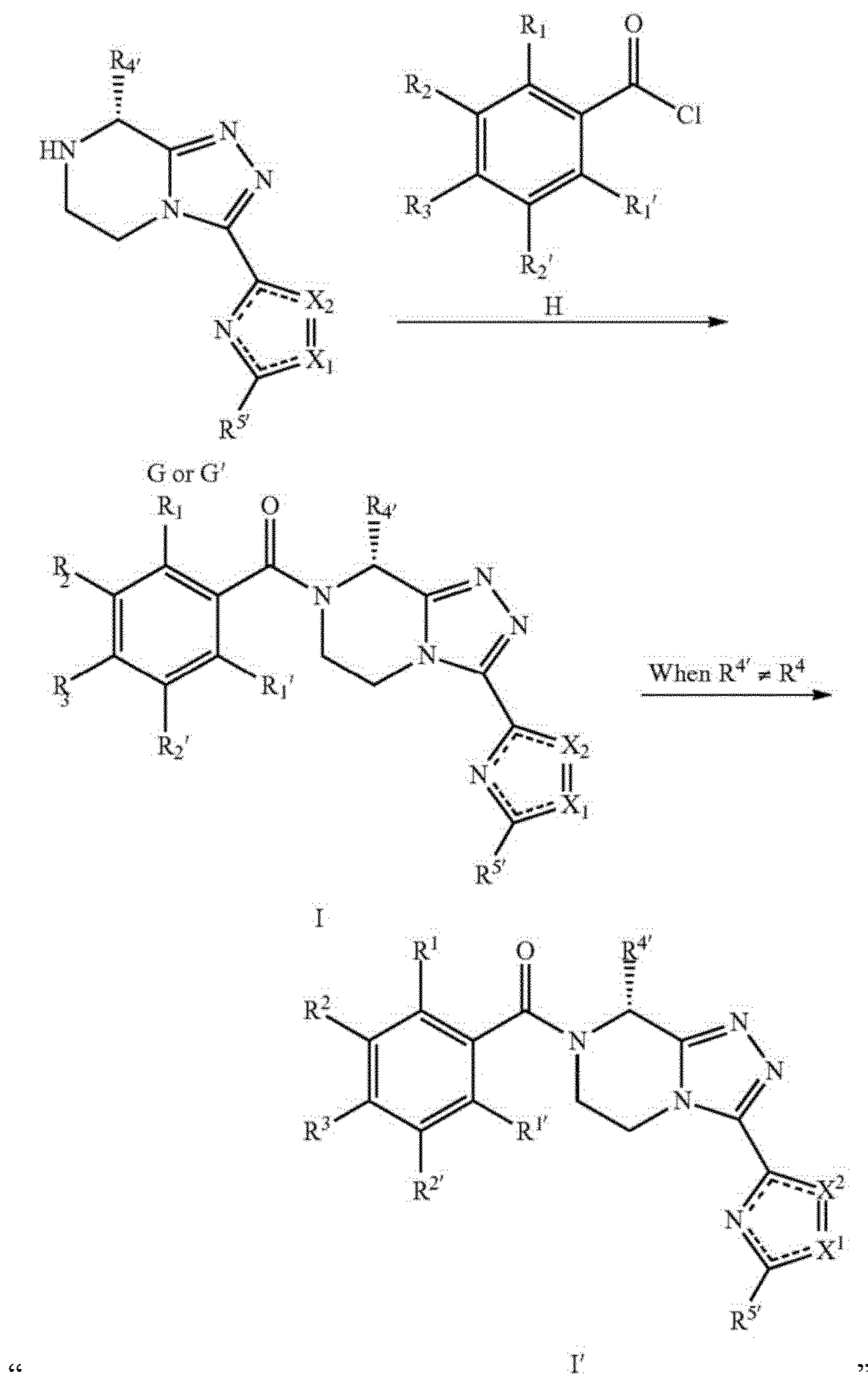
Scheme 16: Acylation.
