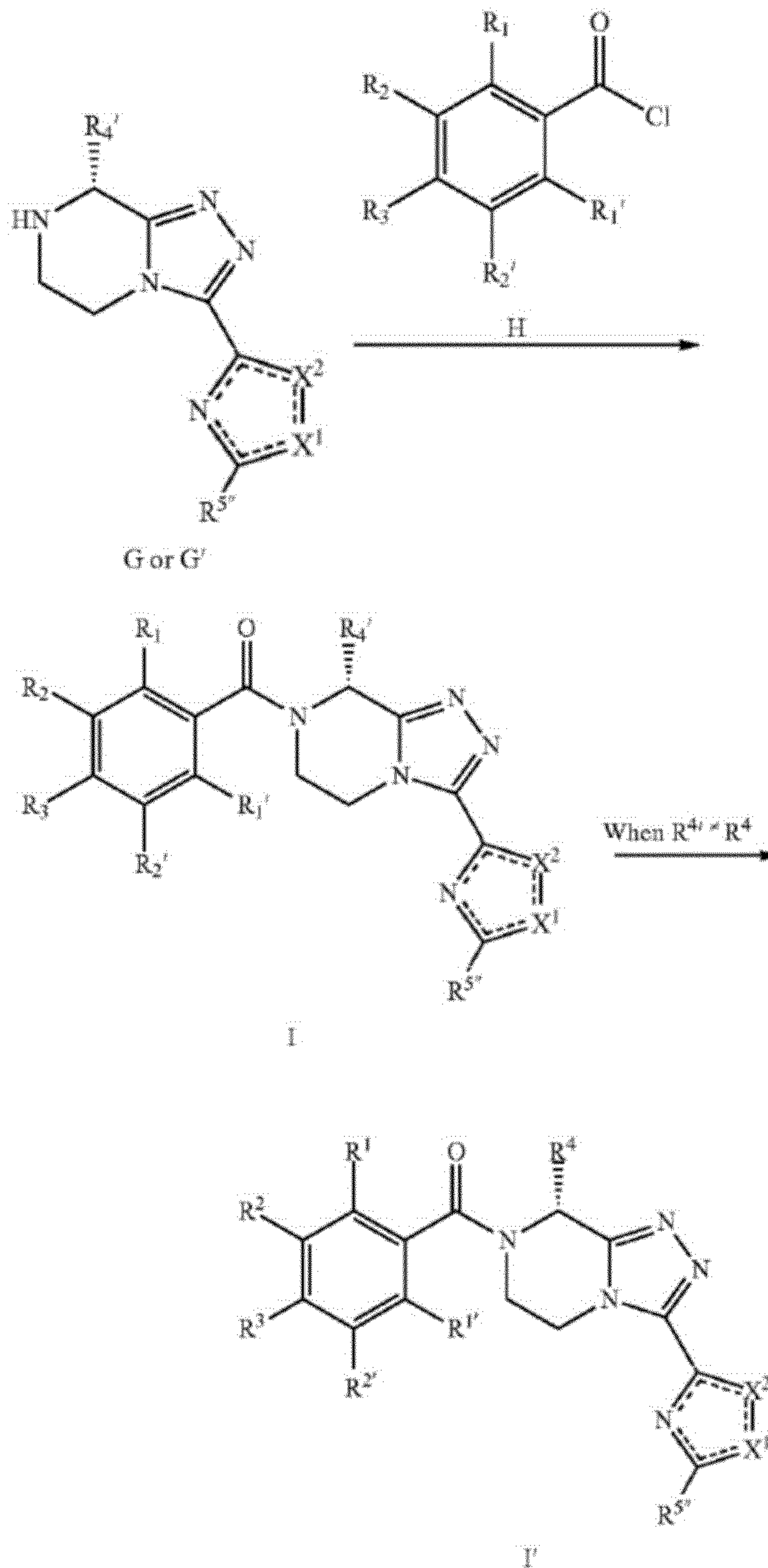
Scheme 16: Acylation.
