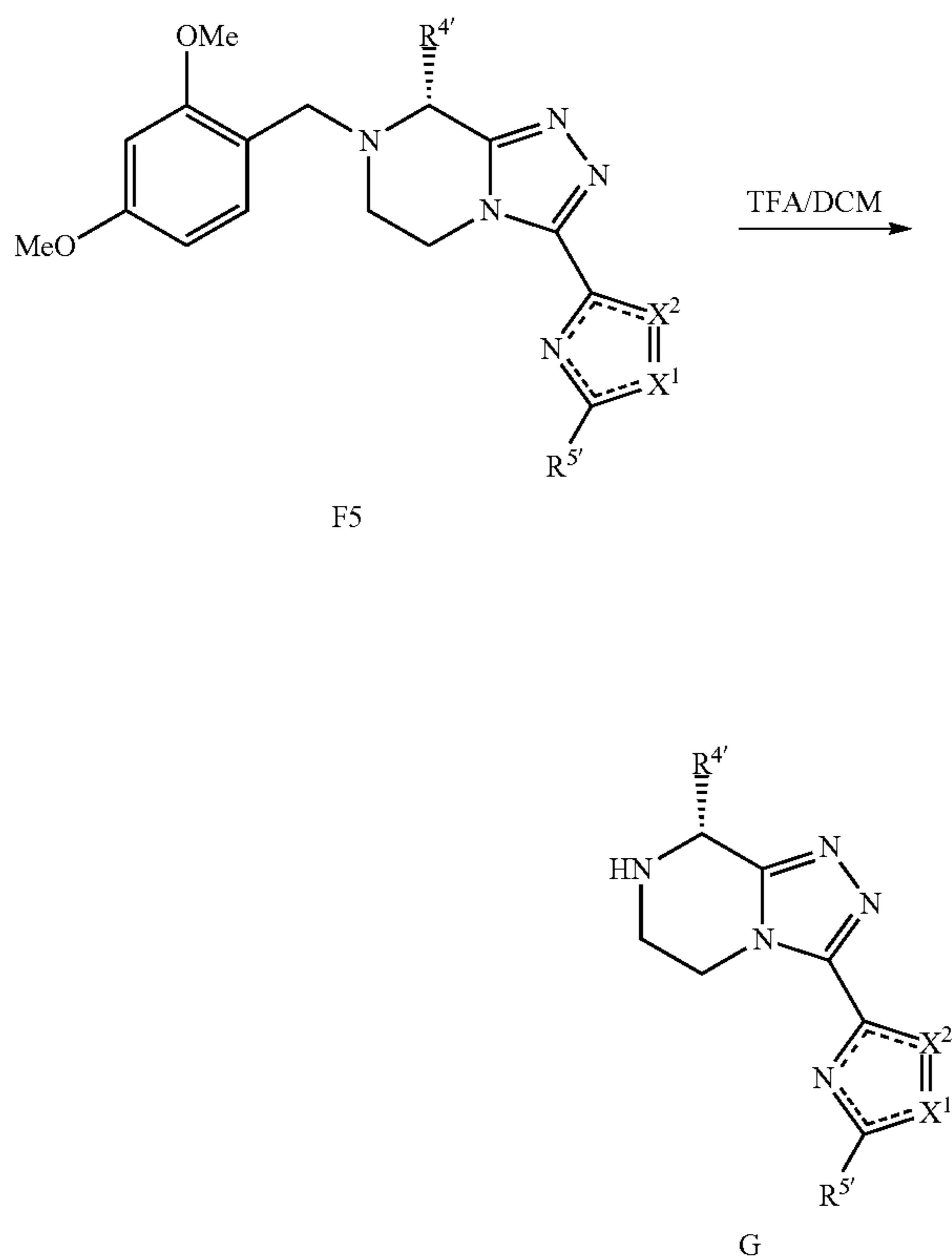
Scheme 14: DMB deprotection.
