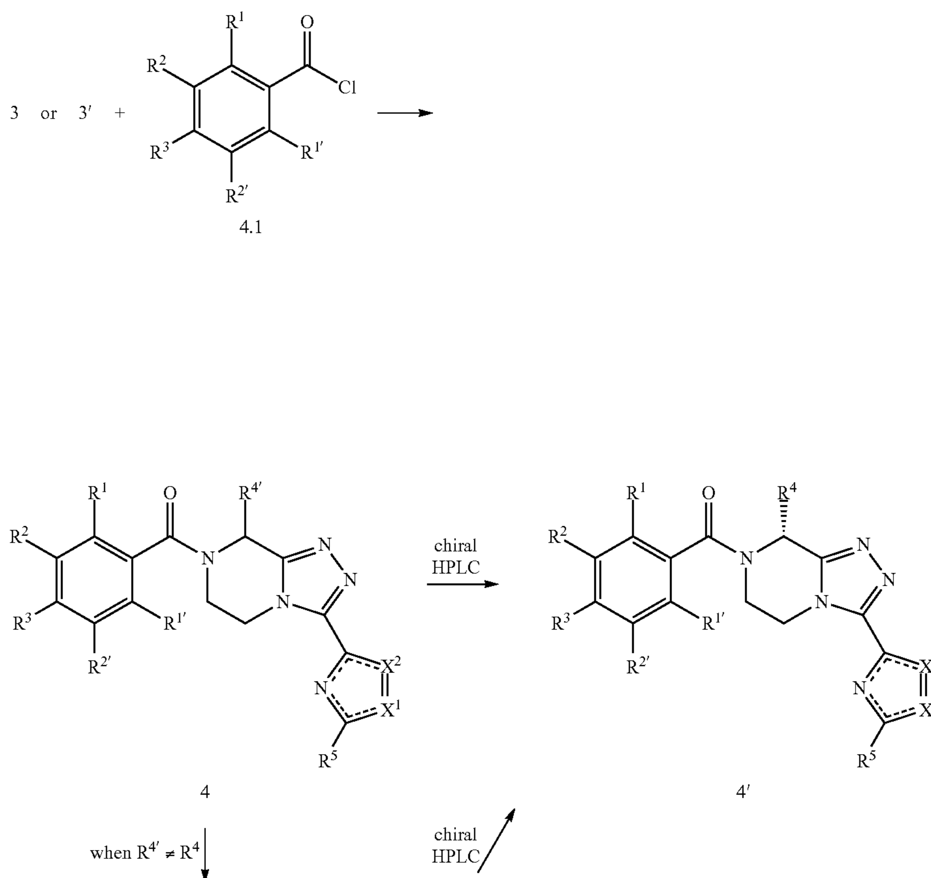
Scheme 6: Acylation and chiral HPLC purification.
