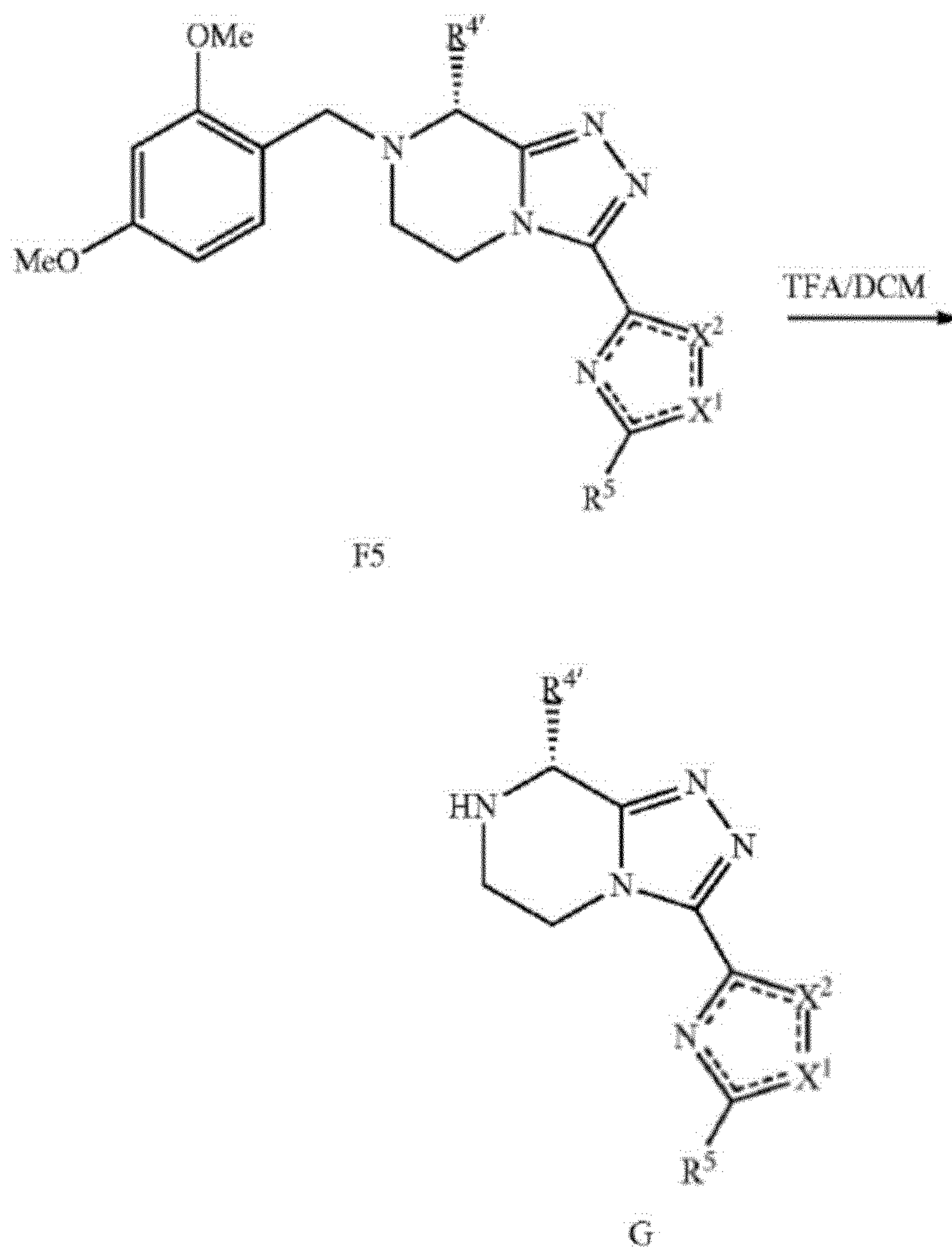
Scheme 14: DMB deprotection.
