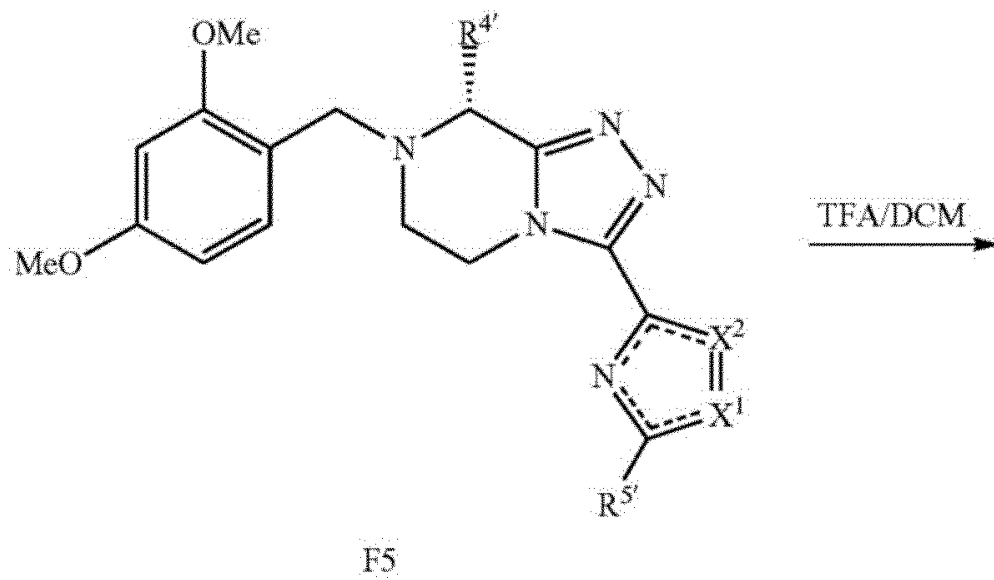
Scheme 14: DMB deprotection.
