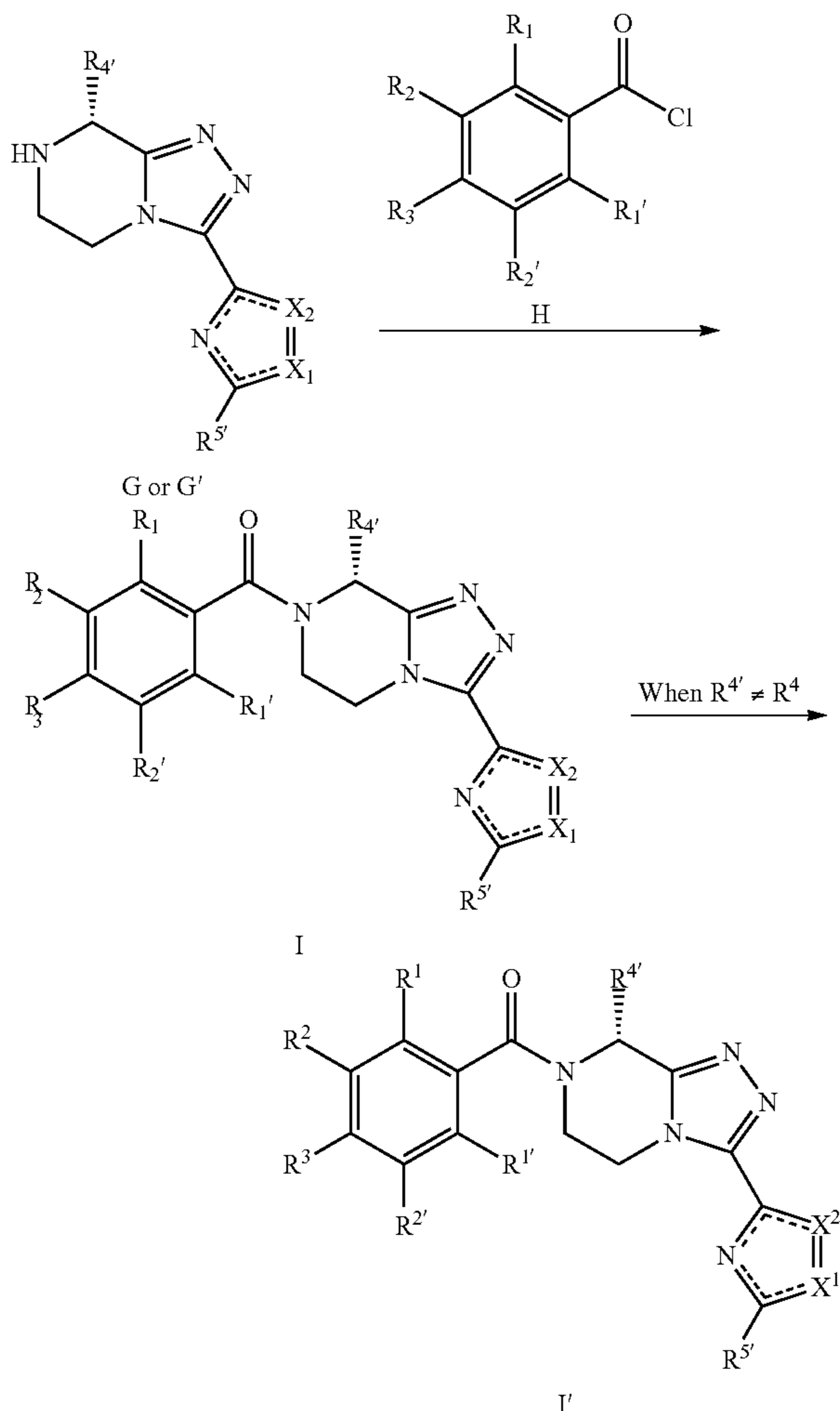
Scheme 16: Acylation.
