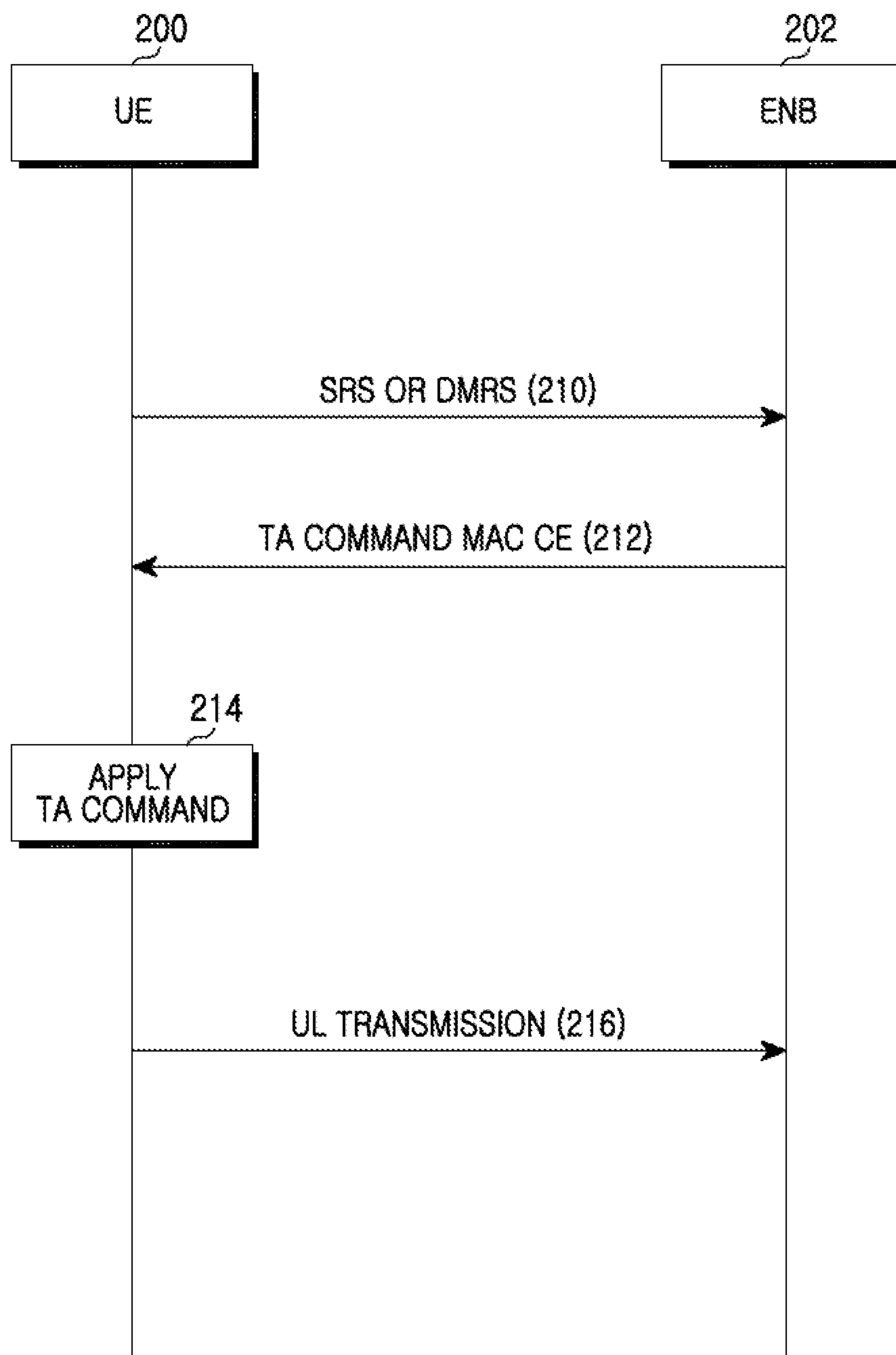
FIG. 2 (PRIOR ART)
