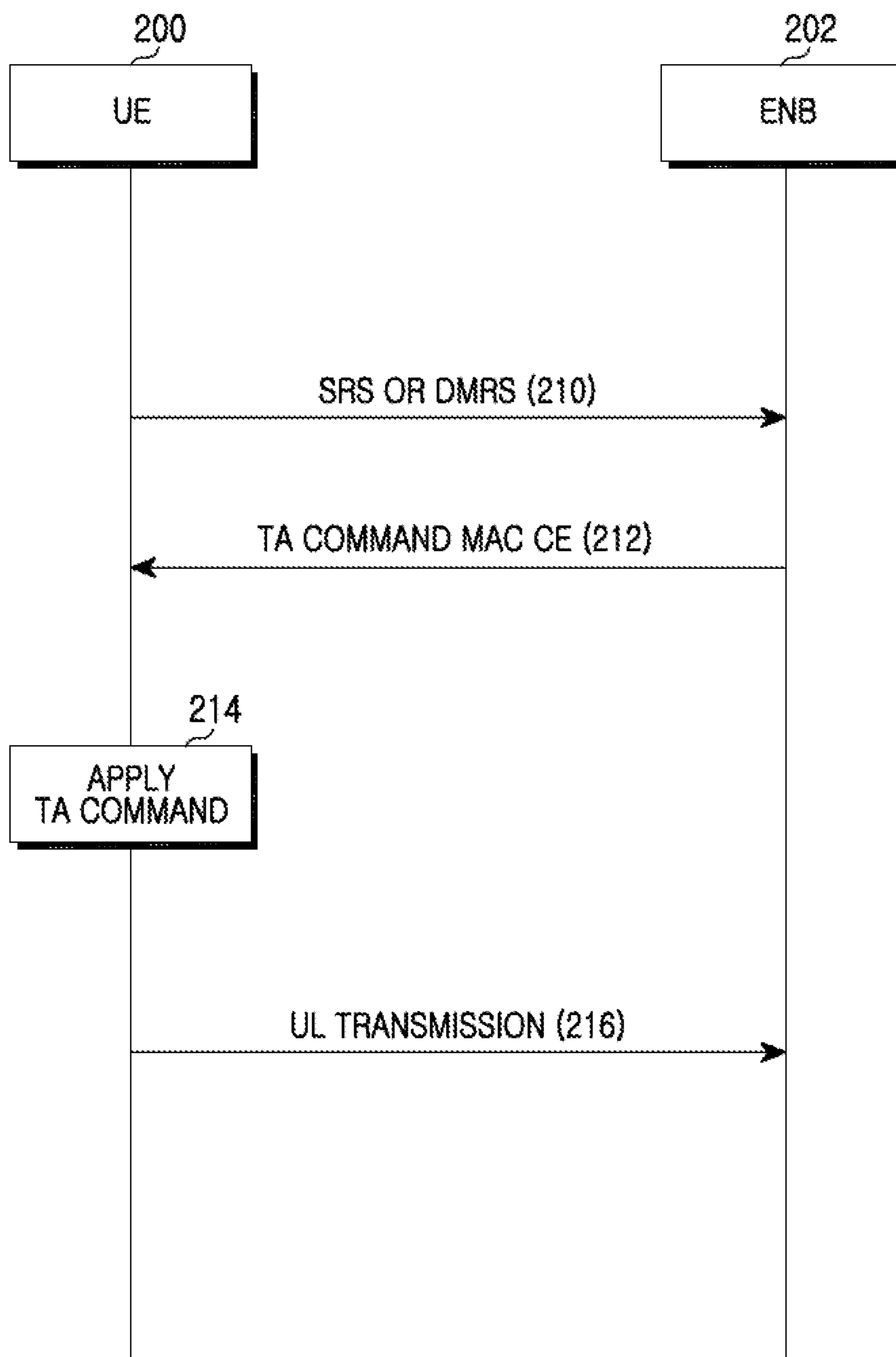
FIG. 2 (PRIOR ART)
