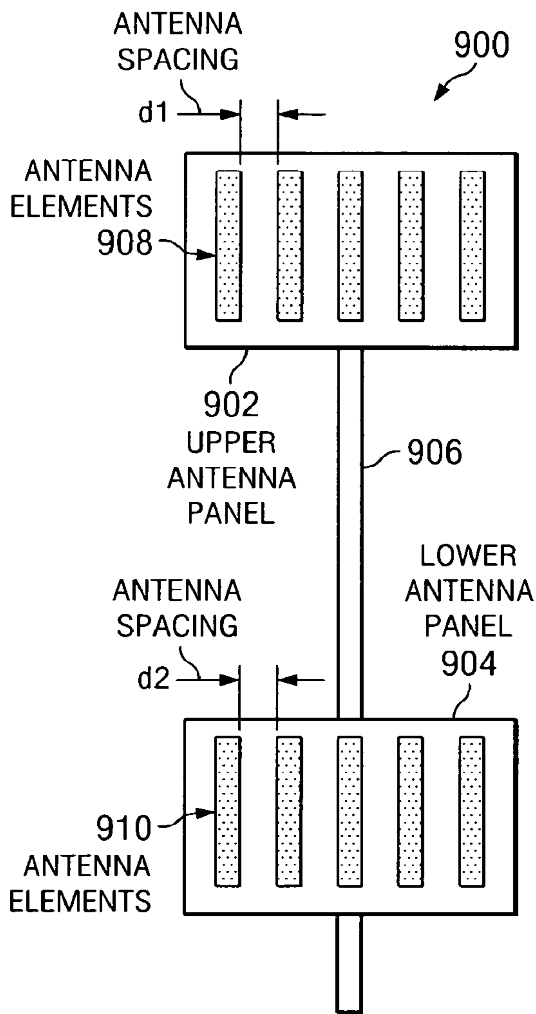
FRONT VIEW
