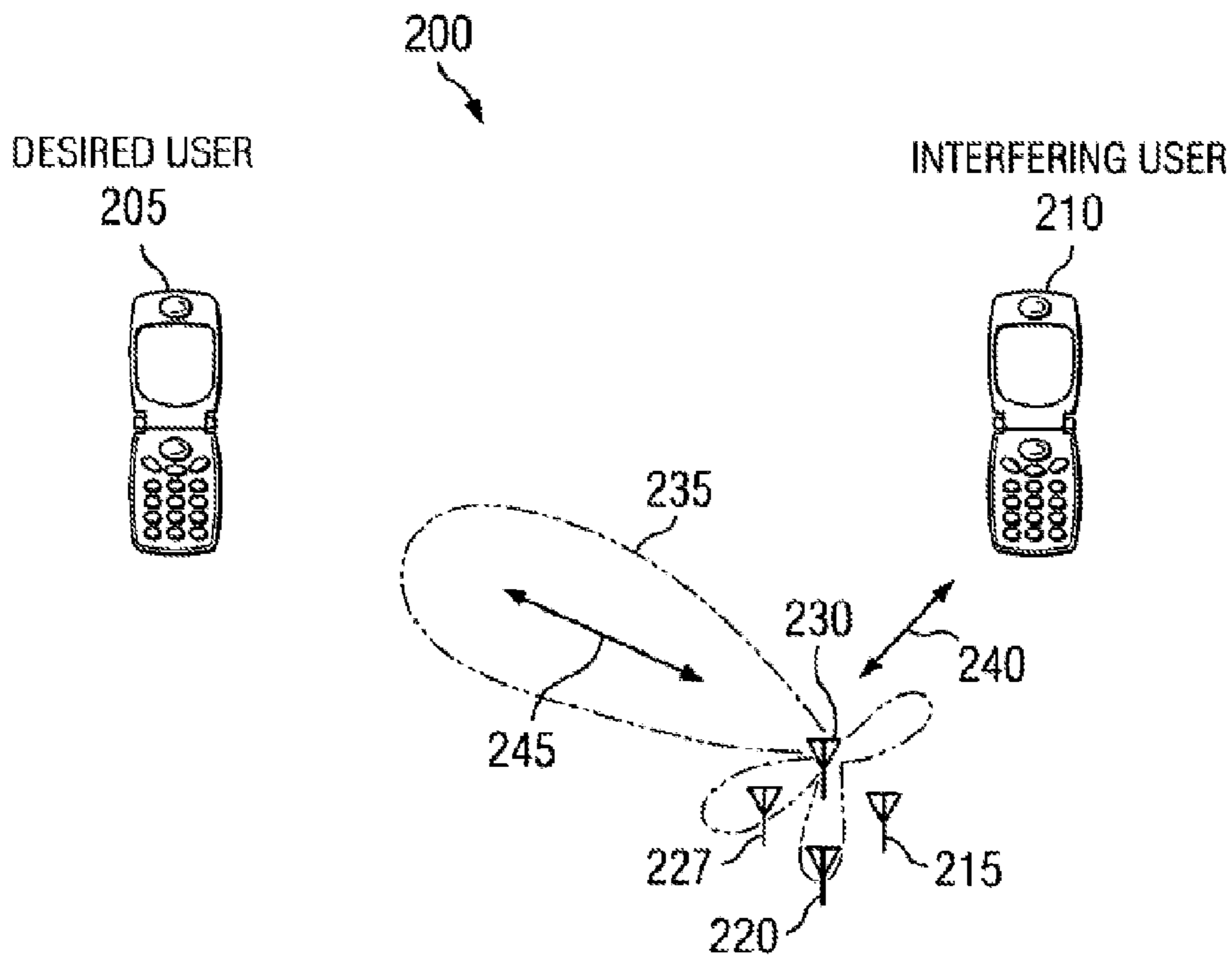
FIG. 2 (PRIOR ART)
