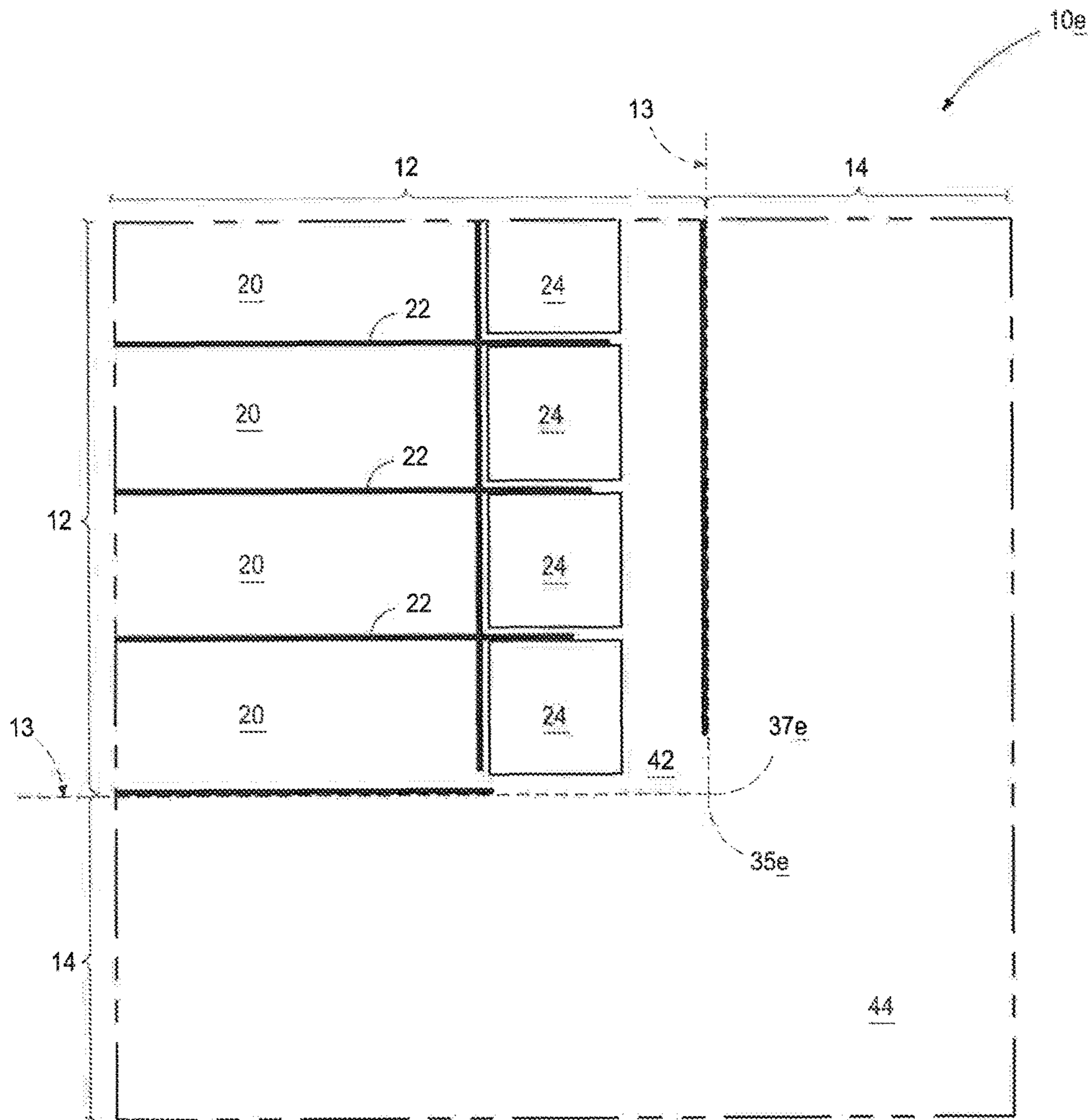
FIG. 8 Predecessor Substrate
