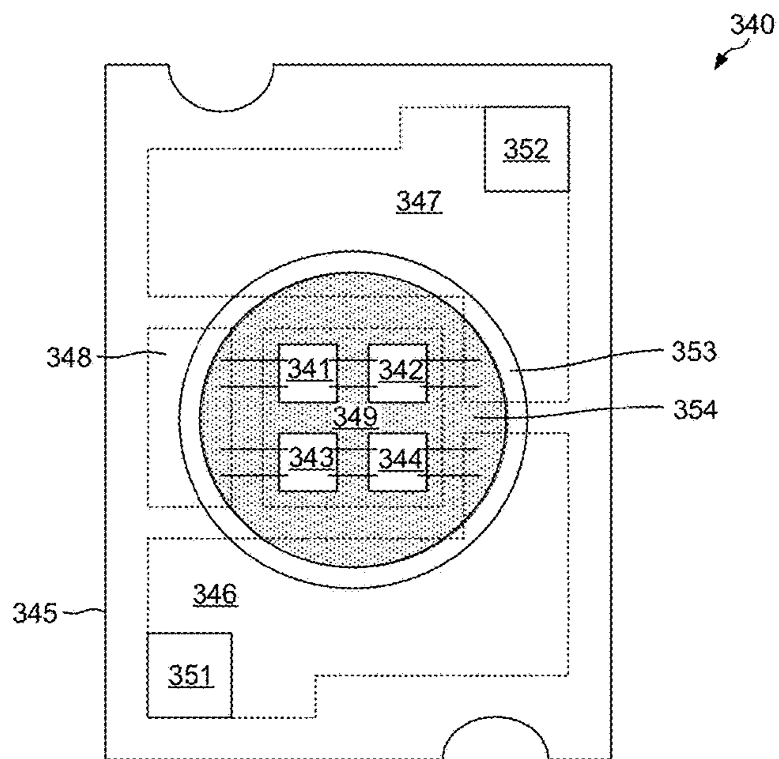
TOP-DOWN VIEW OF A WHITE LED ASSEMBLY
