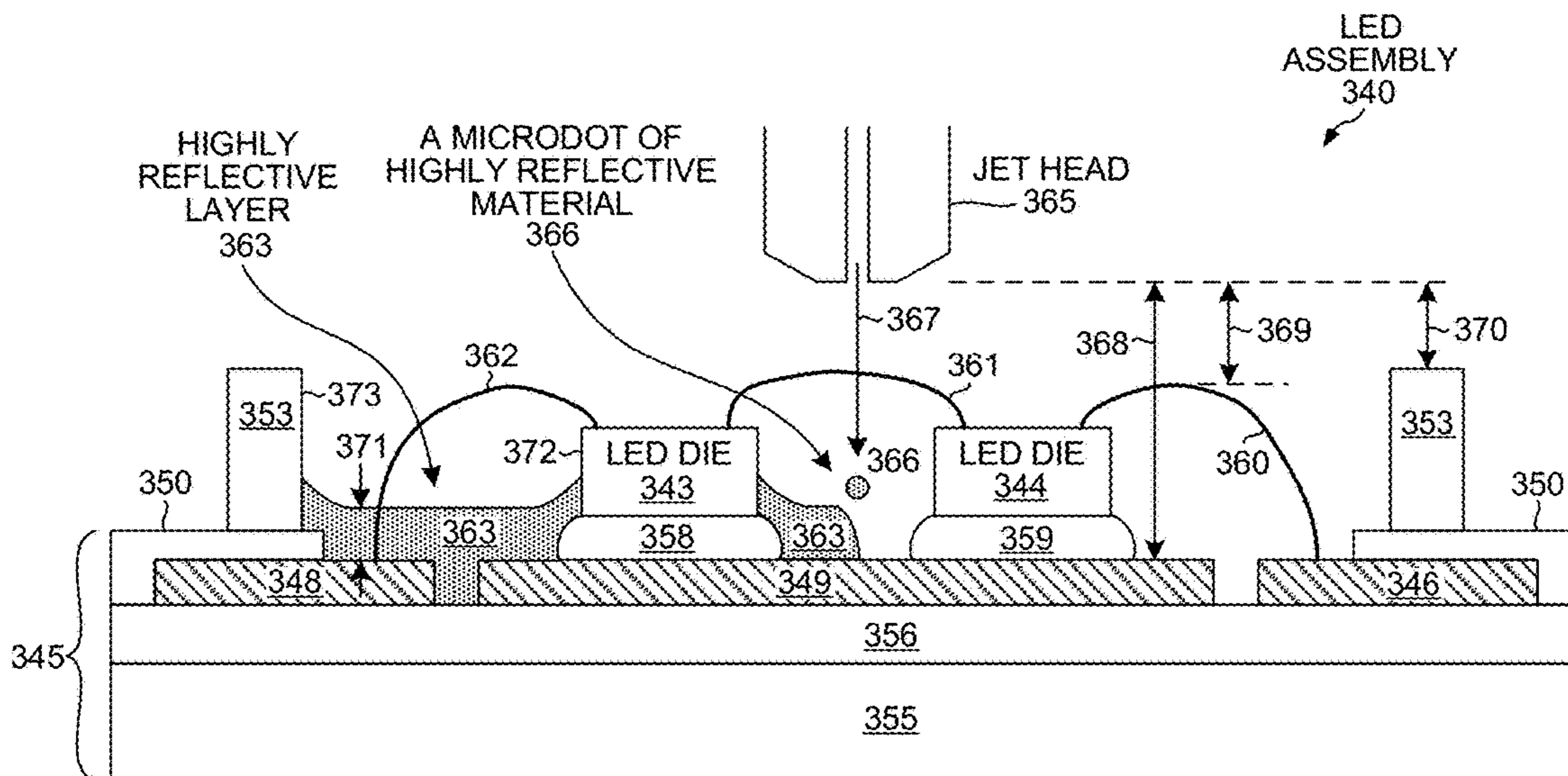
JETTING MICRODOTS OF HR MATERIAL
