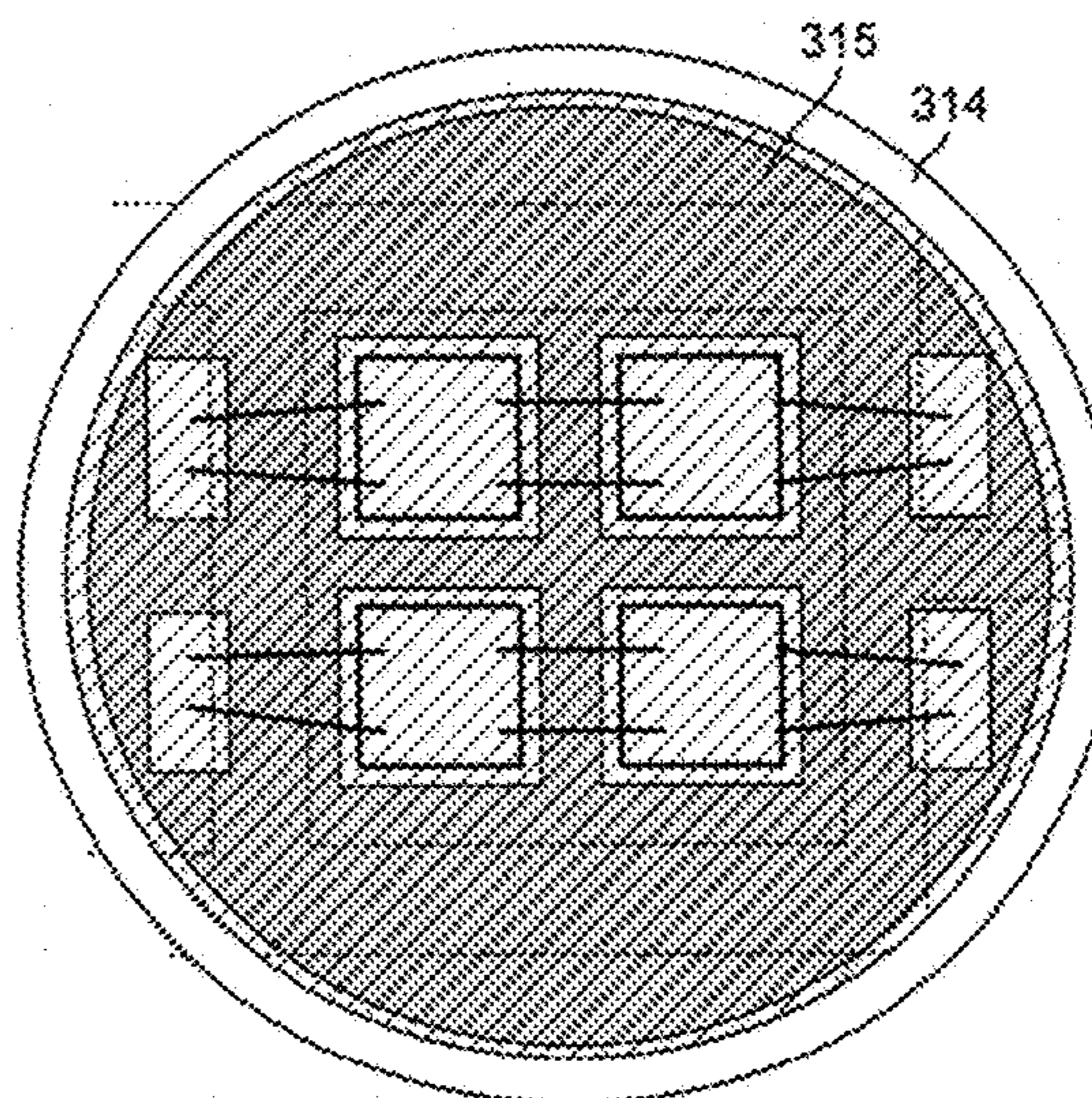
TOP-DOWN VIEW AFTER PLACEMENT OF PHOSPHOR
