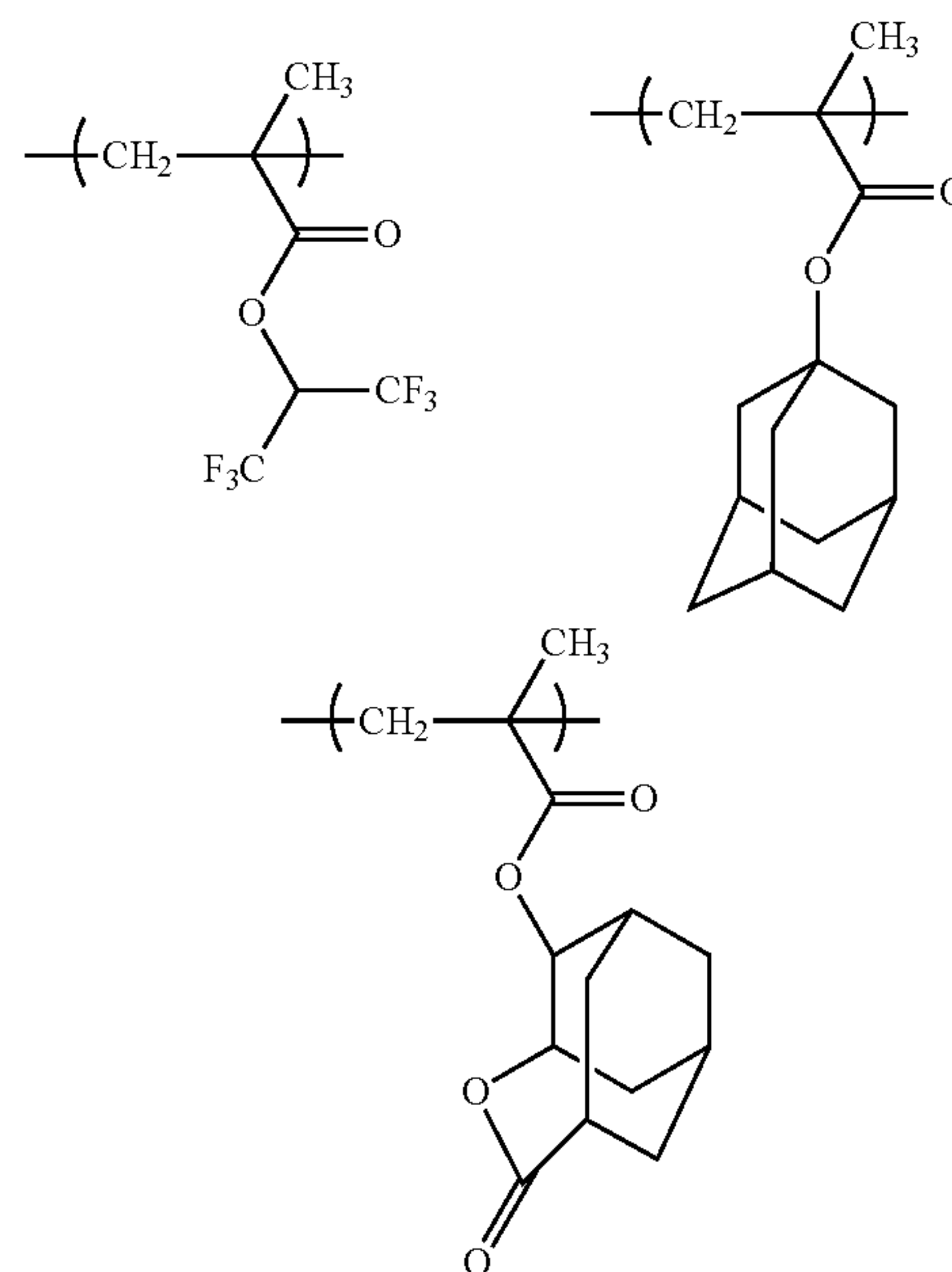
Example 7: Synthesis of Resin A1-7
