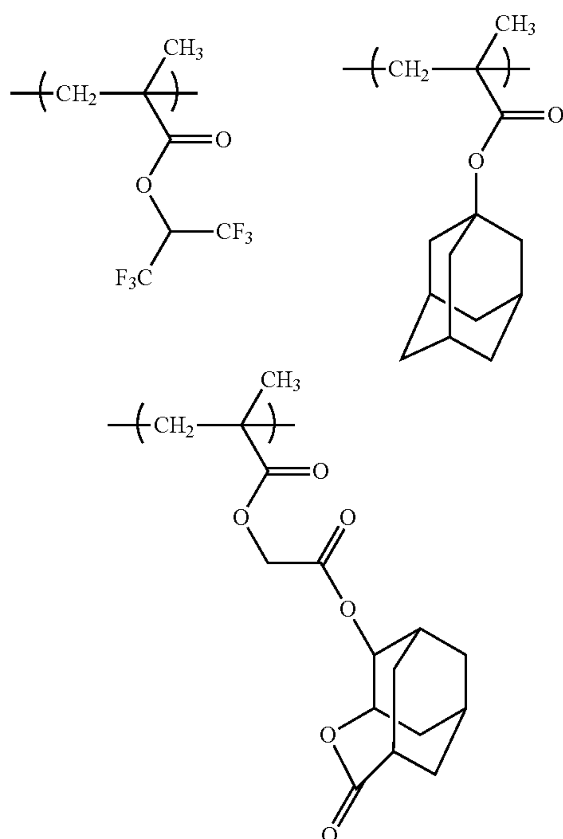
Example 8: Synthesis of Resin A1-8
