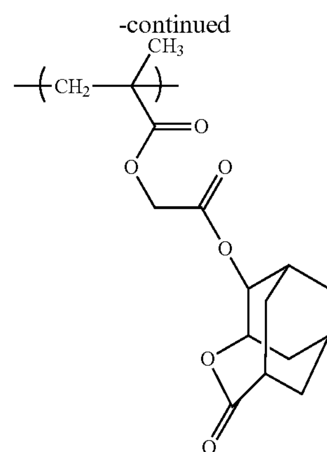
Example 6: Synthesis of Resin A1-6
