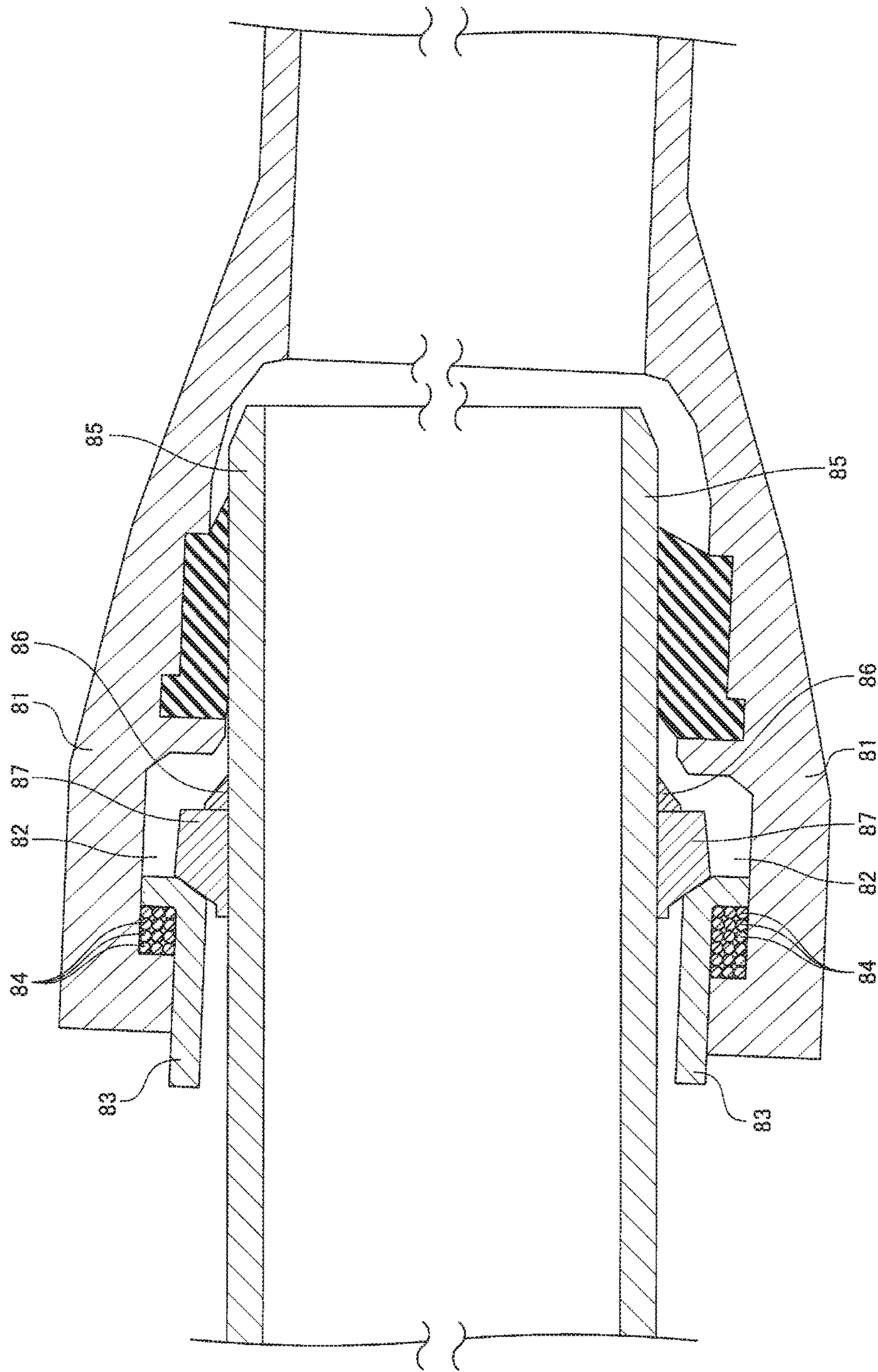
FIG. 10 PRIOR ART
