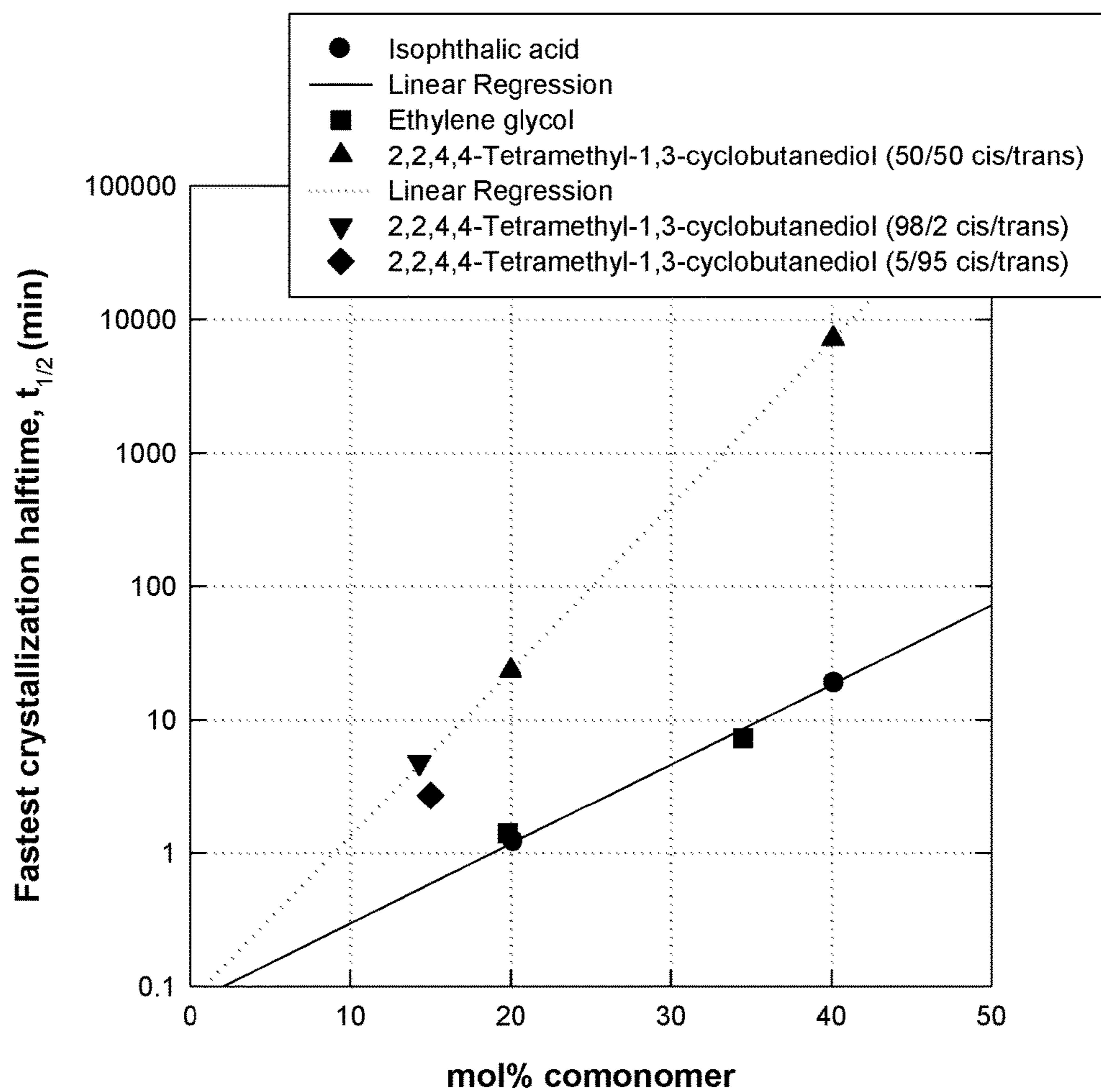
Figure 1: The effect of comonomer on the fastest crystallization half-times of modified PCT copolyesters
