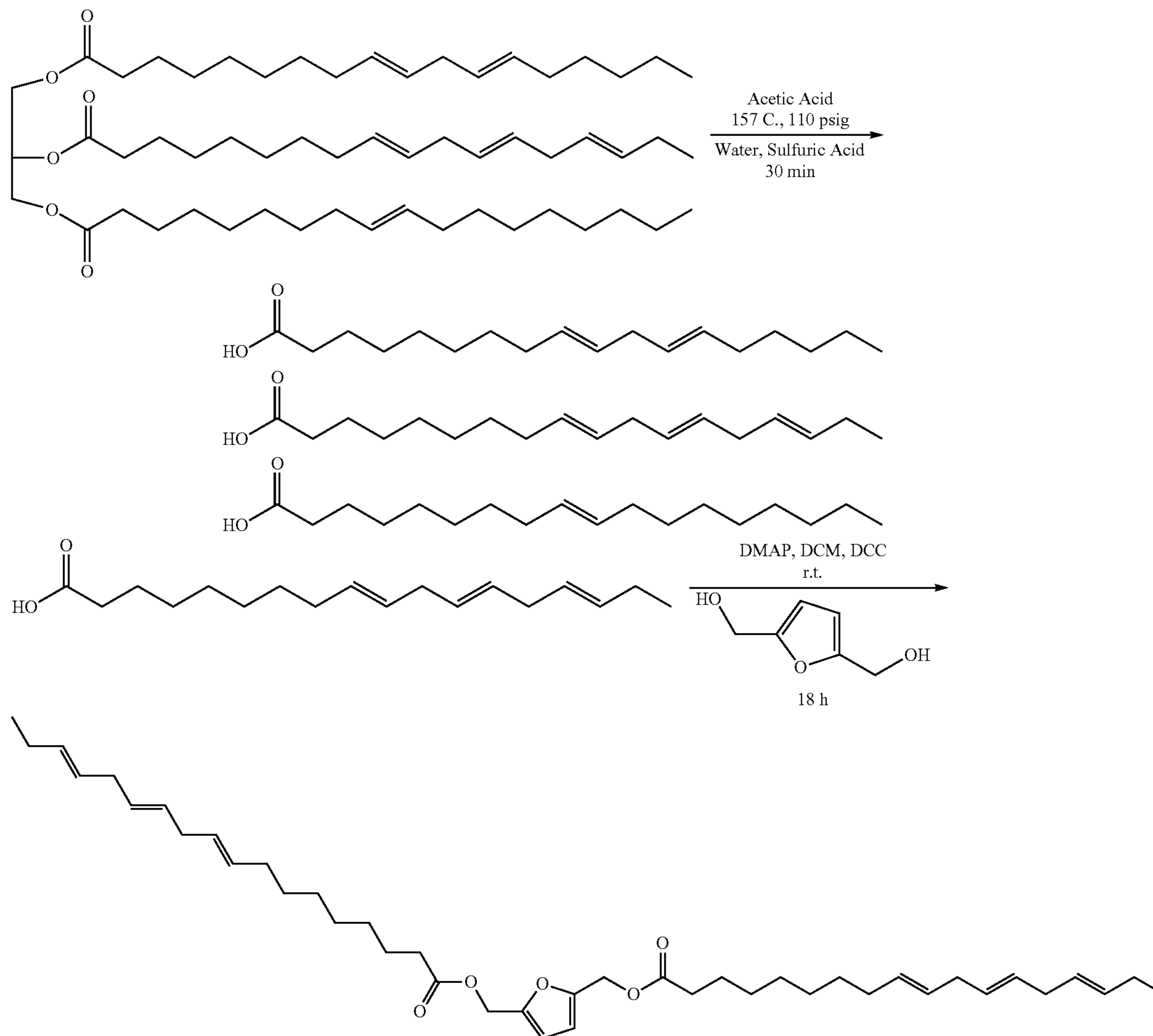
Reaction Scheme 1
