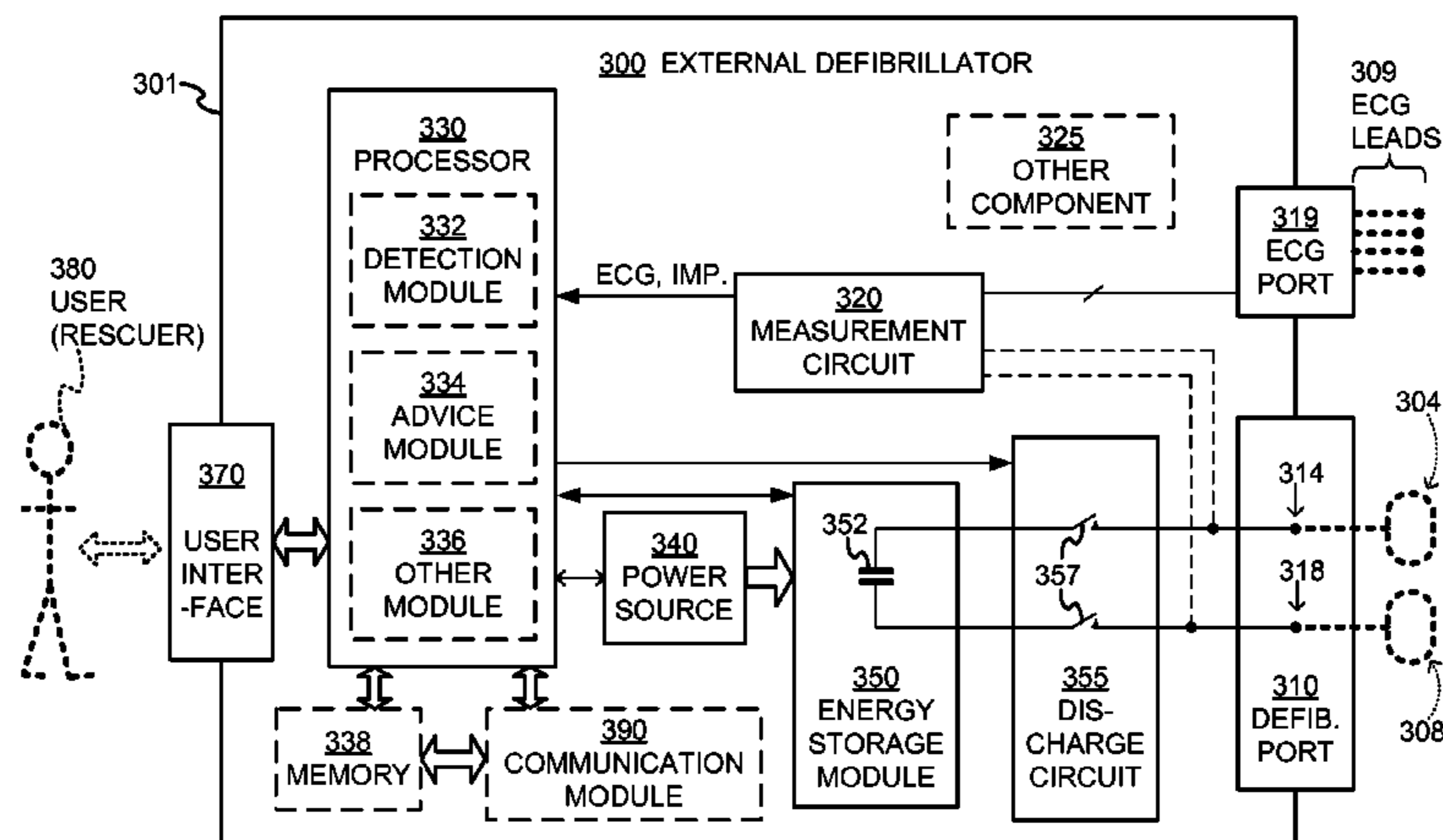
COMPONENTS OF EXTERNAL DEFIBRILLATOR
