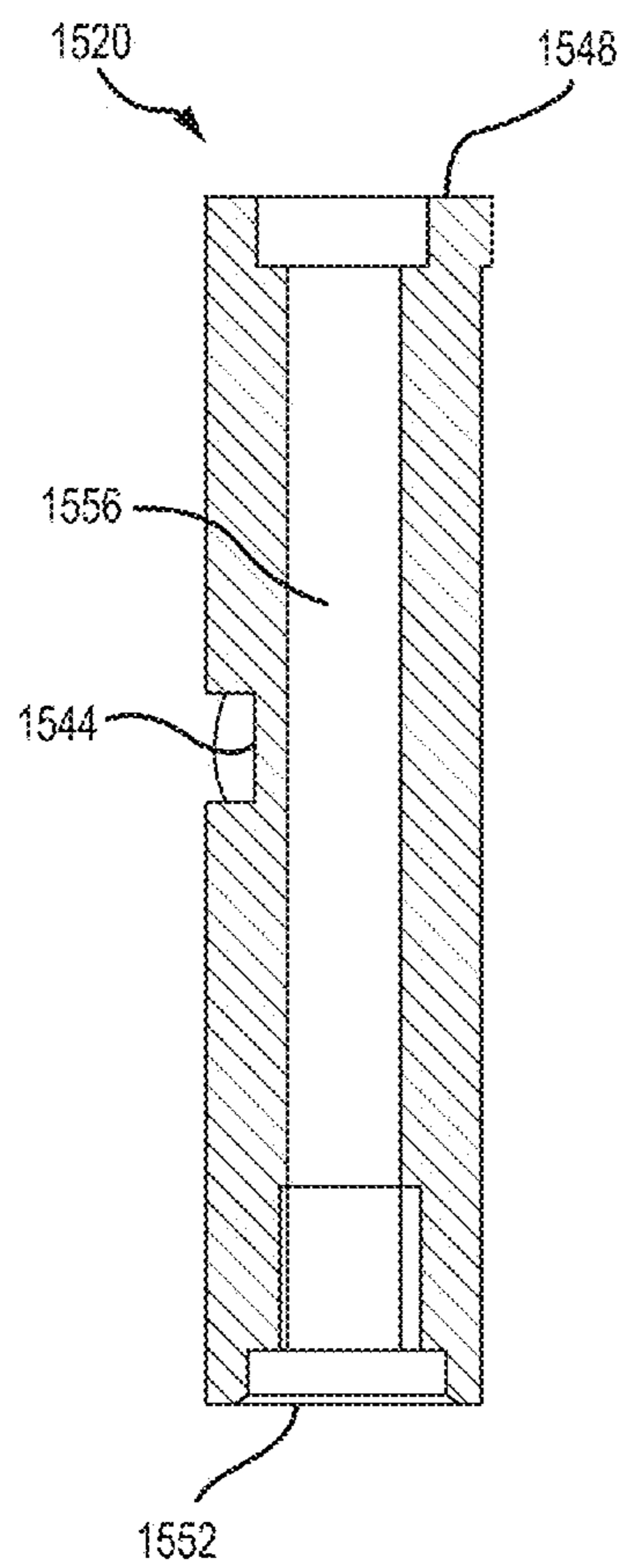
SECTION F-F
