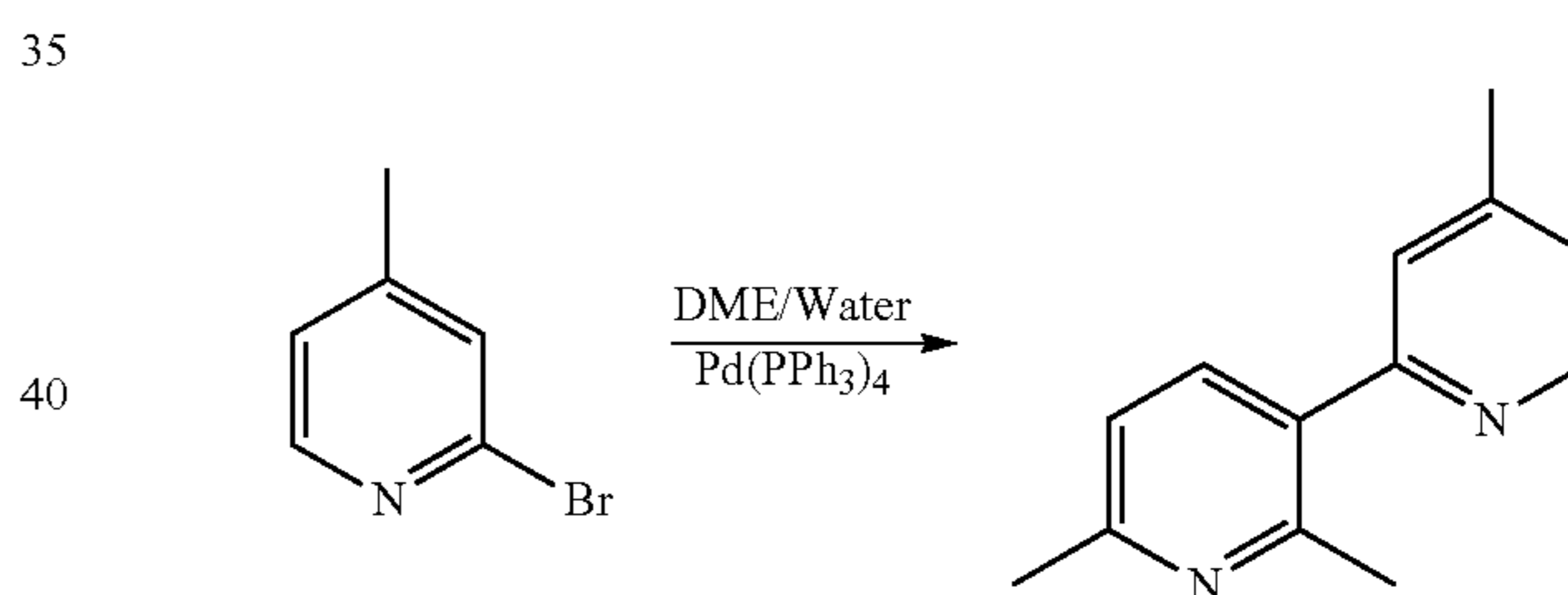
Synthesis of 2',4,6'-trimethyl-2,3'-bipyridine
