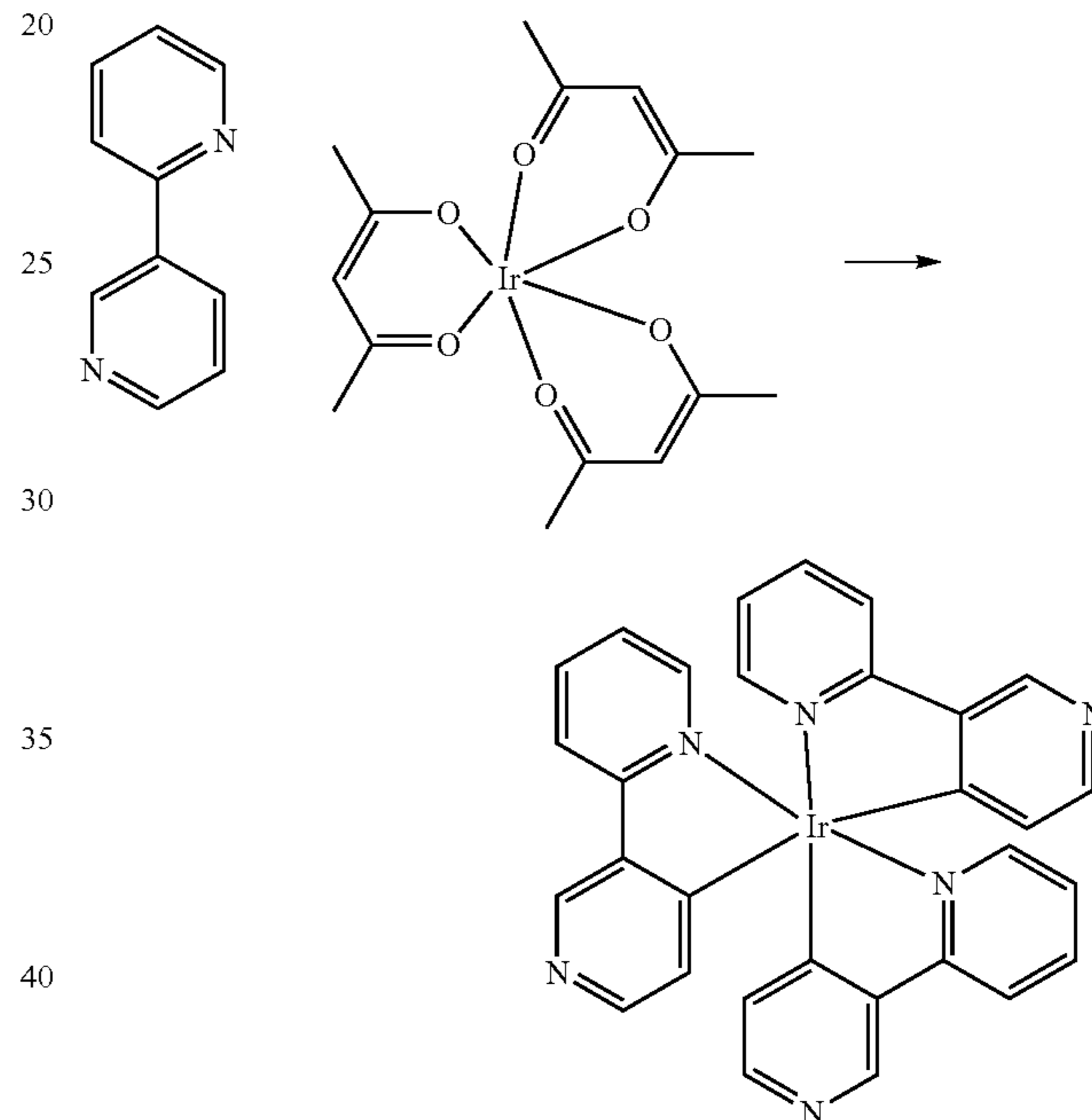
Synthesis of Compound 13
