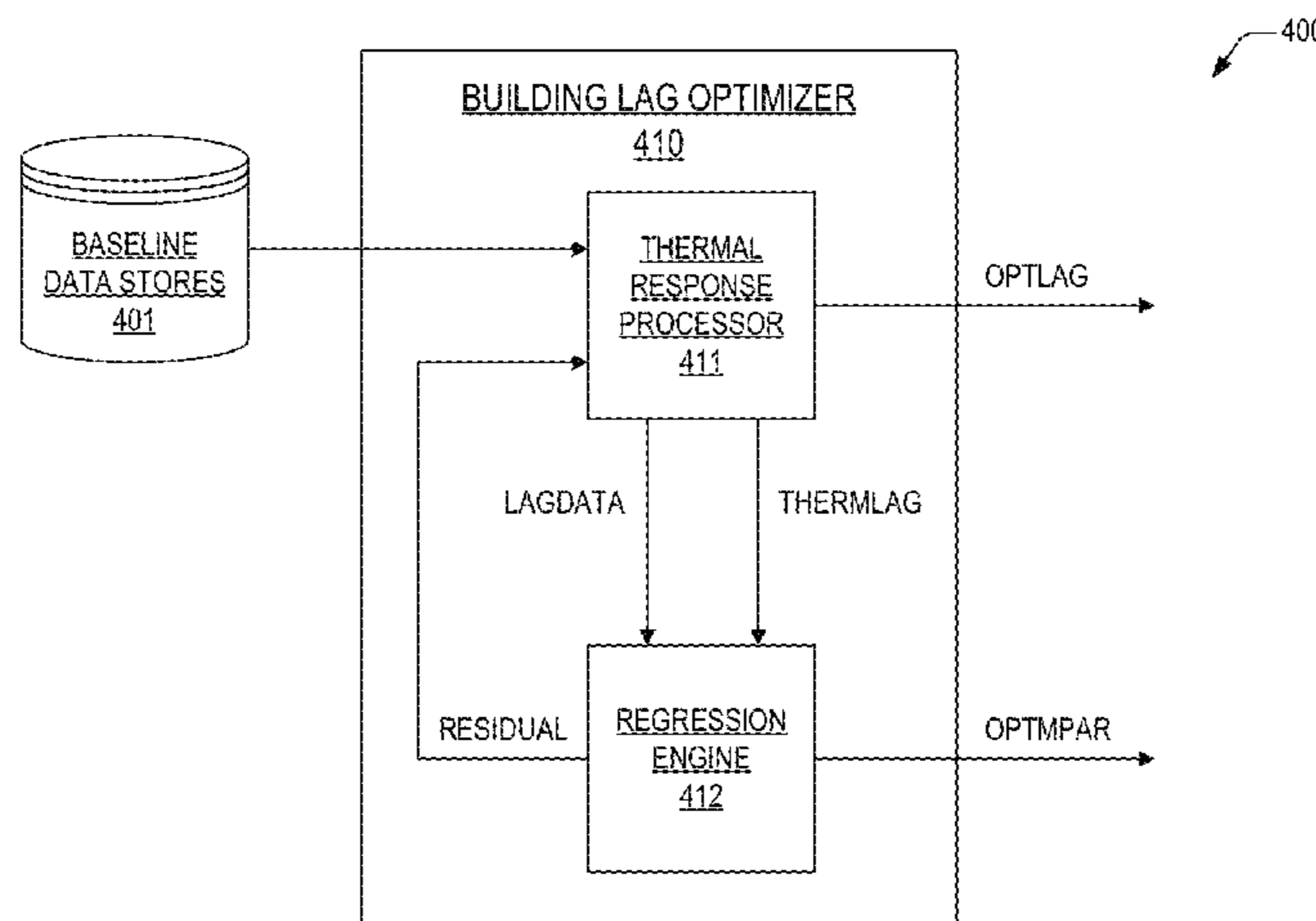
FINE-GRAINED BASELINE ENERGY DATA WEATHER NORMALIZATION APPARATUS
