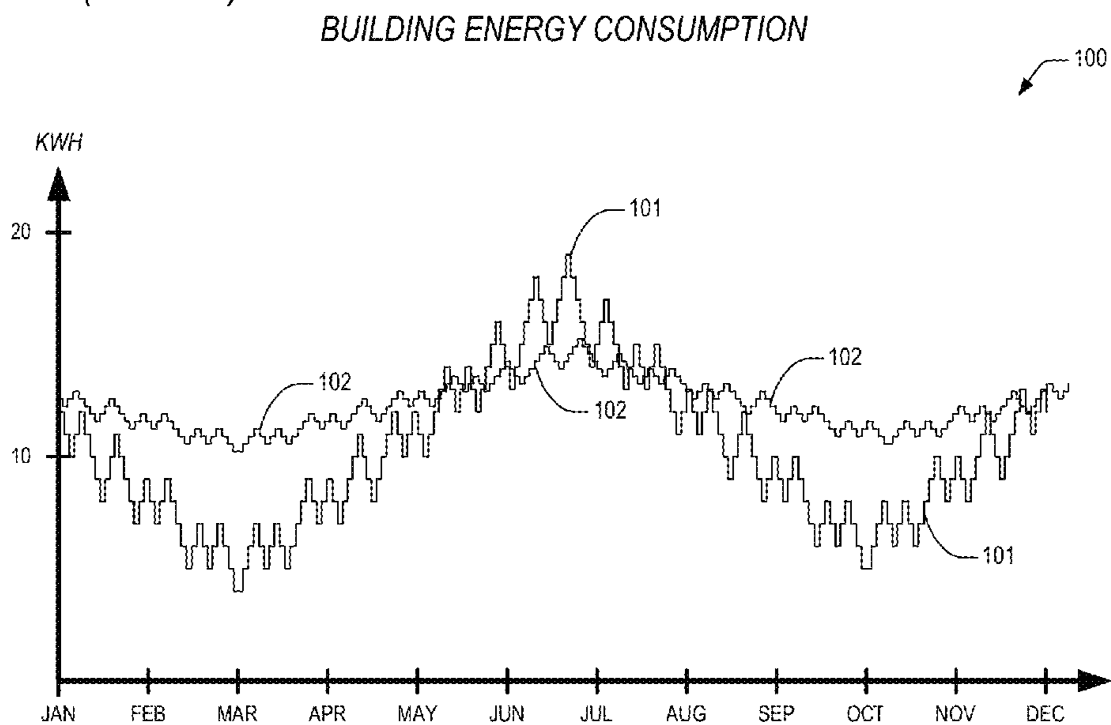
FIG. 1 (Prior Art)
