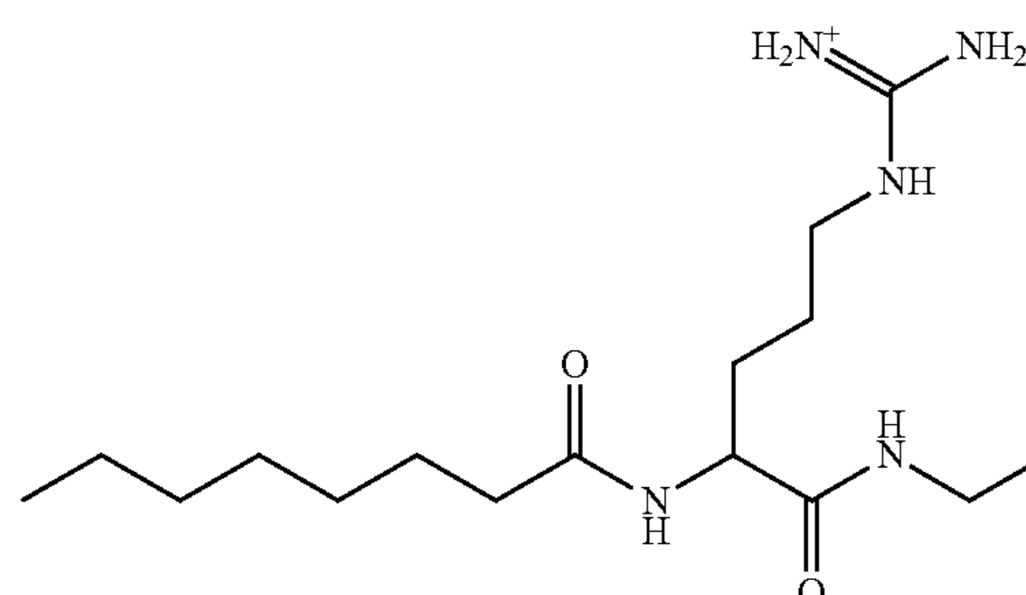
[amino({[4-(ethylcarbamoyl)-4-octanamidobutyl]amino})methylidene]azanium;
