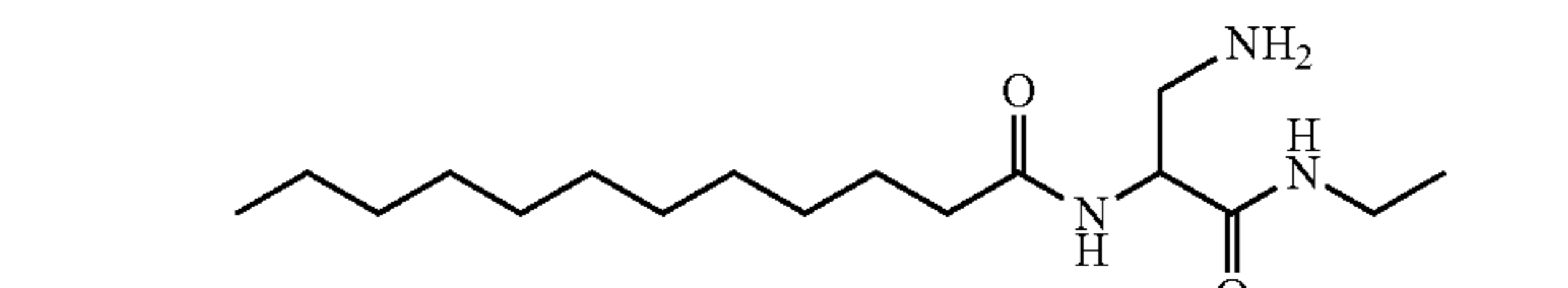
N-[2-amino-1-(ethylcarbamoyl)ethylol]dodecanamide;
