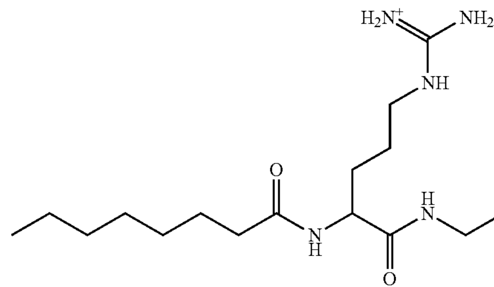
[amino({[4-(ethylcarbamoyl)-4-octanamidobutyl]amino})methylidene]azanium;
