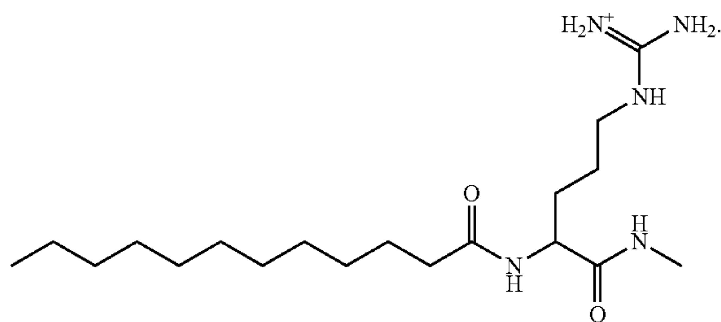
[amino({[4-dodecanamido-4-(methylcarbamoyl)butyl]amino})methylidene]azanium
