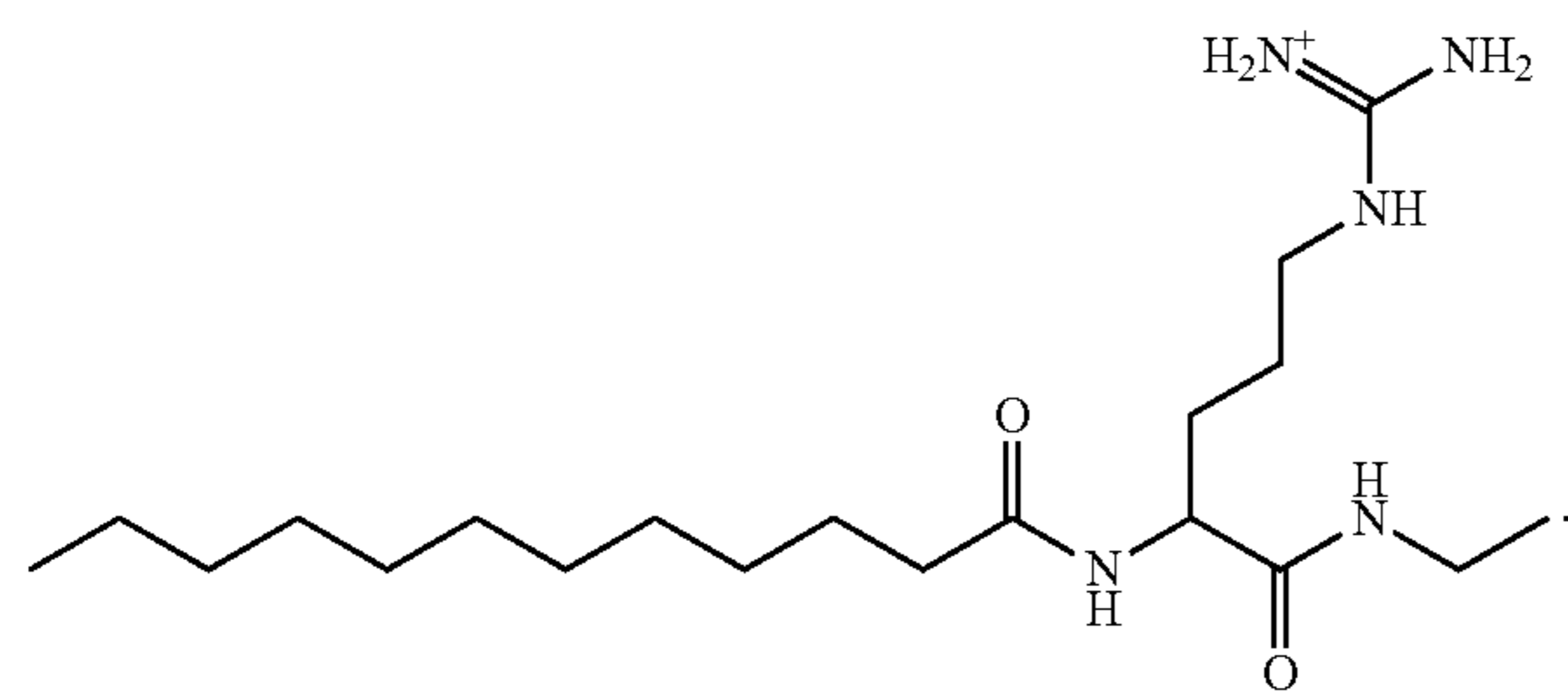
[amino({[4-dodecanamido-4-(ethylcarbamoyl)butyl]amino})methylidene]azanium
