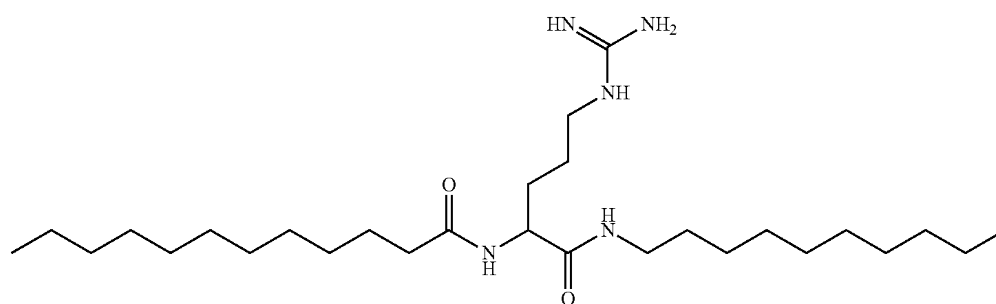
N-1-(decylamino)-5-guanidino-1-oxopentan-2-yl)dodecanamide
