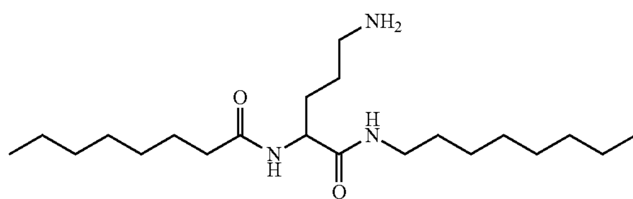
N-(5-amino-1-(octylamino)-1-oxopentan-2-yl)octanamide
