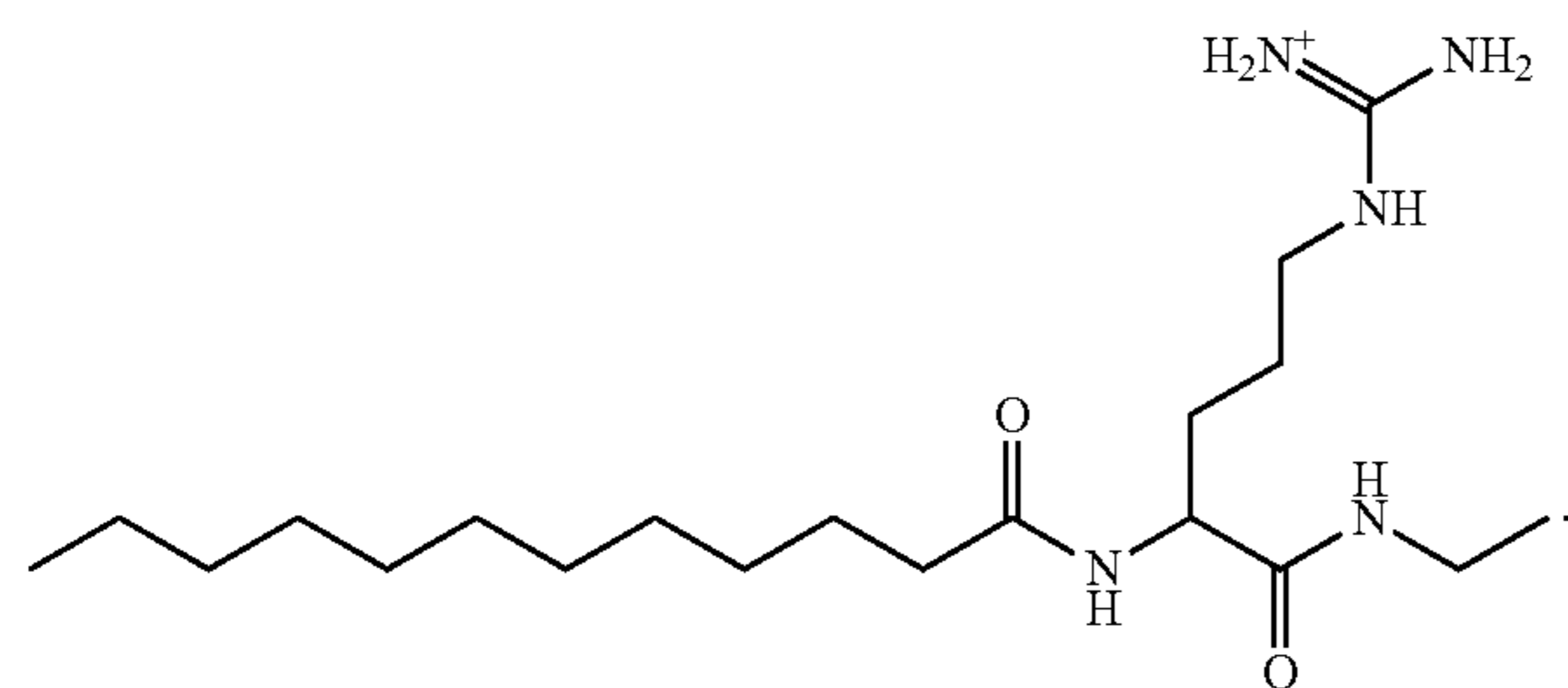
[amino({[4-dodecanamido-4-(ethylcarbamoyl)butyl]amino})methylidene]azanium
