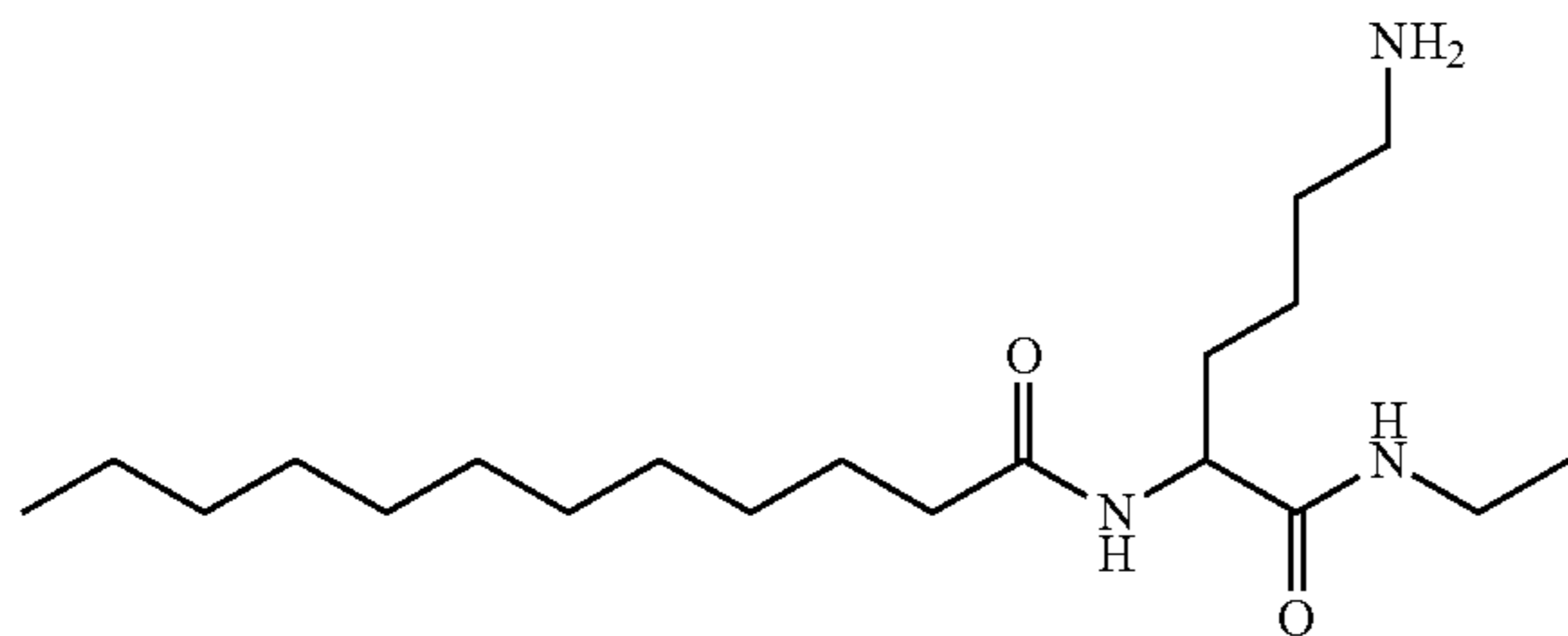
N-[5-amino-1-(ethylcarbamoyl)pentyl]dodecanamide;
