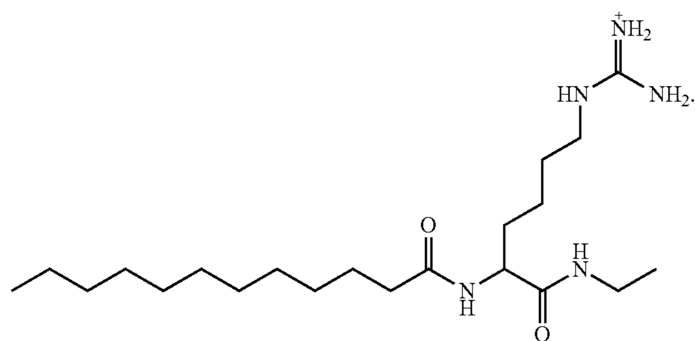
[amino({[5-dodecanamido-5-(ethylcarbamoyl)pentyl]amino})methylidene]azanium
