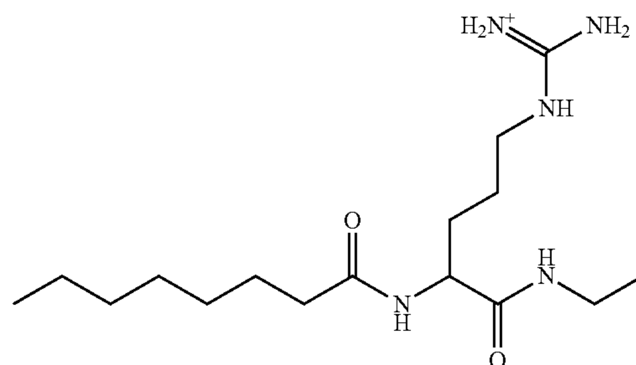
[amino({[4-(ethylcarbamoyl)-4-octanamidobutyl]amino})methylidene]azanium;
