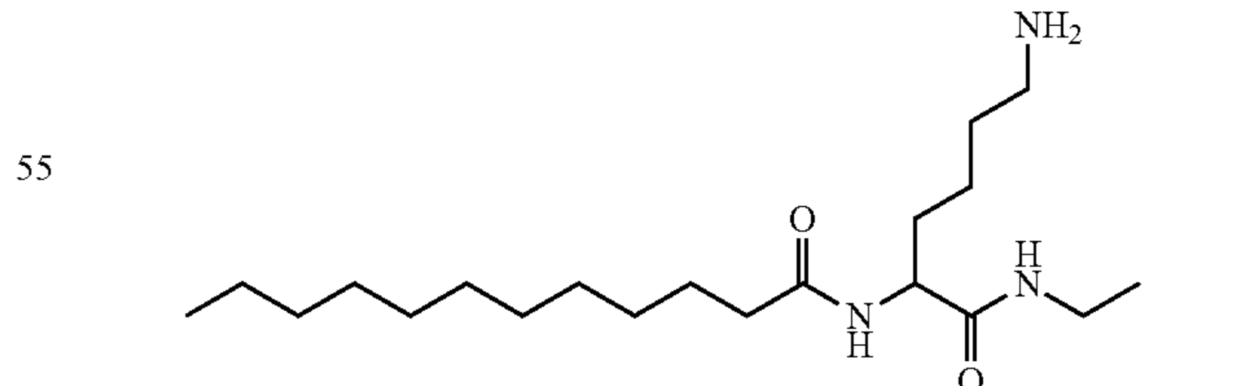
N-[5-amino-1-(ethylcarbamoyl)pentyl]dodecanamide;
