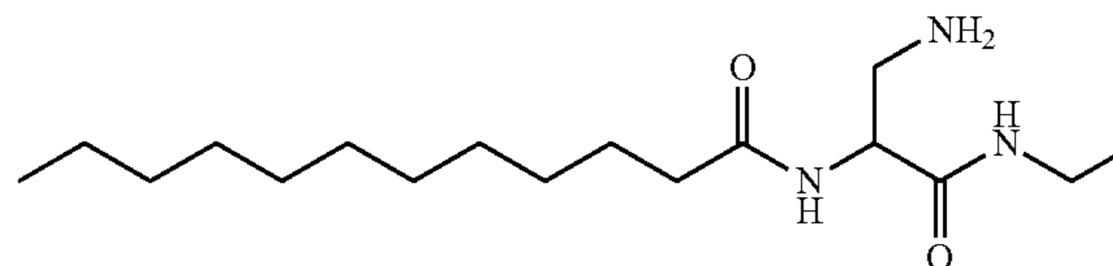
N-[2-amino-1-(ethylcarbamoyl)ethyl]dodecanamide;
