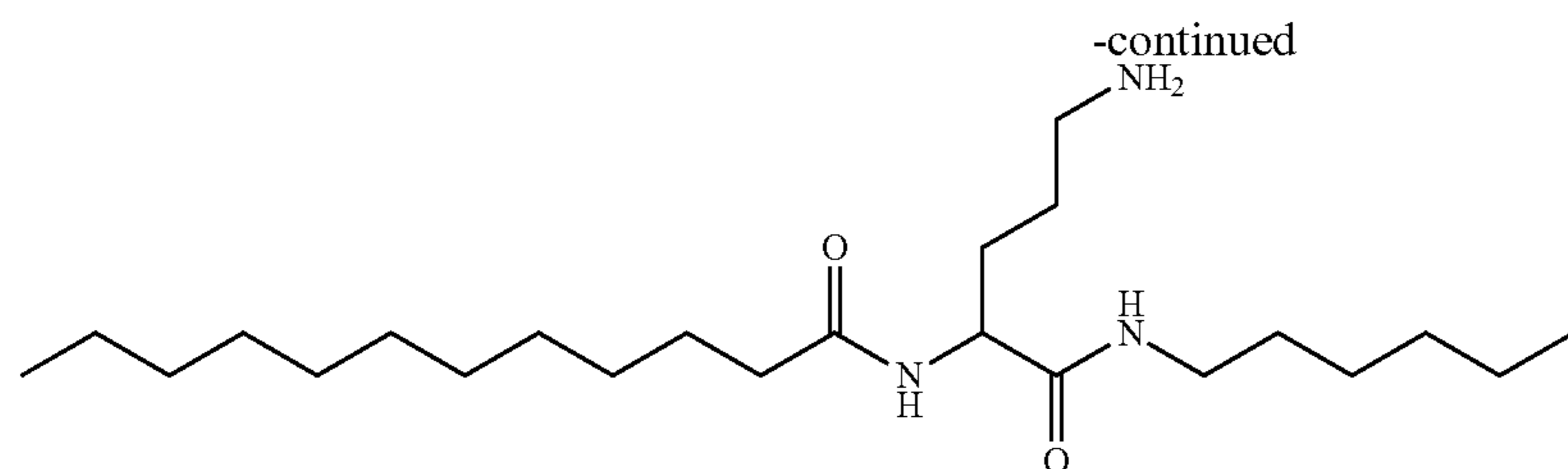
N-(5-amino-1-(hexylamino)-1-oxopentan-2-yl)dodecanamide;
