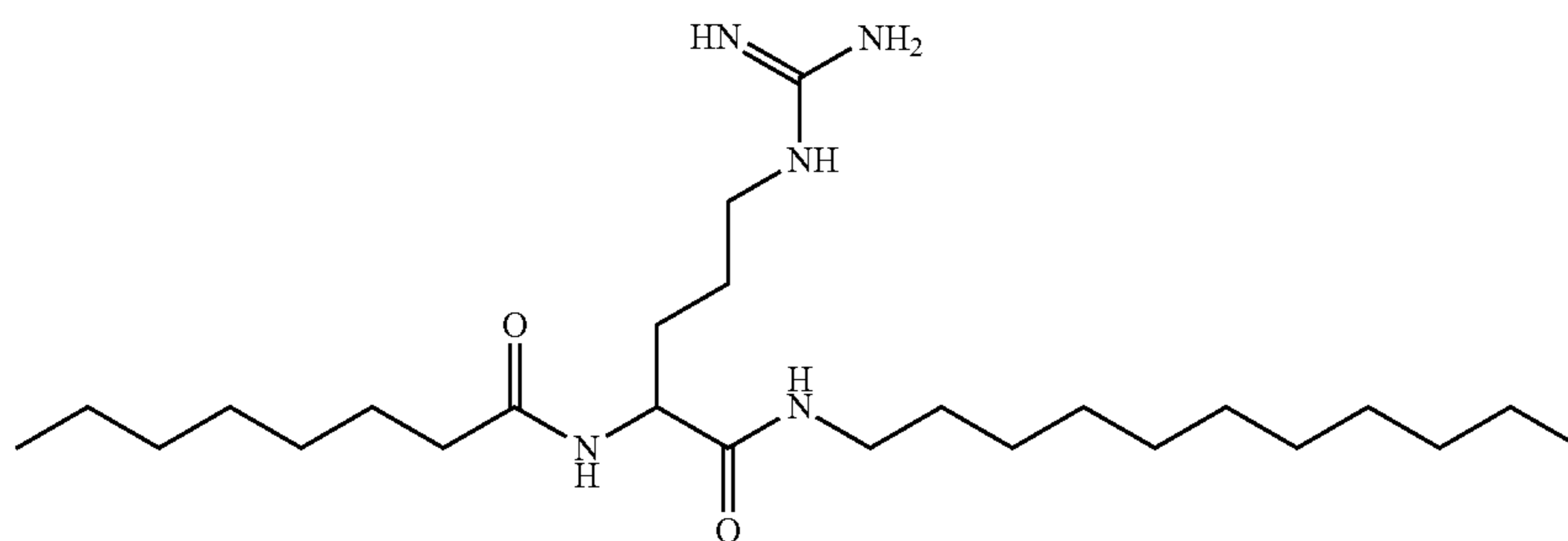
N-(5-guanidino-1-oxo-1-(undecylamino)pentan-2-yl)octamide;
