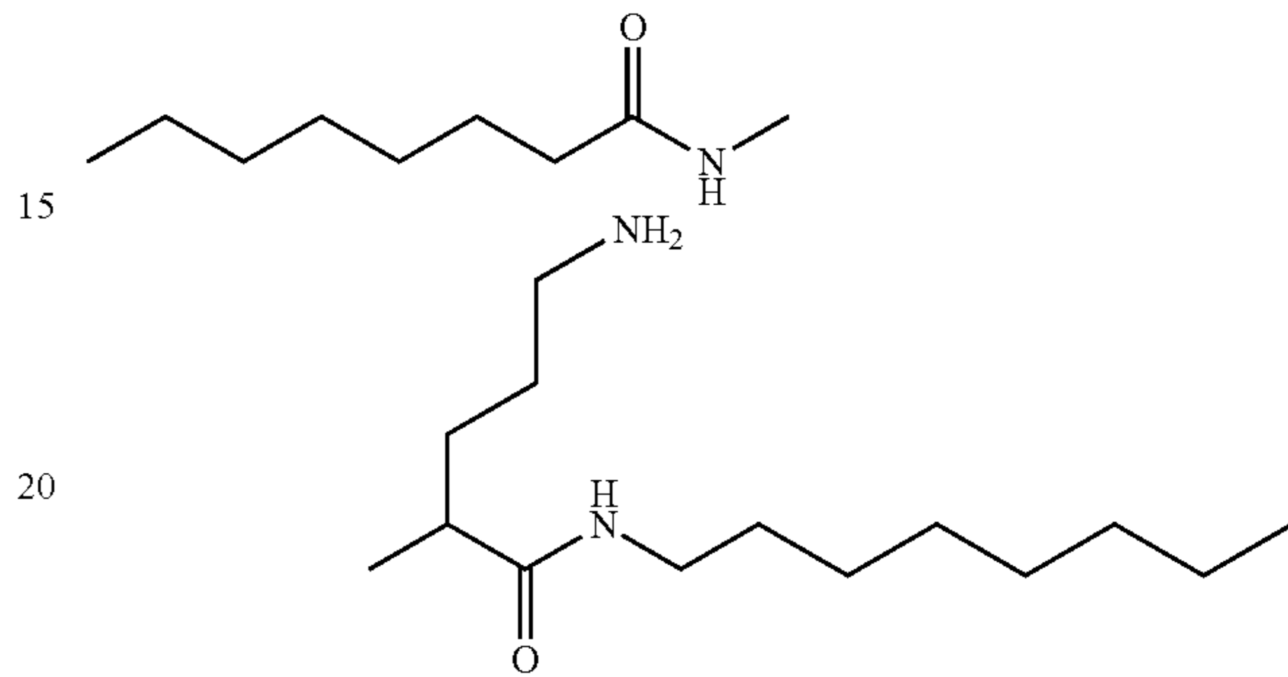
N-(5-amino-1-oxo-1-(undecylamino)pentan-2-yl)octanamide;
