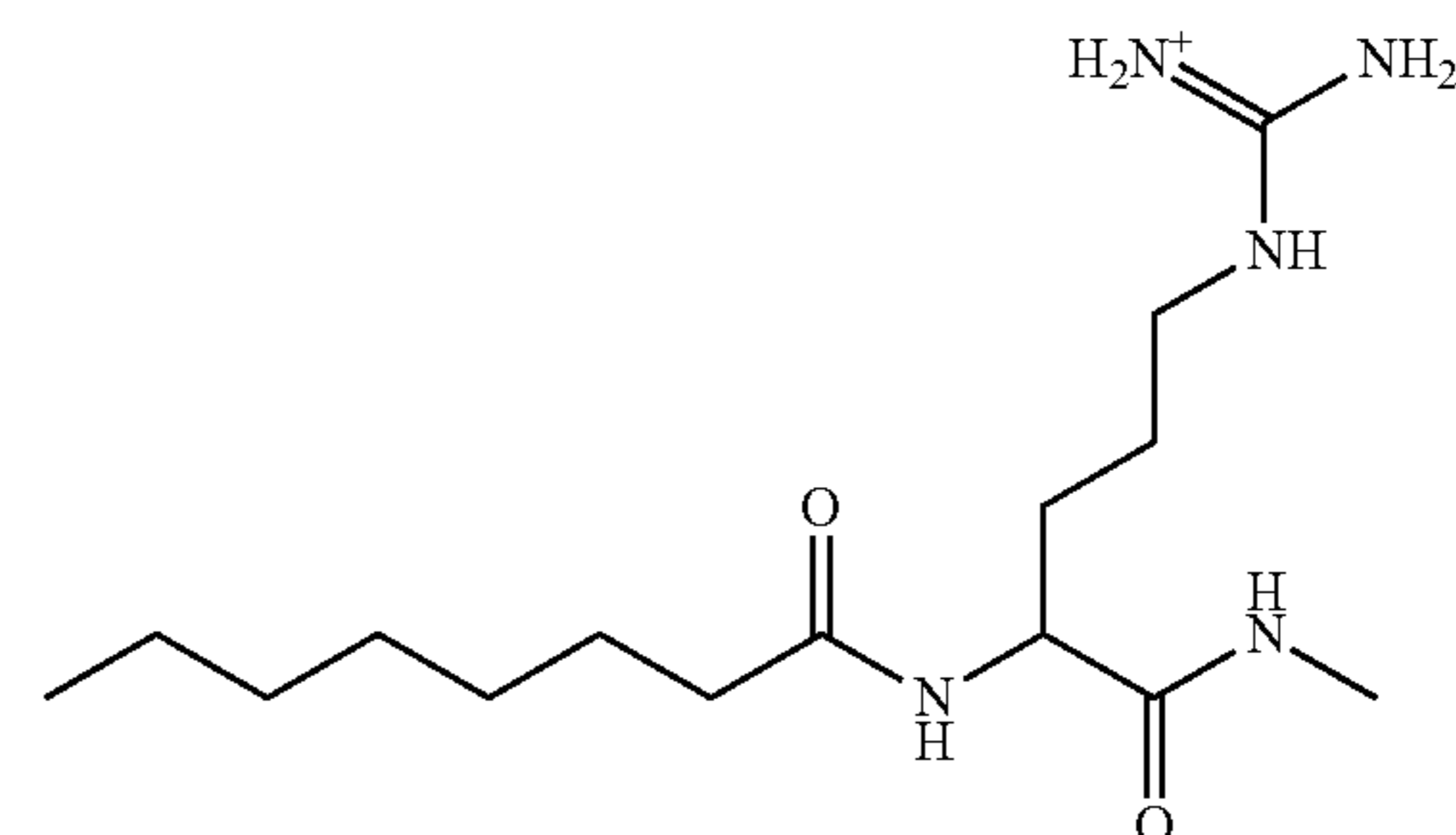
[amino({[4-(methylcarbamoyl)-4-octanamidobutyl]amino})methylidene]azanium;
