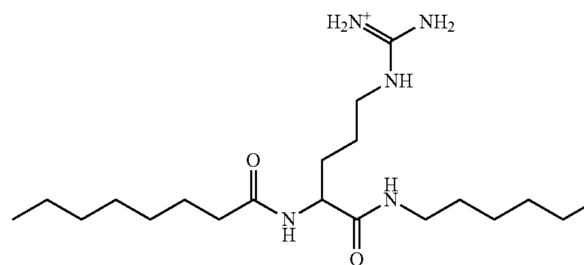
[amino({[4-(hexylcarbamoyl)-4-octanamidobutyl]amino})methylidene]azanium
