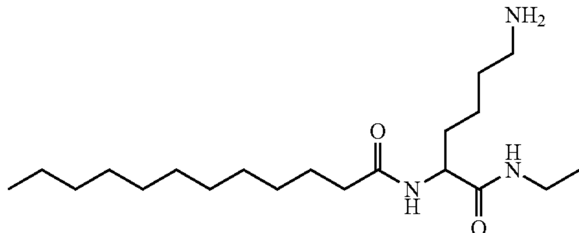
N-[5-amino-1-(ethylcarbamoyl)pentyl]dodecanamide;
