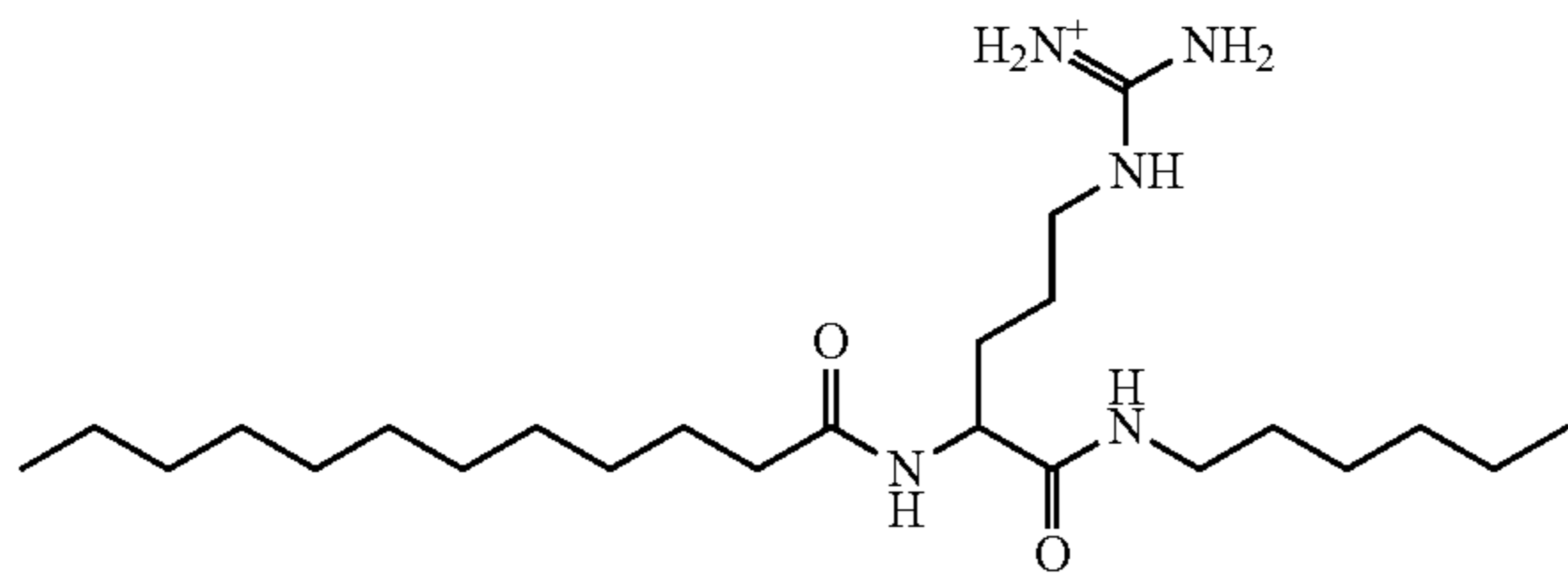
[amino({[4-dodecanamido-4-(hexylcarbamoyl)butyl]amino})methylidene]azanium;
