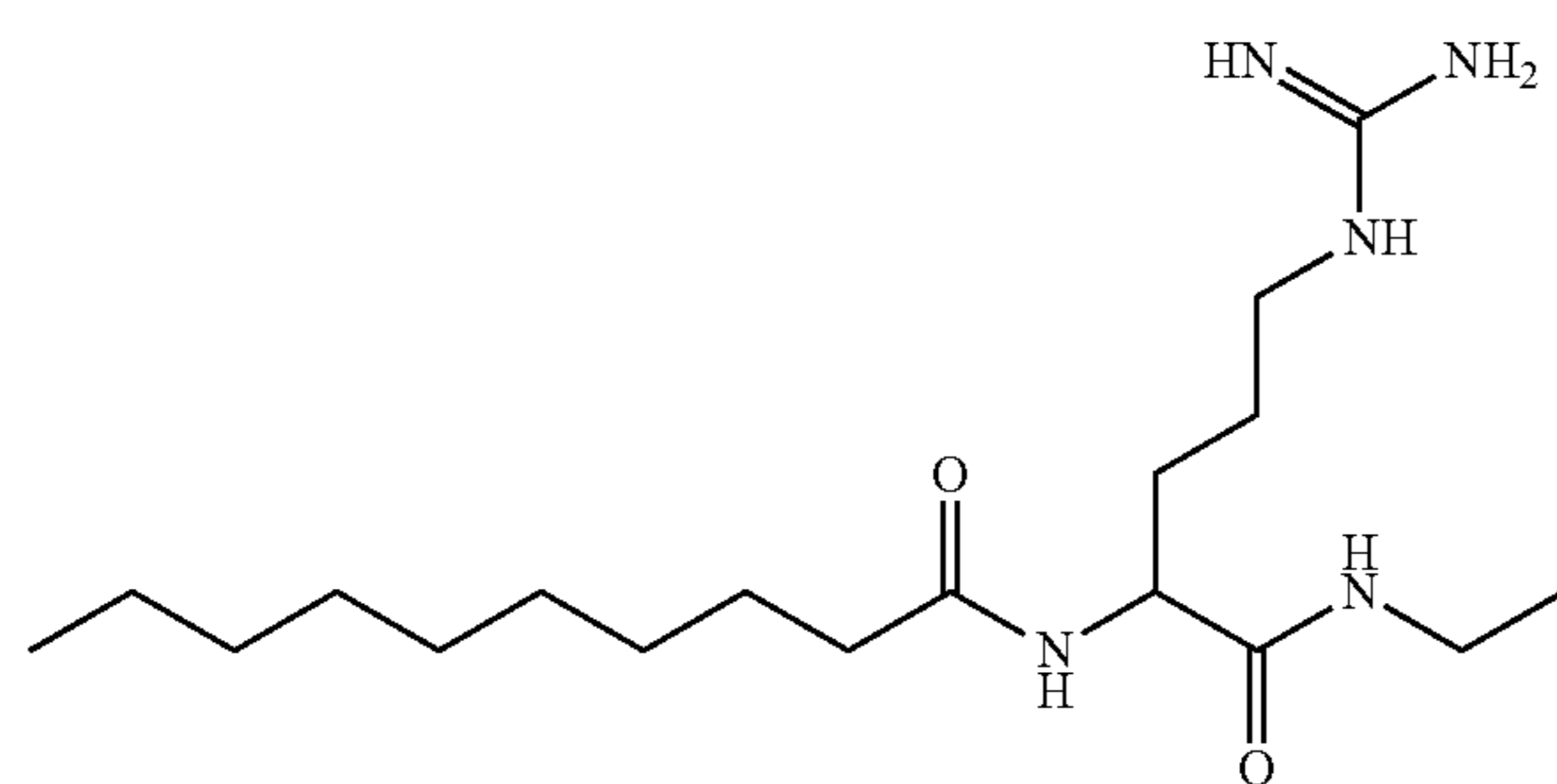
N-1-(ethylamino)-5-guanidino-1-oxopentan-2-yl)decanamide
