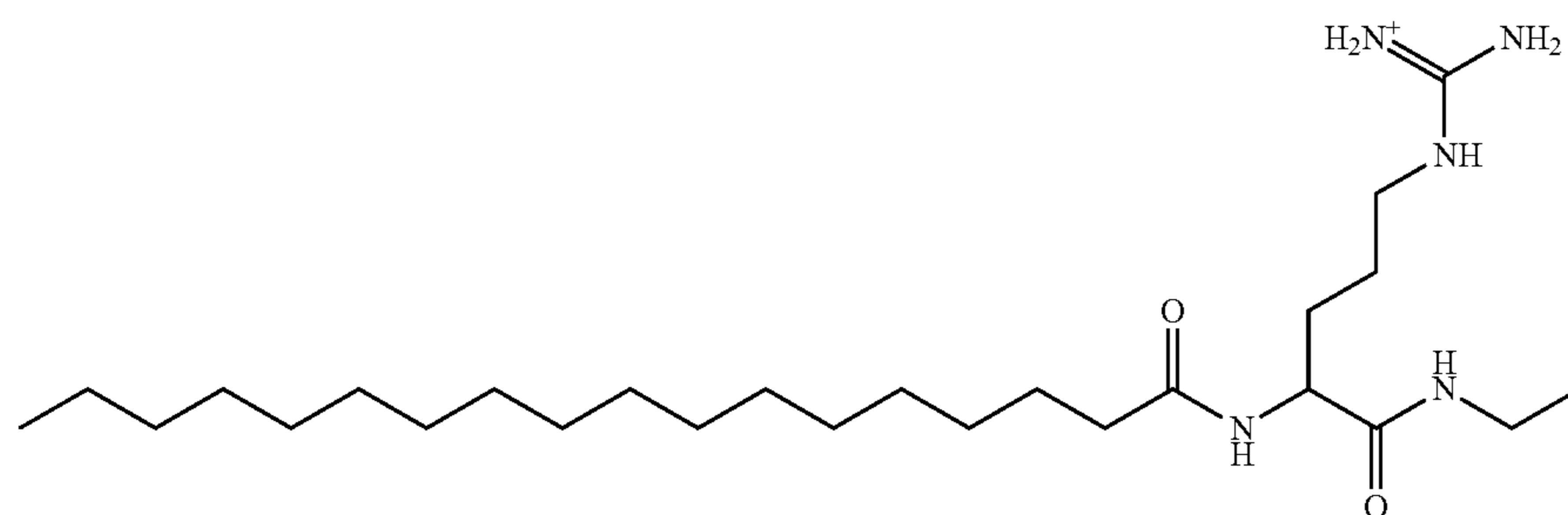
[amino({[4-(ethylcarbamoyl)-4-octadecanamidobutyl]amino})methylidene]azanium;
