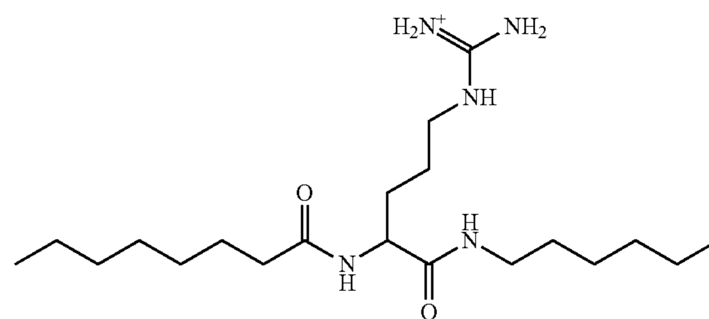
[amino({[4-(hexylcarbamoyl)-4-octanamidobutyl]amino})methylidene]azanium
