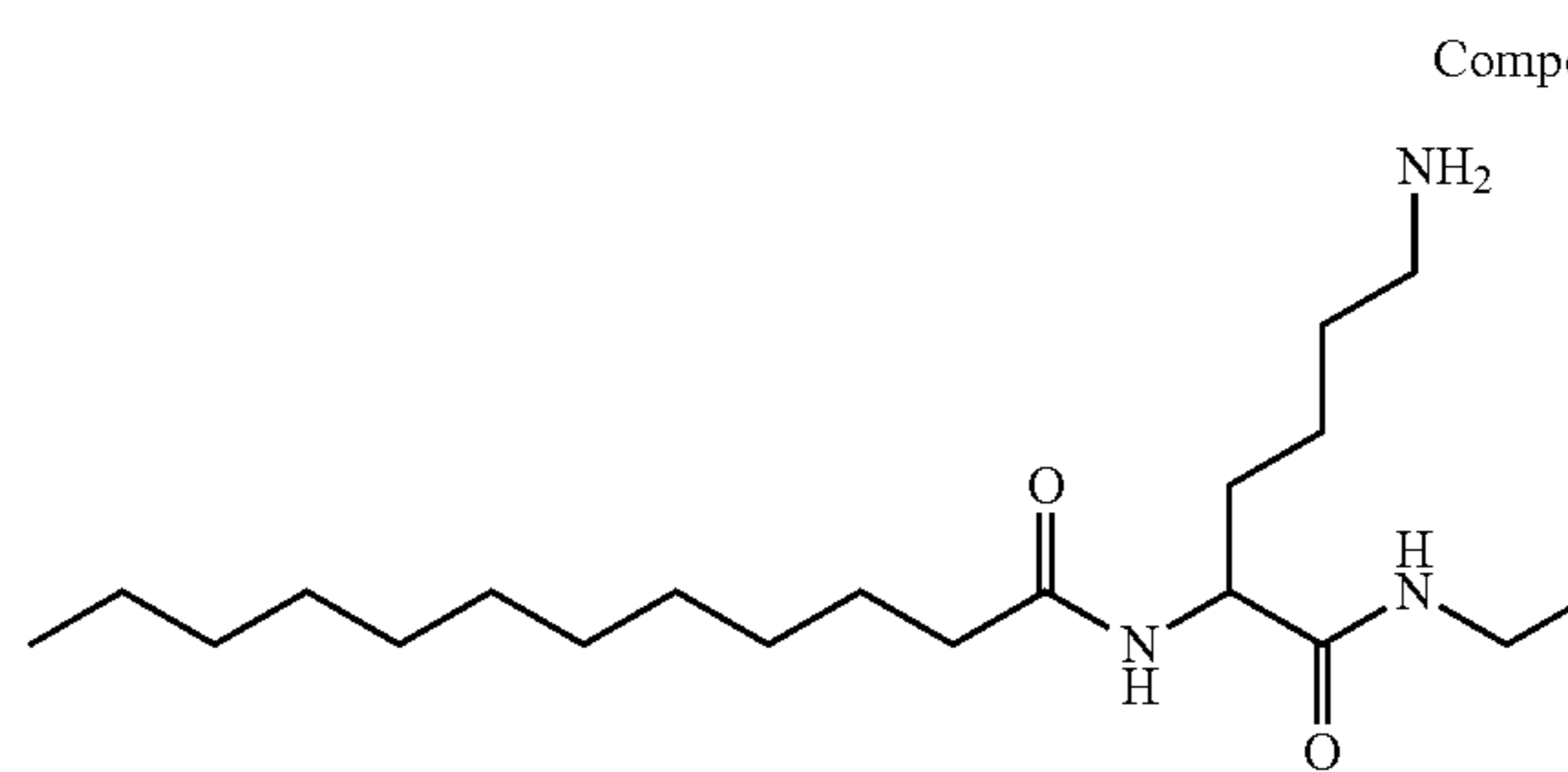
N-[5-amino-1-(ethylcarbamoyl)pentyl]dodecanamide
