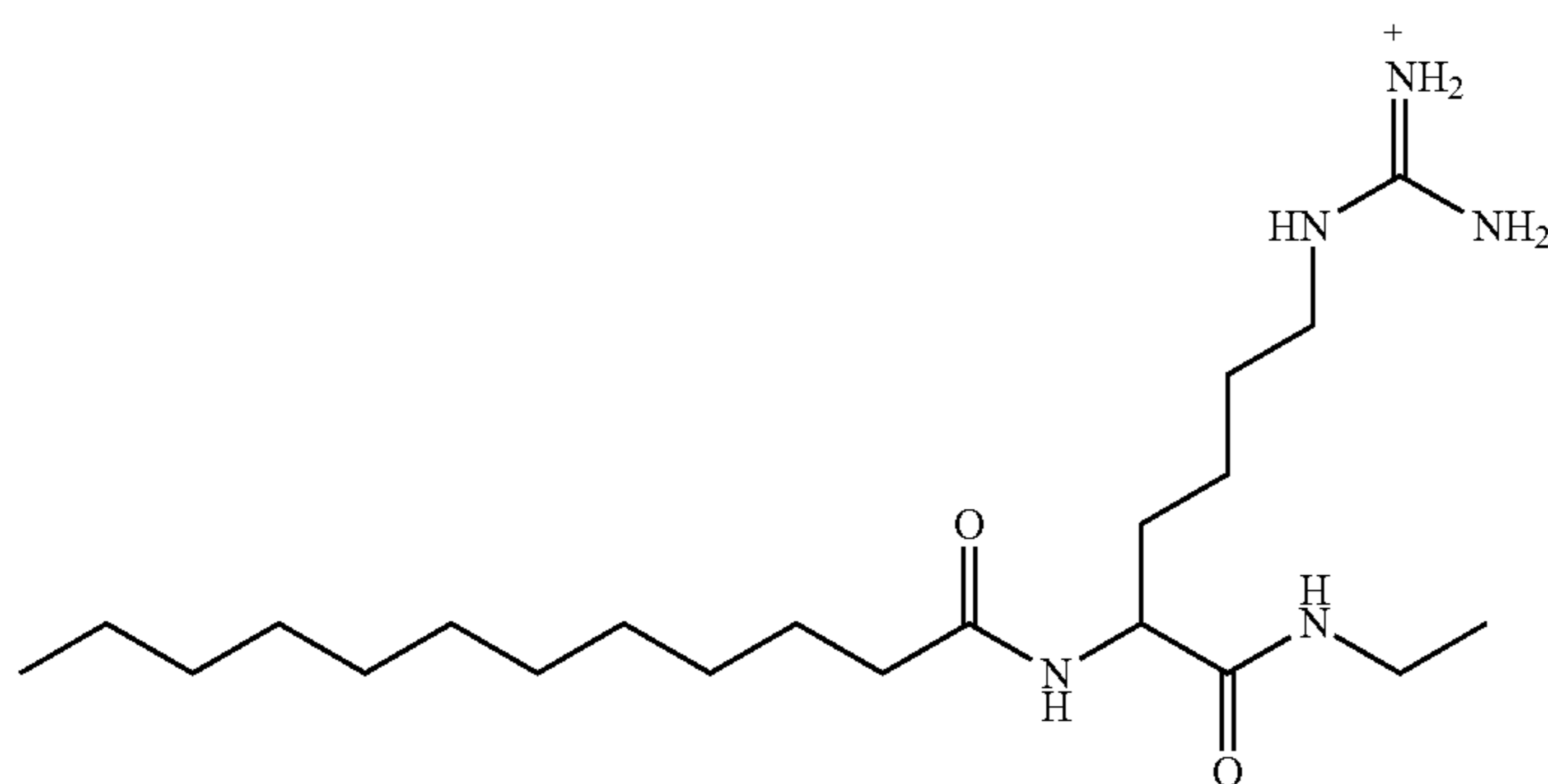
[amino({[5-dodecanamido-5-(ethylcarbamoyl)pentyl]amino})methylidene]azanium.
