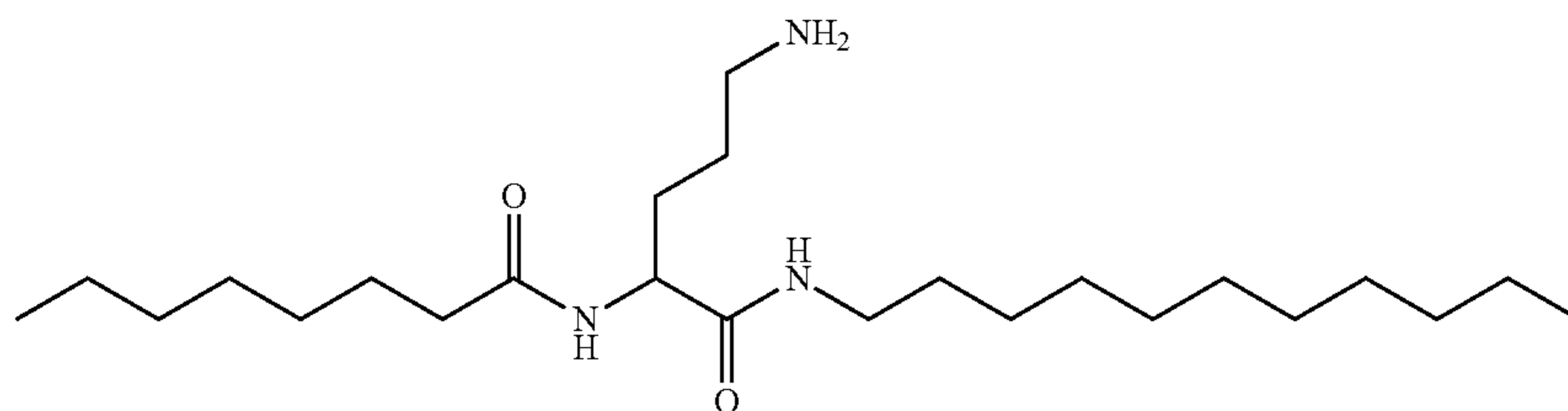
N-(5-amino-1-oxo-1-(undecylamino)pentan-2-yl)dodecanamide
