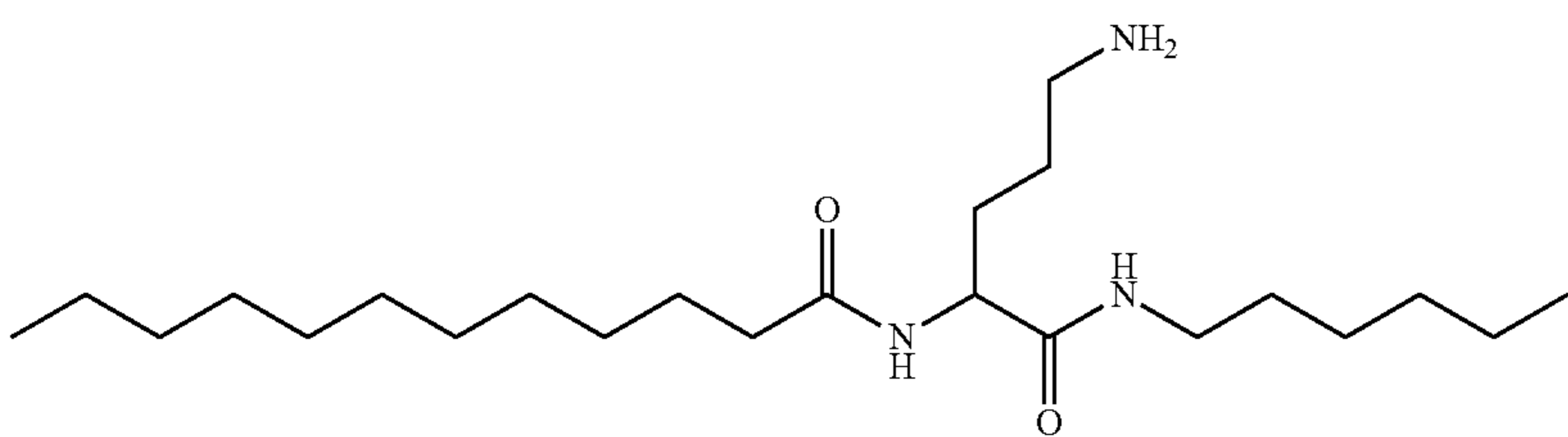
N-(5-amino-1-(hexylamino)-1-oxopentan-2-yl)dodecanamide
