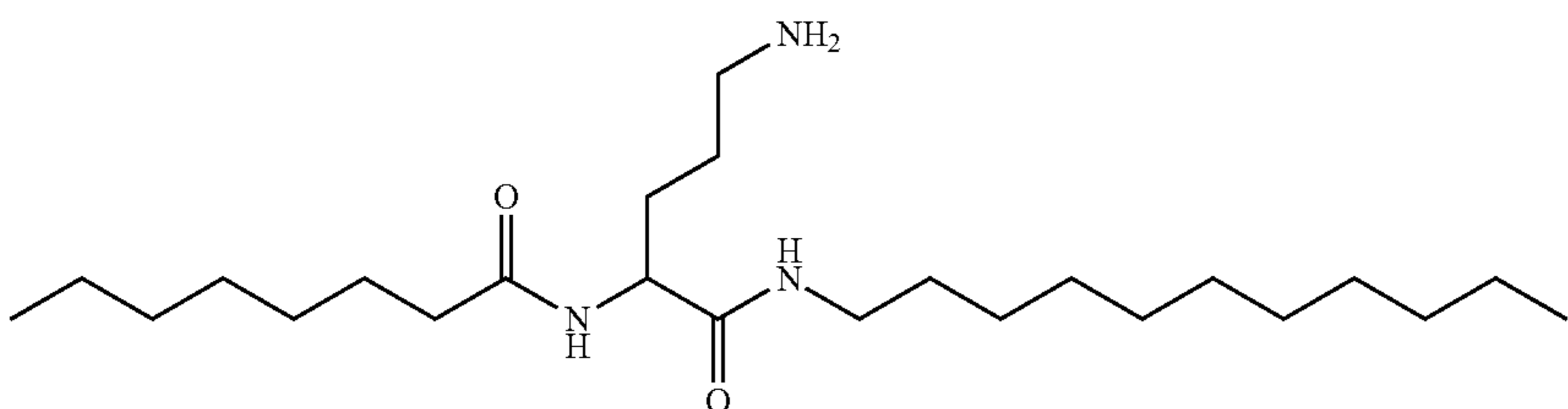
N-(5-amino-1-oxo-1-(undecylamino)pentan-2-yl)octanamide
