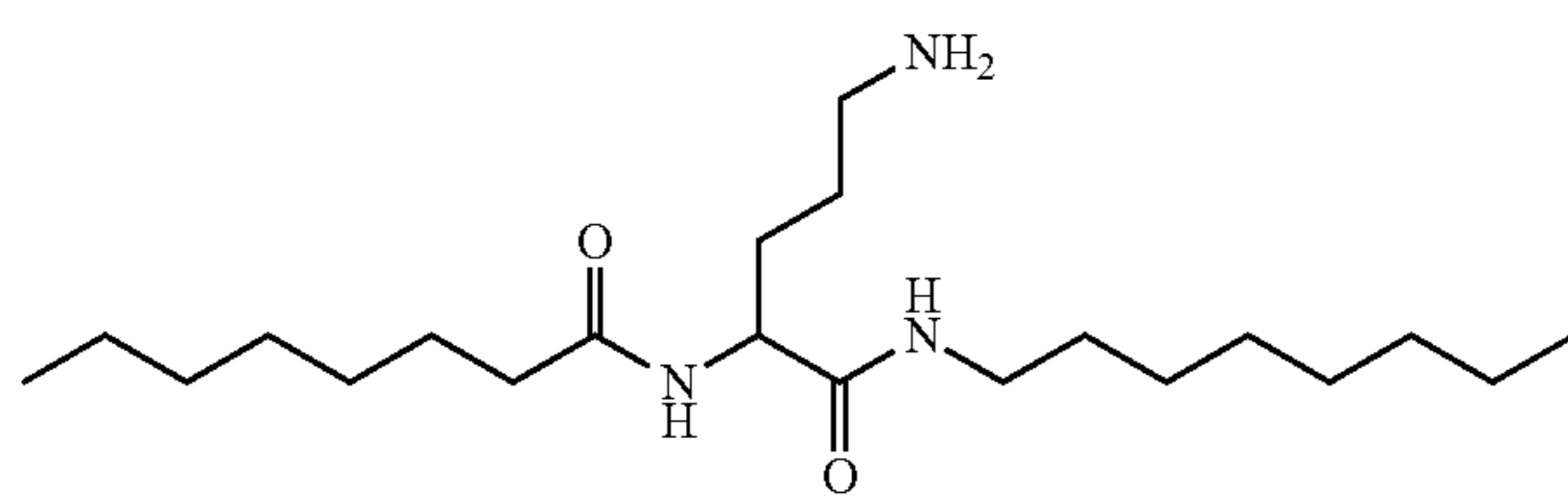
N-(5-amino-1-(octylamino)-1-oxopentan-2-yl)octanamide
