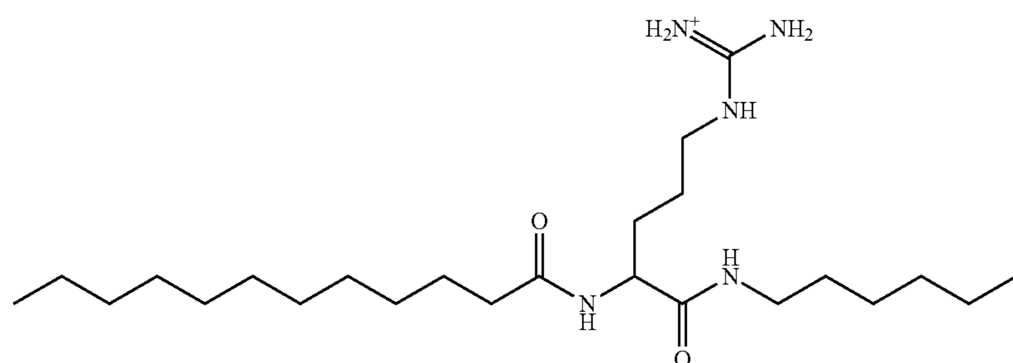
[amino({[4-(dodecanamido)-4-hexylcarbamoyl]butyl]amino})methylidene]azanium;
