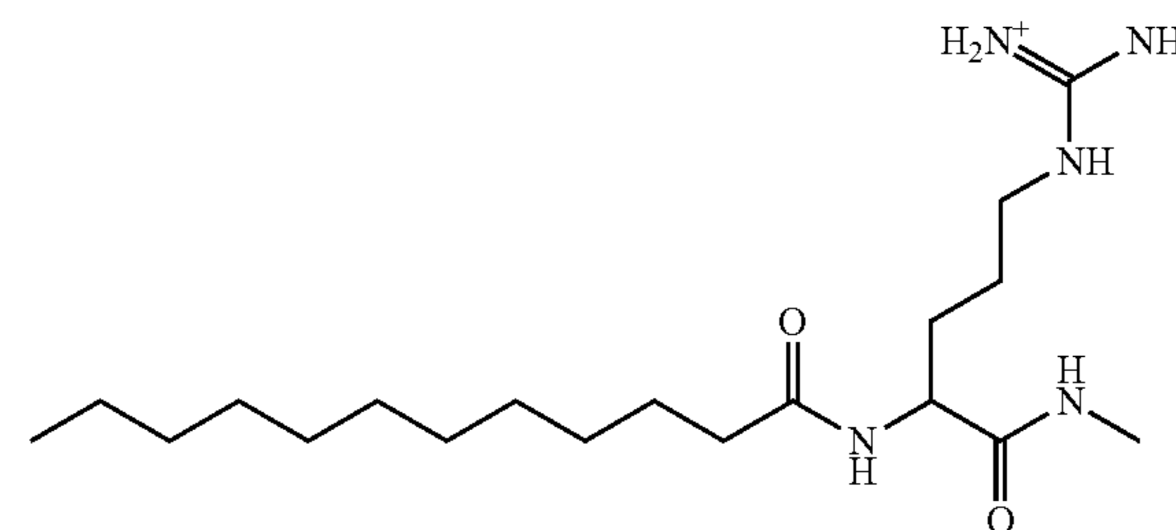
[amino({[4-(dodecanamido-4-(methylcarbamoyl)butyl]amino})methylidene]azanium;
