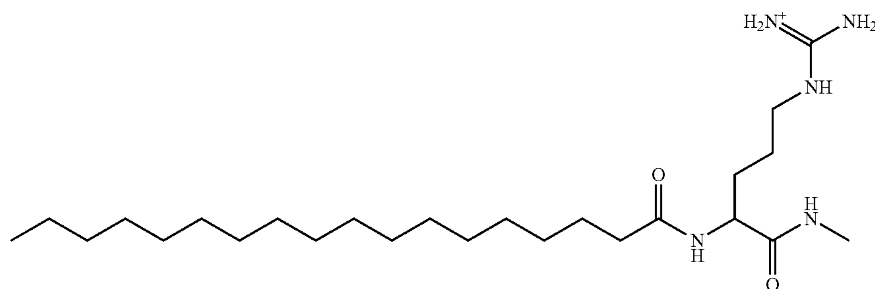
[amino({[4-(methylcarbamoyl)-4-octadecanamidobutyl]amino}) methylidene]azanium;
