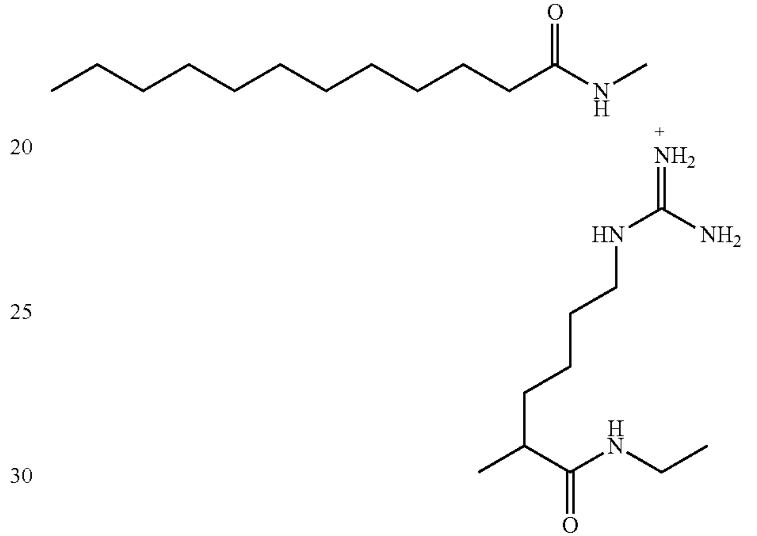
[amino({[5-dodecanamido-5-(ethylcarbamoyl)pentyl]amino})methylidene]azanium;
