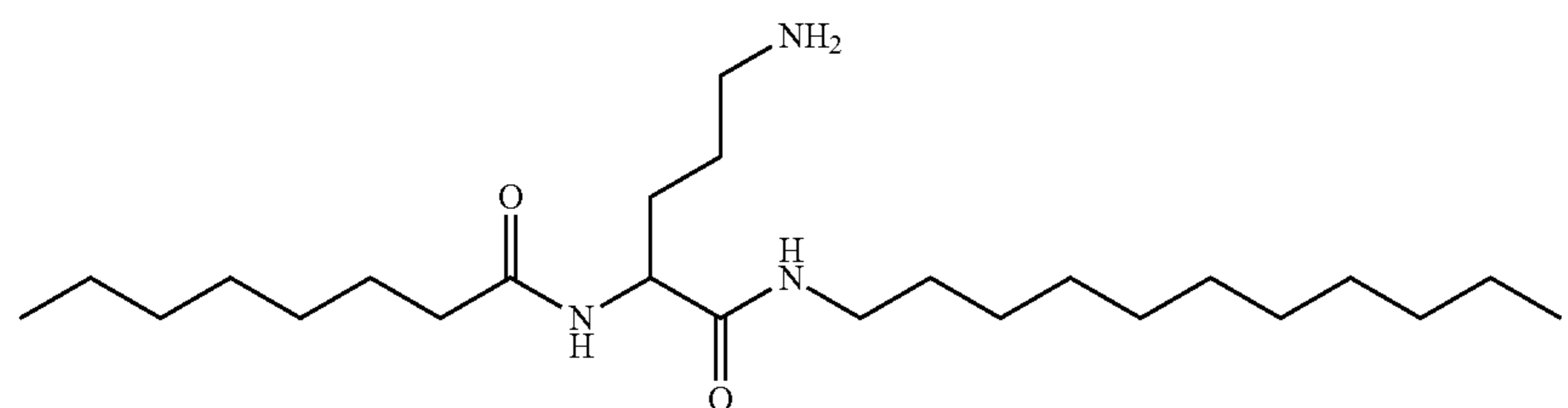
N-(5-amino-1-oxo-1-(undecylamino)pentan-2-yl)octanamide
