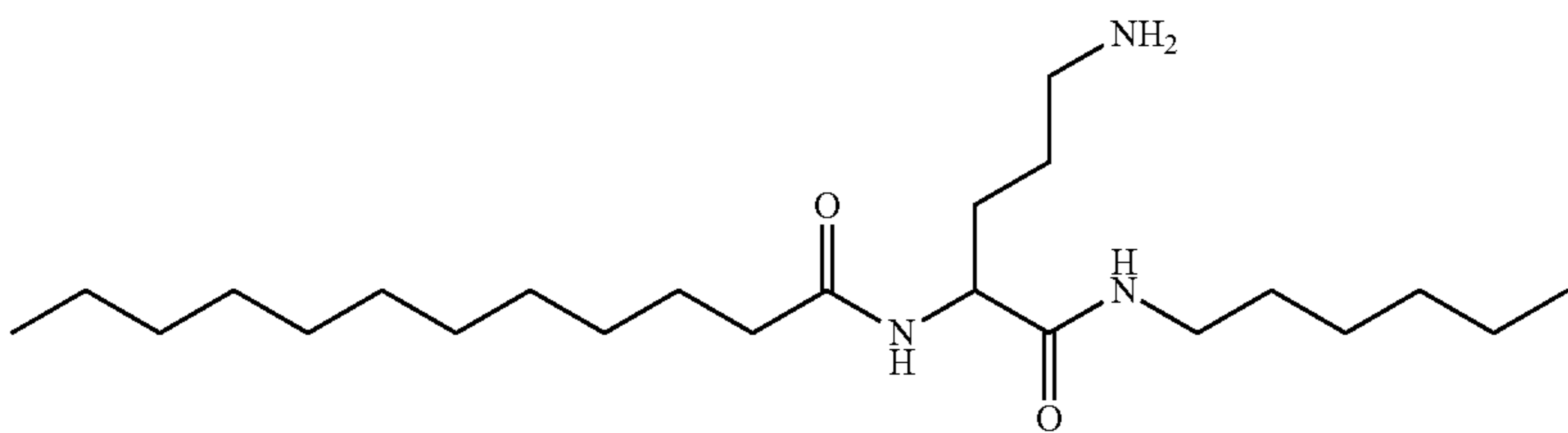
N-(5-amino-1-(hexylamino)-1-oxopentan-2-yl)dodecanamide
