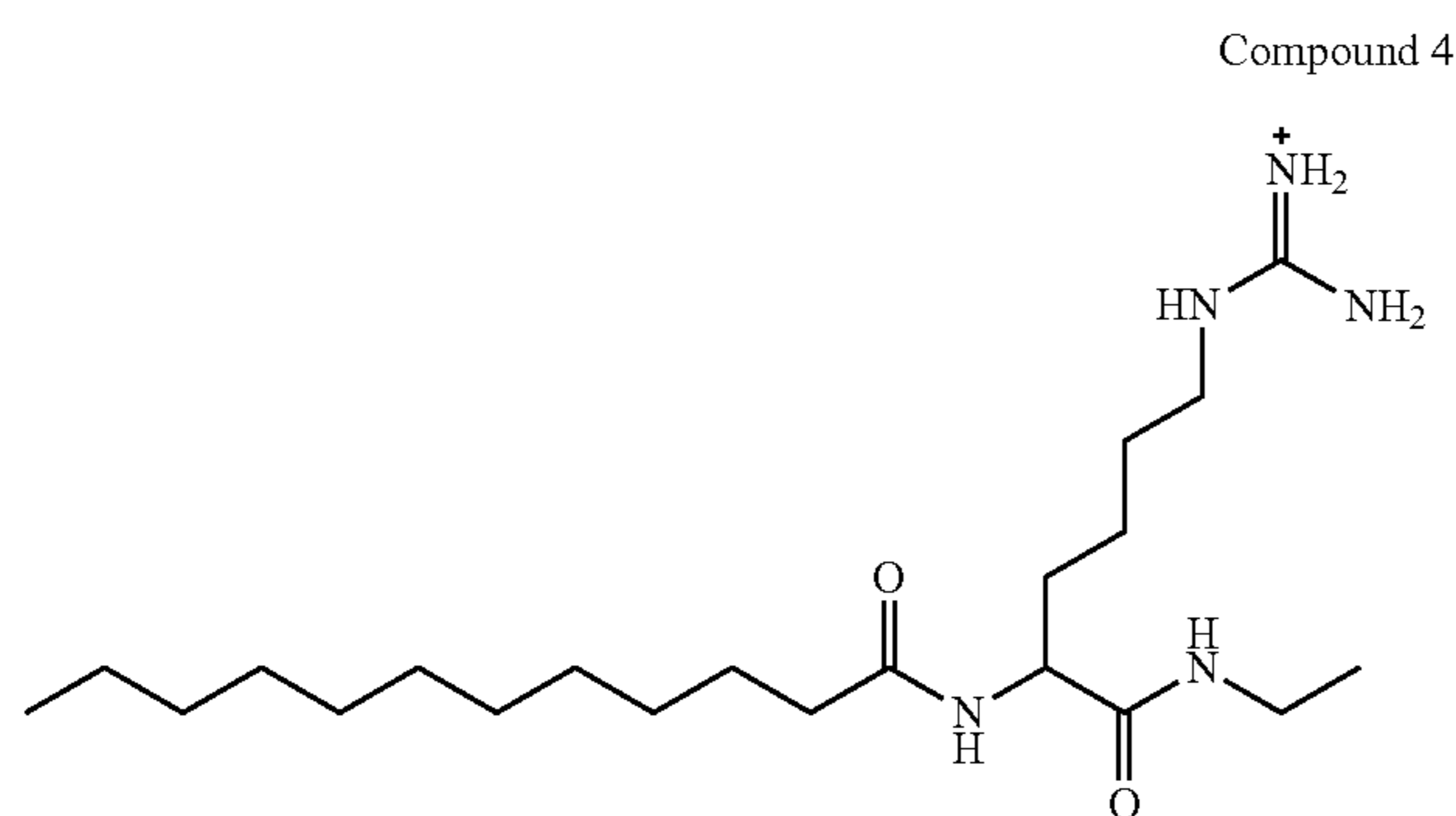
[amino({[5-dodecanamido-5-(ethylcarbamoyl)pentyl]amino})methylidene]azanium
