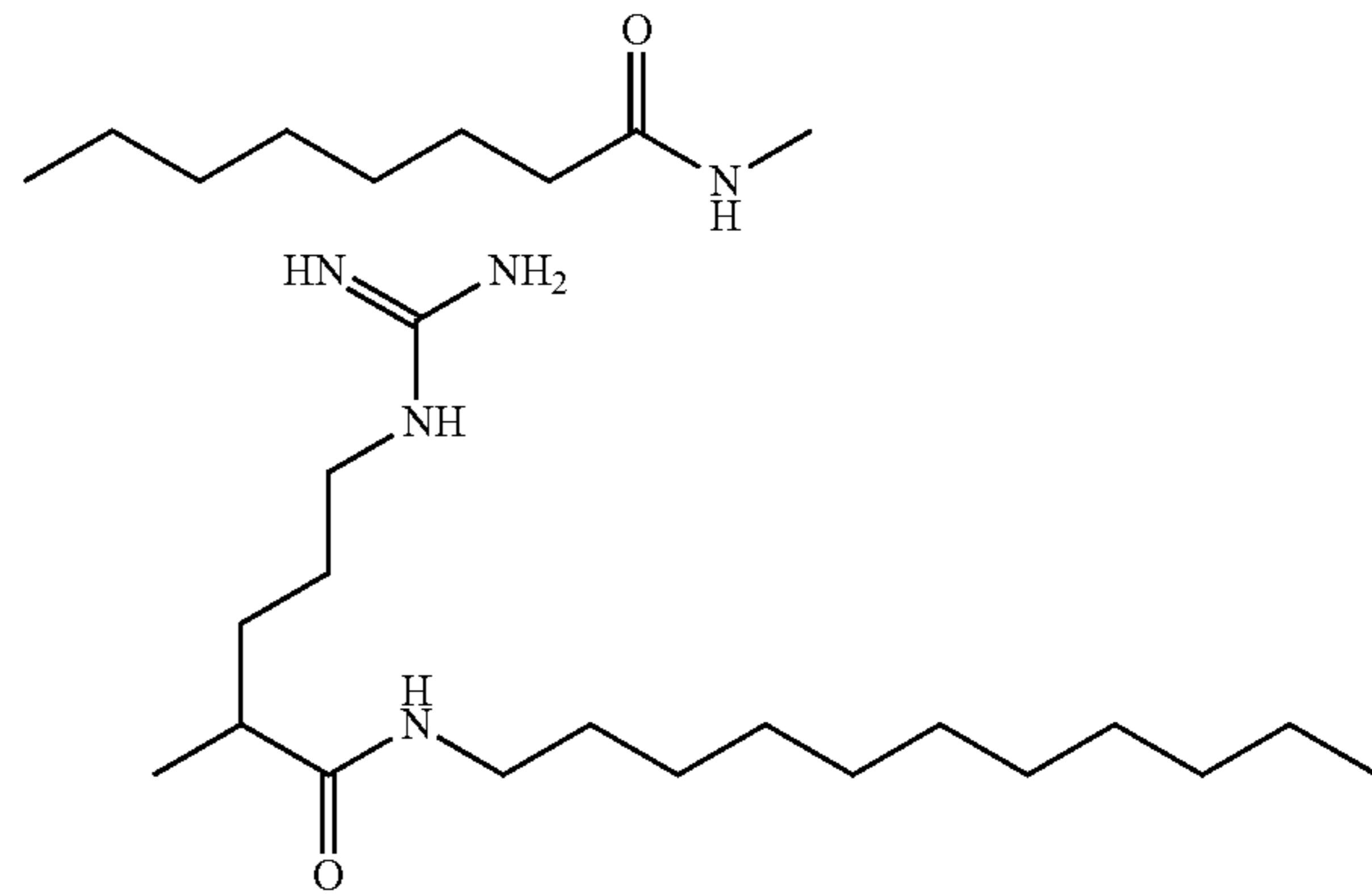
[amino({[5-dodecanamido-5-(ethylcarbamoyl)pentyl]amino})methylidene]azanium;
