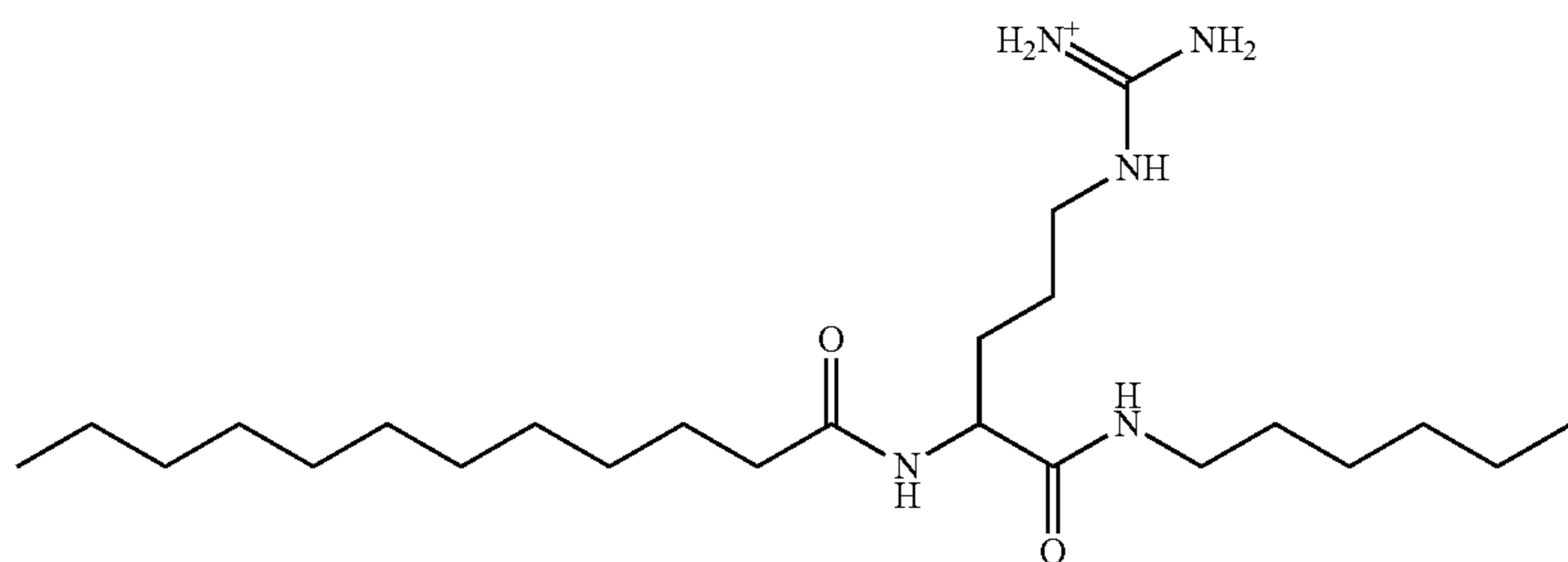
[amino({[4-dodecanamido-4-(hexylcarbamoyl)butyl]amino})methylidene]azanium
