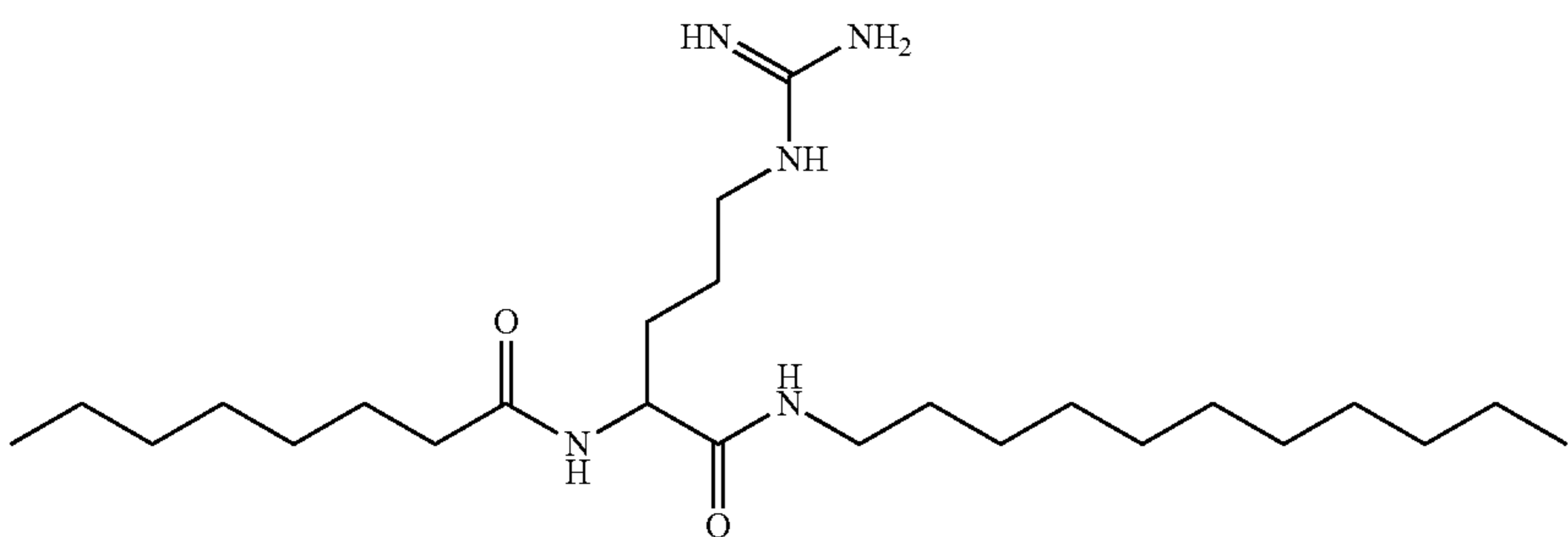
N-(5-guanidino-1-oxo-1-(undecylamino)pentan-2-yl)octanamide
