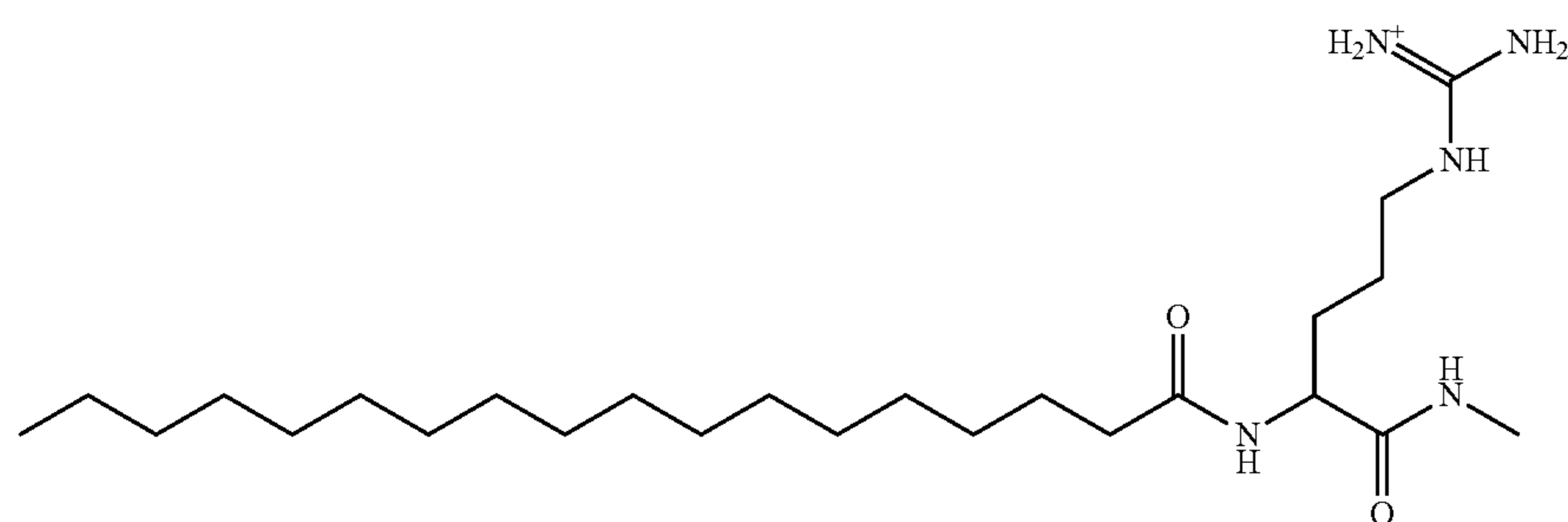
[amino({[4-(methylcarbamoyl)-4-octadecanamidobutyl]amino})methylidene]azanium
