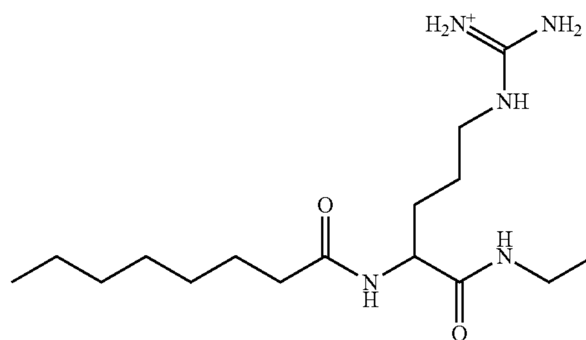
[amino({[4-ethylcarbamoyl]-4-octanamidobutyl}amino)methylidene]azanium;
