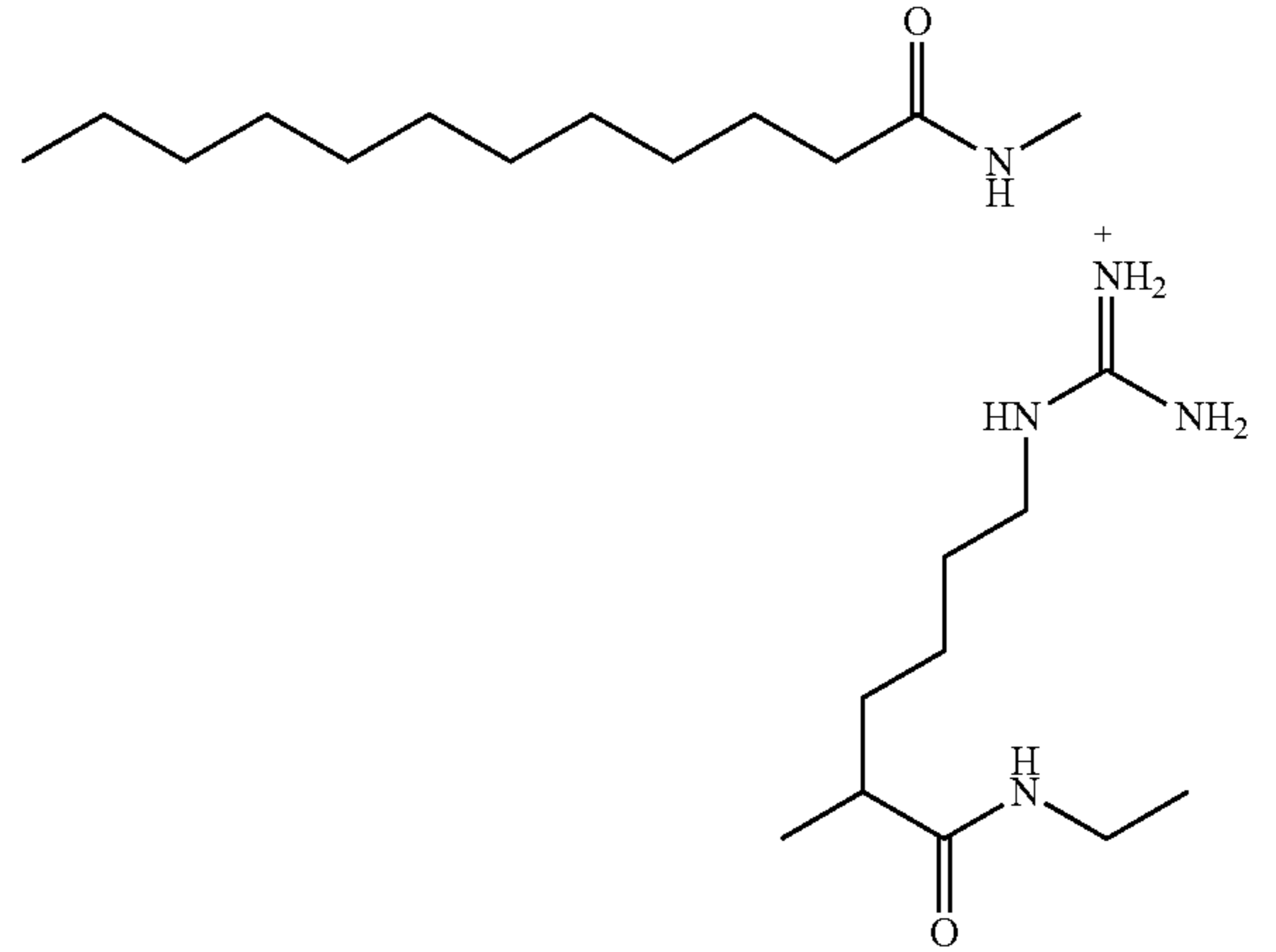
[amino({[5-dodecanamido-5-(ethylcarbamoyl)pentyl]amino})methylidene]azanium;
