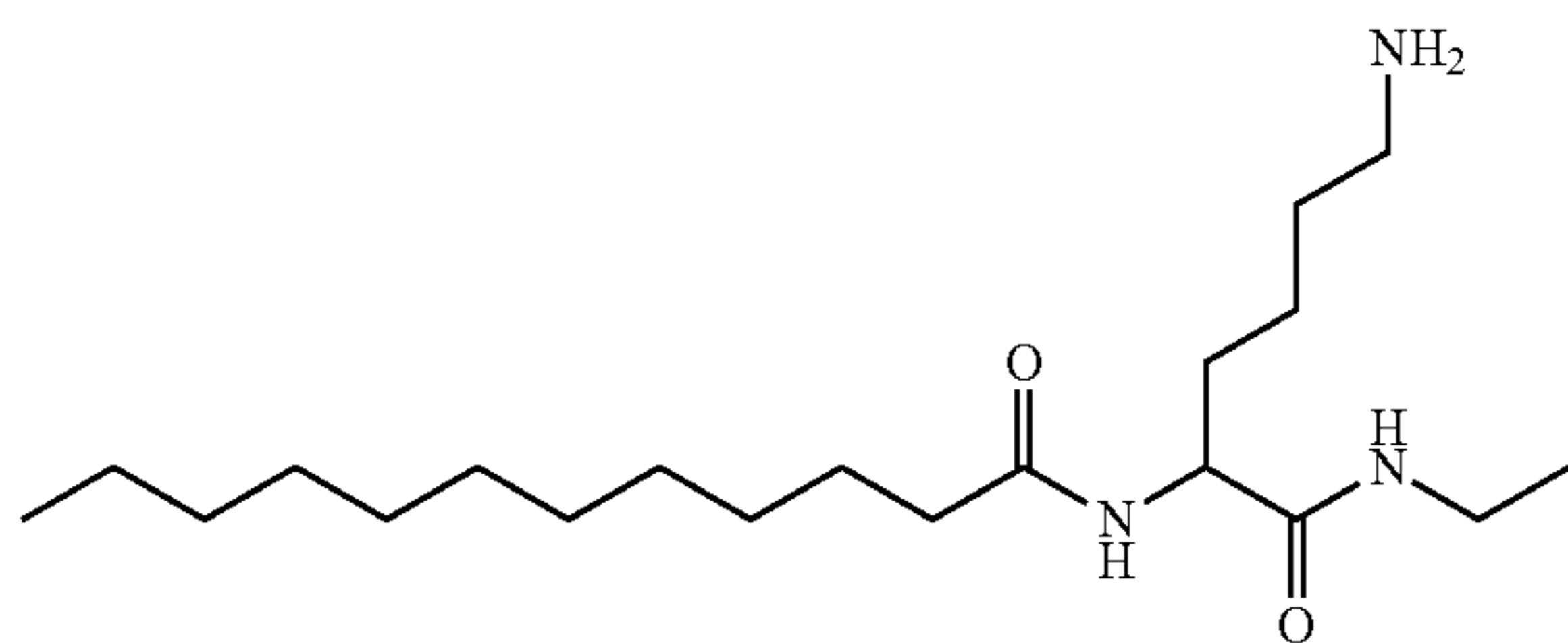
N-[5-amino-1-(ethylcarbamoyl)pentyl]dodecanamide;
