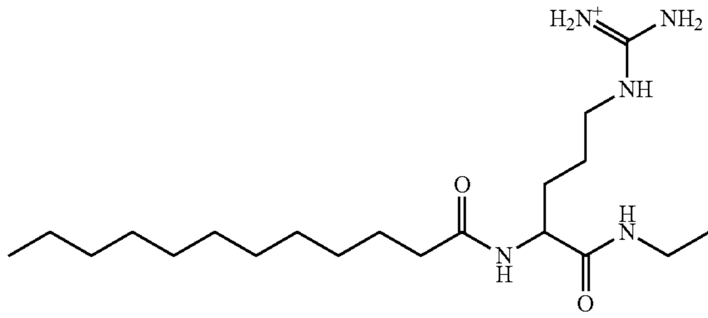
[amino({[4-dodecanamido-4-(ethylcarbamoyl)butyl]amino})methylidene]azanium;
