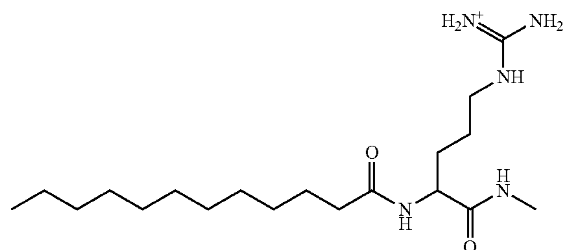
[amino({[4-(dodecanamido)-4-(methylcarbamoyl)butyl]amino})methylidene]azanium;
