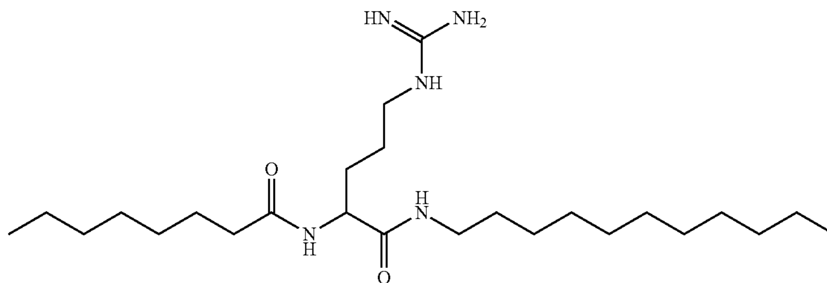
N-(5-guanidino-1-oxo-1-(undecylamino)pentan-2-yl)octanamide
