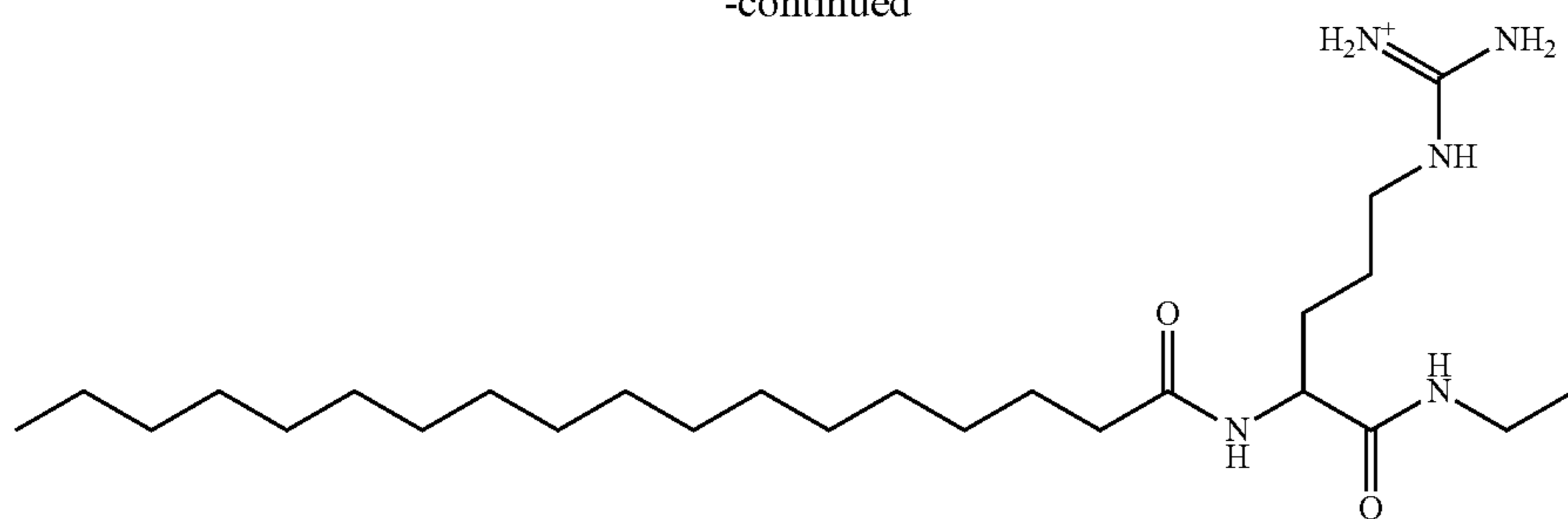
[amino({[4-(ethylcarbamoyl)-4-octadecanamidobutyl]amino})methylidene]azanium; and
