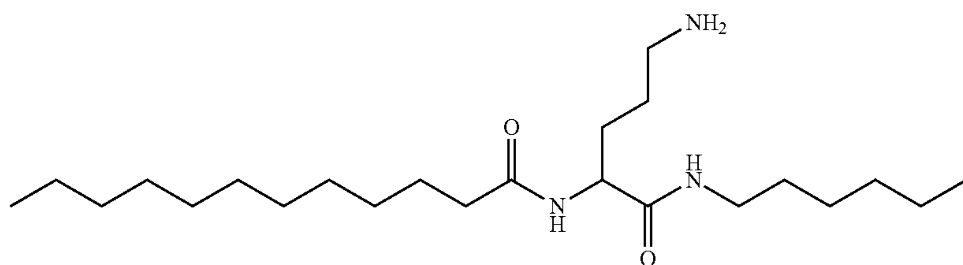
N-(5-amino-1-(hexylamino)-1-oxopentan-2-yl)dodecanamide
