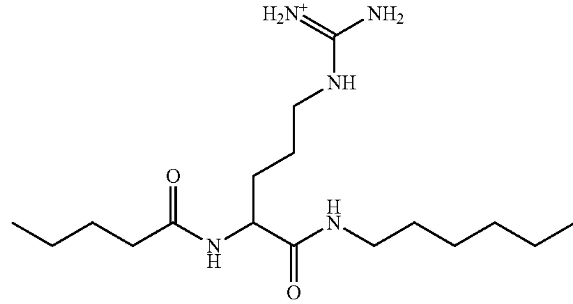
[amino({[4-(hexylcarbamoyl)-4-octadecanamidobutyl]amino})methylidene]azanium;
