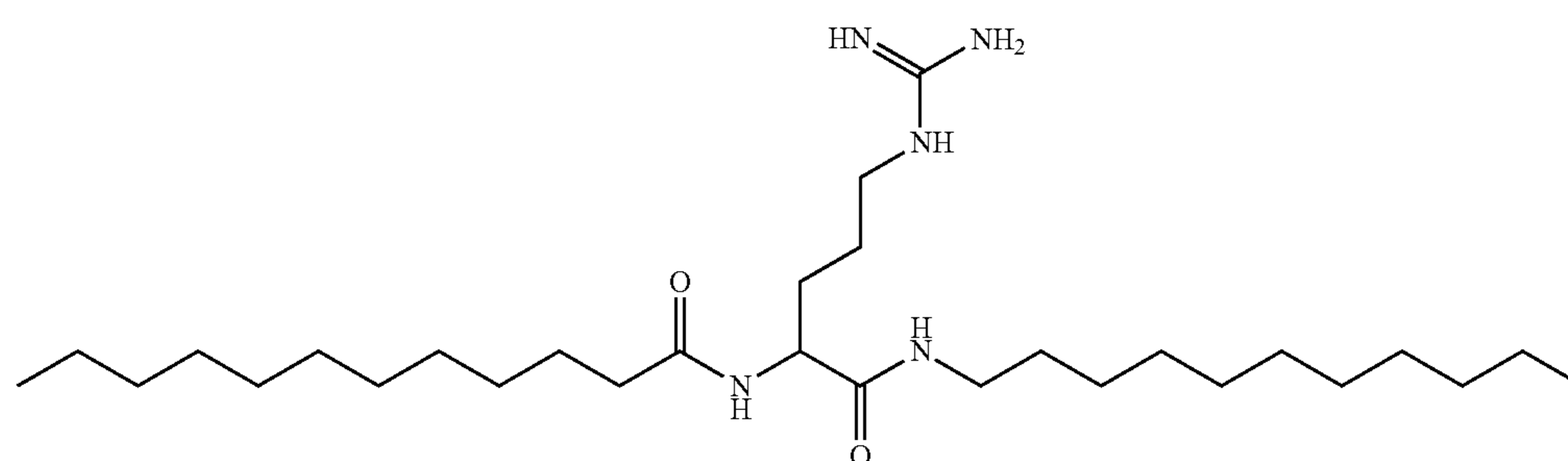
N-(5-guanidino-1-oxo-1-(undecylamino)pentan-2-yl)dodecanamide
