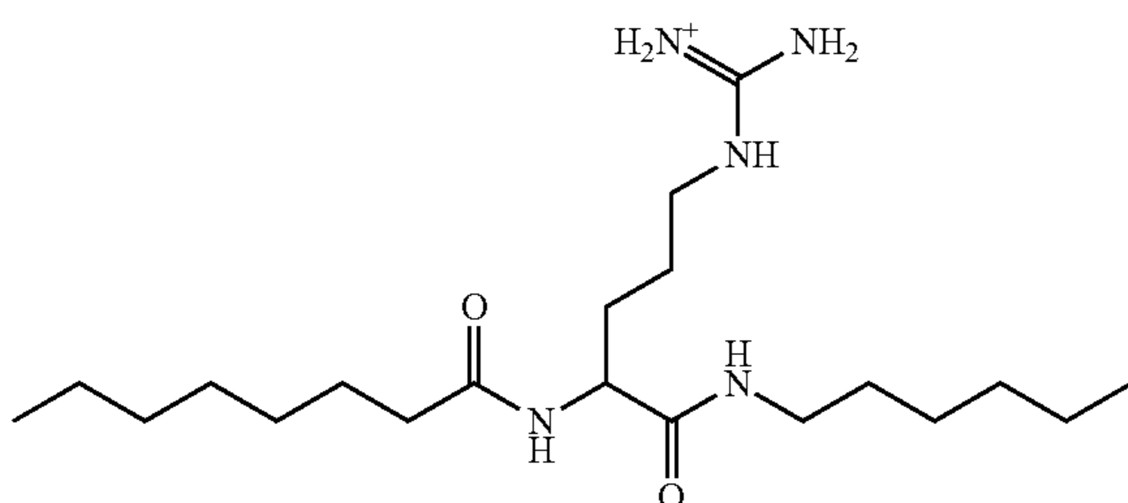
[amino({[4-(hexylcarbamoyl)-4-octanamidobutyl]amino})methylidene]azanium;
