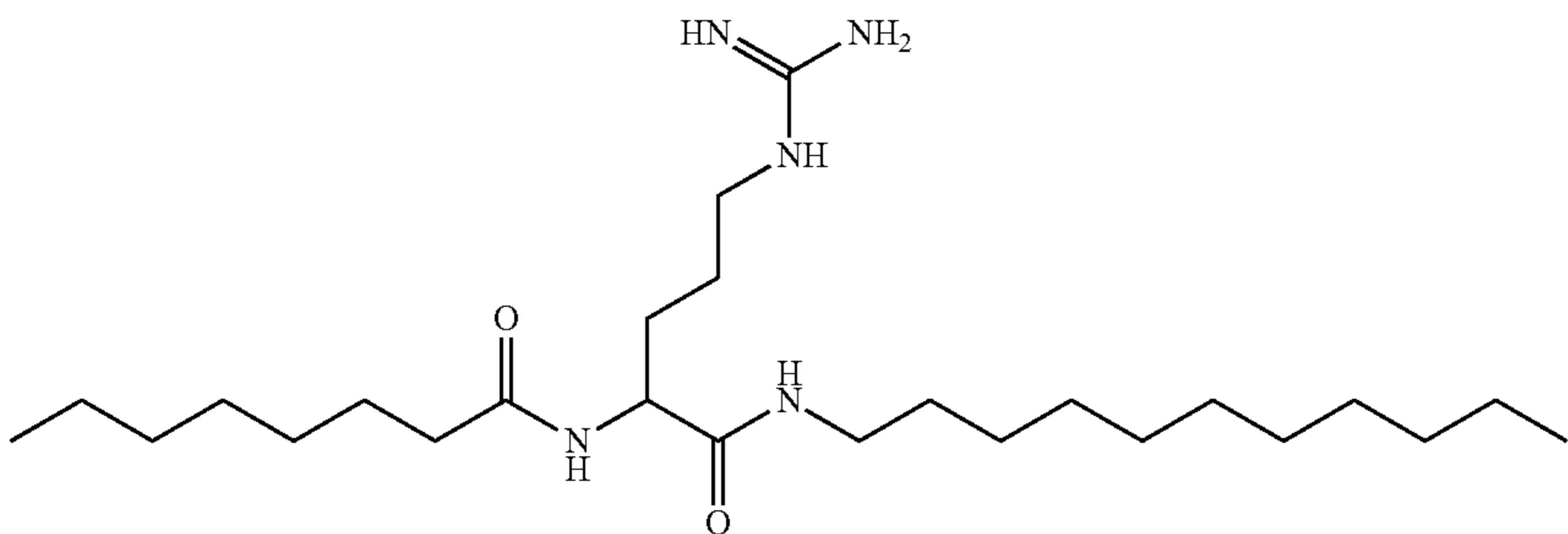
N-(5-guanidino-1-oxo-1-(undecylamino)pentan-2-yl)octanamide
