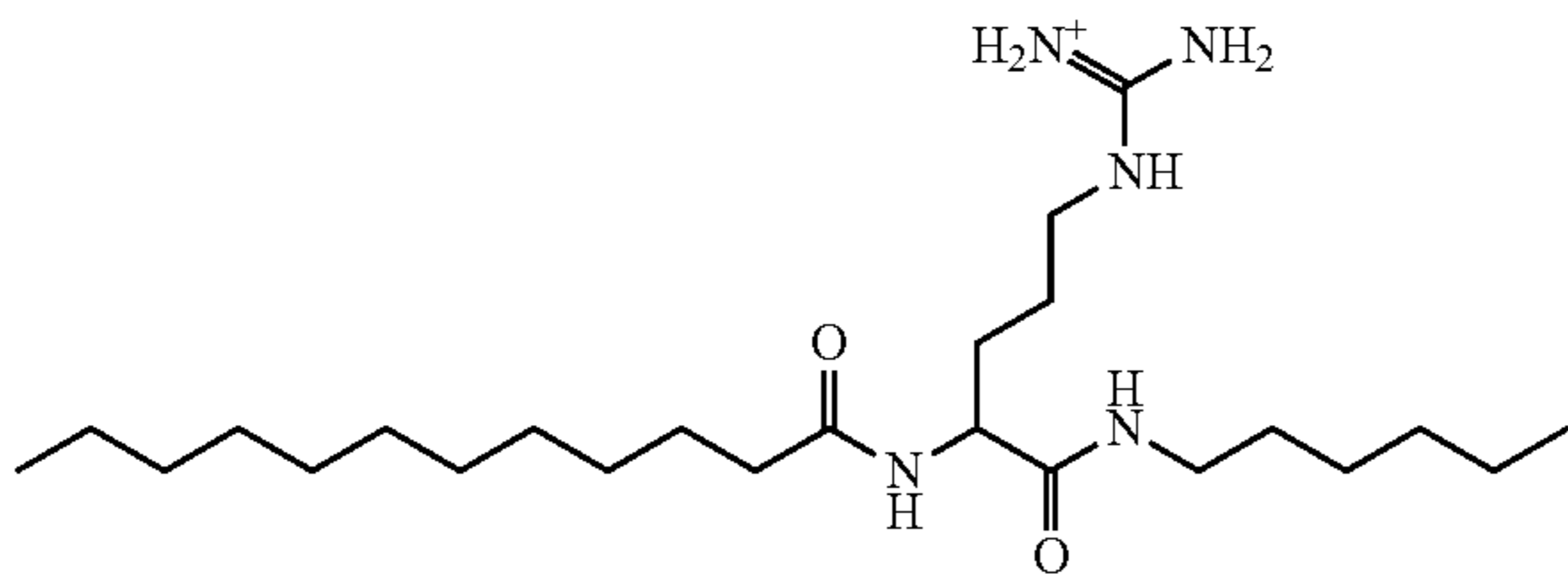
[amino({[4-dodecanamido-4-(hexylcarbamoyl)butyl]amino})methylidene]azanium;
