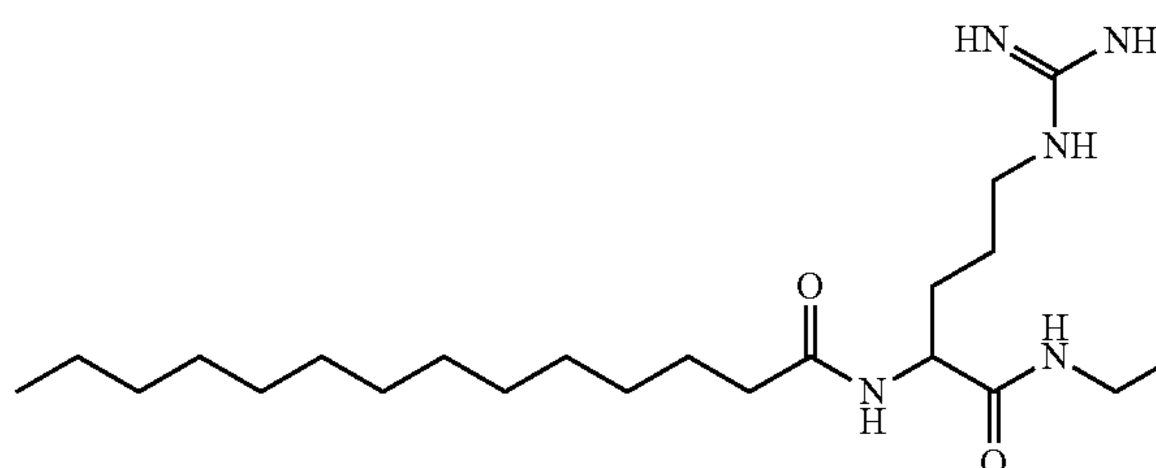
N-(1-(ethylamino)-5-guanidino-1-oxopentan-2-yl)tetradecanamide
