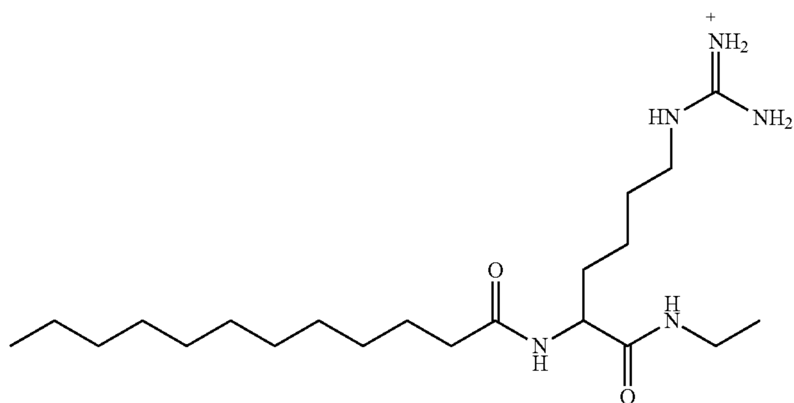
[amino({[5-dodecanamido-5-(ethylcarbamoyl)pentyl]amino}) methylidene]azanium;
