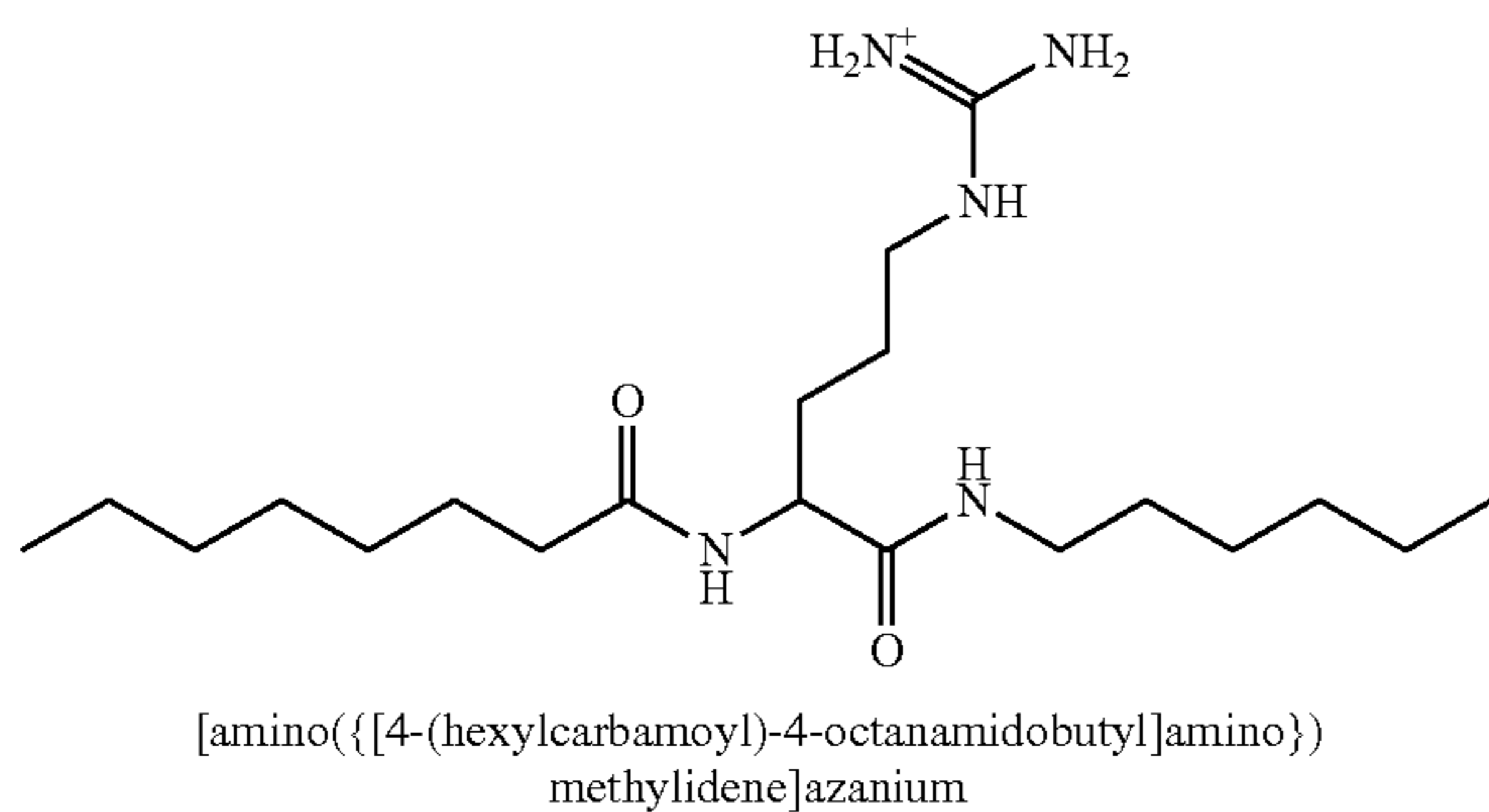
Compound 11
