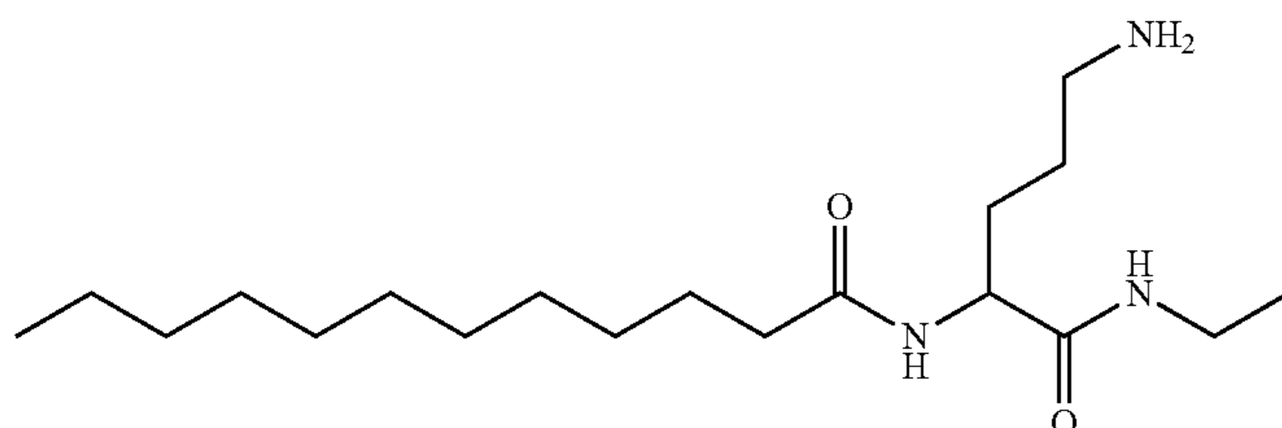
N[4-amino-1-(ethylcarbamoyl)butyl]dodecanamide;
