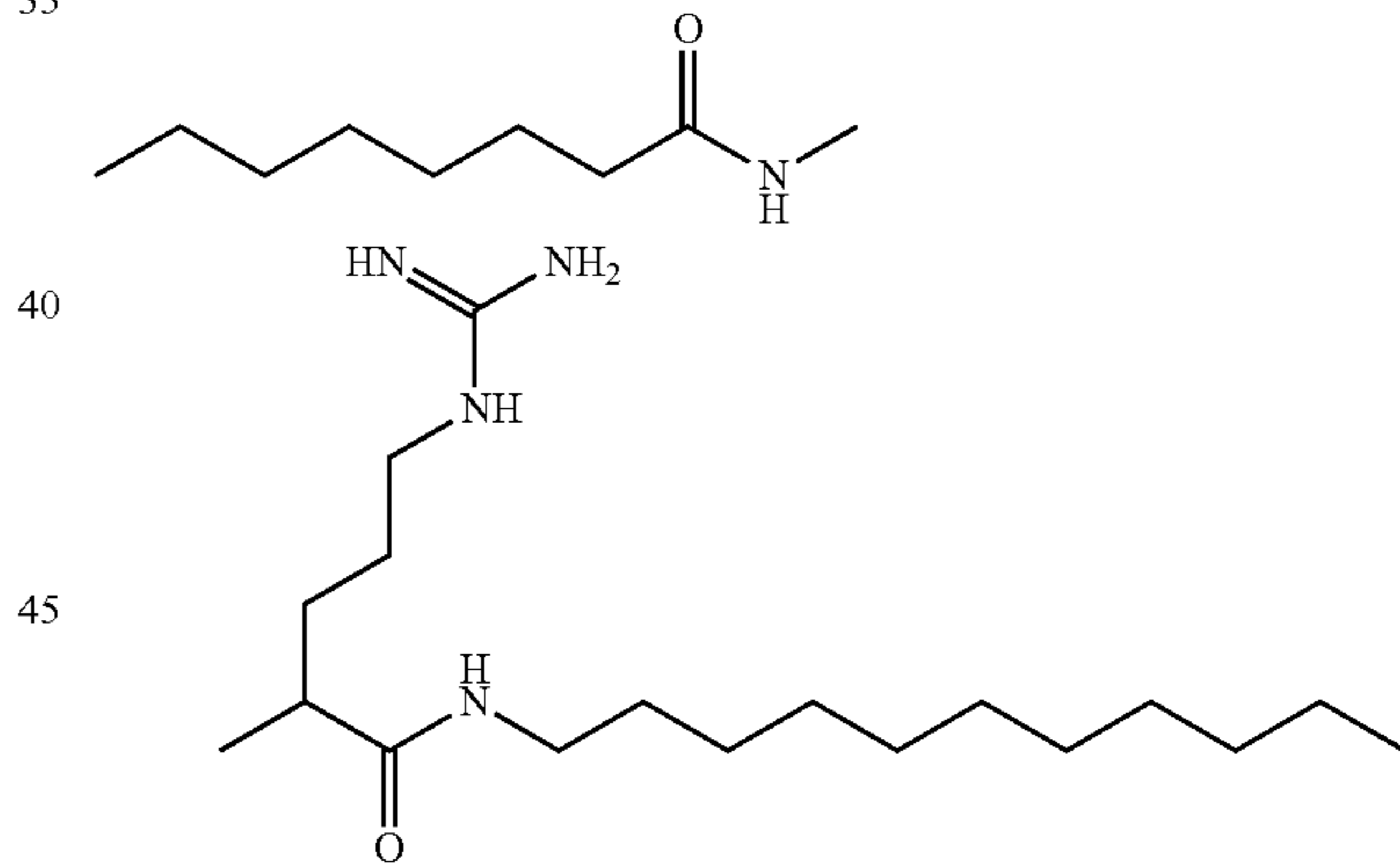
[amino({[5-dodecanamido-5-(ethylcarbamoyl)pentyl]amino})methylidene]azanium;
