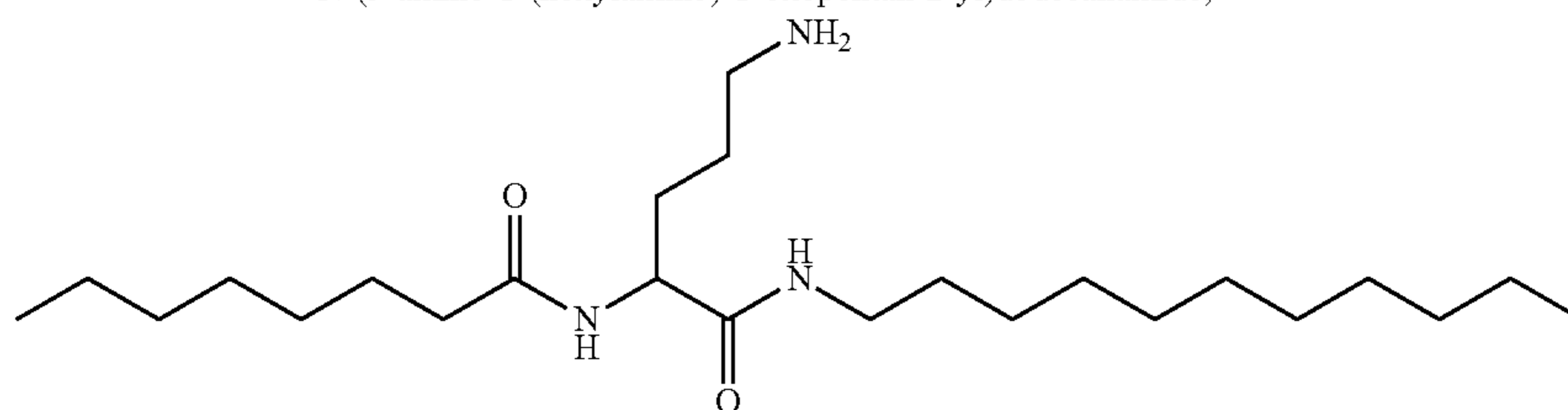
N-(5-amino-1-(hexylamino)-1-oxopentan-2-yl)dodecanamide;
