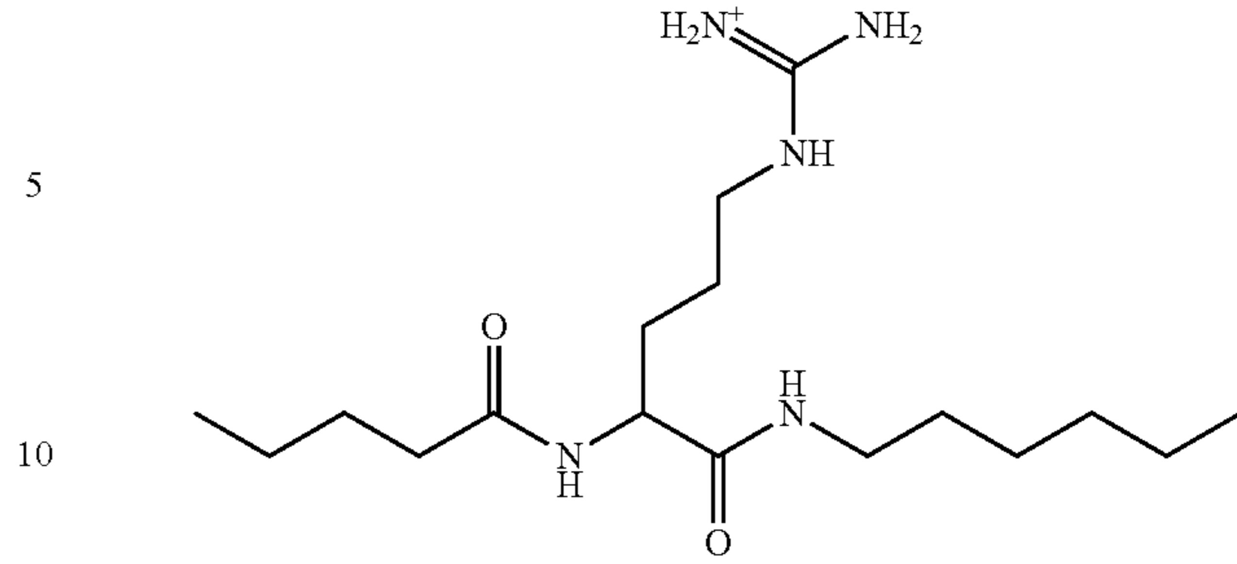
[amino({[4-(hexylcarbamoyl)-4-octadecanamidobutyl]amino})methylidene]azanium;
