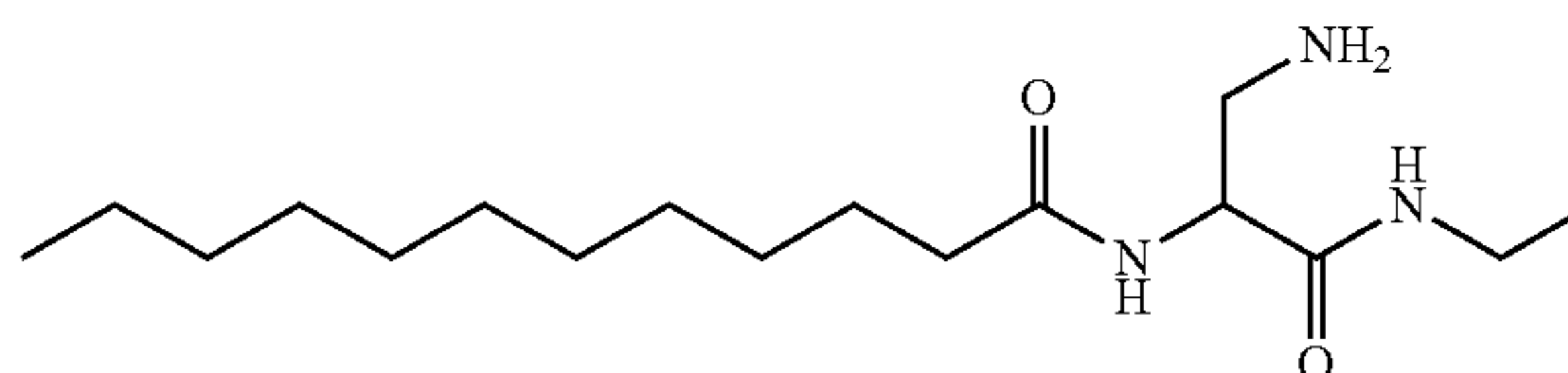
N-[2-amino-1-(ethylcarbamoyl)ethyl]dodecanamide
