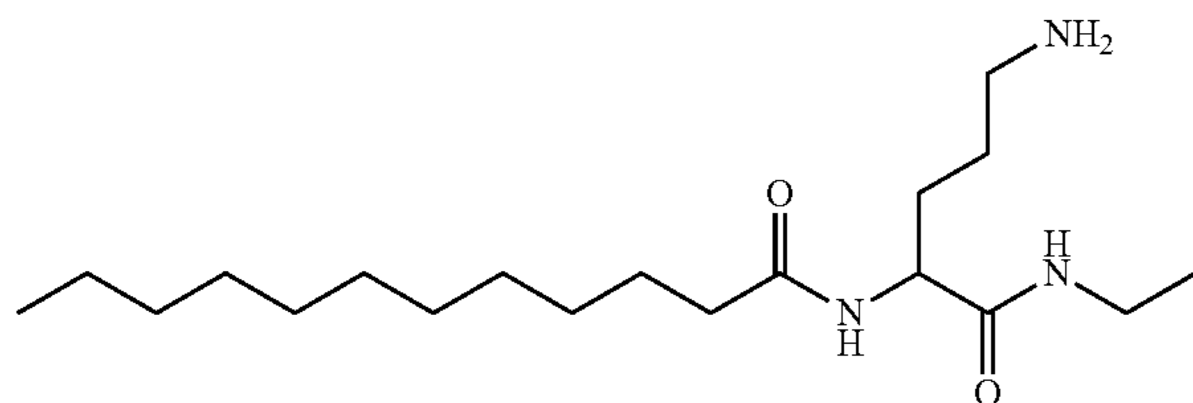
N-[4-amino-1-(ethylcarbamoyl)butyl]dodecanamide
