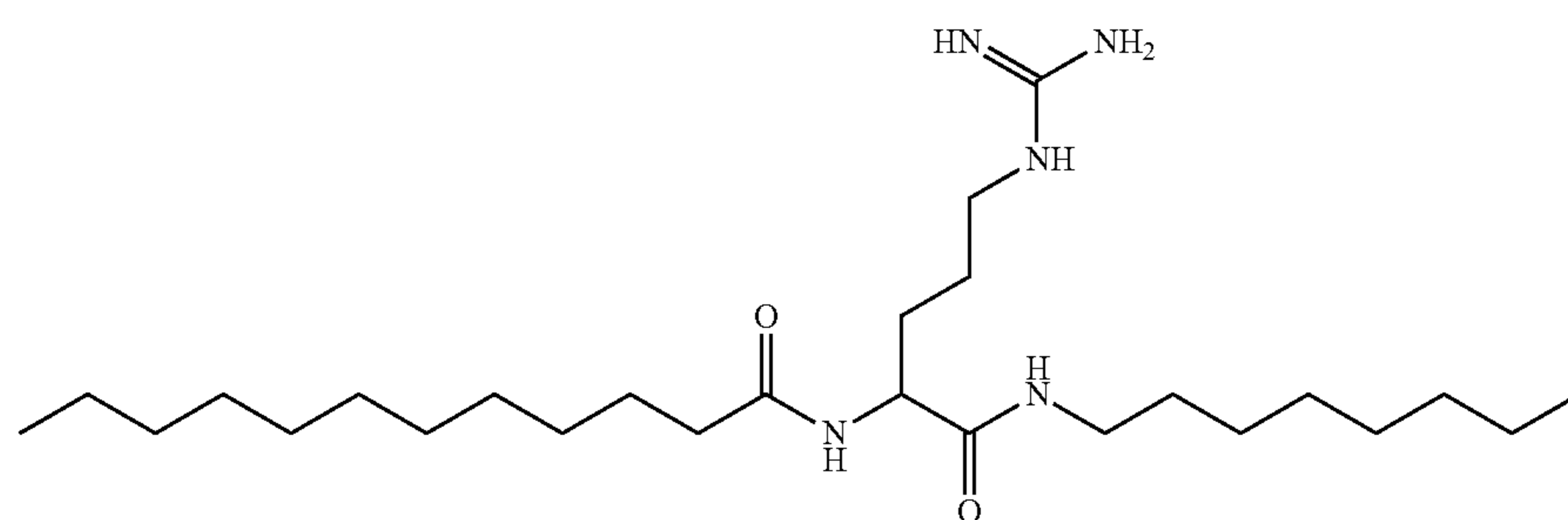
N-(5-guanidino-1-(octylamino)-1-oxopentan-2-yl)dodecanamide
