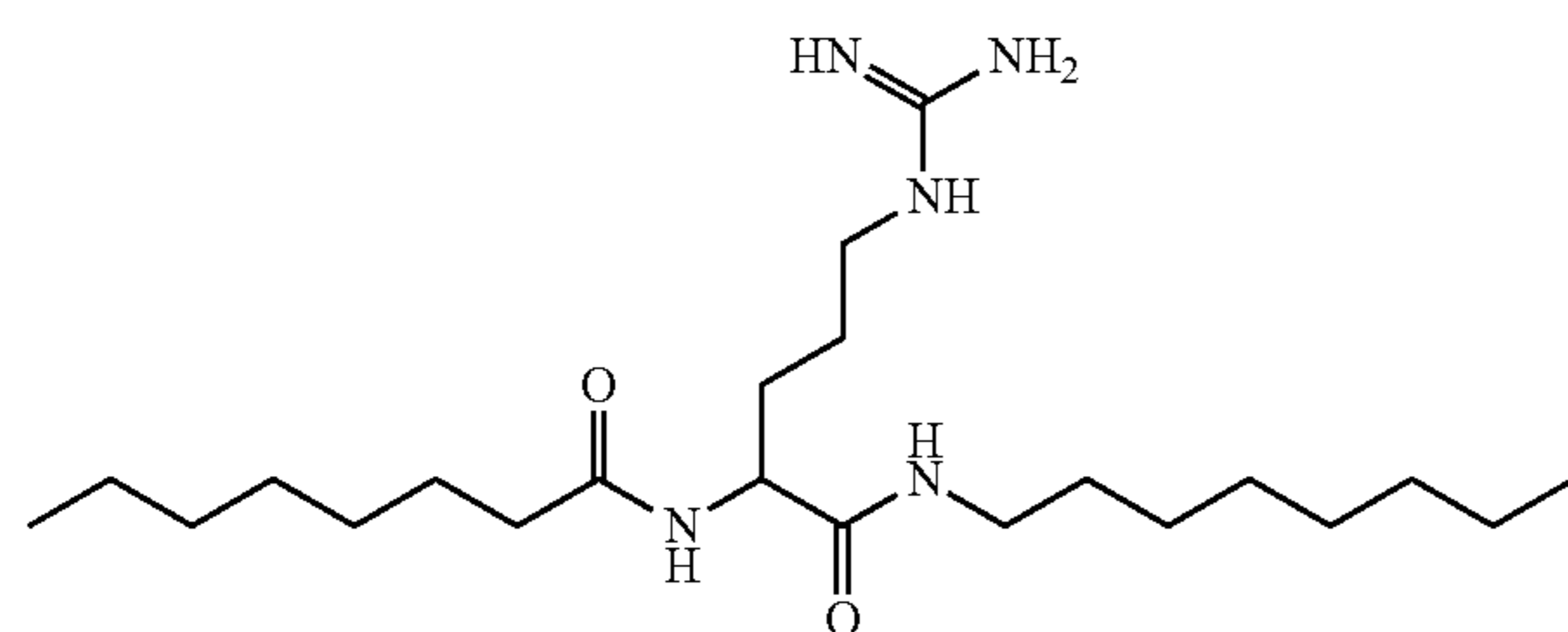
N-(5-guanidino-1-(octylamino)-1-oxopentan-2-yl)octanamide
