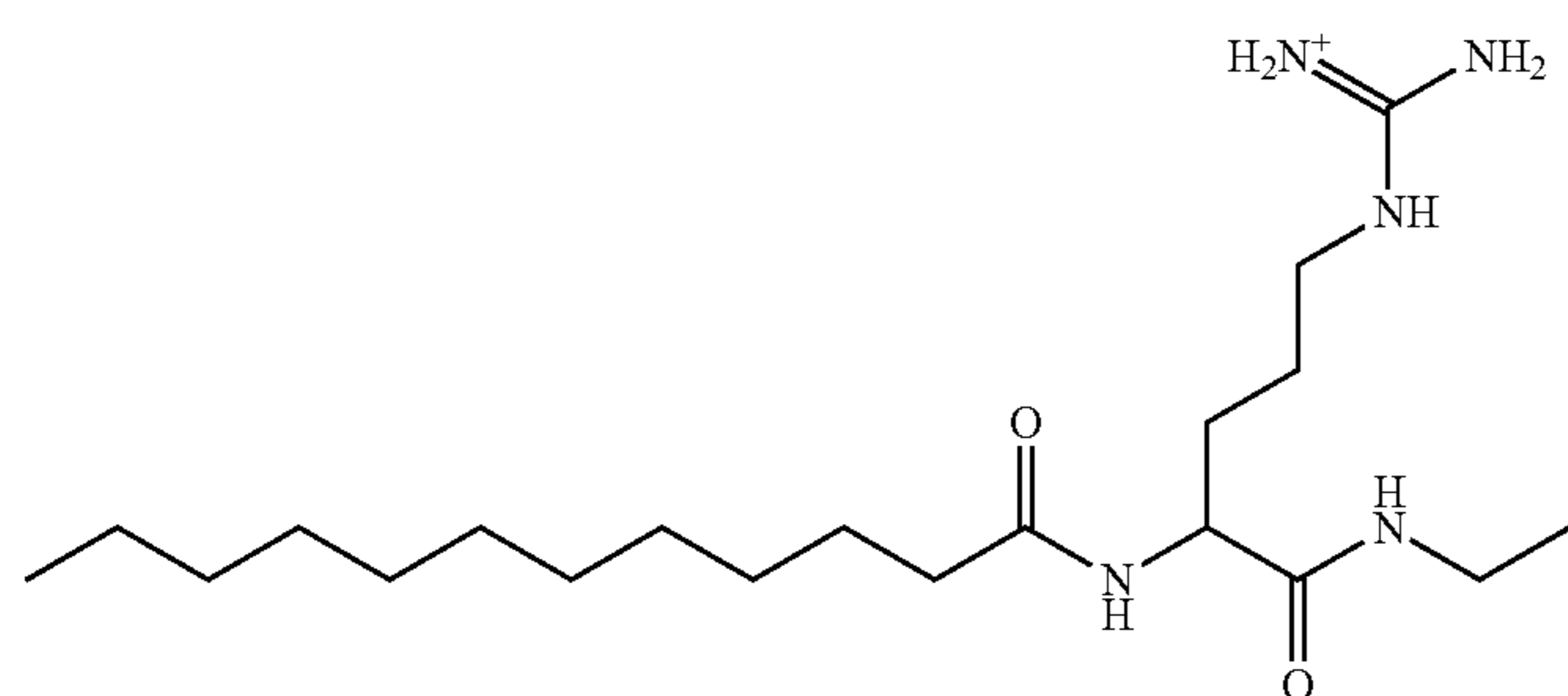
[amino({[4-(dodecanamido)-4-(ethylcarbamoyl)butyl]amino}) methylidene]azanium;
