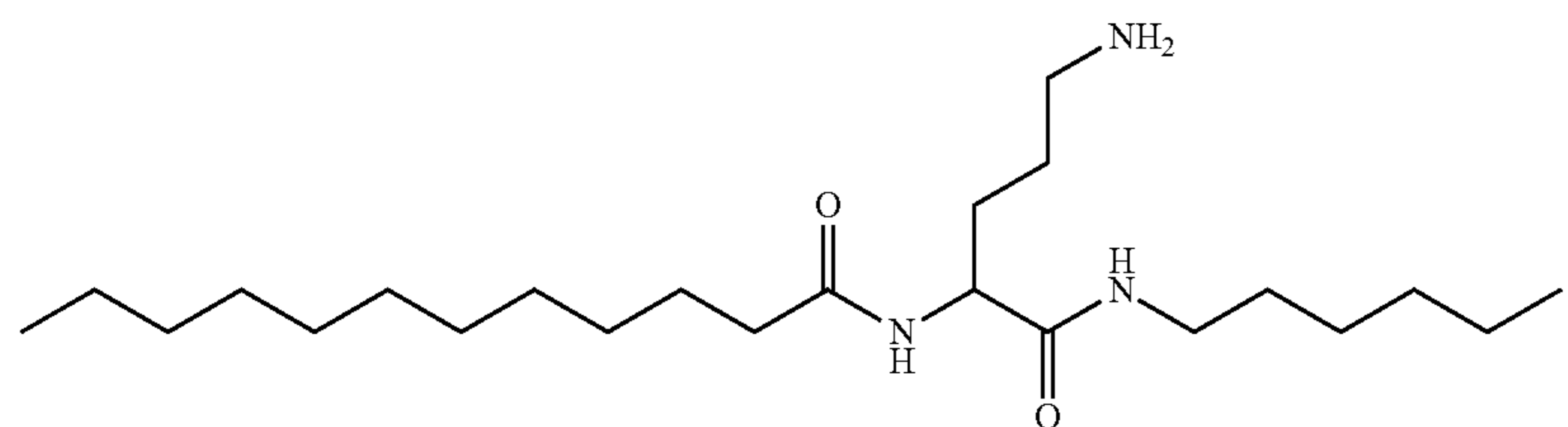
N-(5-amino-1-(hexylamino)-1-oxopentan-2-yl)dodecanamide
