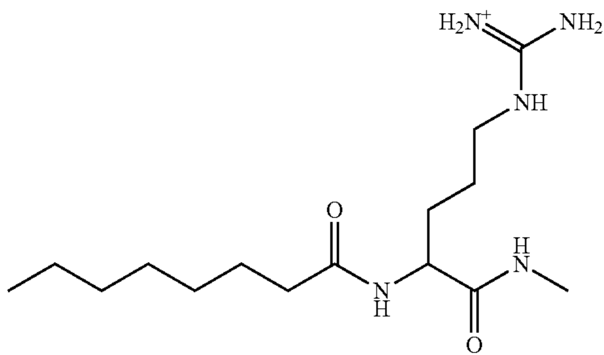
[amino({[4-(methylcarbamoyl)-4-octanamidobutyl]amino})methylidene]azanium;
