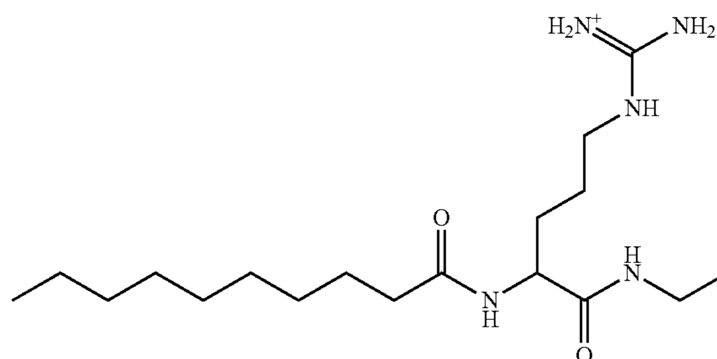
[amino({[4-dodecanamido-4-(ethylcarbamoyl)butyl}amino)methylidene]azanium;
