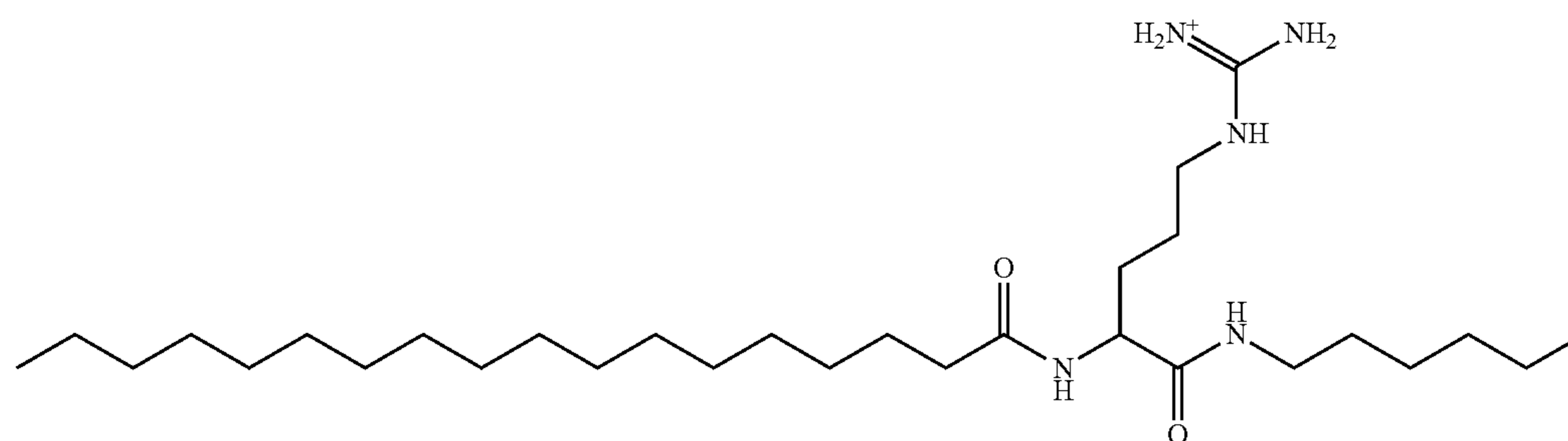
[amino({[4-(hexylcarbamoyl)-4-octadecanamidobutyl]amino})methylidene]azanium;
