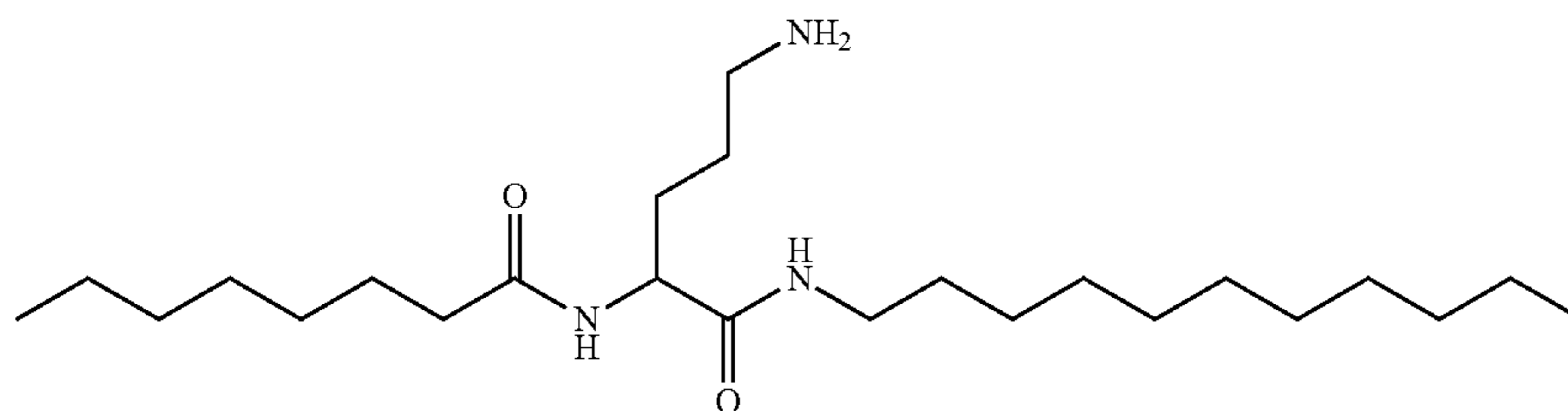
N-(5-amino-1-oxo-1-(undecylamino)pentan-2-yl)dodecanamide
