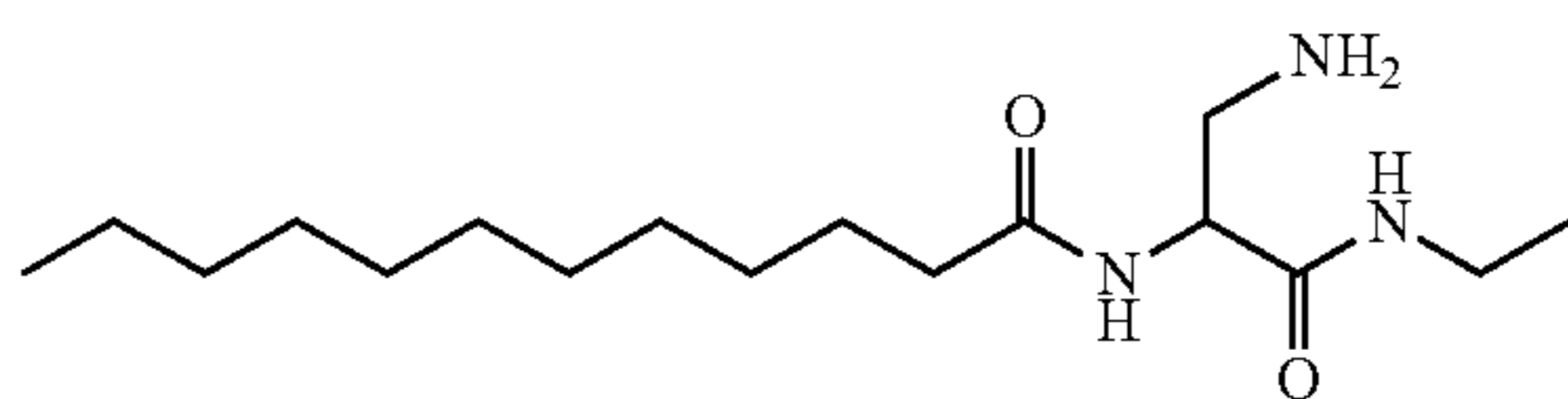
N-[2-amino-1-(ethylcarbamoyl)ethylol]dodecanamide;
