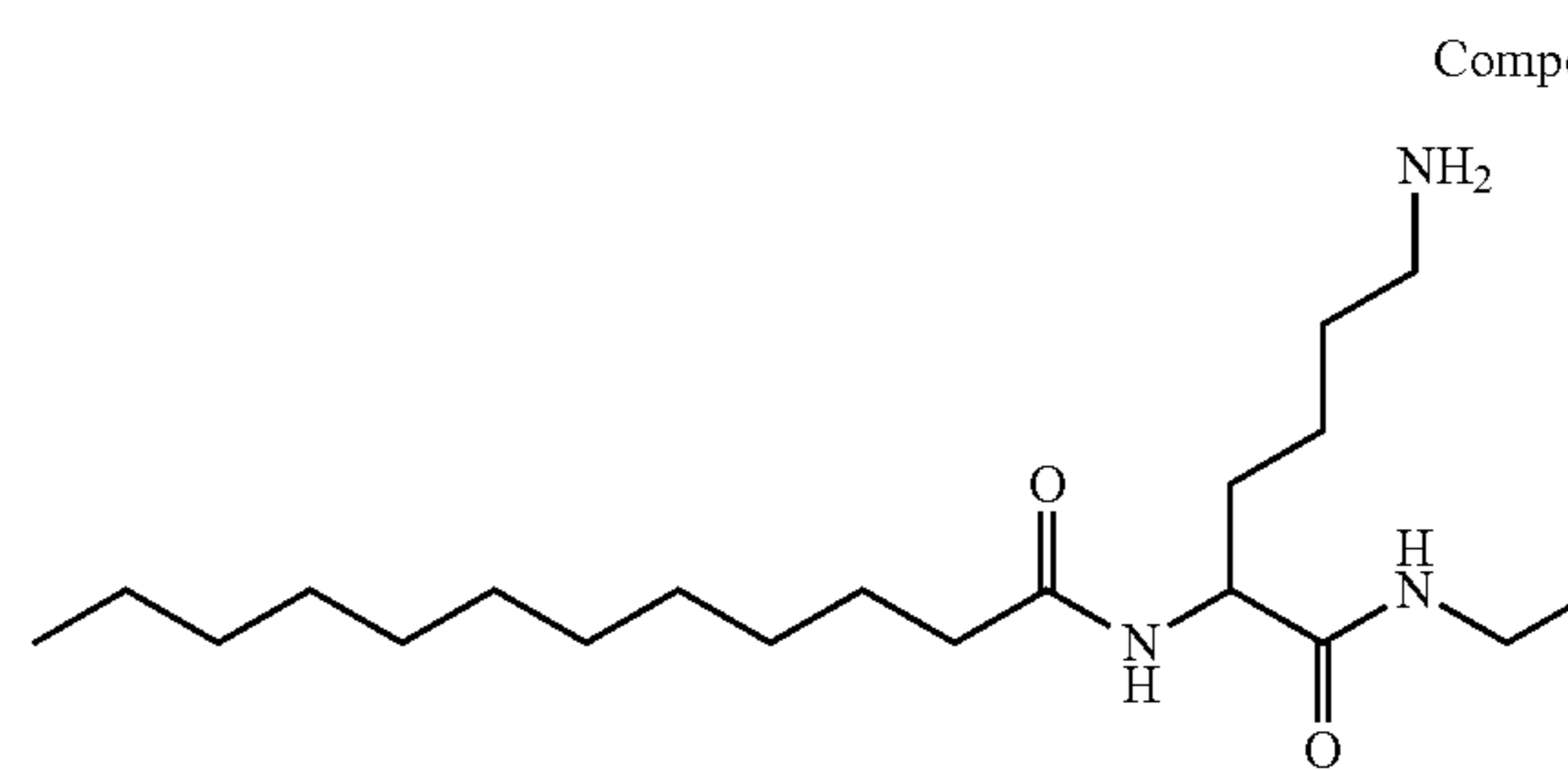
N-[5-amino-1-(ethylcarbamoyl)pentyl]dodecanamide
