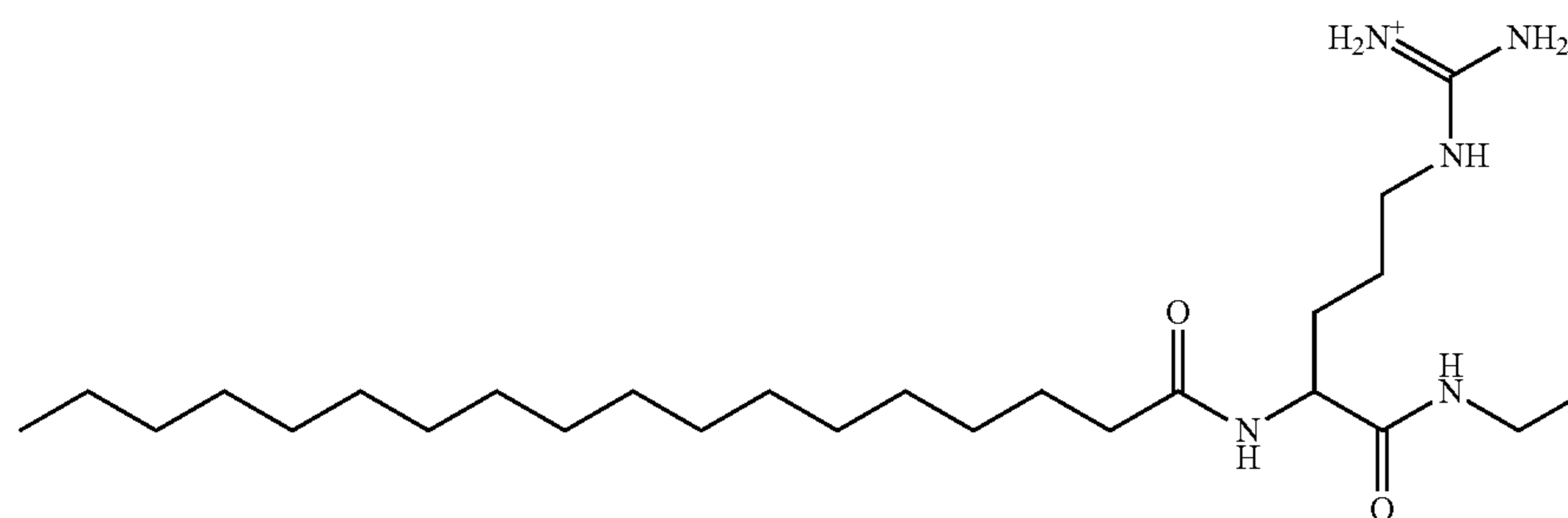
[amino({[4-(ethylcarbamoyl)-4-octadecanamidobutyl]amino})methylidene]azanium
