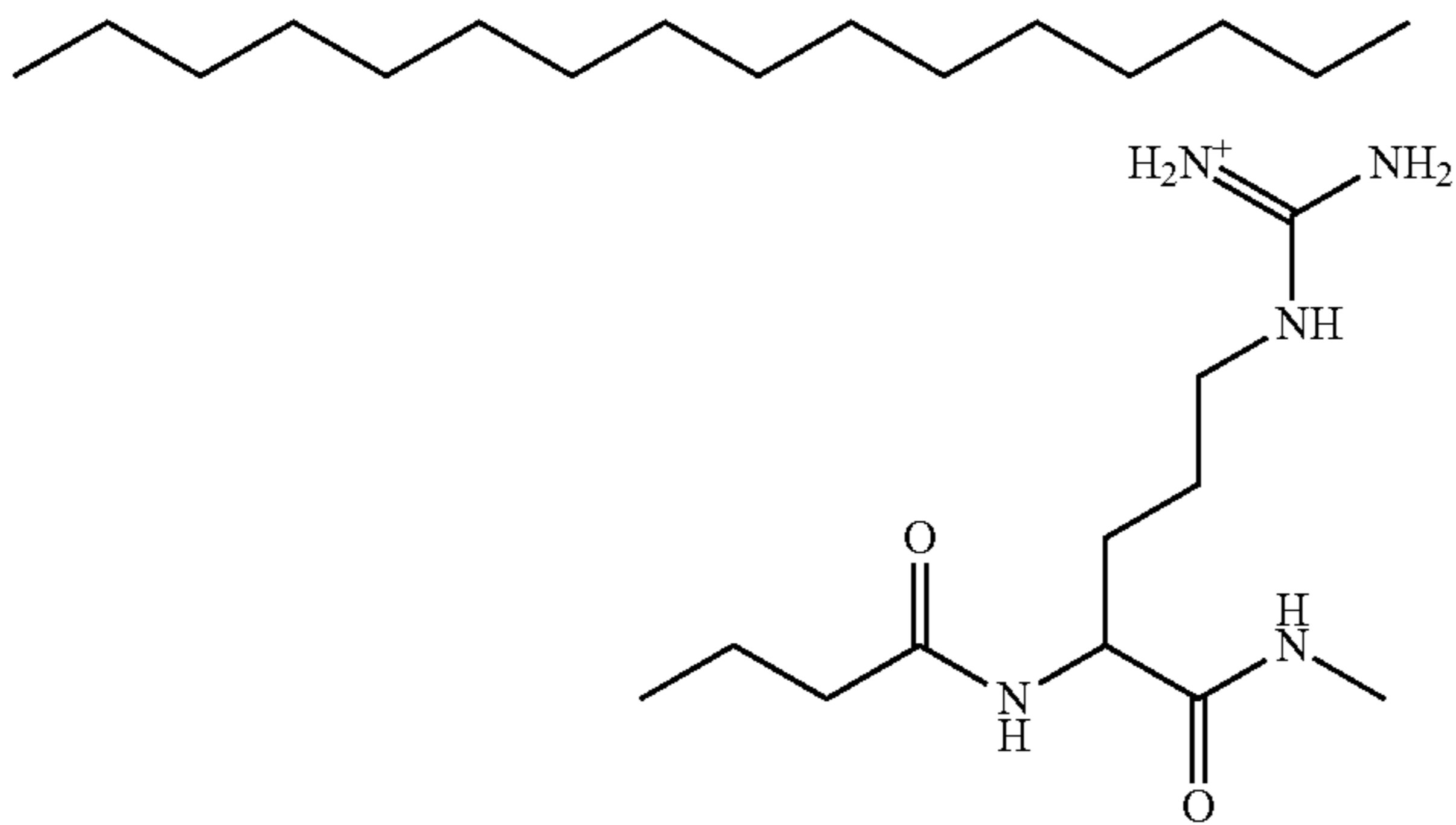
[amino({[4-((methylcarbamoyl)-4-(octadecanamidobutyl)amino})methylidene]azanium);
