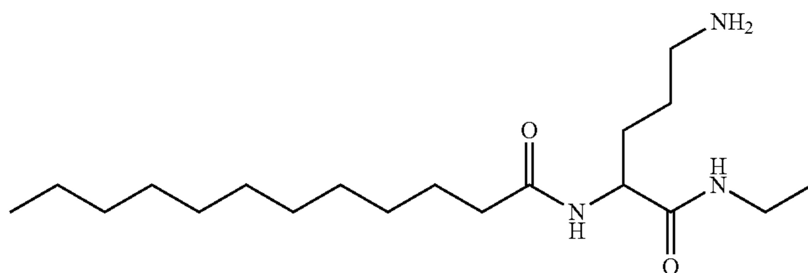
N[4-amino-1-(ethylcarbamoyl)butyl]dodecanamide;
