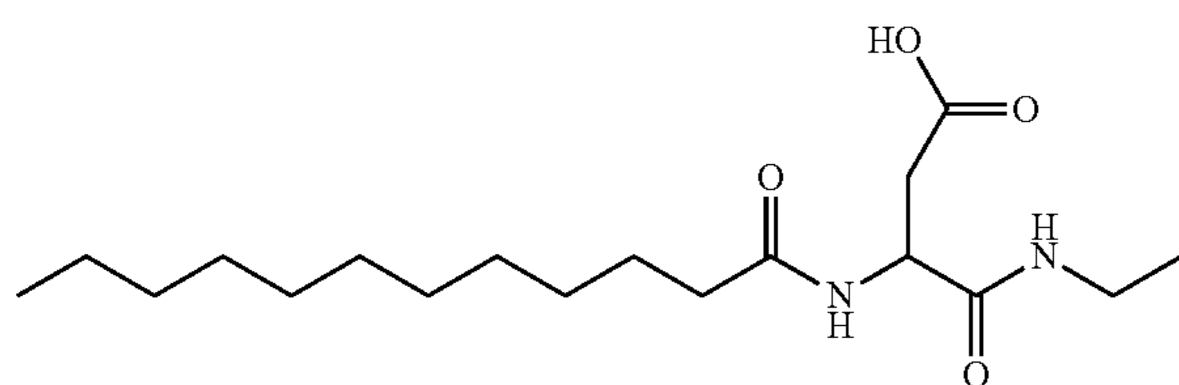
3-dodecanamido-4-(ethylamino)-4-oxobutanoic acid
