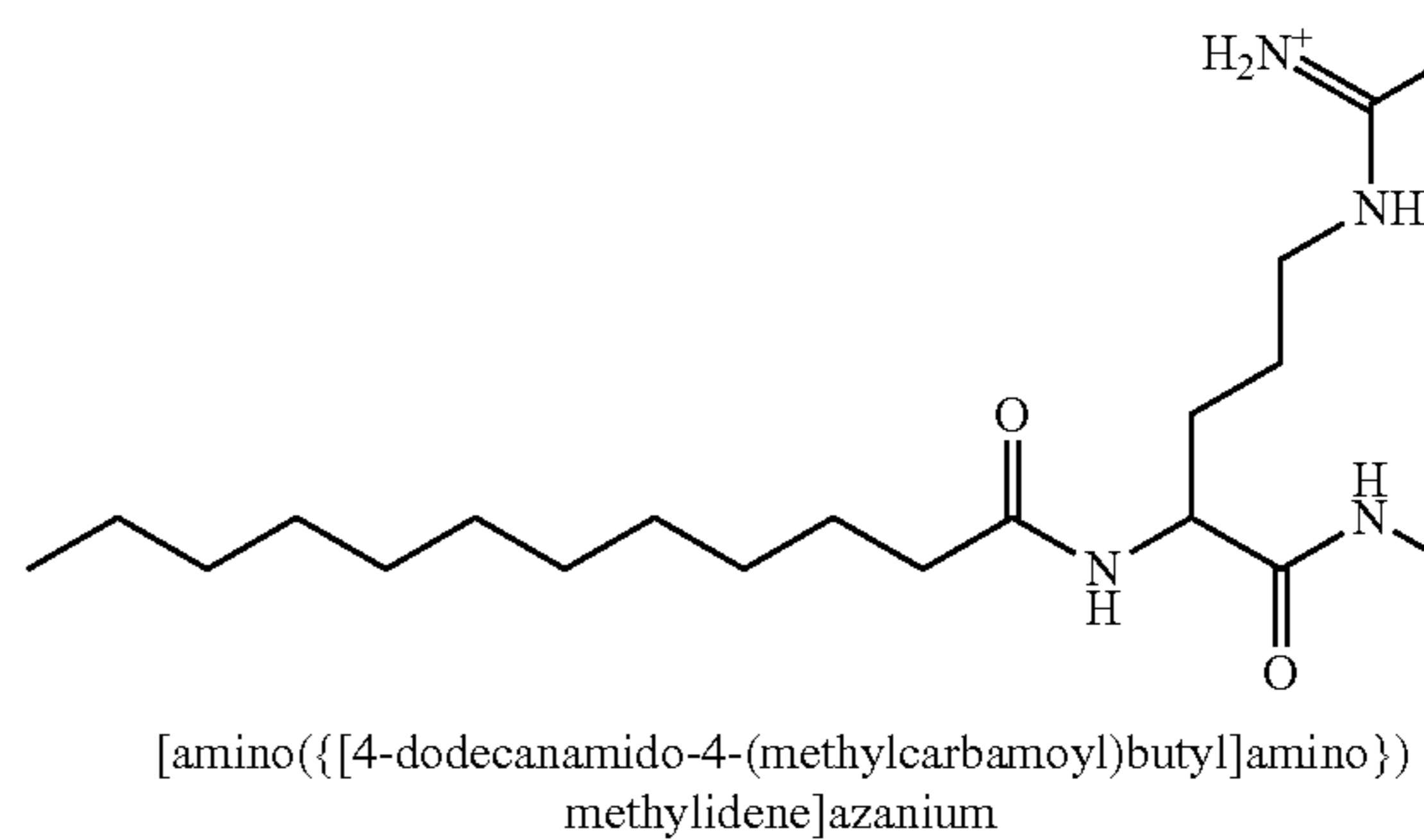
Compound 6
