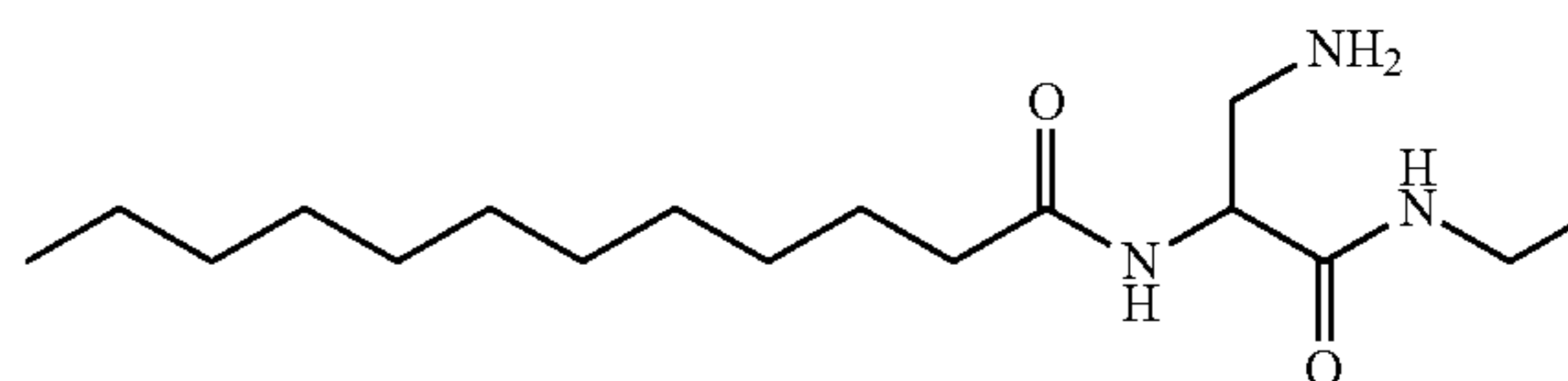
N-[2-amino-1-(ethylcarbamoyl)ethyl]dodecanamide;
