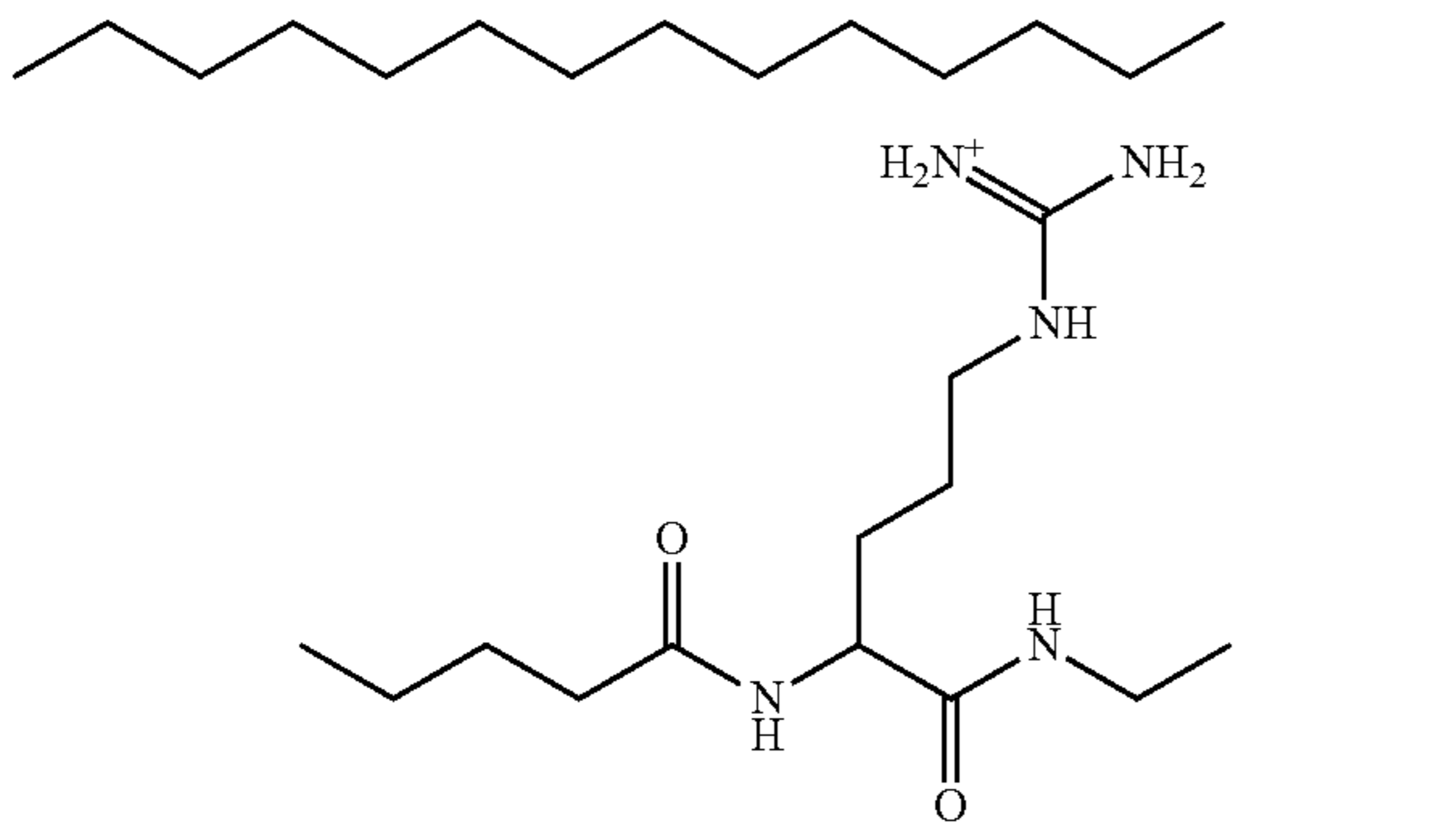
[amino({[4-((methylcarbamoyl)-4-(octadecanamidobutyl)amino})methylidene]azanium);
