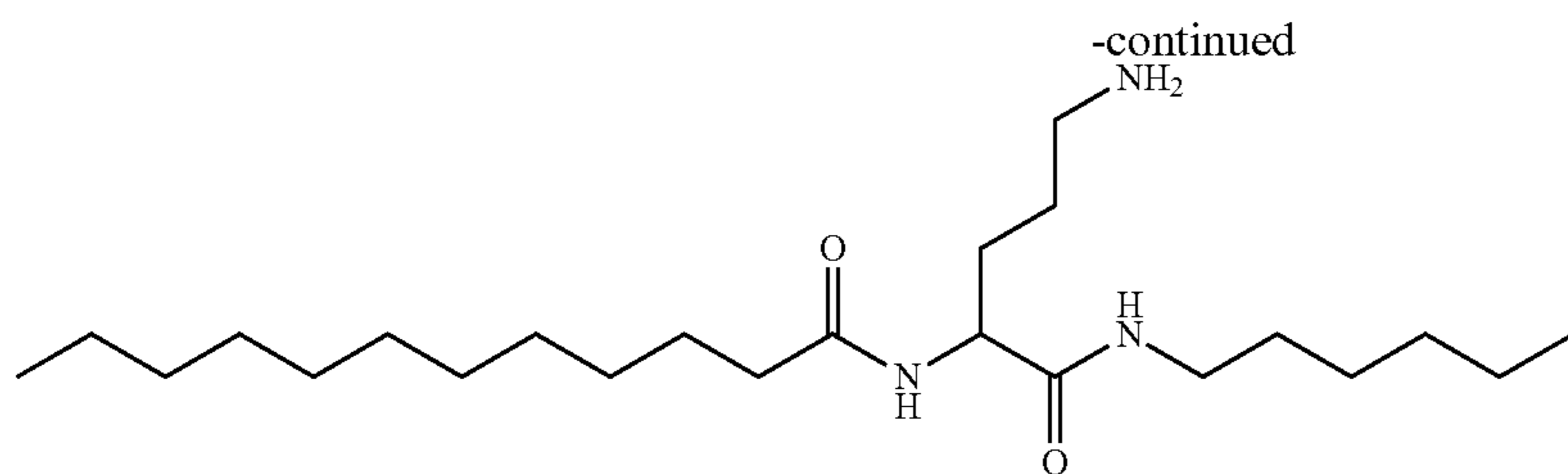
N-(5-amino-1-(hexylamino)-1-oxopentan-2-yl)dodecanamide;
