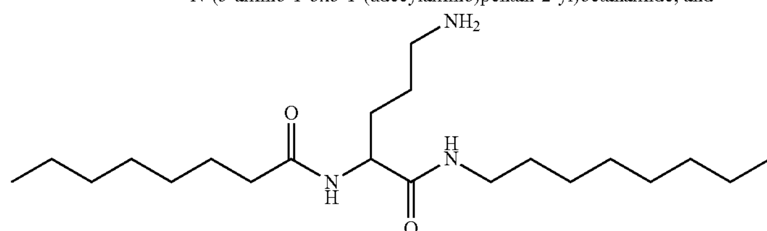
N-(5-amino-1-oxo-1-(decylamino)pentan-2-yl)octanamide; and
