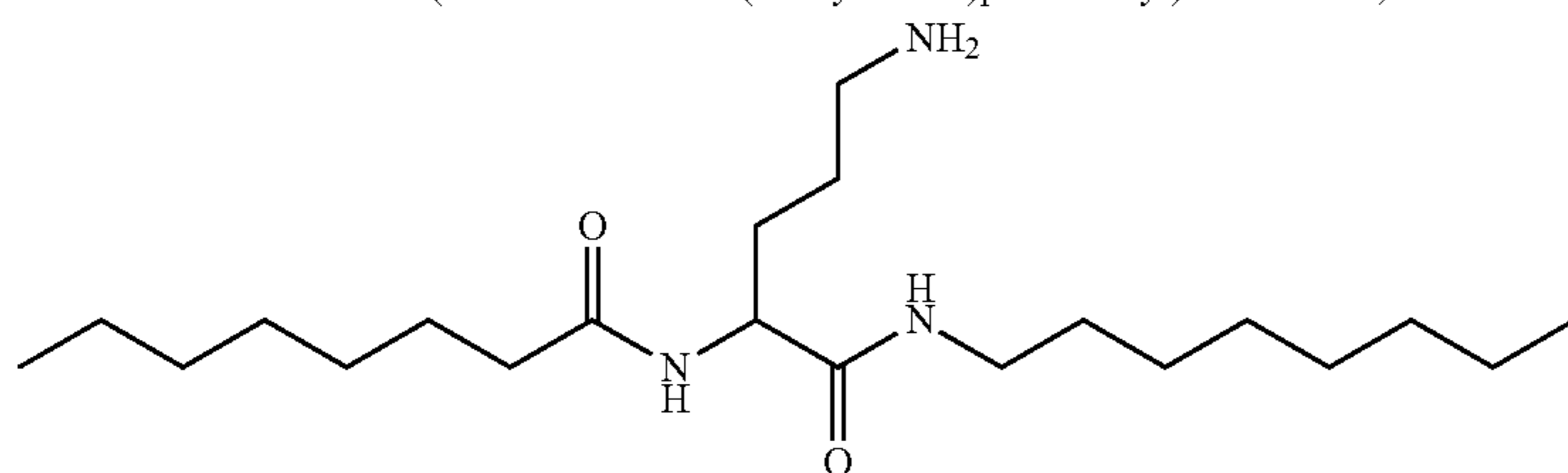
N-(5-amino-1-oxo-1-(decylamino)pentan-2-yl)octanamide; and
