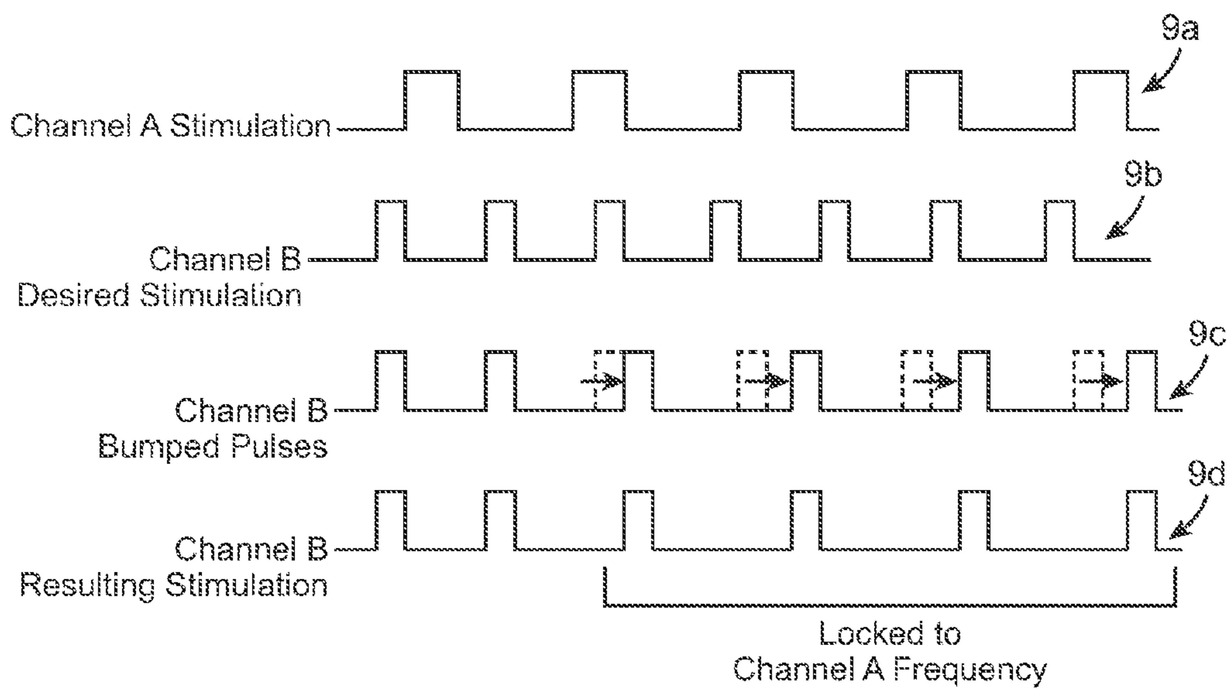
FIG. 4 (PRIOR ART)
