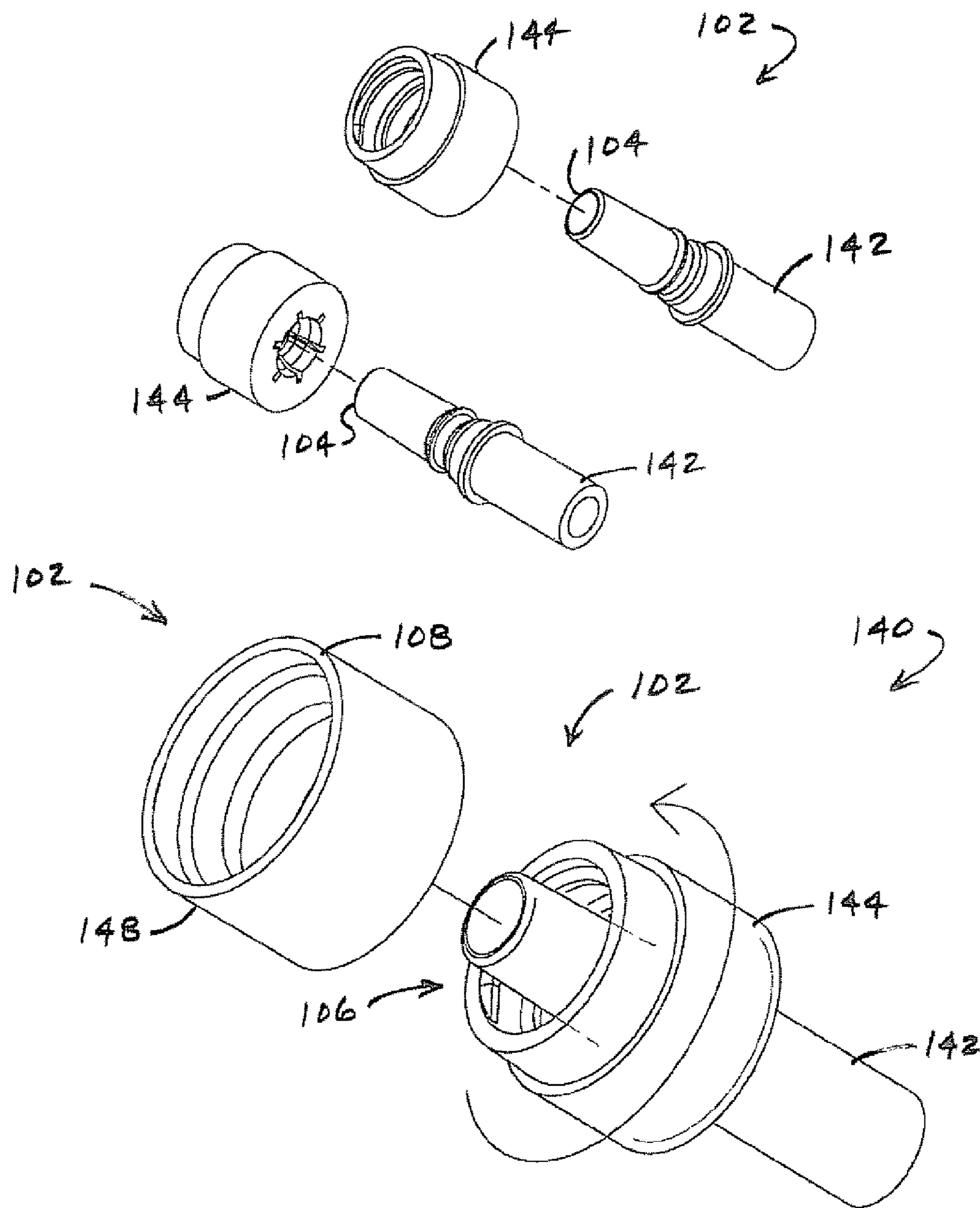
ROTATABLE COLLAR
