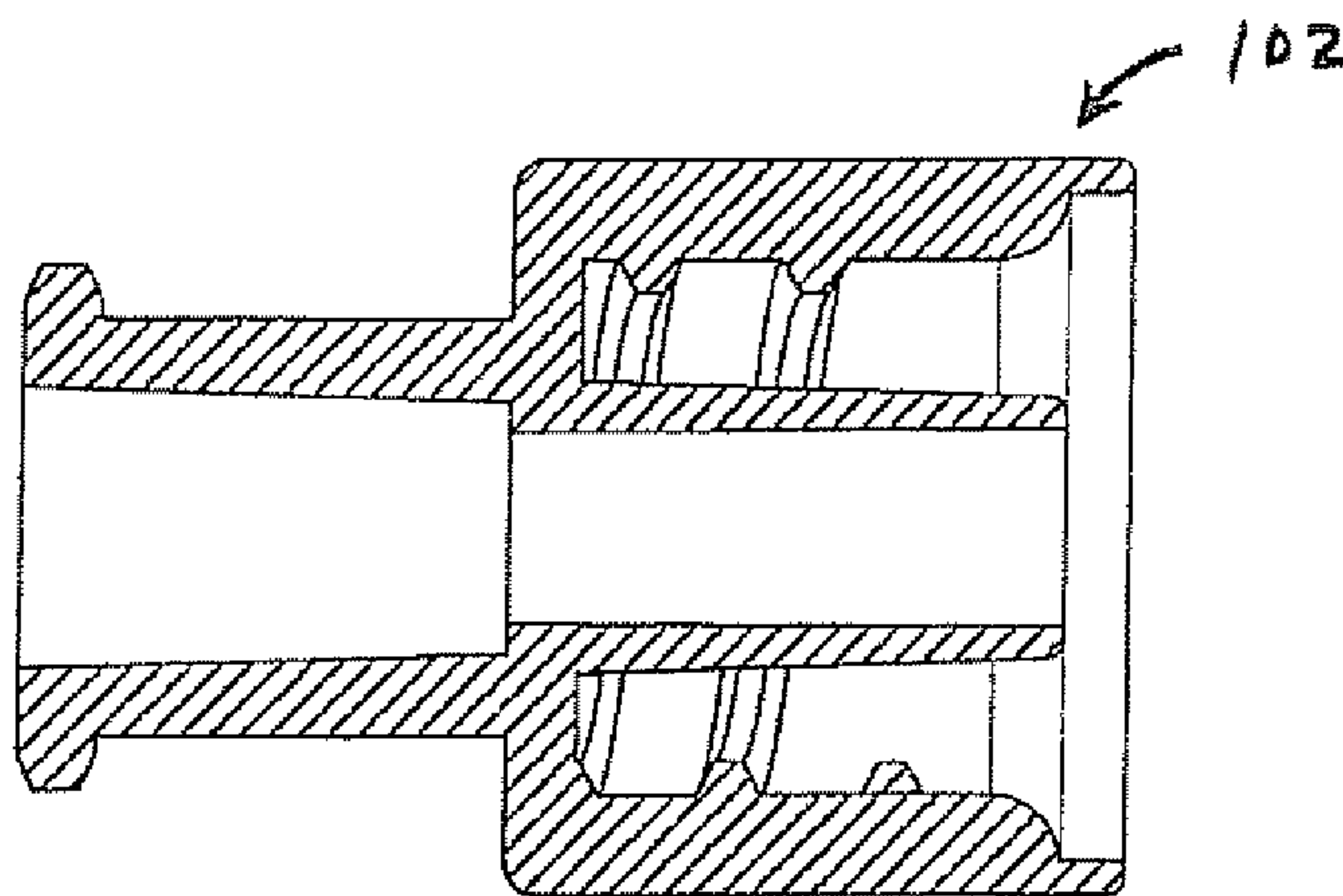
SECTION B-B
