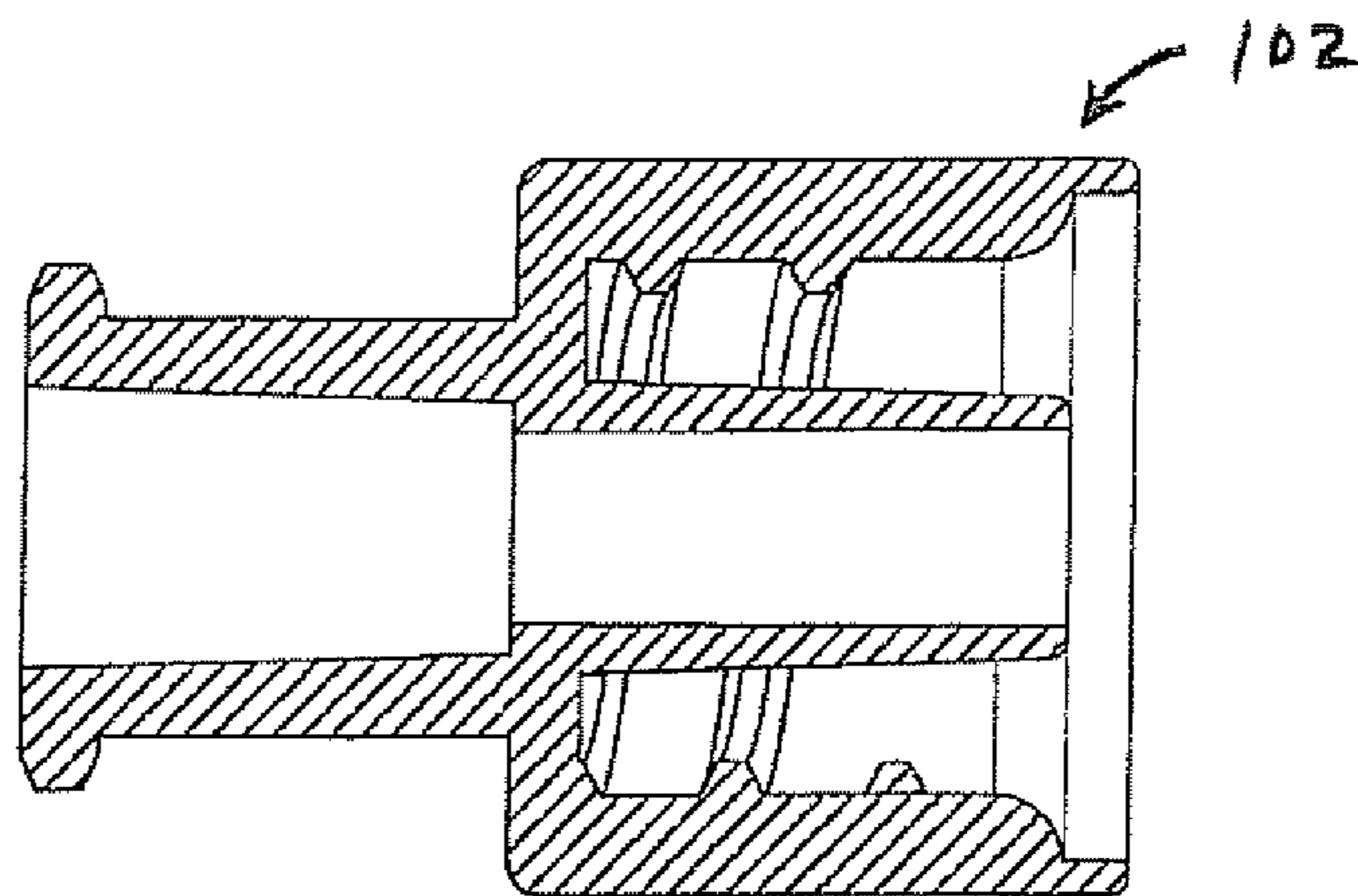
SECTION B-B
