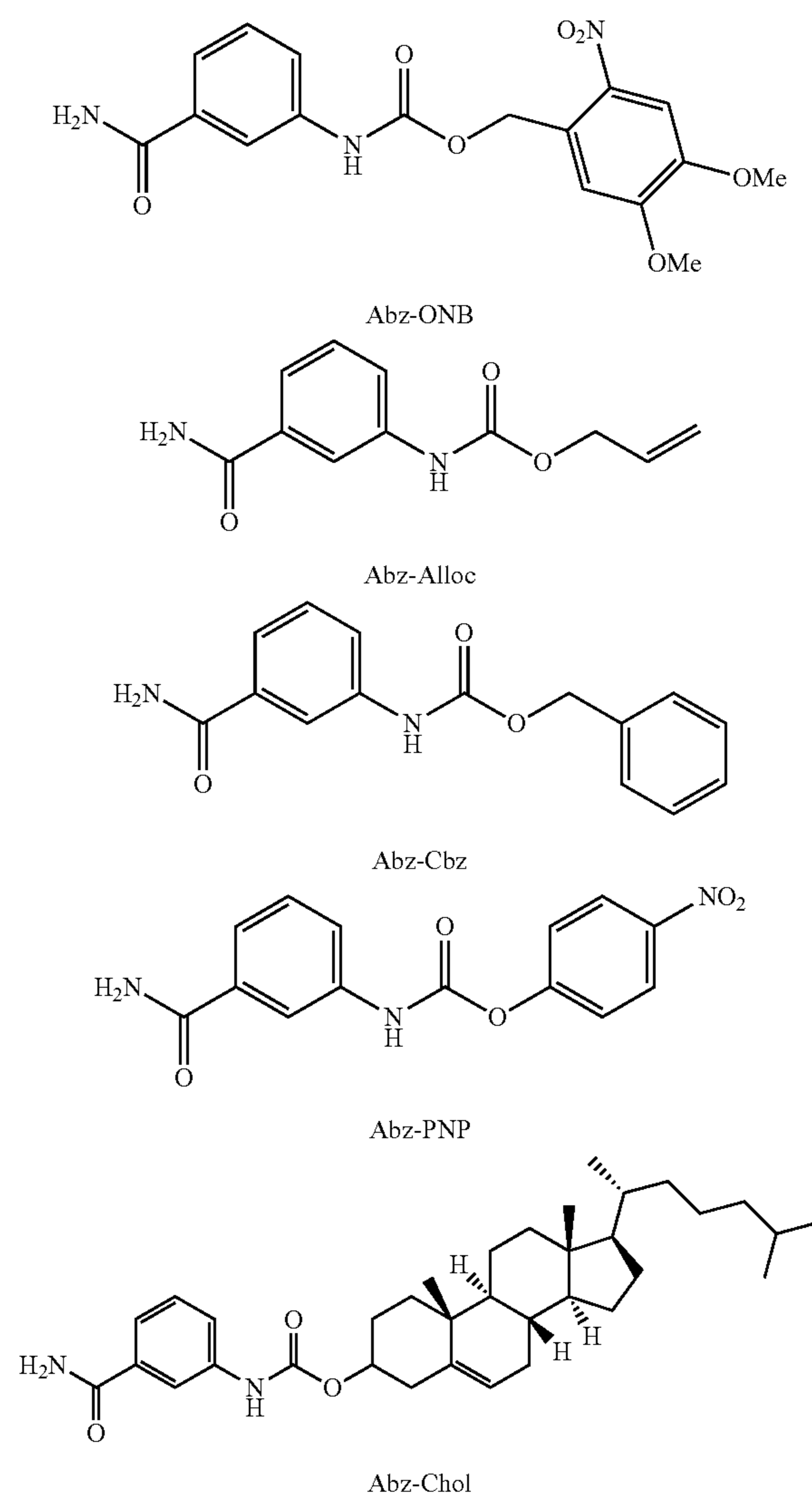
Scheme 3-1. Structures of synthesized Abz-derived amphiphiles.
