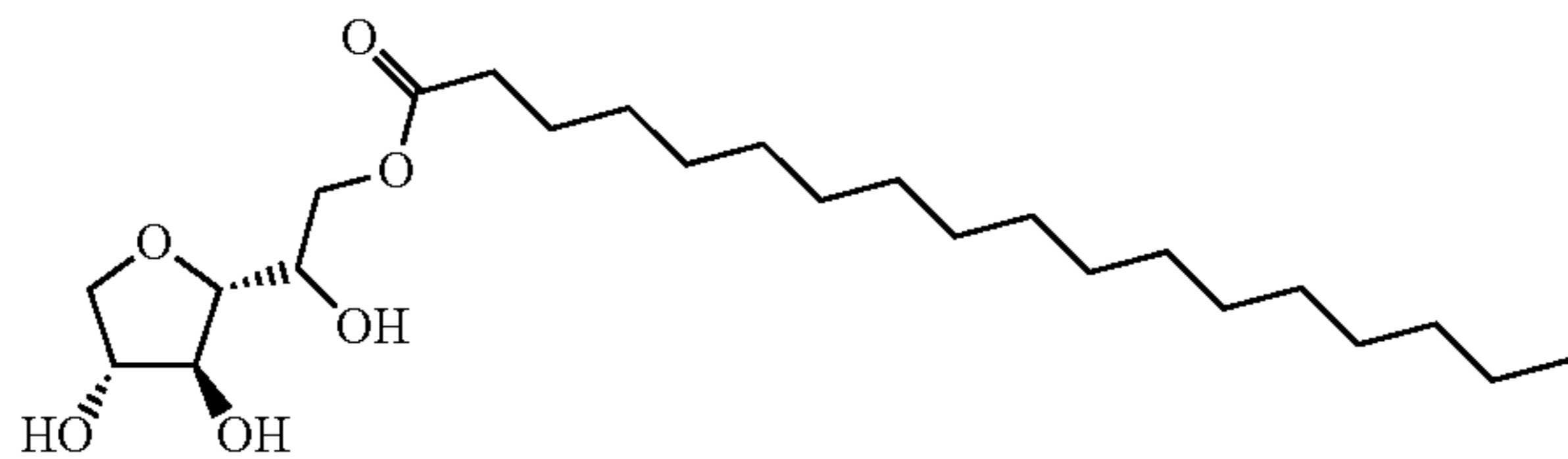
Scheme 4-1. Chemical structure of sorbitan monostearate (SMS).
