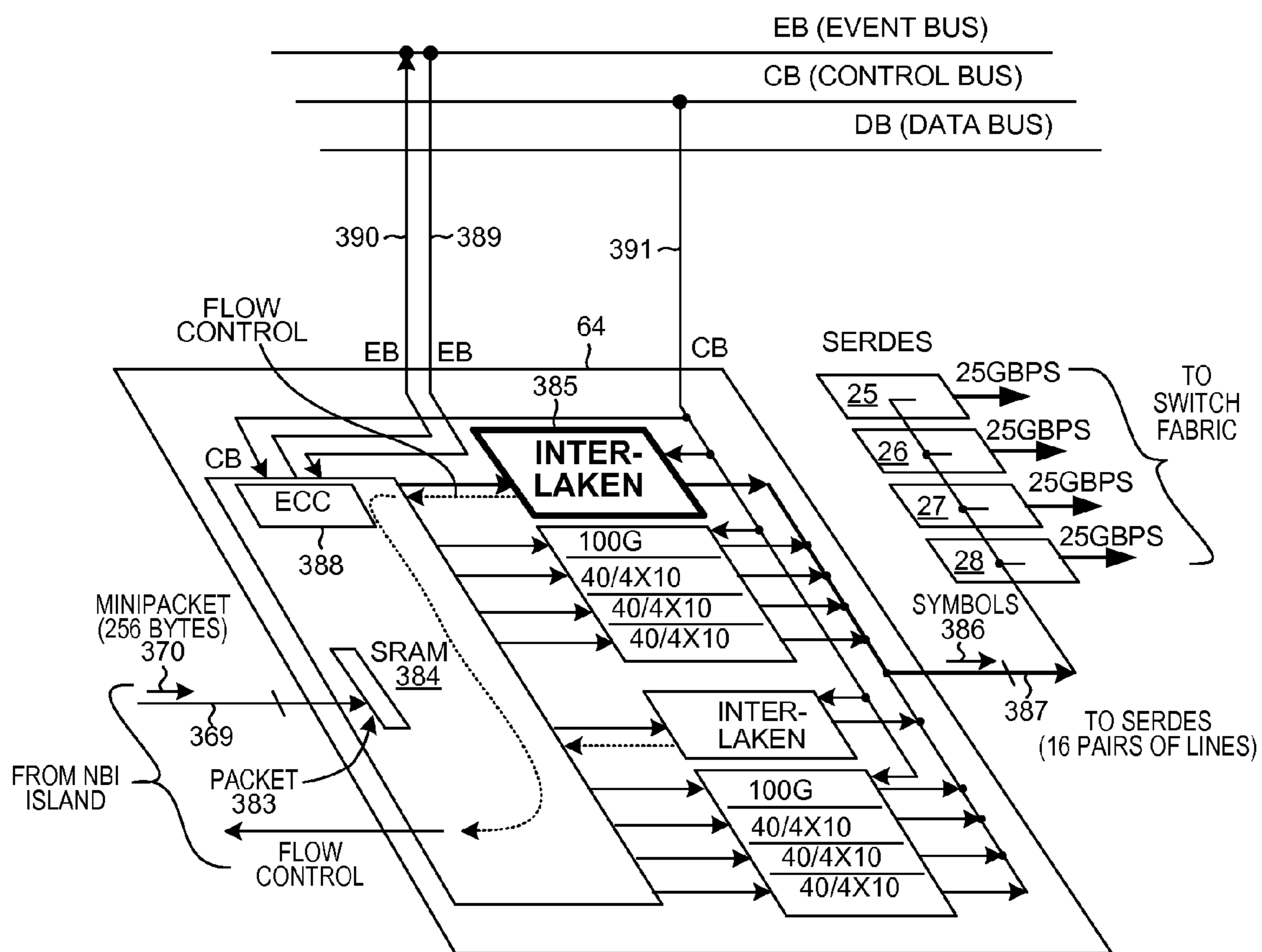
MAC ISLAND (EGRESS)
