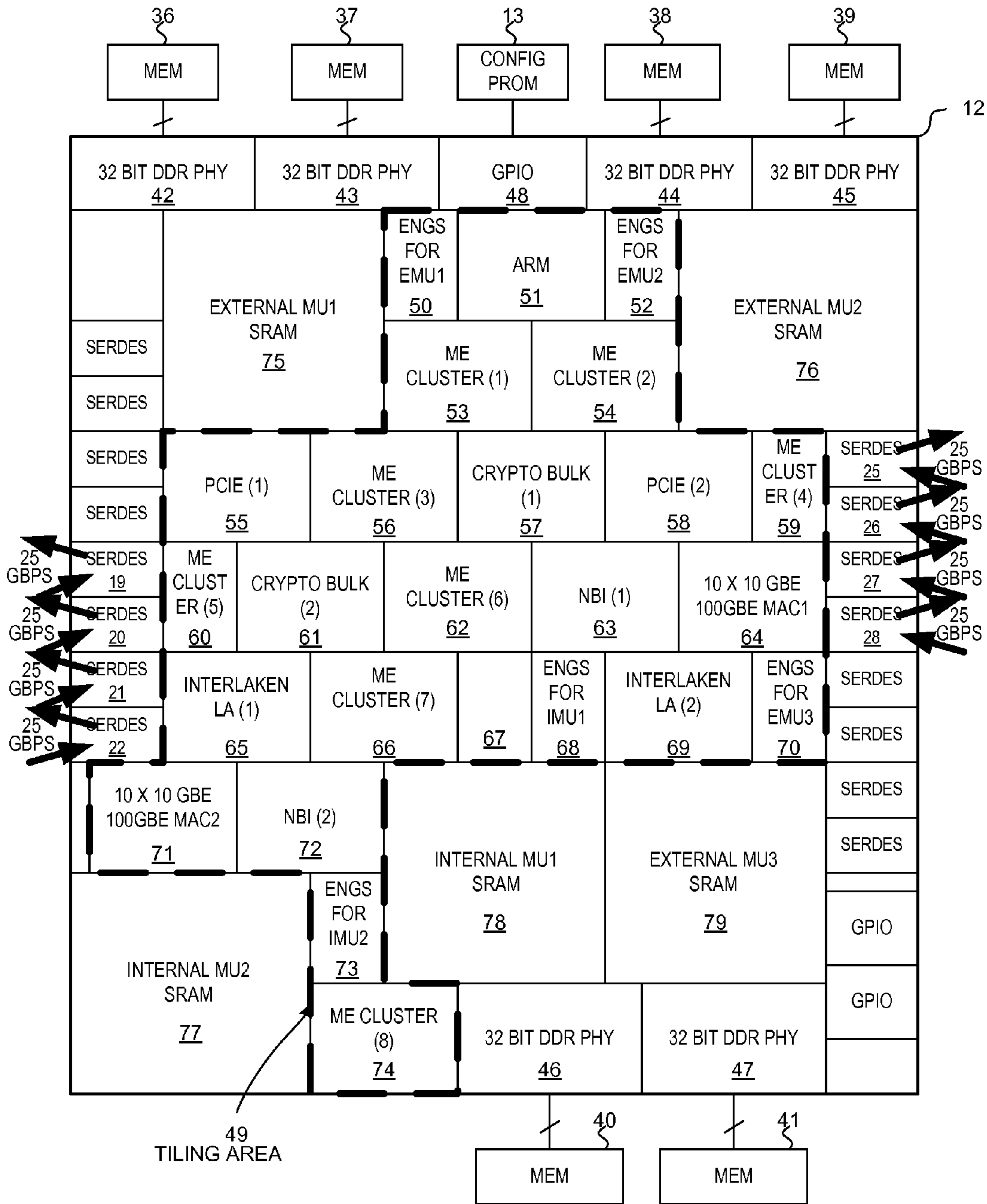
IBNFP INTEGRATED CIRCUIT FIG. 2
