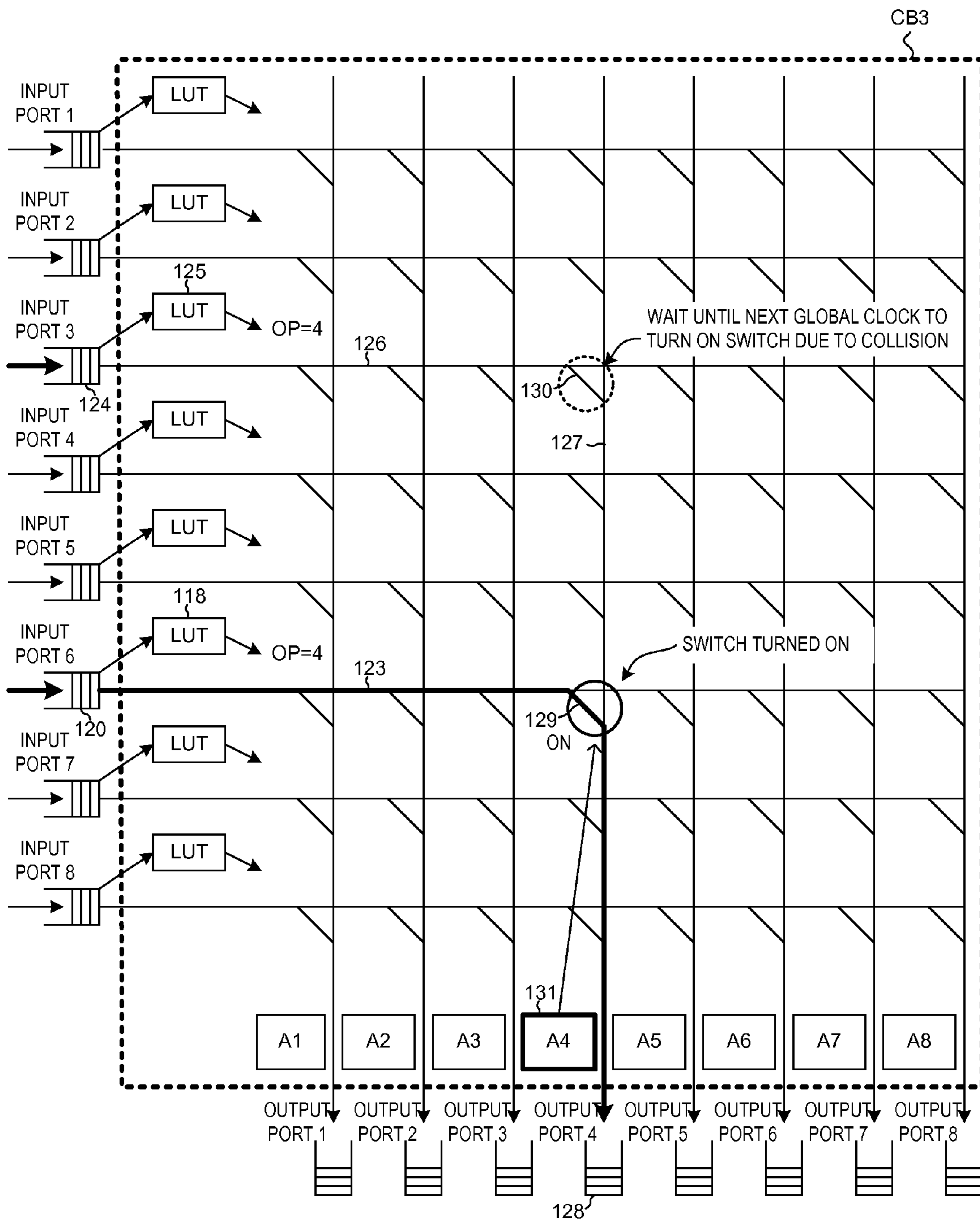
8-WAY CROSSBAR SWITCH
