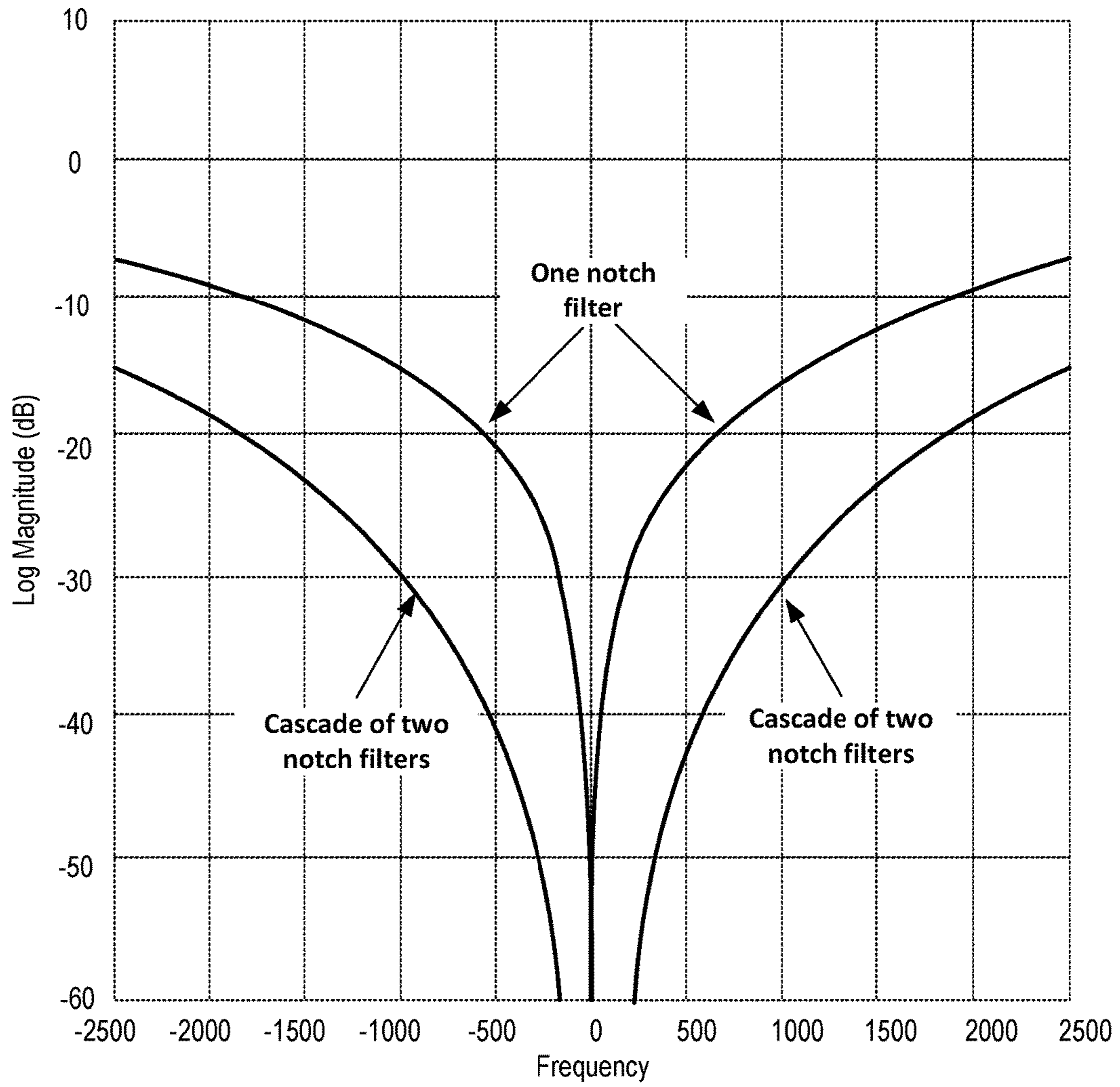
FIG. 6 (Response for One and Two Cascaded Notches)
