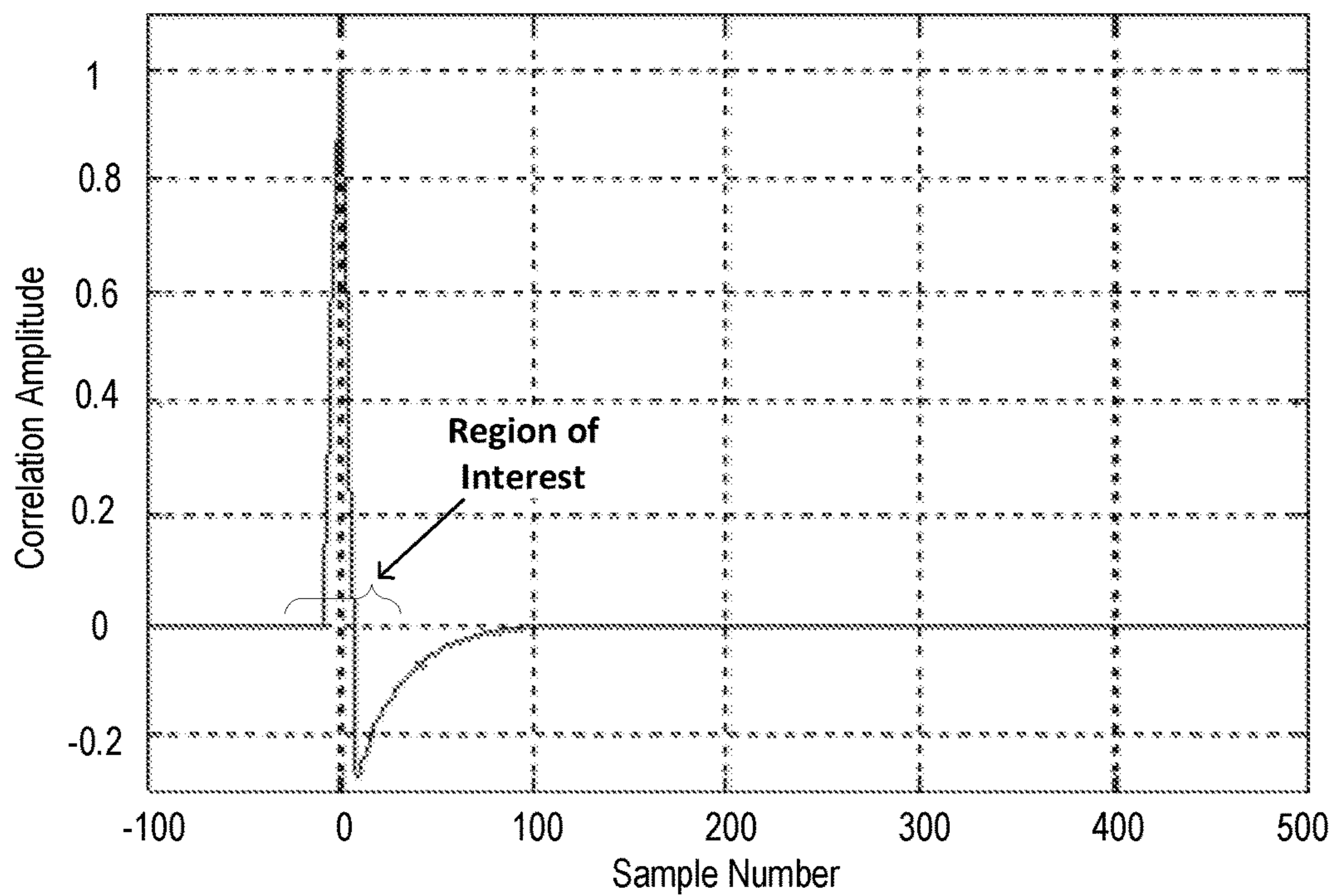
FIG. 4B (Correlation Amplitude, With Notch)
