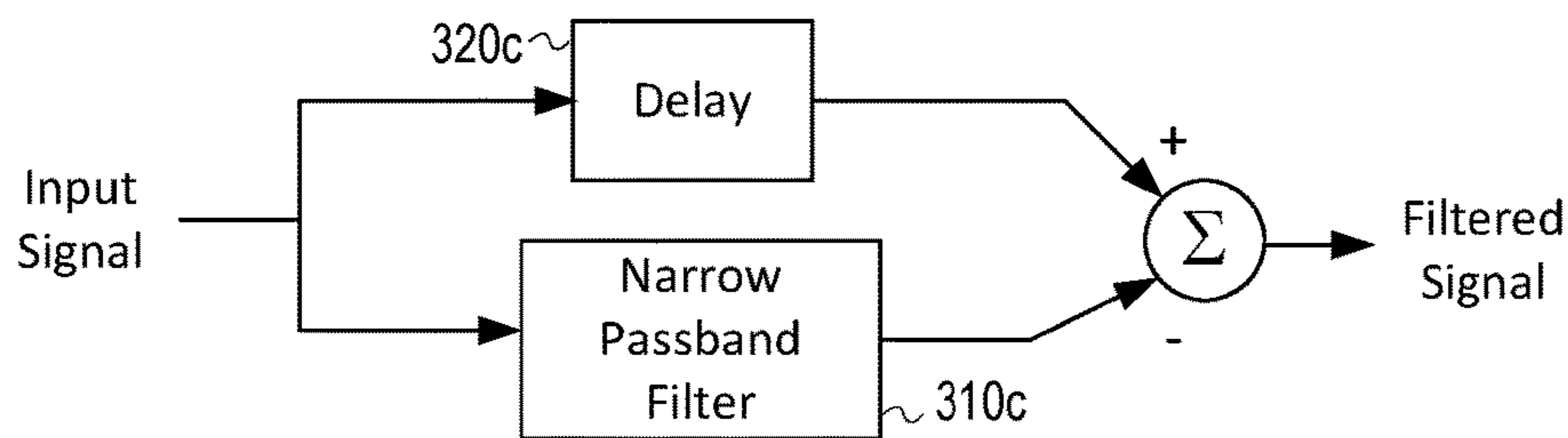
FIG. 3C (Modified Notch Filter With Advanced Passband Filter)
