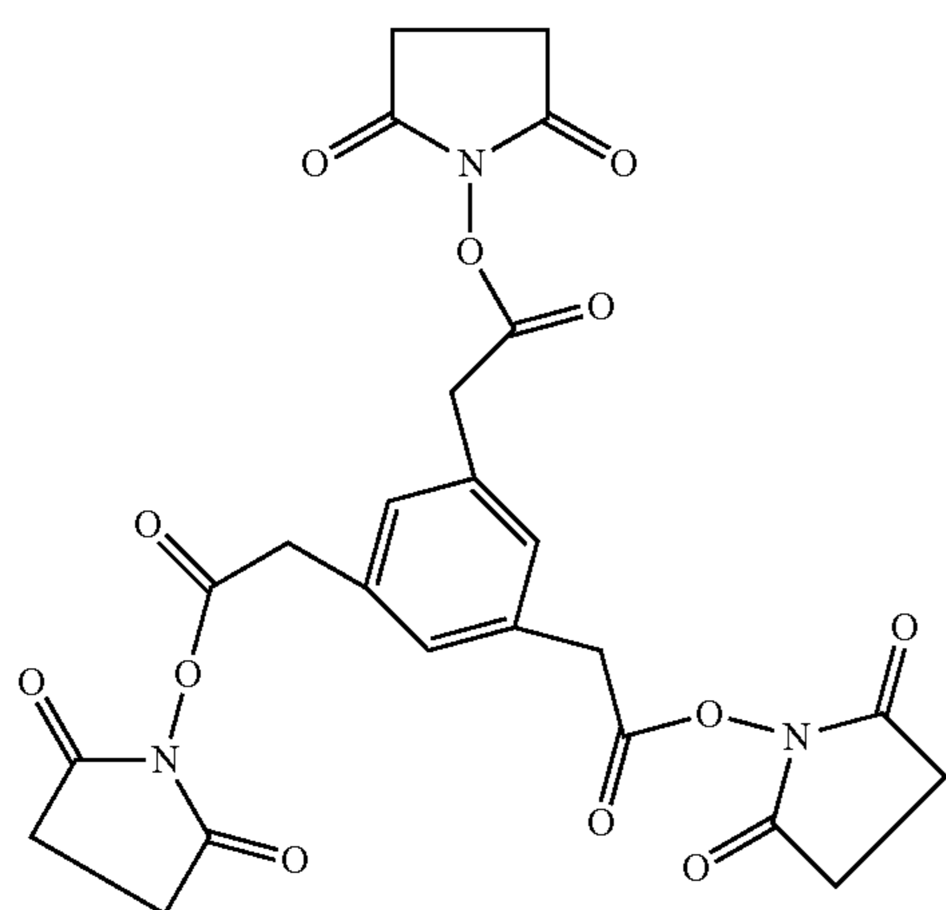
Active ester BTA (NHS) 2
