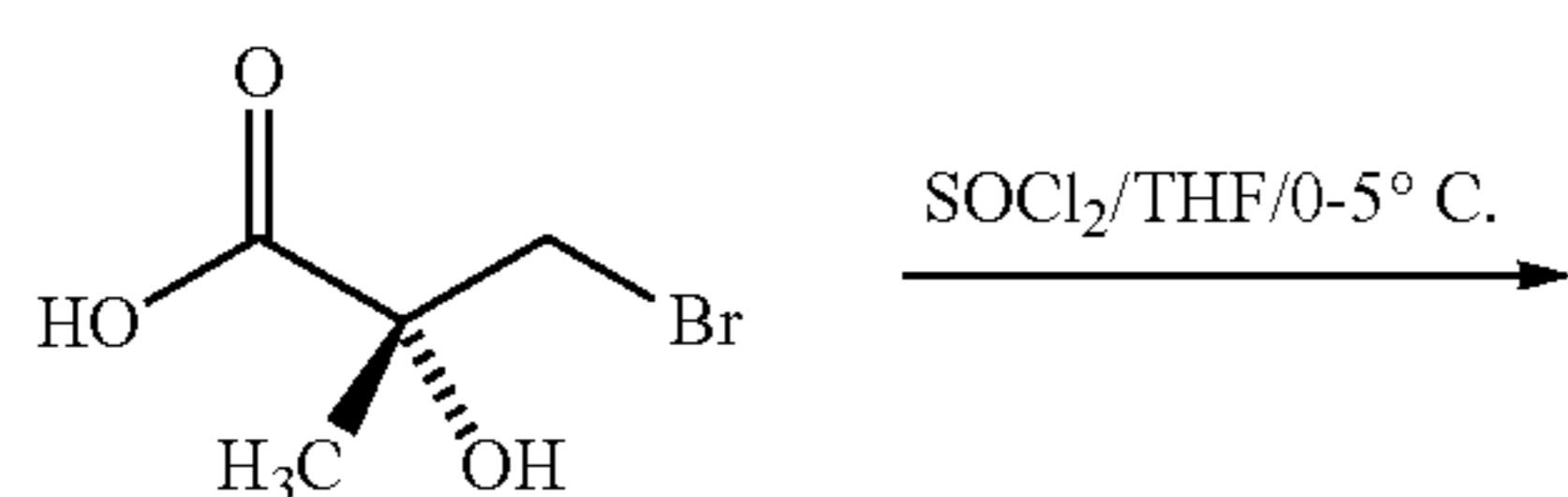
(R)-3-bromo-2-hydroxy-2-methylpropanoic acid R-18
