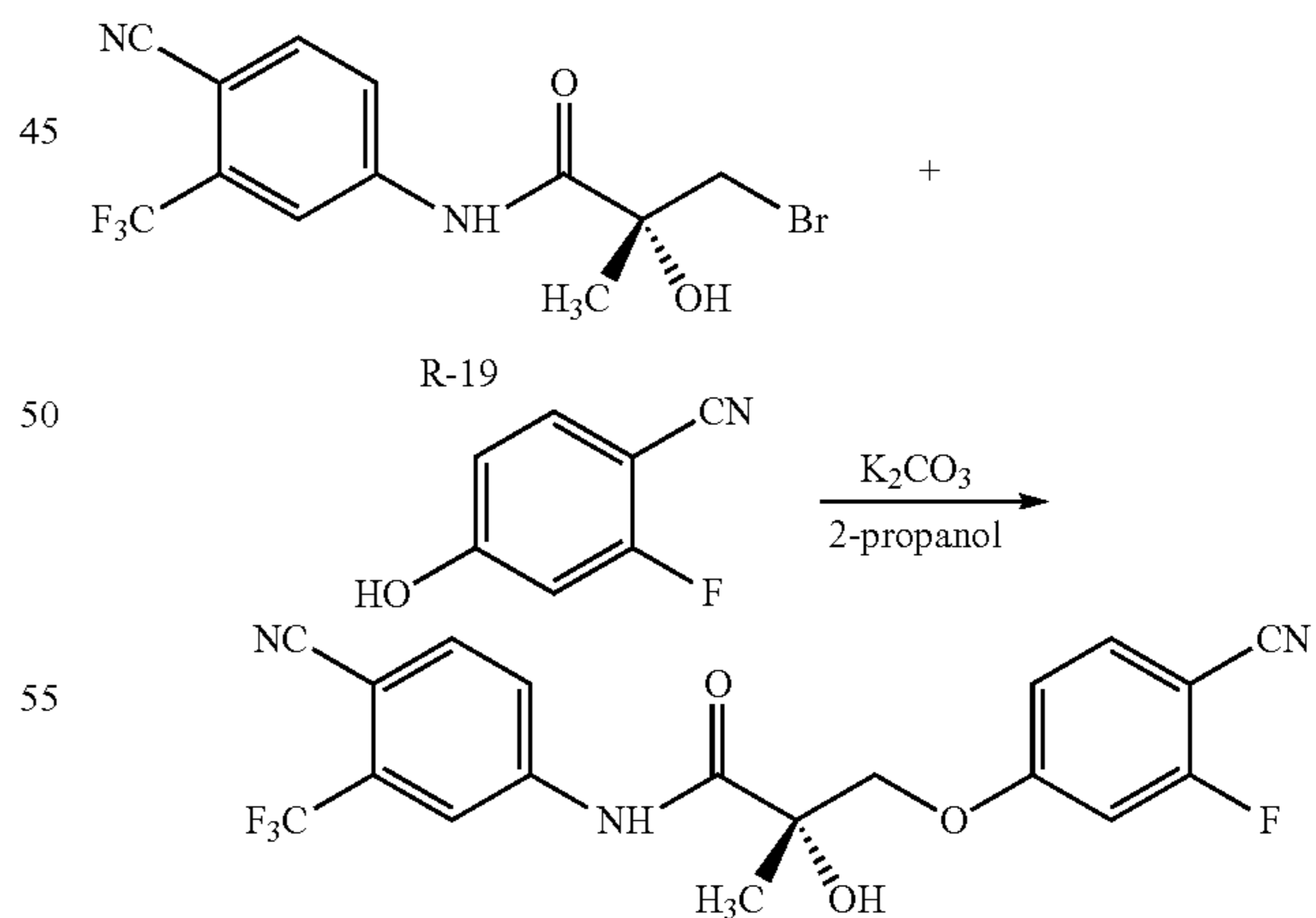
Synthesis of (S)—N-(4-cyano-3-(trifluoromethyl)phenyl)-3-(4-cyano-3-fluorophenoxy)-2-hydroxy-2-methylpropanamide (Formula XIII)
