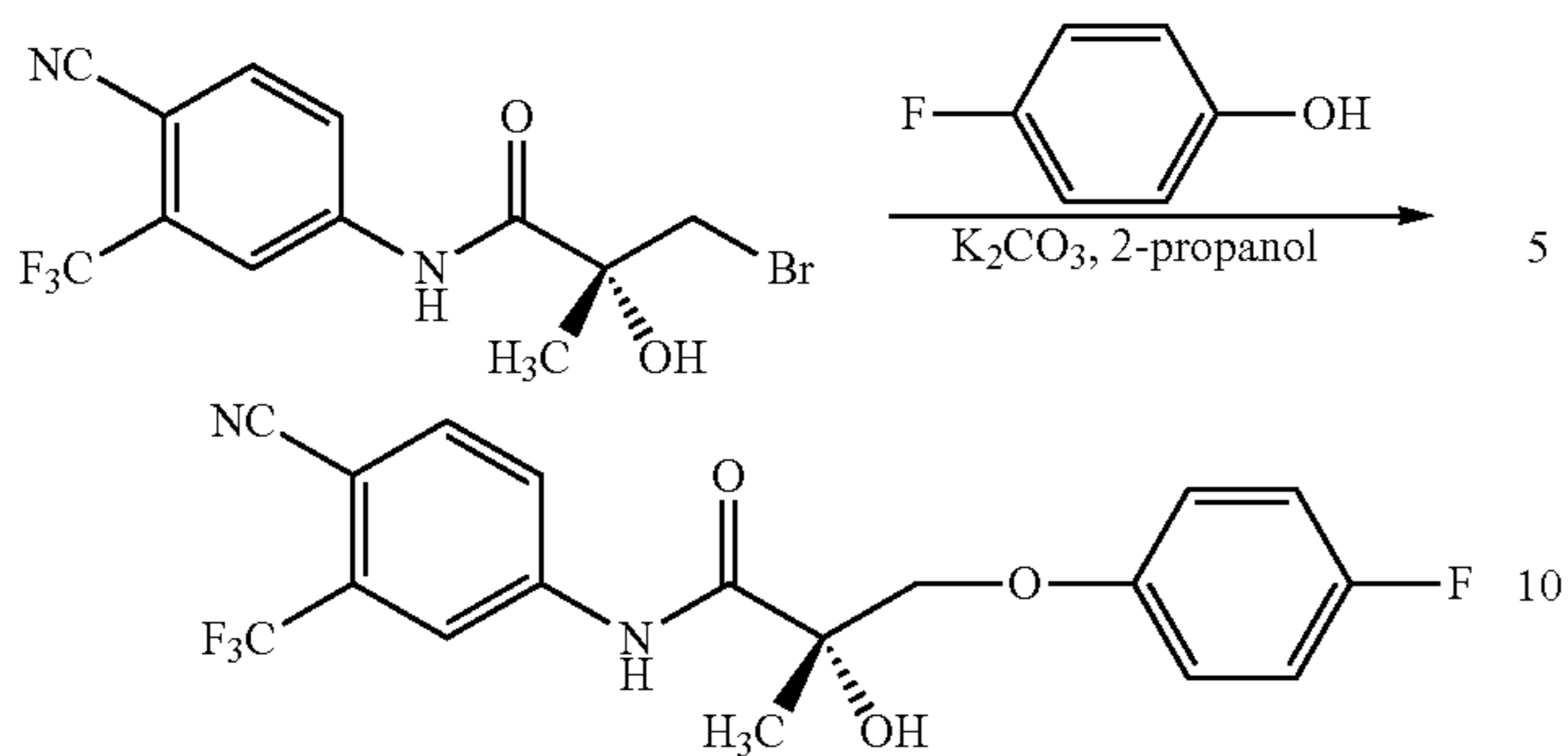
Synthesis of (S)—N-(4-cyano-3-(trifluoromethyl)phenyl)-3-(4-fluorophenoxy)-2-hydroxy-2-methylpropanamide (Formula X)
