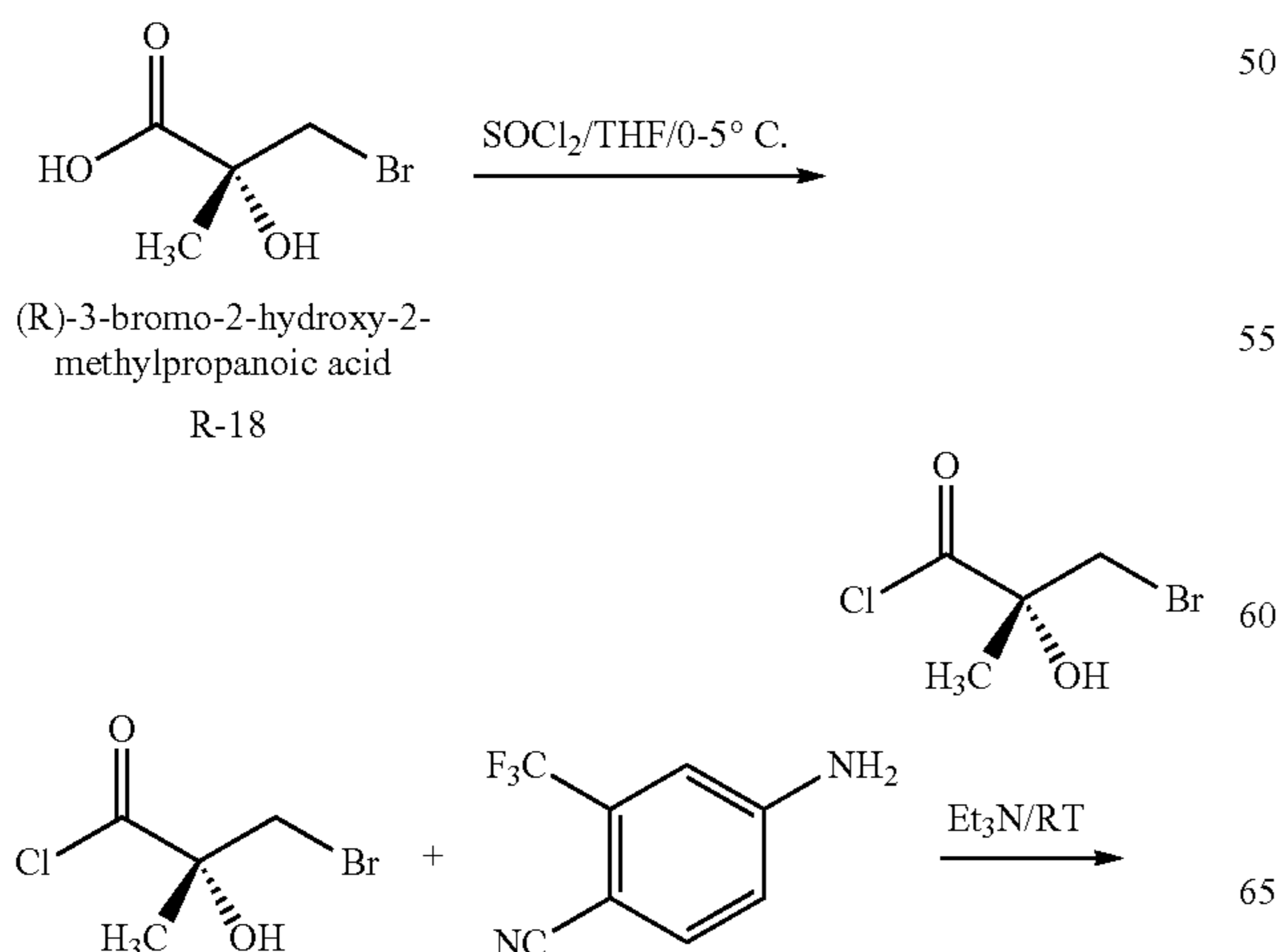
Synthesis of (S)—N-(4-cyano-3-(trifluoromethyl)phenyl)-3-(4-cyano-3-fluorophenoxy)-2-hydroxy-2-methylpropanamide (Formula XIII)
