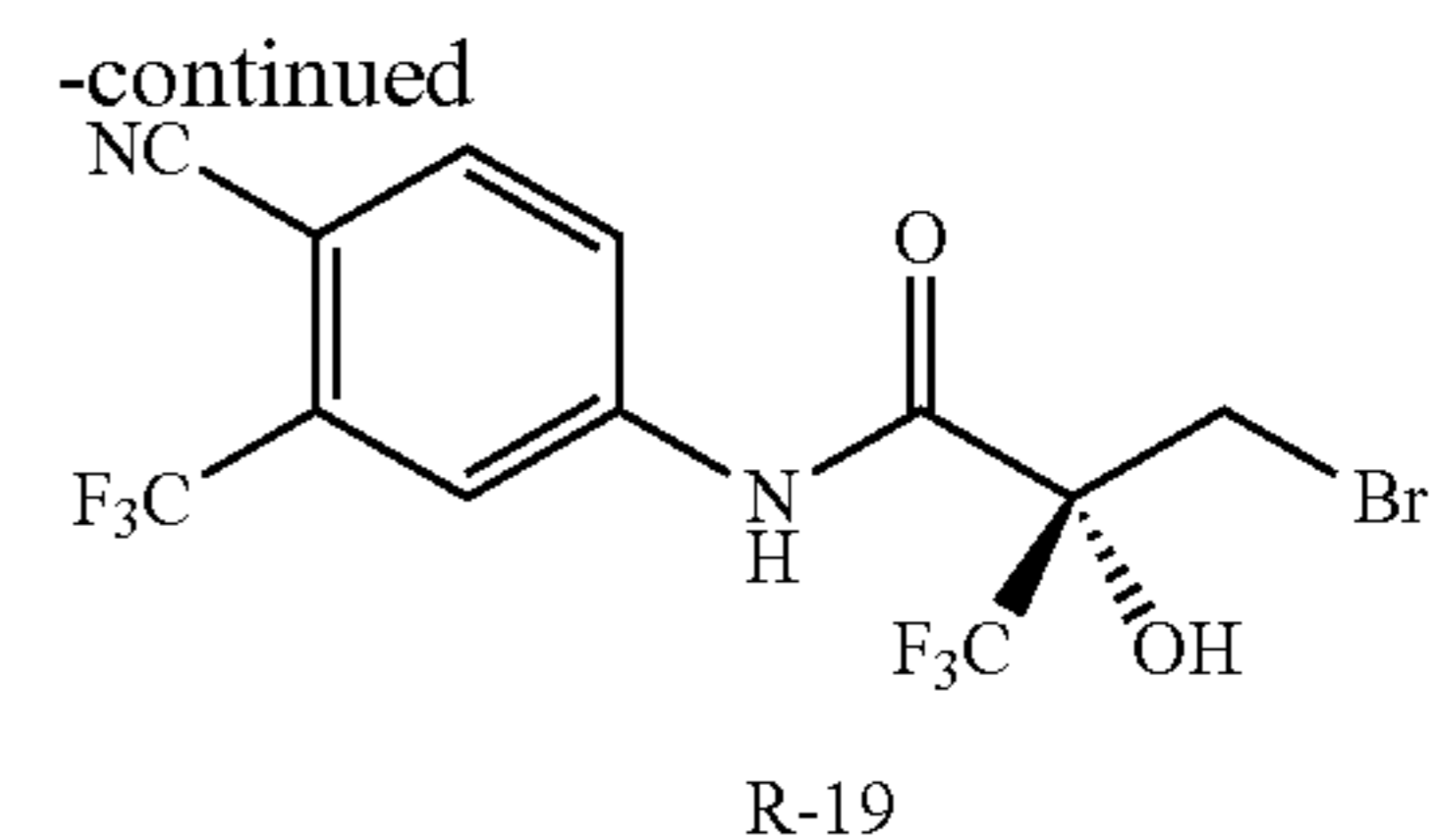
Synthesis of (2R)-3-bromo-N-[4-cyano-3-(trifluoromethyl)phenyl]-2-hydroxy-2-methylpropanamide
