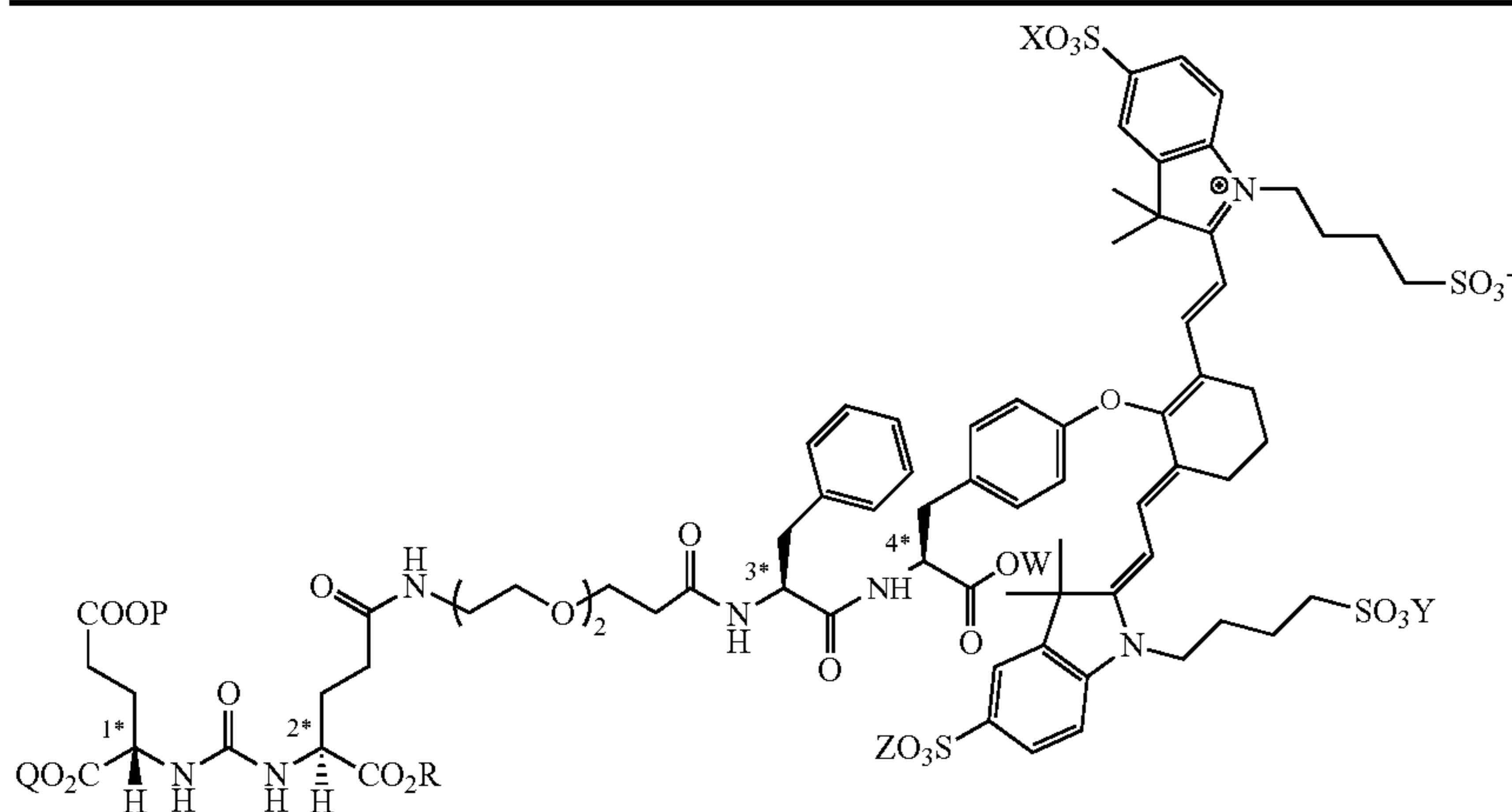
Chiral Center
