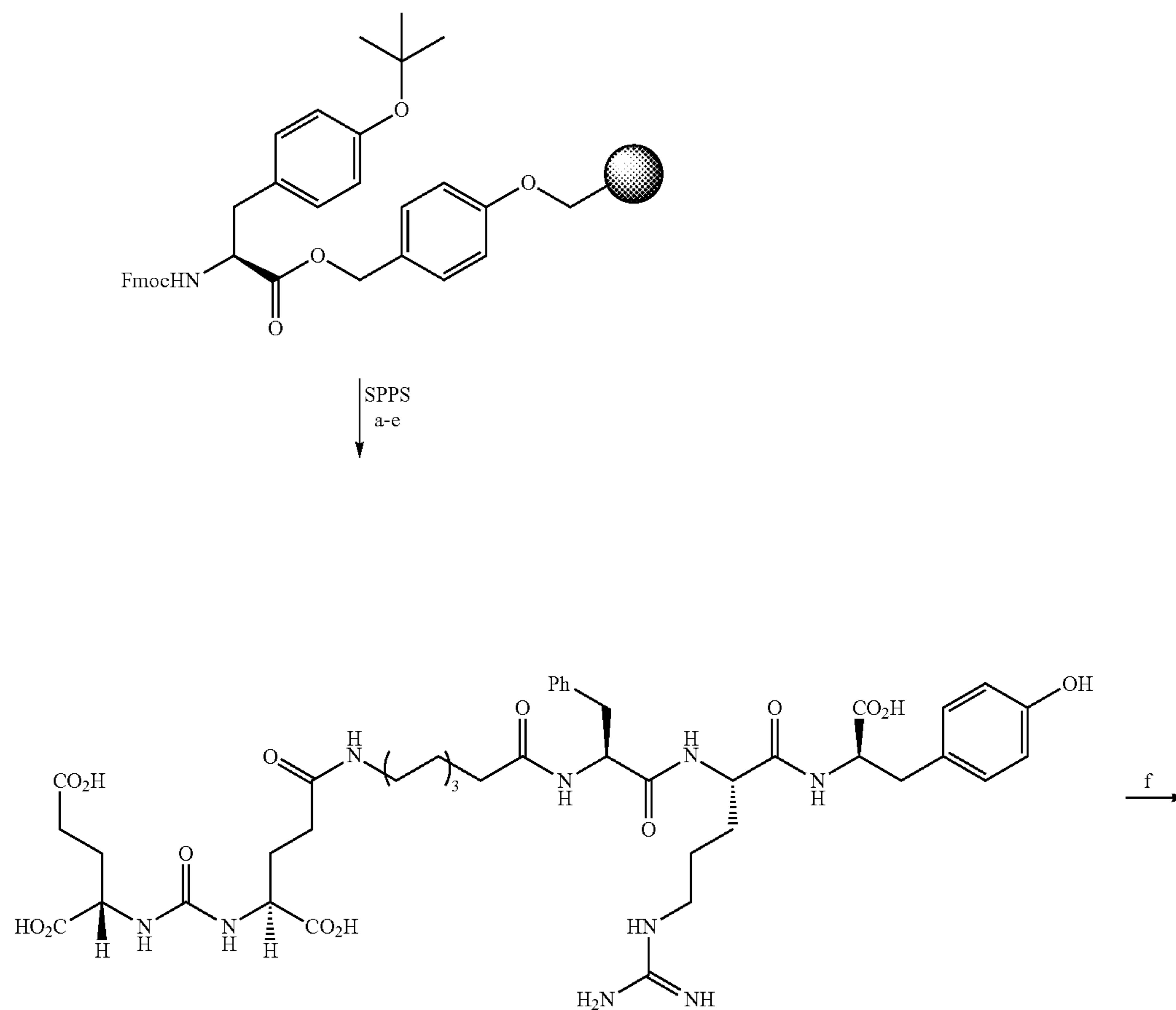
Scheme 4:
