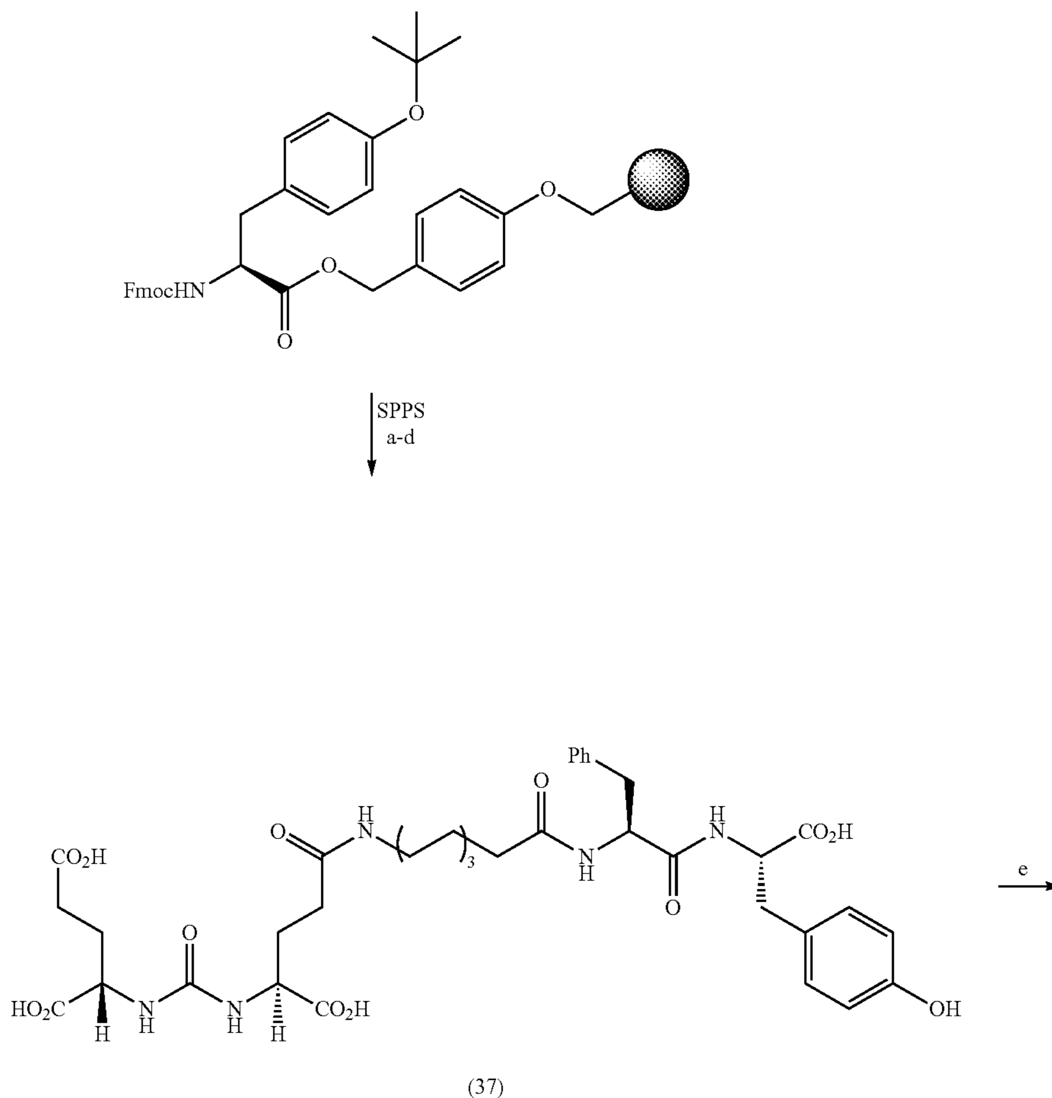
Scheme 3:
