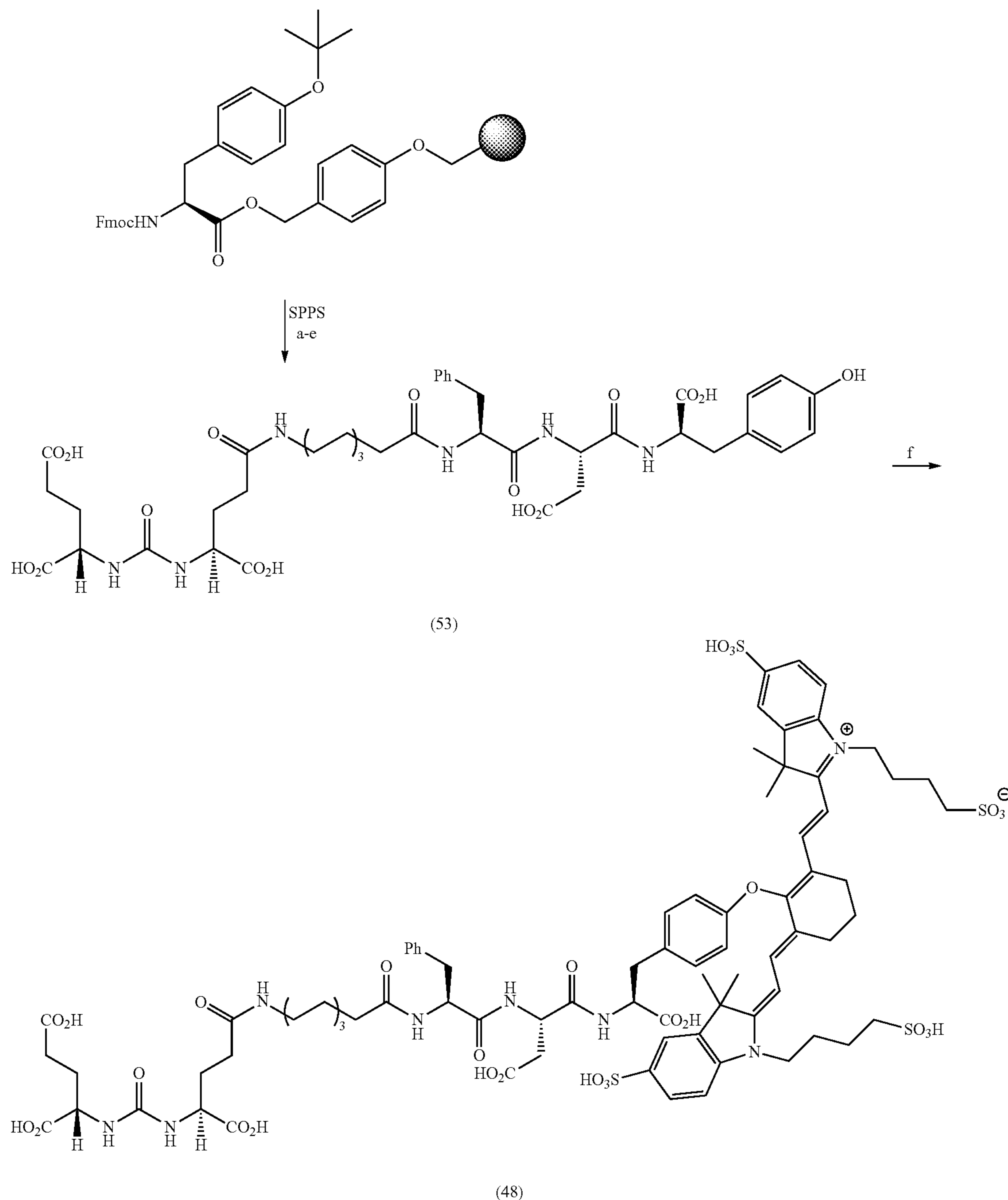
Scheme 5:
