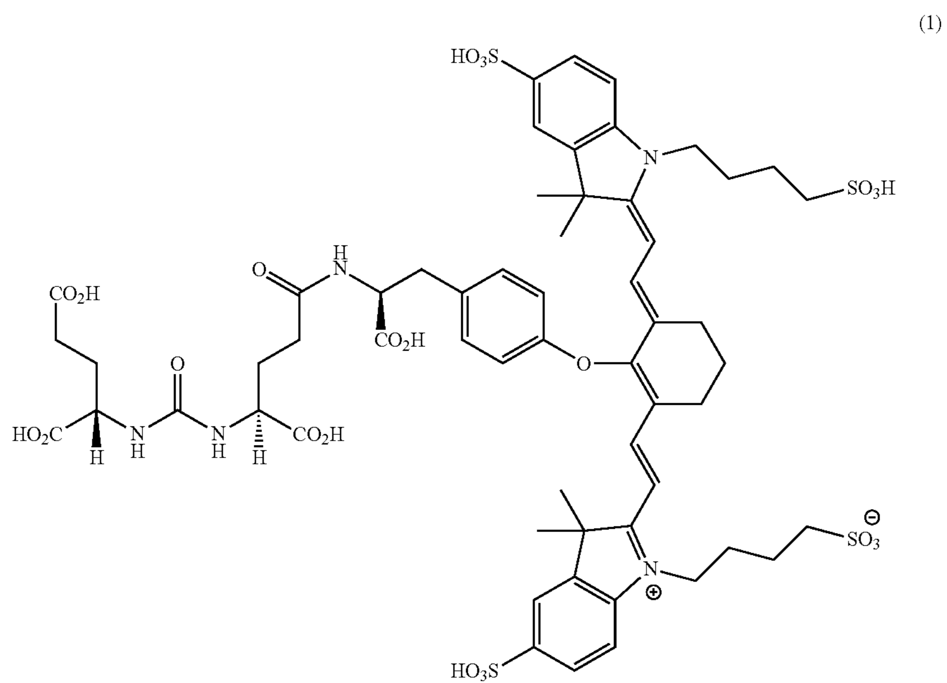
Scheme 1:
