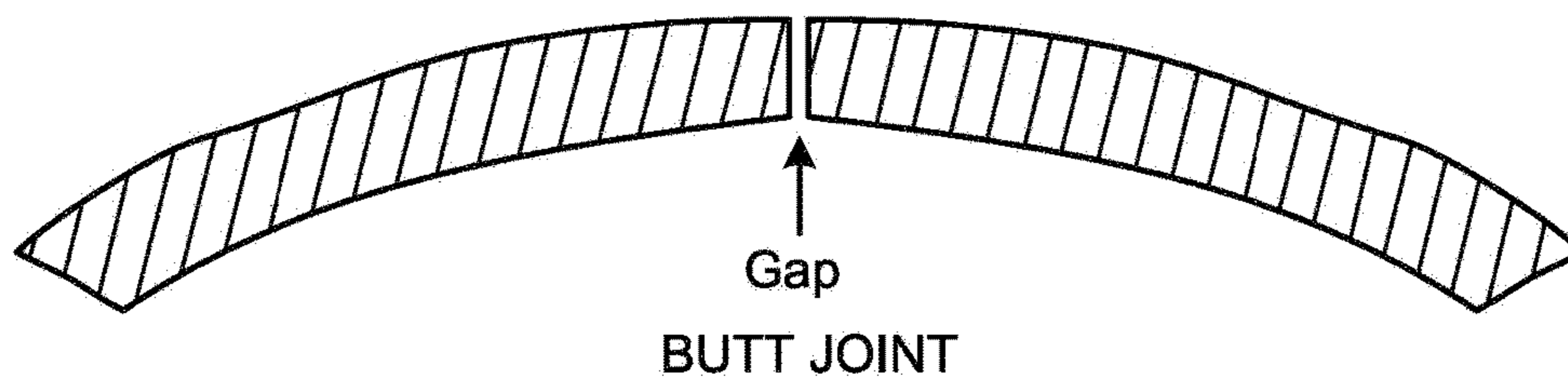
FIG. 1C (PRIOR ART)
