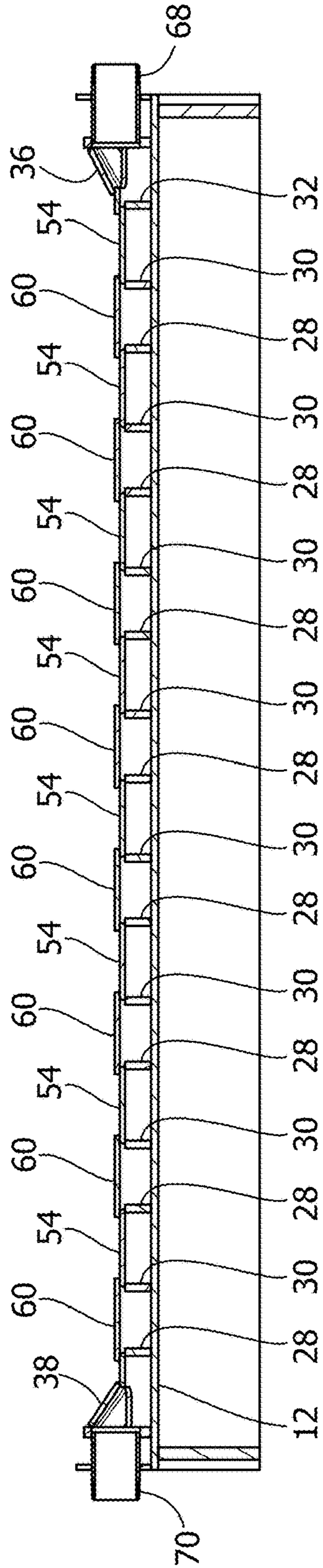
FIG. 7C (Rear View)
