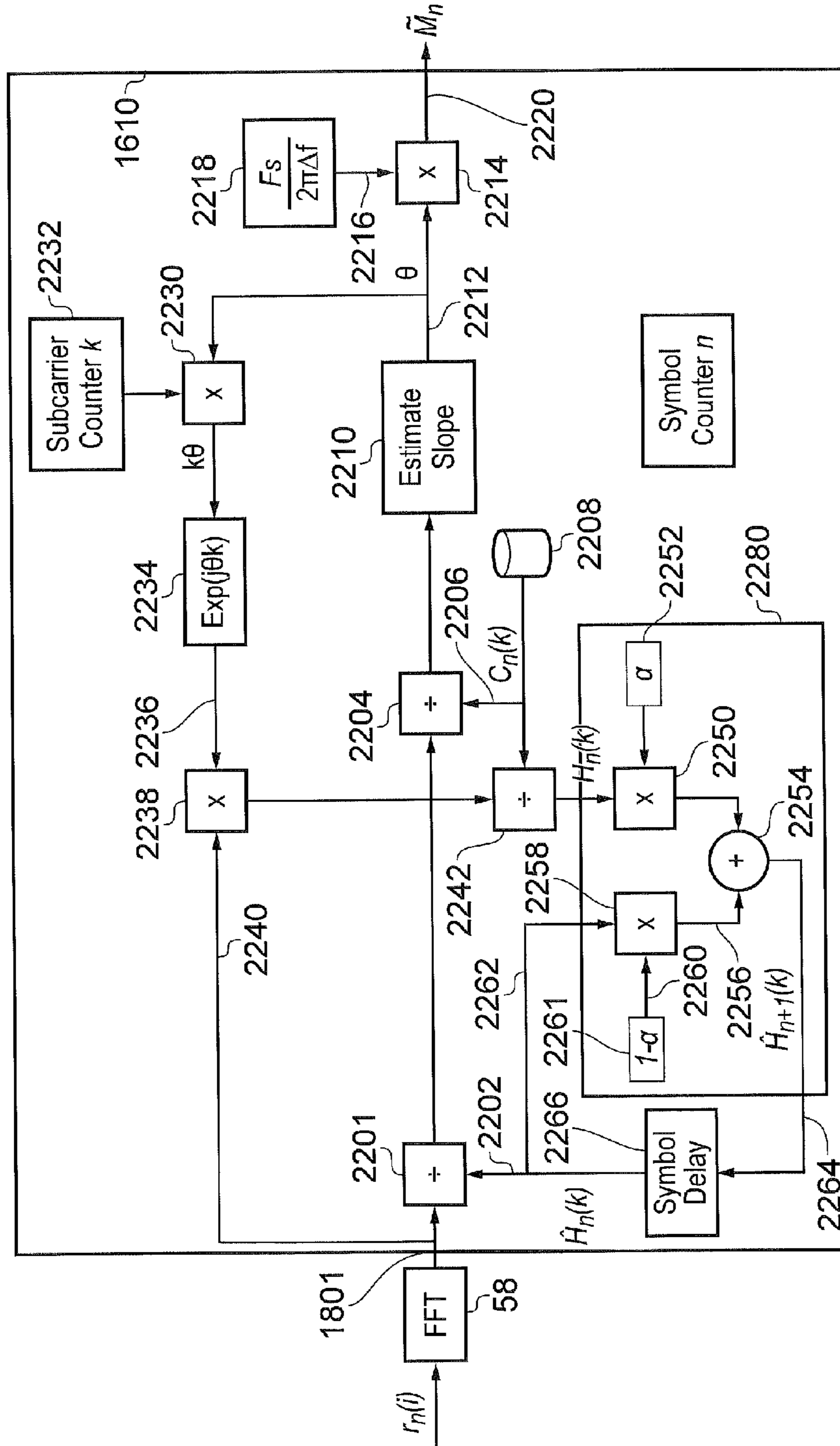
CTF Update Example Based on Frequency Domain Cyclic Shift Estimator
