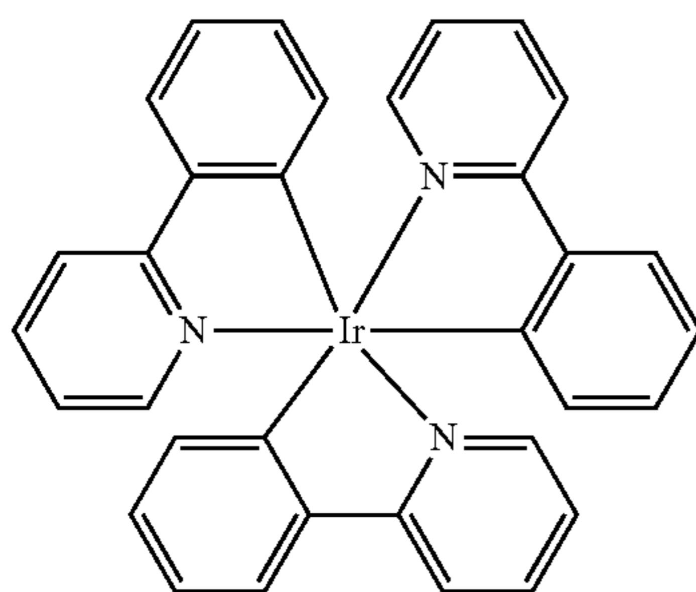
\text{Ir}(\text{ppy})_3
