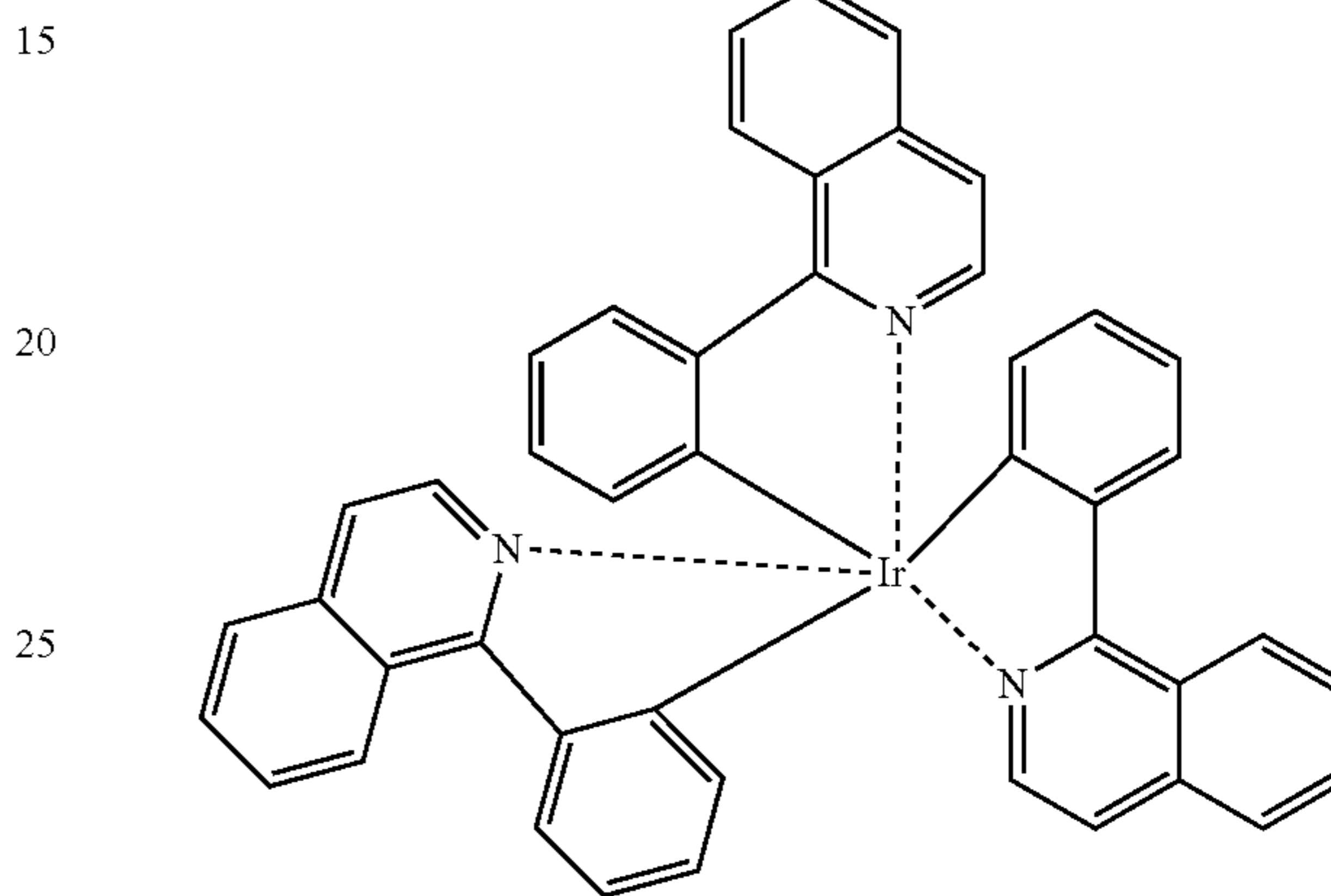
\text{Btp}_2\text{Ir}(\text{acac})
