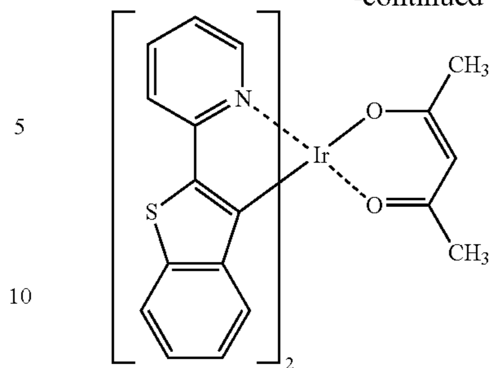
\text{Btp}_2\text{Ir}(\text{acac})
