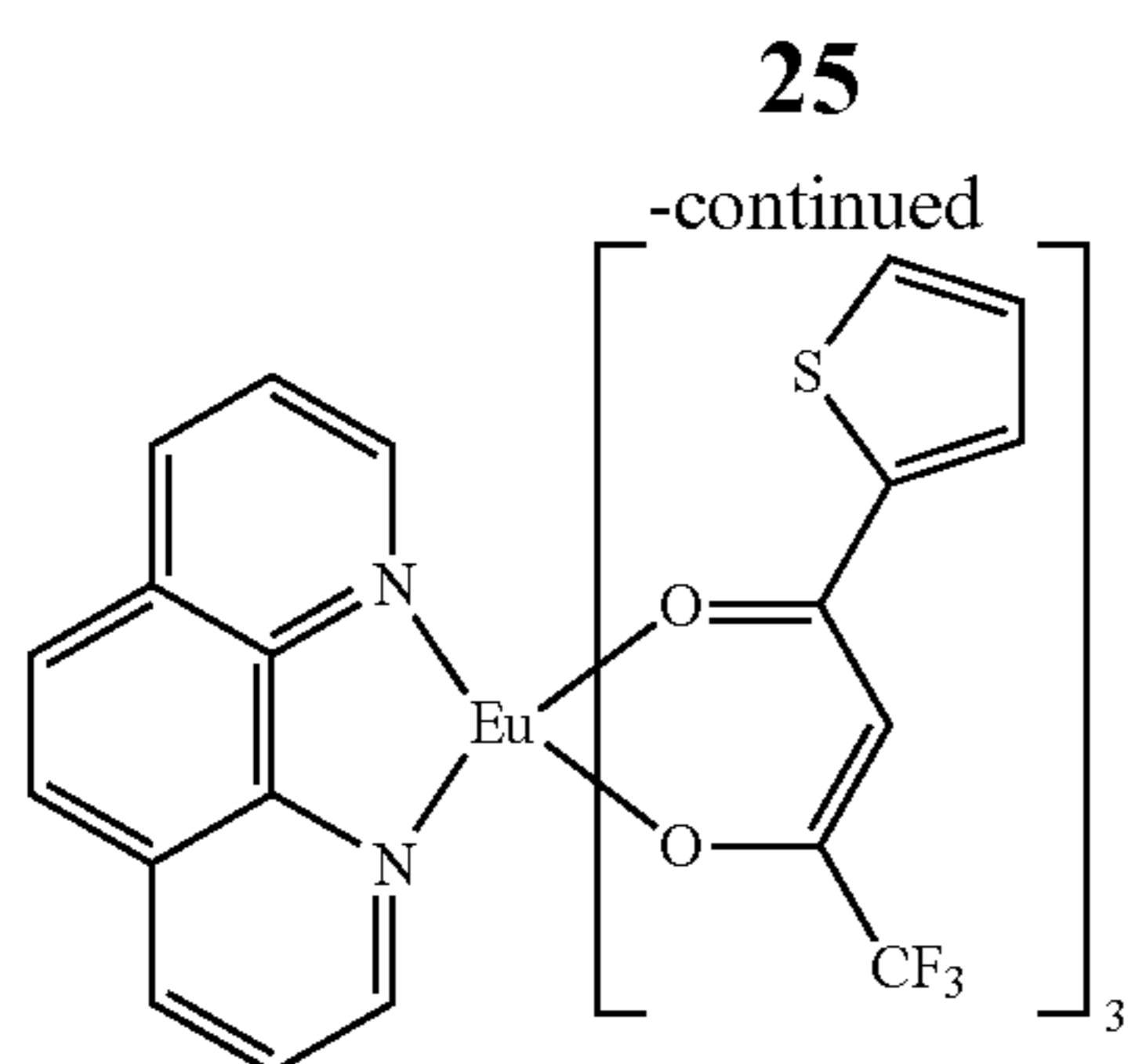
Eu(TTA) 3 phen
