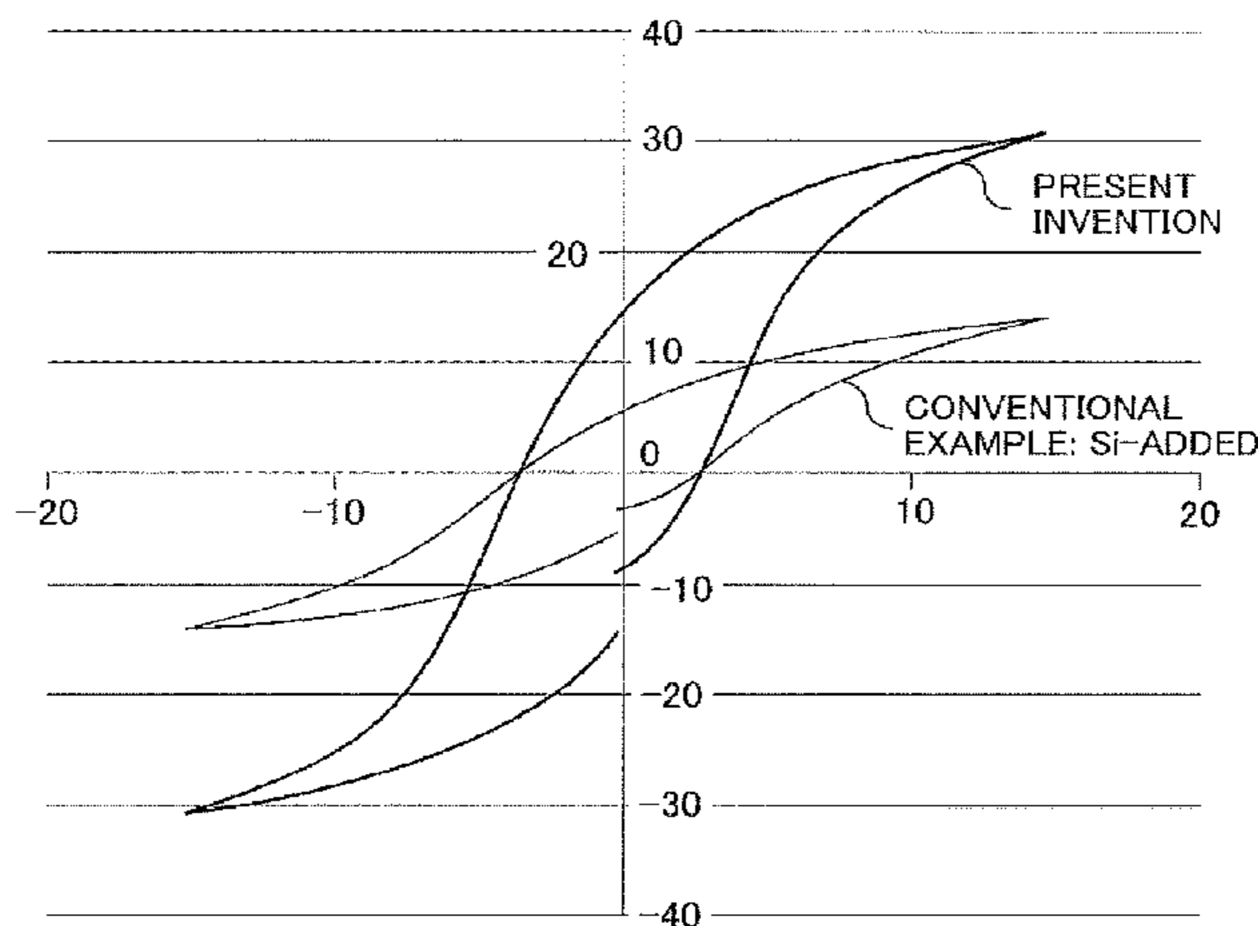
COMPARISON OF HYSTERESIS BEHAVIOR BETWEEN PRESENT INVENTION AND Si-ADDED PZT
